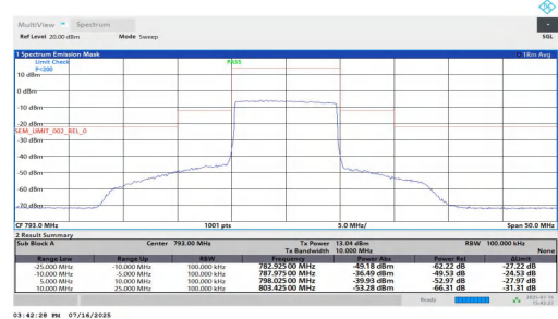
NTNT-n14-PC3-15-10-L-CP-256QAM-Outer_Full-10.00-25.00-PA SS
