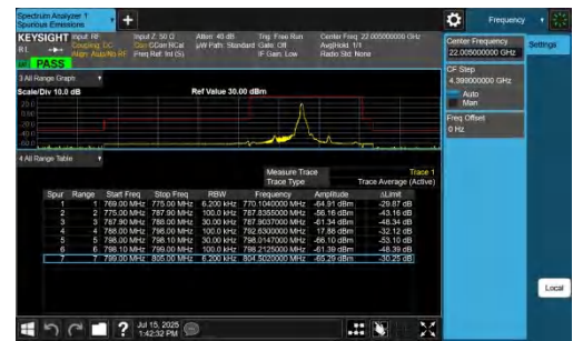
NTNV-n14-PC3-15-5-L-DFT-BPSK-Edge_1RB_Right-PASS
