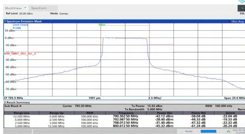
NTNT-n14-PC3-15-5-H-CP-64QAM-Outer_Full--12.50--5.00-PASS
