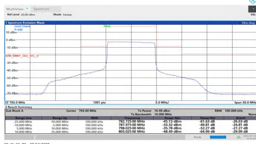
NTNT-n14-PC3-15-10-L-CP-16QAM-Outer Full-5.00-10.00-PASS
