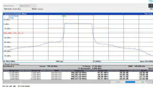
NTNT-n14-PC3-15-5-H-DFT-16QAM-Outer Full--12.50--5.00-PAS
