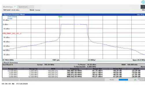
NTNT-n14-PC3-15-5-H-CP-QPSK-Outer_Full-2.50-5.00-PASS
