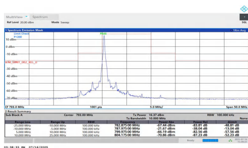
NTNT-n14-PC3-15-10-L-DFT-16QAM-Edge_1RB_Left-5.00-10.00- PASS
