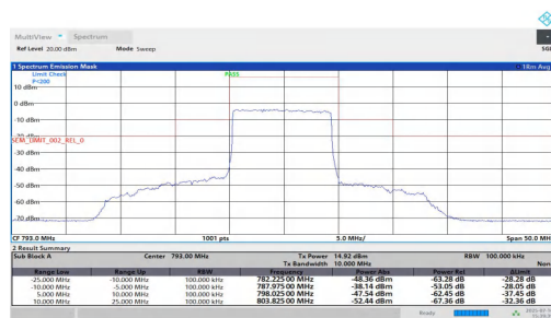
NTNT-n14-PC3-15-10-L-DFT-256QAM-Outer Full-10.00-25.00-P
