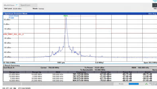
NTNT-n14-PC3-15-10-L-DFT-BPSK-Edge_1RB_Left-25.00--10.0 0-PASS
