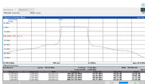
NTNT-n14-PC3-15-5-H-DFT-16QAM-Outer Full-2.50-5.00-PASS
