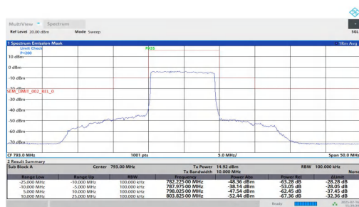
NTNT-n14-PC3-15-10-L-DFT-256QAM-Outer Full-5.00-10.00-PAS
