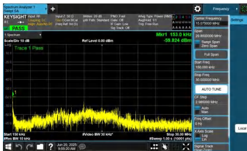
NTNV-n14-PC3-15-5-M-DFT-QPSK-Inner_1RB_Right-0.15-30-P ASS
