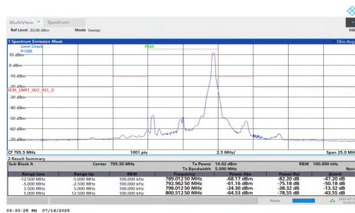
NTNT-n14-PC3-15-5-H-DFT-256QAM-Edge_1RB_Right-5.00-12. 50-PASS
