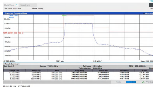
NTNT-n14-PC3-15-5-H-DFT-64QAM-Outer_Full--5.00--2.50-PAS
