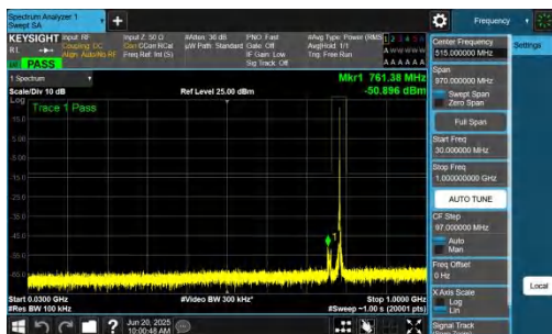
NTNV-n14-PC3-15-10-L-DFT-QPSK-Inner_1RB_Left-30-1000-PA SS
