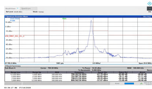
NTNT-n14-PC3-15-5-H-CP-QPSK-Edge_1RB_Right--5.00--2.50- PASS
