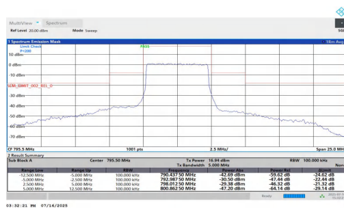
NTNT-n14-PC3-15-5-H-DFT-64QAM-Outer Full-5.00-12.50-PAS
