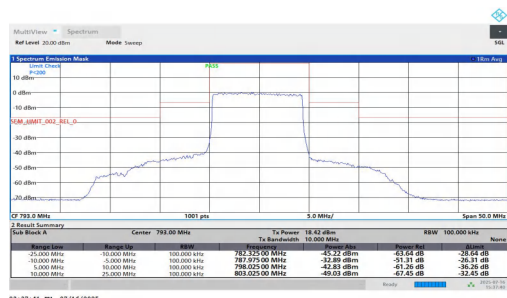
NTNT-n14-PC3-15-10-L-DFT-QPSK-Outer_Full-10.00-25.00-PAS
