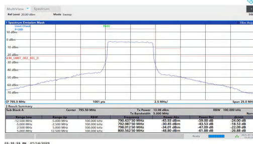
NTNT-n14-PC3-15-5-H-CP-256QAM-Outer Full-5.00-12.50-PAS
