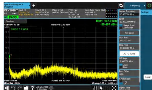
NTNV-n14-PC3-15-5-M-DFT-BPSK-Inner_1RB_Left-0.15-30-PASS
