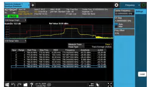
NTNV-n14-PC3-15-5-L-DFT-QPSK-Outer_Full-PASS
