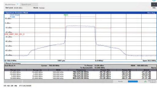
NTNT-n14-PC3-15-10-L-CP-256QAM-Outer_Full--10.00--5.00-PA SS
