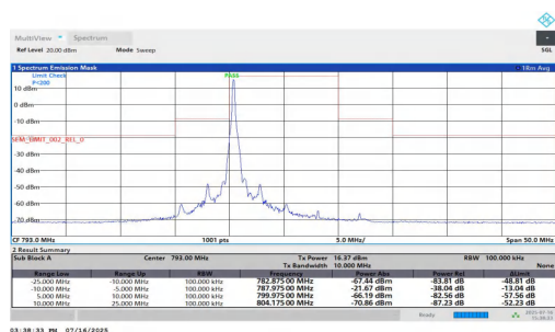
NTNT-n14-PC3-15-10-L-DFT-16QAM-Edge_1RB_Left-10.00-25. 00-PASS
