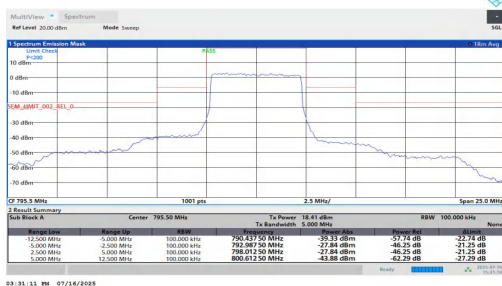
NTNT-n14-PC3-15-5-H-DFT-QPSK-Outer Full--12.50--5.00-PASS
