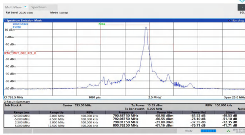
NTNT-n14-PC3-15-5-H-CP-64QAM-Edge_1RB_Right-2.50-5.00-P ASS
