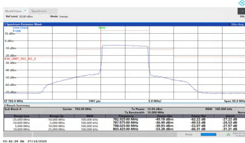
NTNT-n14-PC3-15-10-L-CP-256QAM-Outer_Full-5.00-10.00-PAS S
