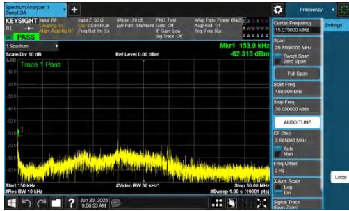
NTNV-n14-PC3-15-5-H-DFT-BPSK-Inner_1RB_Right-0.15-30-PA SS
