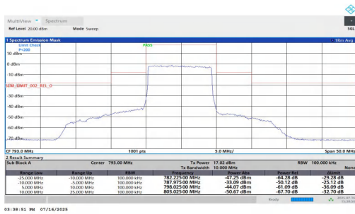
NTNT-n14-PC3-15-10-L-DFT-64QAM-Outer_Full-5.00-10.00-PAS S
