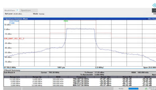
NTNT-n14-PC3-15-5-H-DFT-16QAM-Outer Full-5.00-12.50-PAS
