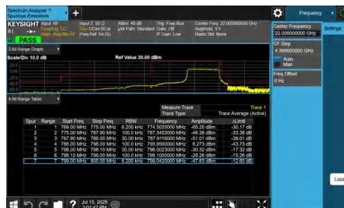
NTNV-n14-PC3-15-5-H-DFT-QPSK-Outer Full-PASS
