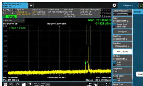
NTNV-n14-PC3-15-5-M-DFT-QPSK-Inner_1RB_Left-30-1000-PA SS
