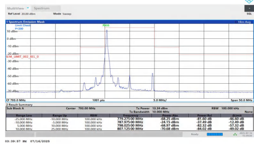
NTNT-n14-PC3-15-10-L-DFT-256QAM-Edge_1RB_Left-10.00-25.00-0-PASS
