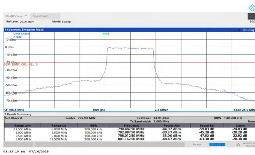
NTNT-n14-PC3-15-5-H-DFT-256QAM-Outer_Full-2.50-5.00-PASS
