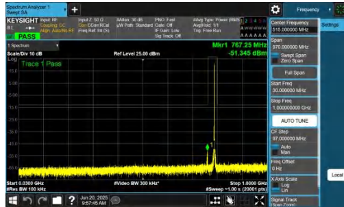
NTNV-n14-PC3-15-5-H-DFT-QPSK-Inner_1RB_Left-30-1000-PA SS
