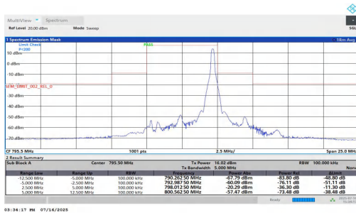
NTNT-n14-PC3-15-5-H-CP-QPSK-Edge_1RB_Right--12.50--5.00- PASS
