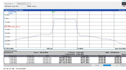
NTNT-n14-PC3-15-5-H-DFT-256QAM-Outer_Full--5.00--2.50-PA SS
