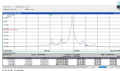
NTNT-n14-PC3-15-5-H-DFT-256QAM-Edge_1RB_Right--5.00--2. 50-PASS
