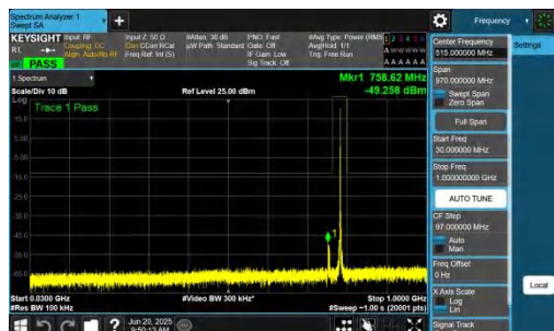
NTNV-n14-PC3-15-5-L-DFT-BPSK-Inner_1RB_Left-30-1000-PAS
