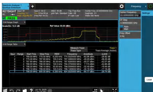
NTNV-n14-PC3-15-5-H-DFT-BPSK-Outer Full-PASS
