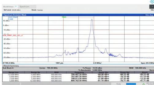
NTNT-n14-PC3-15-5-H-CP-64QAM-Edge_1RB_Right--12.50--5.0 0-PASS
