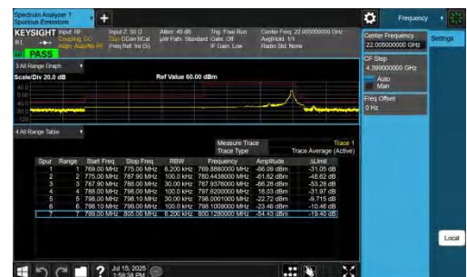
NTNV-n14-PC3-15-5-H-DFT-BPSK-Edge_1RB_Right-PASS
