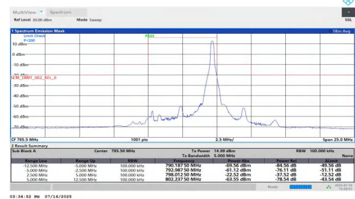
NTNT-n14-PC3-15-5-H-CP-16QAM-Edge_1RB_Right-5.00-12.50-PASS
