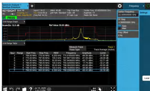
NTNV-n14-PC3-15-5-H-DFT-BPSK-Edge_1RB_Left-PASS
