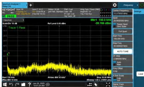
NTVN-n14-PC3-15-10-L-DFT-QPSK-Inner_1RB_Right-0.15-30-P ASS
