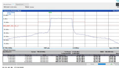
NTNT-n14-PC3-15-5-H-DFT-16QAM-Outer Full--5.00--2.50-PAS
