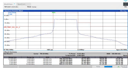
NTNT-n14-PC3-15-5-H-CP-64QAM-Outer_Full--5.00--2.50-PASS
