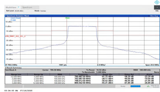
NTNT-n14-PC3-15-5-H-CP-QPSK-Outer_Full-5.00-12.50-PASS
