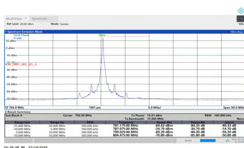
NTNT-n14-PC3-15-10-L-DFT-64QAM-Edge_1RB_Left-5.00-10.00- PASS
