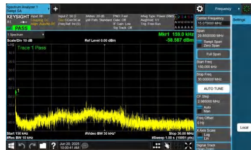
NTNV-n14-PC3-15-10-L-DFT-QPSK-Inner_1RB_Left-0.15-30-PAS S
