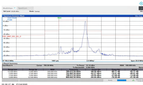
NTNT-n14-PC3-15-5-H-CP-256QAM-Edge_1RB_Right--12.50--5.00-PASS
