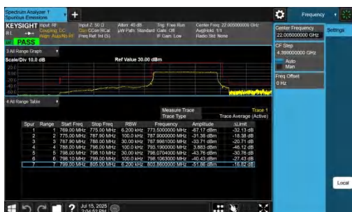
NTNV-n14-PC3-15-10-L-DFT-BPSK-Outer Full-PASS
