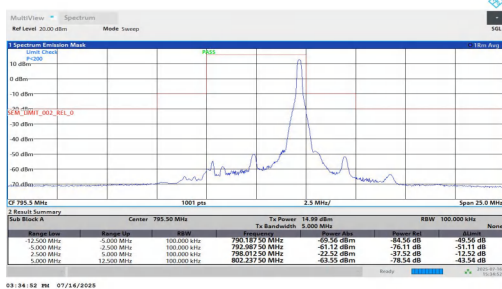
NTNT-n14-PC3-15-5-H-CP-16QAM-Edge_1RB_Right-2.50-5.00-PASS
