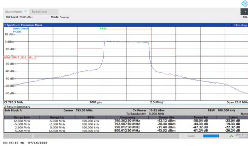
NTNT-n14-PC3-15-5-H-CP-64QAM-Outer_Full-2.50-5.00-PASS
