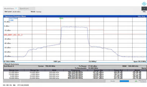
NTNT-n14-PC3-15-10-L-DFT-64QAM-Outer_Full-10.00-25.00-PA SS
