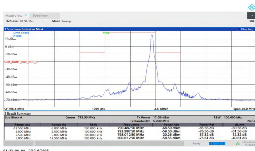
NTNT-n14-PC3-15-5-H-DFT-16QAM-Edge_1RB_Right--12.50--5.0 0-PASS
