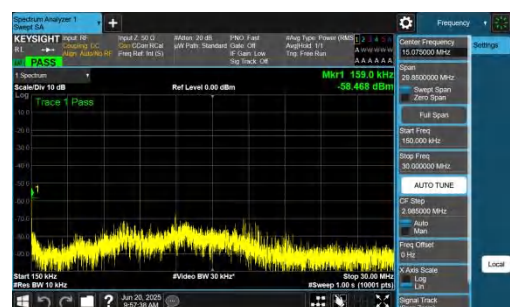
NTNV-n14-PC3-15-5-H-DFT-QPSK-Inner_1RB_Left-0.15-30-PAS S
