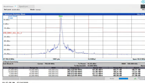
NTNT-n14-PC3-15-10-L-DFT-QPSK-Edge_1RB_Left-5.00-10.00-P ASS
