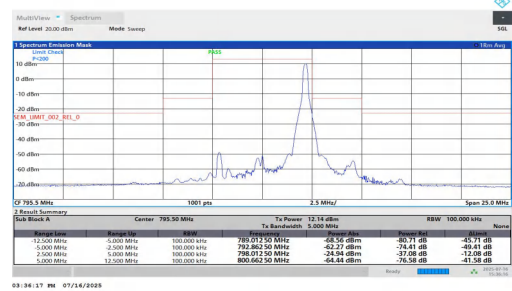
NTNT-n14-PC3-15-5-H-CP-256QAM-Edge_1RB_Right-5.00-12.50-PASS
