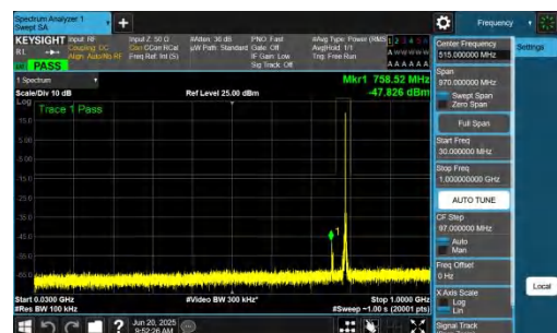
NTNV-n14-PC3-15-5-L-DFT-QPSK-Inner_1RB_Right-30-1000-PA SS
