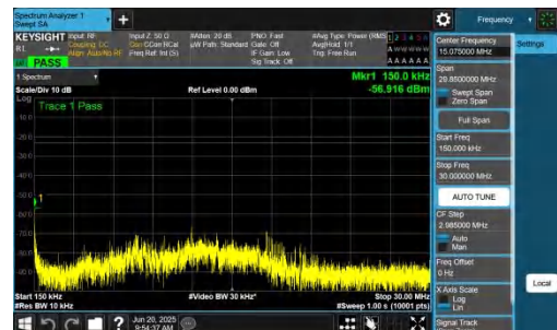
NTNV-n14-PC3-15-5-M-DFT-QPSK-Inner_1RB_Left-0.15-30-PAS S
