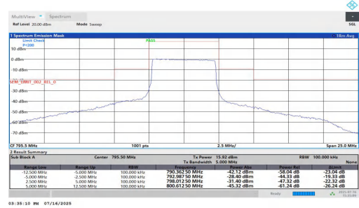
NTNT-n14-PC3-15-5-H-CP-64QAM-Outer_Full-5.00-12.50-PASS
