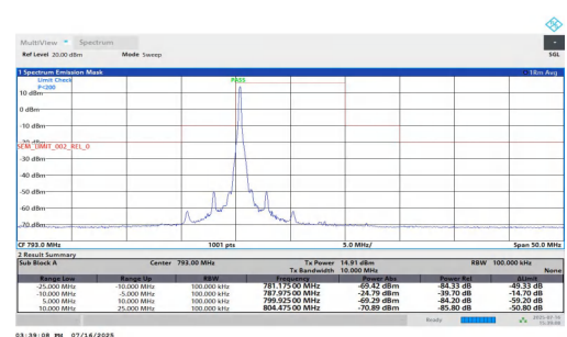
NTNT-n14-PC3-15-10-L-DFT-64QAM-Edge_1RB_Left-10.00-25. 00-PASS
