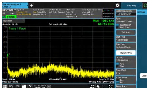
NTNV-n14-PC3-15-10-L-DFT-BPSK-Inner_1RB_Right-0.15-30-PASS
