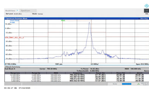
NTNT-n14-PC3-15-5-H-CP-QPSK-Edge_1RB_Right-5.00-12.50- PASS
