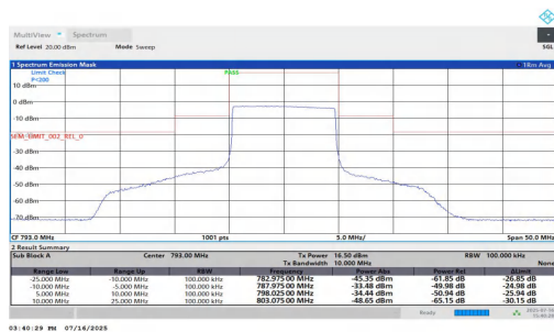
NTNT-n14-PC3-15-10-L-CP-QPSK-Outer Full-5.00-10.00-PASS
