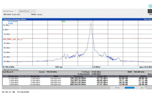
NTNT-n14-PC3-15-5-H-CP-QPSK-Edge_1RB_Right-2.50-5.00-PA SS
