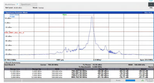
NTNT-n14-PC3-15-5-H-CP-64QAM-Edge_1RB_Right-5.00-12.50 -PASS
