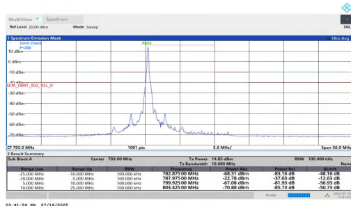
NTNT-n14-PC3-15-10-L-CP-64QAM-Edge_1RB_Left-5.00-10.00-P ASS
