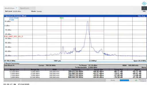
NTNT-n14-PC3-15-5-H-CP-256QAM-Edge_1RB_Right--5.00--2.50-PASS
