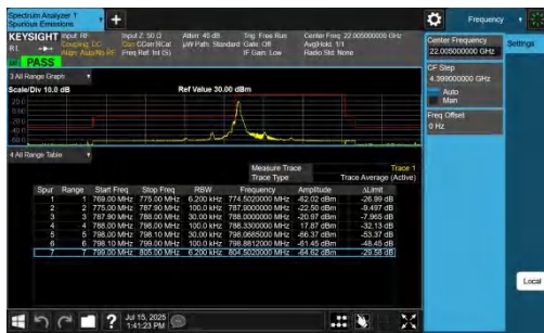
NTNV-n14-PC3-15-5-L-DFT-BPSK-Edge_1RB_Left-PASS
