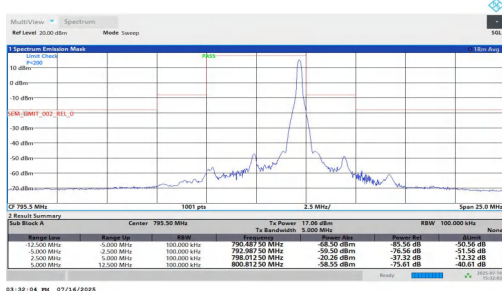
NTNT-n14-PC3-15-5-H-DFT-16QAM-Edge_1RB_Right-2.50-5.00-PASS
