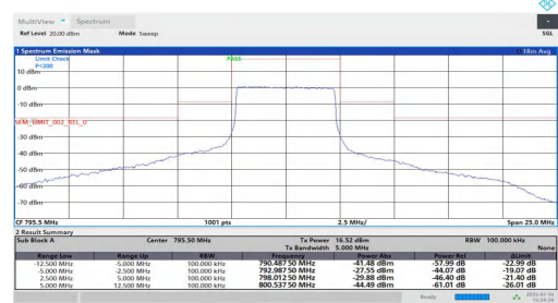
NTNT-n14-PC3-15-5-H-CP-16QAM-Outer_Full-5.00-12.50-PASS
