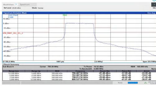
NTNT-n14-PC3-15-5-H-CP-16QAM-Outer_Full--12.50--5.00-PASS
