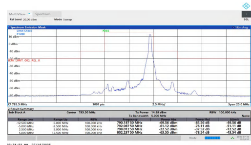
NTNT-n14-PC3-15-5-H-CP-16QAM-Edge_1RB_Right--5.00--2.50-PASS
