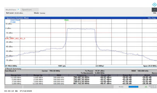
NTNT-n14-PC3-15-5-H-DFT-256QAM-Outer_Full-5.00-12.50-PA SS
