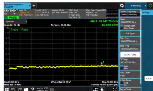
NTNV-n14-PC3-15-5-H-DFT-BPSK-Inner_1RB_Left-3000-12000-P ASS
