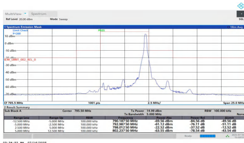
NTNT-n14-PC3-15-5-H-CP-16QAM-Edge_1RB_Right--12.50--5.0-PASS
