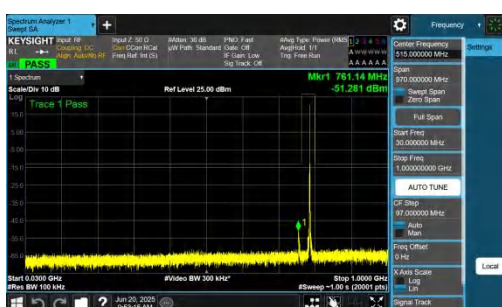
NTNV-n14-PC3-15-5-M-DFT-BPSK-Inner_1RB_Left-30-1000-PASS
