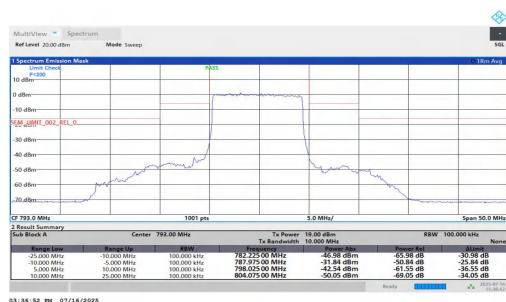
NTNT-n14-PC3-15-10-L-DFT-BPSK-Outer_Full-10.00-25.00-PAS
