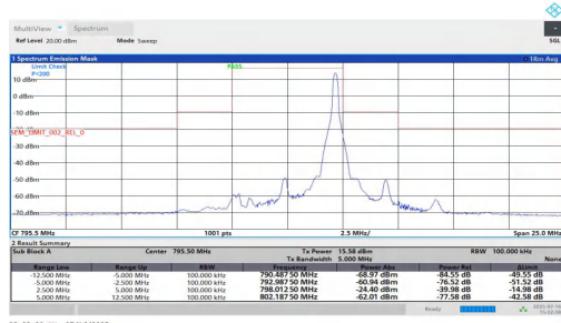
NTNT-n14-PC3-15-5-H-DFT-64QAM-Edge_1RB_Right--12.50--5.0 0-PASS
