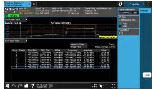
NTNV-n14-PC3-15-10-L-DFT-QPSK-Outer_Full-PASS
