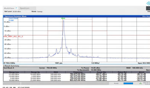
NTNT-n14-PC3-15-10-L-CP-64QAM-Edge_1RB_Left-10.00-25.0 0-PASS
