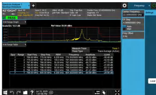
NTNV-n14-PC3-15-5-L-DFT-QPSK-Edge_1RB_Right-PASS
