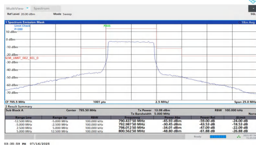
NTNT-n14-PC3-15-5-H-CP-256QAM-Outer_Full--12.50--5.00-PAS
