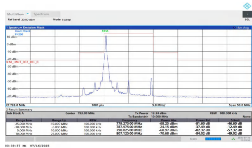
NTNT-n14-PC3-15-10-L-DFT-256QAM-Edge_1RB_Left--10.00--5.00-PASS
