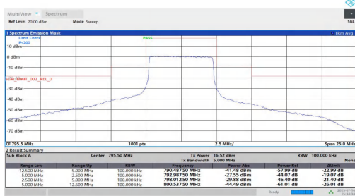
NTNT-n14-PC3-15-5-H-CP-16QAM-Outer_Full-2.50-5.00-PASS
