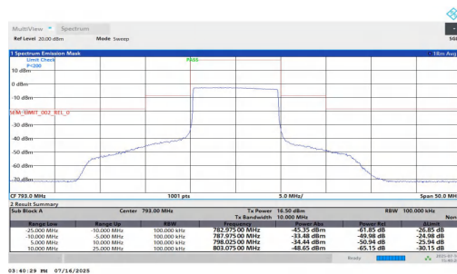
NTNT-n14-PC3-15-10-L-CP-QPSK-Outer Full-10.00-25.00-PAS
