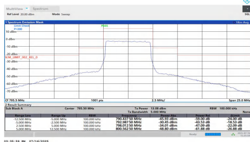
NTNT-n14-PC3-15-5-H-CP-256QAM-Outer Full-2.50-5.00-PASS
