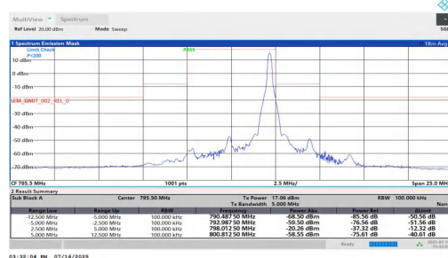
NTNT-n14-PC3-15-5-H-DFT-16QAM-Edge_1RB_Right-5.00-12.5 0-PASS
