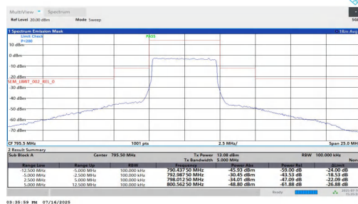
NTNT-n14-PC3-15-5-H-CP-256QAM-Outer_Full--5.00--2.50-PAS
