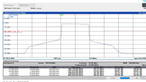
NTNT-n14-PC3-15-10-L-CP-16QAM-Outer_Full-10.00-25.00-PAS
