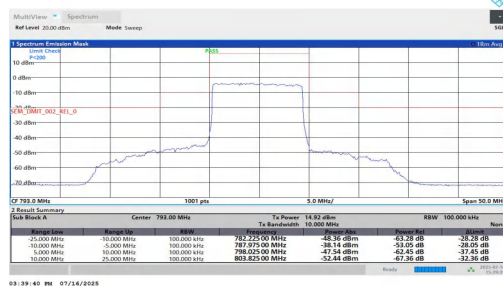
NTNT-n14-PC3-15-10-L-DFT-256QAM-Outer_Full--10.00--5.00-P
