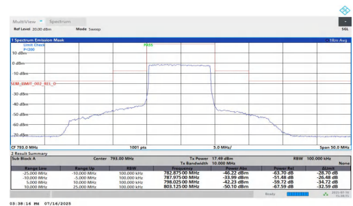
NTNT-n14-PC3-15-10-L-DFT-16QAM-Outer_Full-10.00-25.00-PA SS
