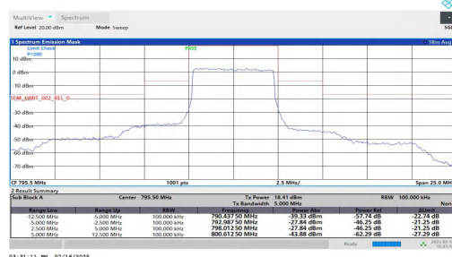
NTNT-n14-PC3-15-5-H-DFT-QPSK-Outer Full-5.00-12.50-PASS
