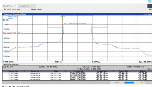
NTNT-n14-PC3-15-5-H-DFT-QPSK-Outer Full-2.50-5.00-PASS
