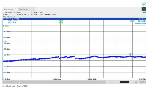
NTNV-n7-PC2-15-25-H-DFT-QPSK-Inner_1RB_Right-3000-12000-PASS
