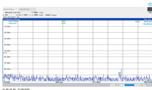
NTNV-n7-PC2-15-20-H-DFT-QPSK-Inner_1RB_Left-0.009-0.15-P ASS
