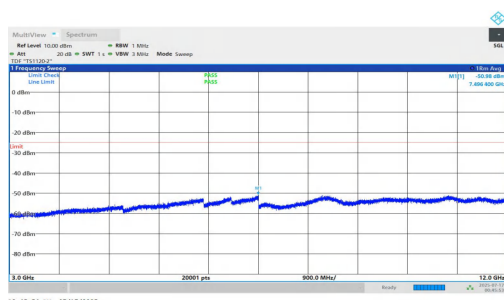
NTNV-n7-PC2-15-20-M-DFT-QPSK-Inner_1RB_Right-3000-1200 0-PASS
