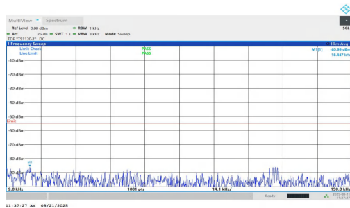
NTNV-n7-PC2-15-25-L-DFT-BPSK-Inner_1RB_Right-0.009-0.15- PASS
