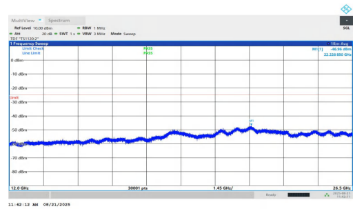
NTNV-n7-PC2-15-25-H-DFT-BPSK-Inner_1RB_Right-12000-2650 0-PASS
