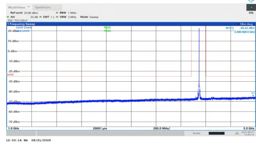
NTNV-n7-PC2-15-25-M-DFT-BPSK-Inner_1RB_Right-1000-3000-P PASS
