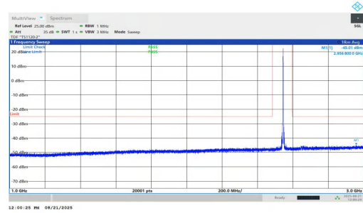
NTNV-n7-PC2-15-20-M-DFT-BPSK-Inner_1RB_Right-1000-3000-P PASS
