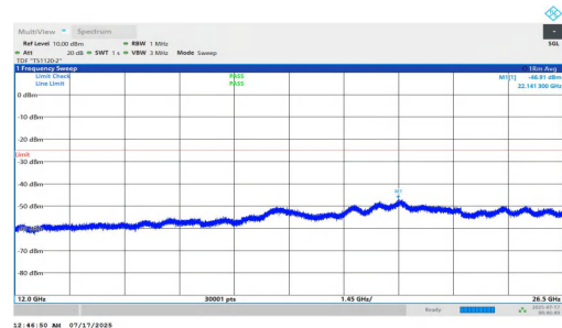
NTNV-n7-PC2-15-20-H-DFT-BPSK-Inner_1RB_Left-12000-26500- PASS
