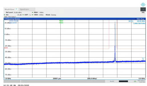
NTNV-n7-PC2-15-20-H-DFT-QPSK-Inner_1RB_Right-1000-3000-PASS
