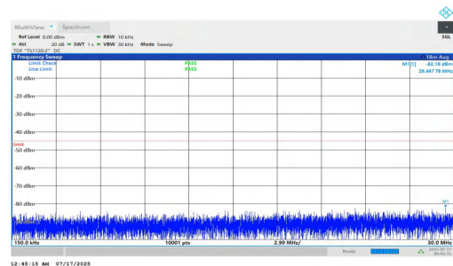
NTNV-n7-PC2-15-20-M-DFT-QPSK-Inner_1RB_Left-0.15-30-PAS S
