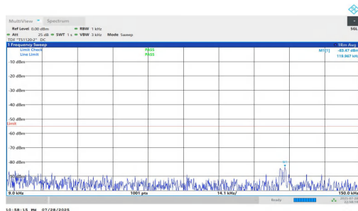
NTNV-n7-PC2-15-20-H-DFT-BPSK-Inner_1RB_Right-0.009-0.15- PASS
