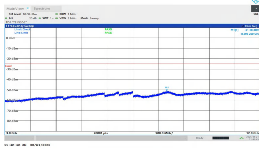
NTNV-n7-PC2-15-25-H-DFT-QPSK-Inner_1RB_Left-3000-12000-PASS
