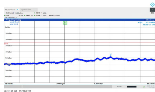
NTNV-n7-PC2-15-25-H-DFT-QPSK-Inner_1RB_Right-12000-26500-PASS
