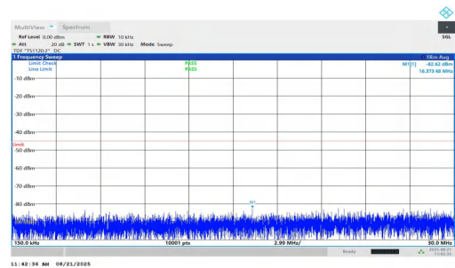
NTNV-n7-PC2-15-25-H-DFT-QPSK-Inner_1RB_Left-0.15-30-PAS S
