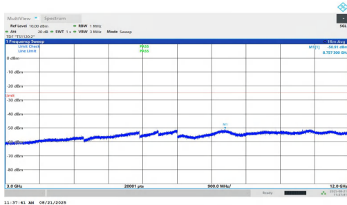
NTNV-n7-PC2-15-25-L-DFT-BPSK-Inner_1RB_Right-3000-12000 -PASS
