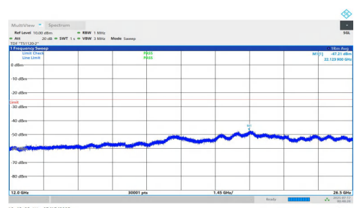
NTNV-n7-PC2-15-20-H-DFT-QPSK-Inner_1RB_Right-12000-26500-PASS
