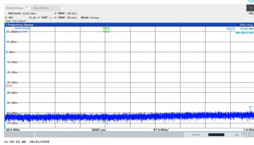
NTNV-n7-PC2-15-25-L-DFT-BPSK-Inner_1RB_Left-30-1000-PAS S
