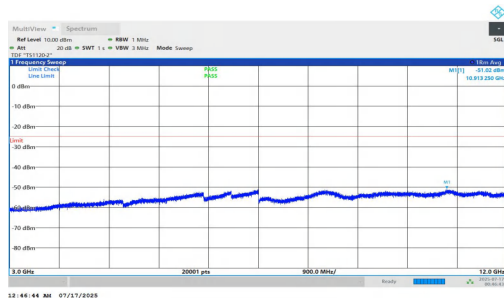
NTNV-n7-PC2-15-20-H-DFT-BPSK-Inner_1RB_Left-3000-12000- PASS
