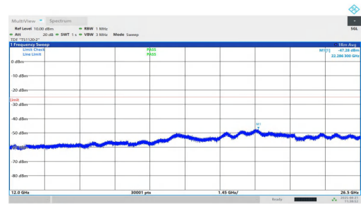
NTNV-n7-PC2-15-25-L-DFT-QPSK-Inner_1RB_Right-12000-26500-PASS
