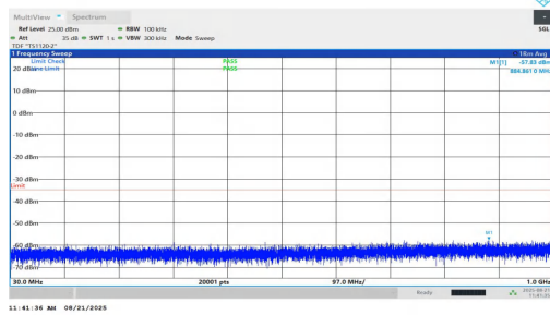
NTNV-n7-PC2-15-25-H-DFT-BPSK-Inner_1RB_Left-30-1000-PASS
