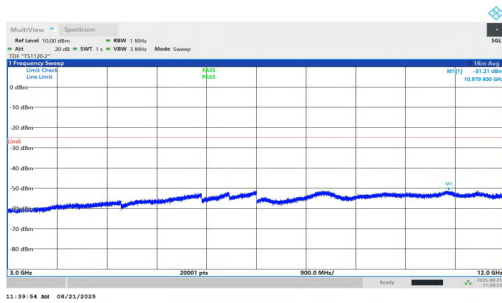
NTNV-n7-PC2-15-25-M-DFT-BPSK-Inner_1RB_Right-3000-1200 0-PASS
