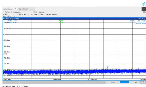
NTNV-n7-PC2-15-20-M-DFT-QPSK-Inner_1RB_Right-30-1000-P ASS
