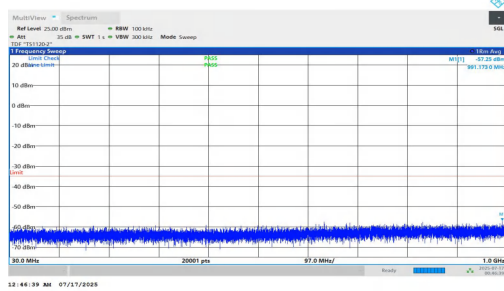
NTNV-n7-PC2-15-20-H-DFT-BPSK-Inner_1RB_Left-30-1000-PASS
