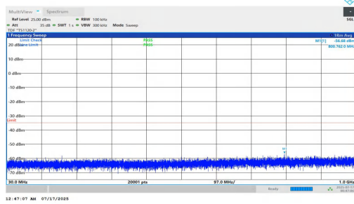
NTNV-n7-PC2-15-20-H-DFT-BPSK-Inner_1RB_Right-30-1000-P ASS
