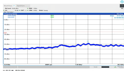
NTNV-n7-PC2-15-25-L-DFT-BPSK-Inner_1RB_Left-12000-26500- PASS
