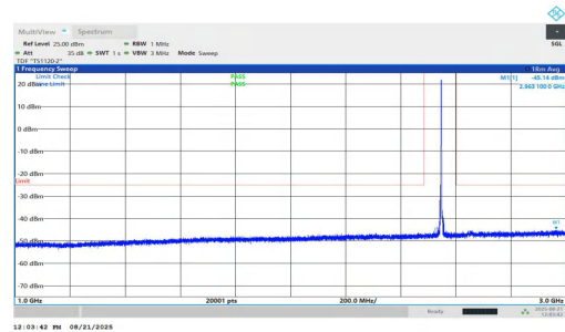
NTNV-n7-PC2-15-25-M-DFT-QPSK-Inner_1RB_Right-1000-3000- PASS
