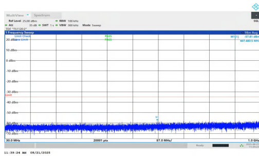
NTNV-n7-PC2-15-25-M-DFT-BPSK-Inner_1RB_Left-30-1000-PASS
