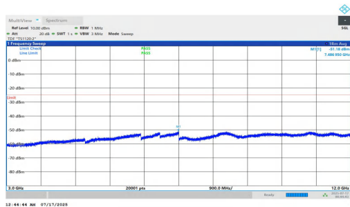
NTNV-n7-PC2-15-20-M-DFT-BPSK-Inner_1RB_Right-3000-1200 0-PASS
