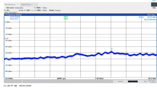
NTNV-n7-PC2-15-25-L-DFT-QPSK-Inner_1RB_Left-12000-26500-PASS
