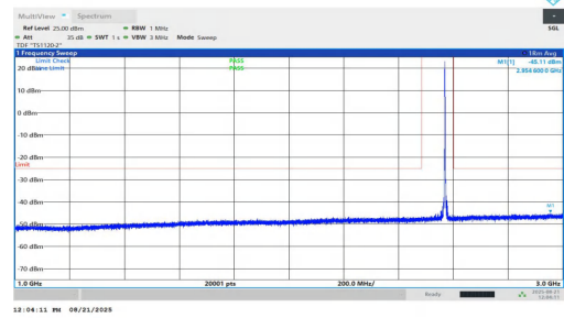
NTNV-n7-PC2-15-25-H-DFT-BPSK-Inner_1RB_Right-1000-3000-P PASS
