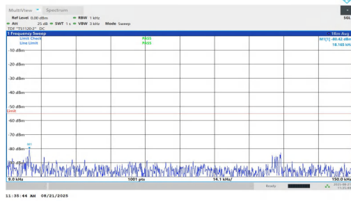
NTNV-n7-PC2-15-25-L-DFT-BPSK-Inner_1RB_Left-0.009-0.15-P ASS
