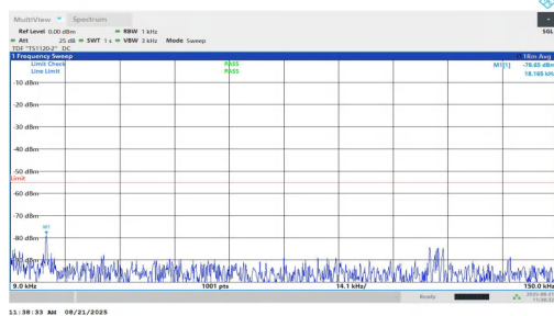
NTNV-n7-PC2-15-25-L-DFT-QPSK-Inner_1RB_Right-0.009-0.15-PASS
