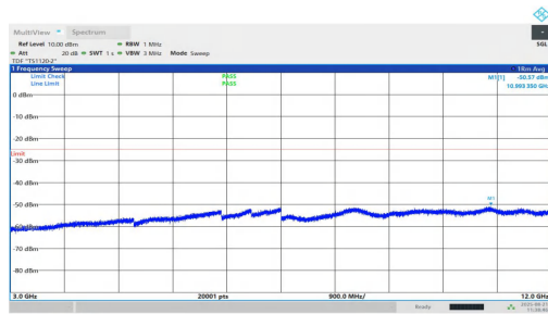
NTNV-n7-PC2-15-25-L-DFT-QPSK-Inner_1RB_Right-3000-12000-PASS
