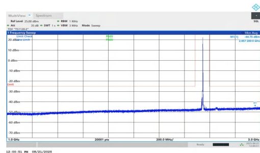
NTNV-n7-PC2-15-20-M-DFT-QPSK-Inner_1RB_Right-1000-3000- PASS
