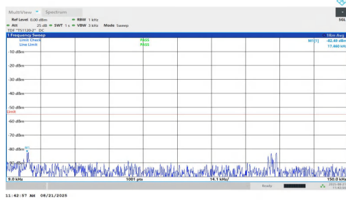
NTNV-n7-PC2-15-25-H-DFT-QPSK-Inner_1RB_Right-0.009-0.15-PASS
