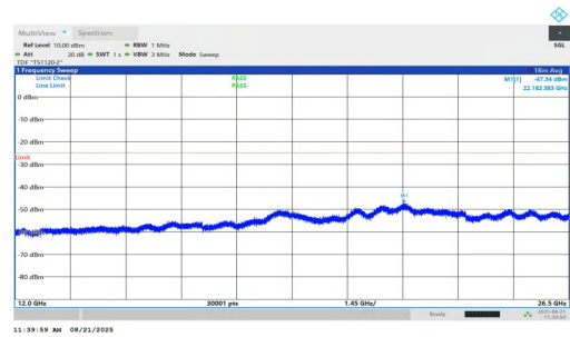
NTNV-n7-PC2-15-25-M-DFT-BPSK-Inner_1RB_Right-12000-2650 0-PASS
