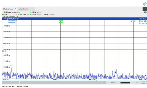
NTNV-n7-PC2-15-25-H-DFT-QPSK-Inner_1RB_Left-0.009-0.15-P ASS
