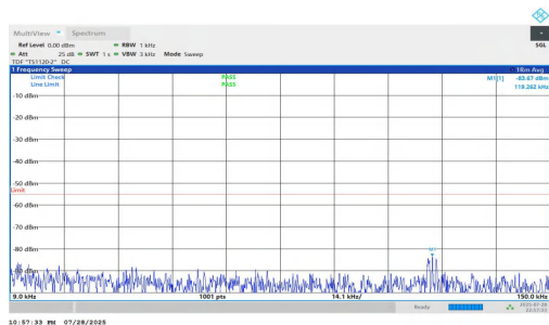
NTNV-n7-PC2-15-20-M-DFT-QPSK-Inner_1RB_Left-0.009-0.15- PASS
