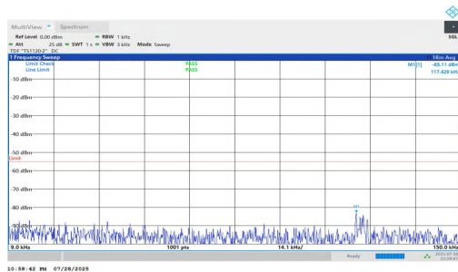
NTNV-n7-PC2-15-20-H-DFT-QPSK-Inner_1RB_Right-0.009-0.15-PASS
