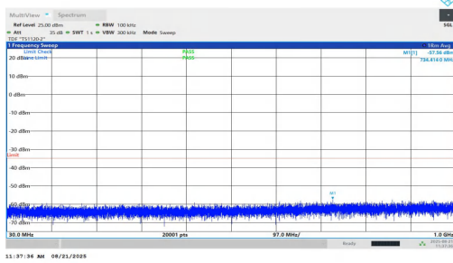
NTNV-n7-PC2-15-25-L-DFT-BPSK-Inner_1RB_Right-30-1000-PA SS
