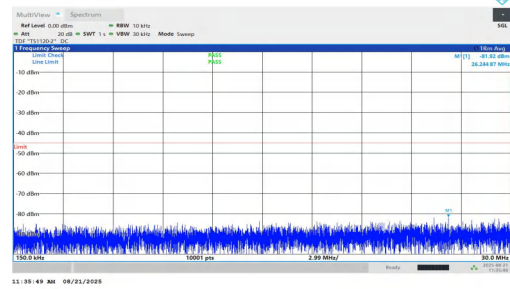
NTNV-n7-PC2-15-25-L-DFT-BPSK-Inner_1RB_Left-0.15-30-PASS
