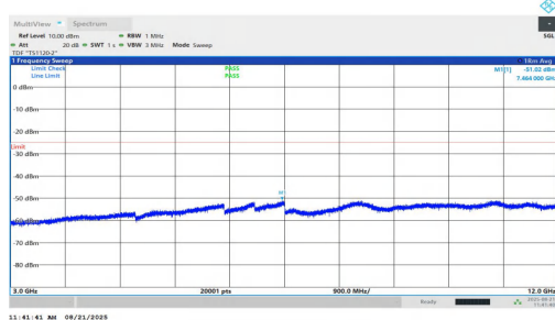
NTNV-n7-PC2-15-25-H-DFT-BPSK-Inner_1RB_Left-3000-12000-PASS
