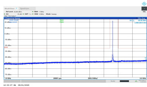
NTNV-n7-PC2-15-25-M-DFT-BPSK-Inner_1RB_Left-1000-3000-PASS
