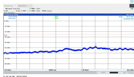
NTNV-n7-PC2-15-25-H-DFT-BPSK-Inner_1RB_Left-12000-26500-PASS
