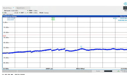
NTNV-n7-PC2-15-25-M-DFT-QPSK-Inner_1RB_Right-3000-1200 0-PASS
