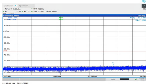
NTNV-n7-PC2-15-25-L-DFT-QPSK-Inner_1RB_Right-30-1000-PASS
