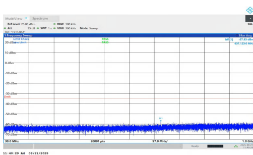
NTNV-n7-PC2-15-25-M-DFT-QPSK-Inner_1RB_Left-30-1000-PA SS
