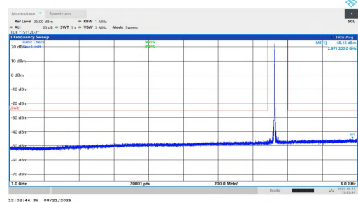
NTNV-n7-PC2-15-25-L-DFT-QPSK-Inner_1RB_Right-1000-3000-PASS
