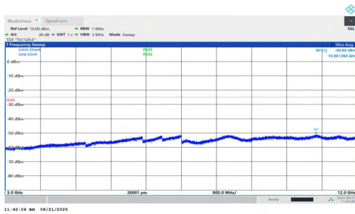
NTNV-n7-PC2-15-25-H-DFT-BPSK-Inner_1RB_Right-3000-1200 0-PASS
