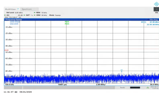
NTNV-n7-PC2-15-25-H-DFT-BPSK-Inner_1RB_Right-0.15-30-PASS
