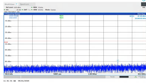
NTNV-n7-PC2-15-25-H-DFT-BPSK-Inner_1RB_Left-0.15-30-PASS
