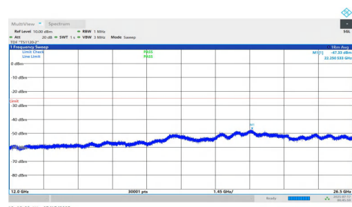
NTNV-n7-PC2-15-20-M-DFT-QPSK-Inner_1RB_Right-12000-2650 0-PASS
