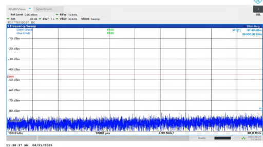
NTNV-n7-PC2-15-25-L-DFT-QPSK-Inner_1RB_Right-0.15-30-PASS
