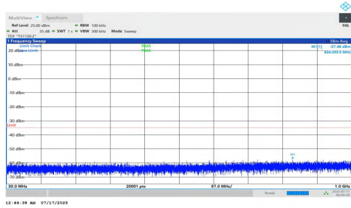
NTNV-n7-PC2-15-20-M-DFT-BPSK-Inner_1RB_Right-30-1000-P ASS
