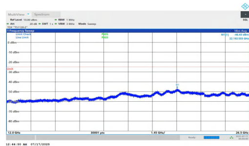
NTNV-n7-PC2-15-20-M-DFT-BPSK-Inner_1RB_Right-12000-2650 0-PASS
