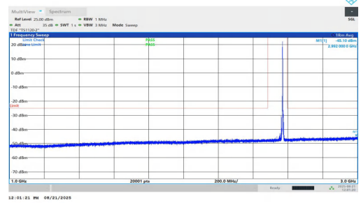
NTNV-n7-PC2-15-20-H-DFT-BPSK-Inner_1RB_Right-1000-3000-P PASS
