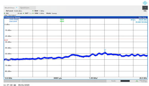
NTNV-n7-PC2-15-25-L-DFT-BPSK-Inner_1RB_Right-12000-2650 0-PASS
