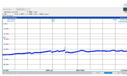
NTNV-n7-PC2-15-20-H-DFT-QPSK-Inner_1RB_Right-3000-12000-PASS
