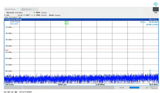
NTNV-n7-PC2-15-20-H-DFT-QPSK-Inner_1RB_Right-0.15-30-PA-SS
