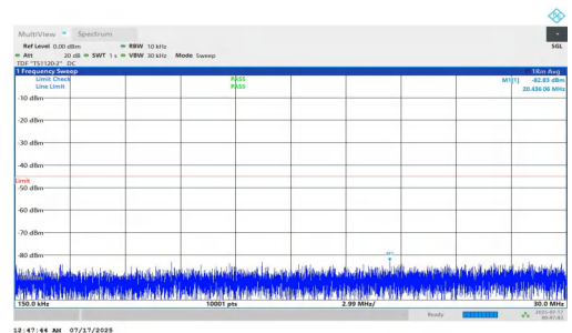
NTNV-n7-PC2-15-20-H-DFT-QPSK-Inner_1RB_Left-0.15-30-PAS S
