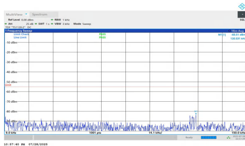
NTNV-n7-PC2-15-20-M-DFT-QPSK-Inner_1RB_Right-0.009-0.15 -PASS
