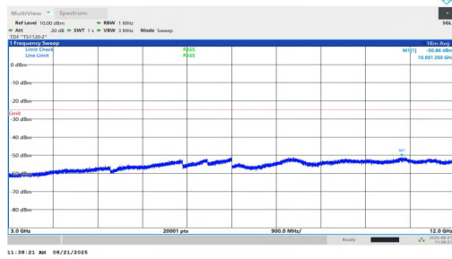
NTNV-n7-PC2-15-25-L-DFT-QPSK-Inner_1RB_Left-3000-12000-PASS
