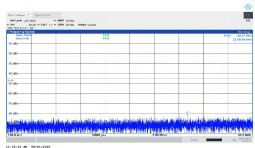
NTNV-n7-PC2-15-25-L-DFT-QPSK-Inner_1RB_Left-0.15-30-PASS
