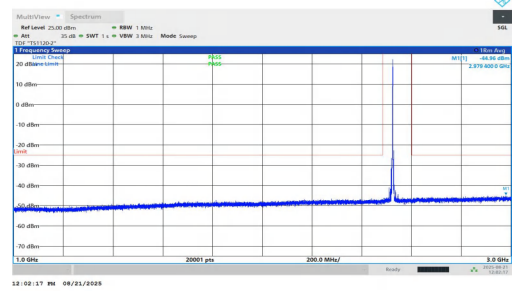
NTNV-n7-PC2-15-25-L-DFT-BPSK-Inner_1RB_Right-1000-3000-P ASS
