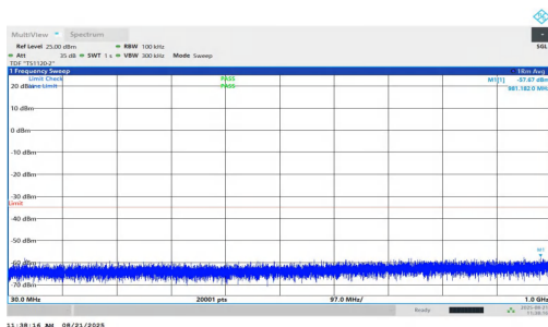
NTNV-n7-PC2-15-25-L-DFT-QPSK-Inner_1RB_Left-30-1000-PA SS
