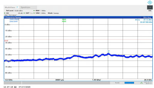
NTNV-n7-PC2-15-20-H-DFT-BPSK-Inner_1RB_Right-12000-2650 0-PASS
