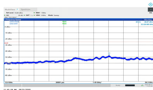
NTNV-n7-PC2-15-25-M-DFT-QPSK-Inner_1RB_Right-12000-2650 0-PASS
