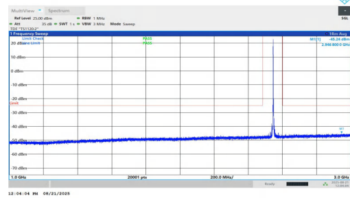
NTNV-n7-PC2-15-25-H-DFT-BPSK-Inner_1RB_Left-1000-3000-PASS
