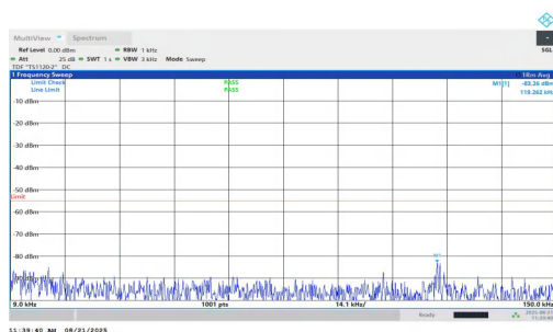
NTNV-n7-PC2-15-25-M-DFT-BPSK-Inner_1RB_Right-0.009-0.15-PASS
