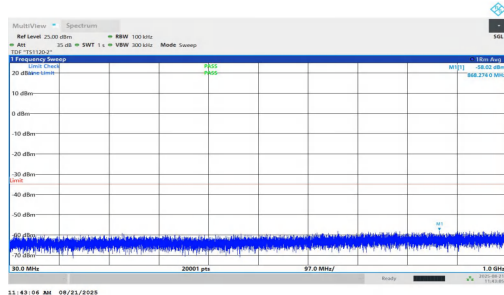
NTNV-n7-PC2-15-25-H-DFT-QPSK-Inner_1RB_Right-30-1000-PASS
