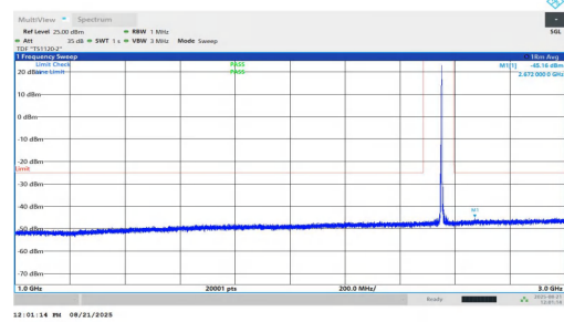
NTNV-n7-PC2-15-20-H-DFT-BPSK-Inner_1RB_Left-1000-3000-P ASS
