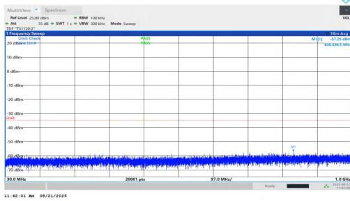
NTNV-n7-PC2-15-25-H-DFT-BPSK-Inner_1RB_Right-30-1000-P ASS
