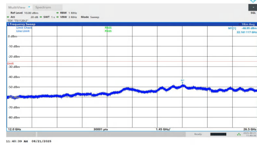
NTNV-n7-PC2-15-25-M-DFT-QPSK-Inner_1RB_Left-12000-26500 -PASS
