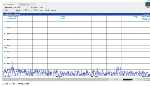
NTNV-n7-PC2-15-25-M-DFT-BPSK-Inner_1RB_Left-0.009-0.15-PASS
