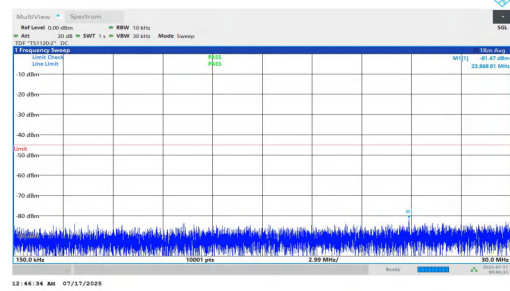
NTNV-n7-PC2-15-20-H-DFT-BPSK-Inner_1RB_Left-0.15-30-PASS
