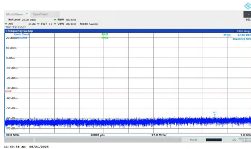
NTNV-n7-PC2-15-25-M-DFT-QPSK-Inner_1RB_Right-30-1000-P ASS
