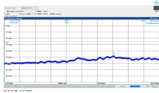
NTNV-n7-PC2-15-20-M-DFT-QPSK-Inner_1RB_Left-12000-26500 -PASS
