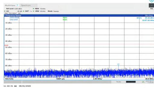
NTNV-n7-PC2-15-25-H-DFT-QPSK-Inner_1RB_Right-0.15-30-PA-SS
