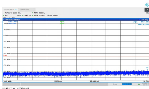
NTNV-n7-PC2-15-20-H-DFT-QPSK-Inner_1RB_Right-30-1000-PASS
