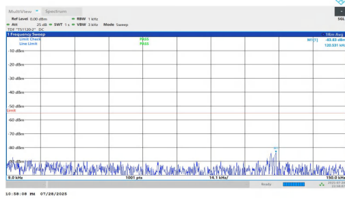
NTNV-n7-PC2-15-20-H-DFT-BPSK-Inner_1RB_Left-0.009-0.15-P ASS
