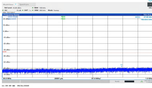
NTNV-n7-PC2-15-25-M-DFT-BPSK-Inner_1RB_Right-30-1000-P ASS
