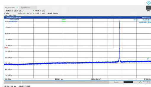
NTNV-n7-PC2-15-25-H-DFT-QPSK-Inner_1RB_Right-1000-3000-PASS
