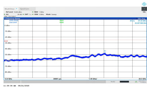
NTNV-n7-PC2-15-25-M-DFT-BPSK-Inner_1RB_Left-12000-26500-PASS
