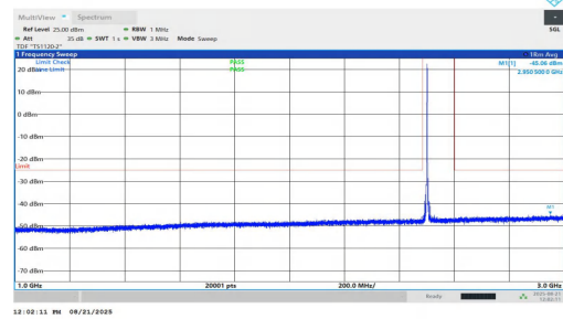
NTNV-n7-PC2-15-25-L-DFT-BPSK-Inner_1RB_Left-1000-3000-PASS SS
