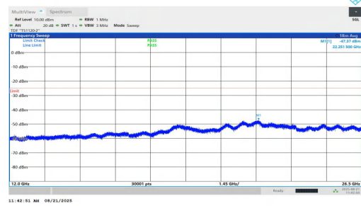
NTNV-n7-PC2-15-25-H-DFT-QPSK-Inner_1RB_Left-12000-26500-PASS
