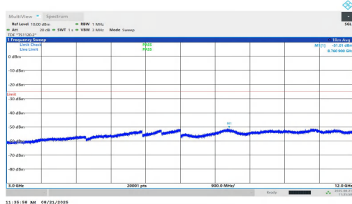
NTNV-n7-PC2-15-25-L-DFT-BPSK-Inner_1RB_Left-3000-12000- PASS
