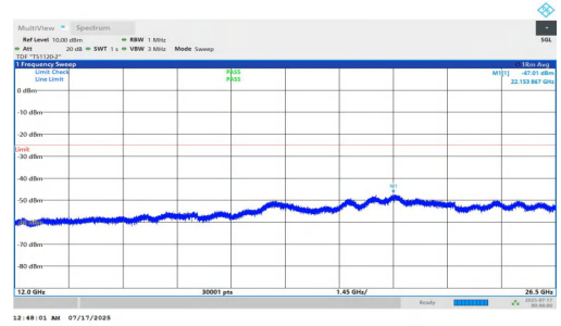
NTNV-n7-PC2-15-20-H-DFT-QPSK-Inner_1RB_Left-12000-26500-PASS
