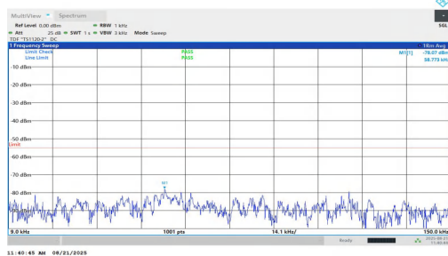
NTNV-n7-PC2-15-25-M-DFT-QPSK-Inner_1RB_Right-0.009-0.15 -PASS
