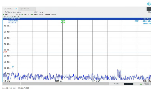
NTNV-n7-PC2-15-25-H-DFT-BPSK-Inner_1RB_Right-0.009-0.15-PASS
