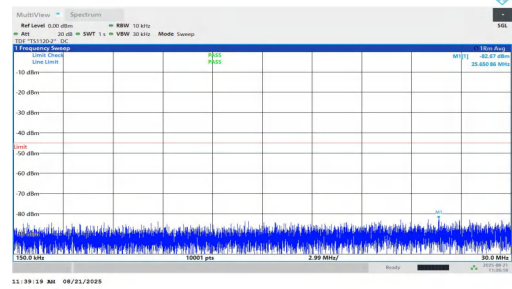
NTNV-n7-PC2-15-25-M-DFT-BPSK-Inner_1RB_Left-0.15-30-PASS
