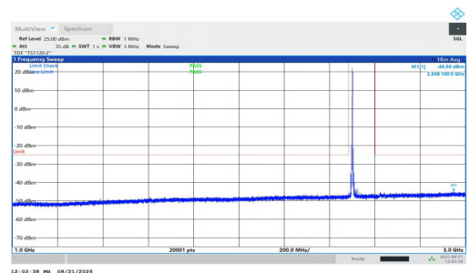
NTNV-n7-PC2-15-25-L-DFT-QPSK-Inner_1RB_Left-1000-3000-PA SS
