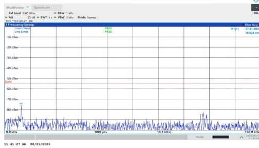
NTNV-n7-PC2-15-25-H-DFT-BPSK-Inner_1RB_Left-0.009-0.15-P ASS
