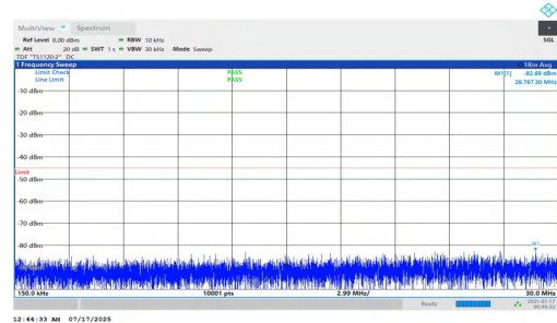
NTNV-n7-PC2-15-20-M-DFT-BPSK-Inner_1RB_Right-0.15-30-PASS
