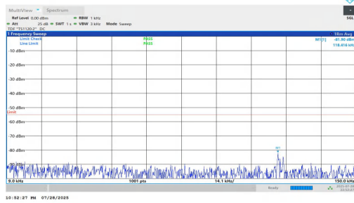
NTNV-n7-PC2-15-15-L-DFT-BPSK-Inner_1RB_Left-0.009-0.15-P ASS
