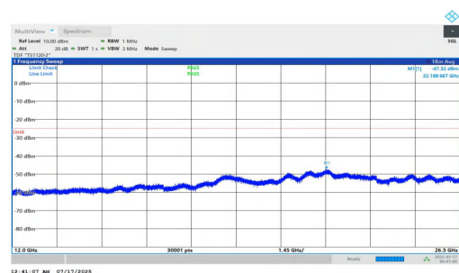
NTNV-n7-PC2-15-15-H-DFT-QPSK-Inner_1RB_Right-12000-26500-PASS
