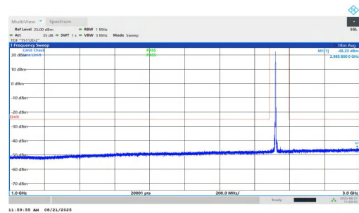
NTNV-n7-PC2-15-20-L-DFT-QPSK-Inner_1RB_Right-1000-3000-PASS
