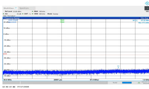
NTNV-n7-PC2-15-20-L-DFT-BPSK-Inner_1RB_Right-30-1000-PA SS
