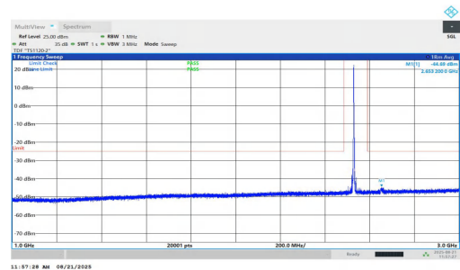
NTNV-n7-PC2-15-15-M-DFT-BPSK-Inner_1RB_Left-1000-3000-PASS
