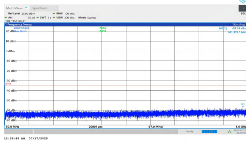
NTNV-n7-PC2-15-15-H-DFT-BPSK-Inner_1RB_Right-30-1000-P ASS
