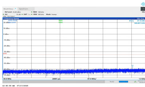
NTNV-n7-PC2-15-15-H-DFT-QPSK-Inner_1RB_Right-30-1000-PASS
