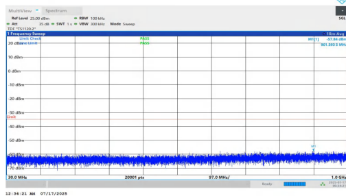
NTNV-n7-PC2-15-15-L-DFT-BPSK-Inner_1RB_Left-30-1000-PAS S
