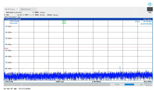
NTNV-n7-PC2-15-20-L-DFT-QPSK-Inner_1RB_Left-0.15-30-PASS
