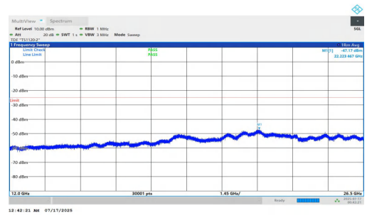
NTNV-n7-PC2-15-20-L-DFT-BPSK-Inner_1RB_Right-12000-2650 0-PASS
