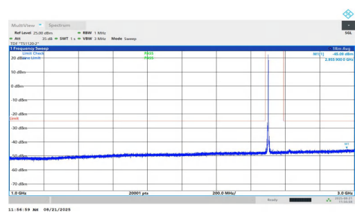
NTNV-n7-PC2-15-15-L-DFT-QPSK-Inner_1RB_Left-1000-3000-PA SS
