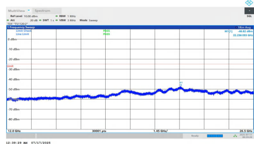
NTNV-n7-PC2-15-15-H-DFT-BPSK-Inner_1RB_Left-12000-26500-PASS
