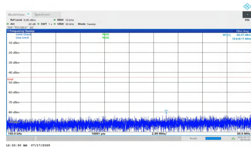
NTNV-n7-PC2-15-10-H-DFT-QPSK-Inner_1RB_Right-0.15-30-PA-SS
