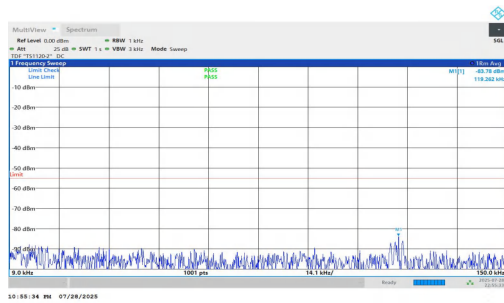
NTNV-n7-PC2-15-15-H-DFT-QPSK-Inner_1RB_Right-0.009-0.15-PASS
