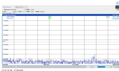
NTNV-n7-PC2-15-10-H-DFT-QPSK-Inner_1RB_Right-0.009-0.15-PASS
