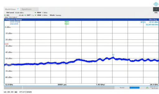
NTNV-n7-PC2-15-15-L-DFT-BPSK-Inner_1RB_Right-12000-2650 0-PASS
