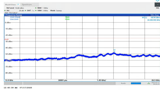
NTNV-n7-PC2-15-15-H-DFT-QPSK-Inner_1RB_Left-12000-26500-PASS
