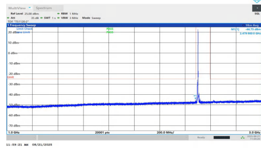
NTNV-n7-PC2-15-20-L-DFT-BPSK-Inner_1RB_Left-1000-3000-PASS
