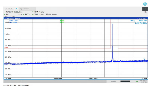
NTNV-n7-PC2-15-15-L-DFT-QPSK-Inner_1RB_Right-1000-3000-PASS
