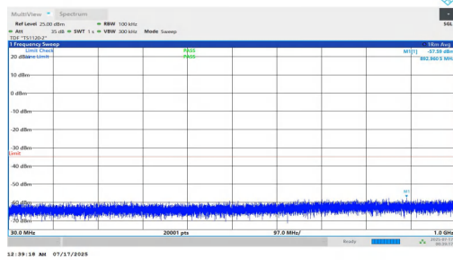
NTNV-n7-PC2-15-15-H-DFT-BPSK-Inner_1RB_Left-30-1000-PASS
