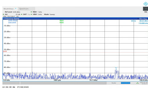
NTNV-n7-PC2-15-20-L-DFT-QPSK-Inner_1RB_Right-0.009-0.15-PASS
