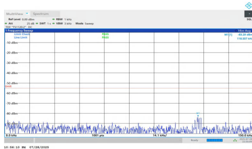
NTNV-n7-PC2-15-20-L-DFT-BPSK-Inner_1RB_Right-0.009-0.15- PASS
