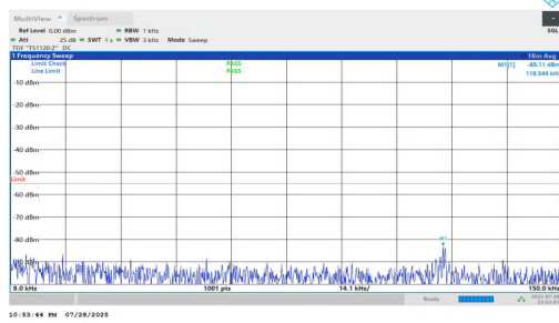
NTNV-n7-PC2-15-15-M-DFT-BPSK-Inner_1RB_Left-0.009-0.15-PASS
