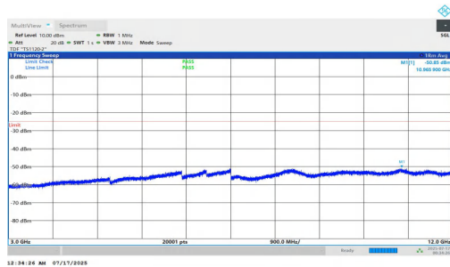
NTNV-n7-PC2-15-15-L-DFT-BPSK-Inner_1RB_Left-3000-12000- PASS
