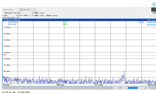
NTNV-n7-PC2-15-15-M-DFT-QPSK-Inner_1RB_Left-0.009-0.15- PASS
