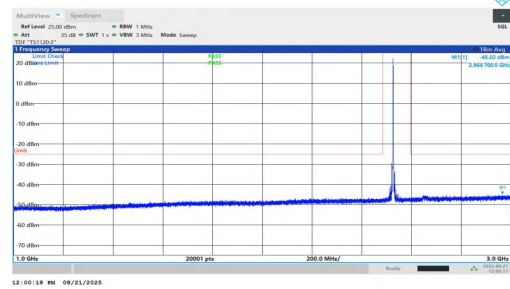
NTNV-n7-PC2-15-20-M-DFT-BPSK-Inner_1RB_Left-1000-3000-PASS
