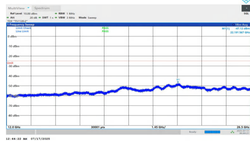
NTNV-n7-PC2-15-20-M-DFT-BPSK-Inner_1RB_Left-12000-26500-PASS
