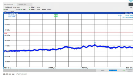
NTNV-n7-PC2-15-15-M-DFT-QPSK-Inner_1RB_Left-12000-26500 -PASS
