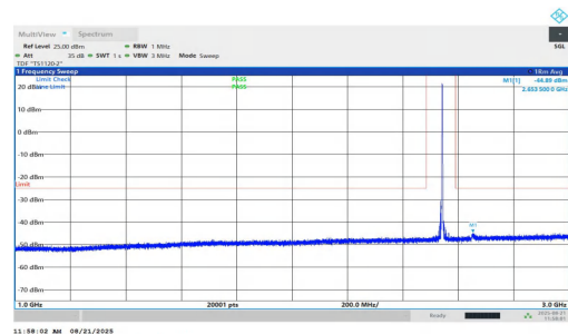
NTNV-n7-PC2-15-15-M-DFT-QPSK-Inner_1RB_Right-1000-3000- PASS
