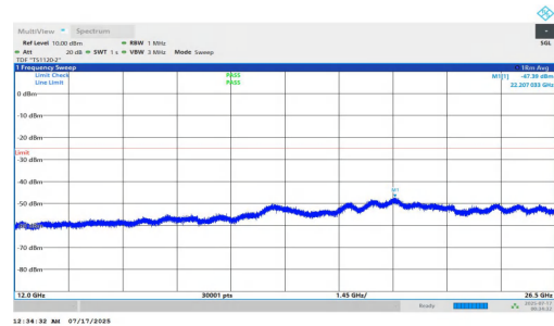
NTNV-n7-PC2-15-15-L-DFT-BPSK-Inner_1RB_Left-12000-26500- PASS
