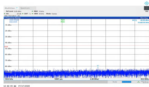
NTNV-n7-PC2-15-20-L-DFT-BPSK-Inner_1RB_Right-0.15-30-PAS S
