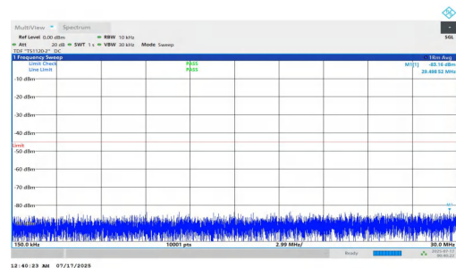
NTNV-n7-PC2-15-15-H-DFT-QPSK-Inner_1RB_Left-0.15-30-PAS S
