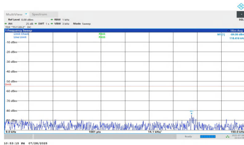
NTNV-n7-PC2-15-15-L-DFT-QPSK-Inner_1RB_Right-0.009-0.15-PASS
