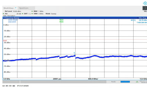
NTNV-n7-PC2-15-15-H-DFT-QPSK-Inner_1RB_Left-3000-12000-PASS
