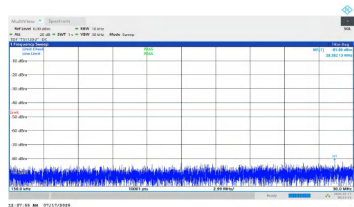
NTNV-n7-PC2-15-15-M-DFT-QPSK-Inner_1RB_Left-0.15-30-PAS S
