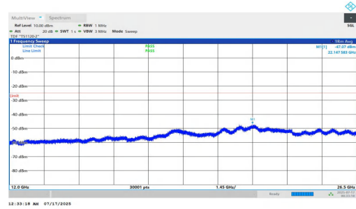
NTNV-n7-PC2-15-10-H-DFT-QPSK-Inner_1RB_Left-12000-26500-PASS
