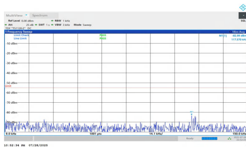
NTNV-n7-PC2-15-15-L-DFT-BPSK-Inner_1RB_Right-0.009-0.15- PASS
