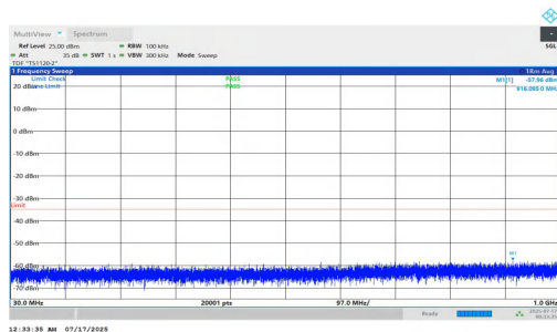
NTNV-n7-PC2-15-10-H-DFT-QPSK-Inner_1RB_Right-30-1000-PASS
