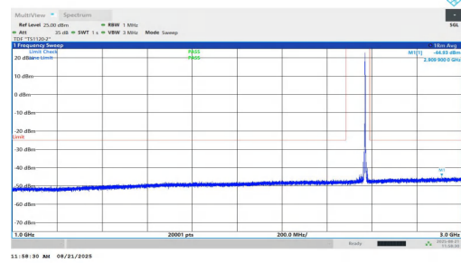
NTNV-n7-PC2-15-15-H-DFT-BPSK-Inner_1RB_Right-1000-3000-P PASS
