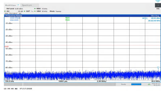
NTNV-n7-PC2-15-15-M-DFT-BPSK-Inner_1RB_Left-0.15-30-PASS
