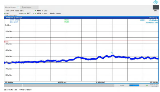
NTNV-n7-PC2-15-15-L-DFT-QPSK-Inner_1RB_Left-12000-26500-PASS
