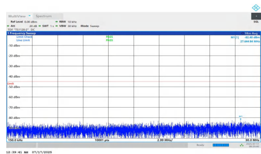
NTNV-n7-PC2-15-15-H-DFT-BPSK-Inner_1RB_Right-0.15-30-PASS
