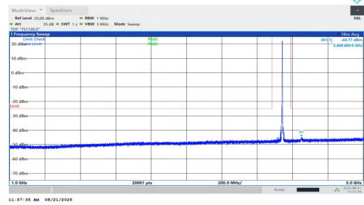
NTNV-n7-PC2-15-15-M-DFT-BPSK-Inner_1RB_Right-1000-3000-P PASS
