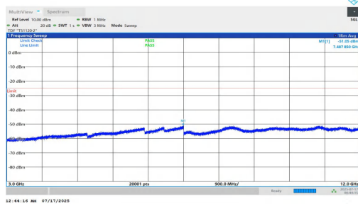
NTNV-n7-PC2-15-20-M-DFT-BPSK-Inner_1RB_Left-3000-12000-PASS
