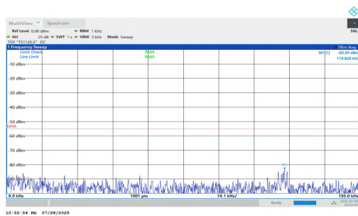
NTNV-n7-PC2-15-15-L-DFT-QPSK-Inner_1RB_Left-0.009-0.15-P ASS
