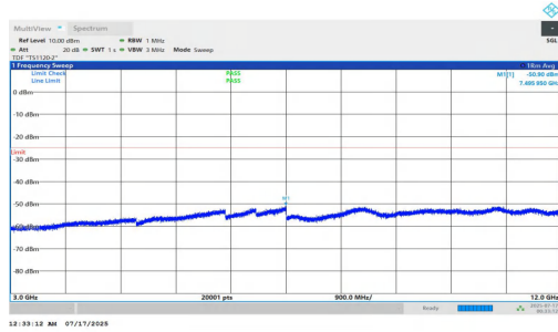
NTNV-n7-PC2-15-10-H-DFT-QPSK-Inner_1RB_Left-3000-12000-PASS
