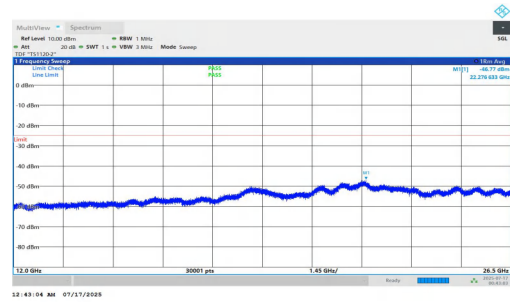
NTNV-n7-PC2-15-20-L-DFT-QPSK-Inner_1RB_Left-12000-26500-PASS
