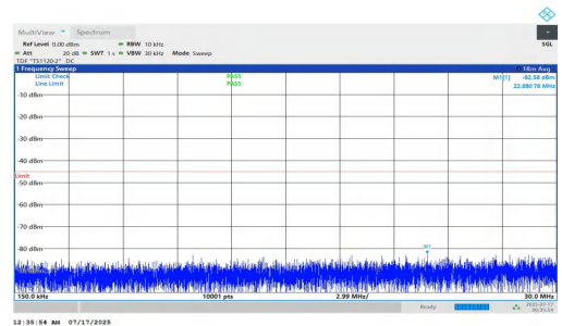
NTNV-n7-PC2-15-15-L-DFT-QPSK-Inner_1RB_Right-0.15-30-PASS
