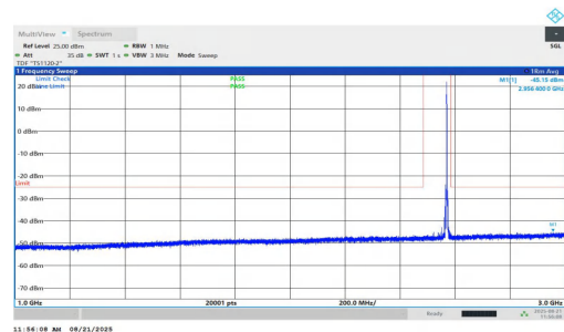
NTNV-n7-PC2-15-10-H-DFT-QPSK-Inner_1RB_Right-1000-3000-PASS
