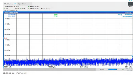
NTNV-n7-PC2-15-15-H-DFT-BPSK-Inner_1RB_Left-0.15-30-PASS
