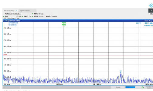
NTNV-n7-PC2-15-15-M-DFT-BPSK-Inner_1RB_Right-0.009-0.15-PASS
