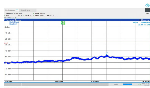
NTNV-n7-PC2-15-15-M-DFT-QPSK-Inner_1RB_Right-12000-2650 0-PASS
