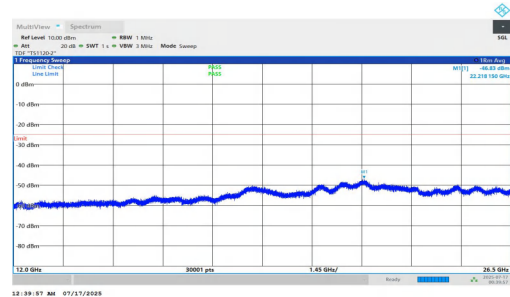
NTNV-n7-PC2-15-15-H-DFT-BPSK-Inner_1RB_Right-12000-2650 0-PASS
