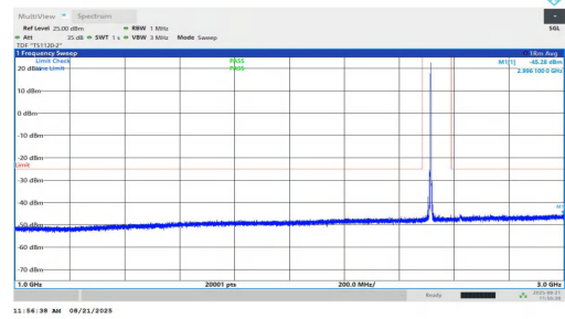
NTNV-n7-PC2-15-15-L-DFT-BPSK-Inner_1RB_Right-1000-3000-P ASS
