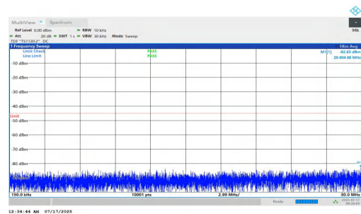
NTNV-n7-PC2-15-15-L-DFT-BPSK-Inner_1RB_Right-0.15-30-PASS
