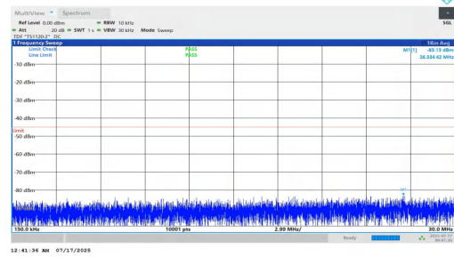
NTNV-n7-PC2-15-20-L-DFT-BPSK-Inner_1RB_Left-0.15-30-PASS
