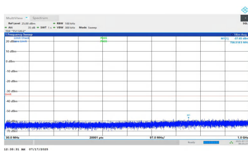
NTNV-n7-PC2-15-15-L-DFT-QPSK-Inner_1RB_Left-30-1000-PA SS
