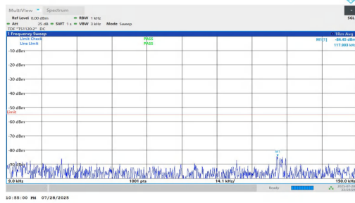
NTNV-n7-PC2-15-15-H-DFT-BPSK-Inner_1RB_Left-0.009-0.15-P ASS
