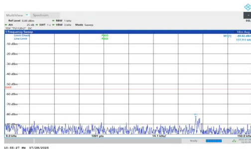
NTNV-n7-PC2-15-15-H-DFT-QPSK-Inner_1RB_Left-0.009-0.15-P ASS
