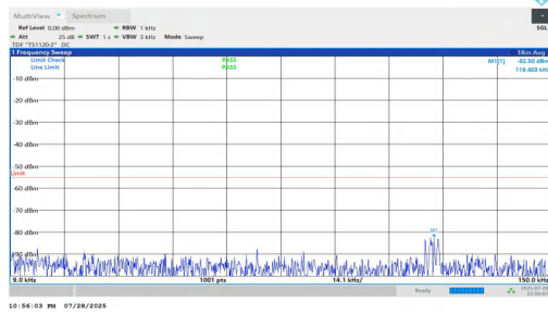
NTNV-n7-PC2-15-20-L-DFT-BPSK-Inner_1RB_Left-0.009-0.15-P ASS
