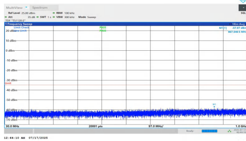
NTNV-n7-PC2-15-20-M-DFT-BPSK-Inner_1RB_Left-30-1000-PASS
