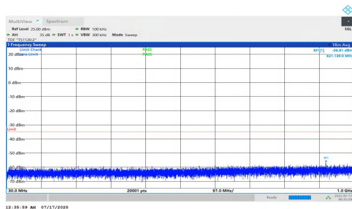
NTNV-n7-PC2-15-15-L-DFT-QPSK-Inner_1RB_Right-30-1000-PASS
