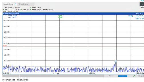
NTNV-n7-PC2-15-20-M-DFT-BPSK-Inner_1RB_Left-0.009-0.15-PASS
