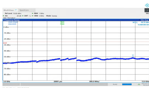
NTNV-n7-PC2-15-15-L-DFT-QPSK-Inner_1RB_Right-3000-12000-PASS
