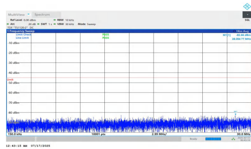
NTNV-n7-PC2-15-20-L-DFT-QPSK-Inner_1RB_Right-0.15-30-PASS
