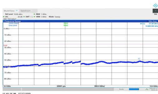
NTNV-n7-PC2-15-20-L-DFT-QPSK-Inner_1RB_Right-3000-12000-PASS
