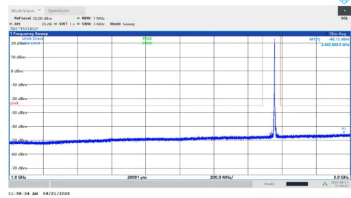
NTNV-n7-PC2-15-15-H-DFT-BPSK-Inner_1RB_Left-1000-3000-PASS
