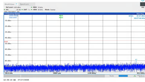
NTNV-n7-PC2-15-15-L-DFT-BPSK-Inner_1RB_Left-0.15-30-PASS
