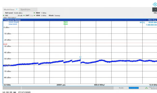
NTNV-n7-PC2-15-15-M-DFT-BPSK-Inner_1RB_Left-3000-12000-PASS
