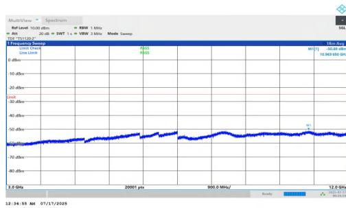
NTNV-n7-PC2-15-15-L-DFT-BPSK-Inner_1RB_Right-3000-12000 -PASS
