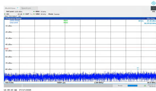
NTNV-n7-PC2-15-15-M-DFT-QPSK-Inner_1RB_Right-0.15-30-PA SS
