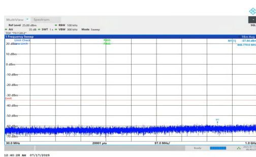
NTNV-n7-PC2-15-15-H-DFT-QPSK-Inner_1RB_Left-30-1000-PA SS
