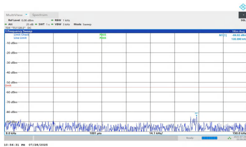
NTNV-n7-PC2-15-20-L-DFT-QPSK-Inner_1RB_Left-0.009-0.15-P ASS
