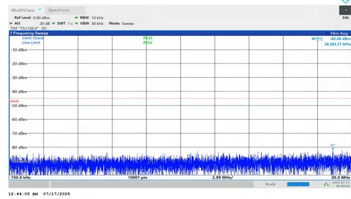
NTNV-n7-PC2-15-20-M-DFT-BPSK-Inner_1RB_Left-0.15-30-PASS
