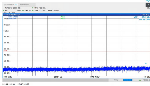
NTNV-n7-PC2-15-20-L-DFT-BPSK-Inner_1RB_Left-30-1000-PAS S
