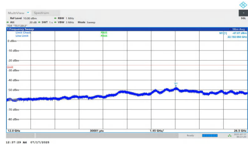
NTNV-n7-PC2-15-15-M-DFT-BPSK-Inner_1RB_Right-12000-2650 0-PASS
