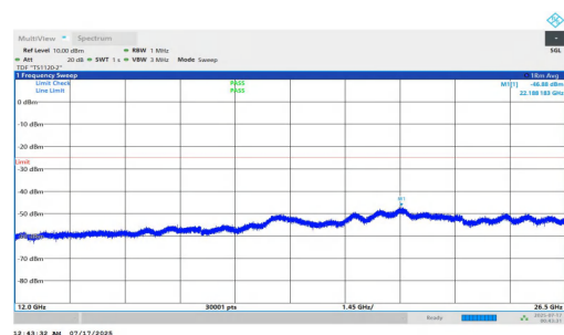
NTNV-n7-PC2-15-20-L-DFT-QPSK-Inner_1RB_Right-12000-26500-PASS
