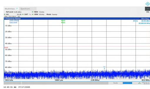
NTNV-n7-PC2-15-15-H-DFT-QPSK-Inner_1RB_Right-0.15-30-PA-SS
