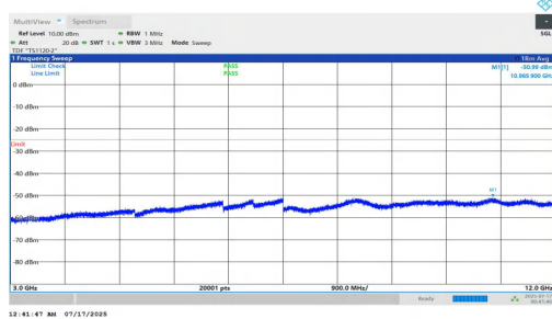
NTNV-n7-PC2-15-20-L-DFT-BPSK-Inner_1RB_Left-3000-12000- PASS
