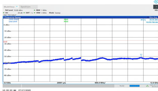
NTNV-n7-PC2-15-15-H-DFT-BPSK-Inner_1RB_Left-3000-12000-PASS
