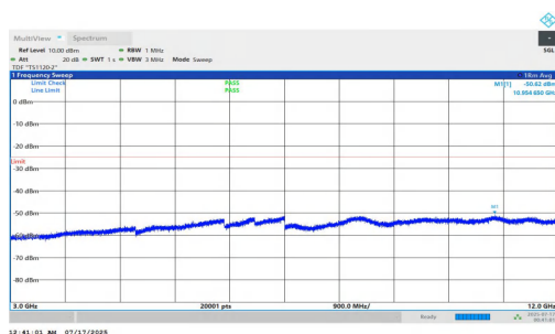
NTNV-n7-PC2-15-15-H-DFT-QPSK-Inner_1RB_Right-3000-12000-PASS
