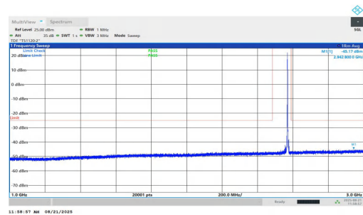
NTNV-n7-PC2-15-15-H-DFT-QPSK-Inner_1RB_Right-1000-3000-PASS
