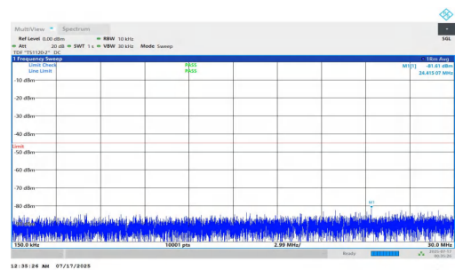
NTNV-n7-PC2-15-15-L-DFT-QPSK-Inner_1RB_Left-0.15-30-PASS
