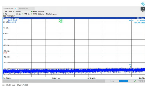
NTNV-n7-PC2-15-15-M-DFT-BPSK-Inner_1RB_Left-30-1000-PASS
