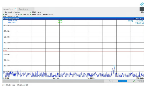
NTNV-n7-PC2-15-15-H-DFT-BPSK-Inner_1RB_Right-0.009-0.15-PASS
