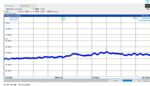
NTNV-n7-PC2-15-20-L-DFT-BPSK-Inner_1RB_Left-12000-26500- PASS
