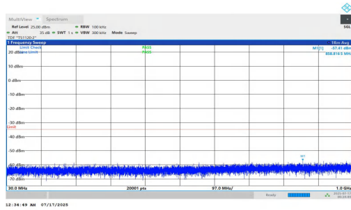
NTNV-n7-PC2-15-15-L-DFT-BPSK-Inner_1RB_Right-30-1000-PA SS
