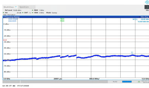
NTNV-n7-PC2-15-15-L-DFT-QPSK-Inner_1RB_Left-3000-12000-PASS
