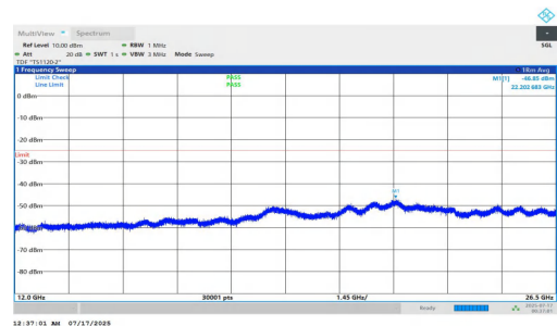
NTNV-n7-PC2-15-15-M-DFT-BPSK-Inner_1RB_Left-12000-26500-PASS
