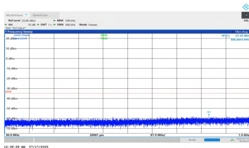
NTNV-n7-PC2-15-15-M-DFT-QPSK-Inner_1RB_Right-30-1000-P ASS
