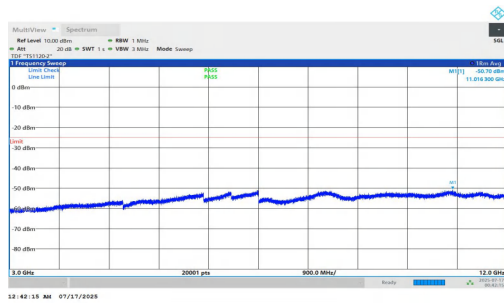
NTNV-n7-PC2-15-20-L-DFT-BPSK-Inner_1RB_Right-3000-12000 -PASS
