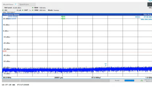
NTNV-n7-PC2-15-15-M-DFT-BPSK-Inner_1RB_Right-30-1000-P ASS
