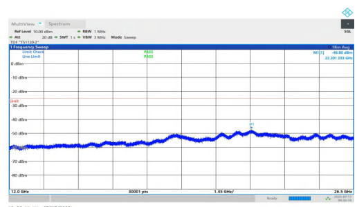
NTNV-n7-PC2-15-15-L-DFT-QPSK-Inner_1RB_Right-12000-26500-PASS
