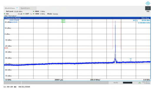
NTNV-n7-PC2-15-20-L-DFT-BPSK-Inner_1RB_Right-1000-3000-P ASS
