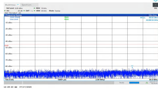
NTNV-n7-PC2-15-10-L-DFT-QPSK-Inner_1RB_Right-0.15-30-PASS
