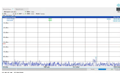
NTNV-n7-PC2-15-5-H-DFT-BPSK-Inner_1RB_Right-0.009-0.15-P ASS
