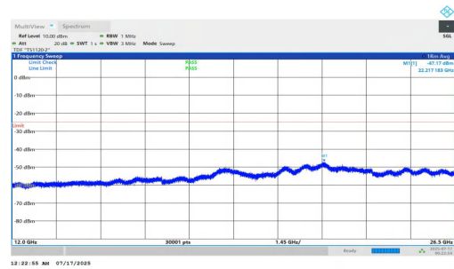
NTNV-n7-PC2-15-5-M-DFT-BPSK-Inner_1RB_Right-12000-26500 -PASS
