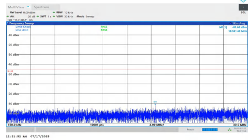
NTNV-n7-PC2-15-10-H-DFT-BPSK-Inner_1RB_Left-0.15-30-PASS
