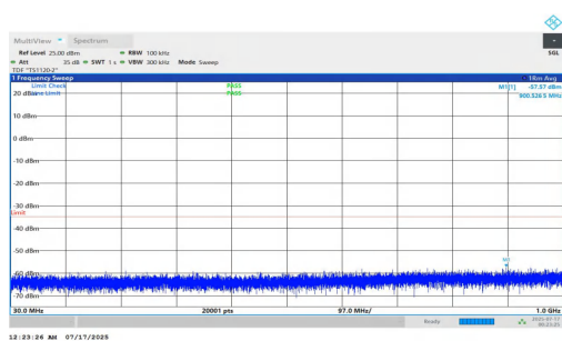
NTNV-n7-PC2-15-5-M-DFT-QPSK-Inner_1RB_Left-30-1000-PAS S
