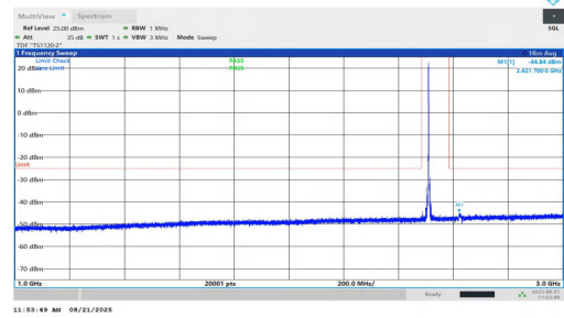
NTNV-n7-PC2-15-10-L-DFT-BPSK-Inner_1RB_Right-1000-3000-P ASS
