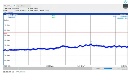
NTNV-n7-PC2-15-10-H-DFT-BPSK-Inner_1RB_Left-12000-26500- PASS
