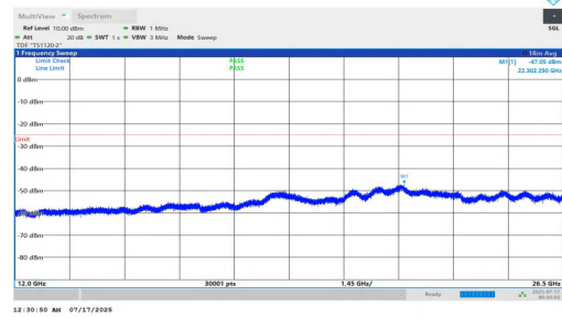
NTNV-n7-PC2-15-10-M-DFT-QPSK-Inner_1RB_Left-12000-26500 -PASS
