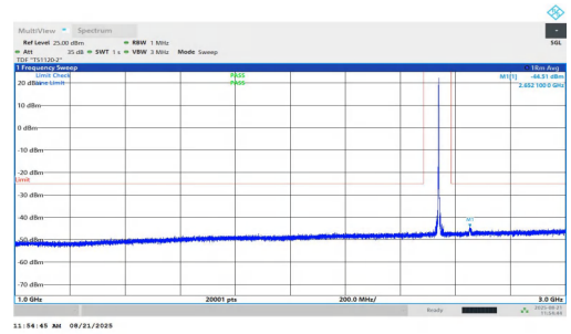
NTNV-n7-PC2-15-10-M-DFT-BPSK-Inner_1RB_Right-1000-3000-P PASS
