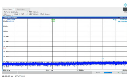
NTNV-n7-PC2-15-10-H-DFT-QPSK-Inner_1RB_Left-30-1000-PA SS
