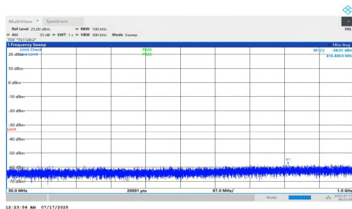
NTNV-n7-PC2-15-5-M-DFT-QPSK-Inner_1RB_Right-30-1000-PASS
