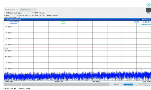
NTNV-n7-PC2-15-10-H-DFT-QPSK-Inner_1RB_Left-0.15-30-PAS S
