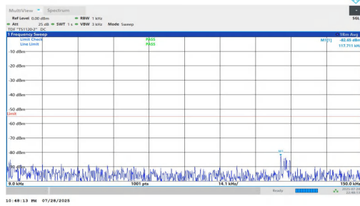
NTNV-n7-PC2-15-5-H-DFT-BPSK-Inner_1RB_Left-0.009-0.15-PA SS
