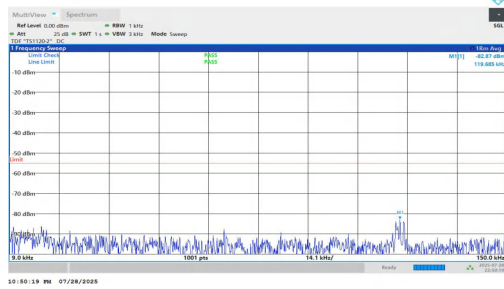
NTNV-n7-PC2-15-10-M-DFT-BPSK-Inner_1RB_Left-0.009-0.15-PASS
