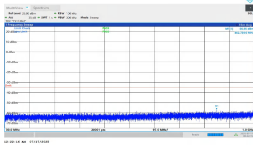
NTNV-n7-PC2-15-5-M-DFT-BPSK-Inner_1RB_Left-30-1000-PASS
