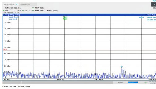
NTNV-n7-PC2-15-10-H-DFT-BPSK-Inner_1RB_Left-0.009-0.15-P ASS
