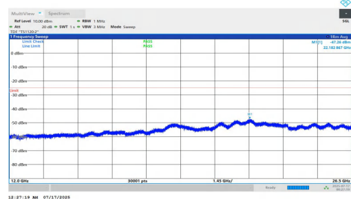
NTNV-n7-PC2-15-10-L-DFT-BPSK-Inner_1RB_Left-12000-26500-PASS
