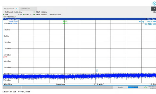
NTNV-n7-PC2-15-10-M-DFT-BPSK-Inner_1RB_Right-30-1000-P ASS
