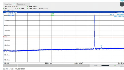
NTNV-n7-PC2-15-10-L-DFT-QPSK-Inner_1RB_Right-1000-3000-PASS
