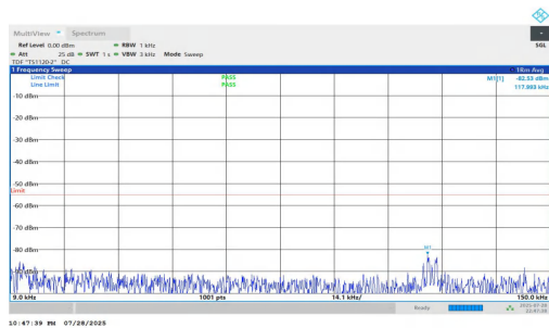
NTNV-n7-PC2-15-5-M-DFT-QPSK-Inner_1RB_Left-0.009-0.15-P ASS
