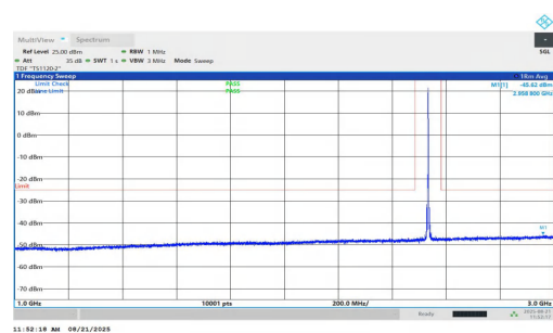
NTNV-n7-PC2-15-5-M-DFT-QPSK-Inner_1RB_Left-1000-3000-PA SS
