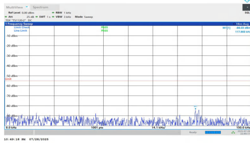
NTNV-n7-PC2-15-10-L-DFT-BPSK-Inner_1RB_Left-0.009-0.15-P ASS
