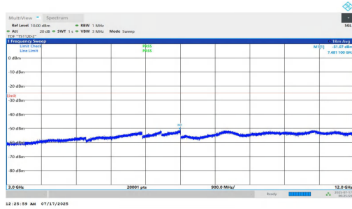
NTNV-n7-PC2-15-5-H-DFT-QPSK-Inner_1RB_Left-3000-12000-P ASS
