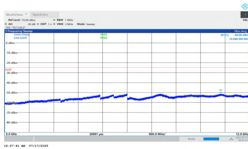
NTNV-n7-PC2-15-10-L-DFT-BPSK-Inner_1RB_Right-3000-12000 -PASS
