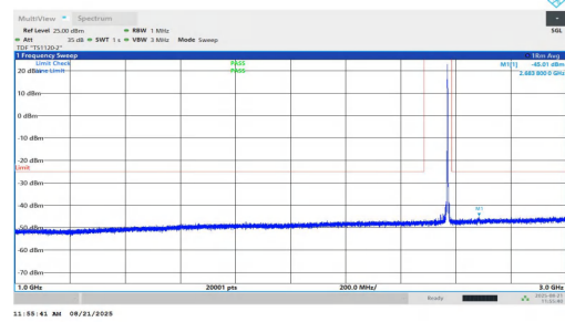
NTNV-n7-PC2-15-10-H-DFT-BPSK-Inner_1RB_Right-1000-3000-P PASS
