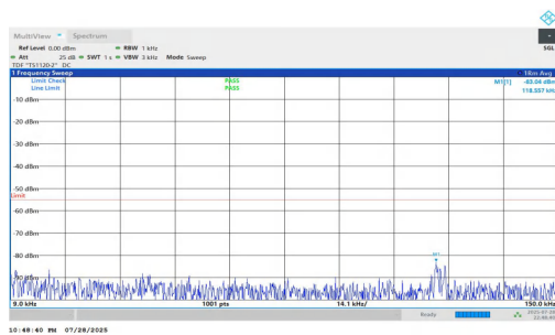
NTNV-n7-PC2-15-5-H-DFT-QPSK-Inner_1RB_Left-0.009-0.15-P ASS
