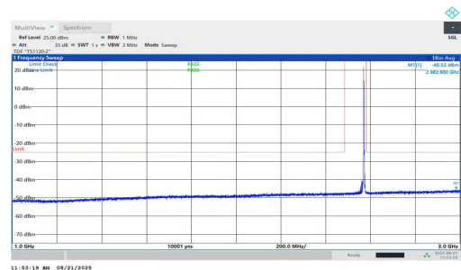
NTNV-n7-PC2-15-5-H-DFT-QPSK-Inner_1RB_Right-1000-3000-P ASS
