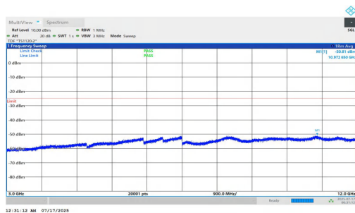
NTNV-n7-PC2-15-10-M-DFT-QPSK-Inner_1RB_Right-3000-1200 0-PASS
