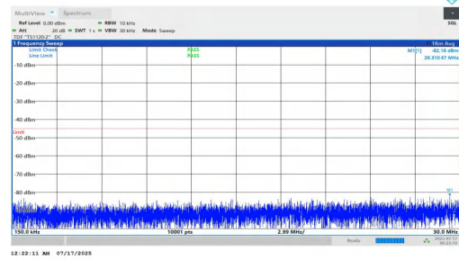
NTNV-n7-PC2-15-5-M-DFT-BPSK-Inner_1RB_Left-0.15-30-PASS
