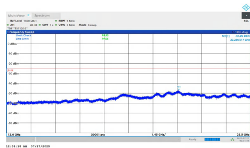
NTNV-n7-PC2-15-10-M-DFT-QPSK-Inner_1RB_Right-12000-2650 0-PASS
