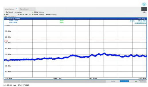
NTNV-n7-PC2-15-10-M-DFT-BPSK-Inner_1RB_Right-12000-2650 0-PASS
