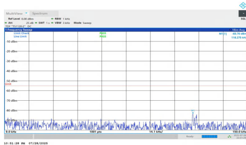
NTNV-n7-PC2-15-10-H-DFT-BPSK-Inner_1RB_Right-0.009-0.15- PASS
