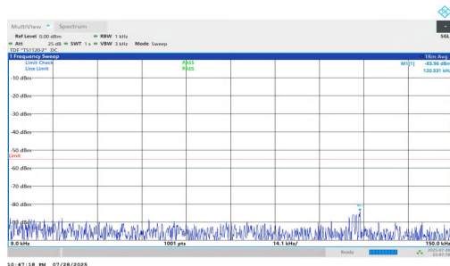
NTNV-n7-PC2-15-5-M-DFT-BPSK-Inner_1RB_Right-0.009-0.15-PASS
