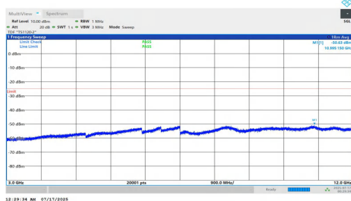
NTNV-n7-PC2-15-10-M-DFT-BPSK-Inner_1RB_Left-3000-12000-PASS
