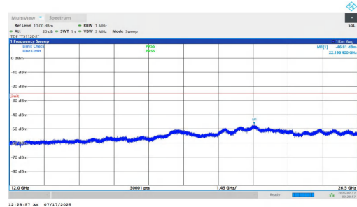
NTNV-n7-PC2-15-10-L-DFT-QPSK-Inner_1RB_Right-12000-26500-PASS
