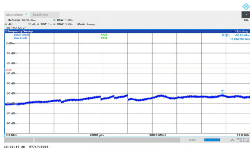
NTNV-n7-PC2-15-5-M-DFT-BPSK-Inner_1RB_Right-3000-12000 -PASS
