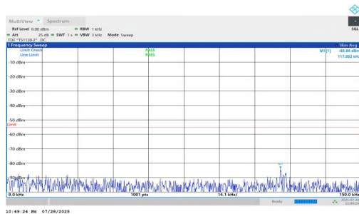
NTNV-n7-PC2-15-10-L-DFT-BPSK-Inner_1RB_Right-0.009-0.15-PASS
