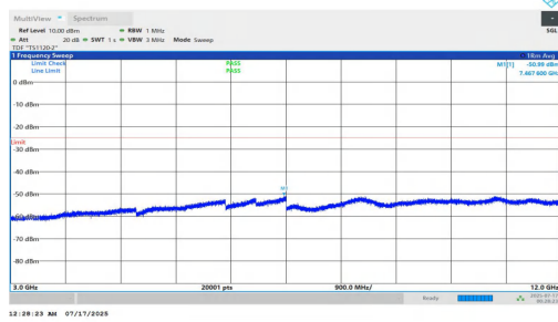
NTNV-n7-PC2-15-10-L-DFT-QPSK-Inner_1RB_Left-3000-12000-PASS
