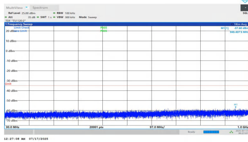
NTNV-n7-PC2-15-10-L-DFT-BPSK-Inner_1RB_Left-30-1000-PAS S
