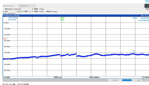
NTNV-n7-PC2-15-10-L-DFT-BPSK-Inner_1RB_Left-3000-12000-PASS
