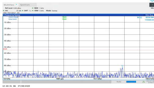
NTNV-n7-PC2-15-10-L-DFT-QPSK-Inner_1RB_Right-0.009-0.15-PASS
