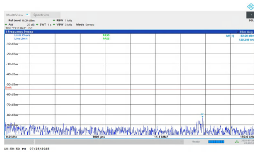
NTNV-n7-PC2-15-10-M-DFT-QPSK-Inner_1RB_Right-0.009-0.15 -PASS
