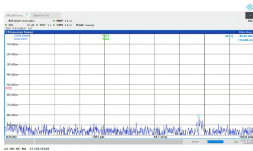
NTNV-n7-PC2-15-10-L-DFT-QPSK-Inner_1RB_Left-0.009-0.15-P ASS
