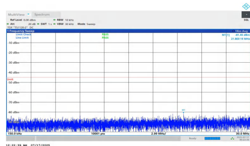
NTNV-n7-PC2-15-5-M-DFT-BPSK-Inner_1RB_Right-0.15-30-PASS
