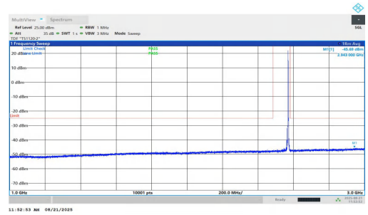
NTNV-n7-PC2-15-5-H-DFT-BPSK-Inner_1RB_Right-1000-3000-P ASS
