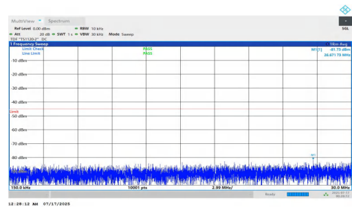
NTNV-n7-PC2-15-10-L-DFT-QPSK-Inner_1RB_Left-0.15-30-PASS
