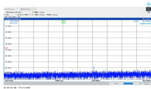
NTNV-n7-PC2-15-5-M-DFT-QPSK-Inner_1RB_Left-0.15-30-PASS
