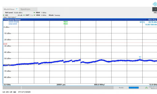
NTNV-n7-PC2-15-5-H-DFT-BPSK-Inner_1RB_Right-3000-12000- PASS
