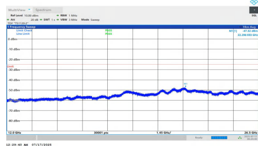
NTNV-n7-PC2-15-10-M-DFT-BPSK-Inner_1RB_Left-12000-26500-PASS
