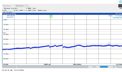
NTNV-n7-PC2-15-5-M-DFT-QPSK-Inner_1RB_Left-3000-12000-PASS
