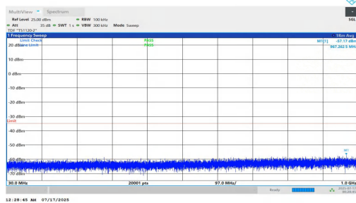
NTNV-n7-PC2-15-10-L-DFT-QPSK-Inner_1RB_Right-30-1000-PASS
