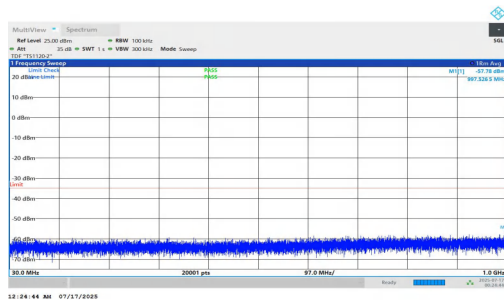
NTNV-n7-PC2-15-5-H-DFT-BPSK-Inner_1RB_Left-30-1000-PAS S
