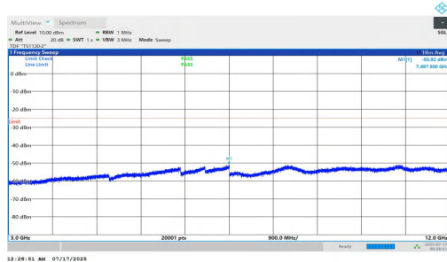
NTNV-n7-PC2-15-10-L-DFT-QPSK-Inner_1RB_Right-3000-12000-PASS
