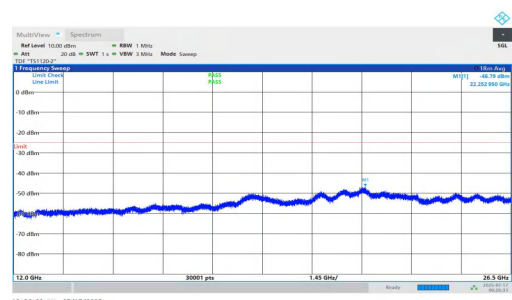
NTNV-n7-PC2-15-5-H-DFT-QPSK-Inner_1RB_Right-12000-26500 -PASS
