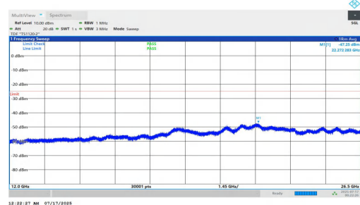
NTNV-n7-PC2-15-5-M-DFT-BPSK-Inner_1RB_Left-12000-26500-PASS
