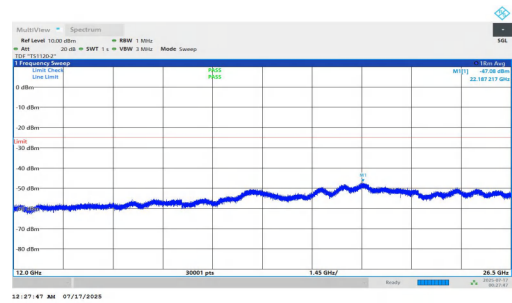
NTNV-n7-PC2-15-10-L-DFT-BPSK-Inner_1RB_Right-12000-2650 0-PASS
