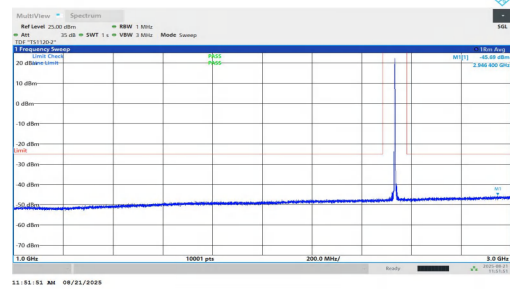
NTNV-n7-PC2-15-5-M-DFT-BPSK-Inner_1RB_Left-1000-3000-PASS
