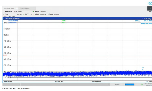
NTNV-n7-PC2-15-10-L-DFT-BPSK-Inner_1RB_Right-30-1000-PA SS
