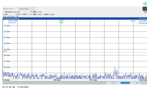
NTNV-n7-PC2-15-5-M-DFT-QPSK-Inner_1RB_Right-0.009-0.15-PASS
