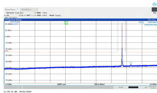
NTNV-n7-PC2-15-10-M-DFT-QPSK-Inner_1RB_Right-1000-3000- PASS
