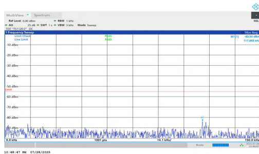
NTNV-n7-PC2-15-5-H-DFT-QPSK-Inner_1RB_Right-0.009-0.15- PASS
