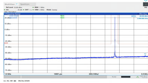
NTNV-n7-PC2-15-5-M-DFT-BPSK-Inner_1RB_Right-1000-3000-P ASS
