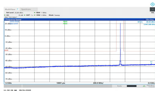
NTNV-n7-PC2-15-5-M-DFT-QPSK-Inner_1RB_Right-1000-3000-PASS
