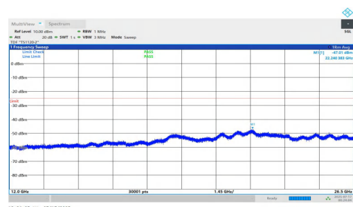
NTNV-n7-PC2-15-5-M-DFT-QPSK-Inner_1RB_Right-12000-26500-PASS
