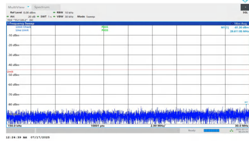
NTNV-n7-PC2-15-5-H-DFT-BPSK-Inner_1RB_Left-0.15-30-PASS
