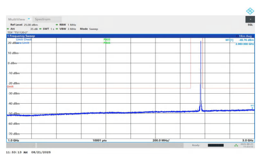
NTNV-n7-PC2-15-5-H-DFT-QPSK-Inner_1RB_Left-1000-3000-PA SS
