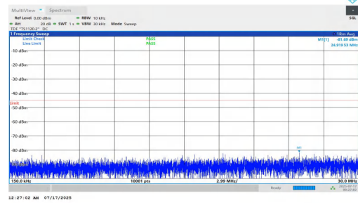
NTNV-n7-PC2-15-10-L-DFT-BPSK-Inner_1RB_Left-0.15-30-PASS
