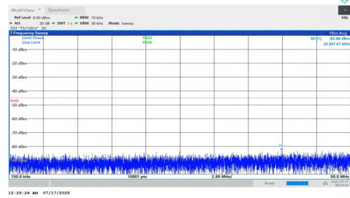
NTNV-n7-PC2-15-10-M-DFT-BPSK-Inner_1RB_Left-0.15-30-PASS
