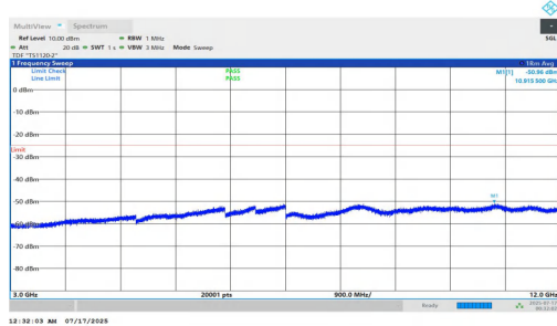
NTNV-n7-PC2-15-10-H-DFT-BPSK-Inner_1RB_Left-3000-12000- PASS
