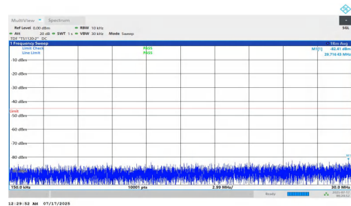
NTNV-n7-PC2-15-10-M-DFT-BPSK-Inner_1RB_Right-0.15-30-PASS
