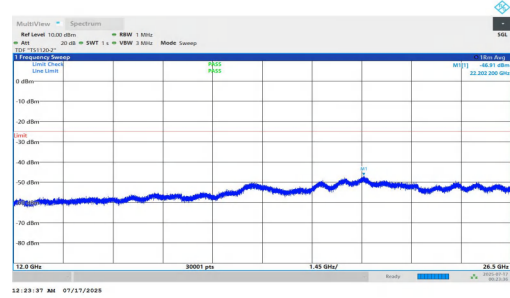
NTNV-n7-PC2-15-5-M-DFT-QPSK-Inner_1RB_Left-12000-26500-PASS
