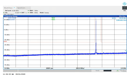
NTNV-n7-PC2-15-10-L-DFT-QPSK-Inner_1RB_Left-1000-3000-PA SS
