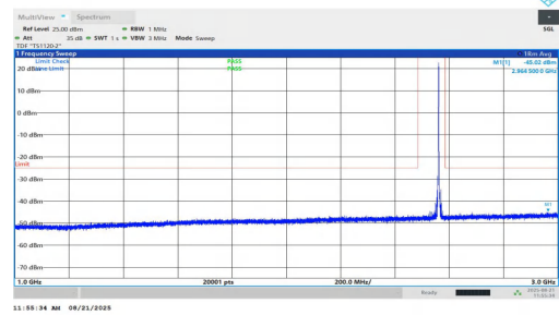
NTNV-n7-PC2-15-10-H-DFT-BPSK-Inner_1RB_Left-1000-3000-P ASS
