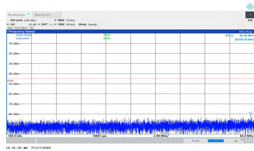
NTNV-n7-PC2-15-10-M-DFT-QPSK-Inner_1RB_Right-0.15-30-PA SS
