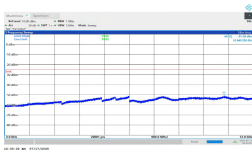
NTNV-n7-PC2-15-10-M-DFT-BPSK-Inner_1RB_Right-3000-1200 0-PASS
