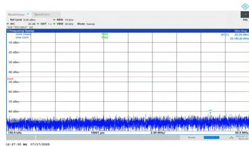
NTNV-n7-PC2-15-10-L-DFT-BPSK-Inner_1RB_Right-0.15-30-PASS
