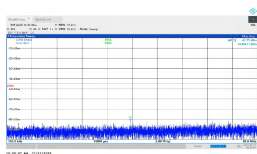
NTNV-n7-PC2-15-5-H-DFT-BPSK-Inner_1RB_Right-0.15-30-PAS S
