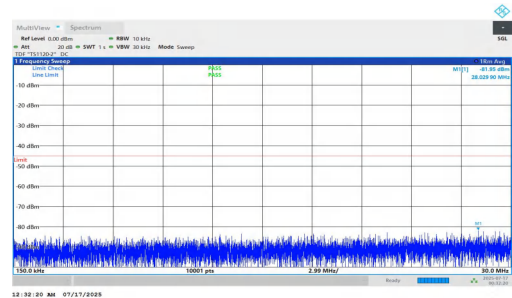
NTNV-n7-PC2-15-10-H-DFT-BPSK-Inner_1RB_Right-0.15-30-PAS S
