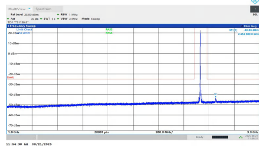
NTNV-n7-PC2-15-10-M-DFT-BPSK-Inner_1RB_Left-1000-3000-PASS
