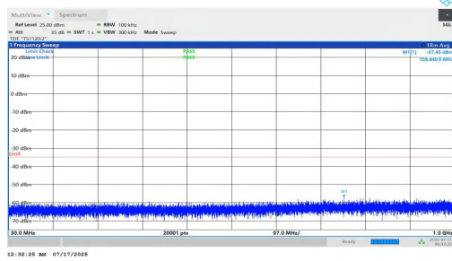
NTNV-n7-PC2-15-10-H-DFT-BPSK-Inner_1RB_Right-30-1000-P ASS
