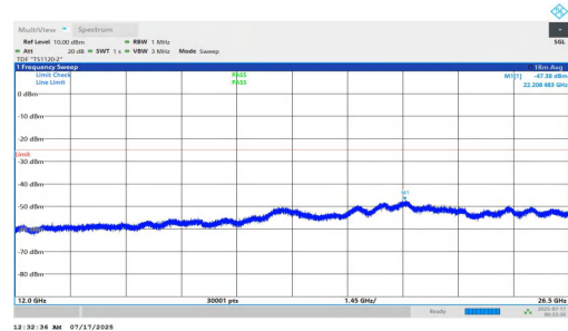
NTNV-n7-PC2-15-10-H-DFT-BPSK-Inner_1RB_Right-12000-2650 0-PASS
