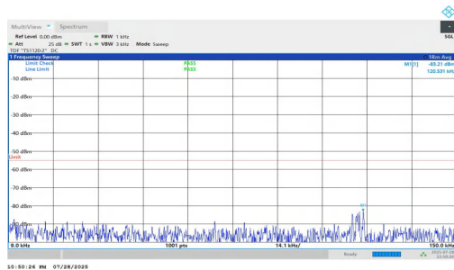
NTNV-n7-PC2-15-10-M-DFT-BPSK-Inner_1RB_Right-0.009-0.15-PASS
