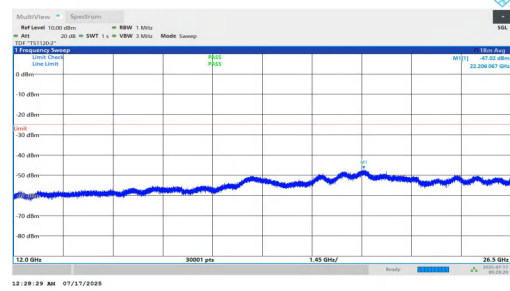
NTNV-n7-PC2-15-10-L-DFT-QPSK-Inner_1RB_Left-12000-26500-PASS
