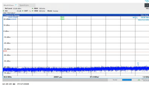
NTNV-n7-PC2-15-10-M-DFT-BPSK-Inner_1RB_Left-30-1000-PASS
