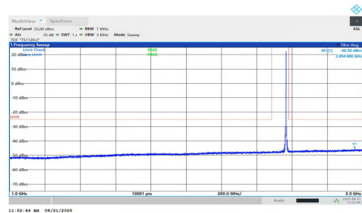
NTNV-n7-PC2-15-5-H-DFT-BPSK-Inner_1RB_Left-1000-3000-PA SS
