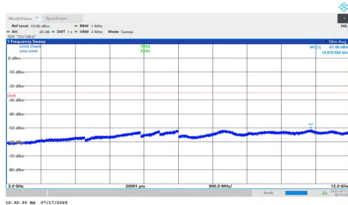
NTNV-n7-PC2-15-10-H-DFT-BPSK-Inner_1RB_Right-3000-1200 0-PASS
