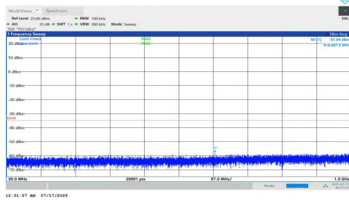
NTNV-n7-PC2-15-10-H-DFT-BPSK-Inner_1RB_Left-30-1000-PASS
