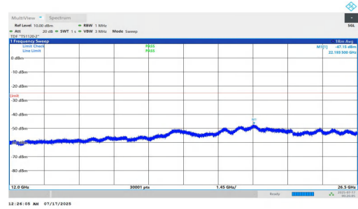
NTNV-n7-PC2-15-5-H-DFT-QPSK-Inner_1RB_Left-12000-26500-P PASS
