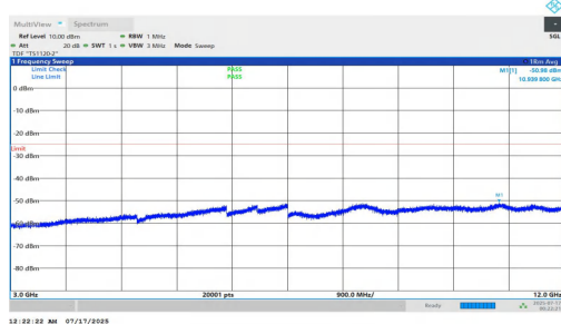
NTNV-n7-PC2-15-5-M-DFT-BPSK-Inner_1RB_Left-3000-12000-PASS
