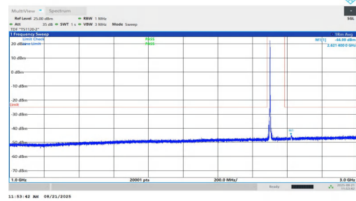
NTNV-n7-PC2-15-10-L-DFT-BPSK-Inner_1RB_Left-1000-3000-PASS
