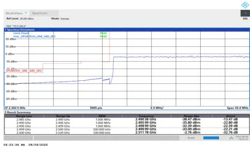
NTNV-n7-PC2-15-30-L-DFT-QPSK-Outer Full-PASS
