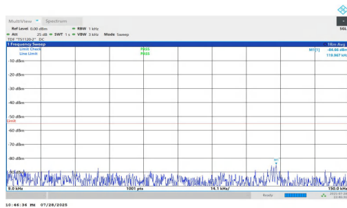
NTNV-n7-PC2-15-5-L-DFT-QPSK-Inner_1RB_Left-0.009-0.15-PA SS
