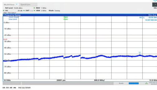
NTNV-n7-PC3-15-50-H-DFT-QPSK-Inner_1RB_Left-3000-12000-PASS
