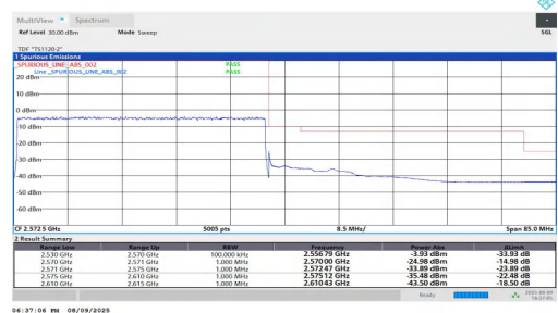
NTNV-n7-PC2-15-40-H-DFT-QPSK-Outer_Full-PASS
