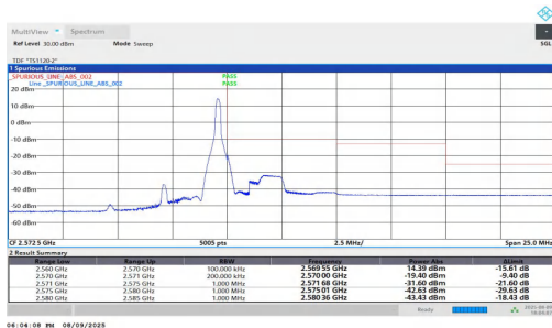
NTNV-n7-PC2-15-10-H-DFT-BPSK-Edge_1RB_Right-PASS
