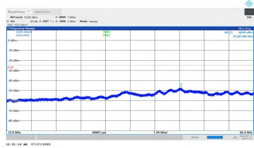
NTNV-n7-PC2-15-5-L-DFT-QPSK-Inner_1RB_Left-12000-26500-P ASS
