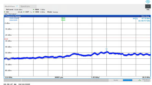
NTNV-n7-PC3-15-50-H-DFT-BPSK-Inner_1RB_Left-12000-26500- PASS
