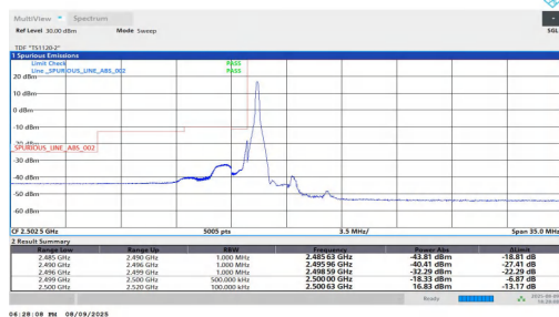
NTNV-n7-PC2-15-35-L-DFT-BPSK-Edge_1RB_Left-PASS
