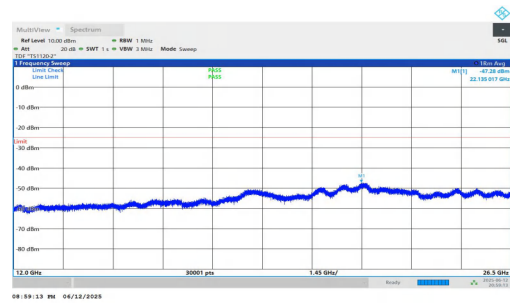
NTNV-n7-PC3-15-50-H-DFT-BPSK-Inner_1RB_Right-12000-2650 0-PASS
