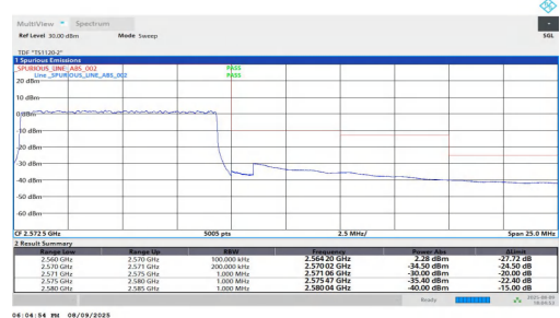
NTNV-n7-PC2-15-10-H-DFT-QPSK-Outer_Full-PASS
