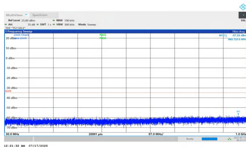
NTNV-n7-PC2-15-5-L-DFT-QPSK-Inner_1RB_Right-30-1000-PA SS
