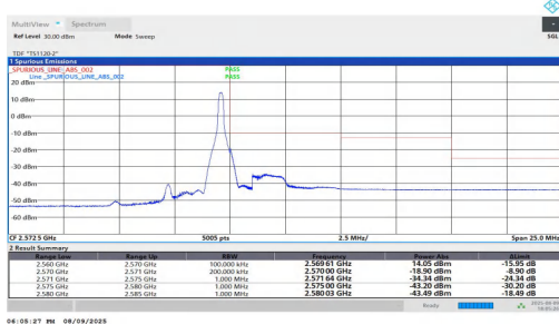
NTNV-n7-PC2-15-10-H-DFT-QPSK-Edge_1RB_Right-PASS
