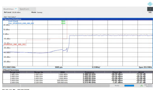
NTNV-n7-PC2-15-30-L-DFT-BPSK-Outer Full-PASS
