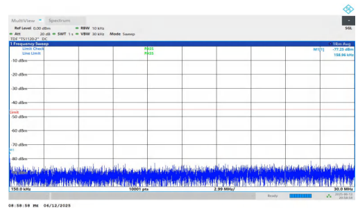
NTNV-n7-PC3-15-50-H-DFT-BPSK-Inner_1RB_Right-0.15-30-PAS S
