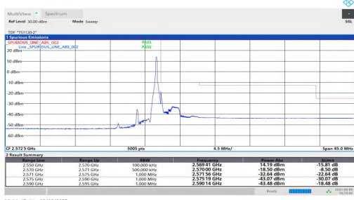
NTNV-n7-PC2-15-20-H-DFT-BPSK-Edge_1RB_Right-PASS
