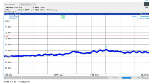
NTNV-n7-PC3-15-50-H-DFT-QPSK-Inner_1RB_Left-12000-26500-PASS
