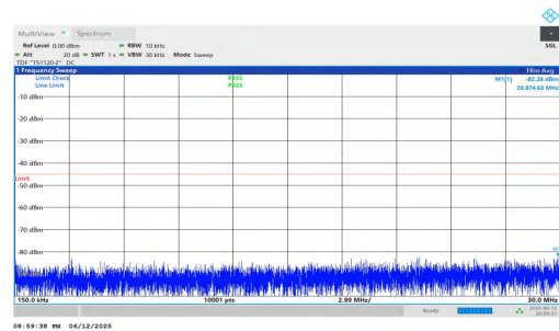
NTNV-n7-PC3-15-50-H-DFT-QPSK-Inner_1RB_Left-0.15-30-PAS S
