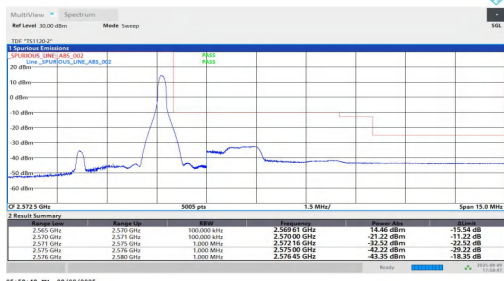
NTNV-n7-PC2-15-5-H-DFT-BPSK-Edge 1RB Right-PASS
