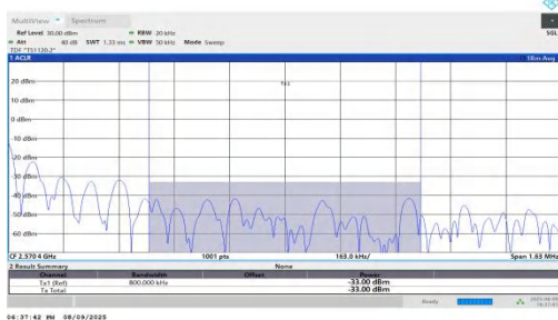
NTNV-n7-PC2-15-40-H-DFT-QPSK-Edge_1RB_Right-PASS
