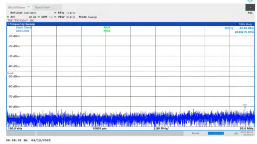
NTNV-n7-PC3-15-50-H-DFT-BPSK-Inner_1RB_Left-0.15-30-PASS
