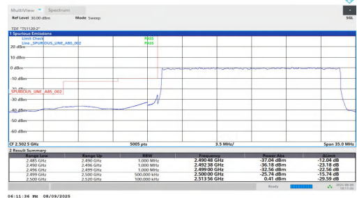
NTNV-n7-PC2-15-20-L-DFT-BPSK-Outer_Full-PASS
