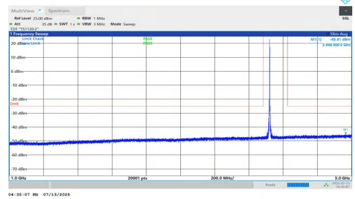
NTNV-n7-PC3-15-50-H-DFT-BPSK-Inner_1RB_Left-1000-3000-P ASS
