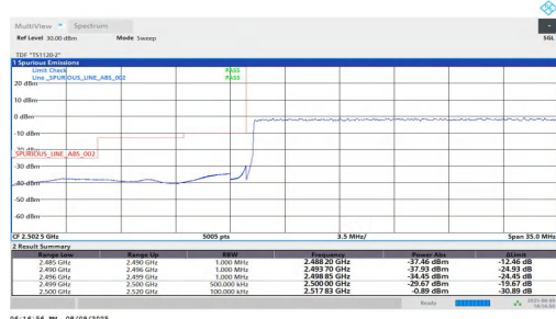
NTNV-n7-PC2-15-25-L-DFT-BPSK-Outer Full-PASS
