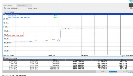
NTNV-n7-PC2-15-25-L-DFT-QPSK-Outer Full-PASS
