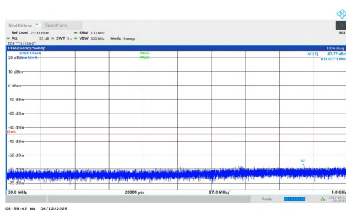
NTNV-n7-PC3-15-50-H-DFT-QPSK-Inner_1RB_Left-30-1000-PA SS
