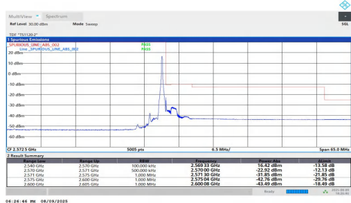
NTNV-n7-PC2-15-30-H-DFT-QPSK-Edge_1RB_Right-PASS
