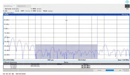
NTNV-n7-PC2-15-40-H-DFT-BPSK-Edge_1RB_Right-PASS
