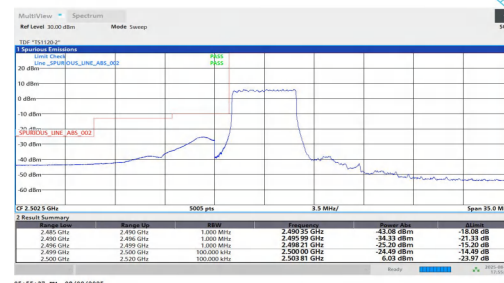
NTNV-n7-PC2-15-5-L-DFT-BPSK-Outer Full-PASS
