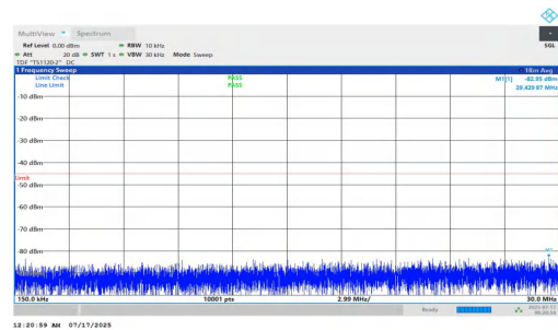
NTNV-n7-PC2-15-5-L-DFT-QPSK-Inner_1RB_Left-0.15-30-PASS
