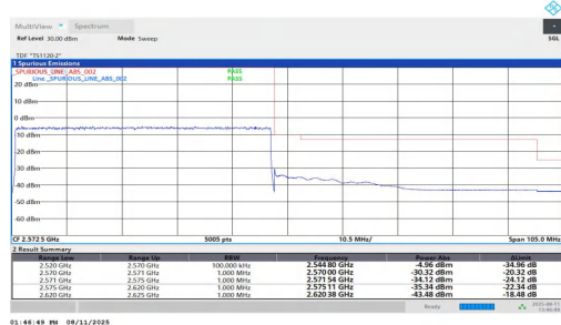
NTNV-n7-PC2-15-50-H-DFT-QPSK-Outer_Full-PASS
