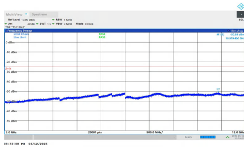
NTNV-n7-PC3-15-50-H-DFT-BPSK-Inner_1RB_Right-3000-1200 0-PASS
