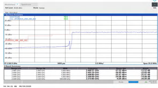
NTNV-n7-PC2-15-40-L-DFT-QPSK-Outer_Full-PASS
