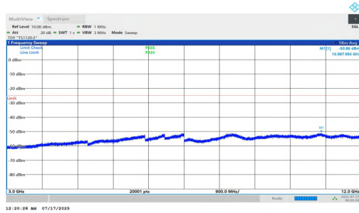
NTNV-n7-PC2-15-5-L-DFT-BPSK-Inner_1RB_Right-3000-12000- PASS
