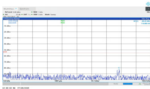
NTNV-n7-PC2-15-5-L-DFT-QPSK-Inner_1RB_Right-0.009-0.15-P ASS
