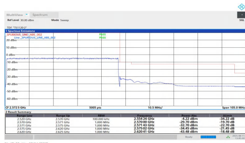
NTNV-n7-PC2-15-50-H-DFT-BPSK-Outer Full-PASS
