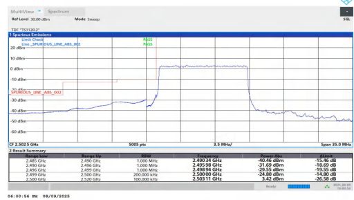
NTNV-n7-PC2-15-10-L-DFT-BPSK-Outer_Full-PASS
