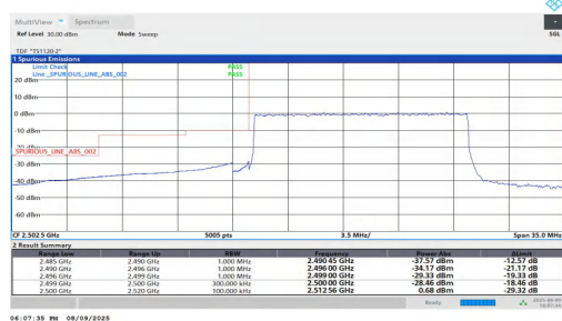
NTNV-n7-PC2-15-15-L-DFT-QPSK-Outer Full-PASS
