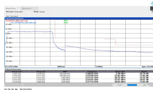
NTNV-n7-PC2-15-5-H-DFT-QPSK-Outer Full-PASS
