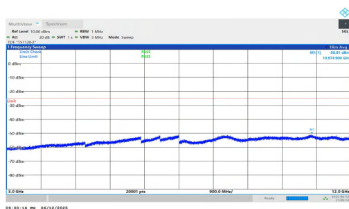
NTNV-n7-PC3-15-50-H-DFT-QPSK-Inner_1RB_Right-3000-12000-PASS
