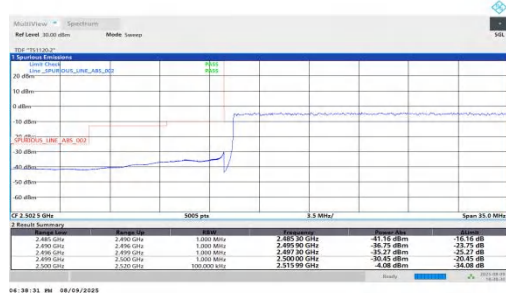
NTNV-n7-PC2-15-50-L-DFT-BPSK-Outer Full-PASS
