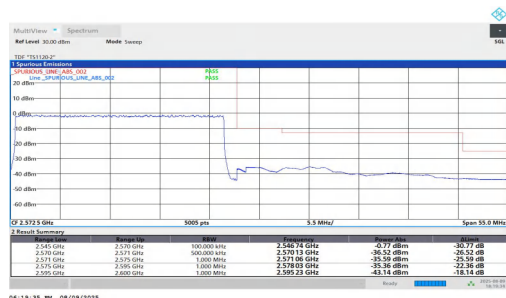
NTNV-n7-PC2-15-25-H-DFT-BPSK-Outer Full-PASS
