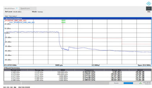
NTNV-n7-PC2-15-10-H-DFT-BPSK-Outer_Full-PASS
