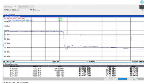
NTNV-n7-PC2-15-25-H-DFT-QPSK-Outer Full-PASS
