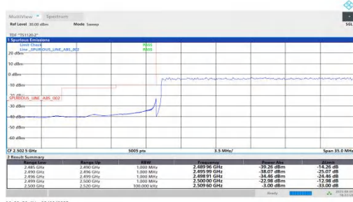
NTNV-n7-PC2-15-40-L-DFT-BPSK-Outer_Full-PASS
