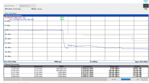
NTNV-n7-PC2-15-20-H-DFT-BPSK-Outer_Full-PASS
