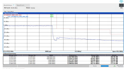
NTNV-n7-PC2-15-20-H-DFT-QPSK-Outer_Full-PASS
