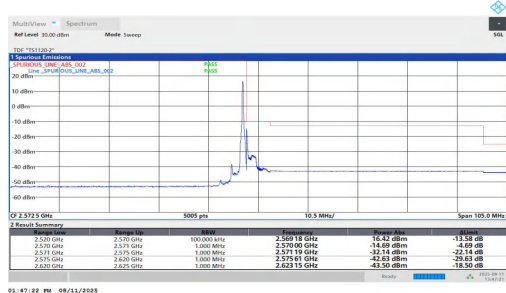
NTNV-n7-PC2-15-50-H-DFT-QPSK-Edge_1RB_Right-PASS
