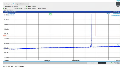
NTNV-n7-PC2-15-5-L-DFT-BPSK-Inner_1RB_Right-1000-3000-PA SS
