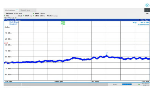
NTNV-n7-PC2-15-5-L-DFT-QPSK-Inner_1RB_Right-12000-26500- PASS
