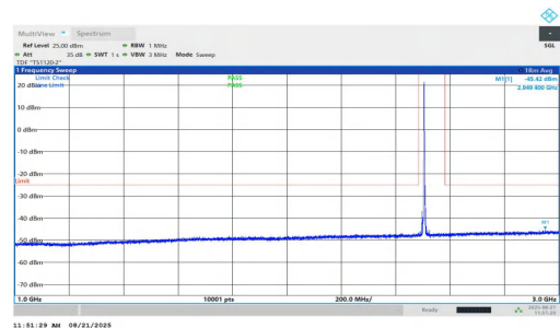
NTNV-n7-PC2-15-5-L-DFT-QPSK-Inner_1RB_Right-1000-3000-P ASS
