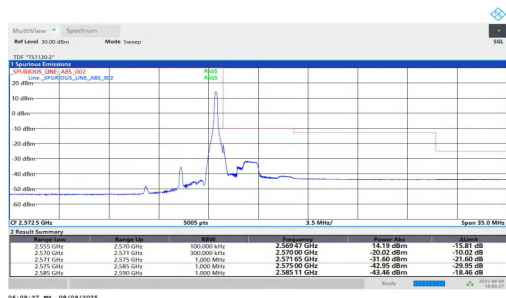
NTNV-n7-PC2-15-15-H-DFT-BPSK-Edge 1RB Right-PASS
