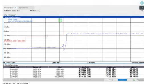
NTNV-n7-PC2-15-50-L-DFT-QPSK-Outer Full-PASS
