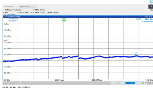
NTNV-n7-PC3-15-50-H-DFT-BPSK-Inner_1RB_Left-3000-12000- PASS
