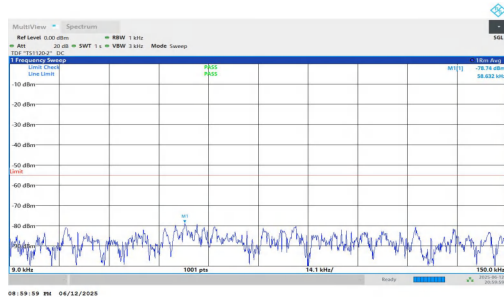
NTNV-n7-PC3-15-50-H-DFT-QPSK-Inner_1RB_Right-0.009-0.15-PASS
