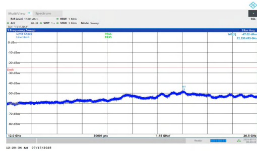
NTNV-n7-PC2-15-5-L-DFT-BPSK-Inner_1RB_Right-12000-26500- PASS
