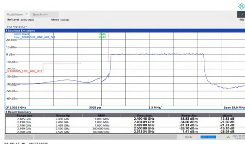
NTNV-n7-PC2-15-15-L-DFT-BPSK-Outer Full-PASS
