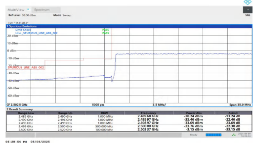
NTNV-n7-PC2-15-35-L-DFT-QPSK-Outer_Full-PASS
