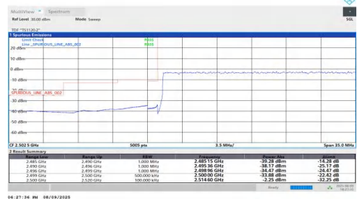
NTNV-n7-PC2-15-35-L-DFT-BPSK-Outer_Full-PASS
