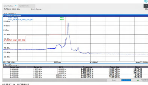
NTNV-n7-PC2-15-35-L-DFT-QPSK-Edge_1RB_Left-PASS
