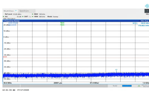
NTNV-n7-PC2-15-5-L-DFT-QPSK-Inner_1RB_Left-30-1000-PAS S
