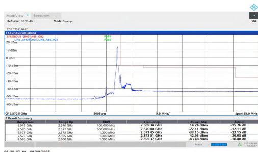
NTNV-n7-PC2-15-25-H-DFT-BPSK-Edge 1RB Right-PASS
