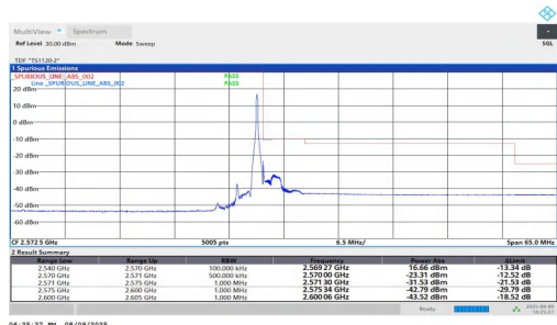
NTNV-n7-PC2-15-30-H-DFT-BPSK-Edge 1RB Right-PASS
