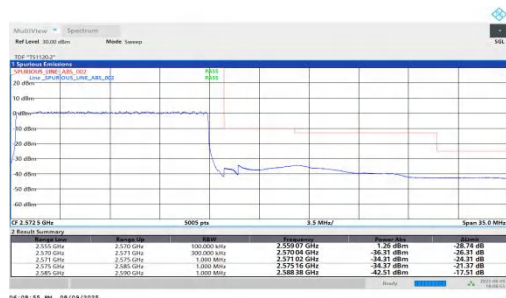
NTNV-n7-PC2-15-15-H-DFT-BPSK-Outer Full-PASS
