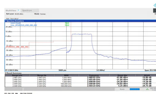
NTNV-n7-PC2-15-5-L-DFT-QPSK-Outer Full-PASS
