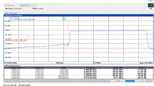
NTNV-n7-PC2-15-20-L-DFT-QPSK-Outer_Full-PASS
