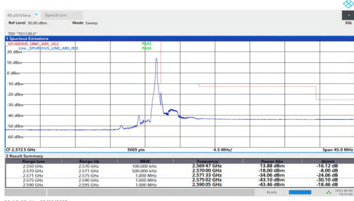
NTNV-n7-PC2-15-20-H-DFT-QPSK-Edge_1RB_Right-PASS
