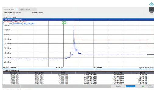
NTNV-n7-PC2-15-50-H-DFT-BPSK-Edge 1RB Right-PASS
