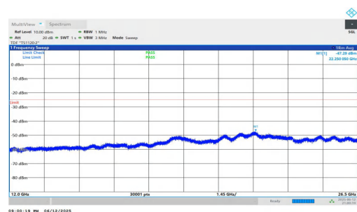
NTNV-n7-PC3-15-50-H-DFT-QPSK-Inner_1RB_Right-12000-26500-PASS
