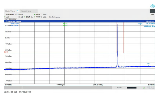
NTNV-n7-PC2-15-5-L-DFT-QPSK-Inner_1RB_Left-1000-3000-PA SS
