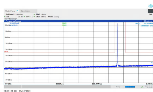
NTNV-n7-PC3-15-50-H-DFT-QPSK-Inner_1RB_Left-1000-3000-P ASS
