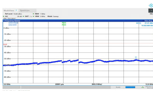
NTNV-n7-PC2-15-5-L-DFT-QPSK-Inner_1RB_Right-3000-12000- PASS
