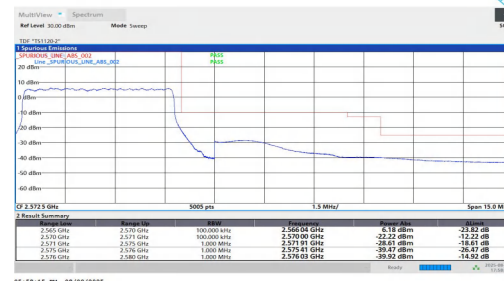
NTNV-n7-PC2-15-5-H-DFT-BPSK-Outer Full-PASS
