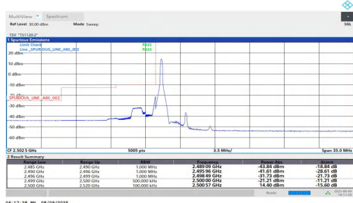
NTNV-n7-PC2-15-25-L-DFT-BPSK-Edge 1RB Left-PASS
