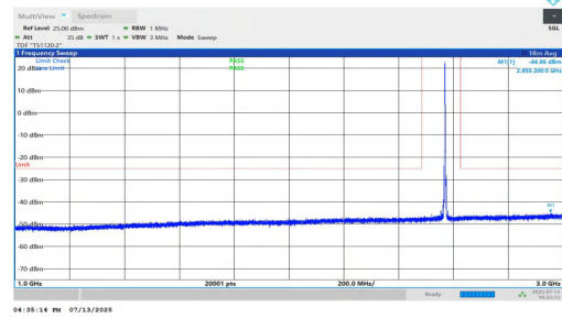
NTNV-n7-PC3-15-50-H-DFT-BPSK-Inner_1RB_Right-1000-3000-P PASS
