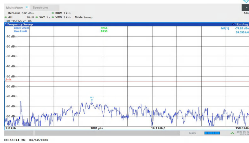
NTNV-n7-PC3-15-40-H-DFT-QPSK-Inner_1RB_Right-0.009-0.15-PASS
