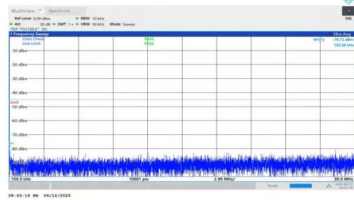
NTNV-n7-PC3-15-40-H-DFT-QPSK-Inner_1RB_Right-0.15-30-PA-SS
