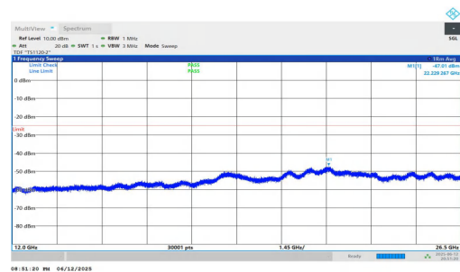
NTNV-n7-PC3-15-40-M-DFT-QPSK-Inner_1RB_Right-12000-2650 0-PASS
