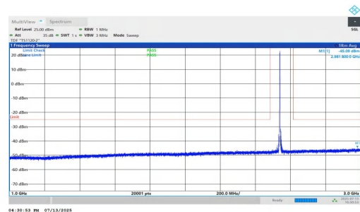
NTNV-n7-PC3-15-40-L-DFT-QPSK-Inner_1RB_Right-1000-3000-PASS
