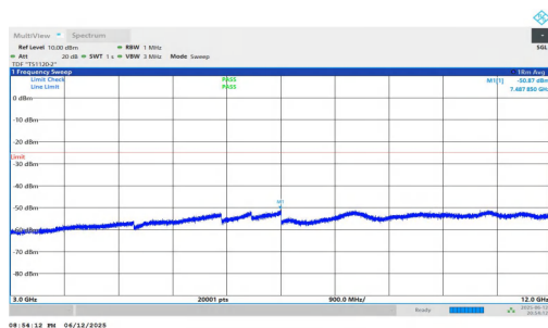
NTNV-n7-PC3-15-50-L-DFT-BPSK-Inner_1RB_Left-3000-12000-PASS
