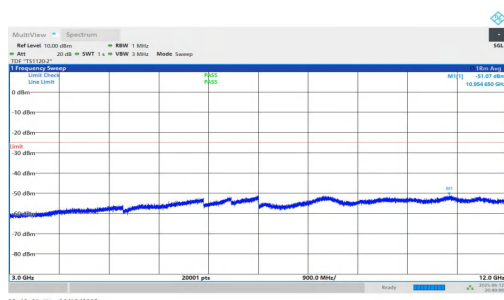
NTNV-n7-PC3-15-40-L-DFT-QPSK-Inner_1RB_Right-3000-12000-PASS
