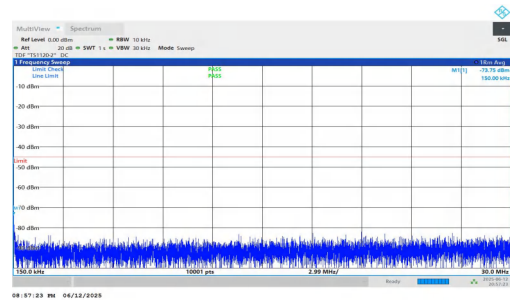
NTNV-n7-PC3-15-50-M-DFT-QPSK-Inner_1RB_Left-0.15-30-PAS S
