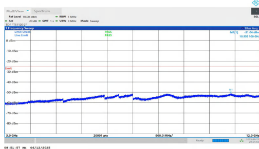
NTNV-n7-PC3-15-40-H-DFT-BPSK-Inner_1RB_Left-3000-12000-PASS
