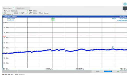
NTNV-n7-PC3-15-40-M-DFT-BPSK-Inner_1RB_Left-3000-12000-PASS
