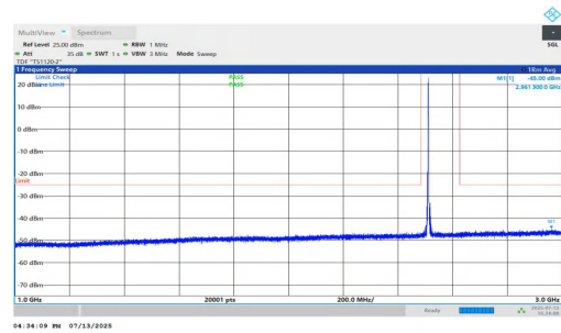
NTNV-n7-PC3-15-50-M-DFT-BPSK-Inner_1RB_Left-1000-3000-P ASS
