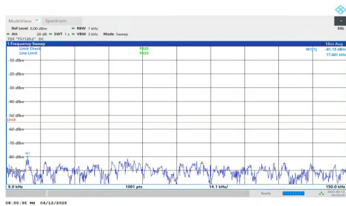
NTNV-n7-PC3-15-40-M-DFT-QPSK-Inner_1RB_Left-0.009-0.15- PASS
