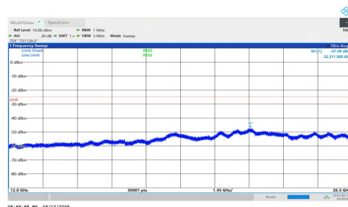
NTNV-n7-PC3-15-40-M-DFT-BPSK-Inner_1RB_Left-12000-26500-PASS
