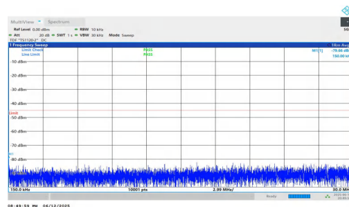
NTNV-n7-PC3-15-40-M-DFT-BPSK-Inner_1RB_Right-0.15-30-PASS
