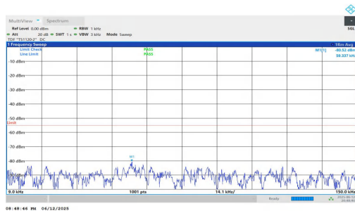
NTNV-n7-PC3-15-40-L-DFT-QPSK-Inner_1RB_Right-0.009-0.15-PASS
