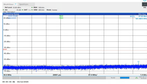
NTNV-n7-PC3-15-40-M-DFT-BPSK-Inner_1RB_Right-30-1000-P ASS
