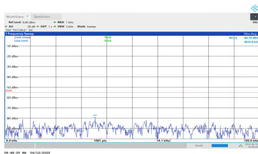
NTNV-n7-PC3-15-40-L-DFT-QPSK-Inner_1RB_Left-0.009-0.15-P ASS
