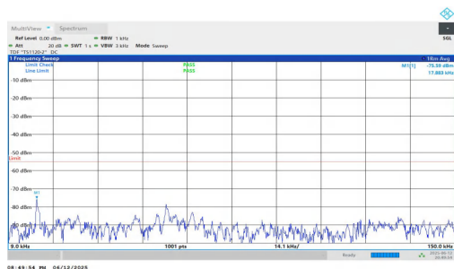
NTNV-n7-PC3-15-40-M-DFT-BPSK-Inner_1RB_Right-0.009-0.15 -PASS
