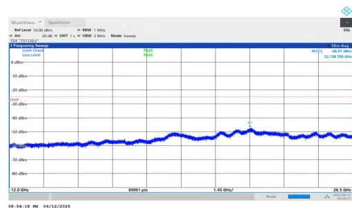
NTNV-n7-PC3-15-50-L-DFT-BPSK-Inner_1RB_Left-12000-26500-PASS
