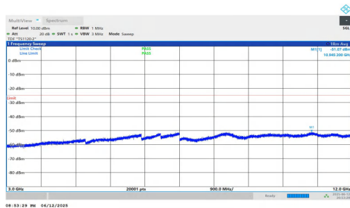
NTNV-n7-PC3-15-40-H-DFT-QPSK-Inner_1RB_Right-3000-12000-PASS
