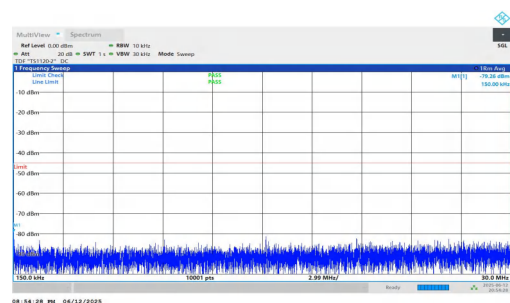
NTNV-n7-PC3-15-50-L-DFT-BPSK-Inner_1RB_Right-0.15-30-PASS S
