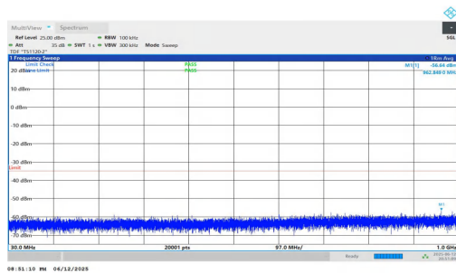
NTNV-n7-PC3-15-40-M-DFT-QPSK-Inner_1RB_Right-30-1000-P ASS
