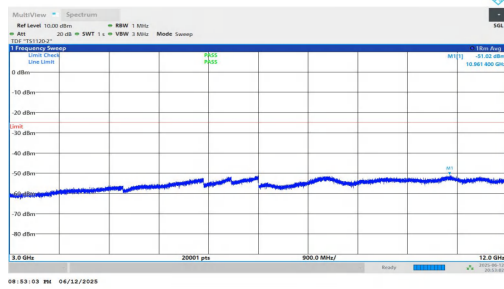
NTNV-n7-PC3-15-40-H-DFT-QPSK-Inner_1RB_Left-3000-12000-PASS
