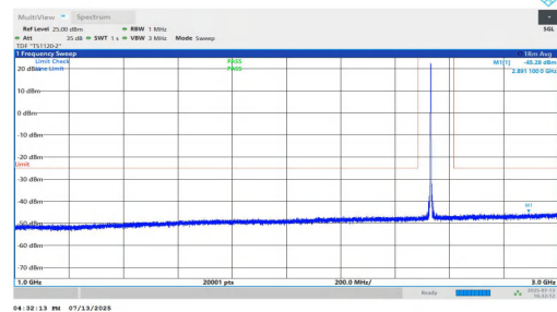
NTNV-n7-PC3-15-40-H-DFT-BPSK-Inner_1RB_Left-1000-3000-PASS
