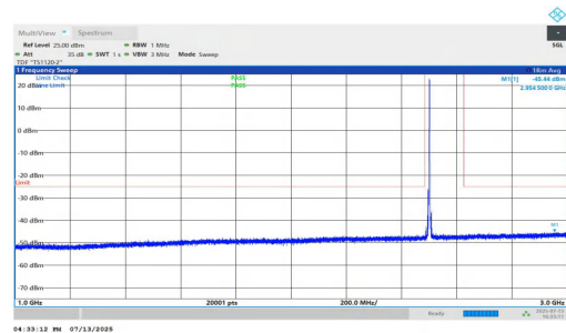
NTNV-n7-PC3-15-50-L-DFT-BPSK-Inner_1RB_Left-1000-3000-PASS SS
