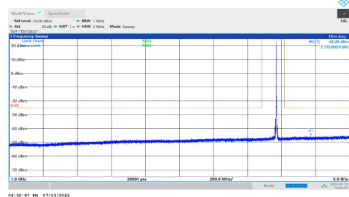
NTNV-n7-PC3-15-40-H-DFT-QPSK-Inner_1RB_Right-1000-3000-PASS
