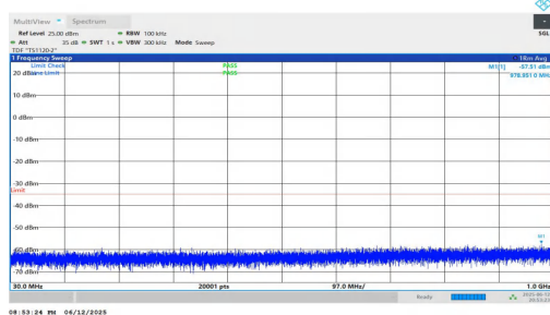
NTNV-n7-PC3-15-40-H-DFT-QPSK-Inner_1RB_Right-30-1000-PASS
