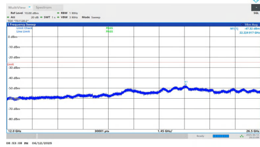
NTNV-n7-PC3-15-40-H-DFT-QPSK-Inner_1RB_Left-12000-26500-PASS
