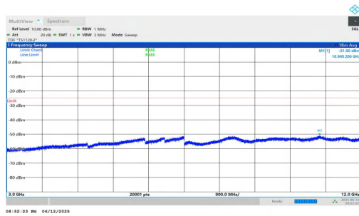
NTNV-n7-PC3-15-40-H-DFT-BPSK-Inner_1RB_Right-3000-1200 0-PASS
