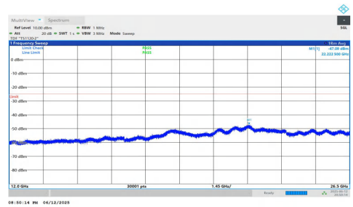
NTNV-n7-PC3-15-40-M-DFT-BPSK-Inner_1RB_Right-12000-2650 0-PASS
