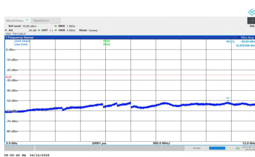
NTNV-n7-PC3-15-50-L-DFT-QPSK-Inner_1RB_Right-3000-12000-PASS
