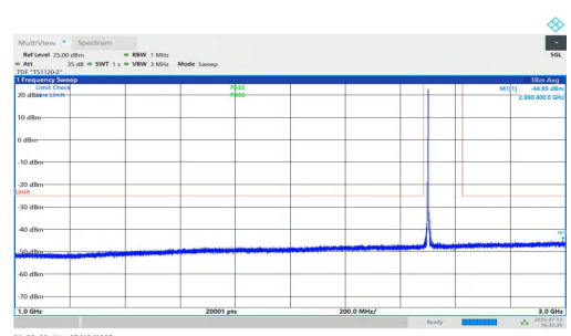
NTNV-n7-PC3-15-50-L-DFT-QPSK-Inner_1RB_Left-1000-3000-PA SS
