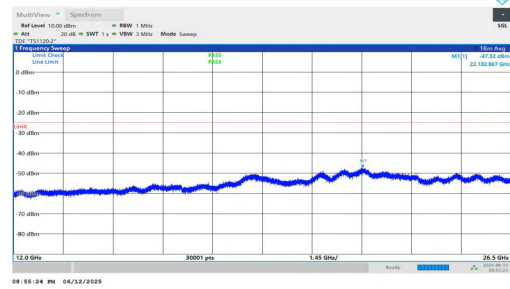
NTNV-n7-PC3-15-50-L-DFT-QPSK-Inner_1RB_Left-12000-26500-PASS
