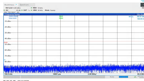
NTNV-n7-PC3-15-40-M-DFT-BPSK-Inner_1RB_Left-0.15-30-PAS S
