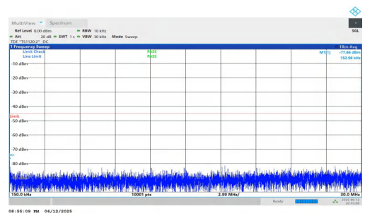
NTNV-n7-PC3-15-50-L-DFT-QPSK-Inner_1RB_Left-0.15-30-PASS
