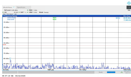
NTNV-n7-PC3-15-50-M-DFT-QPSK-Inner_1RB_Left-0.009-0.15- PASS
