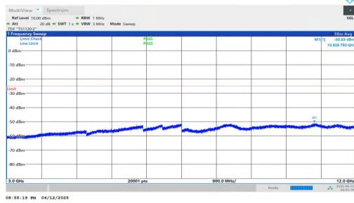
NTNV-n7-PC3-15-50-L-DFT-QPSK-Inner_1RB_Left-3000-12000-PASS
