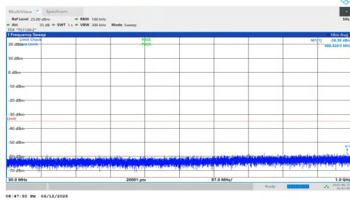
NTNV-n7-PC3-15-40-L-DFT-BPSK-Inner_1RB_Right-30-1000-PA SS
