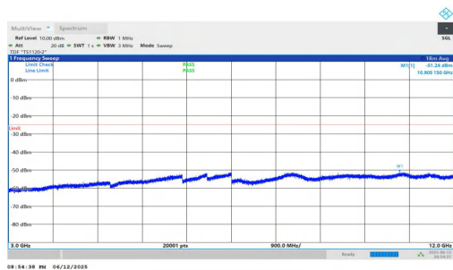
NTNV-n7-PC3-15-50-L-DFT-BPSK-Inner_1RB_Right-3000-12000 -PASS
