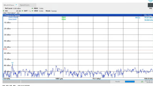
NTNV-n7-PC3-15-40-M-DFT-BPSK-Inner_1RB_Left-0.009-0.15-P ASS
