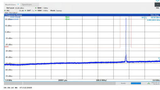
NTNV-n7-PC3-15-50-M-DFT-BPSK-Inner_1RB_Right-1000-3000-P PASS
