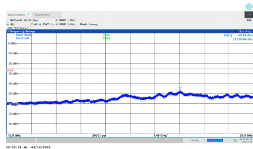
NTNV-n7-PC3-15-40-H-DFT-QPSK-Inner_1RB_Right-12000-26500-PASS
