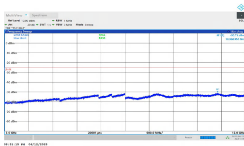
NTNV-n7-PC3-15-40-M-DFT-QPSK-Inner_1RB_Right-3000-1200 0-PASS
