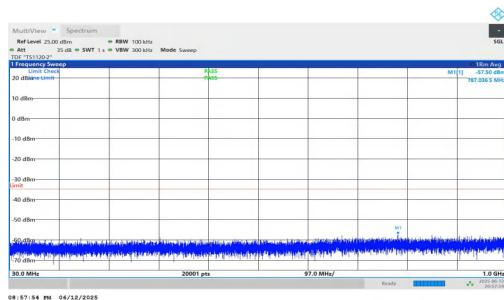
NTNV-n7-PC3-15-50-M-DFT-QPSK-Inner_1RB_Right-30-1000-P ASS
