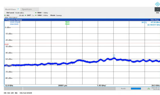
NTNV-n7-PC3-15-40-H-DFT-BPSK-Inner_1RB_Right-12000-2650 0-PASS
