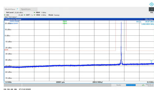
NTNV-n7-PC3-15-50-M-DFT-QPSK-Inner_1RB_Right-1000-3000- PASS
