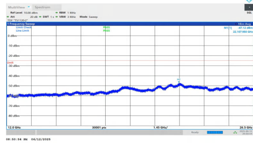
NTNV-n7-PC3-15-40-M-DFT-QPSK-Inner_1RB_Left-12000-26500 -PASS
