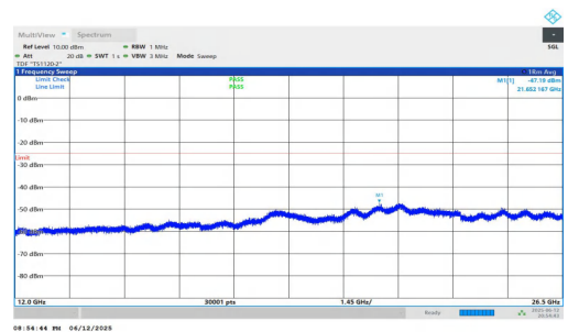
NTNV-n7-PC3-15-50-L-DFT-BPSK-Inner_1RB_Right-12000-2650 0-PASS
