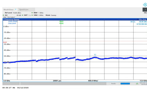
NTNV-n7-PC3-15-50-M-DFT-BPSK-Inner_1RB_Left-3000-12000- PASS
