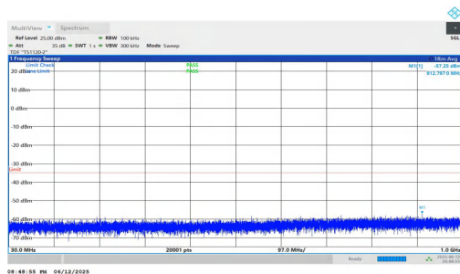
NTNV-n7-PC3-15-40-L-DFT-QPSK-Inner_1RB_Right-30-1000-PASS
