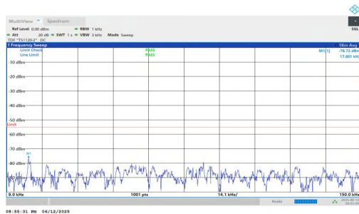
NTNV-n7-PC3-15-50-L-DFT-QPSK-Inner_1RB_Right-0.009-0.15-PASS
