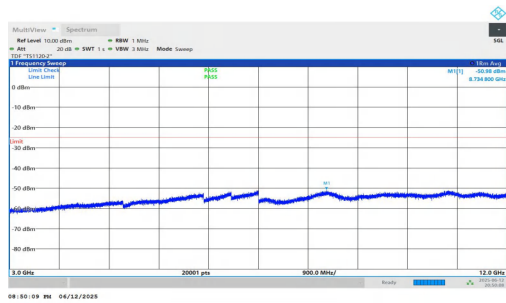
NTNV-n7-PC3-15-40-M-DFT-BPSK-Inner_1RB_Right-3000-1200 0-PASS
