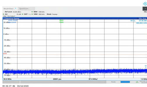
NTNV-n7-PC3-15-50-L-DFT-BPSK-Inner_1RB_Left-30-1000-PAS S
