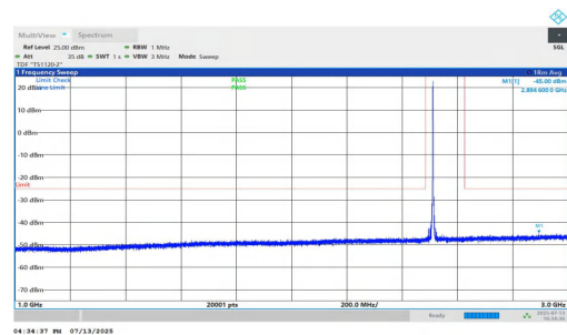
NTNV-n7-PC3-15-50-M-DFT-QPSK-Inner_1RB_Left-1000-3000-P ASS
