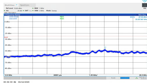
NTNV-n7-PC3-15-50-M-DFT-BPSK-Inner_1RB_Right-12000-2650 0-PASS
