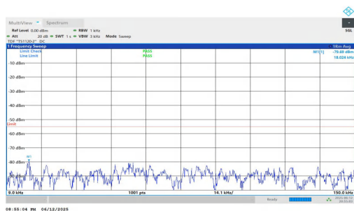
NTNV-n7-PC3-15-50-L-DFT-QPSK-Inner_1RB_Left-0.009-0.15-P ASS
