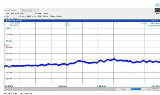
NTNV-n7-PC3-15-50-M-DFT-BPSK-Inner_1RB_Left-12000-26500- PASS
