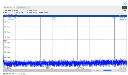
NTNV-n7-PC3-15-40-M-DFT-QPSK-Inner_1RB_Left-0.15-30-PAS S
