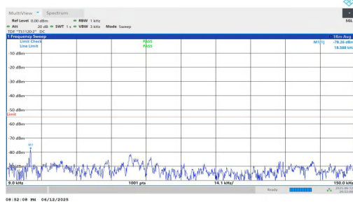
NTNV-n7-PC3-15-40-H-DFT-BPSK-Inner_1RB_Right-0.009-0.15-PASS
