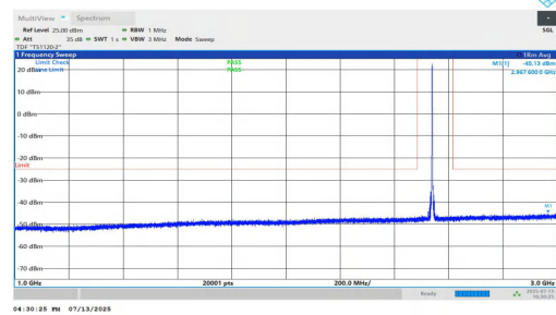
NTNV-n7-PC3-15-40-L-DFT-BPSK-Inner_1RB_Right-1000-3000-P ASS
