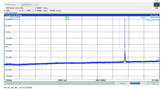
NTNV-n7-PC3-15-40-M-DFT-BPSK-Inner_1RB_Right-1000-3000-P PASS
