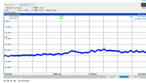
NTNV-n7-PC3-15-40-L-DFT-QPSK-Inner_1RB_Left-12000-26500-PASS
