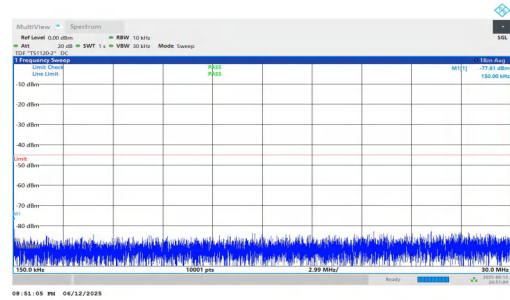
NTNV-n7-PC3-15-40-M-DFT-QPSK-Inner_1RB_Right-0.15-30-PA SS
