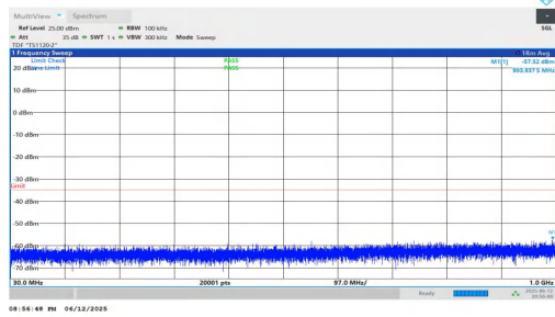
NTNV-n7-PC3-15-50-M-DFT-BPSK-Inner_1RB_Right-30-1000-P ASS
