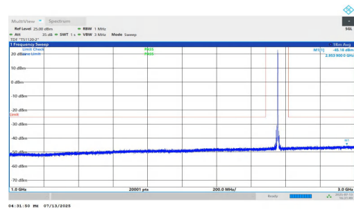
NTNV-n7-PC3-15-40-M-DFT-QPSK-Inner_1RB_Right-1000-3000- PASS
