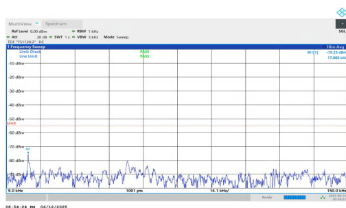
NTNV-n7-PC3-15-50-L-DFT-BPSK-Inner_1RB_Right-0.009-0.15-PASS
