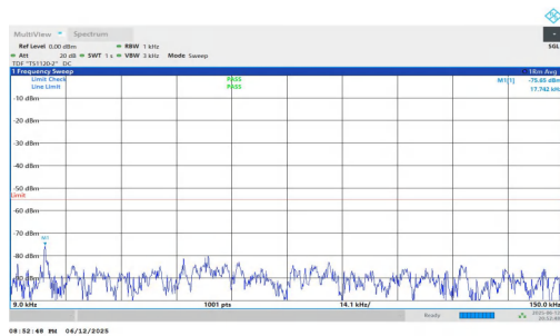
NTNV-n7-PC3-15-40-H-DFT-QPSK-Inner_1RB_Left-0.009-0.15-P ASS
