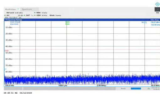
NTNV-n7-PC3-15-40-L-DFT-QPSK-Inner_1RB_Right-0.15-30-PASS
