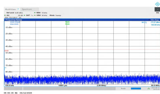
NTNV-n7-PC3-15-50-L-DFT-QPSK-Inner_1RB_Right-0.15-30-PASS
