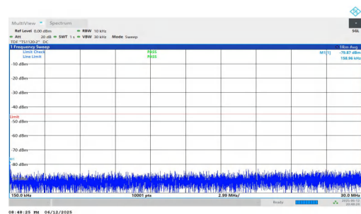
NTNV-n7-PC3-15-40-L-DFT-QPSK-Inner_1RB_Left-0.15-30-PASS
