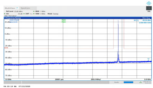
NTNV-n7-PC3-15-50-L-DFT-BPSK-Inner_1RB_Right-1000-3000-P ASS
