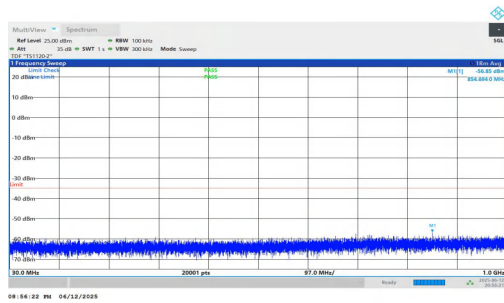
NTNV-n7-PC3-15-50-M-DFT-BPSK-Inner_1RB_Left-30-1000-PASS SS
