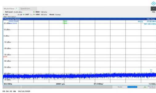
NTNV-n7-PC3-15-50-L-DFT-BPSK-Inner_1RB_Right-30-1000-PA SS
