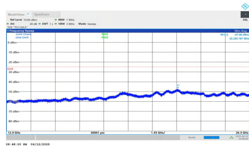
NTNV-n7-PC3-15-40-L-DFT-BPSK-Inner_1RB_Right-12000-2650 0-PASS
