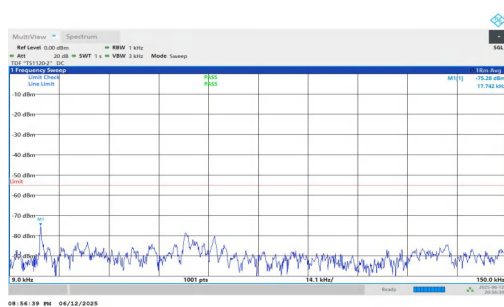
NTNV-n7-PC3-15-50-M-DFT-BPSK-Inner_1RB_Right-0.009-0.15 -PASS
