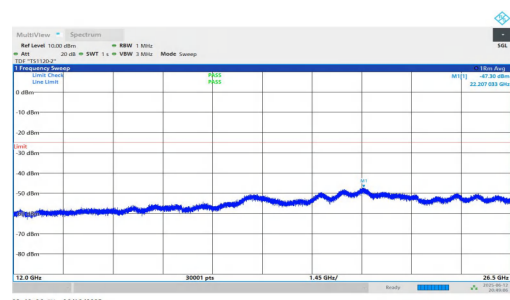
NTNV-n7-PC3-15-40-L-DFT-QPSK-Inner_1RB_Right-12000-26500-PASS
