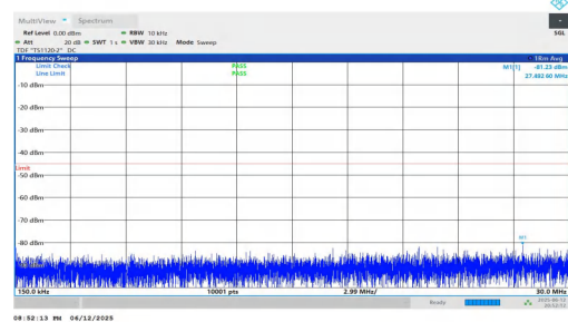
NTNV-n7-PC3-15-40-H-DFT-BPSK-Inner_1RB_Right-0.15-30-PASS
