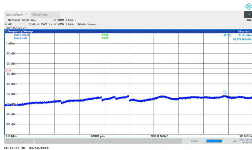
NTNV-n7-PC3-15-40-L-DFT-BPSK-Inner_1RB_Right-3000-12000 -PASS
