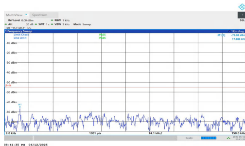
NTNV-n7-PC3-15-35-L-DFT-QPSK-Inner_1RB_Left-0.009-0.15-P ASS
