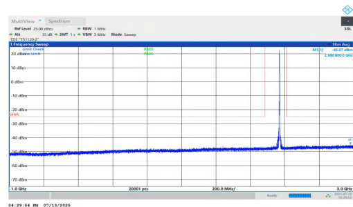
NTVN-n7-PC3-15-35-H-DFT-QPSK-Inner_1RB_Right-1000-3000-PASS
