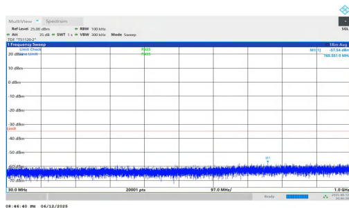
NTVN-n7-PC3-15-35-H-DFT-QPSK-Inner_1RB_Right-30-1000-PASS
