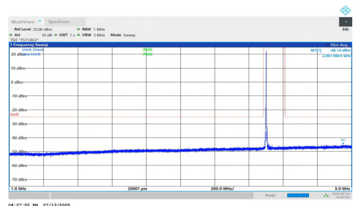
NTNV-n7-PC3-15-35-L-DFT-QPSK-Inner_1RB_Left-1000-3000-PA SS
