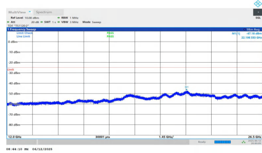
NTNV-n7-PC3-15-35-M-DFT-QPSK-Inner_1RB_Left-12000-26500 -PASS
