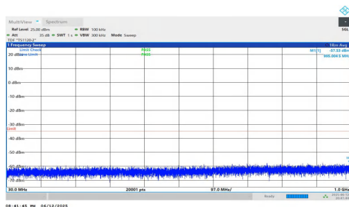
NTNV-n7-PC3-15-35-L-DFT-QPSK-Inner_1RB_Left-30-1000-PA SS
