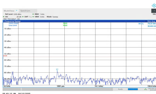
NTNV-n7-PC3-15-35-M-DFT-BPSK-Inner_1RB_Right-0.009-0.15 -PASS
