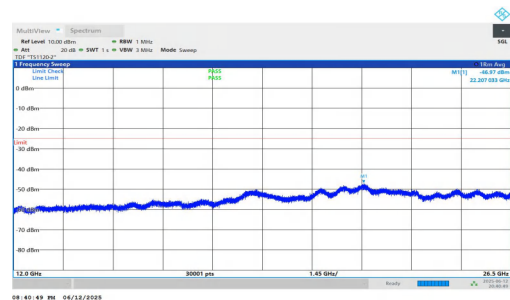
NTNV-n7-PC3-15-35-L-DFT-BPSK-Inner_1RB_Left-12000-26500- PASS
