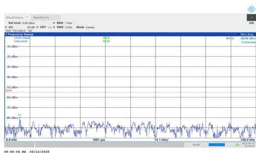
NTNV-n7-PC3-15-35-H-DFT-QPSK-Inner_1RB_Left-0.009-0.15-P ASS
