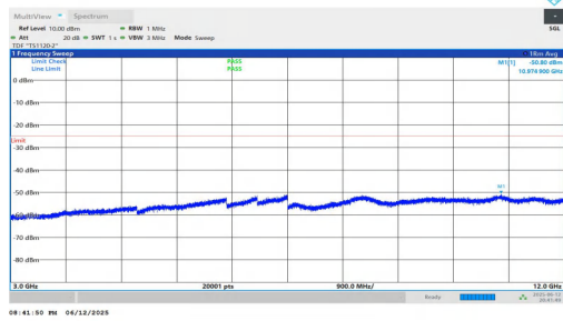
NTNV-n7-PC3-15-35-L-DFT-QPSK-Inner_1RB_Left-3000-12000-PASS
