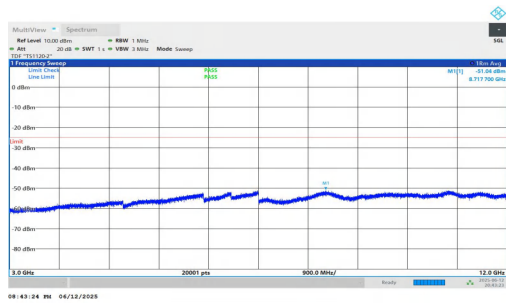
NTNV-n7-PC3-15-35-M-DFT-BPSK-Inner_1RB_Right-3000-1200 0-PASS
