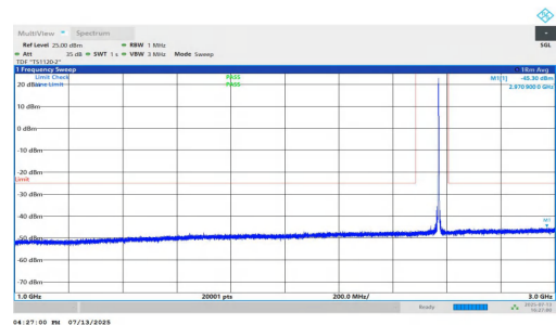
NTVN-n7-PC3-15-30-H-DFT-QPSK-Inner_1RB_Right-1000-3000- PASS
