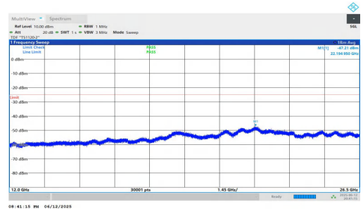
NTNV-n7-PC3-15-35-L-DFT-BPSK-Inner_1RB_Right-12000-2650 0-PASS
