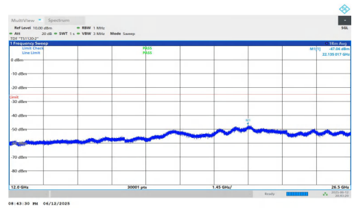
NTNV-n7-PC3-15-35-M-DFT-BPSK-Inner_1RB_Right-12000-2650 0-PASS
