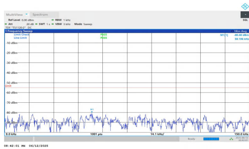
NTNV-n7-PC3-15-35-L-DFT-QPSK-Inner_1RB_Right-0.009-0.15-PASS
