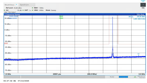
NTNV-n7-PC3-15-35-L-DFT-BPSK-Inner_1RB_Right-1000-3000-P ASS
