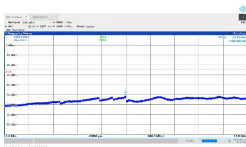
NTNV-n7-PC3-15-30-M-DFT-QPSK-Inner_1RB_Right-3000-1200 0-PASS
