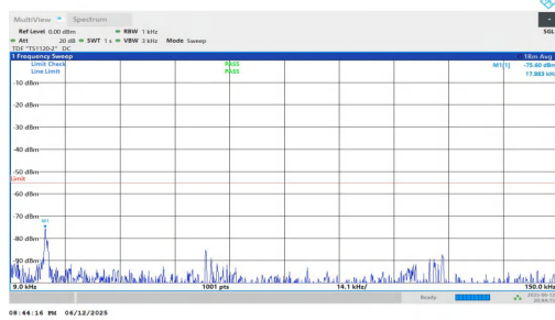
NTNV-n7-PC3-15-35-M-DFT-QPSK-Inner_1RB_Right-0.009-0.15 -PASS
