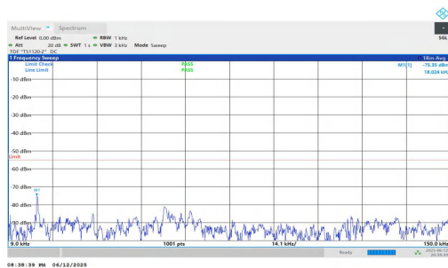
NTNV-n7-PC3-15-30-H-DFT-BPSK-Inner_1RB_Right-0.009-0.15- PASS
