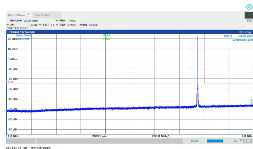
NTNV-n7-PC3-15-30-M-DFT-QPSK-Inner_1RB_Right-1000-3000- PASS
