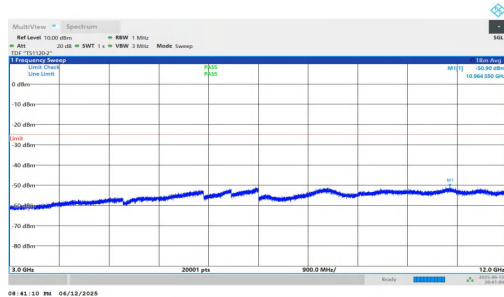
NTNV-n7-PC3-15-35-L-DFT-BPSK-Inner_1RB_Right-3000-12000 -PASS
