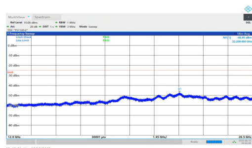
NTVN-n7-PC3-15-35-H-DFT-QPSK-Inner_1RB_Right-12000-26500-PASS
