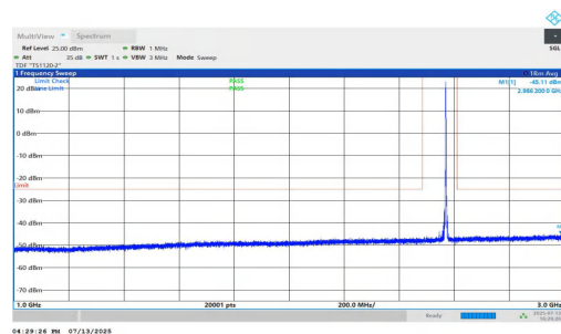
NTNV-n7-PC3-15-35-H-DFT-BPSK-Inner_1RB_Right-1000-3000-P PASS
