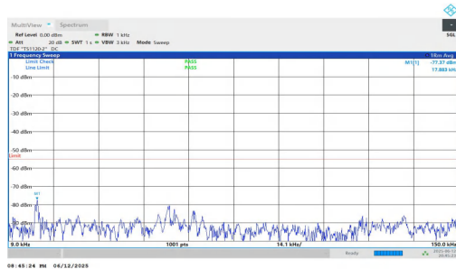
NTNV-n7-PC3-15-35-H-DFT-BPSK-Inner_1RB_Right-0.009-0.15- PASS
