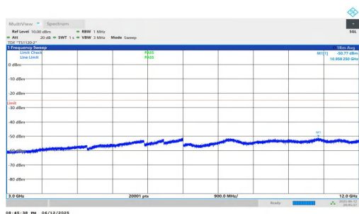
NTNV-n7-PC3-15-35-H-DFT-BPSK-Inner_1RB_Right-3000-1200 0-PASS
