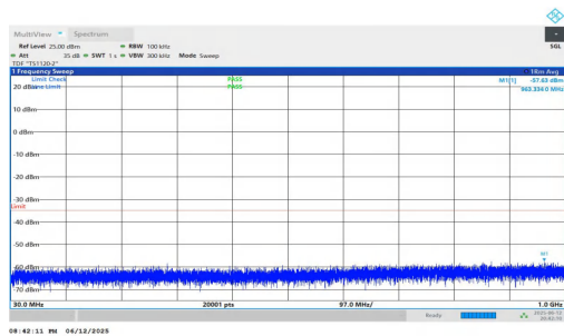
NTNV-n7-PC3-15-35-L-DFT-QPSK-Inner_1RB_Right-30-1000-PASS
