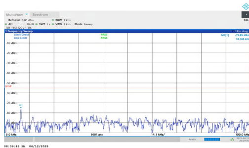
NTVN-n7-PC3-15-30-H-DFT-QPSK-Inner_1RB_Right-0.009-0.15 -PASS
