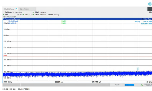
NTNV-n7-PC3-15-35-M-DFT-BPSK-Inner_1RB_Left-30-1000-PASS
