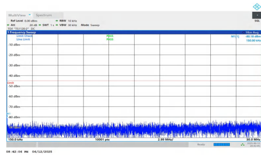
NTNV-n7-PC3-15-35-L-DFT-QPSK-Inner_1RB_Right-0.15-30-PASS
