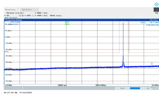
NTNV-n7-PC3-15-35-L-DFT-QPSK-Inner_1RB_Right-1000-3000-PASS
