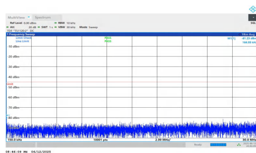
NTNV-n7-PC3-15-35-H-DFT-QPSK-Inner_1RB_Left-0.15-30-PAS S
