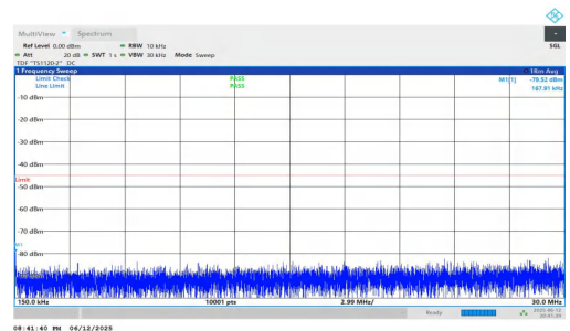
NTNV-n7-PC3-15-35-L-DFT-QPSK-Inner_1RB_Left-0.15-30-PASS
