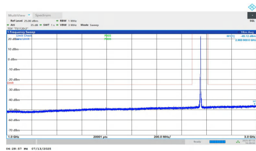
NTNV-n7-PC3-15-35-M-DFT-QPSK-Inner_1RB_Right-1000-3000- PASS
