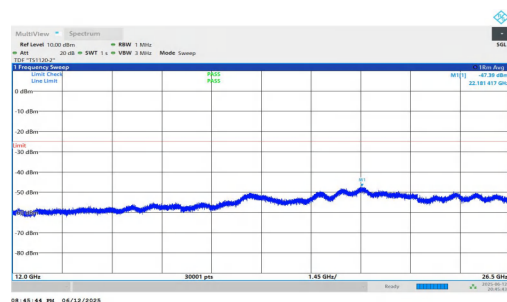
NTNV-n7-PC3-15-35-H-DFT-BPSK-Inner_1RB_Right-12000-2650 0-PASS
