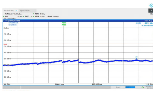
NTVN-n7-PC3-15-30-H-DFT-QPSK-Inner_1RB_Right-3000-1200 0-PASS
