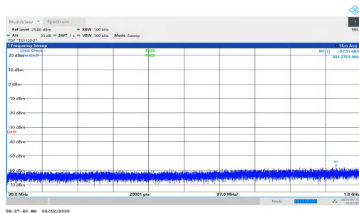
NTNV-n7-PC3-15-30-M-DFT-QPSK-Inner_1RB_Right-30-1000-P ASS
