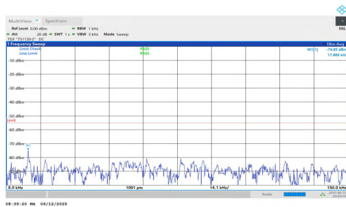
NTNV-n7-PC3-15-30-H-DFT-QPSK-Inner_1RB_Left-0.009-0.15-P ASS
