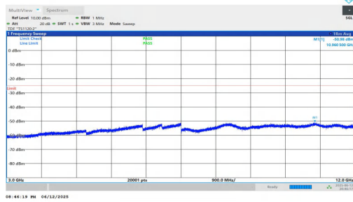
NTVN-n7-PC3-15-35-H-DFT-QPSK-Inner_1RB_Left-3000-12000-PASS
