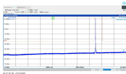
NTNV-n7-PC3-15-35-L-DFT-BPSK-Inner_1RB_Left-1000-3000-PASS
