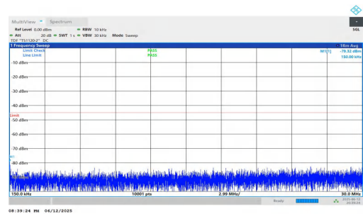
NTNV-n7-PC3-15-30-H-DFT-QPSK-Inner_1RB_Left-0.15-30-PAS S
