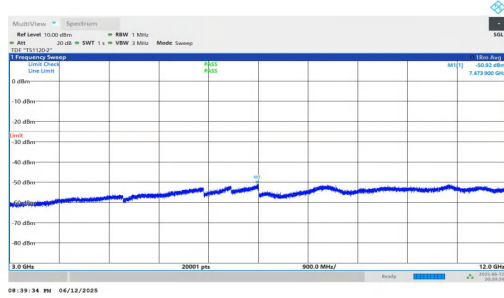
NTVN-n7-PC3-15-30-H-DFT-QPSK-Inner_1RB_Left-3000-12000- PASS
