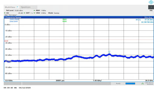
NTVN-n7-PC3-15-30-H-DFT-QPSK-Inner_1RB_Left-12000-26500- PASS
