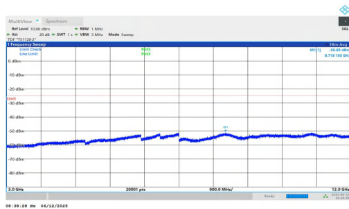
NTNV-n7-PC3-15-30-H-DFT-BPSK-Inner_1RB_Left-3000-12000- PASS
