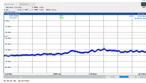
NTVN-n7-PC3-15-35-H-DFT-QPSK-Inner_1RB_Left-12000-26500-PASS
