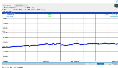
NTNV-n7-PC3-15-30-H-DFT-BPSK-Inner_1RB_Right-3000-1200 0-PASS
