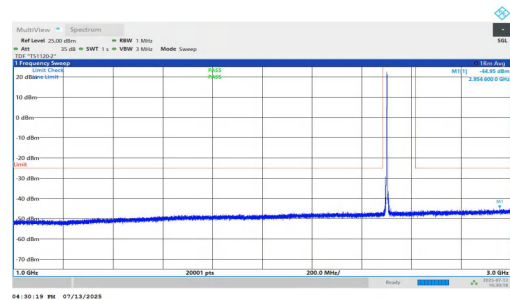
NTNV-n7-PC3-15-40-L-DFT-BPSK-Inner_1RB_Left-1000-3000-PASS SS
