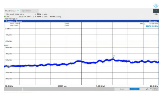
NTVN-n7-PC3-15-30-H-DFT-QPSK-Inner_1RB_Right-12000-2650 0-PASS
