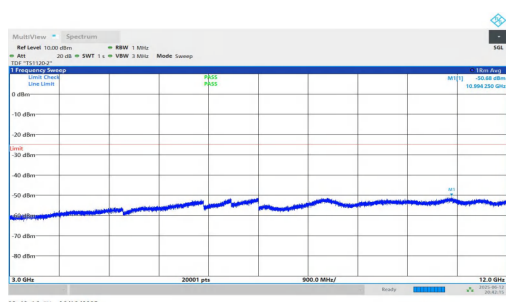
NTNV-n7-PC3-15-35-L-DFT-QPSK-Inner_1RB_Right-3000-12000-PASS
