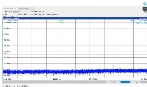
NTNV-n7-PC3-15-35-L-DFT-BPSK-Inner_1RB_Left-30-1000-PAS S
