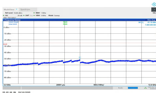
NTNV-n7-PC3-15-35-L-DFT-BPSK-Inner_1RB_Left-3000-12000- PASS
