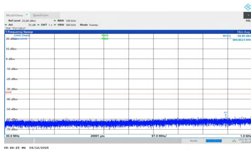
NTNV-n7-PC3-15-35-M-DFT-QPSK-Inner_1RB_Right-30-1000-P ASS
