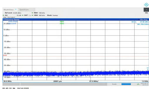
NTNV-n7-PC3-15-35-H-DFT-BPSK-Inner_1RB_Right-30-1000-P ASS
