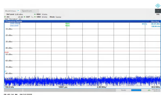
NTNV-n7-PC3-15-35-M-DFT-BPSK-Inner_1RB_Right-0.15-30-PASS
