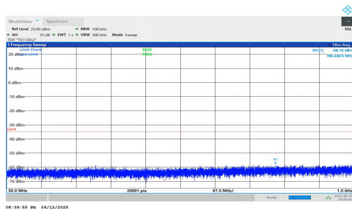
NTVN-n7-PC3-15-30-H-DFT-QPSK-Inner_1RB_Right-30-1000-P ASS
