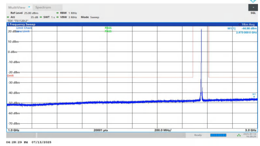
NTNV-n7-PC3-15-35-M-DFT-BPSK-Inner_1RB_Right-1000-3000-P PASS
