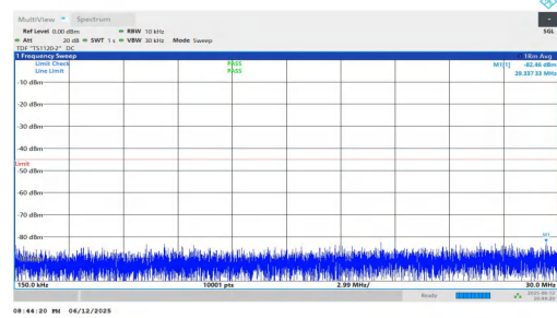
NTNV-n7-PC3-15-35-M-DFT-QPSK-Inner_1RB_Right-0.15-30-PA SS
