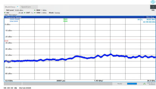
NTNV-n7-PC3-15-30-H-DFT-BPSK-Inner_1RB_Right-12000-2650 0-PASS
