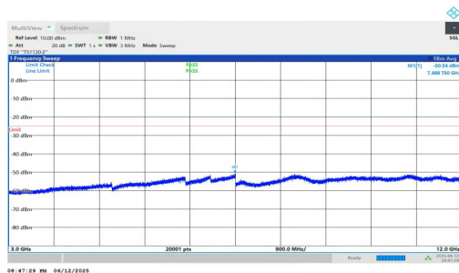
NTNV-n7-PC3-15-40-L-DFT-BPSK-Inner_1RB_Left-3000-12000- PASS
