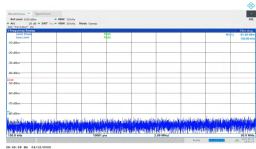
NTNV-n7-PC3-15-35-H-DFT-BPSK-Inner_1RB_Right-0.15-30-PAS S
