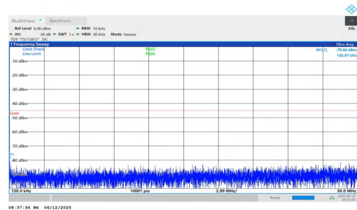
NTNV-n7-PC3-15-30-M-DFT-QPSK-Inner_1RB_Right-0.15-30-PA SS
