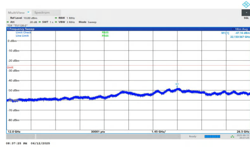
NTNV-n7-PC3-15-30-M-DFT-QPSK-Inner_1RB_Left-12000-26500 -PASS
