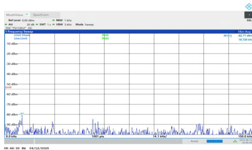
NTVN-n7-PC3-15-35-H-DFT-QPSK-Inner_1RB_Right-0.009-0.15-PASS
