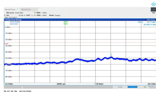
NTNV-n7-PC3-15-40-L-DFT-BPSK-Inner_1RB_Left-12000-26500- PASS
