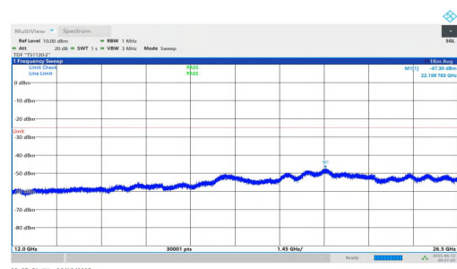
NTNV-n7-PC3-15-30-M-DFT-QPSK-Inner_1RB_Right-12000-2650 0-PASS
