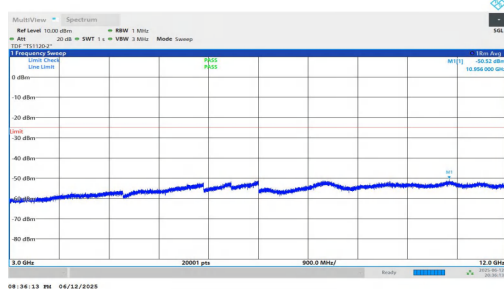
NTNV-n7-PC3-15-30-M-DFT-BPSK-Inner_1RB_Left-3000-12000-PASS
