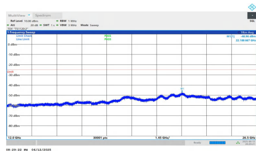
NTNV-n7-PC3-15-25-M-DFT-BPSK-Inner_1RB_Left-12000-26500-PASS
