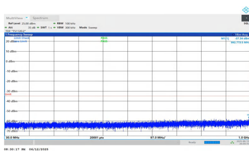
NTNV-n7-PC3-15-25-M-DFT-QPSK-Inner_1RB_Left-30-1000-PA SS
