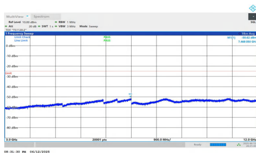
NTNV-n7-PC3-15-25-H-DFT-BPSK-Inner_1RB_Left-3000-12000- PASS
