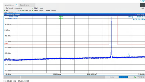
NTNV-n7-PC3-15-30-M-DFT-BPSK-Inner_1RB_Left-1000-3000-P ASS
