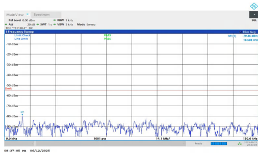
NTNV-n7-PC3-15-30-M-DFT-QPSK-Inner_1RB_Left-0.009-0.15- PASS
