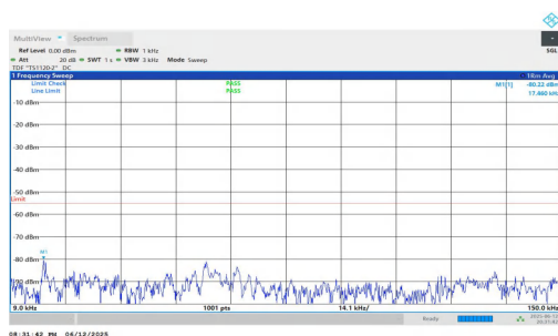
NTNV-n7-PC3-15-25-H-DFT-BPSK-Inner_1RB_Right-0.009-0.15- PASS
