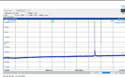
NTNV-n7-PC3-15-30-L-DFT-QPSK-Inner_1RB_Left-1000-3000-PA SS
