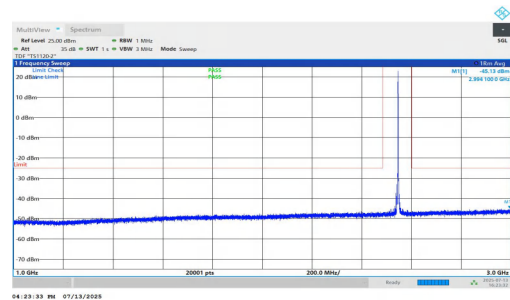
NTNV-n7-PC3-15-25-H-DFT-BPSK-Inner_1RB_Left-1000-3000-P ASS
