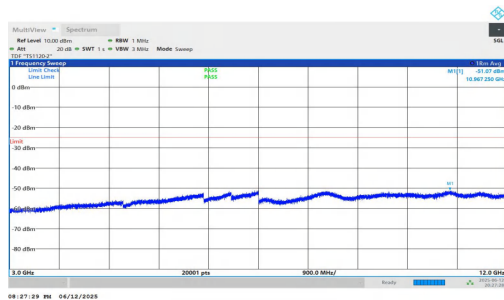
NTNV-n7-PC3-15-25-L-DFT-BPSK-Inner_1RB_Right-3000-12000 -PASS
