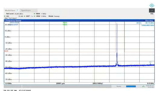
NTNV-n7-PC3-15-25-L-DFT-QPSK-Inner_1RB_Left-1000-3000-PA SS
