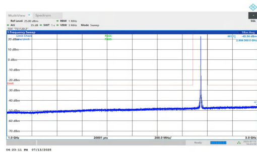
NTNV-n7-PC3-15-25-M-DFT-QPSK-Inner_1RB_Right-1000-3000- PASS
