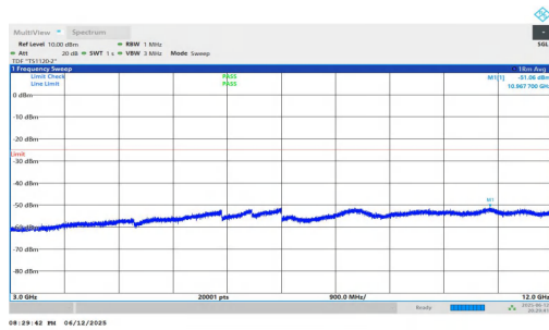
NTNV-n7-PC3-15-25-M-DFT-BPSK-Inner_1RB_Right-3000-1200 0-PASS
