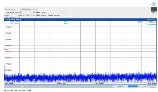
NTNV-n7-PC3-15-25-M-DFT-QPSK-Inner_1RB_Left-0.15-30-PAS S
