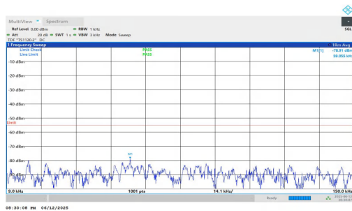
NTNV-n7-PC3-15-25-M-DFT-QPSK-Inner_1RB_Left-0.009-0.15- PASS
