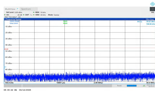
NTNV-n7-PC3-15-30-L-DFT-QPSK-Inner_1RB_Right-0.15-30-PASS
