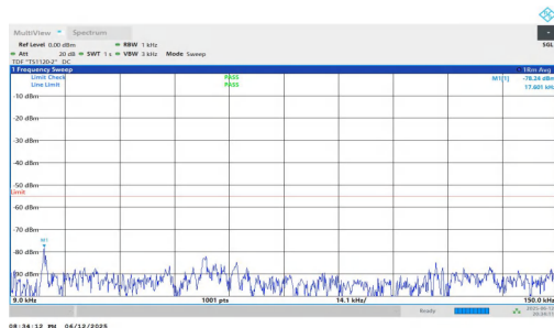
NTNV-n7-PC3-15-30-L-DFT-BPSK-Inner_1RB_Right-0.009-0.15-PASS
