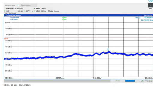
NTNV-n7-PC3-15-30-M-DFT-BPSK-Inner_1RB_Right-12000-2650 0-PASS
