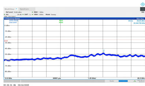
NTNV-n7-PC3-15-30-L-DFT-BPSK-Inner_1RB_Right-12000-2650 0-PASS
