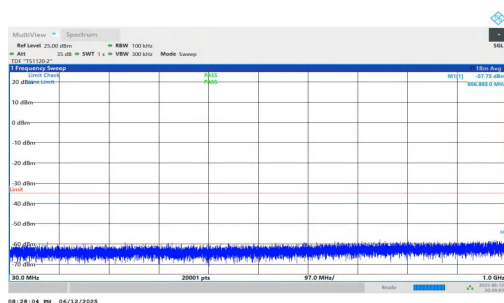
NTNV-n7-PC3-15-25-L-DFT-QPSK-Inner_1RB_Left-30-1000-PA SS
