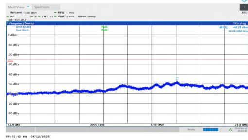
NTNV-n7-PC3-15-25-H-DFT-QPSK-Inner_1RB_Left-12000-26500- PASS
