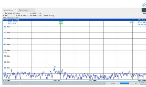
NTNV-n7-PC3-15-25-M-DFT-BPSK-Inner_1RB_Right-0.009-0.15-PASS
