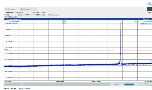
NTNV-n7-PC3-15-25-H-DFT-QPSK-Inner_1RB_Right-1000-3000- PASS
