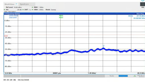
NTNV-n7-PC3-15-25-M-DFT-QPSK-Inner_1RB_Left-12000-26500 -PASS
