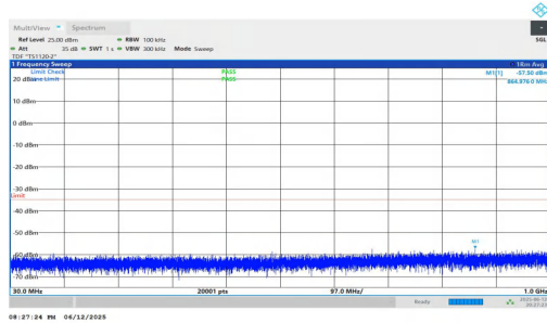
NTNV-n7-PC3-15-25-L-DFT-BPSK-Inner_1RB_Right-30-1000-PA SS
