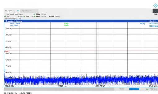
NTNV-n7-PC3-15-30-L-DFT-QPSK-Inner_1RB_Left-0.15-30-PASS
