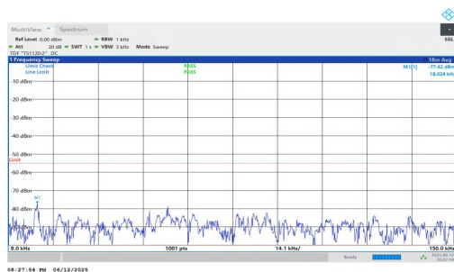
NTNV-n7-PC3-15-25-L-DFT-QPSK-Inner_1RB_Left-0.009-0.15-P ASS
