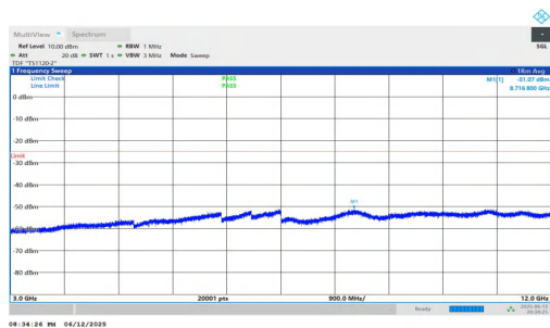
NTNV-n7-PC3-15-30-L-DFT-BPSK-Inner_1RB_Right-3000-12000 -PASS
