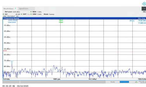
NTNV-n7-PC3-15-30-M-DFT-BPSK-Inner_1RB_Right-0.009-0.15 -PASS
