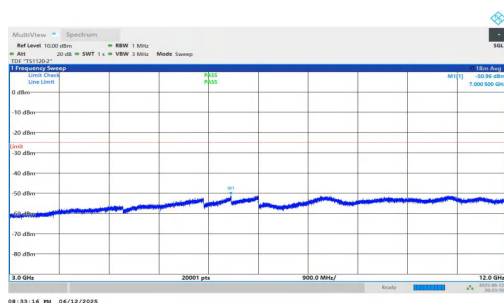
NTNV-n7-PC3-15-25-H-DFT-QPSK-Inner_1RB_Right-3000-1200 0-PASS
