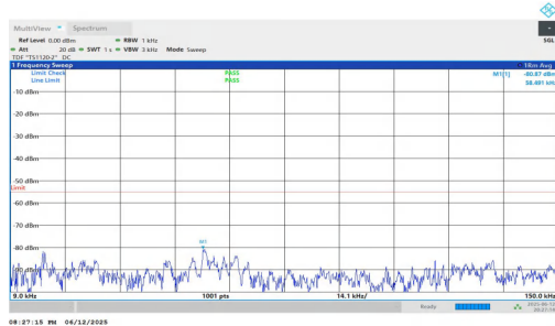
NTNV-n7-PC3-15-25-L-DFT-BPSK-Inner_1RB_Right-0.009-0.15-PASS
