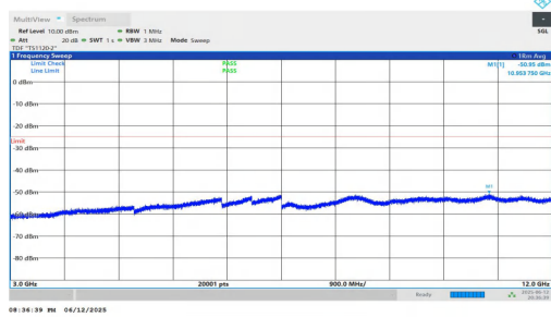
NTNV-n7-PC3-15-30-M-DFT-BPSK-Inner_1RB_Right-3000-1200 0-PASS
