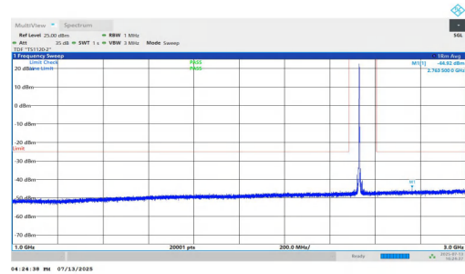
NTNV-n7-PC3-15-30-L-DFT-BPSK-Inner_1RB_Right-1000-3000-P ASS
