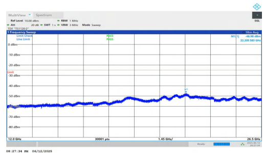
NTNV-n7-PC3-15-25-L-DFT-BPSK-Inner_1RB_Right-12000-2650 0-PASS
