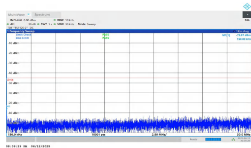
NTNV-n7-PC3-15-30-M-DFT-BPSK-Inner_1RB_Right-0.15-30-PASS
