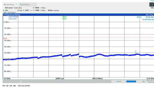
NTNV-n7-PC3-15-25-H-DFT-QPSK-Inner_1RB_Left-3000-12000- PASS
