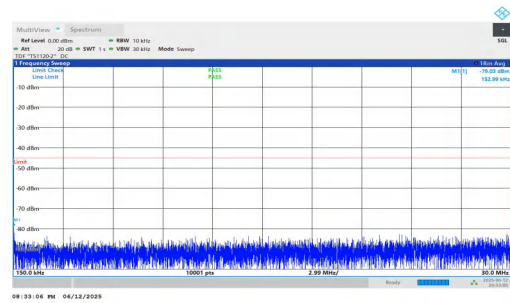
NTNV-n7-PC3-15-25-H-DFT-QPSK-Inner_1RB_Right-0.15-30-PA SS
