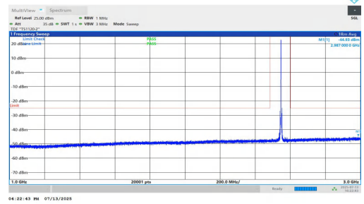
NTNV-n7-PC3-15-25-M-DFT-BPSK-Inner_1RB_Right-1000-3000-P PASS
