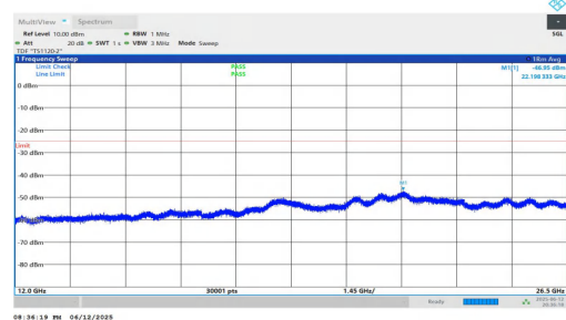
NTNV-n7-PC3-15-30-M-DFT-BPSK-Inner_1RB_Left-12000-26500-PASS
