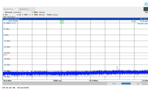
NTNV-n7-PC3-15-25-M-DFT-QPSK-Inner_1RB_Right-30-1000-P ASS
