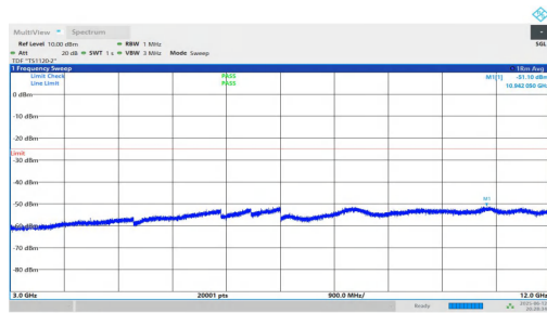
NTNV-n7-PC3-15-25-L-DFT-QPSK-Inner_1RB_Right-3000-12000-PASS
