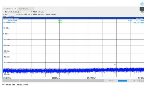
NTNV-n7-PC3-15-25-H-DFT-QPSK-Inner_1RB_Right-30-1000-P ASS
