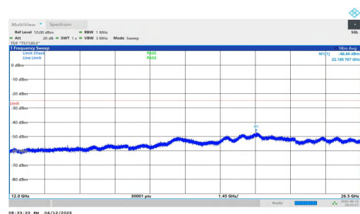
NTNV-n7-PC3-15-25-H-DFT-QPSK-Inner_1RB_Right-12000-2650 0-PASS
