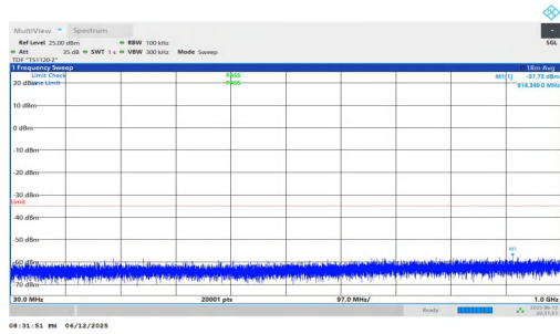
NTNV-n7-PC3-15-25-H-DFT-BPSK-Inner_1RB_Right-30-1000-P ASS
