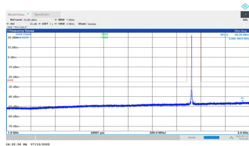
NTNV-n7-PC3-15-25-M-DFT-BPSK-Inner_1RB_Left-1000-3000-PASS
