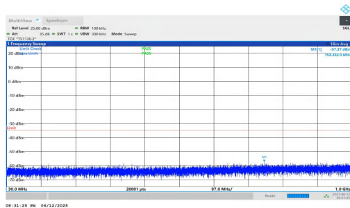
NTNV-n7-PC3-15-25-H-DFT-BPSK-Inner_1RB_Left-30-1000-PASS
