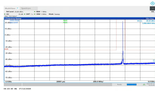
NTNV-n7-PC3-15-25-H-DFT-BPSK-Inner_1RB_Right-1000-3000-P PASS
