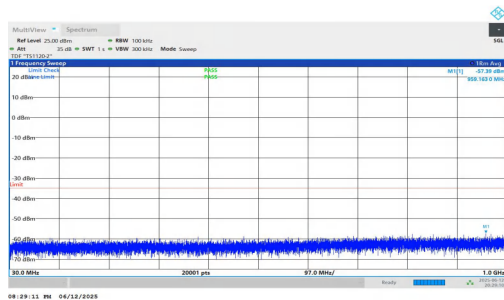
NTNV-n7-PC3-15-25-M-DFT-BPSK-Inner_1RB_Left-30-1000-PASS
