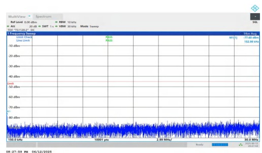
NTNV-n7-PC3-15-25-L-DFT-QPSK-Inner_1RB_Left-0.15-30-PASS
