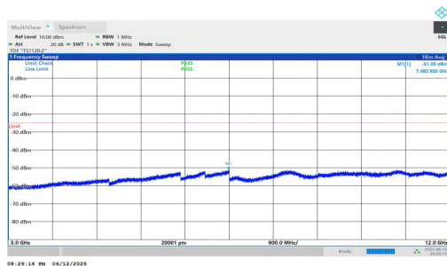
NTNV-n7-PC3-15-25-M-DFT-BPSK-Inner_1RB_Left-3000-12000-PASS
