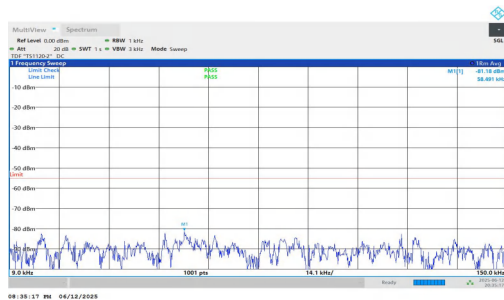
NTNV-n7-PC3-15-30-L-DFT-QPSK-Inner_1RB_Right-0.009-0.15-PASS
