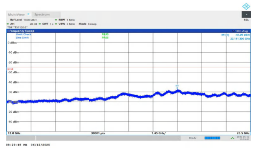
NTNV-n7-PC3-15-25-M-DFT-BPSK-Inner_1RB_Right-12000-2650 0-PASS
