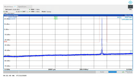
NTNV-n7-PC3-15-25-L-DFT-BPSK-Inner_1RB_Right-1000-3000-P ASS
