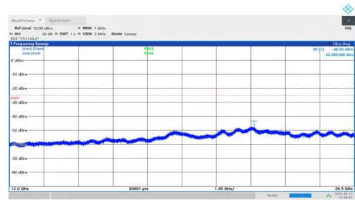
NTNV-n7-PC3-15-25-L-DFT-QPSK-Inner_1RB_Right-12000-26500-PASS
