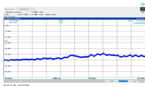
NTNV-n7-PC3-15-25-H-DFT-BPSK-Inner_1RB_Right-12000-2650 0-PASS
