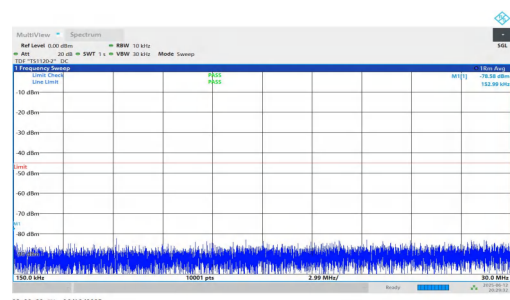
NTNV-n7-PC3-15-25-M-DFT-BPSK-Inner_1RB_Right-0.15-30-PASS
