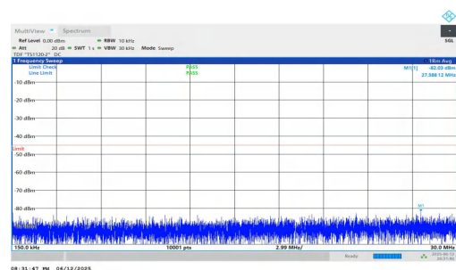
NTNV-n7-PC3-15-25-H-DFT-BPSK-Inner_1RB_Right-0.15-30-PAS S
