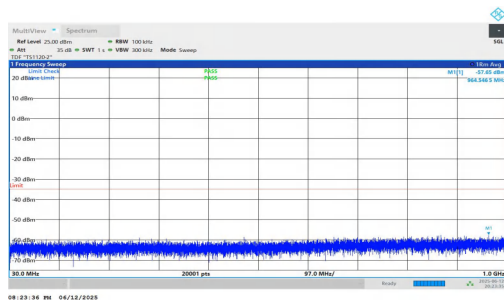
NTNV-n7-PC3-15-20-M-DFT-QPSK-Inner_1RB_Right-30-1000-P ASS
