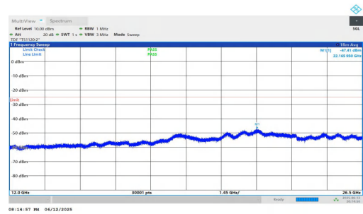
NTNV-n7-PC3-15-15-M-DFT-BPSK-Inner_1RB_Right-12000-2650 0-PASS
