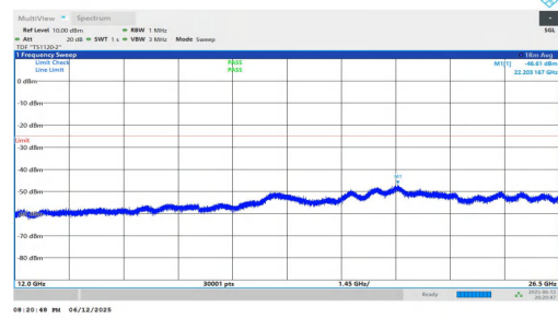
NTNV-n7-PC3-15-20-L-DFT-QPSK-Inner_1RB_Left-12000-26500-PASS
