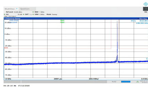
NTVN-n7-PC3-15-15-H-DFT-QPSK-Inner_1RB_Right-1000-3000- PASS
