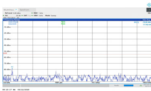
NTNV-n7-PC3-15-15-M-DFT-QPSK-Inner_1RB_Left-0.009-0.15- PASS
