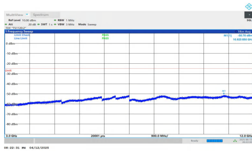
NTNV-n7-PC3-15-20-M-DFT-BPSK-Inner_1RB_Right-3000-12000-P PASS
