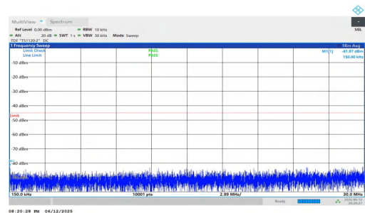
NTNV-n7-PC3-15-20-L-DFT-QPSK-Inner_1RB_Left-0.15-30-PASS
