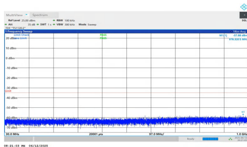
NTNV-n7-PC3-15-20-L-DFT-QPSK-Inner_1RB_Right-30-1000-PASS
