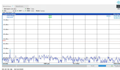
NTNV-n7-PC3-15-20-L-DFT-QPSK-Inner_1RB_Right-0.009-0.15-PASS
