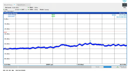
NTNV-n7-PC3-15-20-L-DFT-BPSK-Inner_1RB_Left-12000-26500-PASS
