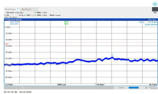
NTNV-n7-PC3-15-20-H-DFT-BPSK-Inner_1RB_Right-12000-2650 0-PASS
