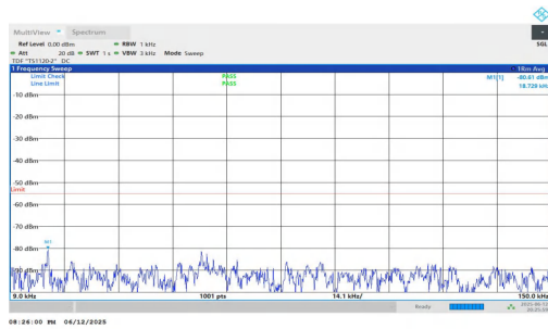
NTNV-n7-PC3-15-20-H-DFT-QPSK-Inner_1RB_Right-0.009-0.15-PASS
