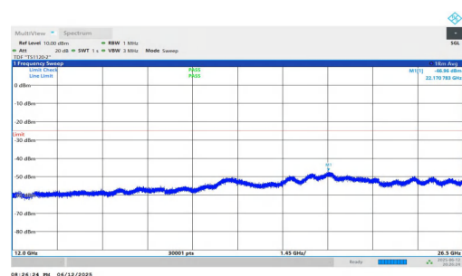
NTNV-n7-PC3-15-20-H-DFT-QPSK-Inner_1RB_Right-12000-26500-PASS
