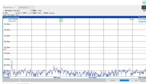
NTNV-n7-PC3-15-20-H-DFT-BPSK-Inner_1RB_Right-0.009-0.15-PASS
