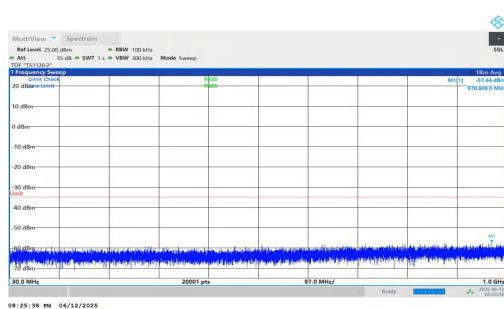
NTNV-n7-PC3-15-20-H-DFT-QPSK-Inner_1RB_Left-30-1000-PA SS
