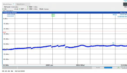
NTNV-n7-PC3-15-20-L-DFT-QPSK-Inner_1RB_Left-3000-12000-PASS
