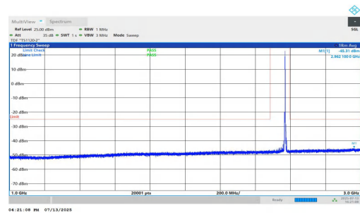
NTNV-n7-PC3-15-20-H-DFT-QPSK-Inner_1RB_Right-1000-3000-PASS
