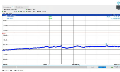
NTNV-n7-PC3-15-15-M-DFT-BPSK-Inner_1RB_Right-3000-1200 0-PASS
