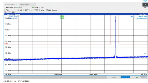
NTNV-n7-PC3-15-20-H-DFT-BPSK-Inner_1RB_Left-1000-3000-PASS
