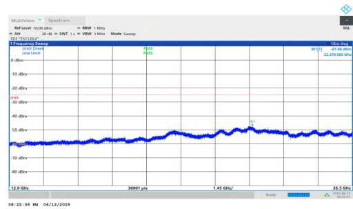
NTNV-n7-PC3-15-20-M-DFT-BPSK-Inner_1RB_Right-12000-26500-P PASS
