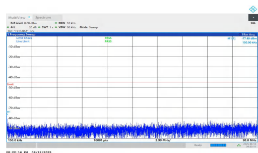
NTNV-n7-PC3-15-20-M-DFT-BPSK-Inner_1RB_Right-0.15-30-PASS SS
