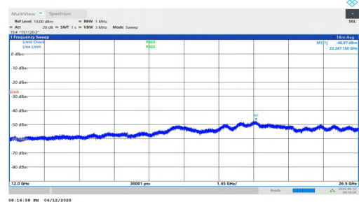
NTNV-n7-PC3-15-15-H-DFT-BPSK-Inner_1RB_Left-12000-26500-PASS
