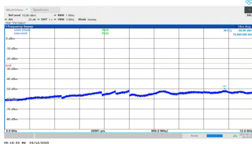
NTNV-n7-PC3-15-15-H-DFT-BPSK-Inner_1RB_Left-3000-12000-PASS
