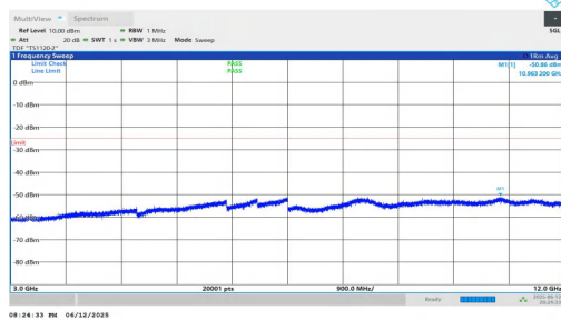
NTNV-n7-PC3-15-20-H-DFT-BPSK-Inner_1RB_Left-3000-12000-PASS
