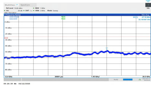
NTNV-n7-PC3-15-20-H-DFT-BPSK-Inner_1RB_Left-12000-26500-PASS
