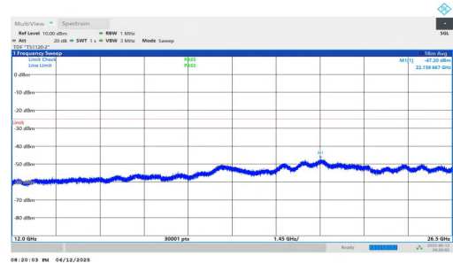
NTNV-n7-PC3-15-20-L-DFT-BPSK-Inner_1RB_Right-12000-2650 0-PASS
