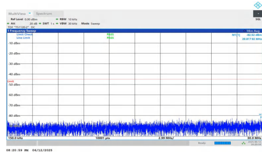
NTNV-n7-PC3-15-20-L-DFT-QPSK-Inner_1RB_Right-0.15-30-PASS
