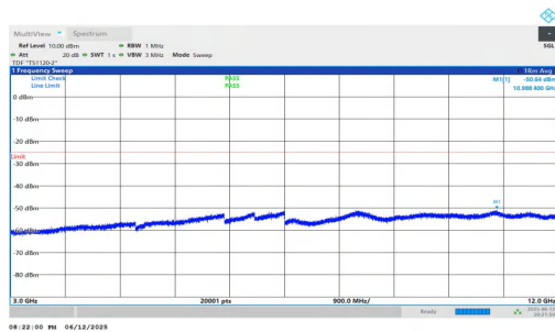
NTNV-n7-PC3-15-20-M-DFT-BPSK-Inner_1RB_Left-3000-12000-PASS PASS
