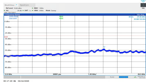
NTNV-n7-PC3-15-15-H-DFT-BPSK-Inner_1RB_Right-12000-26500-P PASS
