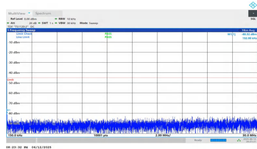
NTNV-n7-PC3-15-20-M-DFT-QPSK-Inner_1RB_Right-0.15-30-PA SS
