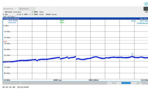
NTNV-n7-PC3-15-20-H-DFT-BPSK-Inner_1RB_Right-3000-1200 0-PASS
