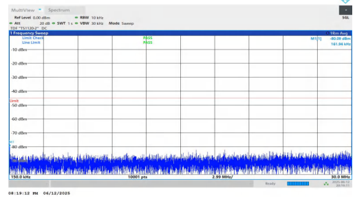
NTNV-n7-PC3-15-20-L-DFT-BPSK-Inner_1RB_Left-0.15-30-PASS
