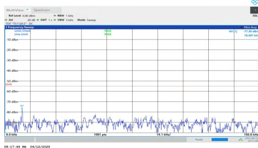
NTNV-n7-PC3-15-15-H-DFT-QPSK-Inner_1RB_Left-0.009-0.15-P ASS
