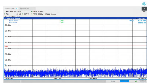
NTNV-n7-PC3-15-15-H-DFT-BPSK-Inner_1RB_Right-0.15-30-PASS
