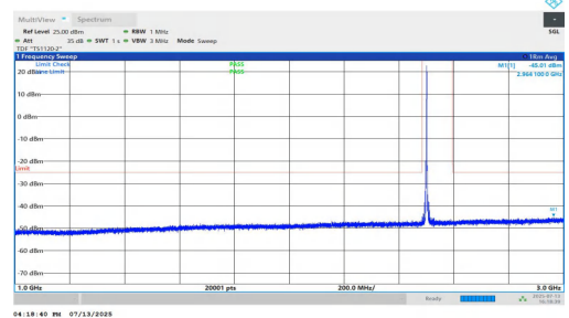
NTNV-n7-PC3-15-20-L-DFT-BPSK-Inner_1RB_Left-1000-3000-PASS
