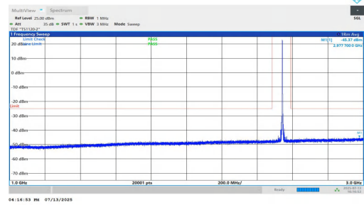
NTNV-n7-PC3-15-15-M-DFT-BPSK-Inner_1RB_Right-1000-3000-P PASS
