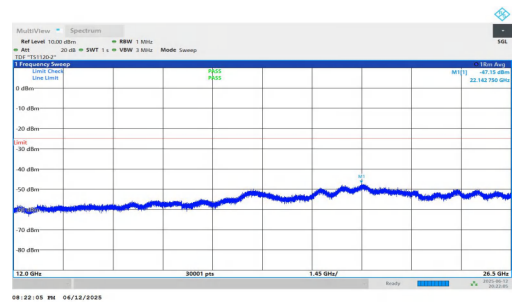
NTNV-n7-PC3-15-20-M-DFT-BPSK-Inner_1RB_Left-12000-26500-PASS PASS
