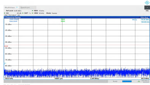
NTNV-n7-PC3-15-20-H-DFT-BPSK-Inner_1RB_Right-0.15-30-PASS
