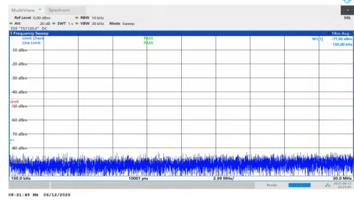
NTNV-n7-PC3-15-20-M-DFT-BPSK-Inner_1RB_Left-0.15-30-PAS S
