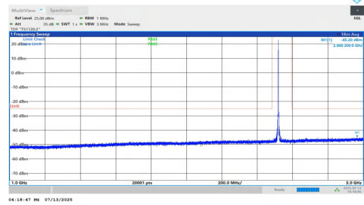
NTNV-n7-PC3-15-20-L-DFT-BPSK-Inner_1RB_Right-1000-3000-P ASS
