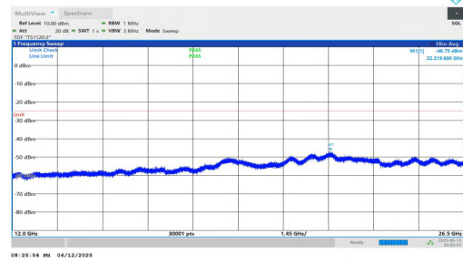
NTNV-n7-PC3-15-20-H-DFT-QPSK-Inner_1RB_Left-12000-26500-PASS
