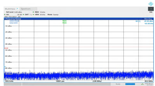
NTNV-n7-PC3-15-20-L-DFT-BPSK-Inner_1RB_Right-0.15-30-PASS
