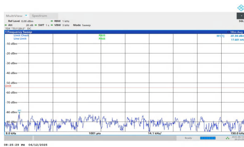
NTNV-n7-PC3-15-20-H-DFT-QPSK-Inner_1RB_Left-0.009-0.15-P ASS
