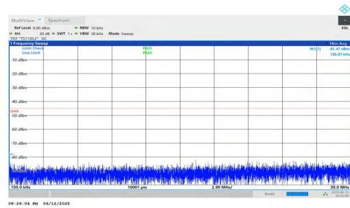
NTNV-n7-PC3-15-20-H-DFT-QPSK-Inner_1RB_Right-0.15-30-PA-SS
