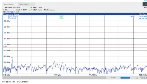
NTNV-n7-PC3-15-20-M-DFT-BPSK-Inner_1RB_Left-0.009-0.15-P ASS
