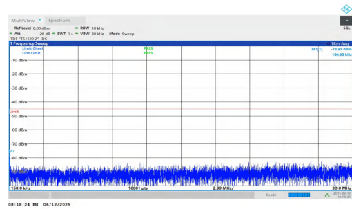
NTVN-n7-PC3-15-15-H-DFT-QPSK-Inner_1RB_Right-0.15-30-PA SS
