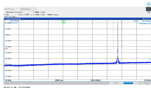
NTNV-n7-PC3-15-20-M-DFT-QPSK-Inner_1RB_Right-1000-3000- PASS
