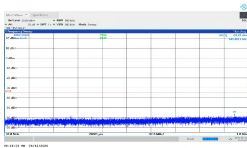
NTNV-n7-PC3-15-20-H-DFT-QPSK-Inner_1RB_Right-30-1000-PASS
