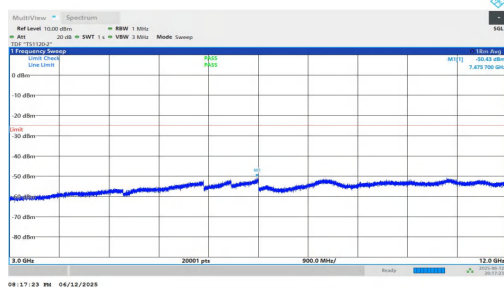
NTNV-n7-PC3-15-15-H-DFT-BPSK-Inner_1RB_Right-3000-12000-P PASS
