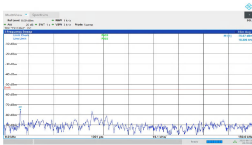
NTNV-n7-PC3-15-20-L-DFT-BPSK-Inner_1RB_Right-0.009-0.15-PASS
