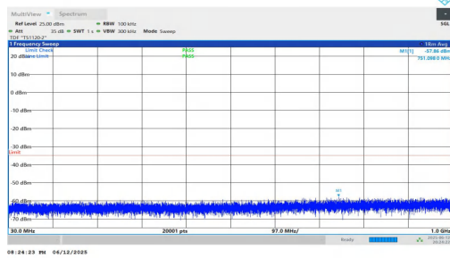
NTNV-n7-PC3-15-20-H-DFT-BPSK-Inner_1RB_Left-30-1000-PASS
