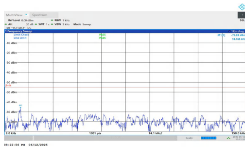
NTNV-n7-PC3-15-20-M-DFT-QPSK-Inner_1RB_Left-0.009-0.15-P PASS
