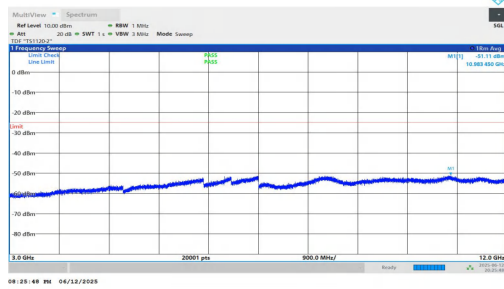
NTNV-n7-PC3-15-20-H-DFT-QPSK-Inner_1RB_Left-3000-12000-PASS
