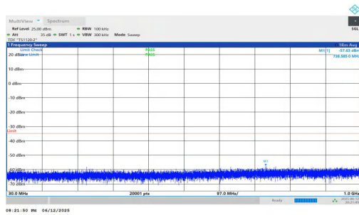
NTNV-n7-PC3-15-20-M-DFT-BPSK-Inner_1RB_Left-30-1000-PASS SS
