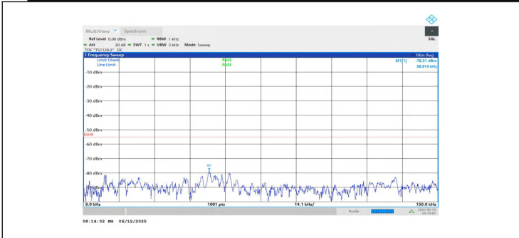
NTNV-n7-PC3-15-15-M-DFT-BPSK-Inner_1RB_Left-0.009-0.15-PASS
