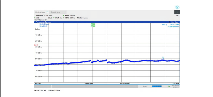
NTNV-n7-PC3-15-10-M-DFT-BPSK-Inner_1RB_Left-3000-12000-PASS PASS
