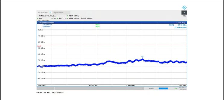
NTNV-n7-PC3-15-15-M-DFT-BPSK-Inner_1RB_Left-12000-26500-PASS
