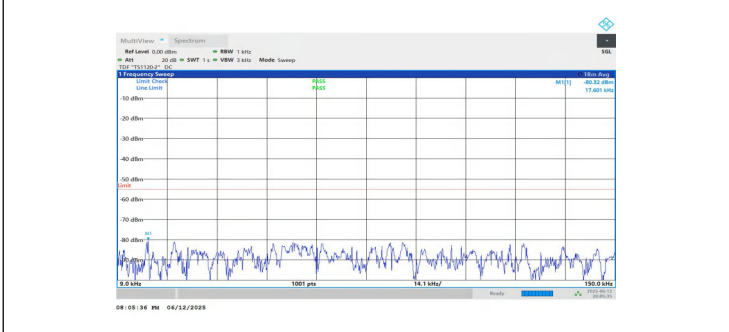
NTNV-n7-PC3-15-10-L-DFT-QPSK-Inner_1RB_Right-0.009-0.15-PASS
