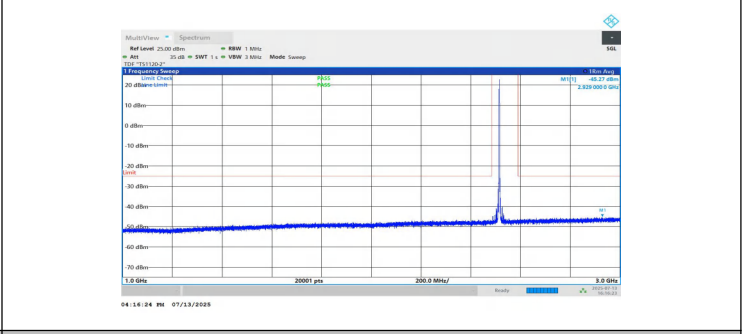
NTNV-n7-PC3-15-15-L-DFT-QPSK-Inner_1RB_Right-1000-3000-PASS
