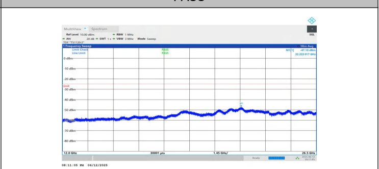
NTNV-n7-PC3-15-10-H-DFT-QPSK-Inner_1RB_Right-12000-26500-PASS
