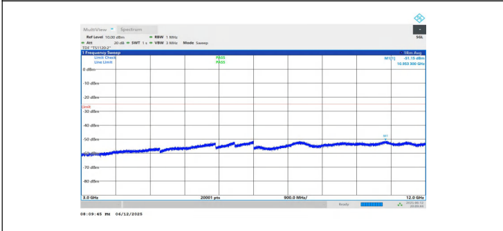
NTNV-n7-PC3-15-10-H-DFT-BPSK-Inner_1RB_Right-3000-1200 0-PASS
