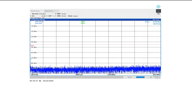
NTNV-n7-PC3-15-10-M-DFT-BPSK-Inner_1RB_Left-0.15-30-PAS S
