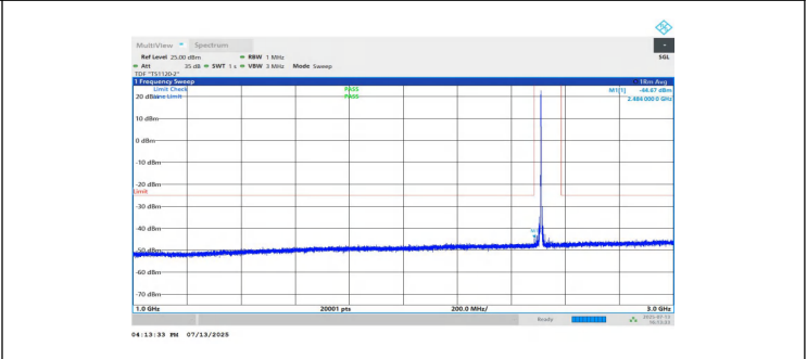
NTNV-n7-PC3-15-10-L-DFT-QPSK-Inner_1RB_Right-1000-3000-PASS
