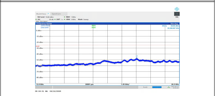
NTNV-n7-PC3-15-10-L-DFT-QPSK-Inner_1RB_Right-12000-26500-0-PASS
