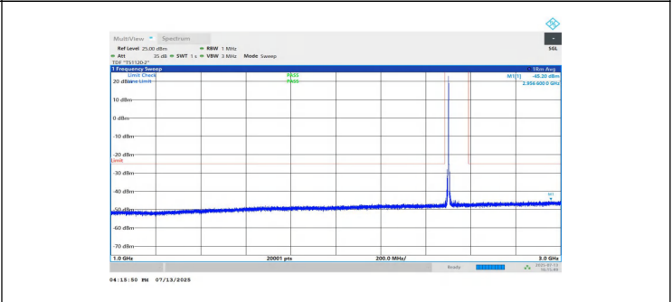
NTNV-n7-PC3-15-15-L-DFT-BPSK-Inner_1RB_Left-1000-3000-PASS
