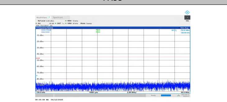
NTNV-n7-PC3-15-10-M-DFT-BPSK-Inner_1RB_Right-0.15-30-PASS SS
