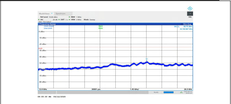
NTNV-n7-PC3-15-10-L-DFT-QPSK-Inner_1RB_Left-12000-26500-PASS
