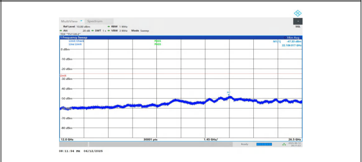
NTNV-n7-PC3-15-15-L-DFT-BPSK-Inner_1RB_Left-12000-26500-PASS
