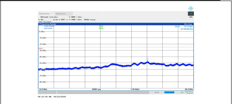
NTNV-n7-PC3-15-10-H-DFT-QPSK-Inner_1RB_Left-12000-26500-PASS
