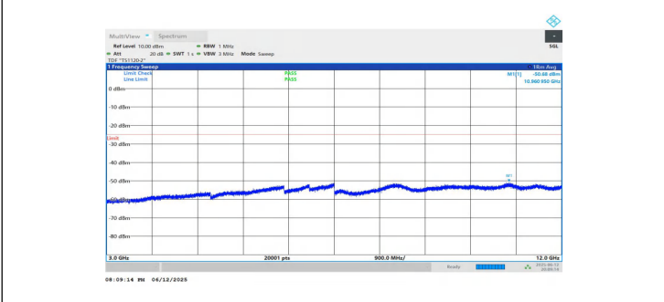
NTNV-n7-PC3-15-10-H-DFT-BPSK-Inner_1RB_Left-3000-12000-PASS
