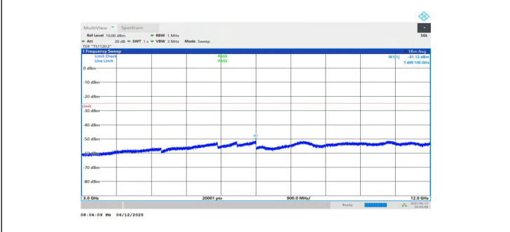
NTNV-n7-PC3-15-10-L-DFT-BPSK-Inner_1RB_Left-3000-12000-PASS
