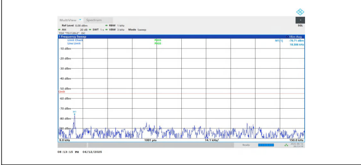
NTNV-n7-PC3-15-15-L-DFT-QPSK-Inner_1RB_Right-0.009-0.15-PASS
