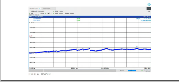
NTNV-n7-PC3-15-15-L-DFT-QPSK-Inner_1RB_Right-3000-12000-PASS
