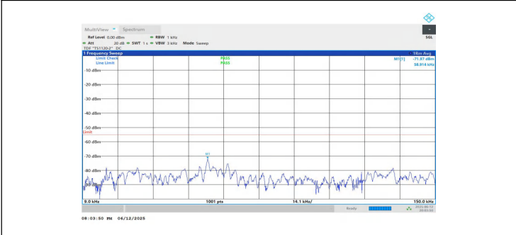
NTNV-n7-PC3-15-10-L-DFT-BPSK-Inner_1RB_Left-0.009-0.15-PASS
