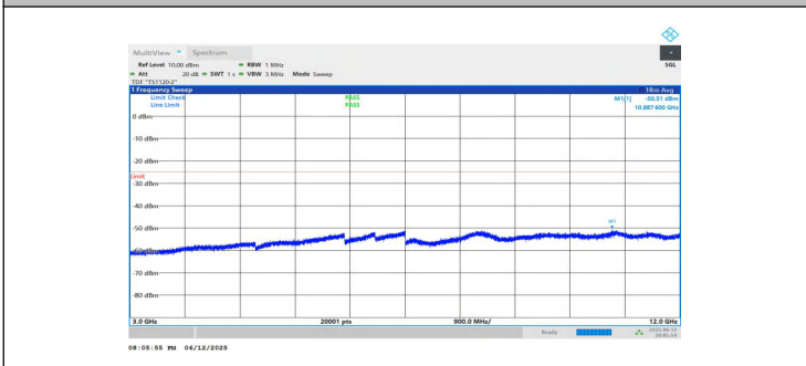
NTNV-n7-PC3-15-10-L-DFT-QPSK-Inner_1RB_Right-3000-12000-0-PASS
