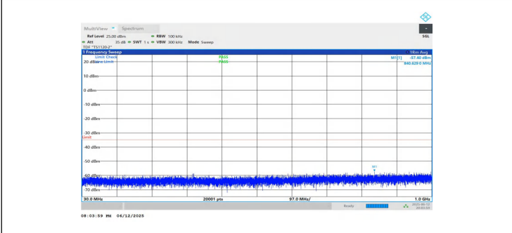
NTNV-n7-PC3-15-10-L-DFT-BPSK-Inner_1RB_Left-30-1000-PASS
