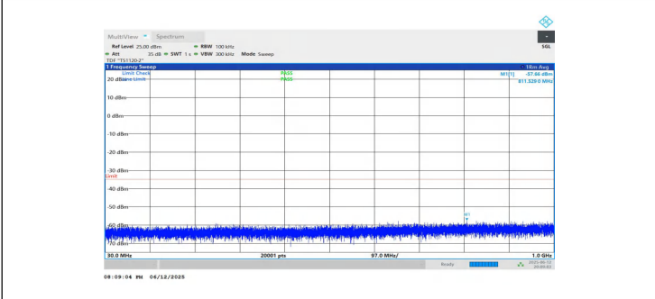
NTNV-n7-PC3-15-10-H-DFT-BPSK-Inner_1RB_Left-30-1000-PASS
