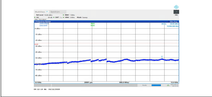
NTNV-n7-PC3-15-15-L-DFT-BPSK-Inner_1RB_Right-3000-12000 -PASS
