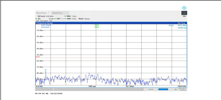
NTNV-n7-PC3-15-10-H-DFT-BPSK-Inner_1RB_Right-0.009-0.15-PASS
