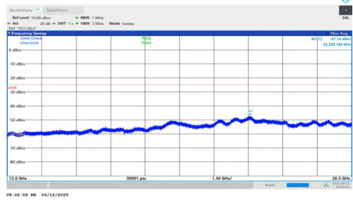
NTNV-n7-PC3-15-5-H-DFT-QPSK-Inner_1RB_Left-12000-26500-P ASS
