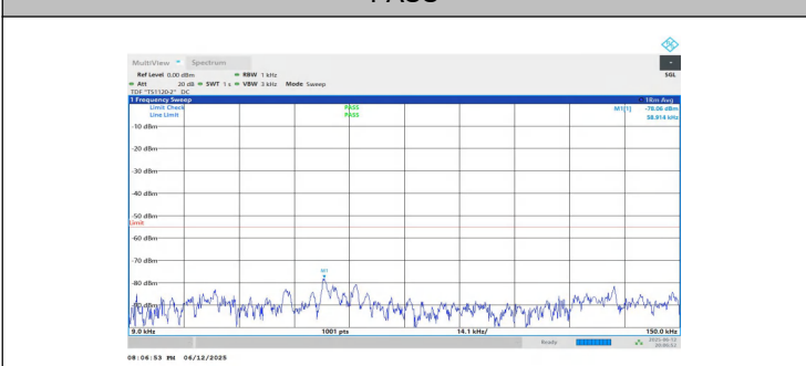
NTNV-n7-PC3-15-10-M-DFT-BPSK-Inner_1RB_Right-0.009-0.15 -PASS
