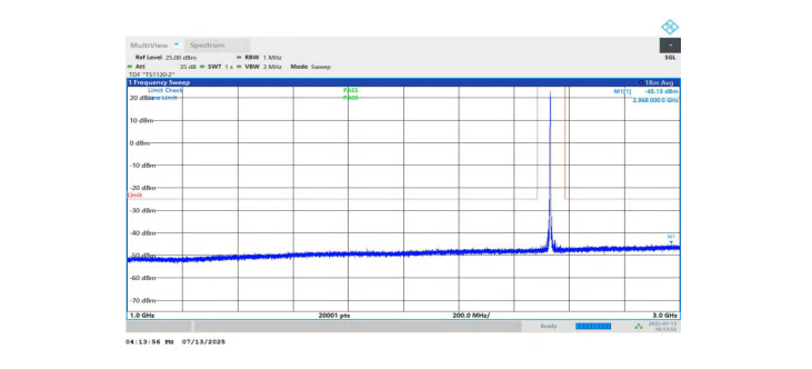
NTNV-n7-PC3-15-10-M-DFT-BPSK-Inner_1RB_Left-1000-3000-P ASS
