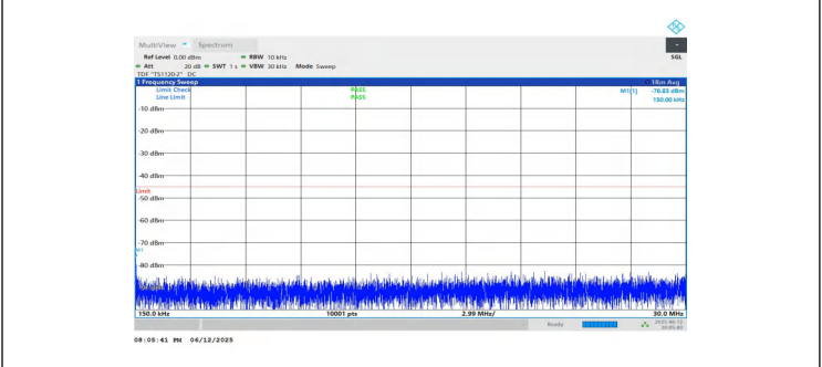
NTNV-n7-PC3-15-10-L-DFT-QPSK-Inner_1RB_Right-0.15-30-PASS
