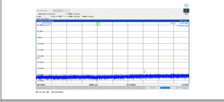
NTNV-n7-PC3-15-15-L-DFT-QPSK-Inner_1RB_Left-30-1000-PA SS
