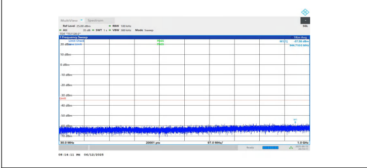
NTNV-n7-PC3-15-15-M-DFT-BPSK-Inner_1RB_Left-30-1000-PASS
