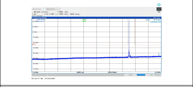
NTNV-n7-PC3-15-15-L-DFT-QPSK-Inner_1RB_Left-1000-3000-PA SS
