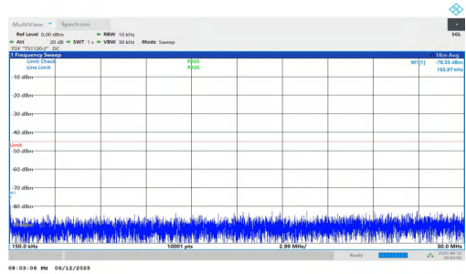
NTNV-n7-PC3-15-5-H-DFT-QPSK-Inner_1RB_Right-0.15-30-P ASS
