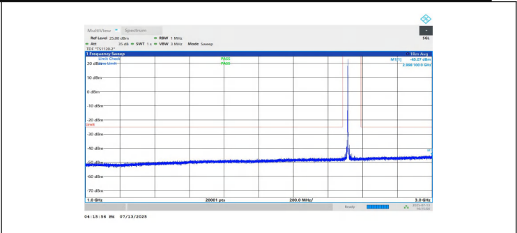
NTNV-n7-PC3-15-15-L-DFT-BPSK-Inner_1RB_Right-1000-3000-PA ASS
