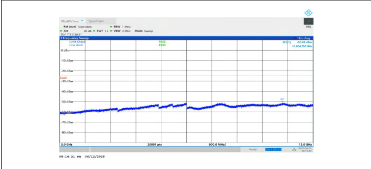
NTNV-n7-PC3-15-15-M-DFT-BPSK-Inner_1RB_Left-3000-12000-PASS
