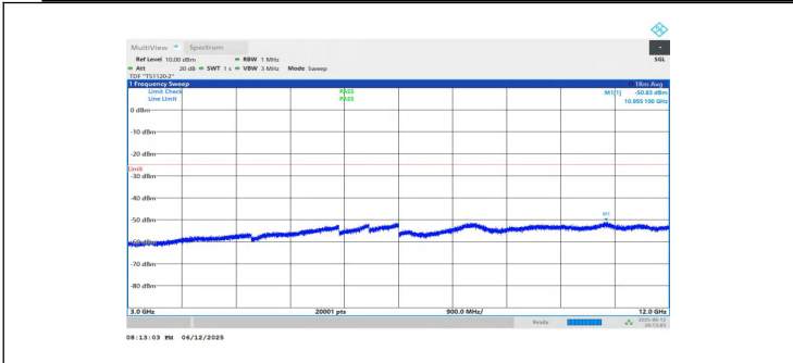
NTNV-n7-PC3-15-15-L-DFT-QPSK-Inner_1RB_Left-3000-12000-PASS
