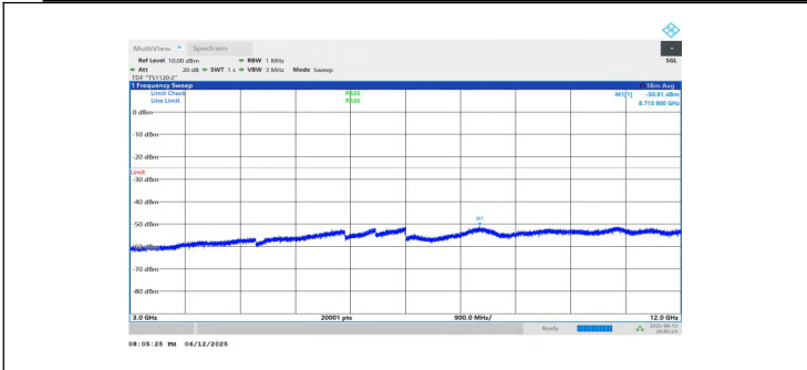
NTNV-n7-PC3-15-10-L-DFT-QPSK-Inner_1RB_Left-3000-12000-PASS
