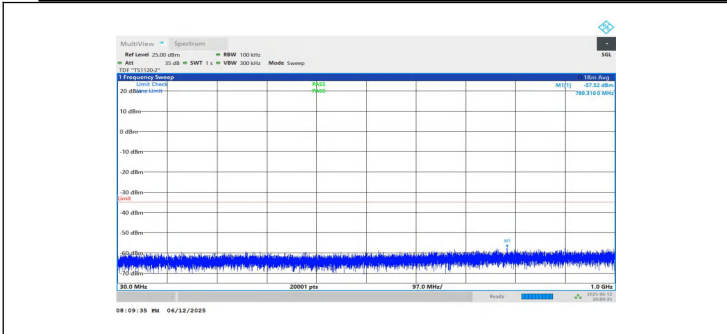
NTNV-n7-PC3-15-10-H-DFT-BPSK-Inner_1RB_Right-30-1000-P ASS
