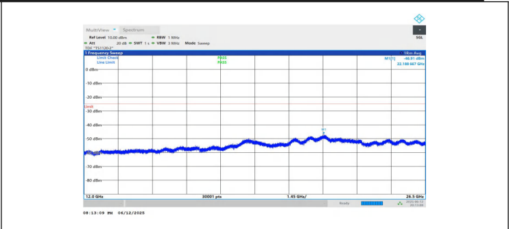
NTNV-n7-PC3-15-15-L-DFT-QPSK-Inner_1RB_Left-12000-26500-PASS
