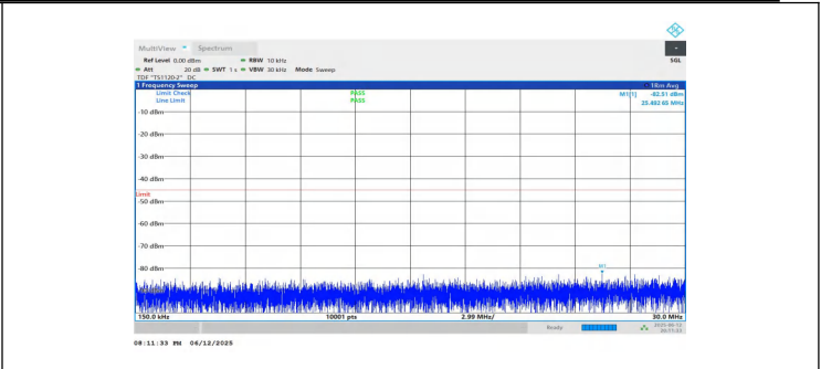
NTNV-n7-PC3-15-15-L-DFT-BPSK-Inner_1RB_Left-0.15-30-PASS
