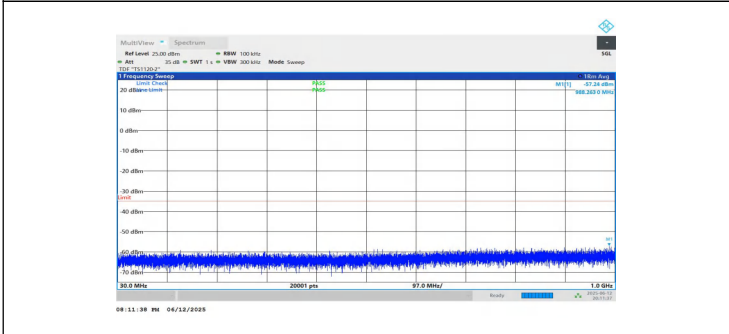
NTNV-n7-PC3-15-15-L-DFT-BPSK-Inner_1RB_Left-30-1000-PASS
