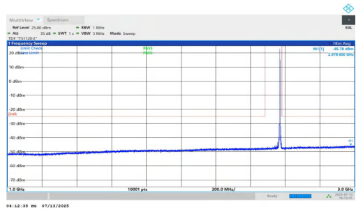
NTNV-n7-PC3-15-5-H-DFT-QPSK-Inner_1RB_Right-1000-3000-P ASS
