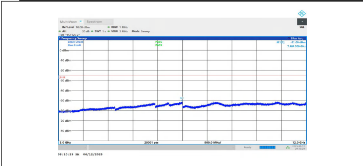
NTNV-n7-PC3-15-10-H-DFT-QPSK-Inner_1RB_Left-3000-12000-PASS
