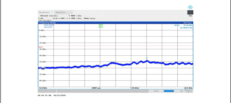
NTNV-n7-PC3-15-10-L-DFT-BPSK-Inner_1RB_Left-12000-26500-PASS
