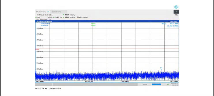
NTNV-n7-PC3-15-15-L-DFT-QPSK-Inner_1RB_Right-0.15-30-PASS
