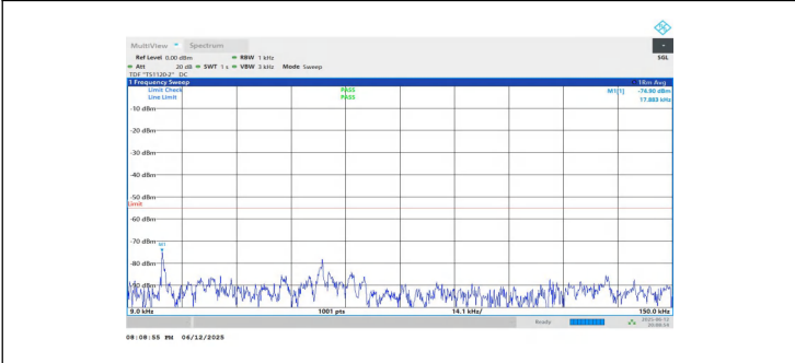
NTNV-n7-PC3-15-10-H-DFT-BPSK-Inner_1RB_Left-0.009-0.15-PASS
