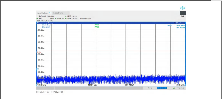
NTNV-n7-PC3-15-15-M-DFT-BPSK-Inner_1RB_Left-0.15-30-PASS
