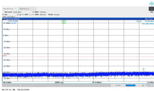
NTNV-n7-PC3-15-5-H-DFT-QPSK-Inner_1RB_Right-30-1000-P ASS
