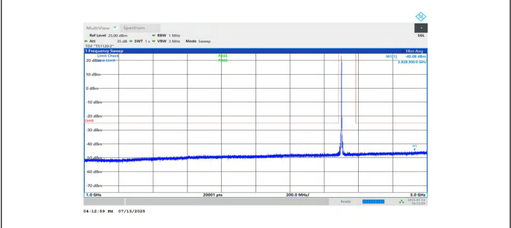
NTNV-n7-PC3-15-10-L-DFT-BPSK-Inner_1RB_Left-1000-3000-PASS
