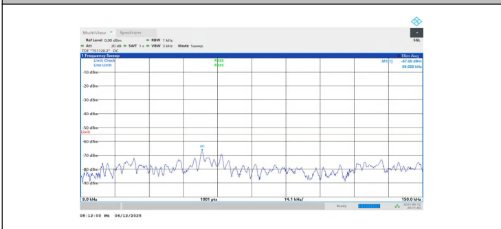
NTNV-n7-PC3-15-15-L-DFT-BPSK-Inner_1RB_Right-0.009-0.15-PASS
