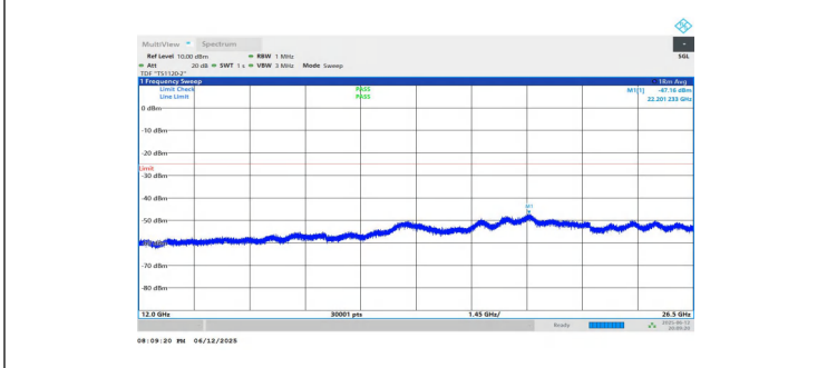
NTNV-n7-PC3-15-10-H-DFT-BPSK-Inner_1RB_Left-12000-26500-PASS
