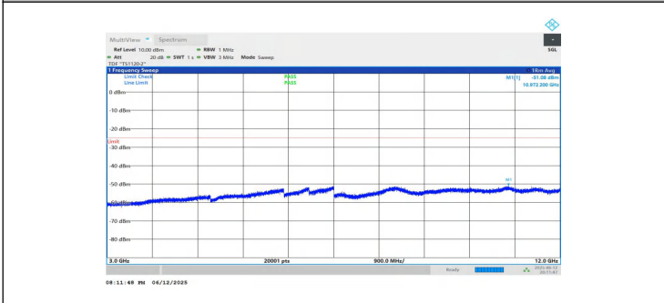
NTNV-n7-PC3-15-15-L-DFT-BPSK-Inner_1RB_Left-3000-12000-PASS
