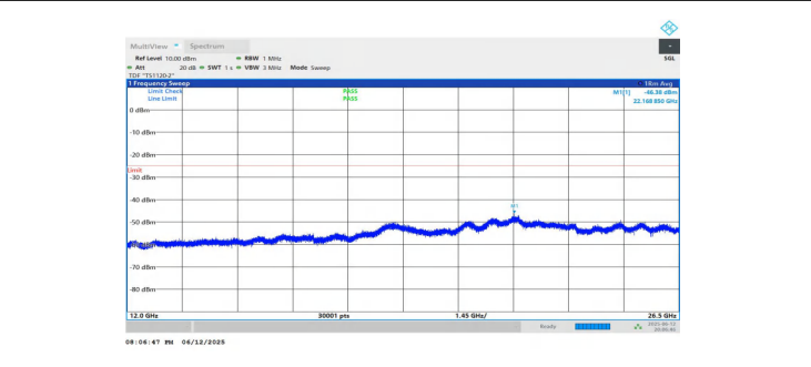
NTNV-n7-PC3-15-10-M-DFT-BPSK-Inner_1RB_Left-12000-26500-PASS PASS
