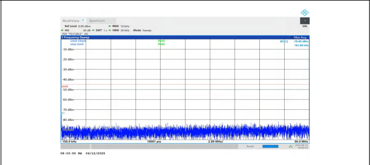
NTNV-n7-PC3-15-10-L-DFT-BPSK-Inner_1RB_Left-0.15-30-PASS
