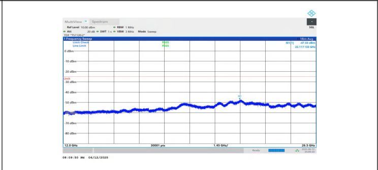
NTNV-n7-PC3-15-10-H-DFT-BPSK-Inner_1RB_Right-12000-2650 0-PASS
