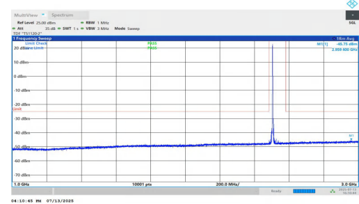
NTNV-n7-PC3-15-5-L-DFT-QPSK-Inner_1RB_Right-1000-3000-P ASS
