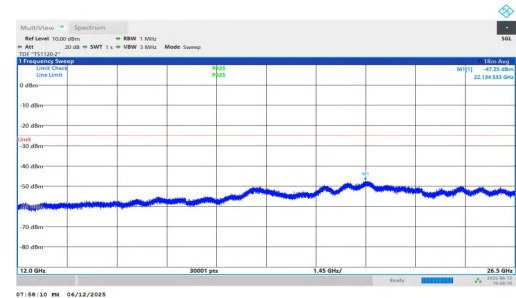
NTNV-n7-PC3-15-5-L-DFT-QPSK-Inner_1RB_Right-12000-26500- PASS
