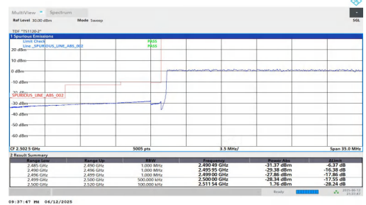
NTNV-n7-PC3-15-30-L-DFT-QPSK-Outer_Full-PASS
