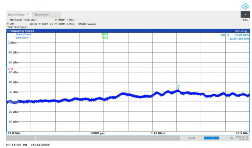
NTNV-n7-PC3-15-5-L-DFT-BPSK-Inner_1RB_Right-12000-26500- PASS
