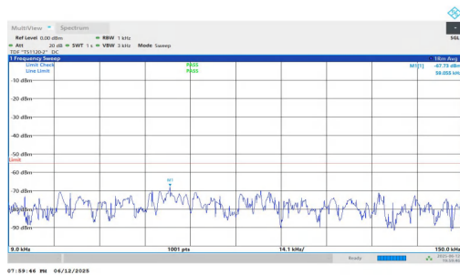
NTNV-n7-PC3-15-5-M-DFT-QPSK-Inner_1RB_Left-0.009-0.15-P ASS
