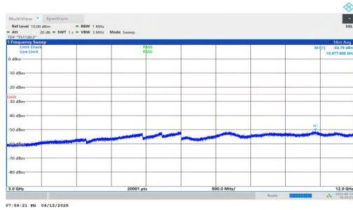
NTNV-n7-PC3-15-5-M-DFT-BPSK-Inner_1RB_Right-3000-12000 -PASS
