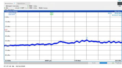
NTNV-n7-PC3-15-5-L-DFT-QPSK-Inner_1RB_Left-12000-26500-P ASS
