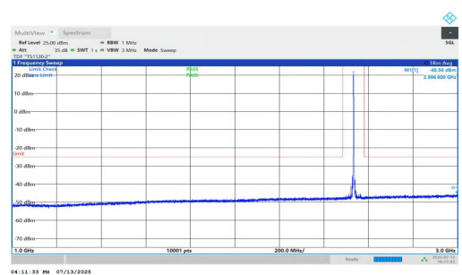
NTNV-n7-PC3-15-5-M-DFT-QPSK-Inner_1RB_Left-1000-3000-PA SS
