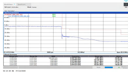
NTNV-n7-PC3-15-40-H-DFT-QPSK-Outer_Full-PASS
