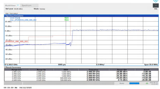
NTNV-n7-PC3-15-25-L-DFT-QPSK-Outer_Full-PASS
