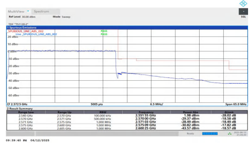
NTNV-n7-PC3-15-30-H-DFT-QPSK-Outer_Full-PASS
