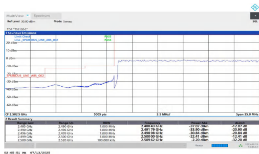
NTNV-n7-PC3-15-40-L-DFT-BPSK-Outer Full-PASS
