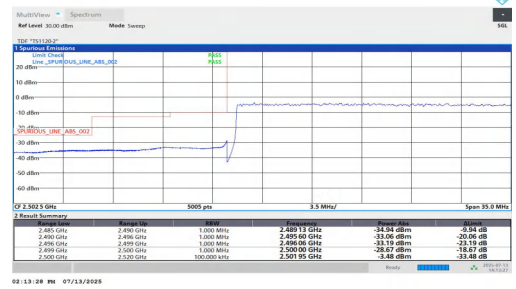
NTNV-n7-PC3-15-50-L-DFT-QPSK-Outer_Full-PASS
