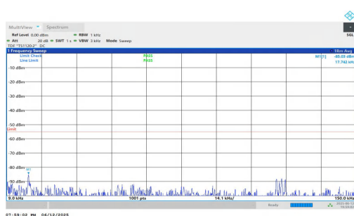
NTNV-n7-PC3-15-5-M-DFT-BPSK-Inner_1RB_Right-0.009-0.15-PASS
