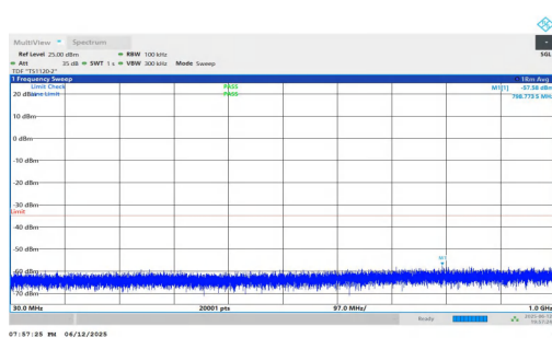
NTNV-n7-PC3-15-5-L-DFT-QPSK-Inner_1RB_Left-30-1000-PAS S
