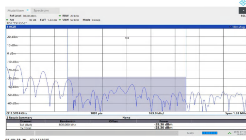
NTNV-n7-PC3-15-40-H-DFT-BPSK-Edge_1RB_Right-PASS
