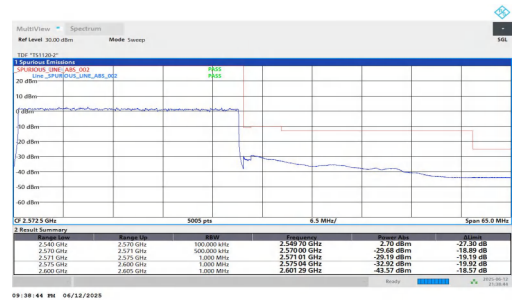
NTNV-n7-PC3-15-30-H-DFT-BPSK-Outer_Full-PASS
