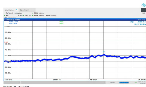
NTNV-n7-PC3-15-5-M-DFT-QPSK-Inner_1RB_Right-12000-26500 -PASS
