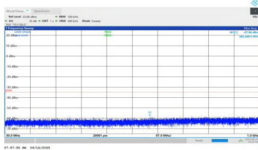
NTNV-n7-PC3-15-5-L-DFT-QPSK-Inner_1RB_Right-30-1000-PA SS
