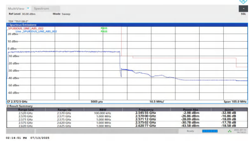
NTNV-n7-PC3-15-50-H-DFT-BPSK-Outer_Full-PASS
