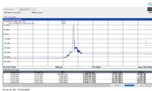
NTNV-n7-PC3-15-50-H-DFT-QPSK-Edge_1RB_Right-PASS
