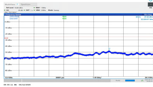
NTNV-n7-PC3-15-5-M-DFT-QPSK-Inner_1RB_Left-12000-26500- PASS
