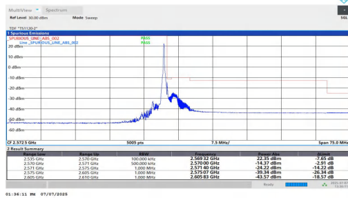
NTNV-n7-PC3-15-35-H-DFT-QPSK-Edge_1RB_Right-PASS
