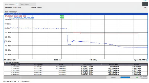
NTNV-n7-PC3-15-35-H-DFT-QPSK-Outer_Full-PASS
