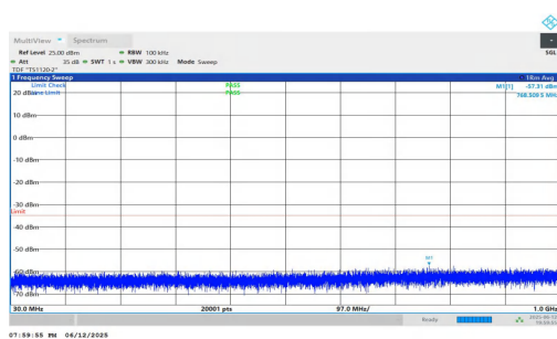
NTNV-n7-PC3-15-5-M-DFT-QPSK-Inner_1RB_Left-30-1000-PAS S
