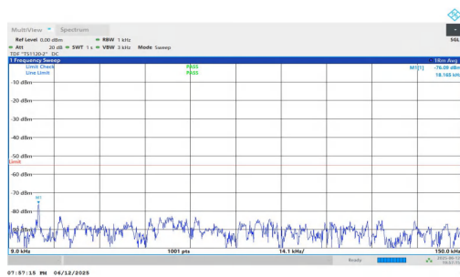
NTNV-n7-PC3-15-5-L-DFT-QPSK-Inner_1RB_Left-0.009-0.15-PA SS
