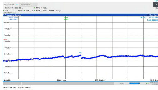
NTNV-n7-PC3-15-5-M-DFT-QPSK-Inner_1RB_Left-3000-12000- PASS
