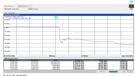
NTNV-n7-PC3-15-25-H-DFT-QPSK-Outer_Full-PASS
