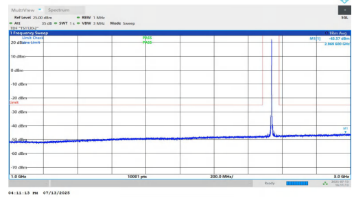
NTNV-n7-PC3-15-5-M-DFT-BPSK-Inner_1RB_Right-1000-3000-P ASS
