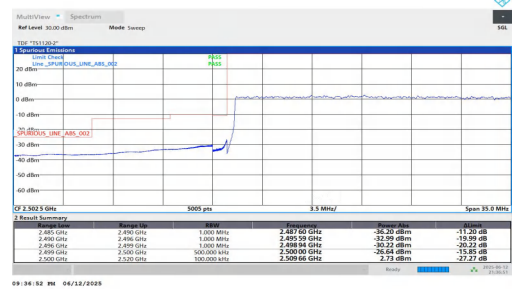
NTNV-n7-PC3-15-30-L-DFT-BPSK-Outer_Full-PASS
