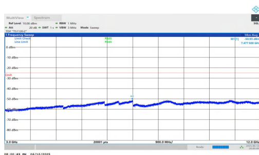
NTNV-n7-PC3-15-5-M-DFT-QPSK-Inner_1RB_Right-3000-12000 -PASS
