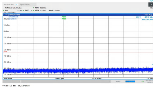
NTNV-n7-PC3-15-5-M-DFT-BPSK-Inner_1RB_Right-30-1000-PA SS
