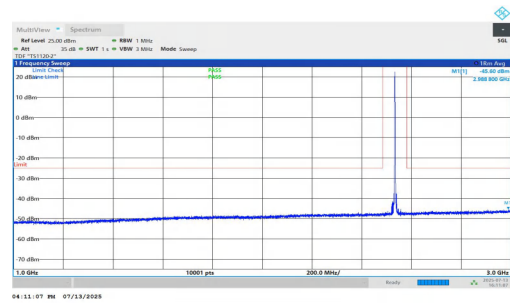
NTNV-n7-PC3-15-5-M-DFT-BPSK-Inner_1RB_Left-1000-3000-PASS
