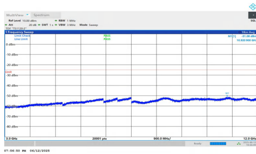
NTNV-n7-PC3-15-5-L-DFT-BPSK-Inner_1RB_Right-3000-12000- PASS
