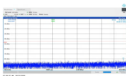
NTNV-n7-PC3-15-5-M-DFT-BPSK-Inner_1RB_Right-0.15-30-PASS
