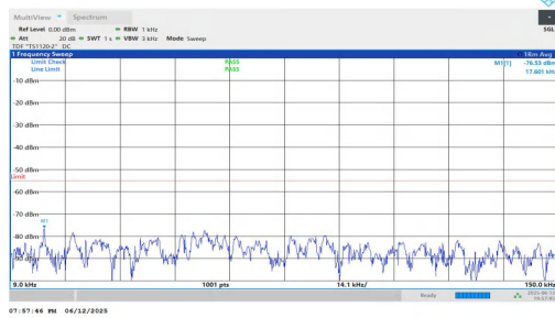
NTNV-n7-PC3-15-5-L-DFT-QPSK-Inner_1RB_Right-0.009-0.15-P ASS
