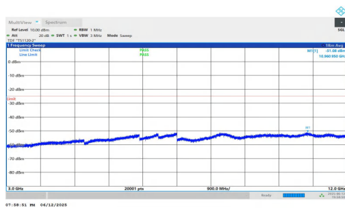
NTNV-n7-PC3-15-5-M-DFT-BPSK-Inner_1RB_Left-3000-12000-PASS
