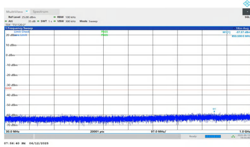
NTNV-n7-PC3-15-5-L-DFT-BPSK-Inner_1RB_Right-30-1000-PA SS
