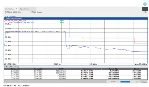
NTNV-n7-PC3-15-25-H-DFT-BPSK-Outer_Full-PASS
