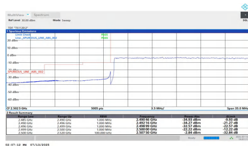
NTNV-n7-PC3-15-40-L-DFT-QPSK-Outer Full-PASS
