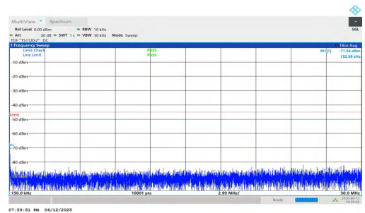
NTNV-n7-PC3-15-5-M-DFT-QPSK-Inner_1RB_Left-0.15-30-PASS
