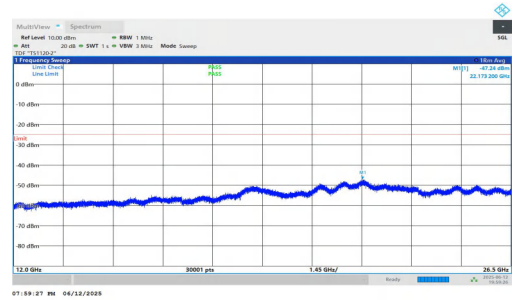
NTNV-n7-PC3-15-5-M-DFT-BPSK-Inner_1RB_Right-12000-26500 -PASS
