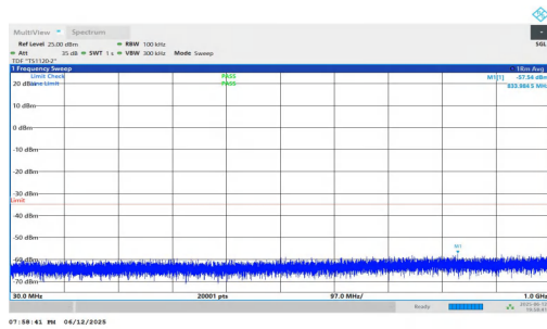
NTNV-n7-PC3-15-5-M-DFT-BPSK-Inner_1RB_Left-30-1000-PASS
