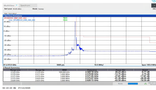
NTNV-n7-PC3-15-50-H-DFT-BPSK-Edge_1RB_Right-PASS
