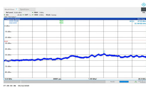
NTNV-n7-PC3-15-5-M-DFT-BPSK-Inner_1RB_Left-12000-26500-PASS
