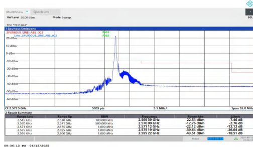
NTNV-n7-PC3-15-25-H-DFT-QPSK-Edge_1RB_Right-PASS
