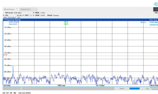
NTNV-n7-PC3-15-5-M-DFT-QPSK-Inner_1RB_Right-0.009-0.15- PASS
