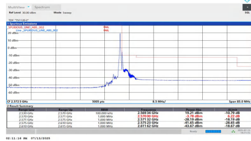
NTNV-n7-PC3-15-40-H-DFT-QPSK-Edge_1RB_Right
