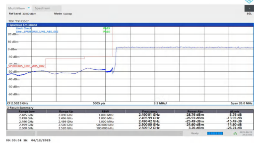
NTNV-n7-PC3-15-25-L-DFT-BPSK-Outer_Full-PASS
