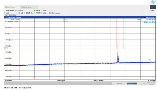
NTNV-n7-PC3-15-5-L-DFT-BPSK-Inner_1RB_Right-1000-3000-PA SS
