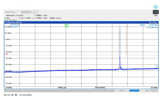
NTNV-n7-PC3-15-5-L-DFT-QPSK-Inner_1RB_Left-1000-3000-PA SS
