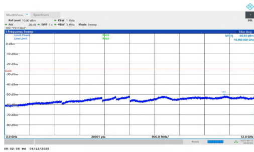
NTNV-n7-PC3-15-5-H-DFT-BPSK-Inner_1RB_Right-3000-12000- PASS
