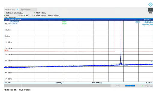
NTNV-n7-PC3-15-5-H-DFT-QPSK-Inner_1RB_Left-1000-3000-PASS
