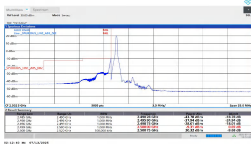
NTNV-n7-PC3-15-50-L-DFT-BPSK-Edge_1RB_Left
