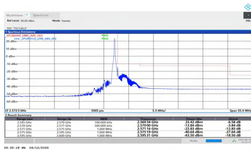
NTNV-n7-PC3-15-25-H-DFT-BPSK-Edge_1RB_Right-PASS
