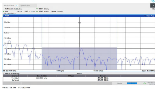
NTNV-n7-PC3-15-40-H-DFT-QPSK-Edge_1RB_Right-PASS
