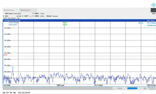
NTNV-n7-PC3-15-5-H-DFT-QPSK-Inner_1RB_Left-0.009-0.15-P ASS
