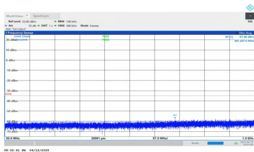
NTNV-n7-PC3-15-5-H-DFT-QPSK-Inner_1RB_Left-30-1000-PAS S
