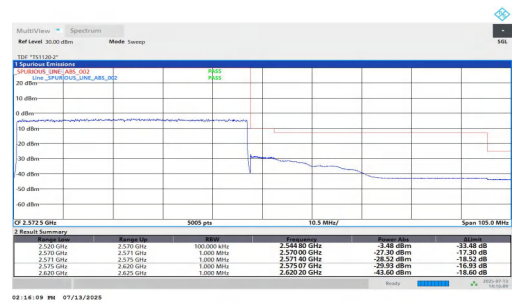
NTNV-n7-PC3-15-50-H-DFT-QPSK-Outer_Full-PASS
