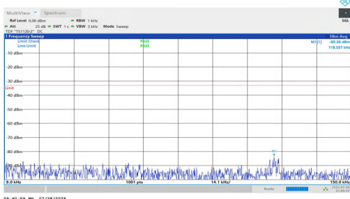
NTNV-n5-PC2-15-15-M-DFT-BPSK-Inner_1RB_Right-0.009-0.15-PA SS
