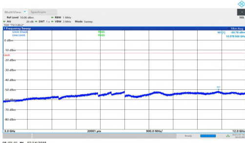
NTNV-n5-PC2-15-15-M-DFT-BPSK-Inner_1RB_Left-3000-12000-PAS S
