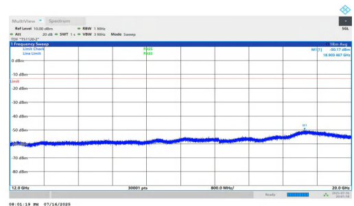
NTNV-n5-PC2-15-15-L-DFT-QPSK-Inner_1RB_Right-12000-20000-PA
