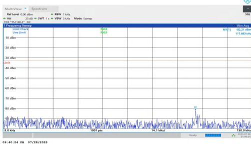
NTNV-n5-PC2-15-15-L-DFT-QPSK-Inner_1RB_Right-0.009-0.15-PAS
