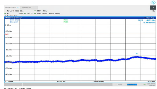
NTNV-n5-PC2-15-15-M-DFT-BPSK-Inner_1RB_Left-12000-20000-PAS S
