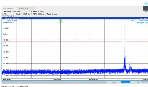
NTNV-n5-PC2-15-15-M-DFT-QPSK-Inner_1RB_Right-30-1000-PASS
