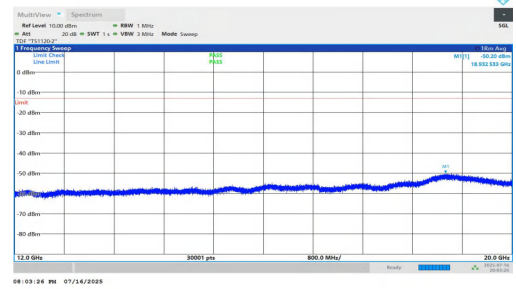
NTNV-n5-PC2-15-15-M-DFT-QPSK-Inner_1RB_Left-12000-20000-PA SS
