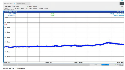
NTNV-n5-PC2-15-15-L-DFT-QPSK-Inner_1RB_Left-12000-20000-PAS
