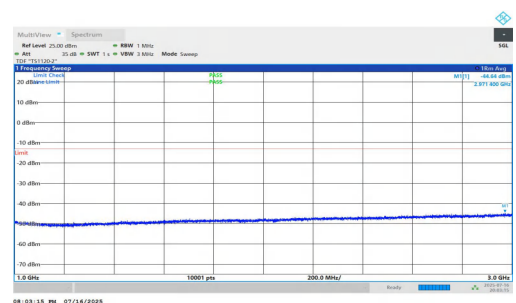
NTNV-n5-PC2-15-15-M-DFT-QPSK-Inner_1RB_Left-1000-3000-PASS
