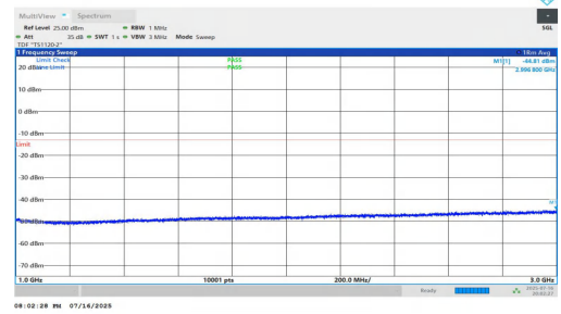
NTNV-n5-PC2-15-15-M-DFT-BPSK-Inner_1RB_Right-1000-3000-PASS S
