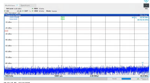
NTNV-n5-PC2-15-15-M-DFT-BPSK-Inner_1RB_Right-0.15-30-PASS
