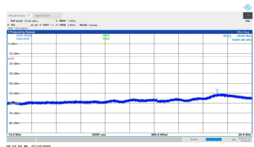
NTNV-n5-PC2-15-15-M-DFT-QPSK-Inner_1RB_Right-12000-20000-P ASS
