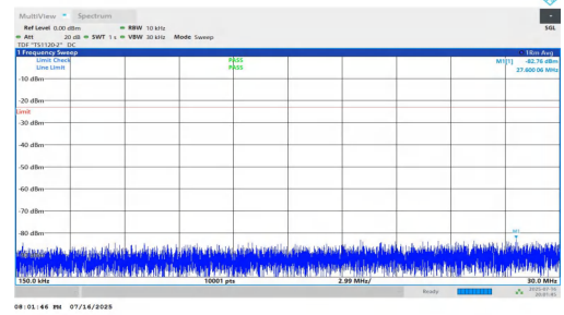
NTNV-n5-PC2-15-15-M-DFT-BPSK-Inner_1RB_Left-0.15-30-PASS
