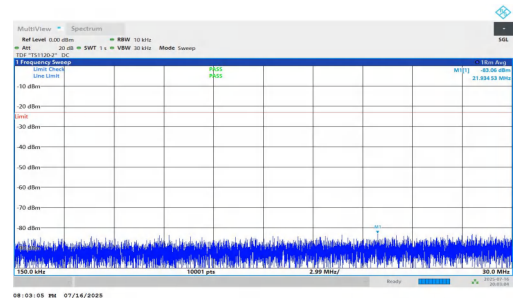
NTNV-n5-PC2-15-15-M-DFT-QPSK-Inner_1RB_Left-0.15-30-PASS
