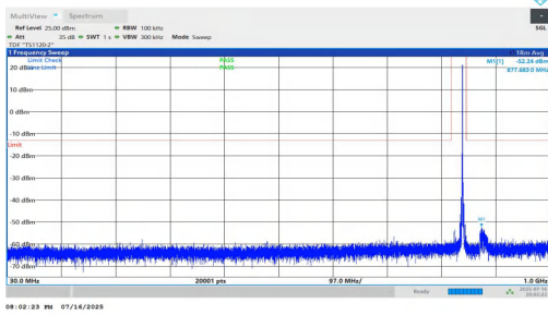
NTNV-n5-PC2-15-15-M-DFT-BPSK-Inner_1RB_Right-30-1000-PASS
