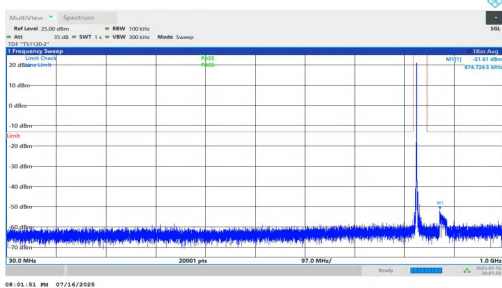
NTNV-n5-PC2-15-15-M-DFT-BPSK-Inner_1RB_Left-30-1000-PASS
