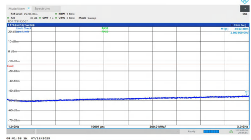
NTNV-n5-PC2-15-15-M-DFT-BPSK-Inner_1RB_Left-1000-3000-PASS
