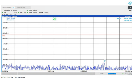
NTNV-n5-PC2-15-15-M-DFT-QPSK-Inner_1RB_Left-0.009-0.15-PASS S
