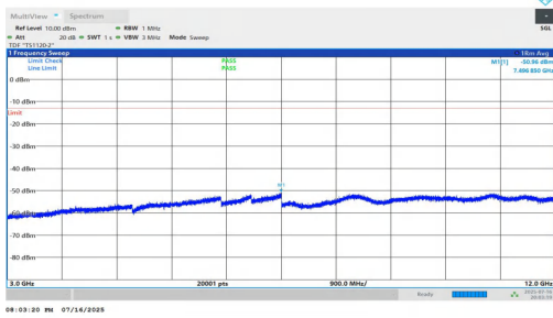
NTNV-n5-PC2-15-15-M-DFT-QPSK-Inner_1RB_Left-3000-12000-PA SS
