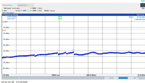
NTNV-n5-PC2-15-15-M-DFT-BPSK-Inner_1RB_Right-3000-12000-PASS SS
