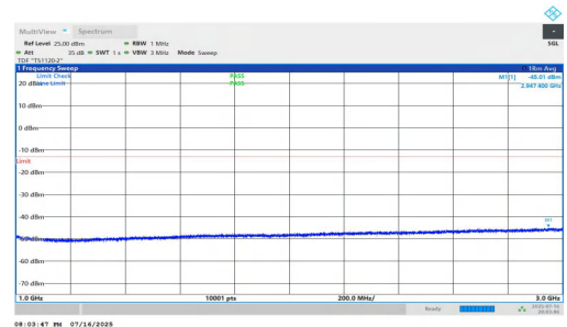
NTNV-n5-PC2-15-15-M-DFT-QPSK-Inner_1RB_Right-1000-3000-PASS S
