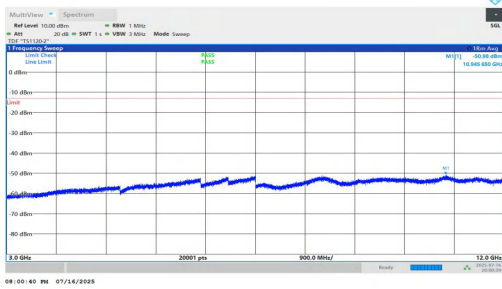
NTNV-n5-PC2-15-15-L-DFT-QPSK-Inner_1RB_Left-3000-12000-PAS
