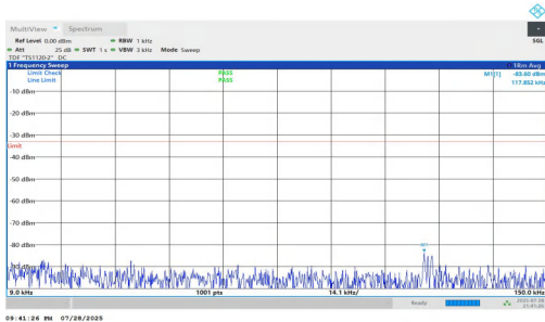
NTNV-n5-PC2-15-15-M-DFT-QPSK-Inner_1RB_Right-0.009-0.15-PA SS
