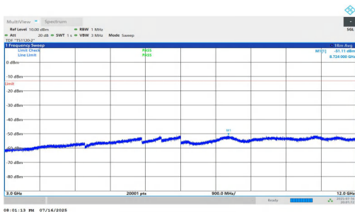
NTNV-n5-PC2-15-15-L-DFT-QPSK-Inner_1RB_Right-3000-12000-PA
