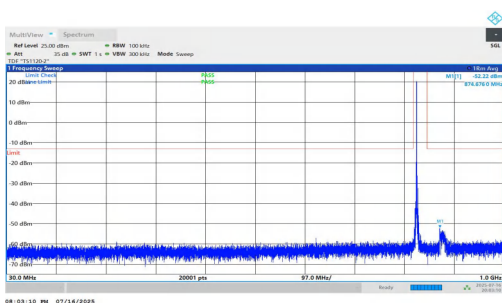
NTNV-n5-PC2-15-15-M-DFT-QPSK-Inner_1RB_Left-30-1000-PASS
