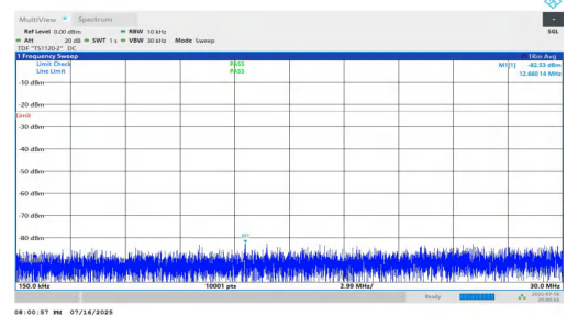
NTNV-n5-PC2-15-15-L-DFT-QPSK-Inner_1RB_Right-0.15-30-PASS
