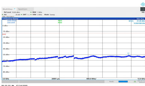
NTNV-n5-PC2-15-15-M-DFT-QPSK-Inner_1RB_Right-3000-12000-P ASS
