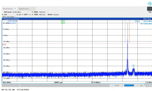
NTNV-n5-PC2-15-15-L-DFT-QPSK-Inner_1RB_Right-30-1000-PASS
