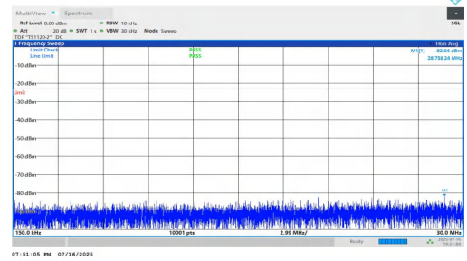
NTNV-n5-PC2-15-10-L-DFT-BPSK-Inner_1RB_Left-0.15-30-PASS
