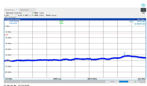
NTVN-n5-PC2-15-10-H-DFT-QPSK-Inner_1RB_Right-12000-20000-PA
