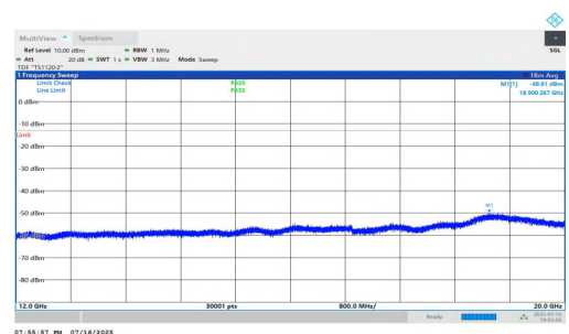
NTNV-n5-PC2-15-10-M-DFT-QPSK-Inner_1RB_Right-12000-20000-P ASS
