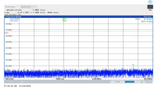
NTNV-n5-PC2-15-10-M-DFT-QPSK-Inner_1RB_Right-0.15-30-PASS
