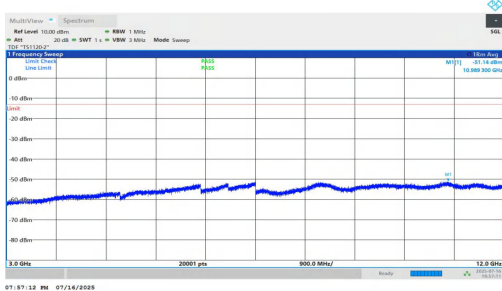
NTNV-n5-PC2-15-10-H-DFT-BPSK-Inner_1RB_Right-3000-12000-PASS SS
