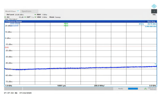
NTNV-n5-PC2-15-10-H-DFT-QPSK-Inner_1RB_Left-1000-3000-PASS
