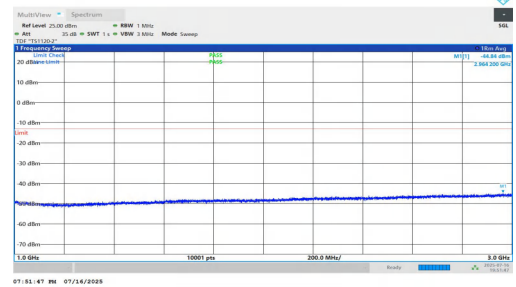
NTNV-n5-PC2-15-10-L-DFT-BPSK-Inner_1RB_Right-1000-3000-PASS
