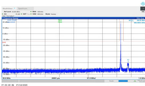
NTNV-n5-PC2-15-10-M-DFT-BPSK-Inner_1RB_Left-30-1000-PASS
