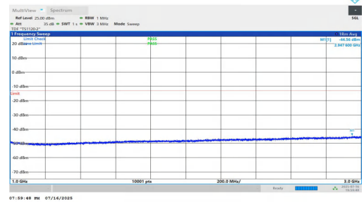
NTNV-n5-PC2-15-15-L-DFT-BPSK-Inner_1RB_Right-1000-3000-PASS
