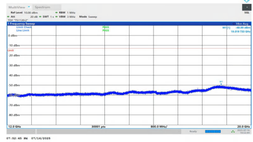
NTNV-n5-PC2-15-10-L-DFT-QPSK-Inner_1RB_Left-12000-20000-PAS
