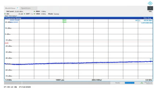
NTNV-n5-PC2-15-10-M-DFT-QPSK-Inner_1RB_Left-1000-3000-PASS
