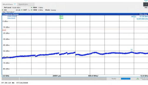
NTNV-n5-PC2-15-10-M-DFT-QPSK-Inner_1RB_Left-3000-12000-PA SS
