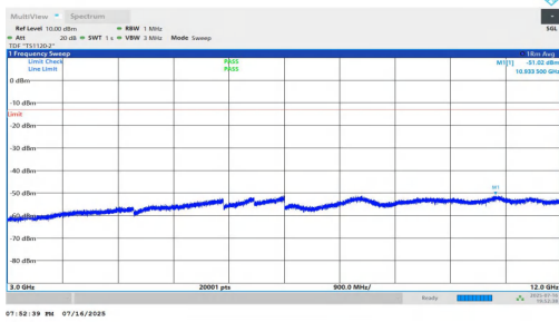
NTNV-n5-PC2-15-10-L-DFT-QPSK-Inner_1RB_Left-3000-12000-PAS
