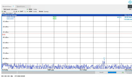
NTNV-n5-PC2-15-5-H-DFT-QPSK-Inner_1RB_Left-0.009-0.15-PASS
