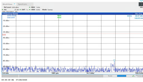
NTNV-n5-PC2-15-5-H-DFT-BPSK-Inner_1RB_Left-0.009-0.15-PASS
