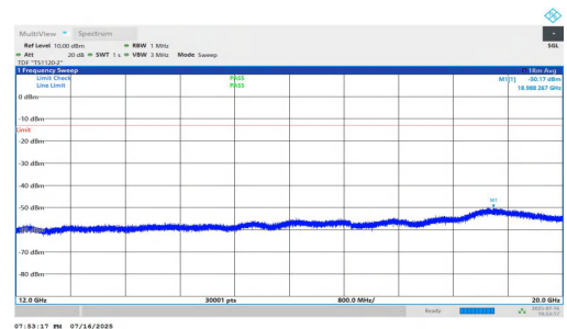
NTNV-n5-PC2-15-10-L-DFT-QPSK-Inner_1RB_Right-12000-20000-PA
