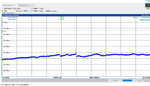
NTNV-n5-PC2-15-5-H-DFT-BPSK-Inner_1RB_Right-3000-12000-PAS
