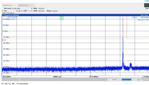
NTNV-n5-PC2-15-15-L-DFT-BPSK-Inner_1RB_Left-30-1000-PASS
