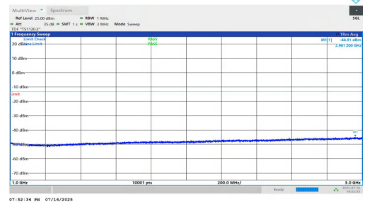
NTNV-n5-PC2-15-10-L-DFT-QPSK-Inner_1RB_Left-1000-3000-PASS
