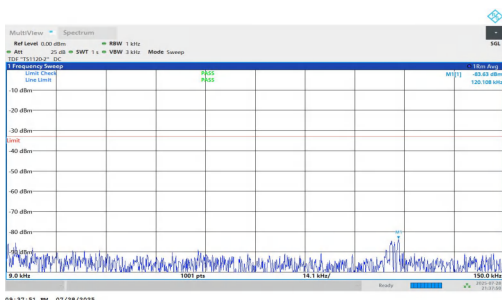
NTNV-n5-PC2-15-10-M-DFT-BPSK-Inner_1RB_Right-0.009-0.15-PA SS
