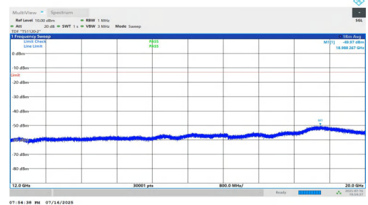
NTNV-n5-PC2-15-10-M-DFT-BPSK-Inner_1RB_Right-12000-20000-PASS
