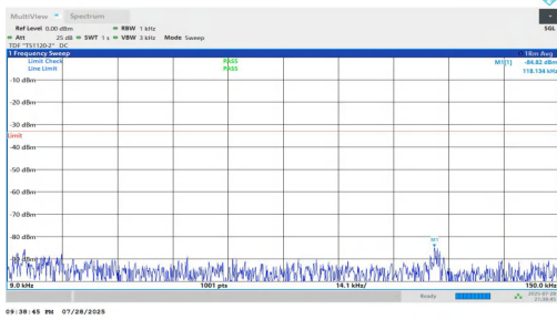
NTNV-n5-PC2-15-10-H-DFT-BPSK-Inner_1RB_Left-0.009-0.15-PASS
