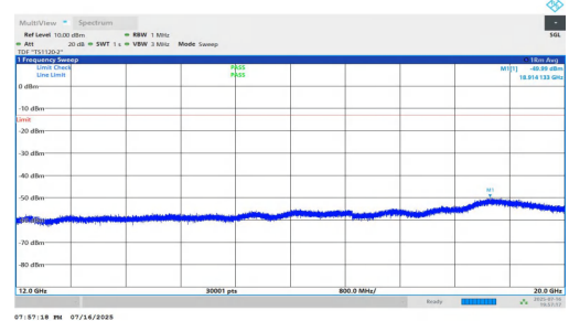
NTNV-n5-PC2-15-10-H-DFT-BPSK-Inner_1RB_Right-12000-20000-PASS SS
