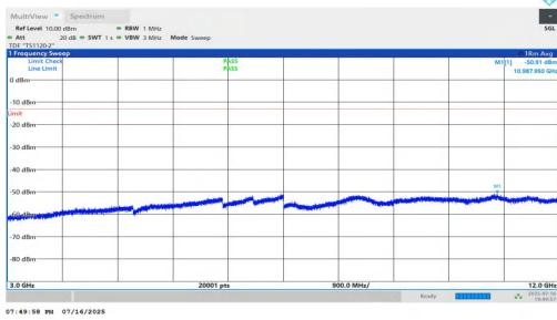
NTNV-n5-PC2-15-5-H-DFT-QPSK-Inner_1RB_Left-3000-12000-PAS
