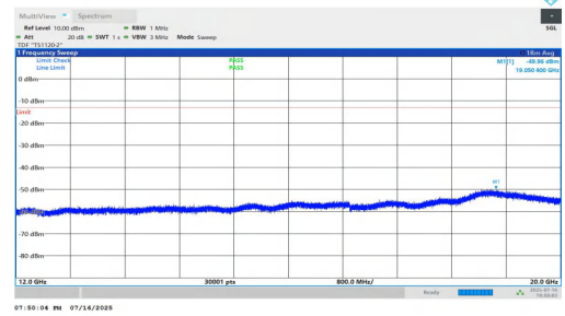
NTNV-n5-PC2-15-5-H-DFT-QPSK-Inner_1RB_Left-12000-20000-PAS
