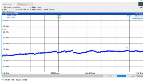
NTVN-n5-PC2-15-10-H-DFT-QPSK-Inner_1RB_Left-3000-12000-PAS
