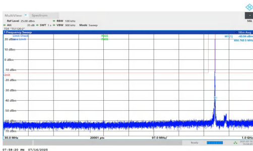
NTVN-n5-PC2-15-10-H-DFT-QPSK-Inner_1RB_Right-30-1000-PASS
