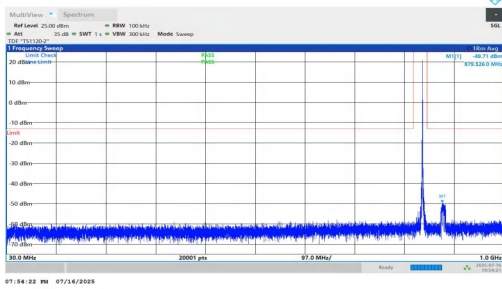
NTNV-n5-PC2-15-10-M-DFT-BPSK-Inner_1RB_Right-30-1000-PASS
