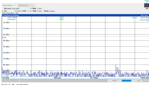
NTNV-n5-PC2-15-15-L-DFT-QPSK-Inner_1RB_Left-0.009-0.15-PASS
