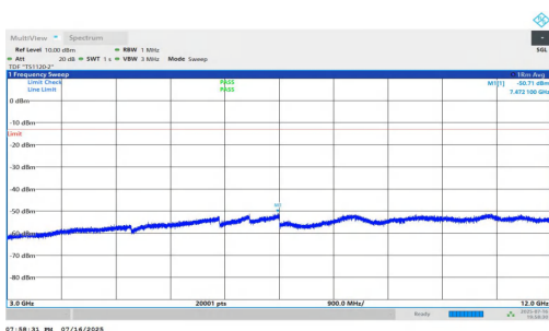
NTVN-n5-PC2-15-10-H-DFT-QPSK-Inner_1RB_Right-3000-12000-PA
