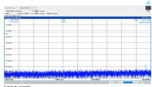
NTNV-n5-PC2-15-10-H-DFT-BPSK-Inner_1RB_Right-0.15-30-PASS
