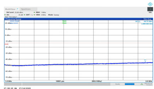
NTVN-n5-PC2-15-10-H-DFT-QPSK-Inner_1RB_Right-1000-3000-PAS
