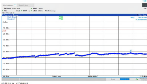
NTNV-n5-PC2-15-15-L-DFT-BPSK-Inner_1RB_Right-3000-12000-PA SS
