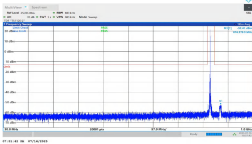
NTNV-n5-PC2-15-10-L-DFT-BPSK-Inner_1RB_Right-30-1000-PASS
