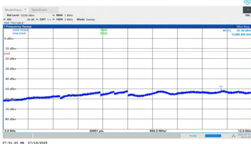
NTNV-n5-PC2-15-10-L-DFT-BPSK-Inner_1RB_Left-3000-12000-PAS
