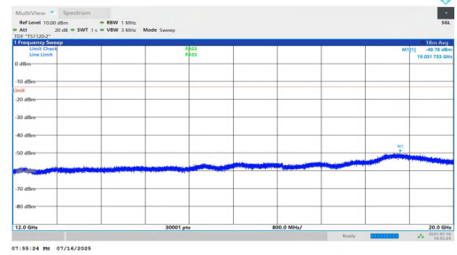
NTNV-n5-PC2-15-10-M-DFT-QPSK-Inner_1RB_Left-12000-20000-PA SS
