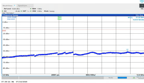
NTNV-n5-PC2-15-15-L-DFT-BPSK-Inner_1RB_Left-3000-12000-PAS
