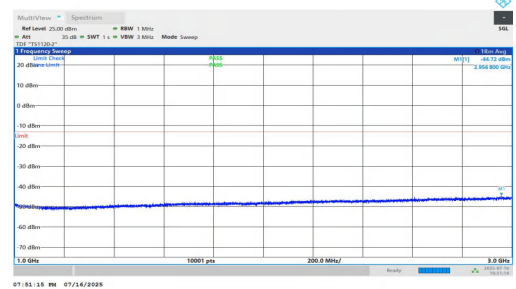
NTNV-n5-PC2-15-10-L-DFT-BPSK-Inner_1RB_Left-1000-3000-PASS
