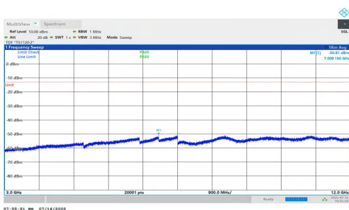
NTNV-n5-PC2-15-10-M-DFT-QPSK-Inner_1RB_Right-3000-12000-P ASS
