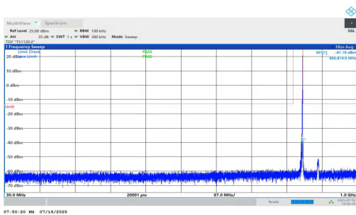
NTNV-n5-PC2-15-5-H-DFT-QPSK-Inner_1RB_Right-30-1000-PASS
