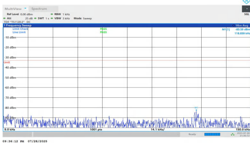
NTNV-n5-PC2-15-5-H-DFT-QPSK-Inner_1RB_Right-0.009-0.15-PAS
