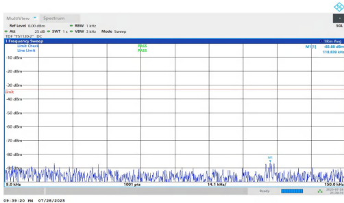
NTVN-n5-PC2-15-10-H-DFT-QPSK-Inner_1RB_Right-0.009-0.15-PA
