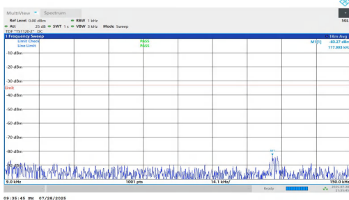
NTNV-n5-PC2-15-5-H-DFT-BPSK-Inner_1RB_Right-0.009-0.15-PAS
