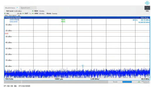
NTNV-n5-PC2-15-10-L-DFT-QPSK-Inner_1RB_Right-0.15-30-PASS
