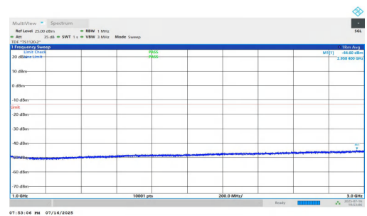
NTNV-n5-PC2-15-10-L-DFT-QPSK-Inner_1RB_Right-1000-3000-PASS
