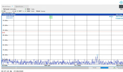
NTNV-n5-PC2-15-10-L-DFT-QPSK-Inner_1RB_Right-0.009-0.15-PAS
