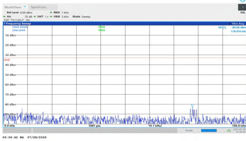
NTNV-n5-PC2-15-10-L-DFT-BPSK-Inner_1RB_Left-0.009-0.15-PASS
