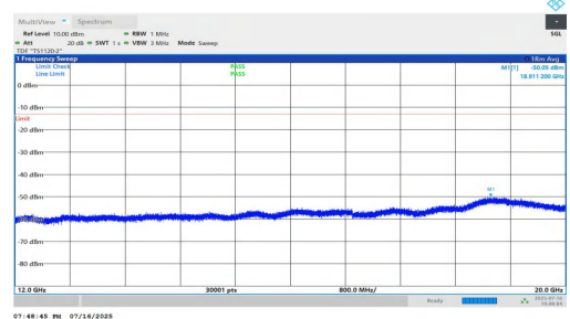
NTNV-n5-PC2-15-5-H-DFT-BPSK-Inner_1RB_Left-12000-20000-PASS
