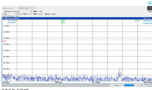
NTNV-n5-PC2-15-10-H-DFT-BPSK-Inner_1RB_Right-0.009-0.15-PAS
