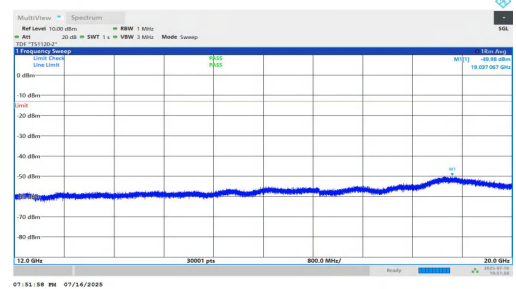
NTNV-n5-PC2-15-10-L-DFT-BPSK-Inner_1RB_Right-12000-20000-PA SS
