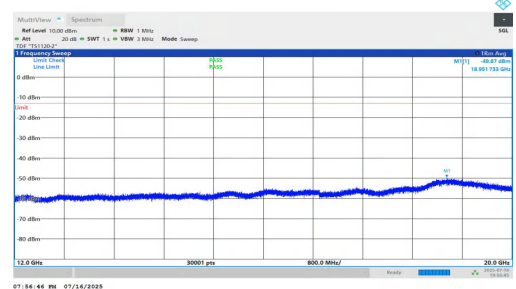
NTNV-n5-PC2-15-10-H-DFT-BPSK-Inner_1RB_Left-12000-20000-PAS
