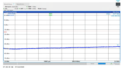
NTNV-n5-PC2-15-10-H-DFT-BPSK-Inner_1RB_Left-1000-3000-PASS
