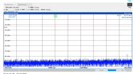
NTNV-n5-PC2-15-15-L-DFT-QPSK-Inner_1RB_Left-0.15-30-PASS
