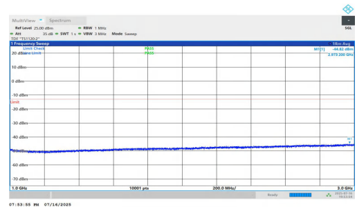
NTNV-n5-PC2-15-10-M-DFT-BPSK-Inner_1RB_Left-1000-3000-PASS
