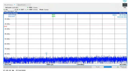
NTNV-n5-PC2-15-10-M-DFT-QPSK-Inner_1RB_Left-0.15-30-PASS
