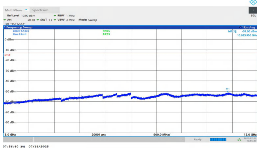
NTNV-n5-PC2-15-10-H-DFT-BPSK-Inner_1RB_Left-3000-12000-PAS
