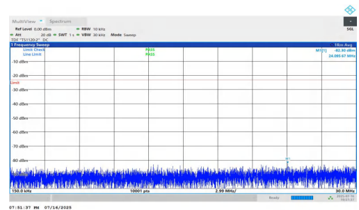
NTNV-n5-PC2-15-10-L-DFT-BPSK-Inner_1RB_Right-0.15-30-PASS
