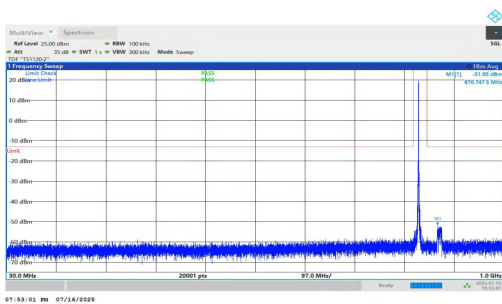
NTNV-n5-PC2-15-10-L-DFT-QPSK-Inner_1RB_Right-30-1000-PASS
