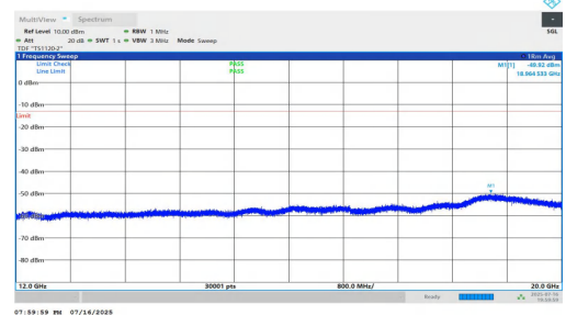
NTNV-n5-PC2-15-15-L-DFT-BPSK-Inner_1RB_Right-12000-20000-PA SS
