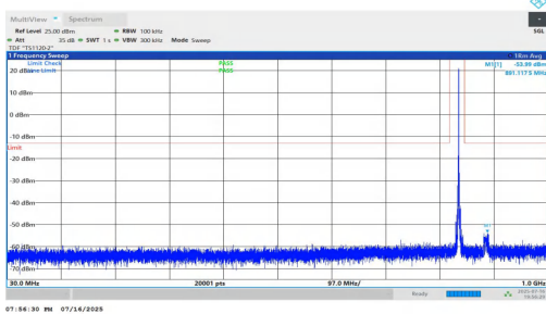
NTNV-n5-PC2-15-10-H-DFT-BPSK-Inner_1RB_Left-30-1000-PASS
