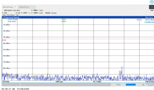
NTNV-n5-PC2-15-10-M-DFT-QPSK-Inner_1RB_Right-0.009-0.15-PA SS
