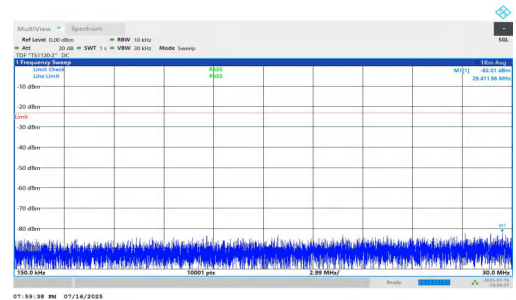
NTNV-n5-PC2-15-15-L-DFT-BPSK-Inner_1RB_Right-0.15-30-PASS
