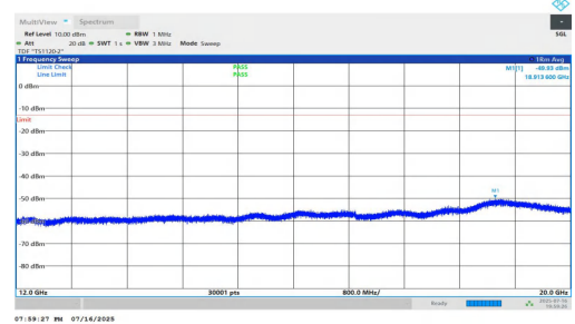
NTNV-n5-PC2-15-15-L-DFT-BPSK-Inner_1RB_Left-12000-20000-PAS
