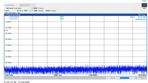
NTNV-n5-PC2-15-5-H-DFT-QPSK-Inner_1RB_Right-0.15-30-PASS
