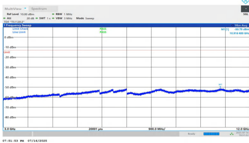
NTNV-n5-PC2-15-10-L-DFT-BPSK-Inner_1RB_Right-3000-12000-PA SS
