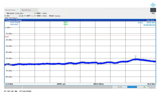
NTNV-n5-PC2-15-5-H-DFT-QPSK-Inner_1RB_Right-12000-20000-PA
