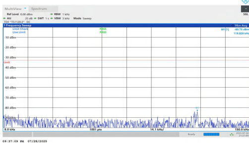
NTNV-n5-PC2-15-10-L-DFT-QPSK-Inner_1RB_Left-0.009-0.15-PASS
