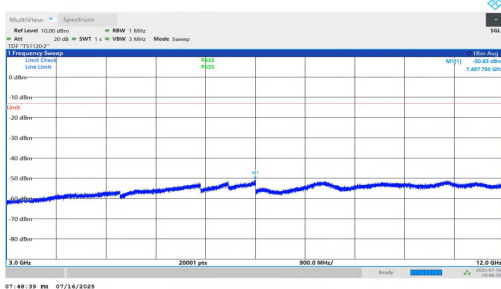
NTNV-n5-PC2-15-5-H-DFT-BPSK-Inner_1RB_Left-3000-12000-PASS
