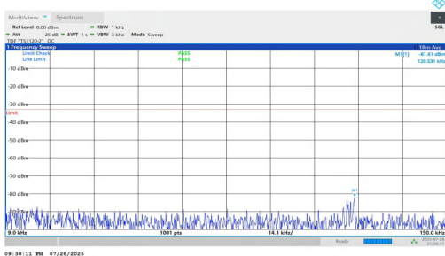
NTNV-n5-PC2-15-10-M-DFT-QPSK-Inner_1RB_Left-0.009-0.15-PASS
