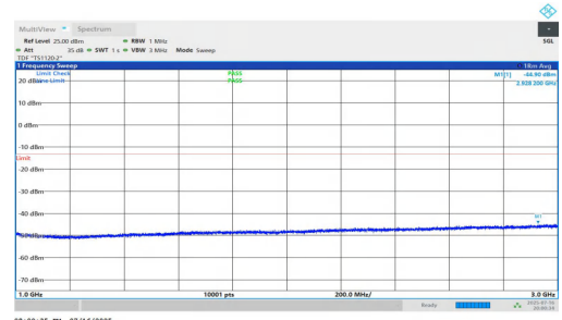
NTNV-n5-PC2-15-15-L-DFT-QPSK-Inner_1RB_Left-1000-3000-PASS
