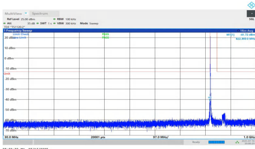
NTNV-n5-PC2-15-15-L-DFT-QPSK-Inner_1RB_Left-30-1000-PASS
