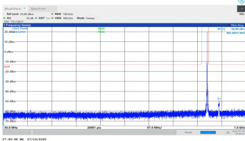
NTNV-n5-PC2-15-5-H-DFT-QPSK-Inner_1RB_Left-30-1000-PASS
