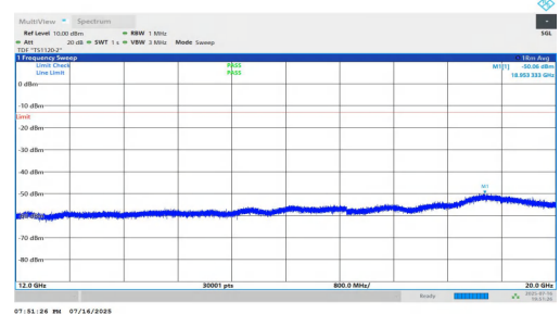
NTNV-n5-PC2-15-10-L-DFT-BPSK-Inner_1RB_Left-12000-20000-PAS
