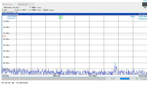
NTNV-n5-PC2-15-15-L-DFT-BPSK-Inner_1RB_Left-0.009-0.15-PASS
