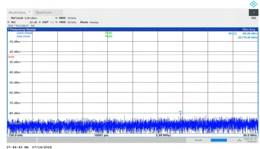
NTNV-n5-PC2-15-5-H-DFT-QPSK-Inner_1RB_Left-0.15-30-PASS
