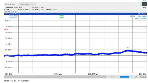
NTVN-n5-PC2-15-10-H-DFT-QPSK-Inner_1RB_Left-12000-20000-PAS
