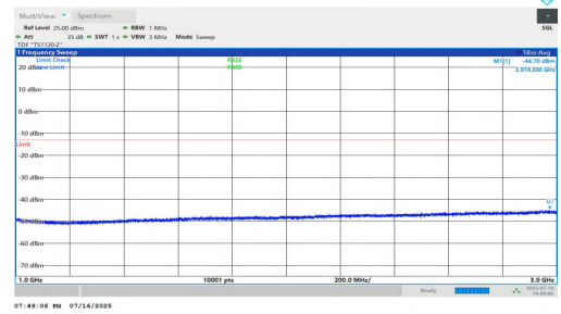
NTNV-n5-PC2-15-5-H-DFT-BPSK-Inner_1RB_Right-1000-3000-PASS
