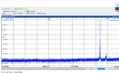
NTNV-n5-PC2-15-10-H-DFT-QPSK-Inner_1RB_Left-30-1000-PASS
