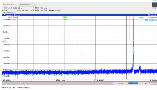
NTNV-n5-PC2-15-10-H-DFT-BPSK-Inner_1RB_Right-30-1000-PASS
