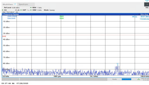
NTNV-n5-PC2-15-10-M-DFT-BPSK-Inner_1RB_Left-0.009-0.15-PAS S
