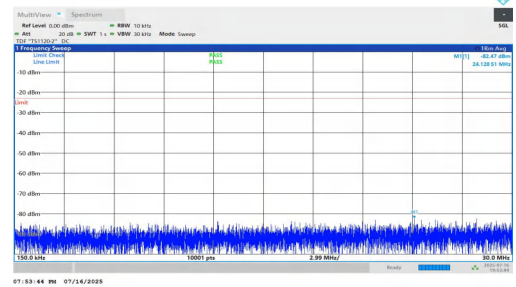
NTNV-n5-PC2-15-10-M-DFT-BPSK-Inner_1RB_Left-0.15-30-PASS
