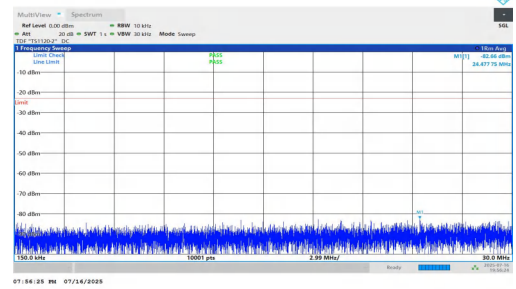
NTNV-n5-PC2-15-10-H-DFT-BPSK-Inner_1RB_Left-0.15-30-PASS
