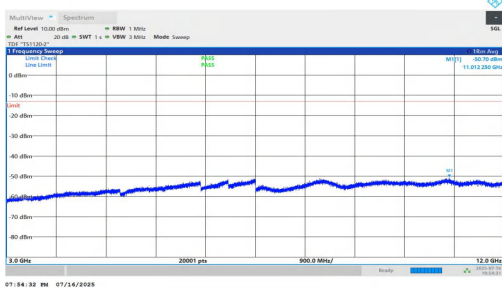
NTNV-n5-PC2-15-10-M-DFT-BPSK-Inner_1RB_Right-3000-12000-PASS
