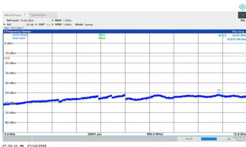
NTNV-n5-PC2-15-10-L-DFT-QPSK-Inner_1RB_Right-3000-12000-PA
