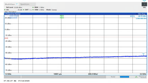
NTNV-n5-PC2-15-10-M-DFT-BPSK-Inner_1RB_Right-1000-3000-PASS
