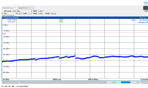
NTNV-n5-PC2-15-10-M-DFT-BPSK-Inner_1RB_Left-3000-12000-PAS S
