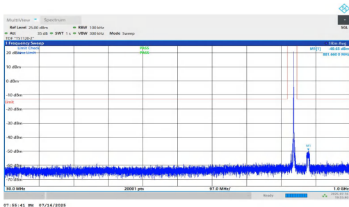
NTNV-n5-PC2-15-10-M-DFT-QPSK-Inner_1RB_Right-30-1000-PASS
