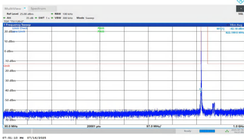
NTNV-n5-PC2-15-10-L-DFT-BPSK-Inner_1RB_Left-30-1000-PASS
