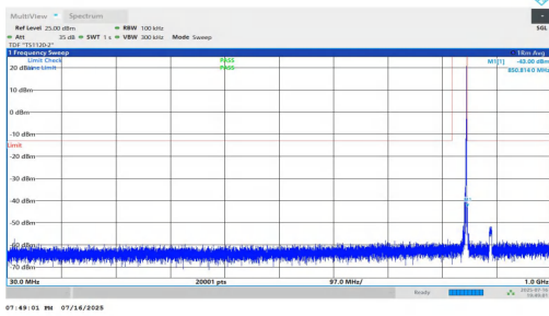
NTNV-n5-PC2-15-5-H-DFT-BPSK-Inner_1RB_Right-30-1000-PASS
