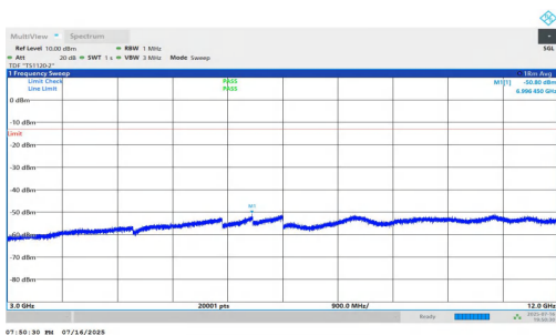
NTNV-n5-PC2-15-5-H-DFT-QPSK-Inner_1RB_Right-3000-12000-PA
