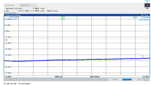
NTNV-n5-PC2-15-5-H-DFT-BPSK-Inner_1RB_Left-1000-3000-PASS
