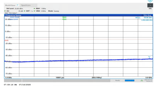
NTNV-n5-PC2-15-15-L-DFT-BPSK-Inner_1RB_Left-1000-3000-PASS
