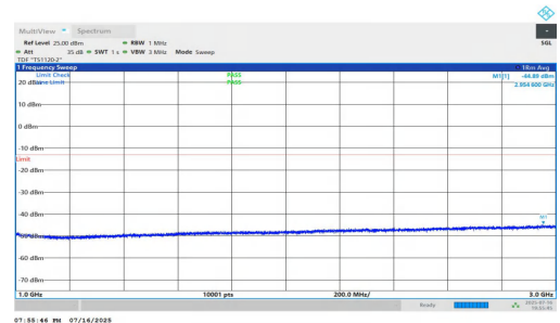
NTNV-n5-PC2-15-10-M-DFT-QPSK-Inner_1RB_Right-1000-3000-PASS S
