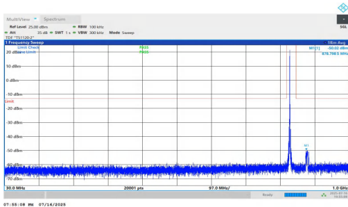
NTNV-n5-PC2-15-10-M-DFT-QPSK-Inner_1RB_Left-30-1000-PASS
