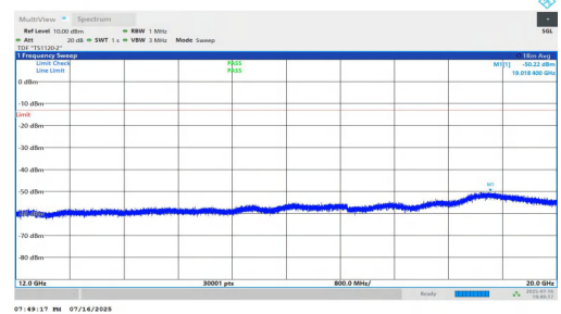
NTNV-n5-PC2-15-5-H-DFT-BPSK-Inner_1RB_Right-12000-20000-PAS
