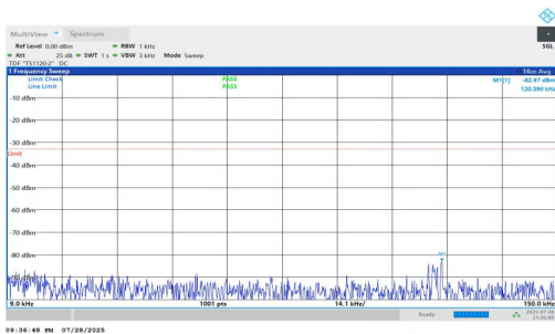
NTNV-n5-PC2-15-10-L-DFT-BPSK-Inner_1RB_Right-0.009-0.15-PAS
