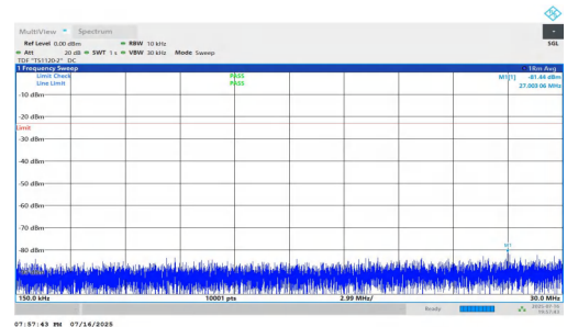
NTNV-n5-PC2-15-10-H-DFT-QPSK-Inner_1RB_Left-0.15-30-PASS
