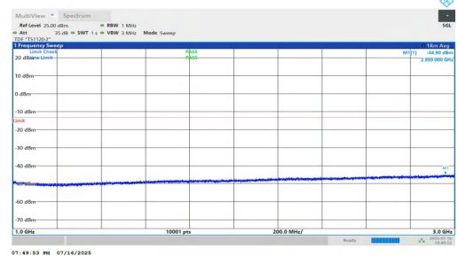
NTNV-n5-PC2-15-5-H-DFT-QPSK-Inner_1RB_Left-1000-3000-PASS
