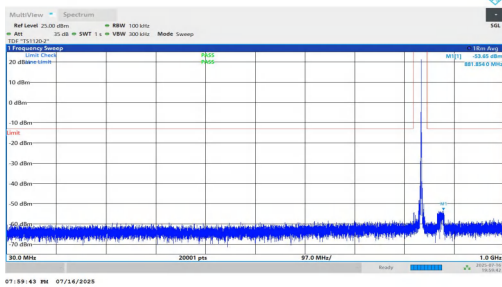
NTNV-n5-PC2-15-15-L-DFT-BPSK-Inner_1RB_Right-30-1000-PASS
