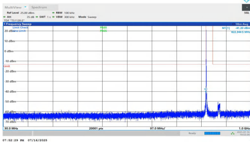
NTNV-n5-PC2-15-10-L-DFT-QPSK-Inner_1RB_Left-30-1000-PASS
