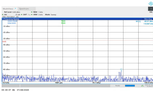
NTNV-n5-PC2-15-15-L-DFT-BPSK-Inner_1RB_Right-0.009-0.15-PAS
