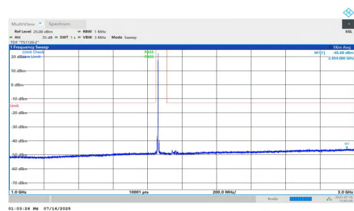
NTNV-n2-PC2-15-40-M-DFT-QPSK-Inner_1RB_Left-1000-3000-P ASS
