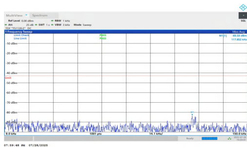
NTNV-n2-PC2-15-40-L-DFT-QPSK-Inner_1RB_Right-0.009-0.15- PASS
