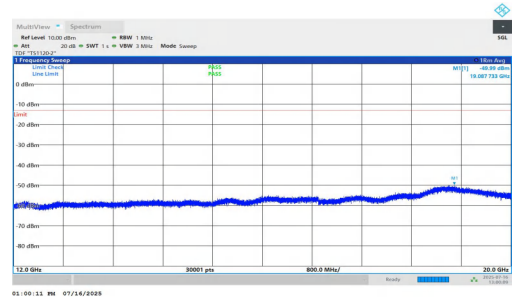
NTVN-n2-PC2-15-40-L-DFT-BPSK-Inner_1RB_Right-12000-2000 0-PASS
