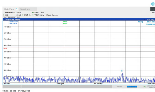
NTNV-n2-PC2-15-40-H-DFT-QPSK-Inner_1RB_Right-0.009-0.15-PASS
