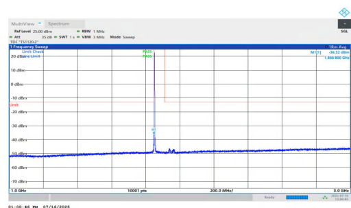
NTVN-n2-PC2-15-40-L-DFT-QPSK-Inner_1RB_Left-1000-3000-PA SS
