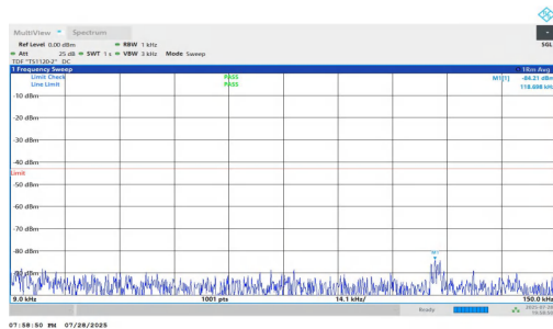
NTNV-n2-PC2-15-35-H-DFT-QPSK-Inner_1RB_Right-0.009-0.15-PASS
