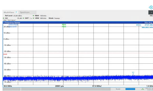
NTNV-n2-PC2-15-40-H-DFT-QPSK-Inner_1RB_Left-30-1000-P ASS
