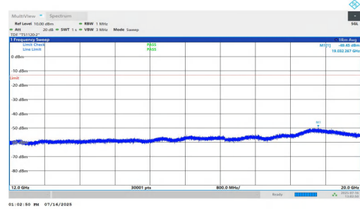
NTNV-n2-PC2-15-40-M-DFT-BPSK-Inner_1RB_Right-12000-2000 0-PASS
