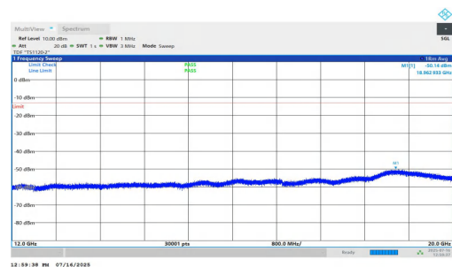
NTNV-n2-PC2-15-40-L-DFT-BPSK-Inner_1RB_Left-12000-20000- PASS
