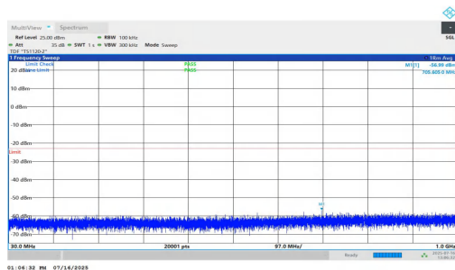
NTNV-n2-PC2-15-40-H-DFT-QPSK-Inner_1RB_Right-30-1000-PASS
