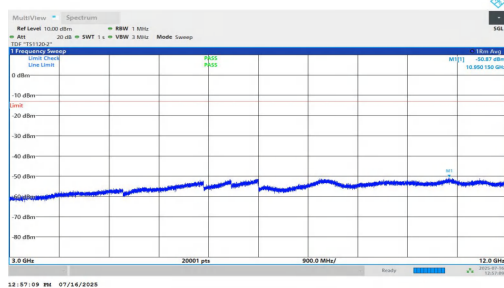
NTNV-n2-PC2-15-35-H-DFT-BPSK-Inner_1RB_Right-3000-1200 0-PASS
