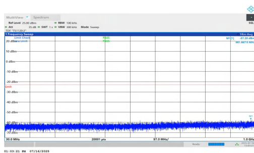
NTNV-n2-PC2-15-40-M-DFT-QPSK-Inner_1RB_Left-30-1000-PA SS
