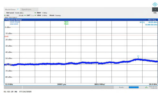
NTNV-n2-PC2-15-40-M-DFT-BPSK-Inner_1RB_Left-12000-20000-PASS
