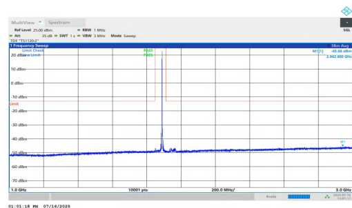
NTNV-n2-PC2-15-40-L-DFT-QPSK-Inner_1RB_Right-1000-3000-P ASS
