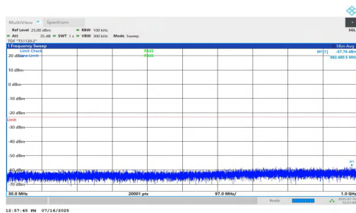
NTNV-n2-PC2-15-35-H-DFT-QPSK-Inner_1RB_Left-30-1000-PA SS
