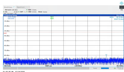
NTNV-n2-PC2-15-40-H-DFT-BPSK-Inner_1RB_Right-0.15-30-PASS
