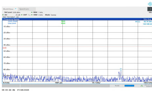
NTNV-n2-PC2-15-40-M-DFT-QPSK-Inner_1RB_Right-0.009-0.15 -PASS
