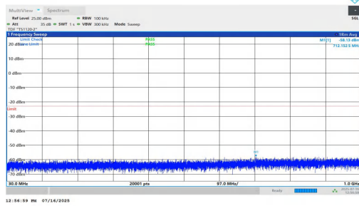
NTNV-n2-PC2-15-35-H-DFT-BPSK-Inner_1RB_Right-30-1000-P ASS
