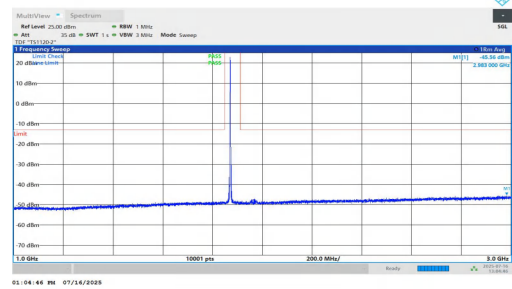
NTNV-n2-PC2-15-40-H-DFT-BPSK-Inner_1RB_Left-1000-3000-PASS
