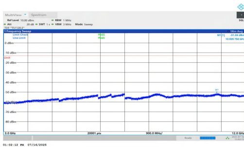
NTNV-n2-PC2-15-40-M-DFT-BPSK-Inner_1RB_Left-3000-12000-PASS
