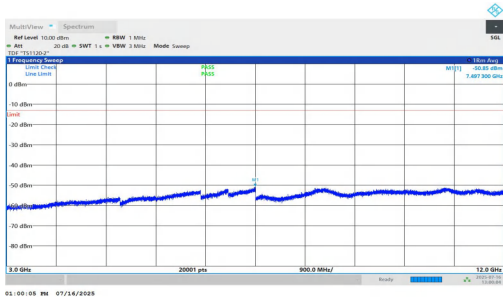
NTVN-n2-PC2-15-40-L-DFT-BPSK-Inner_1RB_Right-3000-12000 -PASS
