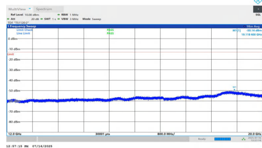
NTNV-n2-PC2-15-35-H-DFT-BPSK-Inner_1RB_Right-12000-2000 0-PASS
