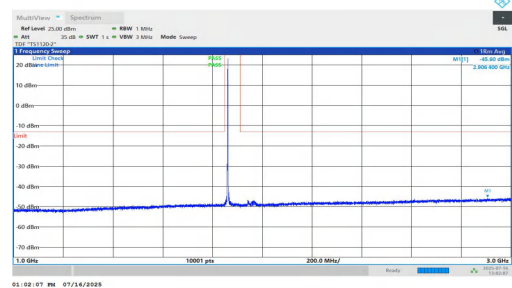
NTNV-n2-PC2-15-40-M-DFT-BPSK-Inner_1RB_Left-1000-3000-P ASS
