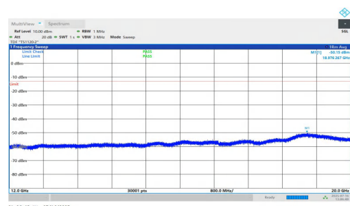
NTNV-n2-PC2-15-40-H-DFT-QPSK-Inner_1RB_Right-12000-20000-PASS
