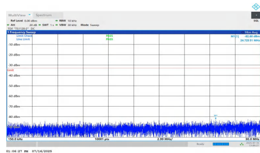
NTNV-n2-PC2-15-40-H-DFT-QPSK-Inner_1RB_Right-0.15-30-PA-SS
