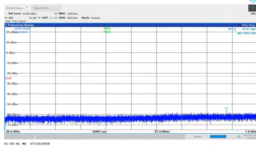
NTNV-n2-PC2-15-40-H-DFT-BPSK-Inner_1RB_Left-30-1000-PASS
