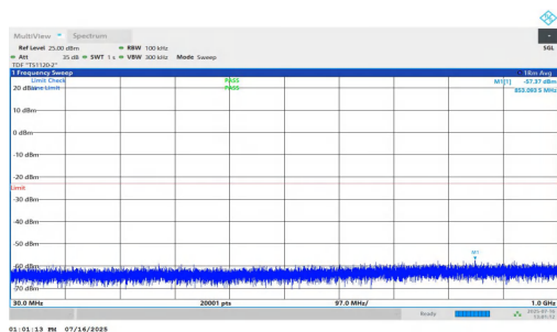
NTNV-n2-PC2-15-40-L-DFT-QPSK-Inner_1RB_Right-30-1000-P ASS
