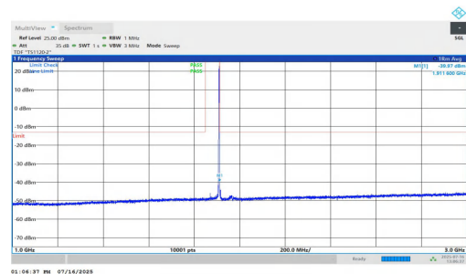
NTNV-n2-PC2-15-40-H-DFT-QPSK-Inner_1RB_Right-1000-3000-PASS
