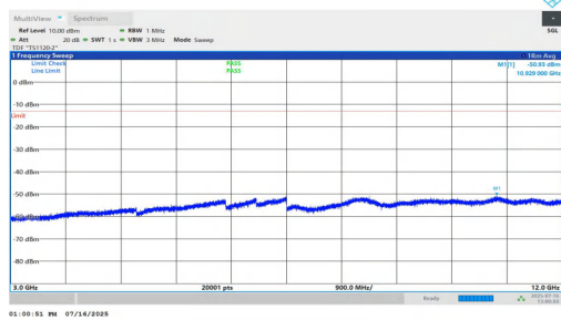
NTNV-n2-PC2-15-40-L-DFT-QPSK-Inner_1RB_Left-3000-12000- PASS
