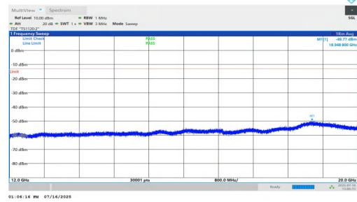
NTNV-n2-PC2-15-40-H-DFT-QPSK-Inner_1RB_Left-12000-20000-PASS
