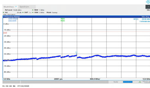
NTNV-n2-PC2-15-40-M-DFT-BPSK-Inner_1RB_Right-3000-1200 0-PASS
