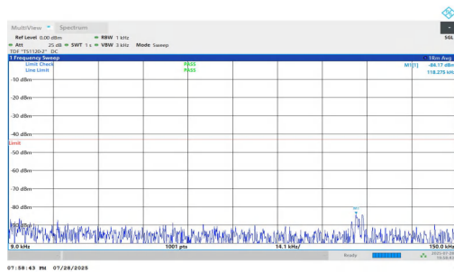
NTNV-n2-PC2-15-35-H-DFT-QPSK-Inner_1RB_Left-0.009-0.15-P ASS
