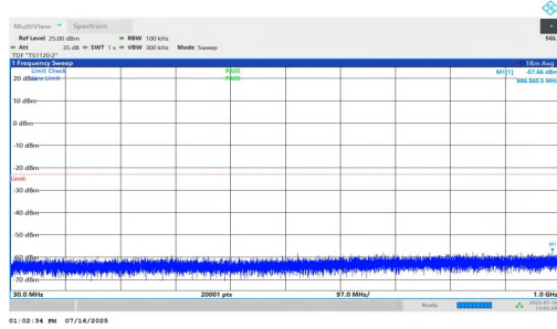
NTNV-n2-PC2-15-40-M-DFT-BPSK-Inner_1RB_Right-30-1000-P ASS
