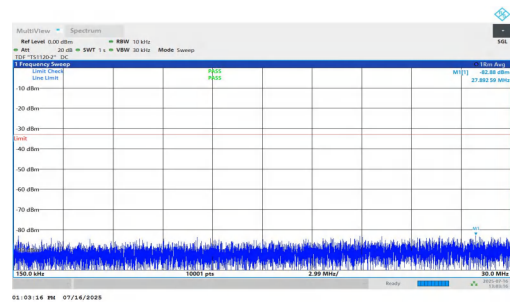
NTNV-n2-PC2-15-40-M-DFT-QPSK-Inner_1RB_Left-0.15-30-PAS S
