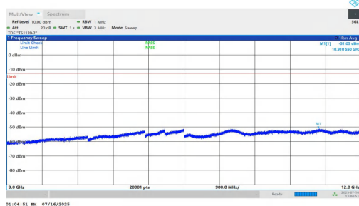
NTNV-n2-PC2-15-40-H-DFT-BPSK-Inner_1RB_Left-3000-12000-PASS
