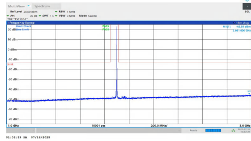
NTNV-n2-PC2-15-40-M-DFT-BPSK-Inner_1RB_Right-1000-3000-P PASS
