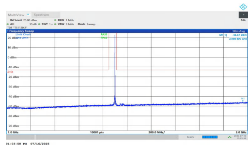
NTNV-n2-PC2-15-40-M-DFT-QPSK-Inner_1RB_Right-1000-3000- PASS
