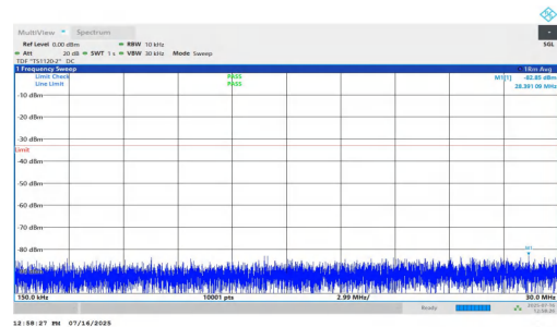
NTNV-n2-PC2-15-35-H-DFT-QPSK-Inner_1RB_Right-0.15-30-PA-SS
