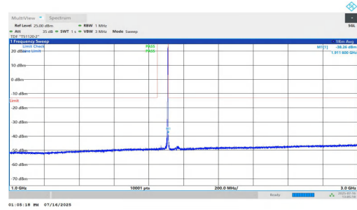
NTNV-n2-PC2-15-40-H-DFT-BPSK-Inner_1RB_Right-1000-3000-P PASS
