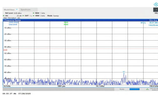
NTNV-n2-PC2-15-40-M-DFT-QPSK-Inner_1RB_Left-0.009-0.15- PASS
