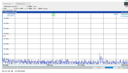
NTNV-n2-PC2-15-40-H-DFT-BPSK-Inner_1RB_Left-0.009-0.15-P ASS
