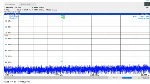
NTNV-n2-PC2-15-40-M-DFT-BPSK-Inner_1RB_Left-0.15-30-PAS S
