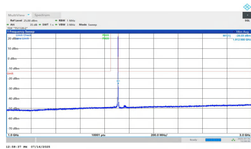
NTNV-n2-PC2-15-35-H-DFT-QPSK-Inner_1RB_Right-1000-3000-PASS
