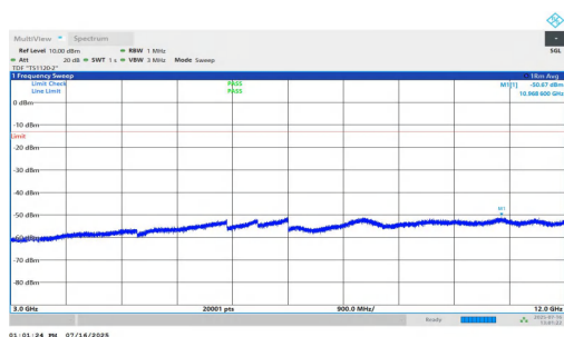
NTNV-n2-PC2-15-40-L-DFT-QPSK-Inner_1RB_Right-3000-1200 0-PASS
