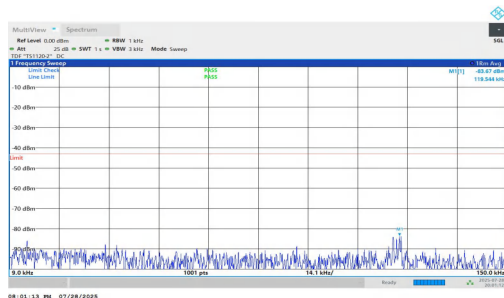
NTNV-n2-PC2-15-40-H-DFT-BPSK-Inner_1RB_Right-0.009-0.15-PASS
