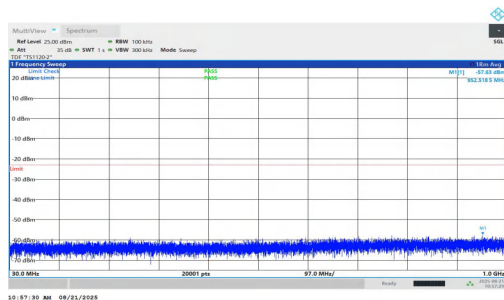
NTNV-n2-PC2-15-35-M-DFT-QPSK-Inner_1RB_Right-30-1000-P ASS
