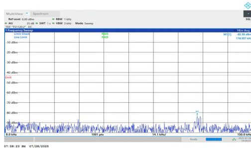
NTNV-n2-PC2-15-35-H-DFT-BPSK-Inner_1RB_Right-0.009-0.15- PASS
