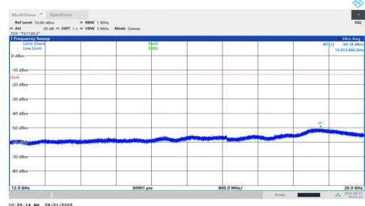
NTNV-n2-PC2-15-35-L-DFT-QPSK-Inner_1RB_Right-12000-20000-PASS
