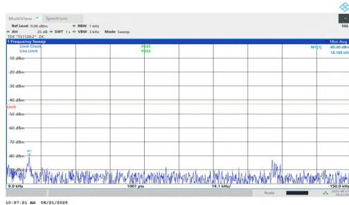
NTNV-n2-PC2-15-35-M-DFT-QPSK-Inner_1RB_Right-0.009-0.15 -PASS
