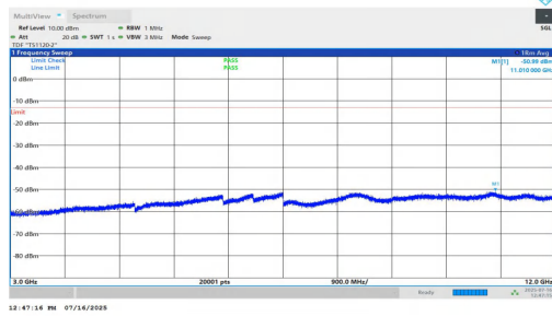
NTNV-n2-PC2-15-30-M-DFT-QPSK-Inner_1RB_Left-3000-12000 -PASS
