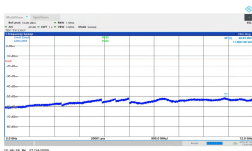
NTNV-n2-PC2-15-30-L-DFT-QPSK-Inner_1RB_Right-3000-12000-PASS
