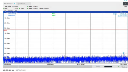
NTNV-n2-PC2-15-35-M-DFT-BPSK-Inner_1RB_Left-0.15-30-PAS S
