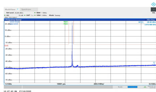
NTNV-n2-PC2-15-30-M-DFT-QPSK-Inner_1RB_Right-1000-3000- PASS
