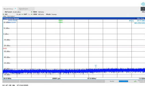
NTNV-n2-PC2-15-30-M-DFT-QPSK-Inner_1RB_Right-30-1000-P ASS
