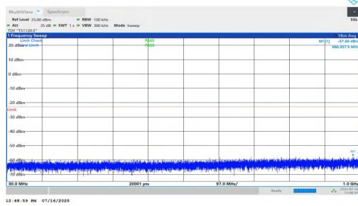
NTNV-n2-PC2-15-30-H-DFT-BPSK-Inner_1RB_Right-30-1000-P ASS
