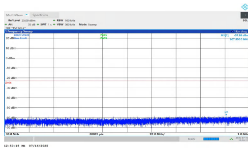
NTNV-n2-PC2-15-30-H-DFT-QPSK-Inner_1RB_Right-30-1000-PASS
