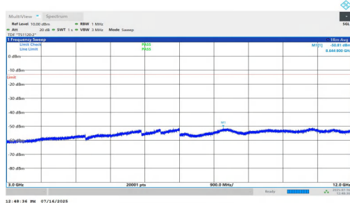
NTNV-n2-PC2-15-30-H-DFT-BPSK-Inner_1RB_Left-3000-12000- PASS
