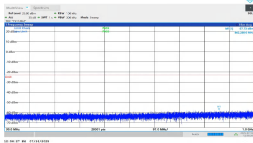
NTNV-n2-PC2-15-35-H-DFT-BPSK-Inner_1RB_Left-30-1000-PASS
