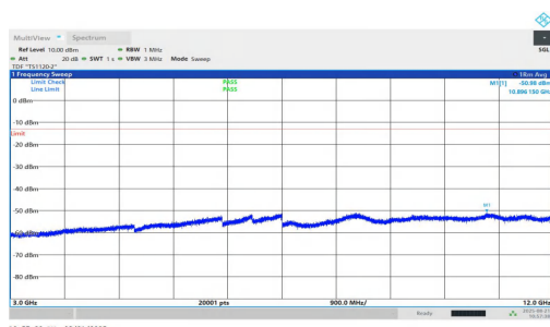
NTNV-n2-PC2-15-35-M-DFT-QPSK-Inner_1RB_Right-3000-1200 0-PASS
