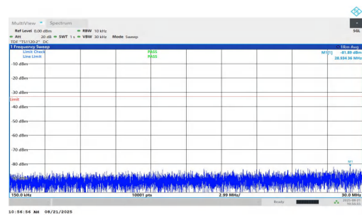
NTNV-n2-PC2-15-35-M-DFT-QPSK-Inner_1RB_Left-0.15-30-PAS S
