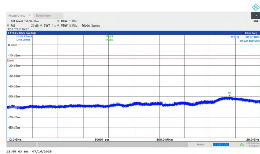
NTNV-n2-PC2-15-35-H-DFT-BPSK-Inner_1RB_Left-12000-20000- PASS
