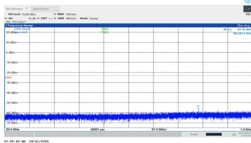
NTNV-n2-PC2-15-35-M-DFT-BPSK-Inner_1RB_Left-30-1000-PASS
