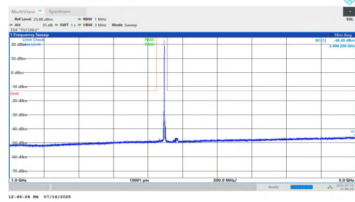
NTNV-n2-PC2-15-30-M-DFT-BPSK-Inner_1RB_Right-1000-3000-P PASS
