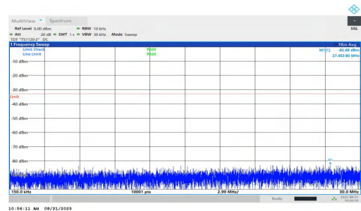
NTNV-n2-PC2-15-35-M-DFT-BPSK-Inner_1RB_Right-0.15-30-PASS
