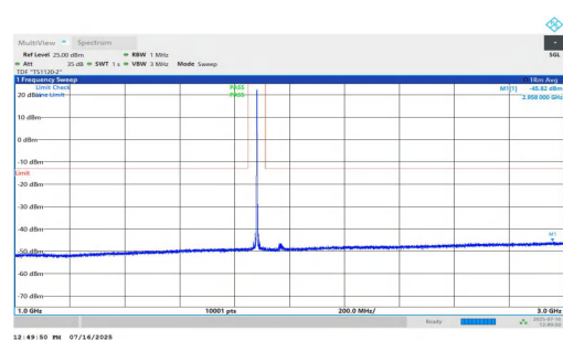
NTNV-n2-PC2-15-30-H-DFT-QPSK-Inner_1RB_Left-1000-3000-P ASS
