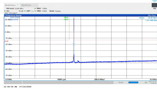
NTNV-n2-PC2-15-30-H-DFT-BPSK-Inner_1RB_Right-1000-3000-P PASS
