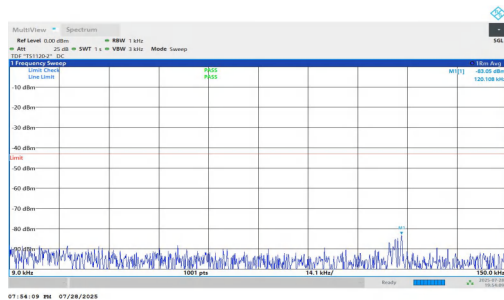
NTNV-n2-PC2-15-30-L-DFT-QPSK-Inner_1RB_Right-0.009-0.15-PASS
