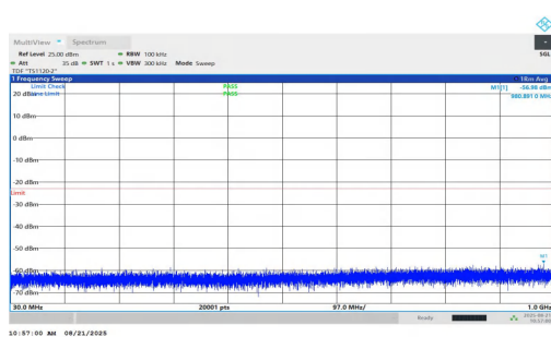
NTNV-n2-PC2-15-35-M-DFT-QPSK-Inner_1RB_Left-30-1000-PA SS
