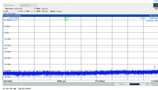
NTNV-n2-PC2-15-35-L-DFT-QPSK-Inner_1RB_Right-30-1000-PASS
