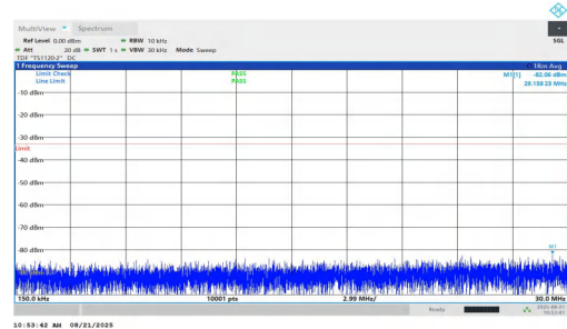
NTNV-n2-PC2-15-35-L-DFT-BPSK-Inner_1RB_Right-0.15-30-PASS
