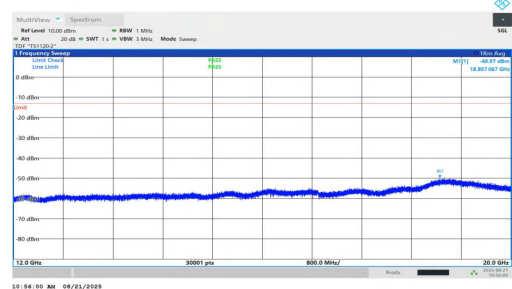
NTNV-n2-PC2-15-35-M-DFT-BPSK-Inner_1RB_Left-12000-20000-PASS
