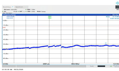
NTNV-n2-PC2-15-35-L-DFT-BPSK-Inner_1RB_Right-3000-12000 -PASS
