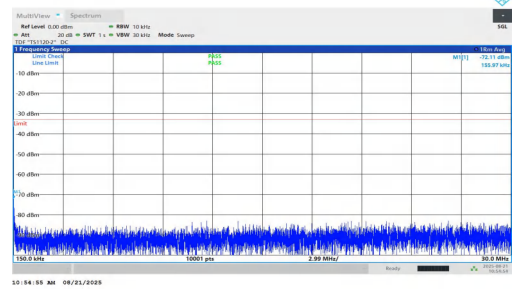
NTNV-n2-PC2-15-35-L-DFT-QPSK-Inner_1RB_Right-0.15-30-PASS
