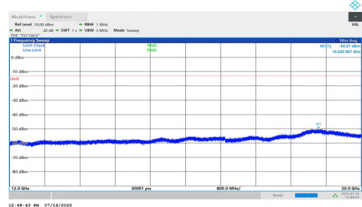
NTNV-n2-PC2-15-30-H-DFT-BPSK-Inner_1RB_Left-12000-20000- PASS
