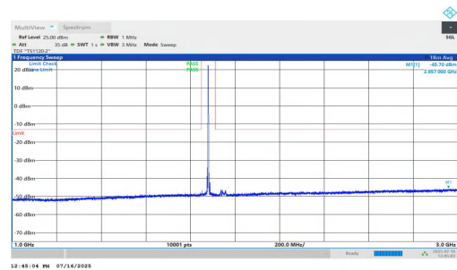
NTNV-n2-PC2-15-30-L-DFT-QPSK-Inner_1RB_Right-1000-3000-PASS
