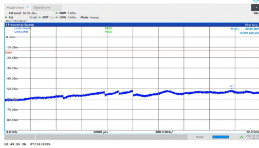
NTNV-n2-PC2-15-30-H-DFT-QPSK-Inner_1RB_Left-3000-12000-PASS
