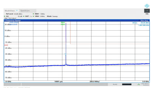
NTNV-n2-PC2-15-35-L-DFT-QPSK-Inner_1RB_Left-1000-3000-PA SS
