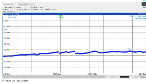
NTNV-n2-PC2-15-35-L-DFT-QPSK-Inner_1RB_Left-3000-12000-PASS
