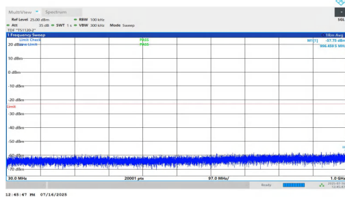
NTNV-n2-PC2-15-30-M-DFT-BPSK-Inner_1RB_Left-30-1000-PASS SS
