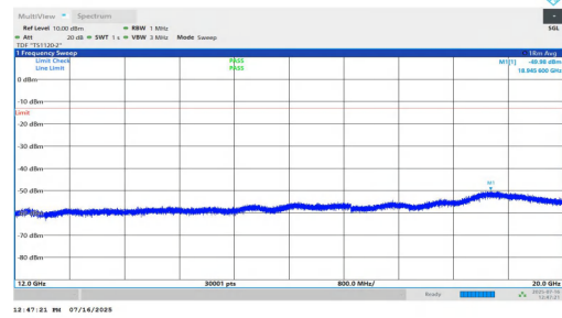
NTNV-n2-PC2-15-30-M-DFT-QPSK-Inner_1RB_Left-12000-20000 -PASS
