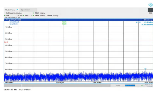
NTNV-n2-PC2-15-30-H-DFT-QPSK-Inner_1RB_Left-0.15-30-PAS S
