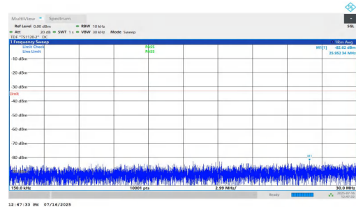
NTNV-n2-PC2-15-30-M-DFT-QPSK-Inner_1RB_Right-0.15-30-PA SS
