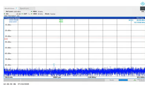
NTNV-n2-PC2-15-30-L-DFT-QPSK-Inner_1RB_Right-0.15-30-PASS
