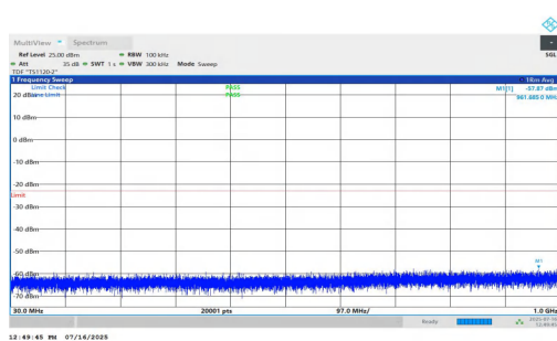
NTNV-n2-PC2-15-30-H-DFT-QPSK-Inner_1RB_Left-30-1000-PA SS
