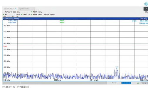
NTNV-n2-PC2-15-30-M-DFT-BPSK-Inner_1RB_Right-0.009-0.15 -PASS
