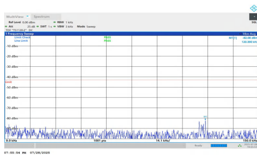
NTNV-n2-PC2-15-30-H-DFT-QPSK-Inner_1RB_Left-0.009-0.15-P ASS
