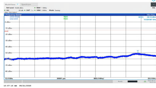
NTNV-n2-PC2-15-35-M-DFT-QPSK-Inner_1RB_Left-12000-20000 -PASS
