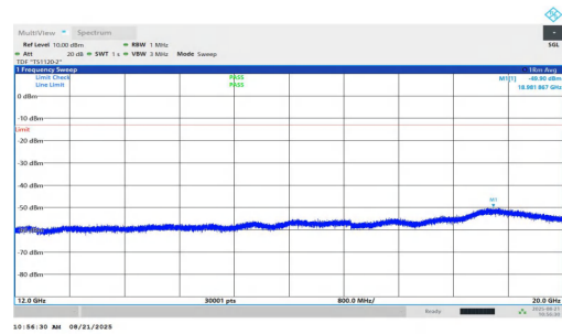
NTNV-n2-PC2-15-35-M-DFT-BPSK-Inner_1RB_Right-12000-2000 0-PASS
