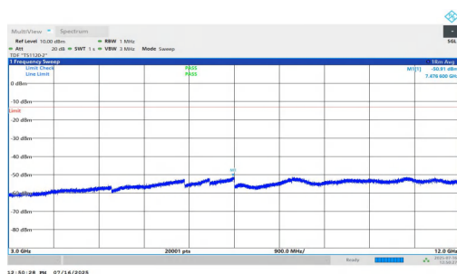
NTNV-n2-PC2-15-30-H-DFT-QPSK-Inner_1RB_Right-3000-12000-PASS
