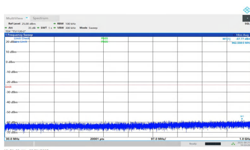
NTNV-n2-PC2-15-35-L-DFT-QPSK-Inner_1RB_Left-30-1000-PA SS
