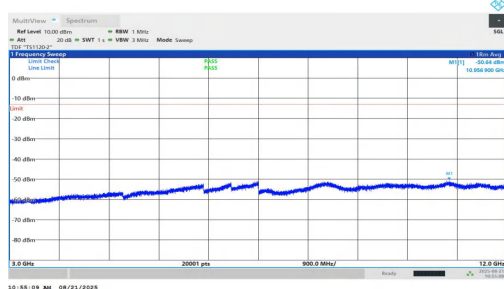
NTNV-n2-PC2-15-35-L-DFT-QPSK-Inner_1RB_Right-3000-12000-PASS
