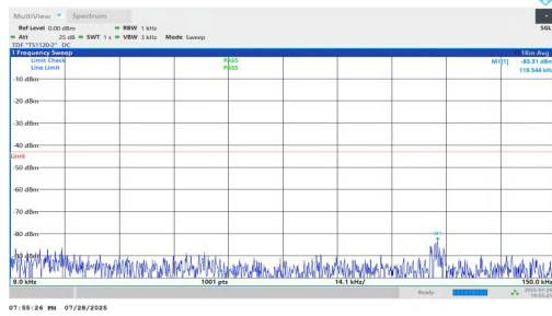
NTNV-n2-PC2-15-30-H-DFT-BPSK-Inner_1RB_Left-0.009-0.15-P ASS
