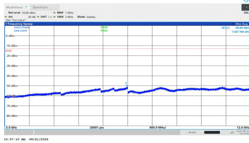
NTNV-n2-PC2-15-35-M-DFT-QPSK-Inner_1RB_Left-3000-12000 -PASS
