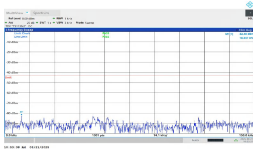
NTNV-n2-PC2-15-35-L-DFT-BPSK-Inner_1RB_Right-0.009-0.15-PASS
