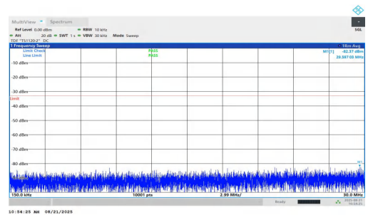
NTNV-n2-PC2-15-35-L-DFT-QPSK-Inner_1RB_Left-0.15-30-PASS
