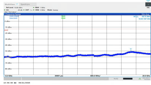
NTNV-n2-PC2-15-35-L-DFT-QPSK-Inner_1RB_Left-12000-20000-PASS
