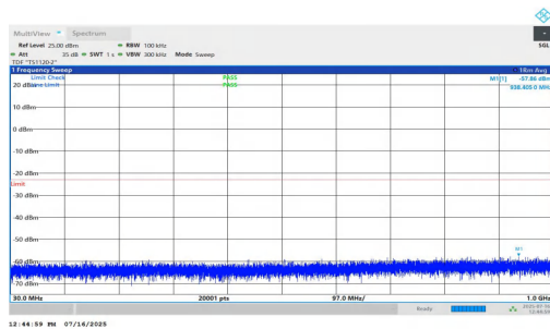
NTNV-n2-PC2-15-30-L-DFT-QPSK-Inner_1RB_Right-30-1000-PASS
