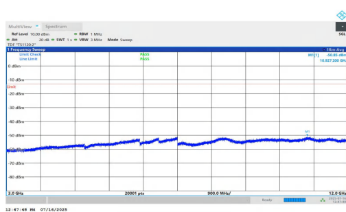
NTNV-n2-PC2-15-30-M-DFT-QPSK-Inner_1RB_Right-3000-1200 0-PASS
