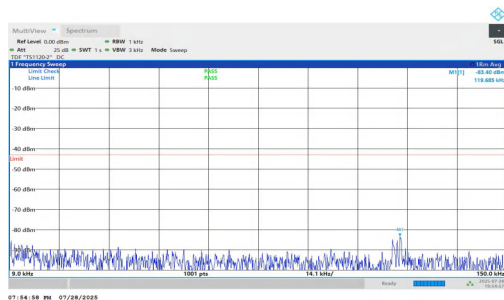
NTNV-n2-PC2-15-30-M-DFT-QPSK-Inner_1RB_Left-0.009-0.15- PASS
