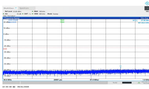
NTNV-n2-PC2-15-35-L-DFT-BPSK-Inner_1RB_Right-30-1000-PA SS
