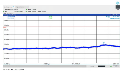
NTNV-n2-PC2-15-35-L-DFT-BPSK-Inner_1RB_Right-12000-2000 0-PASS
