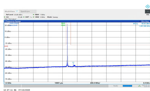
NTNV-n2-PC2-15-30-M-DFT-QPSK-Inner_1RB_Left-1000-3000-P ASS
