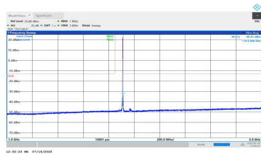
NTNV-n2-PC2-15-30-H-DFT-QPSK-Inner_1RB_Right-1000-3000-PASS
