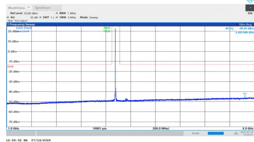
NTNV-n2-PC2-15-35-H-DFT-BPSK-Inner_1RB_Left-1000-3000-P ASS
