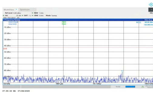
NTNV-n2-PC2-15-30-H-DFT-BPSK-Inner_1RB_Right-0.009-0.15- PASS
