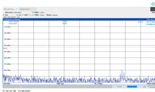
NTNV-n2-PC2-15-30-H-DFT-QPSK-Inner_1RB_Right-0.009-0.15-PASS
