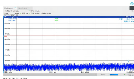
NTNV-n2-PC2-15-30-M-DFT-QPSK-Inner_1RB_Left-0.15-30-PAS S
