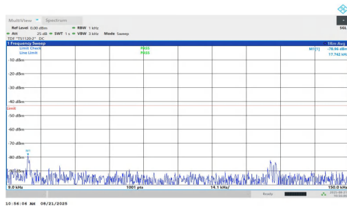
NTNV-n2-PC2-15-35-M-DFT-BPSK-Inner_1RB_Right-0.009-0.15-PASS
