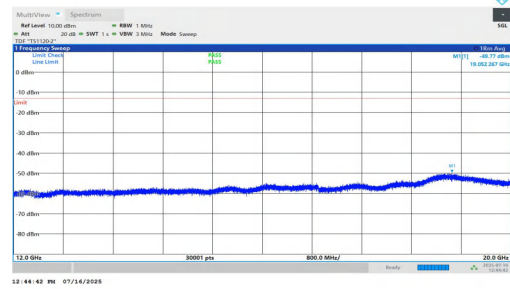
NTNV-n2-PC2-15-30-L-DFT-QPSK-Inner_1RB_Left-12000-20000-PASS
