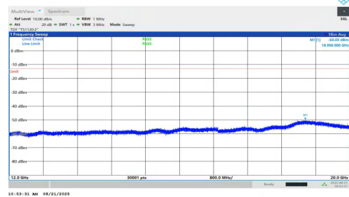
NTNV-n2-PC2-15-35-L-DFT-BPSK-Inner_1RB_Left-12000-20000-PASS
