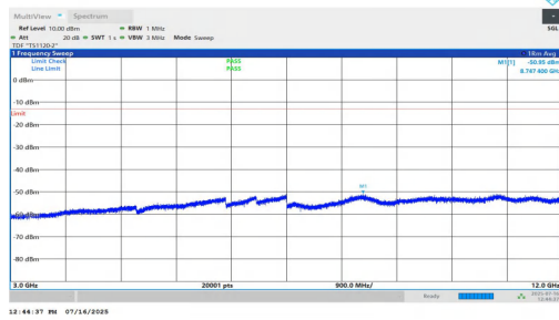
NTNV-n2-PC2-15-30-L-DFT-QPSK-Inner_1RB_Left-3000-12000-PASS
