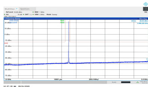
NTNV-n2-PC2-15-35-M-DFT-QPSK-Inner_1RB_Right-1000-3000- PASS
