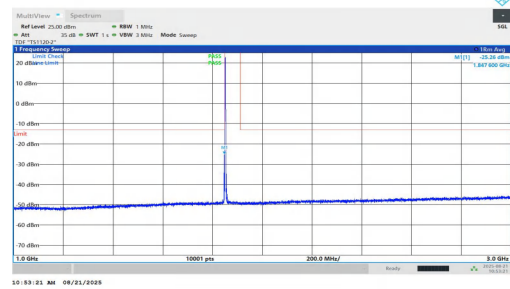
NTNV-n2-PC2-15-35-L-DFT-BPSK-Inner_1RB_Left-1000-3000-PASS
