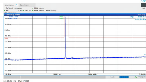
NTNV-n2-PC2-15-30-M-DFT-BPSK-Inner_1RB_Left-1000-3000-P ASS
