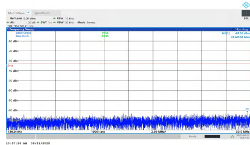
NTNV-n2-PC2-15-35-M-DFT-QPSK-Inner_1RB_Right-0.15-30-PA SS
