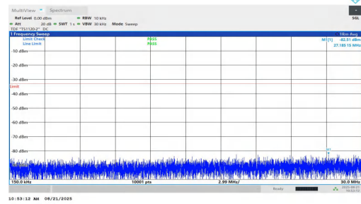
NTNV-n2-PC2-15-35-L-DFT-BPSK-Inner_1RB_Left-0.15-30-PASS
