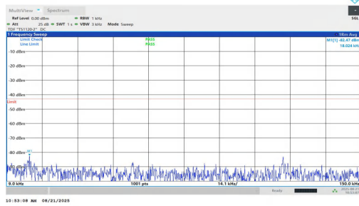
NTNV-n2-PC2-15-35-L-DFT-BPSK-Inner_1RB_Left-0.009-0.15-PASS
