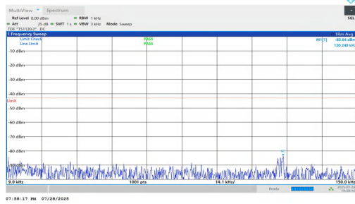
NTNV-n2-PC2-15-35-H-DFT-BPSK-Inner_1RB_Left-0.009-0.15-P ASS
