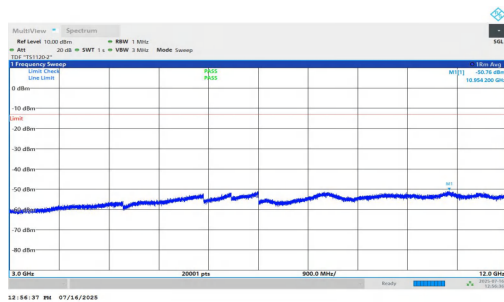
NTNV-n2-PC2-15-35-H-DFT-BPSK-Inner_1RB_Left-3000-12000- PASS
