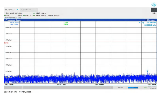
NTNV-n2-PC2-15-30-H-DFT-BPSK-Inner_1RB_Right-0.15-30-PAS S
