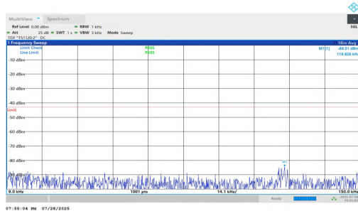
NTNV-n2-PC2-15-30-M-DFT-QPSK-Inner_1RB_Right-0.009-0.15 -PASS
