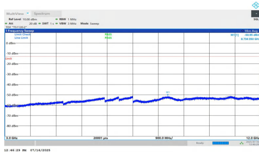
NTNV-n2-PC2-15-30-M-DFT-BPSK-Inner_1RB_Right-3000-1200 0-PASS
