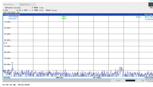
NTNV-n2-PC2-15-35-M-DFT-BPSK-Inner_1RB_Left-0.009-0.15-P ASS
