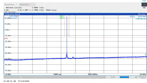
NTNV-n2-PC2-15-30-H-DFT-BPSK-Inner_1RB_Left-1000-3000-P ASS
