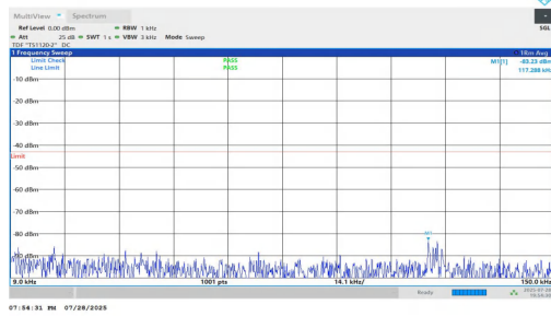
NTNV-n2-PC2-15-30-M-DFT-BPSK-Inner_1RB_Left-0.009-0.15-P ASS
