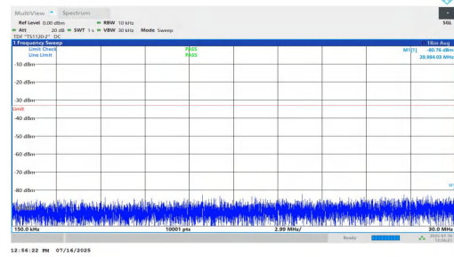
NTNV-n2-PC2-15-35-H-DFT-BPSK-Inner_1RB_Left-0.15-30-PASS
