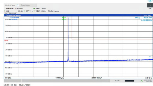
NTNV-n2-PC2-15-35-M-DFT-BPSK-Inner_1RB_Left-1000-3000-PASS
