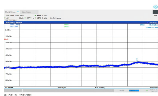
NTNV-n2-PC2-15-30-M-DFT-QPSK-Inner_1RB_Right-12000-2000 0-PASS
