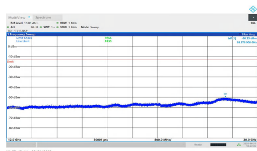
NTNV-n2-PC2-15-35-M-DFT-QPSK-Inner_1RB_Right-12000-2000 0-PASS
