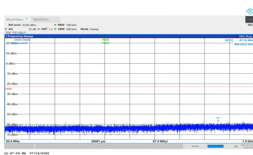
NTNV-n2-PC2-15-30-M-DFT-QPSK-Inner_1RB_Left-30-1000-PA SS
