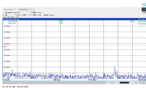
NTNV-n2-PC2-15-35-M-DFT-QPSK-Inner_1RB_Left-0.009-0.15- PASS
