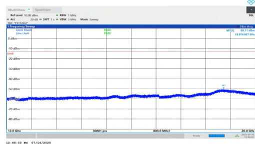
NTNV-n2-PC2-15-30-M-DFT-BPSK-Inner_1RB_Left-12000-20000-PASS PASS
