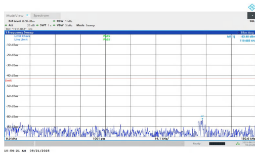
NTNV-n2-PC2-15-35-L-DFT-QPSK-Inner_1RB_Left-0.009-0.15-P ASS
