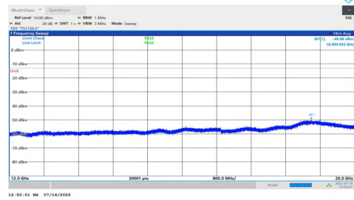
NTNV-n2-PC2-15-30-H-DFT-QPSK-Inner_1RB_Left-12000-20000-PASS
