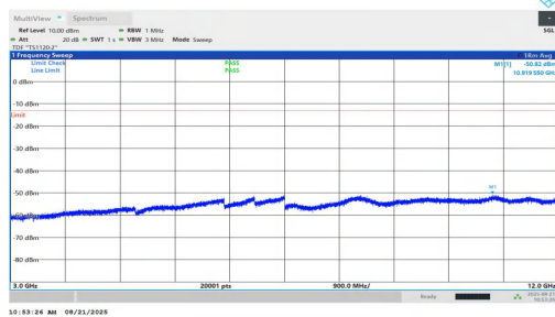
NTNV-n2-PC2-15-35-L-DFT-BPSK-Inner_1RB_Left-3000-12000-PASS
