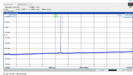
NTNV-n2-PC2-15-35-L-DFT-QPSK-Inner_1RB_Right-1000-3000-PASS
