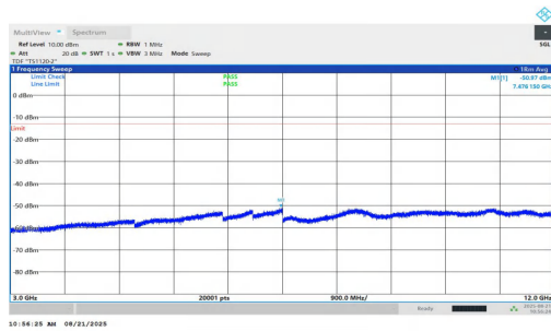
NTNV-n2-PC2-15-35-M-DFT-BPSK-Inner_1RB_Right-3000-1200 0-PASS
