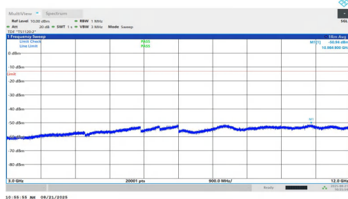
NTNV-n2-PC2-15-35-M-DFT-BPSK-Inner_1RB_Left-3000-12000-PASS
