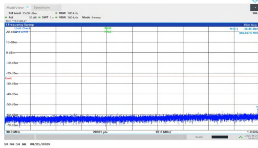
NTNV-n2-PC2-15-35-M-DFT-BPSK-Inner_1RB_Right-30-1000-P ASS
