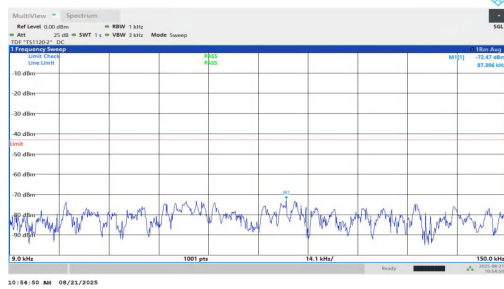
NTNV-n2-PC2-15-35-L-DFT-QPSK-Inner_1RB_Right-0.009-0.15-PASS
