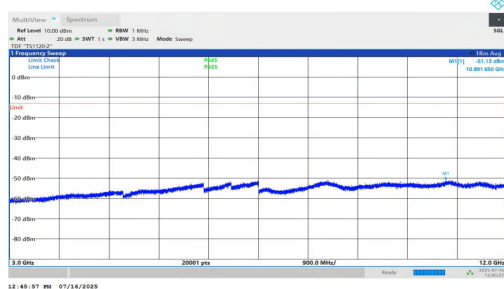
NTNV-n2-PC2-15-30-M-DFT-BPSK-Inner_1RB_Left-3000-12000-PASS PASS
