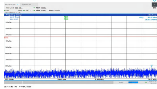
NTNV-n2-PC2-15-30-M-DFT-BPSK-Inner_1RB_Left-0.15-30-PAS S
