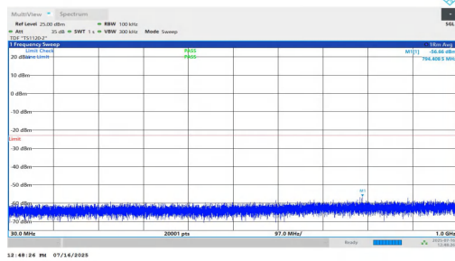
NTNV-n2-PC2-15-30-H-DFT-BPSK-Inner_1RB_Left-30-1000-PASS
