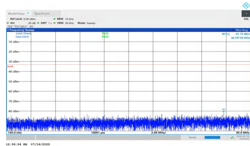
NTNV-n2-PC2-15-35-H-DFT-BPSK-Inner_1RB_Right-0.15-30-PAS S
