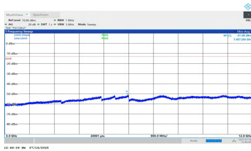
NTNV-n2-PC2-15-30-H-DFT-BPSK-Inner_1RB_Right-3000-1200 0-PASS
