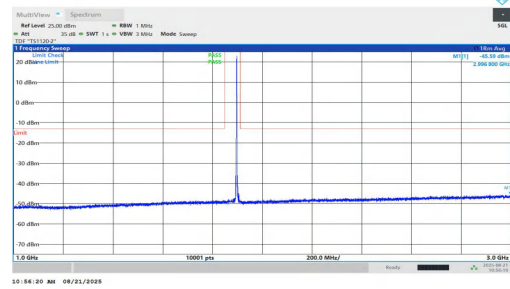
NTNV-n2-PC2-15-35-M-DFT-BPSK-Inner_1RB_Right-1000-3000- PASS
