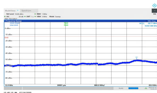
NTNV-n2-PC2-15-30-L-DFT-QPSK-Inner_1RB_Right-12000-20000-PASS
