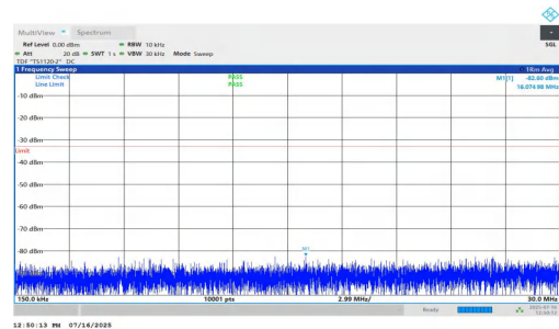
NTNV-n2-PC2-15-30-H-DFT-QPSK-Inner_1RB_Right-0.15-30-PA-SS
