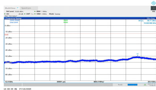
NTNV-n2-PC2-15-30-M-DFT-BPSK-Inner_1RB_Right-12000-2000 0-PASS
