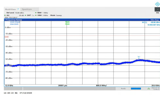
NTNV-n2-PC2-15-30-H-DFT-BPSK-Inner_1RB_Right-12000-2000 0-PASS
