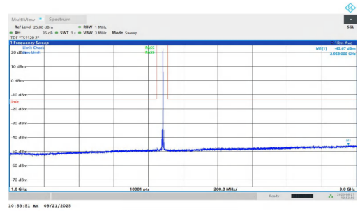
NTNV-n2-PC2-15-35-L-DFT-BPSK-Inner_1RB_Right-1000-3000-P ASS
