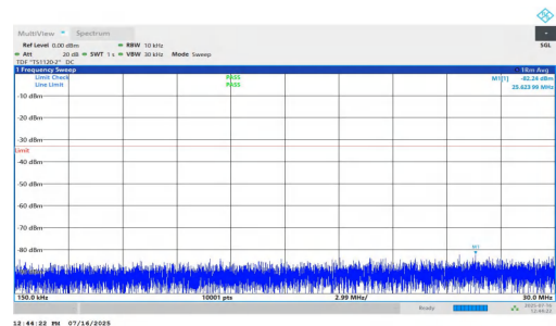
NTNV-n2-PC2-15-30-L-DFT-QPSK-Inner_1RB_Left-0.15-30-PASS
