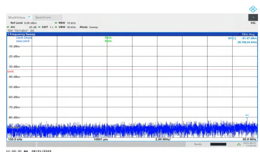
NTNV-n2-PC2-15-25-M-DFT-BPSK-Inner_1RB_Right-0.15-30-PASS SS
