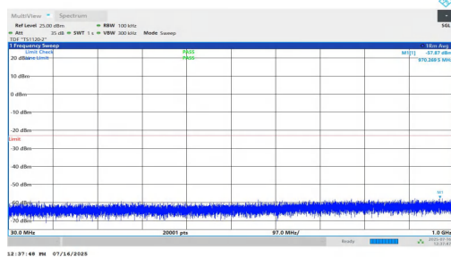
NTNV-n2-PC2-15-20-M-DFT-BPSK-Inner_1RB_Left-30-1000-PASS
