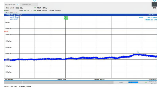
NTNV-n2-PC2-15-15-M-DFT-QPSK-Inner_1RB_Left-12000-20000 -PASS
