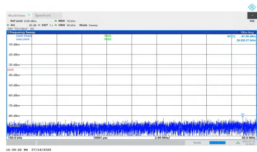
NTNV-n2-PC2-15-20-L-DFT-QPSK-Inner_1RB_Left-0.15-30-PASS
