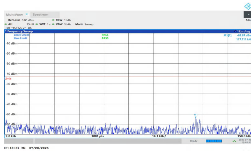
NTNV-n2-PC2-15-15-L-DFT-QPSK-Inner_1RB_Right-0.009-0.15-PASS
