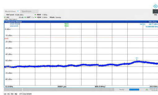
NTNV-n2-PC2-15-15-M-DFT-QPSK-Inner_1RB_Right-12000-20000 0-PASS
