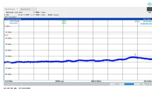
NTNV-n2-PC2-15-20-L-DFT-BPSK-Inner_1RB_Left-12000-20000-PASS
