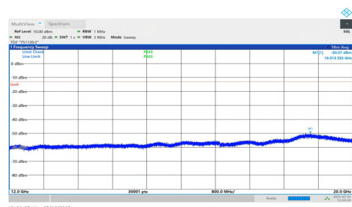
NTNV-n2-PC2-15-15-H-DFT-QPSK-Inner_1RB_Right-12000-20000-PASS
