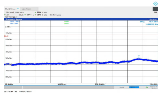
NTNV-n2-PC2-15-15-H-DFT-BPSK-Inner_1RB_Left-12000-20000-PASS
