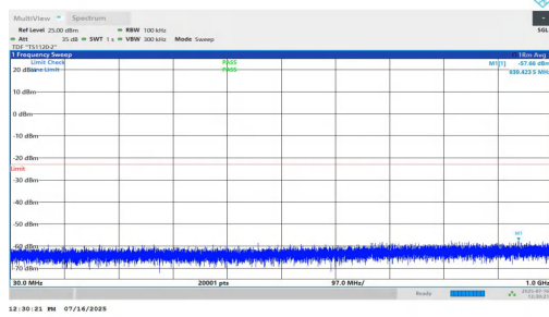
NTNV-n2-PC2-15-15-M-DFT-BPSK-Inner_1RB_Right-30-1000-P ASS
