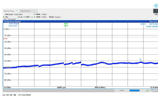
NTNV-n2-PC2-15-20-M-DFT-QPSK-Inner_1RB_Right-3000-1200 0-PASS
