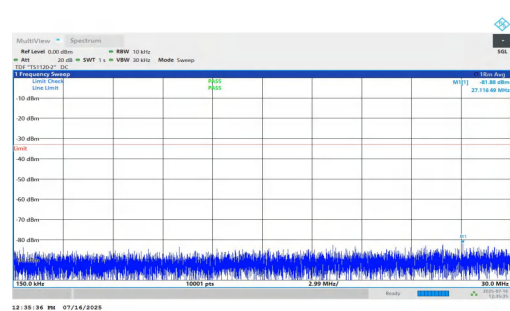
NTNV-n2-PC2-15-20-L-DFT-BPSK-Inner_1RB_Right-0.15-30-PASS
