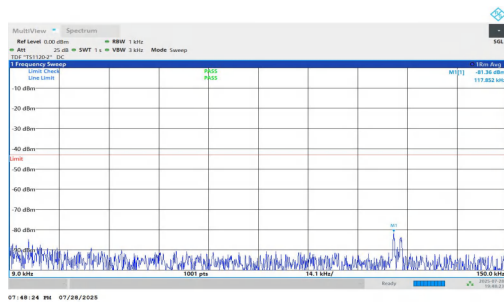
NTNV-n2-PC2-15-15-L-DFT-QPSK-Inner_1RB_Left-0.009-0.15-P ASS
