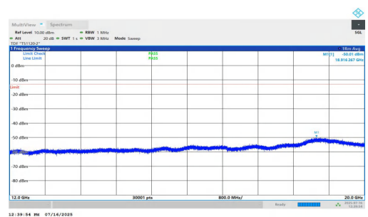
NTNV-n2-PC2-15-20-M-DFT-QPSK-Inner_1RB_Right-12000-2000 0-PASS
