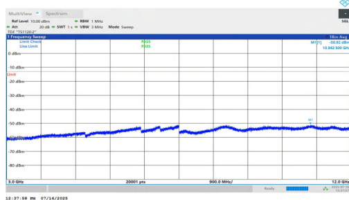
NTNV-n2-PC2-15-20-M-DFT-BPSK-Inner_1RB_Left-3000-12000-PASS
