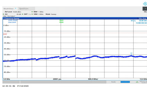
NTNV-n2-PC2-15-15-M-DFT-BPSK-Inner_1RB_Right-3000-1200 0-PASS
