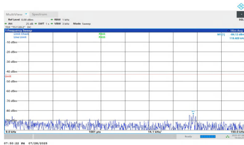
NTNV-n2-PC2-15-15-H-DFT-QPSK-Inner_1RB_Right-0.009-0.15-PASS
