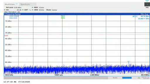
NTNV-n2-PC2-15-20-M-DFT-BPSK-Inner_1RB_Left-0.15-30-PASS
