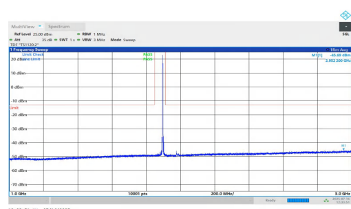
NTNV-n2-PC2-15-15-H-DFT-QPSK-Inner_1RB_Left-1000-3000-P ASS
