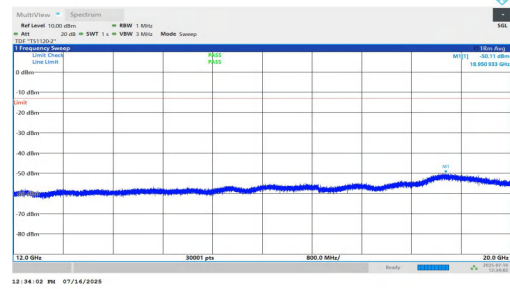
NTNV-n2-PC2-15-15-H-DFT-QPSK-Inner_1RB_Left-12000-20000-PASS
