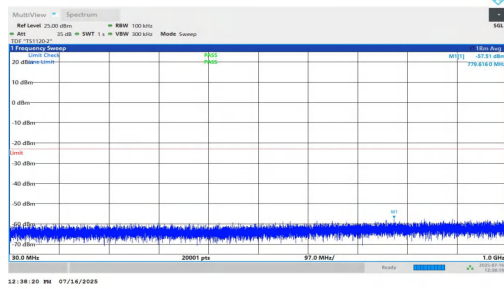
NTNV-n2-PC2-15-20-M-DFT-BPSK-Inner_1RB_Right-30-1000-P ASS
