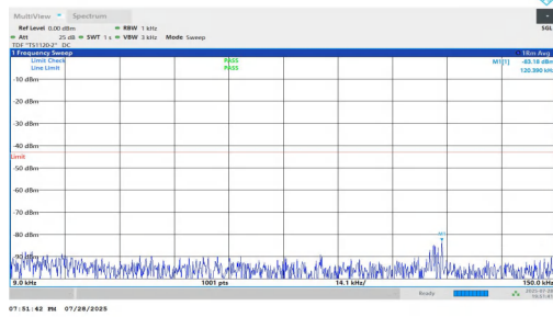
NTNV-n2-PC2-15-20-M-DFT-BPSK-Inner_1RB_Left-0.009-0.15-PASS
