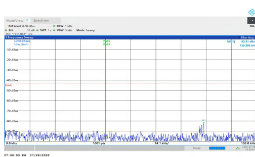
NTNV-n2-PC2-15-20-L-DFT-BPSK-Inner_1RB_Right-0.009-0.15-PASS
