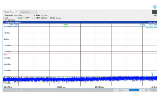
NTNV-n2-PC2-15-15-H-DFT-QPSK-Inner_1RB_Left-30-1000-P ASS
