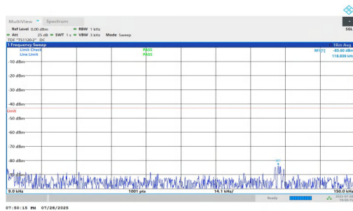
NTNV-n2-PC2-15-15-H-DFT-QPSK-Inner_1RB_Left-0.009-0.15-P ASS
