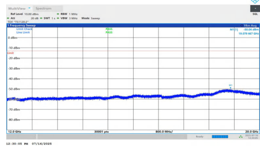
NTNV-n2-PC2-15-15-M-DFT-BPSK-Inner_1RB_Left-12000-20000-PASS
