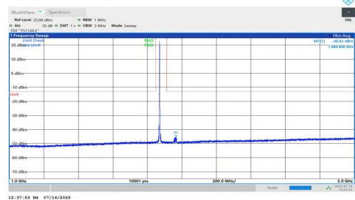
NTNV-n2-PC2-15-20-M-DFT-BPSK-Inner_1RB_Left-1000-3000-PASS
