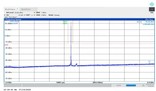
NTNV-n2-PC2-15-20-M-DFT-QPSK-Inner_1RB_Right-1000-3000- PASS
