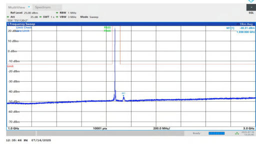
NTNV-n2-PC2-15-20-L-DFT-BPSK-Inner_1RB_Right-1000-3000-P ASS
