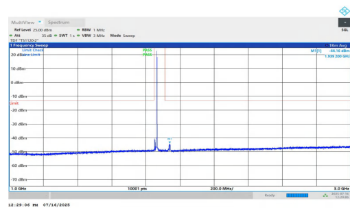
NTNV-n2-PC2-15-15-L-DFT-QPSK-Inner_1RB_Right-1000-3000-PASS
