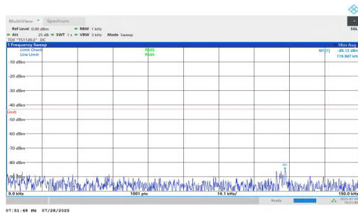
NTNV-n2-PC2-15-20-M-DFT-BPSK-Inner_1RB_Right-0.009-0.15-PASS
