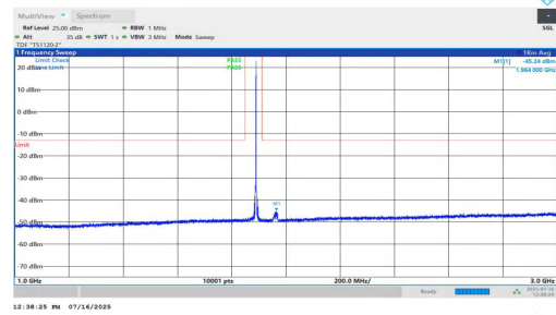
NTNV-n2-PC2-15-20-M-DFT-BPSK-Inner_1RB_Right-1000-3000-P PASS
