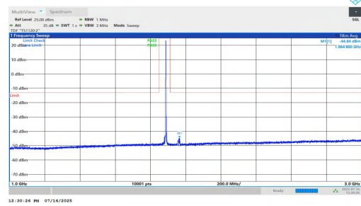
NTNV-n2-PC2-15-15-M-DFT-BPSK-Inner_1RB_Right-1000-3000-P PASS
