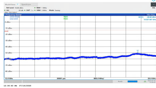
NTNV-n2-PC2-15-20-L-DFT-QPSK-Inner_1RB_Left-12000-20000-PASS
