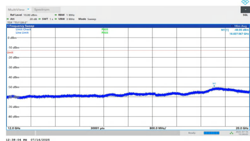
NTNV-n2-PC2-15-20-M-DFT-BPSK-Inner_1RB_Left-12000-20000-PASS
