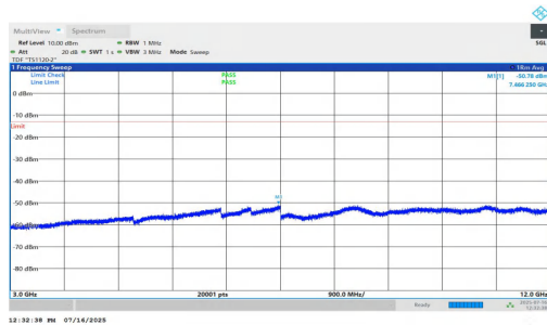
NTNV-n2-PC2-15-15-H-DFT-BPSK-Inner_1RB_Left-3000-12000-PASS
