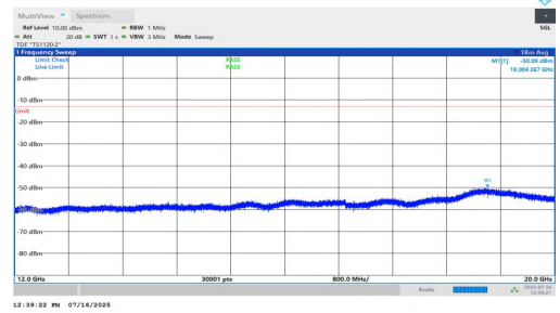
NTNV-n2-PC2-15-20-M-DFT-QPSK-Inner_1RB_Left-12000-20000 -PASS
