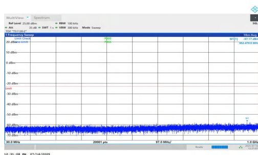
NTNV-n2-PC2-15-15-M-DFT-QPSK-Inner_1RB_Left-30-1000-PA SS
