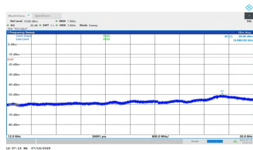
NTNV-n2-PC2-15-20-L-DFT-QPSK-Inner_1RB_Right-12000-20000-0-PASS
