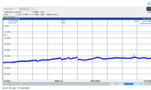
NTNV-n2-PC2-15-15-L-DFT-BPSK-Inner_1RB_Right-3000-12000 -PASS
