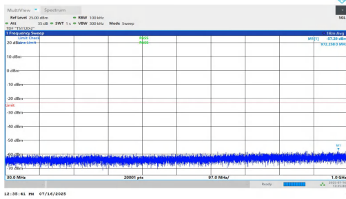
NTNV-n2-PC2-15-20-L-DFT-BPSK-Inner_1RB_Right-30-1000-PA SS
