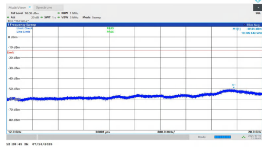
NTNV-n2-PC2-15-15-L-DFT-QPSK-Inner_1RB_Left-12000-20000-PASS
