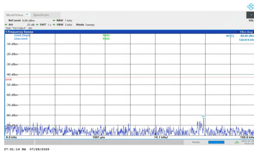
NTNV-n2-PC2-15-20-L-DFT-QPSK-Inner_1RB_Right-0.009-0.15-PASS
