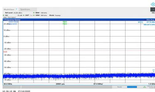
NTNV-n2-PC2-15-15-H-DFT-QPSK-Inner_1RB_Right-30-1000-PASS
