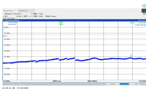
NTNV-n2-PC2-15-15-L-DFT-QPSK-Inner_1RB_Right-3000-12000-PASS
