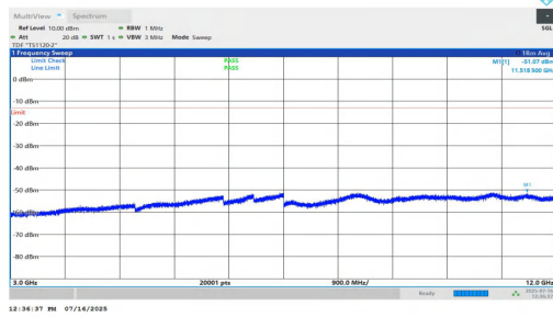
NTNV-n2-PC2-15-20-L-DFT-QPSK-Inner_1RB_Left-3000-12000-PASS
