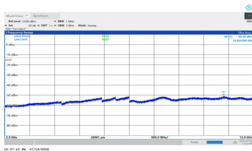
NTNV-n2-PC2-15-20-L-DFT-QPSK-Inner_1RB_Right-3000-12000-0-PASS
