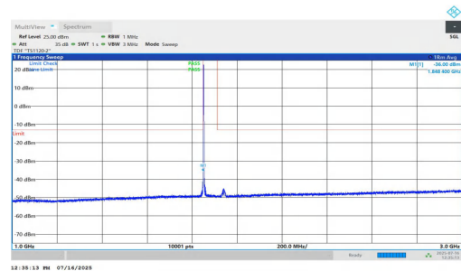
NTNV-n2-PC2-15-20-L-DFT-BPSK-Inner_1RB_Left-1000-3000-PASS
