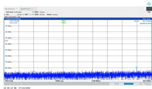
NTNV-n2-PC2-15-20-M-DFT-BPSK-Inner_1RB_Right-0.15-30-PASS
