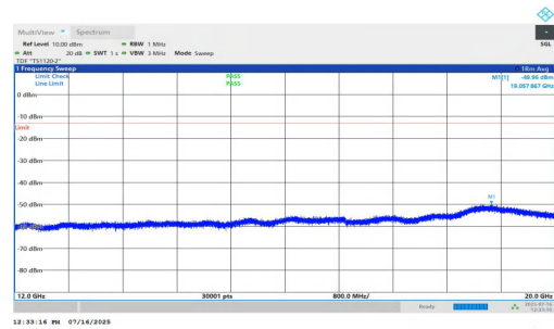
NTNV-n2-PC2-15-15-H-DFT-BPSK-Inner_1RB_Right-12000-20000-P PASS
