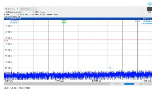
NTNV-n2-PC2-15-15-H-DFT-QPSK-Inner_1RB_Right-0.15-30-PA-SS
