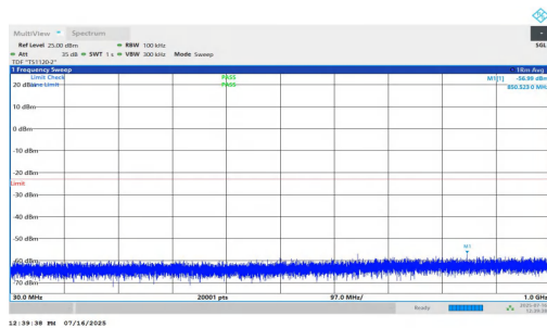
NTNV-n2-PC2-15-20-M-DFT-QPSK-Inner_1RB_Right-30-1000-P ASS
