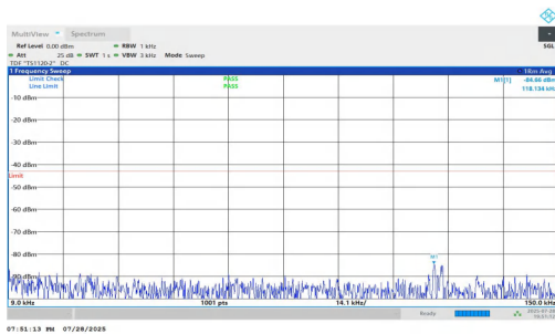
NTNV-n2-PC2-15-20-L-DFT-QPSK-Inner_1RB_Left-0.009-0.15-P ASS
