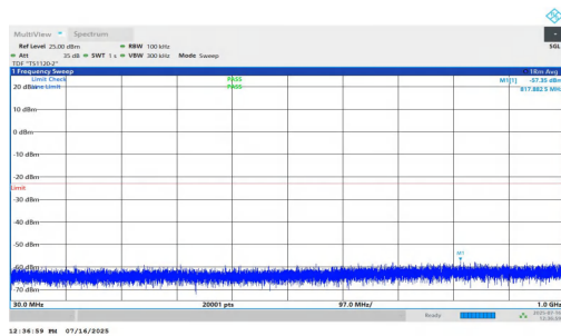
NTNV-n2-PC2-15-20-L-DFT-QPSK-Inner_1RB_Right-30-1000-PASS
