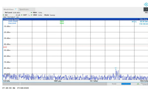
NTNV-n2-PC2-15-15-H-DFT-BPSK-Inner_1RB_Right-0.009-0.15-PASS
