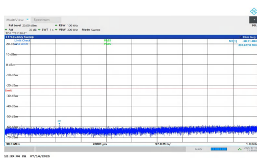
NTNV-n2-PC2-15-20-M-DFT-QPSK-Inner_1RB_Left-30-1000-PA SS
