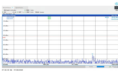
NTNV-n2-PC2-15-20-M-DFT-QPSK-Inner_1RB_Left-0.009-0.15- PASS
