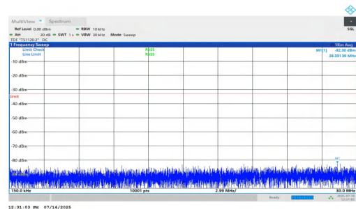
NTNV-n2-PC2-15-15-M-DFT-QPSK-Inner_1RB_Left-0.15-30-PAS S
