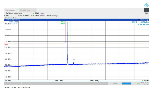
NTNV-n2-PC2-15-15-M-DFT-QPSK-Inner_1RB_Left-1000-3000-P ASS
