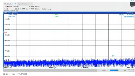
NTNV-n2-PC2-15-15-M-DFT-BPSK-Inner_1RB_Left-0.15-30-PASS
