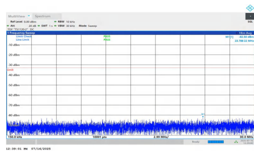
NTNV-n2-PC2-15-20-M-DFT-QPSK-Inner_1RB_Left-0.15-30-PAS S
