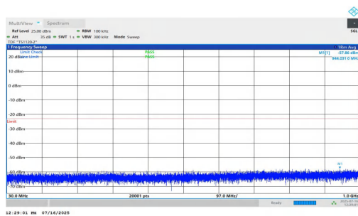
NTNV-n2-PC2-15-15-L-DFT-QPSK-Inner_1RB_Right-30-1000-PASS
