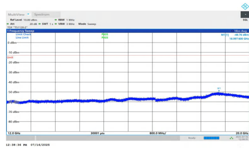
NTNV-n2-PC2-15-20-M-DFT-BPSK-Inner_1RB_Right-12000-20000 PASS
