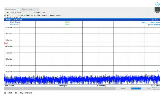
NTNV-n2-PC2-15-15-L-DFT-QPSK-Inner_1RB_Right-0.15-30-PASS
