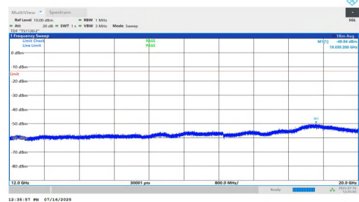
NTNV-n2-PC2-15-20-L-DFT-BPSK-Inner_1RB_Right-12000-2000 0-PASS
