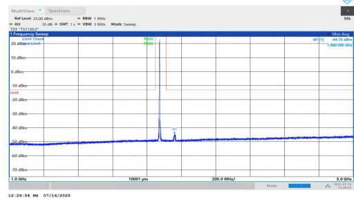
NTNV-n2-PC2-15-15-M-DFT-BPSK-Inner_1RB_Left-1000-3000-PASS
