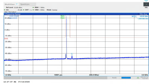
NTNV-n2-PC2-15-15-L-DFT-BPSK-Inner_1RB_Right-1000-3000-P ASS
