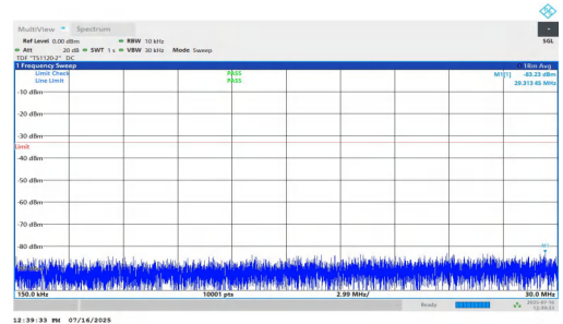
NTNV-n2-PC2-15-20-M-DFT-QPSK-Inner_1RB_Right-0.15-30-PA SS
