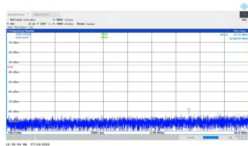
NTNV-n2-PC2-15-20-L-DFT-QPSK-Inner_1RB_Right-0.15-30-PASS
