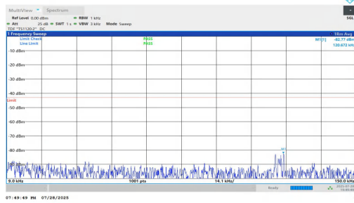
NTNV-n2-PC2-15-15-H-DFT-BPSK-Inner_1RB_Left-0.009-0.15-P ASS
