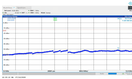
NTNV-n2-PC2-15-15-H-DFT-BPSK-Inner_1RB_Right-3000-12000-P PASS
