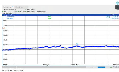
NTNV-n2-PC2-15-20-M-DFT-BPSK-Inner_1RB_Right-3000-12000 PASS
