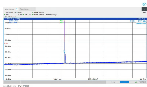
NTNV-n2-PC2-15-15-L-DFT-QPSK-Inner_1RB_Left-1000-3000-PA SS
