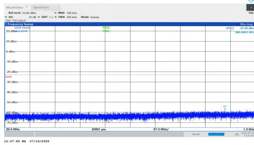
NTNV-n2-PC2-15-15-L-DFT-BPSK-Inner_1RB_Right-30-1000-PA SS
