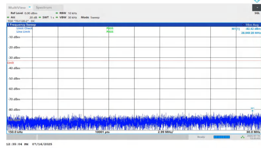
NTNV-n2-PC2-15-20-L-DFT-BPSK-Inner_1RB_Left-0.15-30-PASS
