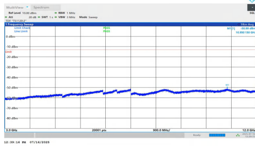
NTNV-n2-PC2-15-20-M-DFT-QPSK-Inner_1RB_Left-3000-12000 -PASS
