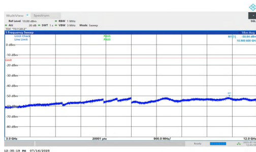
NTNV-n2-PC2-15-20-L-DFT-BPSK-Inner_1RB_Left-3000-12000-PASS
