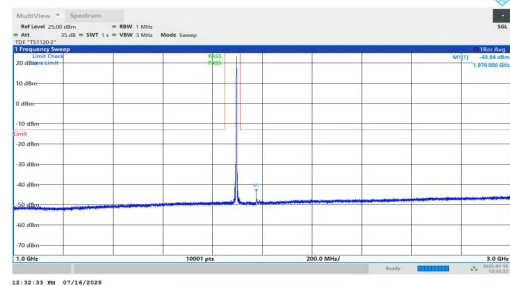
NTNV-n2-PC2-15-15-H-DFT-BPSK-Inner_1RB_Left-1000-3000-PASS
