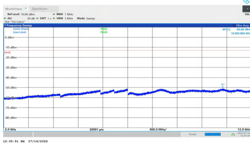
NTNV-n2-PC2-15-20-L-DFT-BPSK-Inner_1RB_Right-3000-12000 -PASS
