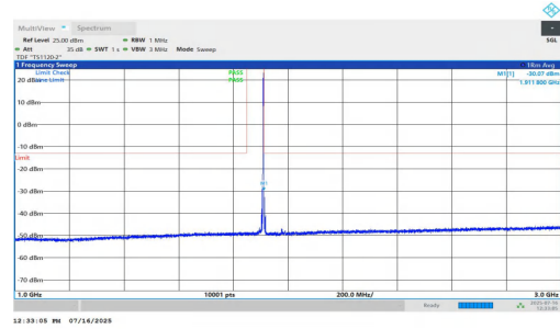
NTNV-n2-PC2-15-15-H-DFT-BPSK-Inner_1RB_Right-1000-3000-P PASS
