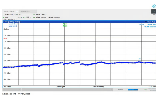
NTNV-n2-PC2-15-15-M-DFT-QPSK-Inner_1RB_Right-3000-12000 0-PASS
