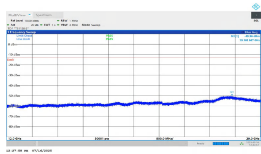
NTNV-n2-PC2-15-15-L-DFT-BPSK-Inner_1RB_Right-12000-2000 0-PASS
