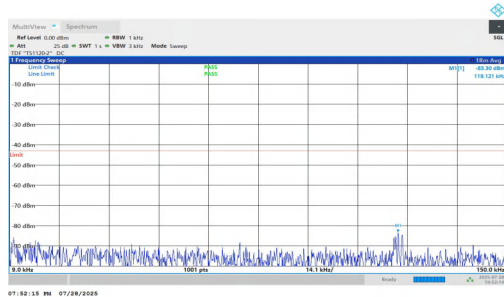
NTNV-n2-PC2-15-20-M-DFT-QPSK-Inner_1RB_Right-0.009-0.15 -PASS
