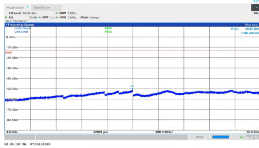
NTNV-n2-PC2-15-15-M-DFT-QPSK-Inner_1RB_Left-3000-12000 -PASS
