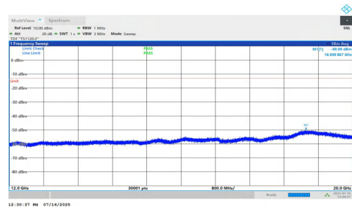
NTNV-n2-PC2-15-15-M-DFT-BPSK-Inner_1RB_Right-12000-2000 0-PASS
