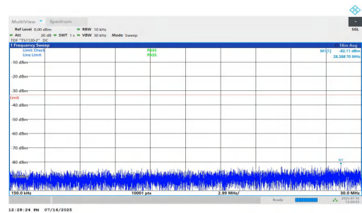
NTNV-n2-PC2-15-15-L-DFT-QPSK-Inner_1RB_Left-0.15-30-PASS
