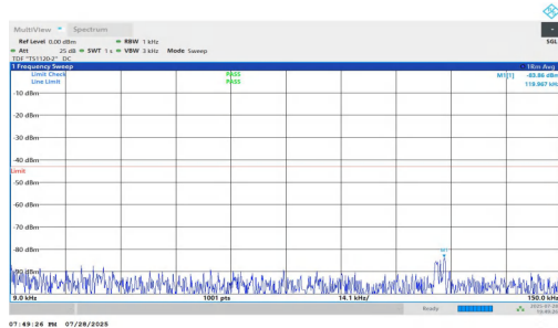
NTNV-n2-PC2-15-15-M-DFT-QPSK-Inner_1RB_Right-0.009-0.15 -PASS
