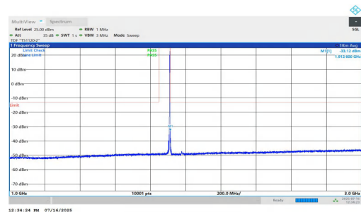
NTNV-n2-PC2-15-15-H-DFT-QPSK-Inner_1RB_Right-1000-3000-PASS
