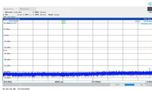
NTNV-n2-PC2-15-20-L-DFT-BPSK-Inner_1RB_Left-30-1000-PAS S
