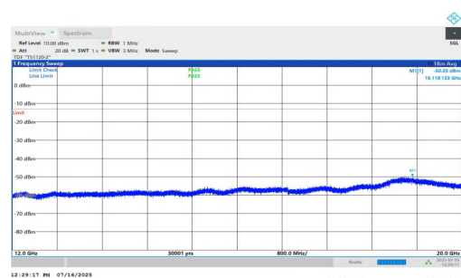
NTNV-n2-PC2-15-15-L-DFT-QPSK-Inner_1RB_Right-12000-20000-PASS
