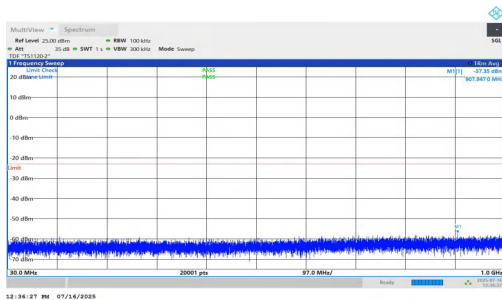
NTNV-n2-PC2-15-20-L-DFT-QPSK-Inner_1RB_Left-30-1000-PA SS
