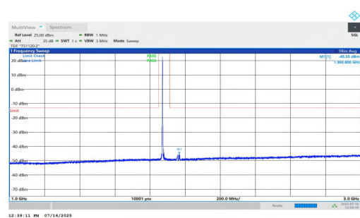
NTNV-n2-PC2-15-20-M-DFT-QPSK-Inner_1RB_Left-1000-3000-P ASS
