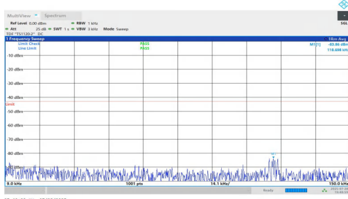
NTNV-n2-PC2-15-15-M-DFT-BPSK-Inner_1RB_Right-0.009-0.15-PASS
