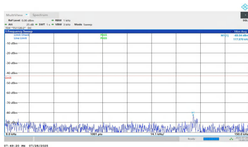
NTNV-n2-PC2-15-15-M-DFT-QPSK-Inner_1RB_Left-0.009-0.15- PASS
