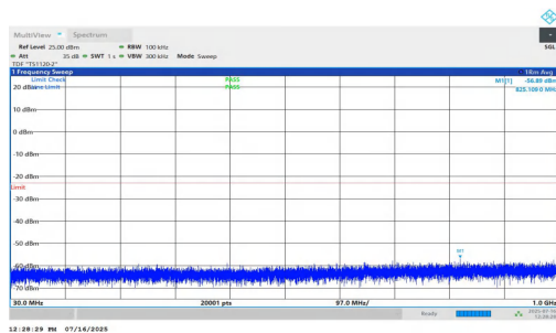
NTNV-n2-PC2-15-15-L-DFT-QPSK-Inner_1RB_Left-30-1000-PA SS
