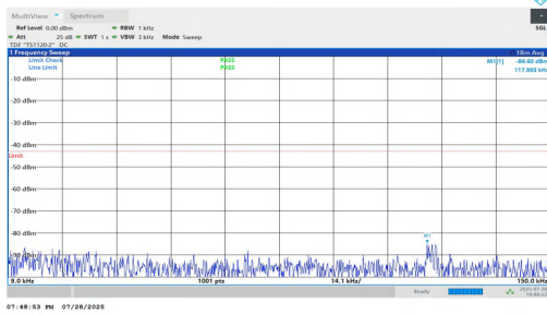
NTNV-n2-PC2-15-15-M-DFT-BPSK-Inner_1RB_Left-0.009-0.15-PASS
