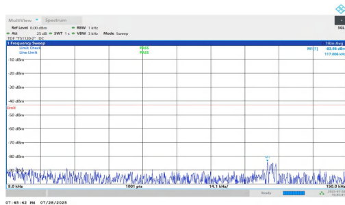
NTNV-n2-PC2-15-10-L-DFT-QPSK-Inner_1RB_Right-0.009-0.15-PASS
