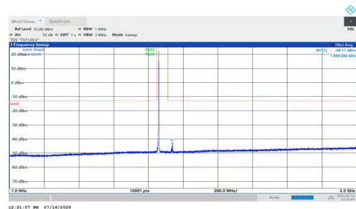
NTNV-n2-PC2-15-10-L-DFT-QPSK-Inner_1RB_Right-1000-3000-PASS
