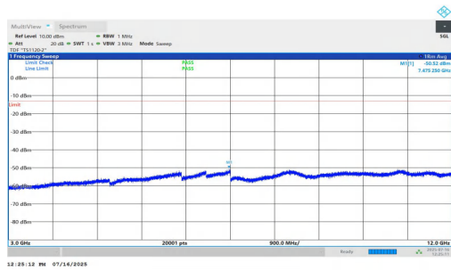
NTNV-n2-PC2-15-10-H-DFT-BPSK-Inner_1RB_Right-3000-1200 0-PASS
