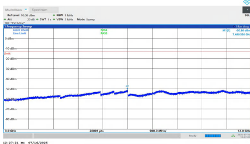
NTNV-n2-PC2-15-15-L-DFT-BPSK-Inner_1RB_Left-3000-12000- PASS
