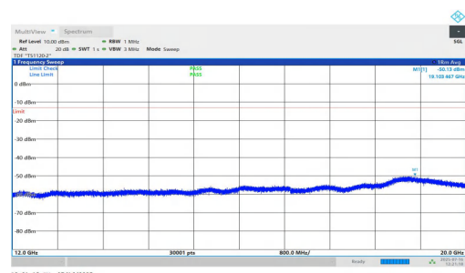
NTNV-n2-PC2-15-10-L-DFT-QPSK-Inner_1RB_Right-12000-20000-PASS
