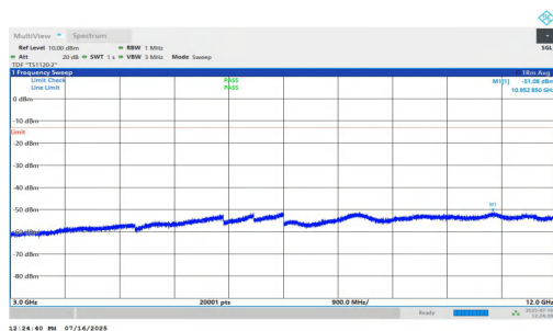
NTNV-n2-PC2-15-10-H-DFT-BPSK-Inner_1RB_Left-3000-12000-PASS
