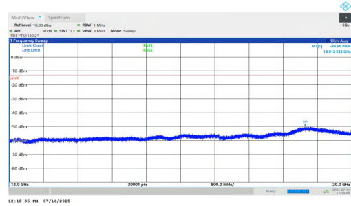
NTNV-n2-PC2-15-5-H-DFT-QPSK-Inner_1RB_Left-12000-20000-P ASS
