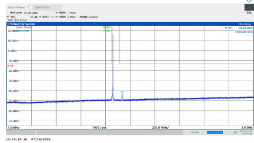
NTNV-n2-PC2-15-10-L-DFT-BPSK-Inner_1RB_Right-1000-3000-P ASS
