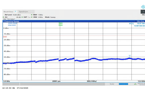
NTNV-n2-PC2-15-5-M-DFT-QPSK-Inner_1RB_Right-3000-12000-PASS
