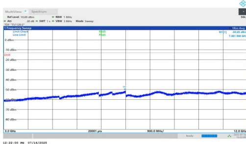
NTNV-n2-PC2-15-10-M-DFT-BPSK-Inner_1RB_Left-3000-12000-PASS PASS
