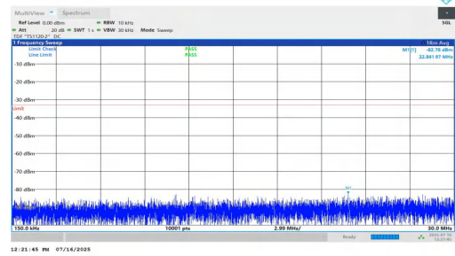
NTNV-n2-PC2-15-10-M-DFT-BPSK-Inner_1RB_Left-0.15-30-PAS S
