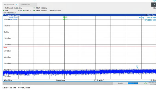
NTNV-n2-PC2-15-5-H-DFT-BPSK-Inner_1RB_Right-30-1000-PA SS
