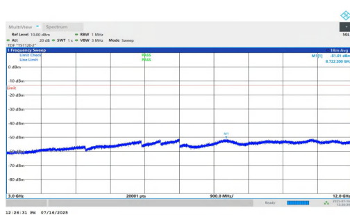
NTNV-n2-PC2-15-10-H-DFT-QPSK-Inner_1RB_Right-3000-12000-PASS
