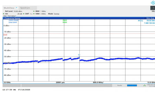
NTNV-n2-PC2-15-5-H-DFT-QPSK-Inner_1RB_Left-3000-12000-P ASS
