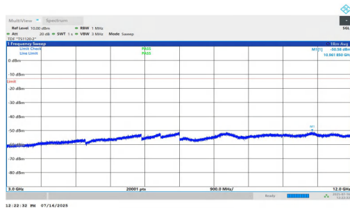
NTNV-n2-PC2-15-10-M-DFT-BPSK-Inner_1RB_Right-3000-12000-P PASS
