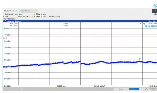
NTNV-n2-PC2-15-10-L-DFT-QPSK-Inner_1RB_Right-3000-12000-PASS
