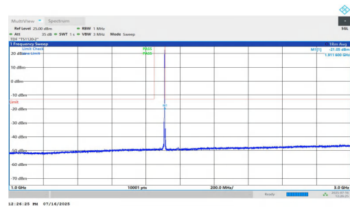
NTNV-n2-PC2-15-10-H-DFT-QPSK-Inner_1RB_Right-1000-3000-PASS
