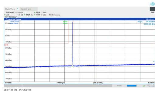
NTNV-n2-PC2-15-5-H-DFT-QPSK-Inner_1RB_Left-1000-3000-PA SS
