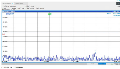
NTNV-n2-PC2-15-15-L-DFT-BPSK-Inner_1RB_Left-0.009-0.15-P ASS
