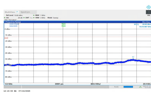
NTNV-n2-PC2-15-5-M-DFT-QPSK-Inner_1RB_Right-12000-20000-PASS
