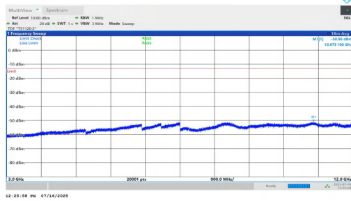
NTNV-n2-PC2-15-10-H-DFT-QPSK-Inner_1RB_Left-3000-12000-PASS
