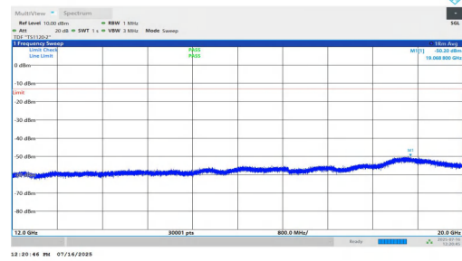
NTNV-n2-PC2-15-10-L-DFT-QPSK-Inner_1RB_Left-12000-20000-PASS
