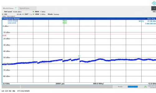
NTNV-n2-PC2-15-10-L-DFT-BPSK-Inner_1RB_Right-3000-12000 -PASS
