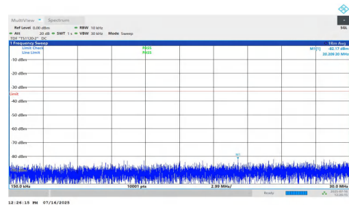
NTNV-n2-PC2-15-10-H-DFT-QPSK-Inner_1RB_Right-0.15-30-PA-SS
