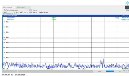
NTNV-n2-PC2-15-5-H-DFT-QPSK-Inner_1RB_Left-0.009-0.15-P ASS
