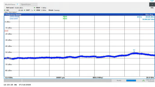
NTNV-n2-PC2-15-10-M-DFT-QPSK-Inner_1RB_Left-12000-20000 -PASS
