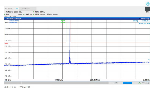
NTNV-n2-PC2-15-10-H-DFT-BPSK-Inner_1RB_Left-1000-3000-PASS
