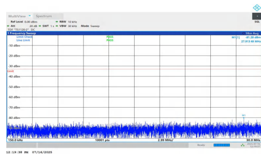
NTNV-n2-PC2-15-10-L-DFT-BPSK-Inner_1RB_Right-0.15-30-PASS S
