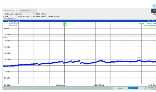
NTNV-n2-PC2-15-5-H-DFT-QPSK-Inner_1RB_Right-3000-12000 -PASS
