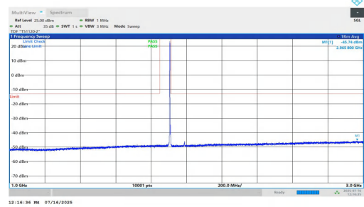
NTNV-n2-PC2-15-5-H-DFT-BPSK-Inner_1RB_Left-1000-3000-PA SS
