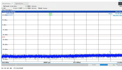
NTNV-n2-PC2-15-10-L-DFT-BPSK-Inner_1RB_Right-30-1000-PA SS
