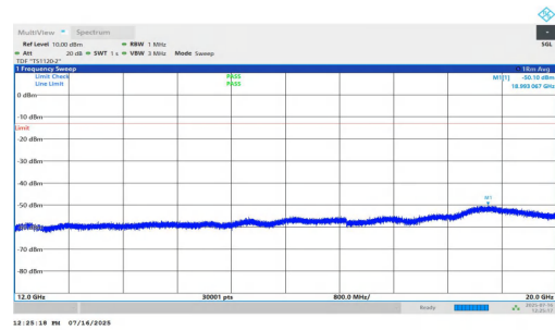
NTNV-n2-PC2-15-10-H-DFT-BPSK-Inner_1RB_Right-12000-2000 0-PASS
