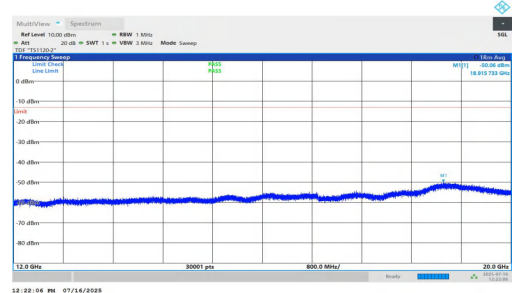
NTNV-n2-PC2-15-10-M-DFT-BPSK-Inner_1RB_Left-12000-20000-PASS PASS
