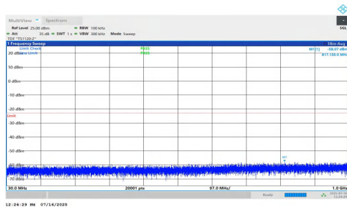
NTNV-n2-PC2-15-10-H-DFT-BPSK-Inner_1RB_Left-30-1000-PASS
