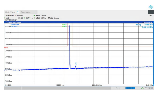
NTNV-n2-PC2-15-10-M-DFT-QPSK-Inner_1RB_Left-1000-3000-P PASS
