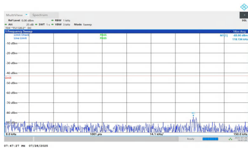
NTNV-n2-PC2-15-10-H-DFT-QPSK-Inner_1RB_Left-0.009-0.15-P ASS
