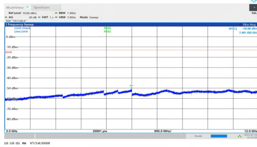
NTNV-n2-PC2-15-5-M-DFT-QPSK-Inner_1RB_Left-3000-12000-PASS
