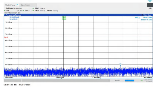
NTNV-n2-PC2-15-5-H-DFT-BPSK-Inner_1RB_Left-0.15-30-PASS
