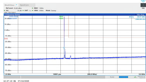
NTNV-n2-PC2-15-15-L-DFT-BPSK-Inner_1RB_Left-1000-3000-PASS
