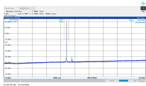
NTNV-n2-PC2-15-10-M-DFT-QPSK-Inner_1RB_Right-1000-3000-P PASS
