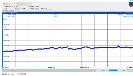
NTNV-n2-PC2-15-10-M-DFT-QPSK-Inner_1RB_Left-3000-12000 -PASS
