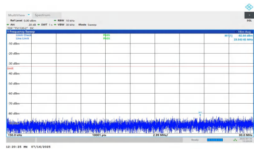
NTNV-n2-PC2-15-10-L-DFT-QPSK-Inner_1RB_Left-0.15-30-PASS
