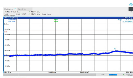
NTNV-n2-PC2-15-5-H-DFT-QPSK-Inner_1RB_Right-12000-20000 -PASS
