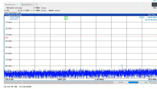
NTNV-n2-PC2-15-10-L-DFT-BPSK-Inner_1RB_Left-0.15-30-PASS
