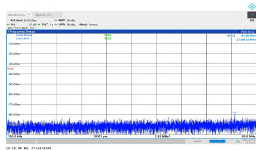
NTNV-n2-PC2-15-5-M-DFT-QPSK-Inner_1RB_Right-0.15-30-PASS
