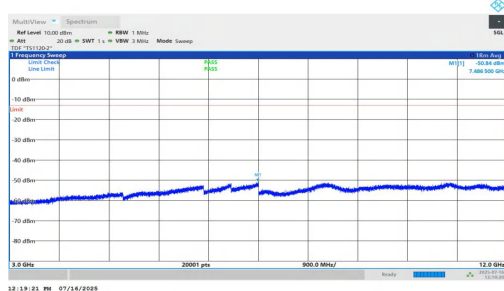
NTNV-n2-PC2-15-10-L-DFT-BPSK-Inner_1RB_Left-3000-12000- PASS
