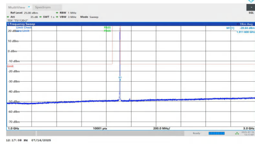
NTNV-n2-PC2-15-5-H-DFT-BPSK-Inner_1RB_Right-1000-3000-P ASS
