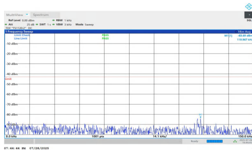
NTNV-n2-PC2-15-5-H-DFT-QPSK-Inner_1RB_Right-0.009-0.15- PASS
