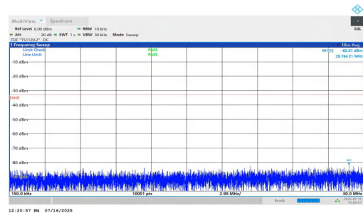
NTNV-n2-PC2-15-10-L-DFT-QPSK-Inner_1RB_Right-0.15-30-PASS
