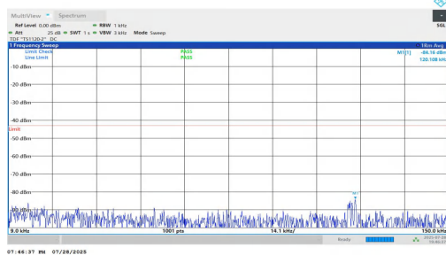
NTNV-n2-PC2-15-10-M-DFT-QPSK-Inner_1RB_Right-0.009-0.15 -PASS
