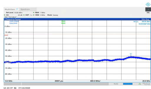
NTNV-n2-PC2-15-10-M-DFT-QPSK-Inner_1RB_Right-12000-2000 0-PASS
