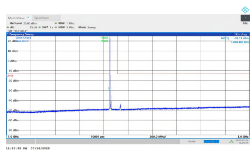
NTNV-n2-PC2-15-10-L-DFT-QPSK-Inner_1RB_Left-1000-3000-PA SS
