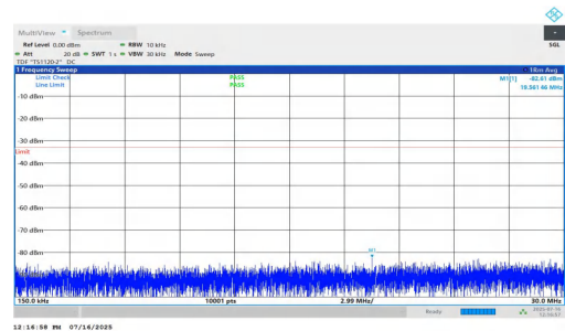
NTNV-n2-PC2-15-5-H-DFT-BPSK-Inner_1RB_Right-0.15-30-PAS S
