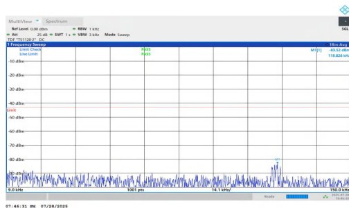
NTNV-n2-PC2-15-10-M-DFT-QPSK-Inner_1RB_Left-0.009-0.15-P PASS
