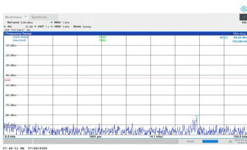
NTNV-n2-PC2-15-10-M-DFT-BPSK-Inner_1RB_Right-0.009-0.15 -PASS
