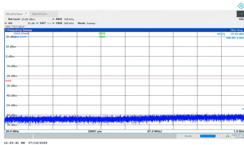
NTNV-n2-PC2-15-10-M-DFT-QPSK-Inner_1RB_Right-30-1000-P ASS
