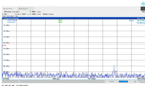
NTNV-n2-PC2-15-15-L-DFT-BPSK-Inner_1RB_Right-0.009-0.15- PASS
