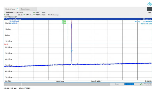
NTNV-n2-PC2-15-5-H-DFT-QPSK-Inner_1RB_Right-1000-3000-P ASS
