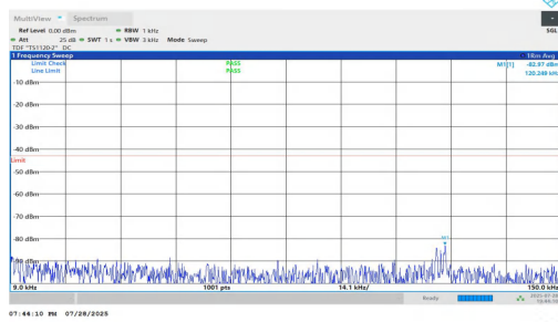
NTNV-n2-PC2-15-5-H-DFT-BPSK-Inner_1RB_Left-0.009-0.15-PA SS
