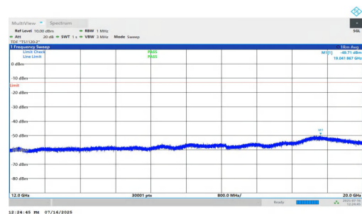
NTNV-n2-PC2-15-10-H-DFT-BPSK-Inner_1RB_Left-12000-20000-PASS
