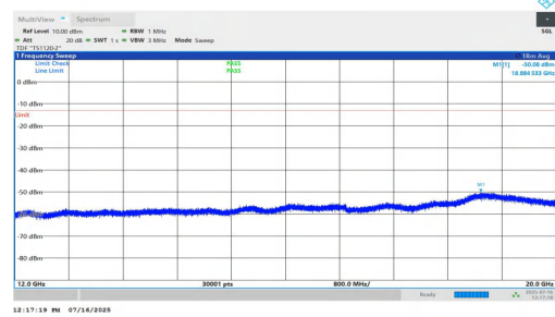
NTNV-n2-PC2-15-5-H-DFT-BPSK-Inner_1RB_Right-12000-20000- PASS
