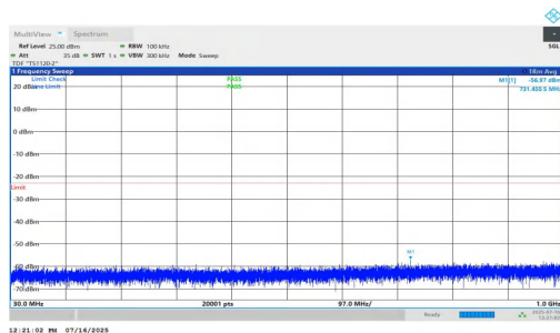
NTNV-n2-PC2-15-10-L-DFT-QPSK-Inner_1RB_Right-30-1000-PASS
