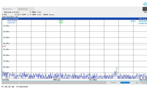
NTNV-n2-PC2-15-10-L-DFT-QPSK-Inner_1RB_Left-0.009-0.15-P ASS
