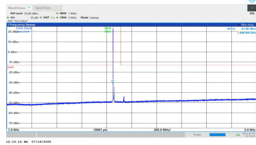
NTNV-n2-PC2-15-10-L-DFT-BPSK-Inner_1RB_Left-1000-3000-PASS S
