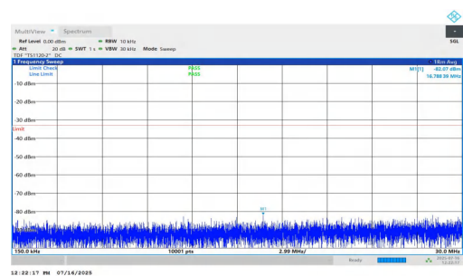
NTNV-n2-PC2-15-10-M-DFT-BPSK-Inner_1RB_Right-0.15-30-PASS SS
