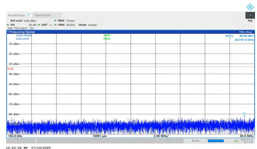
NTNV-n2-PC2-15-10-M-DFT-QPSK-Inner_1RB_Left-0.15-30-P PASS
