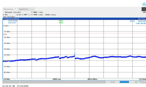
NTNV-n2-PC2-15-10-M-DFT-QPSK-Inner_1RB_Right-3000-1200 0-PASS
