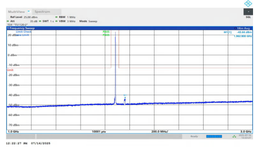
NTNV-n2-PC2-15-10-M-DFT-BPSK-Inner_1RB_Right-1000-3000-P PASS
