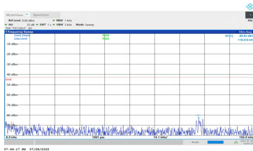
NTNV-n2-PC2-15-5-H-DFT-BPSK-Inner_1RB_Right-0.009-0.15-P ASS
