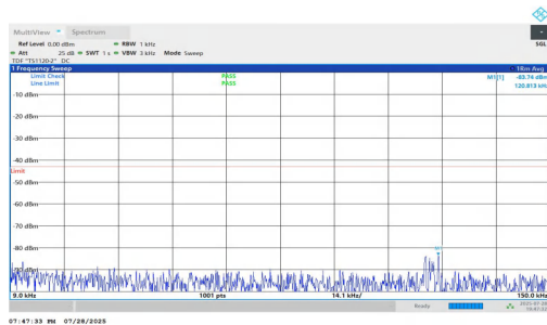
NTNV-n2-PC2-15-10-H-DFT-QPSK-Inner_1RB_Right-0.009-0.15-PASS
