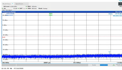
NTNV-n2-PC2-15-10-M-DFT-BPSK-Inner_1RB_Left-30-1000-PASS SS
