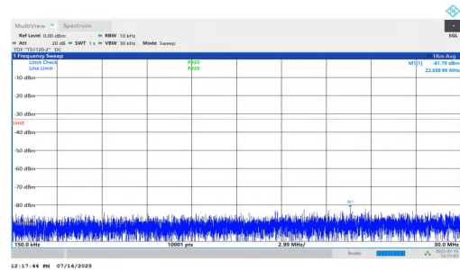
NTNV-n2-PC2-15-5-H-DFT-QPSK-Inner_1RB_Left-0.15-30-PASS
