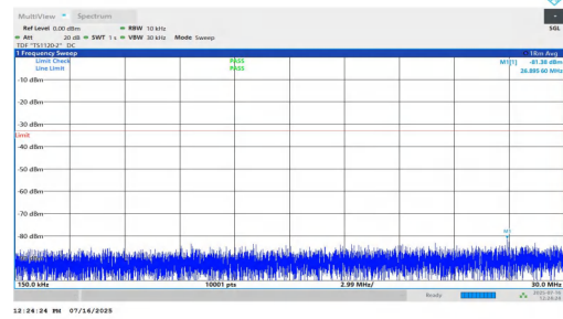
NTNV-n2-PC2-15-10-H-DFT-BPSK-Inner_1RB_Left-0.15-30-PASS
