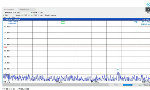
NTNV-n2-PC2-15-10-L-DFT-BPSK-Inner_1RB_Right-0.009-0.15- PASS
