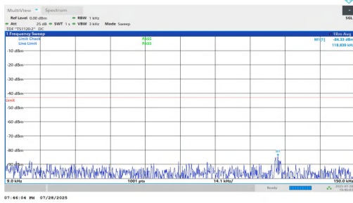
NTNV-n2-PC2-15-10-M-DFT-BPSK-Inner_1RB_Left-0.009-0.15-P ASS
