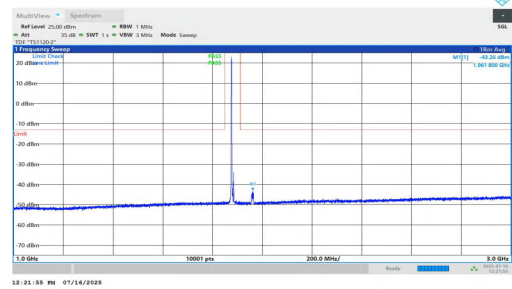
NTNV-n2-PC2-15-10-M-DFT-BPSK-Inner_1RB_Left-1000-3000-P ASS
