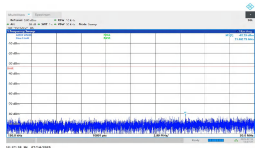
NTNV-n2-PC2-15-15-L-DFT-BPSK-Inner_1RB_Right-0.15-30-PASS
