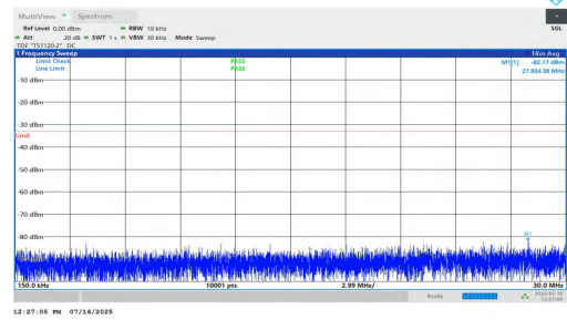
NTNV-n2-PC2-15-15-L-DFT-BPSK-Inner_1RB_Left-0.15-30-PASS
