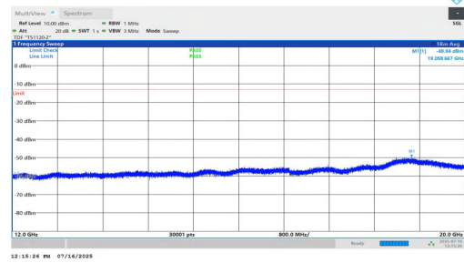
NTNV-n2-PC2-15-5-M-DFT-QPSK-Inner_1RB_Left-12000-20000-PASS
