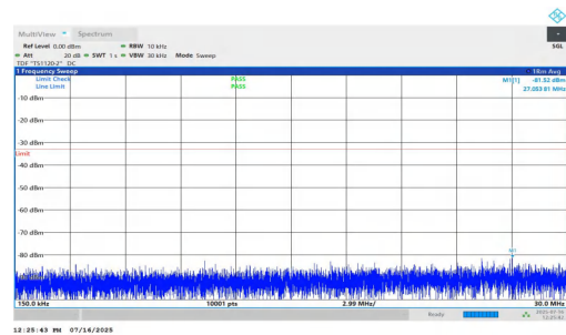
NTNV-n2-PC2-15-10-H-DFT-QPSK-Inner_1RB_Left-0.15-30-PAS S
