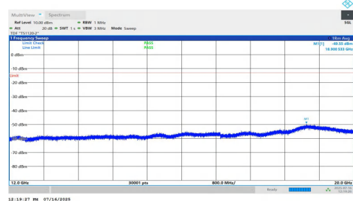
NTNV-n2-PC2-15-10-L-DFT-BPSK-Inner_1RB_Left-12000-20000- PASS
