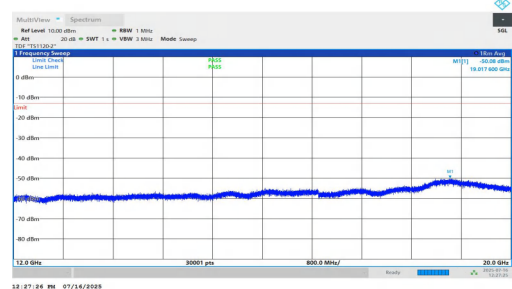
NTNV-n2-PC2-15-15-L-DFT-BPSK-Inner_1RB_Left-12000-20000- PASS
