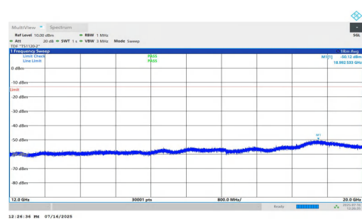
NTNV-n2-PC2-15-10-H-DFT-QPSK-Inner_1RB_Right-12000-20000-PASS
