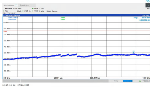
NTNV-n2-PC2-15-5-H-DFT-BPSK-Inner_1RB_Right-3000-12000- PASS
