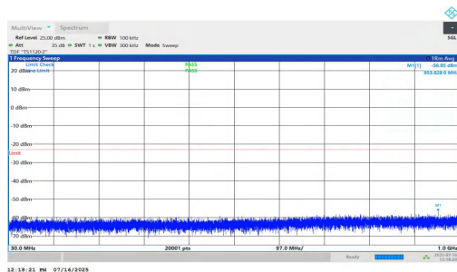
NTNV-n2-PC2-15-5-H-DFT-QPSK-Inner_1RB_Right-30-1000-PA SS
