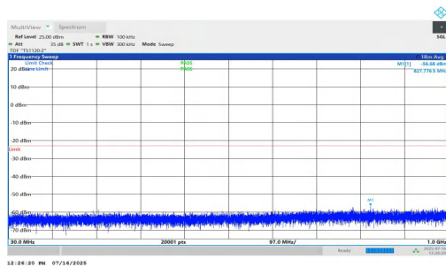
NTNV-n2-PC2-15-10-H-DFT-QPSK-Inner_1RB_Right-30-1000-PASS
