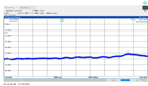
NTNV-n2-PC2-15-10-L-DFT-BPSK-Inner_1RB_Right-12000-2000 0-PASS
