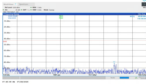
NTNV-n2-PC2-15-10-L-DFT-BPSK-Inner_1RB_Left-0.009-0.15-P ASS
