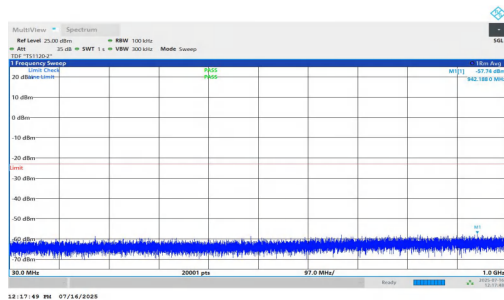
NTNV-n2-PC2-15-5-H-DFT-QPSK-Inner_1RB_Left-30-1000-PAS S
