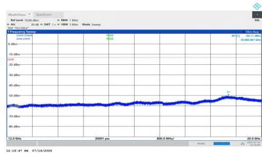
NTNV-n2-PC2-15-5-H-DFT-BPSK-Inner_1RB_Left-12000-20000-P ASS
