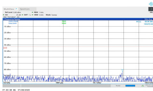
NTNV-n2-PC2-15-5-M-DFT-QPSK-Inner_1RB_Right-0.009-0.15-PASS
