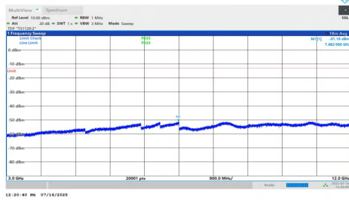
NTNV-n2-PC2-15-10-L-DFT-QPSK-Inner_1RB_Left-3000-12000-PASS
