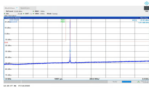
NTNV-n2-PC2-15-10-H-DFT-BPSK-Inner_1RB_Right-1000-3000-P PASS
