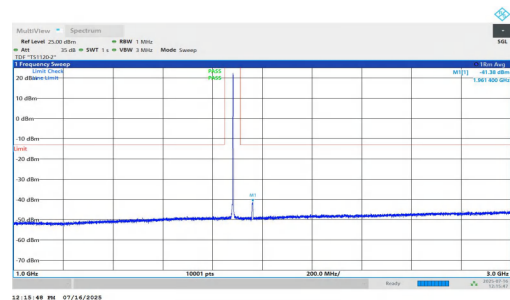
NTNV-n2-PC2-15-5-M-DFT-QPSK-Inner_1RB_Right-1000-3000-PASS
