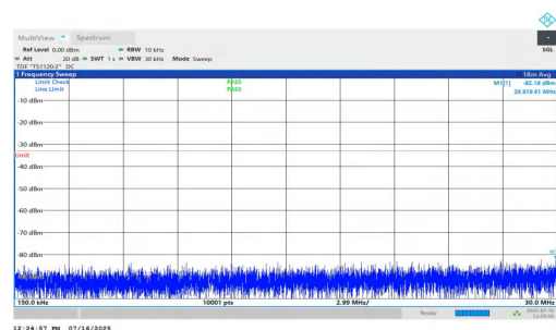
NTNV-n2-PC2-15-10-H-DFT-BPSK-Inner_1RB_Right-0.15-30-PASS
