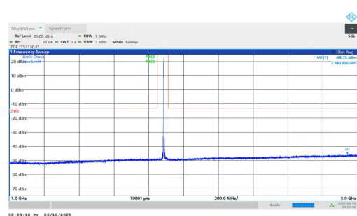
NTNV-n2-PC3-15-25-H-DFT-QPSK-Inner_1RB_Left-1000-3000-P ASS
