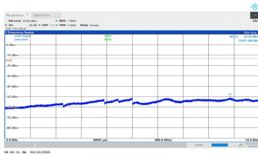
NTNV-n2-PC3-15-30-H-DFT-BPSK-Inner_1RB_Right-3000-12000 0-PASS
