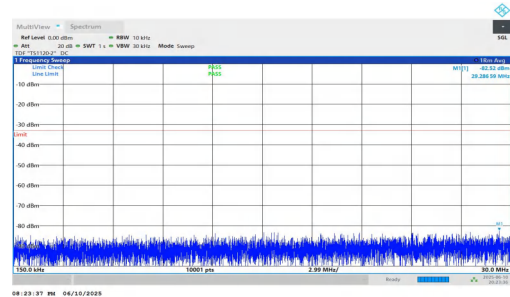
NTVN-n2-PC3-15-25-H-DFT-QPSK-Inner_1RB_Right-0.15-30-PA-SS
