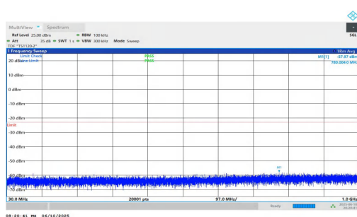
NTNV-n2-PC3-15-25-M-DFT-QPSK-Inner_1RB_Left-30-1000-PA SS
