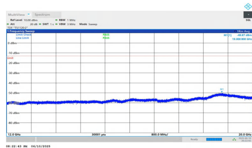
NTNV-n2-PC3-15-25-H-DFT-BPSK-Inner_1RB_Right-12000-20000 0-PASS
