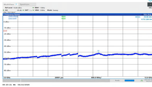
NTVN-n2-PC3-15-25-H-DFT-QPSK-Inner_1RB_Left-3000-12000-PASS
