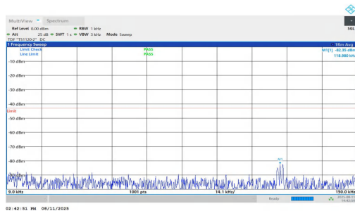
NTNV-n2-PC3-15-30-H-DFT-BPSK-Inner_1RB_Right-0.009-0.15- PASS
