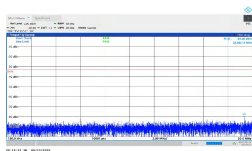
NTNV-n2-PC3-15-25-M-DFT-BPSK-Inner_1RB_Right-0.15-30-PASS SS
