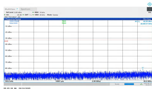
NTNV-n2-PC3-15-25-M-DFT-QPSK-Inner_1RB_Left-0.15-30-PAS S
