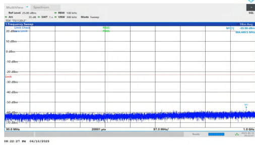
NTNV-n2-PC3-15-25-H-DFT-BPSK-Inner_1RB_Right-30-1000-P ASS
