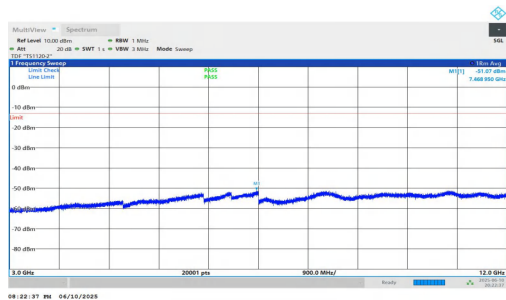
NTNV-n2-PC3-15-25-H-DFT-BPSK-Inner_1RB_Right-3000-12000 0-PASS
