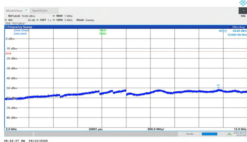
NTNV-n2-PC3-15-25-H-DFT-BPSK-Inner_1RB_Left-3000-12000-PASS
