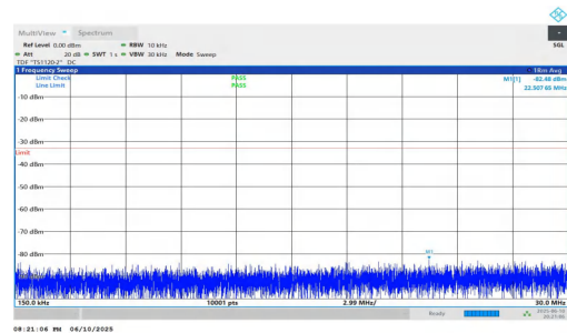
NTNV-n2-PC3-15-25-M-DFT-QPSK-Inner_1RB_Right-0.15-30-PA SS
