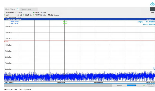
NTNV-n2-PC3-15-30-M-DFT-QPSK-Inner_1RB_Left-0.15-30-PAS S
