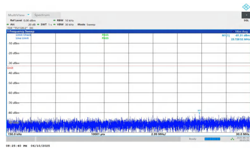
NTNV-n2-PC3-15-30-L-DFT-QPSK-Inner_1RB_Left-0.15-30-PASS
