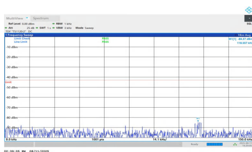
NTNV-n2-PC3-15-25-M-DFT-BPSK-Inner_1RB_Right-0.009-0.15 -PASS
