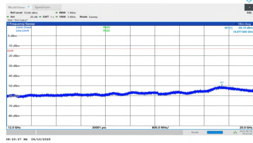
NTVN-n2-PC3-15-25-H-DFT-QPSK-Inner_1RB_Left-12000-20000-PASS
