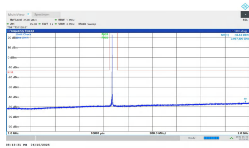
NTNV-n2-PC3-15-25-M-DFT-BPSK-Inner_1RB_Left-1000-3000-P ASS
