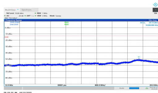
NTNV-n2-PC3-15-30-M-DFT-QPSK-Inner_1RB_Right-12000-2000 0-PASS
