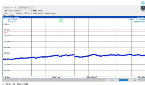
NTNV-n2-PC3-15-25-M-DFT-BPSK-Inner_1RB_Right-3000-1200 0-PASS
