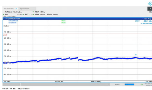
NTNV-n2-PC3-15-30-L-DFT-BPSK-Inner_1RB_Left-3000-12000-PASS
