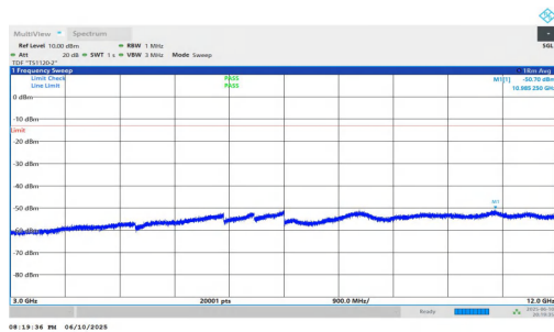
NTNV-n2-PC3-15-25-M-DFT-BPSK-Inner_1RB_Left-3000-12000-PASS PASS
