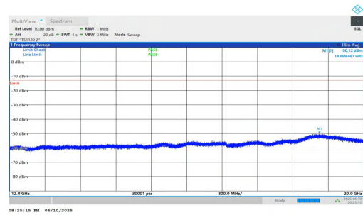
NTNV-n2-PC3-15-30-L-DFT-BPSK-Inner_1RB_Right-12000-2000 0-PASS
