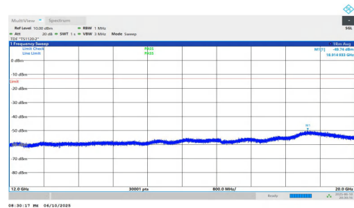
NTNV-n2-PC3-15-30-H-DFT-BPSK-Inner_1RB_Right-12000-20000 0-PASS
