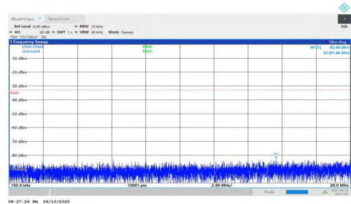
NTNV-n2-PC3-15-30-M-DFT-BPSK-Inner_1RB_Right-0.15-30-PASS
