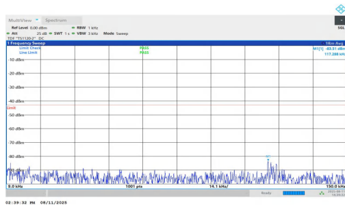
NTNV-n2-PC3-15-25-M-DFT-QPSK-Inner_1RB_Right-0.009-0.15 -PASS
