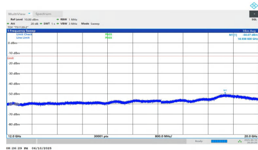
NTNV-n2-PC3-15-30-L-DFT-QPSK-Inner_1RB_Right-12000-2000 0-PASS
