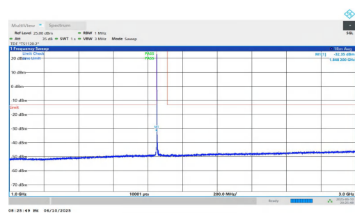
NTNV-n2-PC3-15-30-L-DFT-QPSK-Inner_1RB_Left-1000-3000-PA SS
