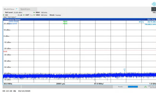
NTNV-n2-PC3-15-25-M-DFT-BPSK-Inner_1RB_Left-30-1000-PASS SS
