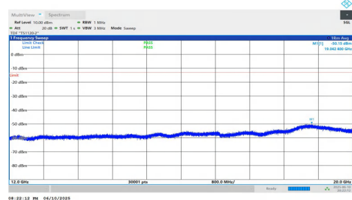
NTNV-n2-PC3-15-25-H-DFT-BPSK-Inner_1RB_Left-12000-20000-PASS
