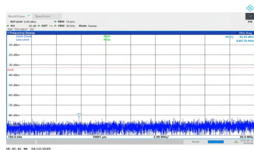
NTNV-n2-PC3-15-30-H-DFT-QPSK-Inner_1RB_Left-0.15-30-PAS S
