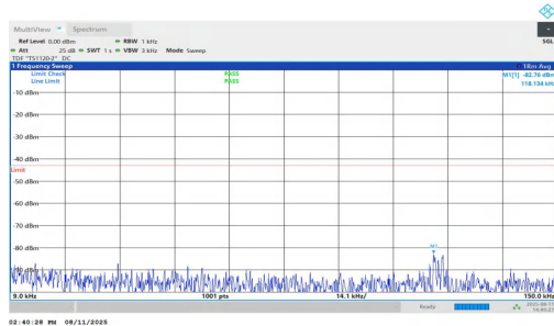
NTVN-n2-PC3-15-25-H-DFT-QPSK-Inner_1RB_Right-0.009-0.15-PASS
