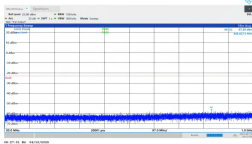
NTNV-n2-PC3-15-30-M-DFT-BPSK-Inner_1RB_Left-30-1000-PASS
