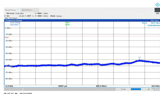
NTVN-n2-PC3-15-25-H-DFT-QPSK-Inner_1RB_Right-12000-20000-PASS
