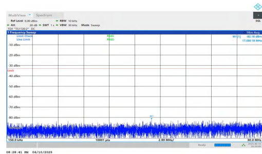
NTNV-n2-PC3-15-30-M-DFT-QPSK-Inner_1RB_Right-0.15-30-PA SS
