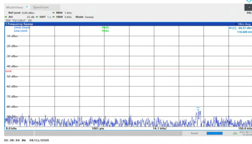
NTNV-n2-PC3-15-25-M-DFT-BPSK-Inner_1RB_Left-0.009-0.15-P ASS
