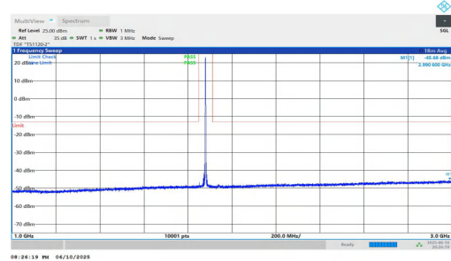
NTNV-n2-PC3-15-30-L-DFT-QPSK-Inner_1RB_Right-1000-3000-P ASS
