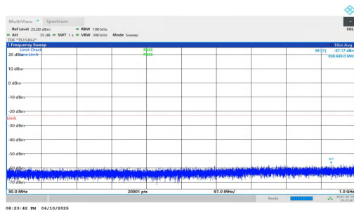
NTVN-n2-PC3-15-25-H-DFT-QPSK-Inner_1RB_Right-30-1000-PASS
