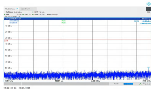
NTNV-n2-PC3-15-25-H-DFT-BPSK-Inner_1RB_Right-0.15-30-PASS
