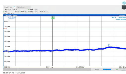
NTNV-n2-PC3-15-30-H-DFT-BPSK-Inner_1RB_Left-12000-20000- PASS
