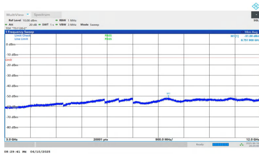
NTNV-n2-PC3-15-30-H-DFT-BPSK-Inner_1RB_Left-3000-12000- PASS
