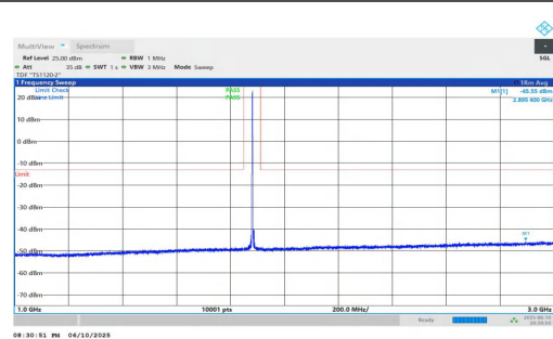
NTNV-n2-PC3-15-30-H-DFT-QPSK-Inner_1RB_Left-1000-3000-P ASS
