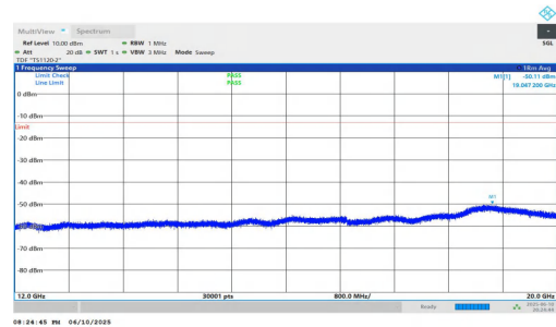
NTNV-n2-PC3-15-30-L-DFT-BPSK-Inner_1RB_Left-12000-20000-PASS
