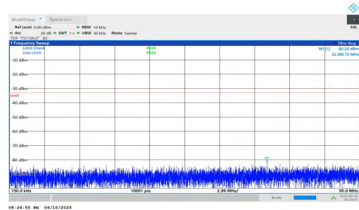
NTNV-n2-PC3-15-30-L-DFT-BPSK-Inner_1RB_Right-0.15-30-PASS S
