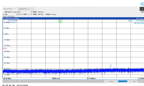
NTNV-n2-PC3-15-30-M-DFT-QPSK-Inner_1RB_Right-30-1000-P ASS
