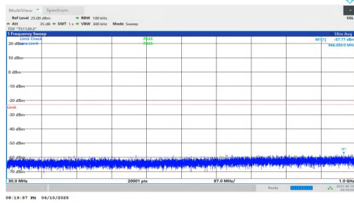
NTNV-n2-PC3-15-25-M-DFT-BPSK-Inner_1RB_Right-30-1000-P ASS
