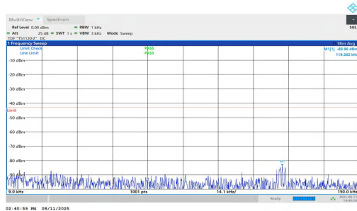
NTNV-n2-PC3-15-30-L-DFT-BPSK-Inner_1RB_Right-0.009-0.15-PASS
