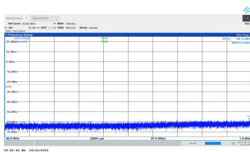
NTNV-n2-PC3-15-30-L-DFT-QPSK-Inner_1RB_Left-30-1000-PA SS
