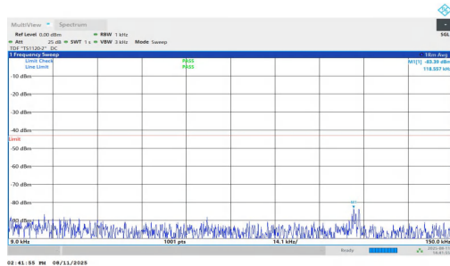
NTNV-n2-PC3-15-30-M-DFT-BPSK-Inner_1RB_Right-0.009-0.15 -PASS
