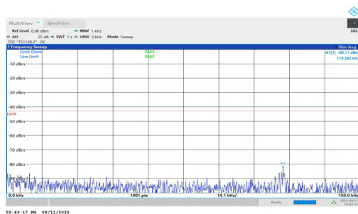
NTNV-n2-PC3-15-30-H-DFT-QPSK-Inner_1RB_Left-0.009-0.15-P ASS
