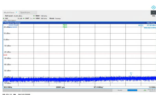
NTNV-n2-PC3-15-25-H-DFT-QPSK-Inner_1RB_Left-30-1000-P ASS
