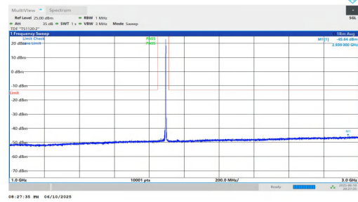
NTNV-n2-PC3-15-30-M-DFT-BPSK-Inner_1RB_Right-1000-3000-P PASS
