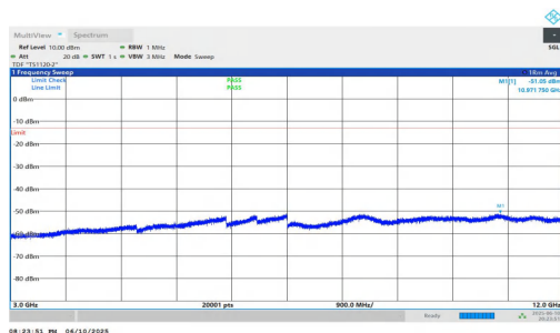
NTVN-n2-PC3-15-25-H-DFT-QPSK-Inner_1RB_Right-3000-12000-PASS
