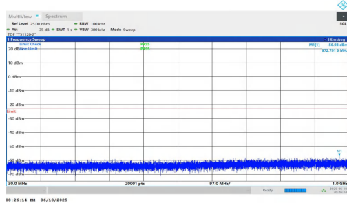
NTNV-n2-PC3-15-30-L-DFT-QPSK-Inner_1RB_Right-30-1000-P ASS
