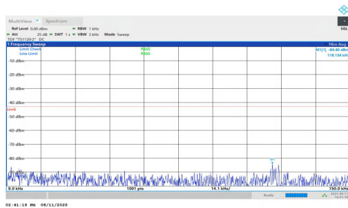
NTNV-n2-PC3-15-30-L-DFT-QPSK-Inner_1RB_Left-0.009-0.15-P ASS
