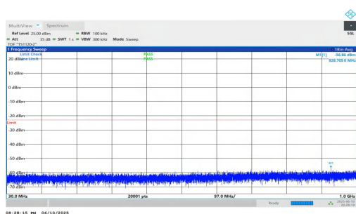
NTNV-n2-PC3-15-30-M-DFT-QPSK-Inner_1RB_Left-30-1000-PA SS
