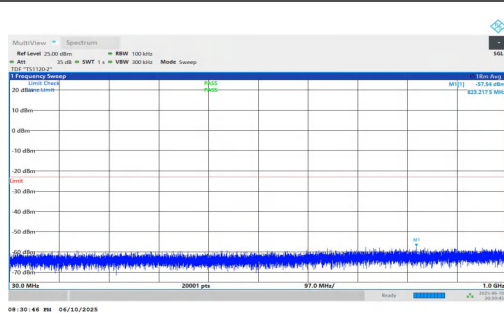
NTNV-n2-PC3-15-30-H-DFT-QPSK-Inner_1RB_Left-30-1000-P ASS
