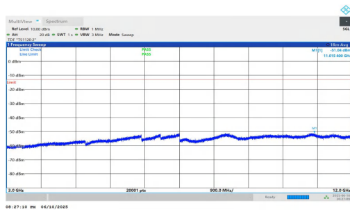
NTNV-n2-PC3-15-30-M-DFT-BPSK-Inner_1RB_Left-3000-12000-PASS
