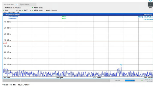
NTNV-n2-PC3-15-25-H-DFT-BPSK-Inner_1RB_Left-0.009-0.15-P ASS
