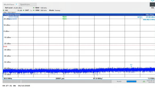
NTNV-n2-PC3-15-30-M-DFT-BPSK-Inner_1RB_Right-30-1000-P ASS
