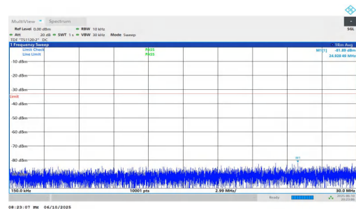
NTNV-n2-PC3-15-25-H-DFT-QPSK-Inner_1RB_Left-0.15-30-PAS S
