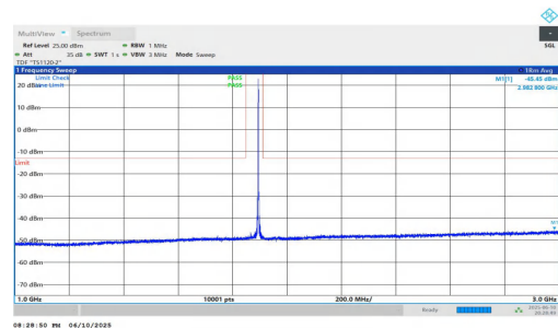
NTNV-n2-PC3-15-30-M-DFT-QPSK-Inner_1RB_Right-1000-3000- PASS
