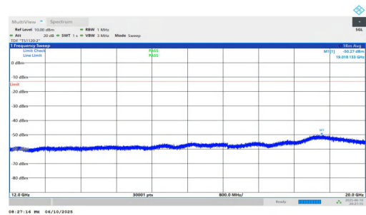
NTNV-n2-PC3-15-30-M-DFT-BPSK-Inner_1RB_Left-12000-20000-PASS
