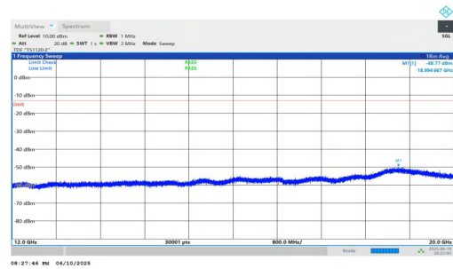
NTNV-n2-PC3-15-30-M-DFT-BPSK-Inner_1RB_Right-12000-2000 0-PASS
