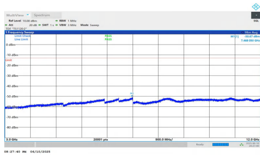
NTNV-n2-PC3-15-30-M-DFT-BPSK-Inner_1RB_Right-3000-1200 0-PASS
