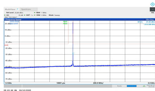
NTVN-n2-PC3-15-25-H-DFT-QPSK-Inner_1RB_Right-1000-3000-PASS
