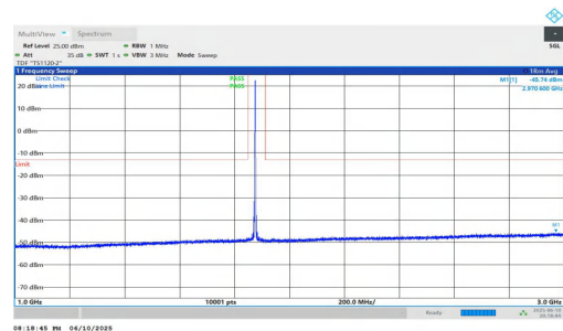
NTNV-n2-PC3-15-25-L-DFT-QPSK-Inner_1RB_Right-1000-3000-PASS
