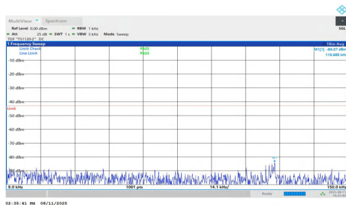
NTNV-n2-PC3-15-20-L-DFT-QPSK-Inner_1RB_Left-0.009-0.15-P ASS
