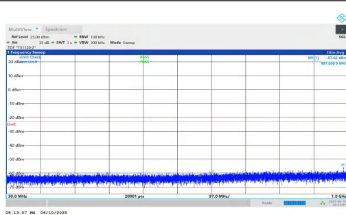
NTNV-n2-PC3-15-20-M-DFT-QPSK-Inner_1RB_Left-30-1000-PA SS
