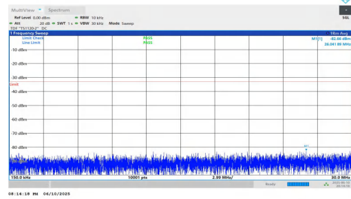
NTNV-n2-PC3-15-20-H-DFT-BPSK-Inner_1RB_Left-0.15-30-PASS
