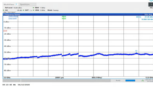
NTNV-n2-PC3-15-20-L-DFT-QPSK-Inner_1RB_Left-3000-12000-PASS
