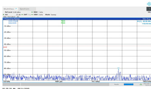
NTNV-n2-PC3-15-20-L-DFT-BPSK-Inner_1RB_Right-0.009-0.15-PASS
