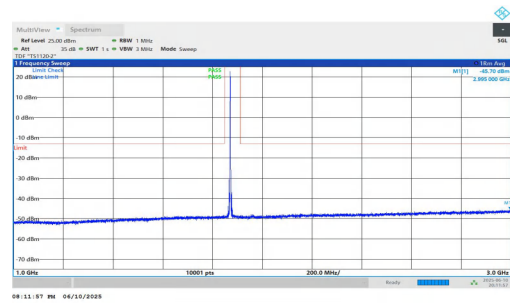
NTNV-n2-PC3-15-20-M-DFT-BPSK-Inner_1RB_Left-1000-3000-PASS
