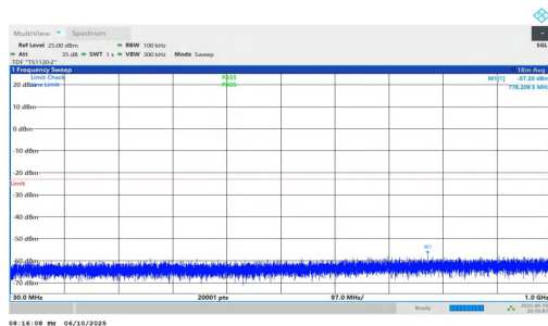
NTNV-n2-PC3-15-20-H-DFT-QPSK-Inner_1RB_Right-30-1000-PASS
