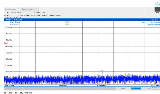
NTNV-n2-PC3-15-25-L-DFT-QPSK-Inner_1RB_Right-0.15-30-PASS
