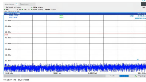
NTNV-n2-PC3-15-20-M-DFT-BPSK-Inner_1RB_Left-0.15-30-PASS
