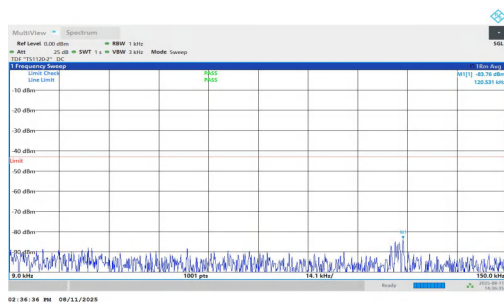
NTNV-n2-PC3-15-20-M-DFT-QPSK-Inner_1RB_Left-0.009-0.15- PASS
