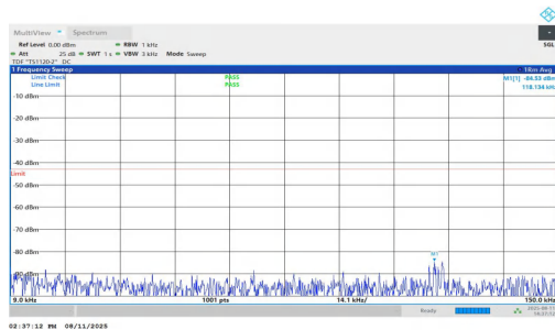
NTNV-n2-PC3-15-20-H-DFT-BPSK-Inner_1RB_Right-0.009-0.15-PASS
