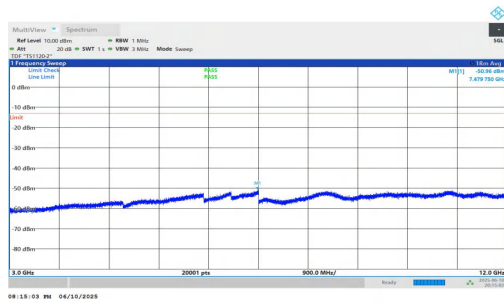
NTNV-n2-PC3-15-20-H-DFT-BPSK-Inner_1RB_Right-3000-1200 0-PASS
