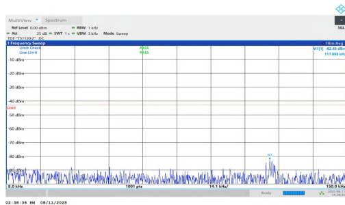
NTNV-n2-PC3-15-25-L-DFT-QPSK-Inner_1RB_Right-0.009-0.15-PASS
