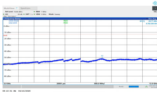
NTNV-n2-PC3-15-20-L-DFT-BPSK-Inner_1RB_Right-3000-12000 -PASS
