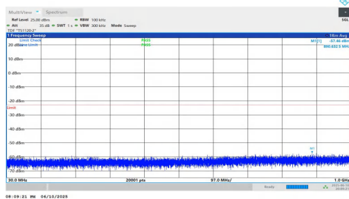
NTNV-n2-PC3-15-20-L-DFT-BPSK-Inner_1RB_Left-30-1000-PAS S
