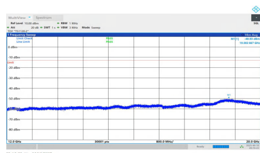
NTNV-n2-PC3-15-20-H-DFT-QPSK-Inner_1RB_Right-12000-20000-PASS
