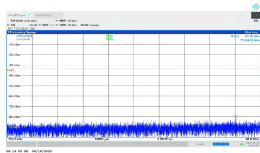
NTNV-n2-PC3-15-20-H-DFT-QPSK-Inner_1RB_Right-0.15-30-PA-SS
