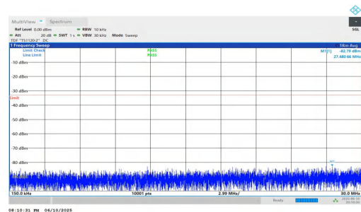
NTNV-n2-PC3-15-20-L-DFT-QPSK-Inner_1RB_Left-0.15-30-PASS
