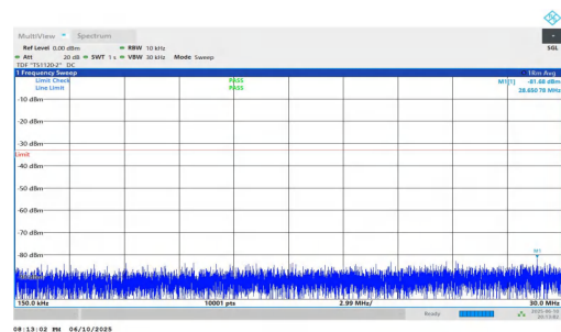
NTNV-n2-PC3-15-20-M-DFT-QPSK-Inner_1RB_Left-0.15-30-PAS S
