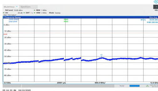
NTNV-n2-PC3-15-20-H-DFT-BPSK-Inner_1RB_Left-3000-12000-PASS
