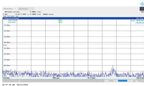
NTNV-n2-PC3-15-20-H-DFT-QPSK-Inner_1RB_Left-0.009-0.15-P ASS
