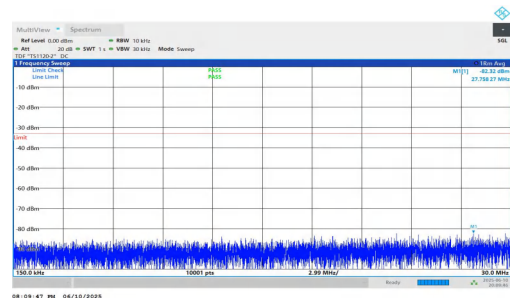
NTNV-n2-PC3-15-20-L-DFT-BPSK-Inner_1RB_Right-0.15-30-PASS S
