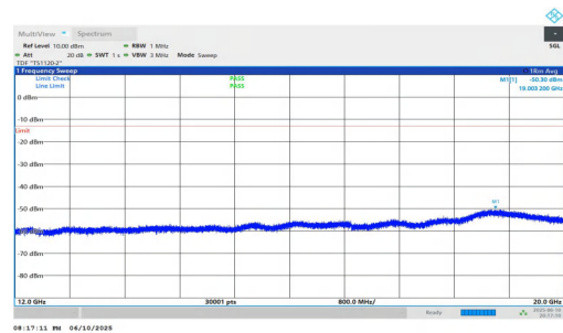
NTNV-n2-PC3-15-25-L-DFT-BPSK-Inner_1RB_Left-12000-20000-PASS
