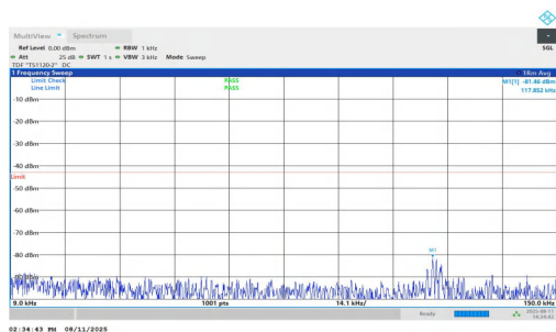
NTNV-n2-PC3-15-15-H-DFT-QPSK-Inner_1RB_Left-0.009-0.15-P ASS
