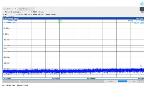
NTNV-n2-PC3-15-25-L-DFT-QPSK-Inner_1RB_Right-30-1000-PASS
