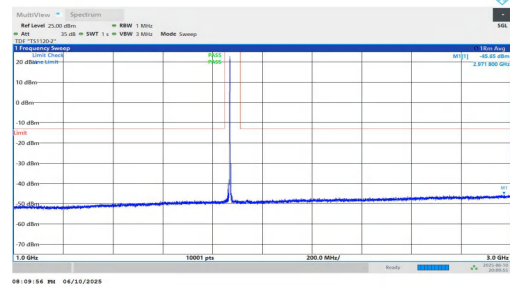
NTNV-n2-PC3-15-20-L-DFT-BPSK-Inner_1RB_Right-1000-3000-P ASS
