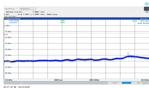
NTNV-n2-PC3-15-15-H-DFT-BPSK-Inner_1RB_Right-12000-2000 0-PASS
