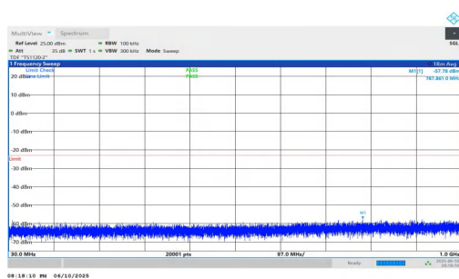
NTNV-n2-PC3-15-25-L-DFT-QPSK-Inner_1RB_Left-30-1000-PA SS
