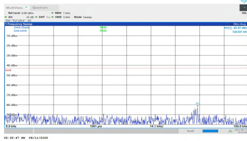
NTNV-n2-PC3-15-20-L-DFT-QPSK-Inner_1RB_Right-0.009-0.15-PASS
