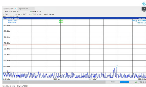
NTNV-n2-PC3-15-15-H-DFT-QPSK-Inner_1RB_Right-0.009-0.15-PASS
