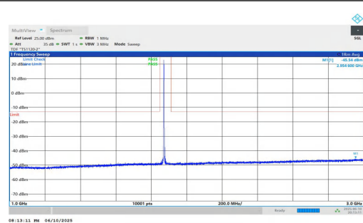
NTNV-n2-PC3-15-20-M-DFT-QPSK-Inner_1RB_Left-1000-3000-P ASS
