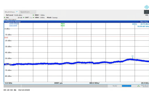
NTNV-n2-PC3-15-25-L-DFT-QPSK-Inner_1RB_Right-12000-20000-PASS
