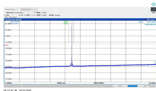
NTNV-n2-PC3-15-20-M-DFT-QPSK-Inner_1RB_Right-1000-3000- PASS
