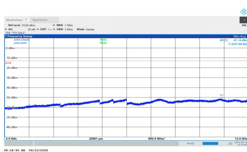
NTNV-n2-PC3-15-25-L-DFT-QPSK-Inner_1RB_Right-3000-12000-PASS
