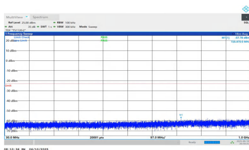
NTNV-n2-PC3-15-20-L-DFT-QPSK-Inner_1RB_Left-30-1000-PA SS
