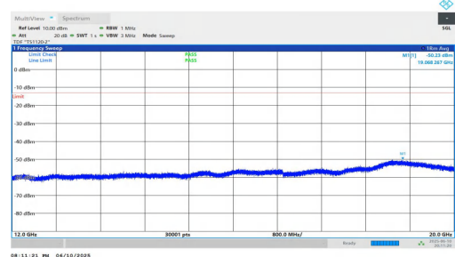
NTNV-n2-PC3-15-20-L-DFT-QPSK-Inner_1RB_Right-12000-20000-PASS
