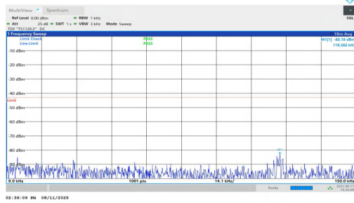
NTNV-n2-PC3-15-20-M-DFT-BPSK-Inner_1RB_Left-0.009-0.15-PASS
