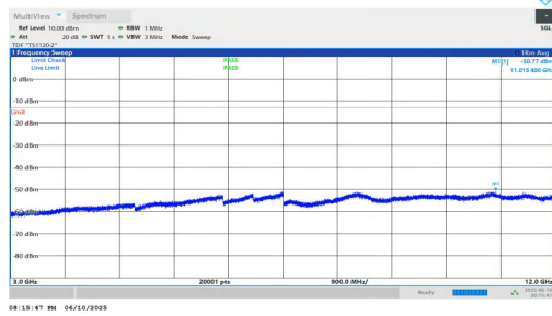
NTNV-n2-PC3-15-20-H-DFT-QPSK-Inner_1RB_Left-3000-12000-PASS
