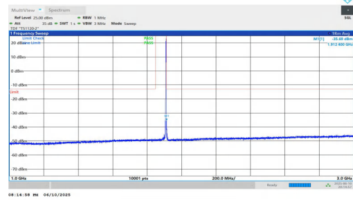
NTNV-n2-PC3-15-20-H-DFT-BPSK-Inner_1RB_Right-1000-3000-P PASS
