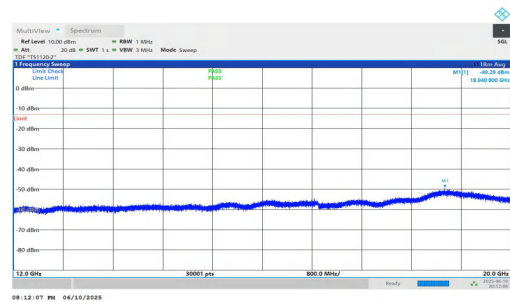
NTNV-n2-PC3-15-20-M-DFT-BPSK-Inner_1RB_Left-12000-20000-PASS
