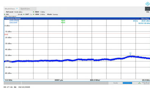
NTNV-n2-PC3-15-25-L-DFT-BPSK-Inner_1RB_Right-12000-2000 0-PASS
