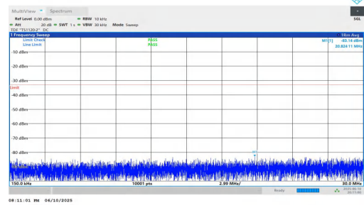
NTNV-n2-PC3-15-20-L-DFT-QPSK-Inner_1RB_Right-0.15-30-PASS
