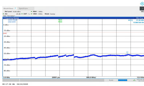
NTNV-n2-PC3-15-25-L-DFT-BPSK-Inner_1RB_Right-3000-12000 -PASS
