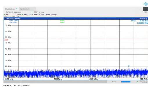
NTNV-n2-PC3-15-25-L-DFT-QPSK-Inner_1RB_Left-0.15-30-PASS
