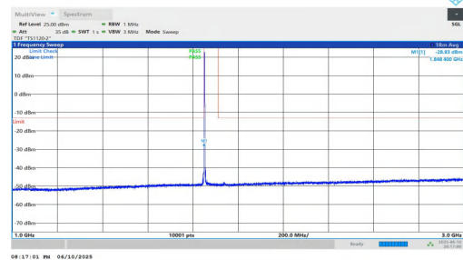
NTNV-n2-PC3-15-25-L-DFT-BPSK-Inner_1RB_Left-1000-3000-PASS
