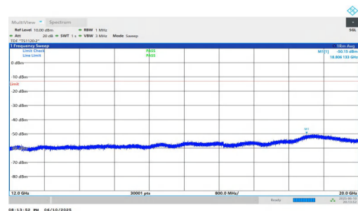
NTNV-n2-PC3-15-20-M-DFT-QPSK-Inner_1RB_Right-12000-2000 0-PASS
