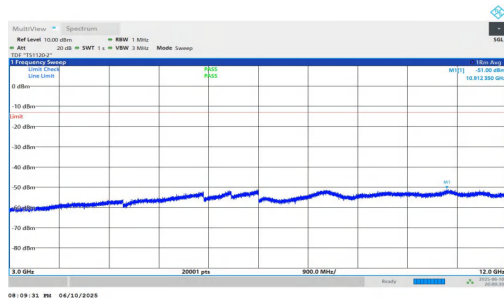
NTNV-n2-PC3-15-20-L-DFT-BPSK-Inner_1RB_Left-3000-12000-PASS
