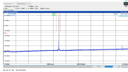
NTNV-n2-PC3-15-20-M-DFT-BPSK-Inner_1RB_Right-1000-3000-P PASS
