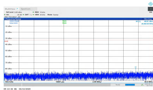
NTNV-n2-PC3-15-20-M-DFT-QPSK-Inner_1RB_Right-0.15-30-PA SS
