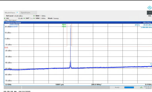
NTNV-n2-PC3-15-15-H-DFT-QPSK-Inner_1RB_Left-1000-3000-P ASS
