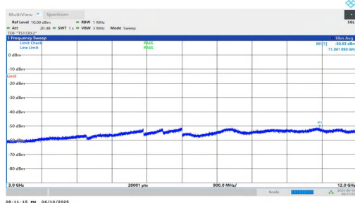
NTNV-n2-PC3-15-20-L-DFT-QPSK-Inner_1RB_Right-3000-12000-PASS
