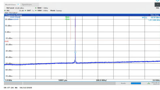
NTNV-n2-PC3-15-15-H-DFT-BPSK-Inner_1RB_Right-1000-3000-P PASS
