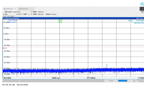
NTNV-n2-PC3-15-15-H-DFT-QPSK-Inner_1RB_Right-30-1000-PASS
