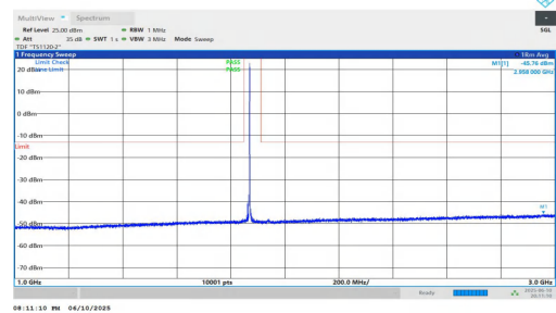
NTNV-n2-PC3-15-20-L-DFT-QPSK-Inner_1RB_Right-1000-3000-PASS
