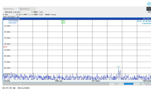
NTNV-n2-PC3-15-20-H-DFT-QPSK-Inner_1RB_Right-0.009-0.15-PASS
