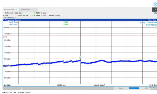
NTNV-n2-PC3-15-20-M-DFT-BPSK-Inner_1RB_Left-3000-12000-PASS
