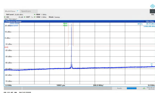
NTNV-n2-PC3-15-20-H-DFT-QPSK-Inner_1RB_Left-1000-3000-P ASS
