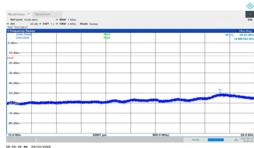
NTNV-n2-PC3-15-20-L-DFT-BPSK-Inner_1RB_Left-12000-20000-PASS
