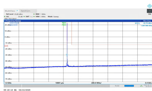
NTNV-n2-PC3-15-25-L-DFT-QPSK-Inner_1RB_Left-1000-3000-PA SS
