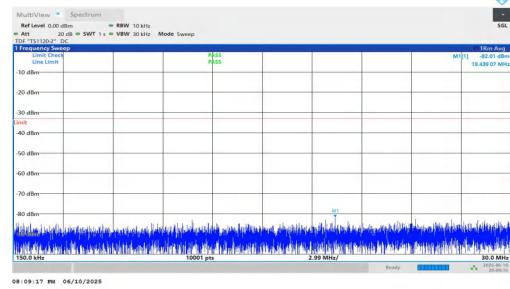
NTNV-n2-PC3-15-20-L-DFT-BPSK-Inner_1RB_Left-0.15-30-PASS
