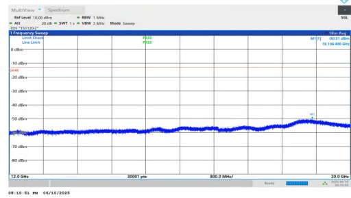
NTNV-n2-PC3-15-20-L-DFT-QPSK-Inner_1RB_Left-12000-20000-PASS
