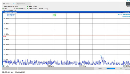
NTNV-n2-PC3-15-20-L-DFT-BPSK-Inner_1RB_Left-0.009-0.15-P ASS
