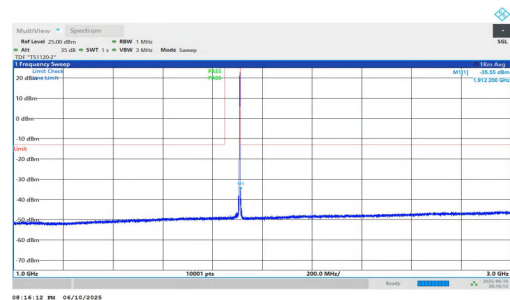
NTNV-n2-PC3-15-20-H-DFT-QPSK-Inner_1RB_Right-1000-3000-PASS
