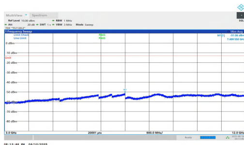
NTNV-n2-PC3-15-20-M-DFT-QPSK-Inner_1RB_Right-3000-1200 0-PASS
