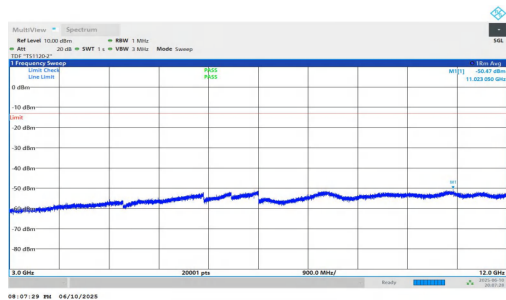
NTNV-n2-PC3-15-15-H-DFT-BPSK-Inner_1RB_Right-3000-1200 0-PASS
