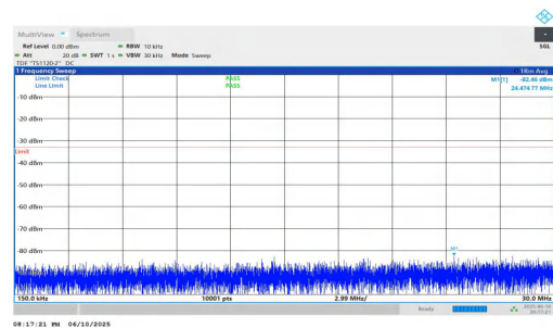
NTNV-n2-PC3-15-25-L-DFT-BPSK-Inner_1RB_Right-0.15-30-PASS
