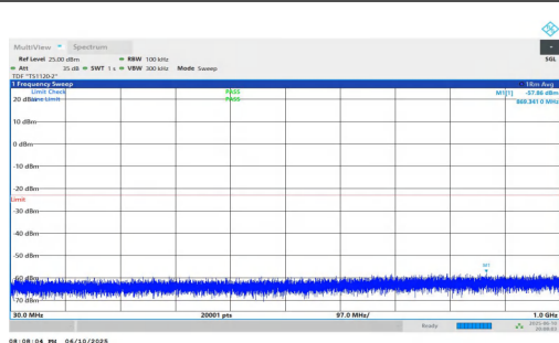
NTNV-n2-PC3-15-15-H-DFT-QPSK-Inner_1RB_Left-30-1000-P ASS
