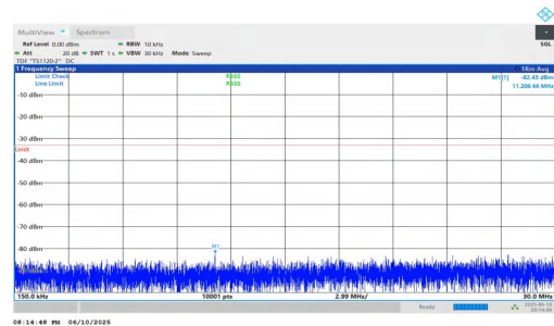
NTNV-n2-PC3-15-20-H-DFT-BPSK-Inner_1RB_Right-0.15-30-PASS
