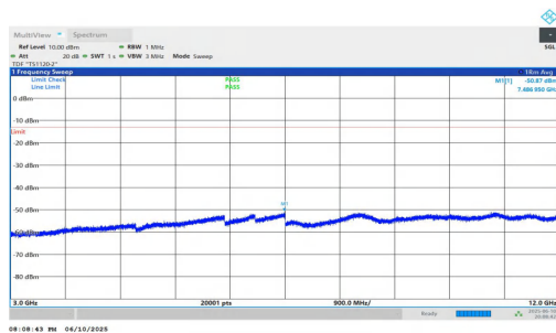
NTNV-n2-PC3-15-15-H-DFT-QPSK-Inner_1RB_Right-3000-12000-PASS
