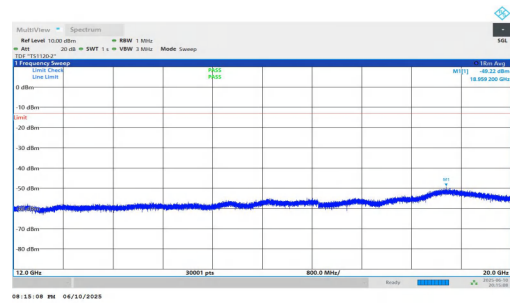
NTNV-n2-PC3-15-20-H-DFT-BPSK-Inner_1RB_Right-12000-2000 0-PASS
