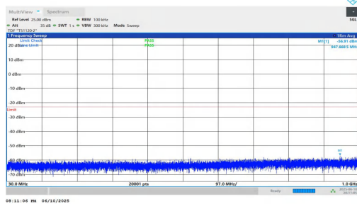
NTNV-n2-PC3-15-20-L-DFT-QPSK-Inner_1RB_Right-30-1000-PASS
