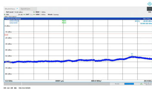
NTNV-n2-PC3-15-20-M-DFT-BPSK-Inner_1RB_Right-12000-2000 0-PASS
