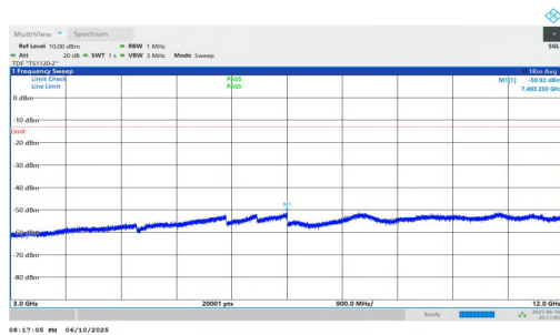
NTNV-n2-PC3-15-25-L-DFT-BPSK-Inner_1RB_Left-3000-12000-PASS
