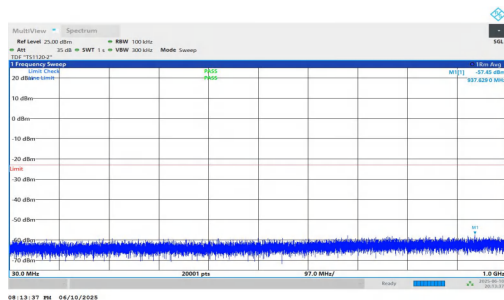
NTNV-n2-PC3-15-20-M-DFT-QPSK-Inner_1RB_Right-30-1000-P ASS
