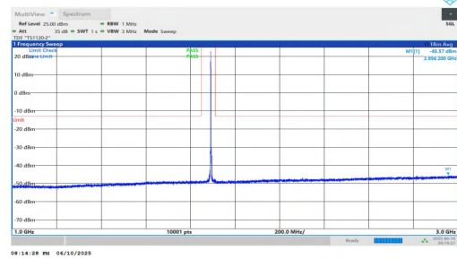
NTNV-n2-PC3-15-20-H-DFT-BPSK-Inner_1RB_Left-1000-3000-PASS
