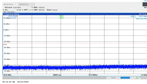
NTNV-n2-PC3-15-20-M-DFT-BPSK-Inner_1RB_Right-30-1000-P ASS
