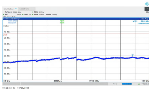
NTNV-n2-PC3-15-20-M-DFT-BPSK-Inner_1RB_Right-3000-1200 0-PASS
