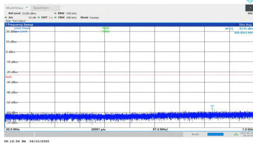
NTNV-n2-PC3-15-25-L-DFT-BPSK-Inner_1RB_Left-30-1000-PASS
