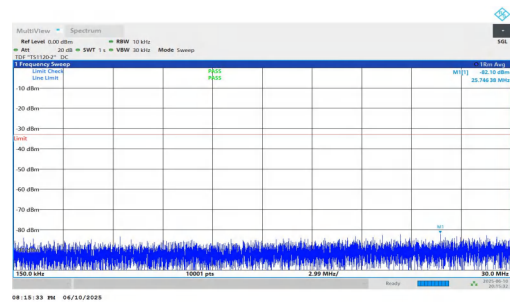
NTNV-n2-PC3-15-20-H-DFT-QPSK-Inner_1RB_Left-0.15-30-PAS S
