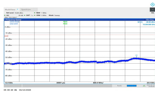
NTNV-n2-PC3-15-15-H-DFT-QPSK-Inner_1RB_Right-12000-20000-PASS
