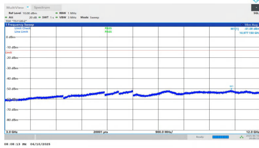
NTNV-n2-PC3-15-15-H-DFT-QPSK-Inner_1RB_Left-3000-12000-PASS
