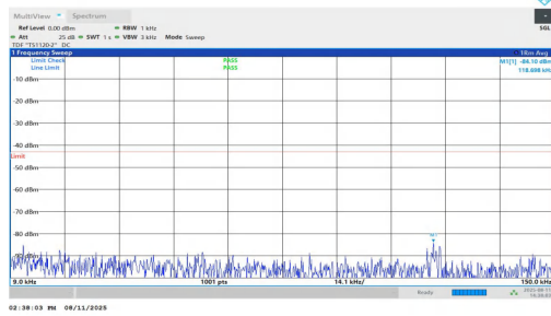
NTNV-n2-PC3-15-25-L-DFT-BPSK-Inner_1RB_Left-0.009-0.15-PASS
