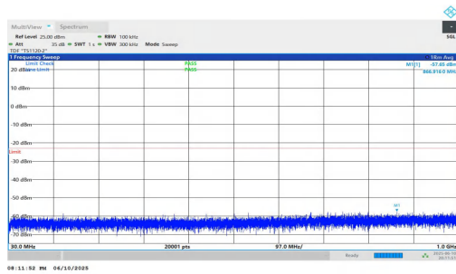
NTNV-n2-PC3-15-20-M-DFT-BPSK-Inner_1RB_Left-30-1000-PASS
