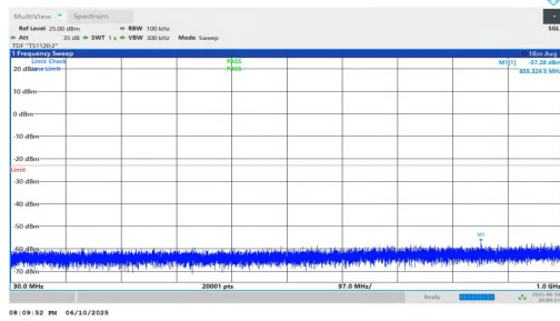
NTNV-n2-PC3-15-20-L-DFT-BPSK-Inner_1RB_Right-30-1000-PA SS
