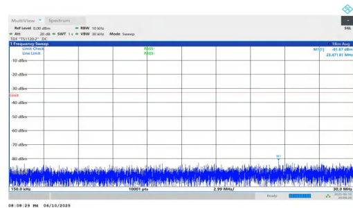
NTNV-n2-PC3-15-15-H-DFT-QPSK-Inner_1RB_Right-0.15-30-PA-SS
