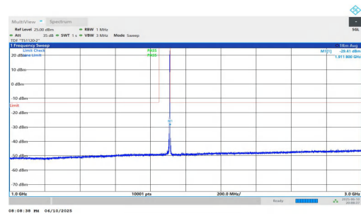
NTNV-n2-PC3-15-15-H-DFT-QPSK-Inner_1RB_Right-1000-3000-PASS
