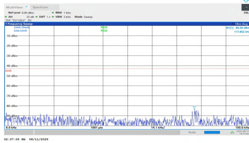
NTNV-n2-PC3-15-20-H-DFT-BPSK-Inner_1RB_Left-0.009-0.15-P ASS
