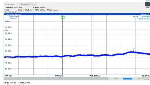
NTNV-n2-PC3-15-20-M-DFT-QPSK-Inner_1RB_Left-12000-20000 -PASS
