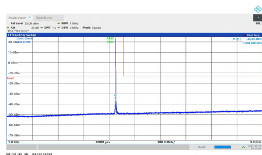
NTNV-n2-PC3-15-20-L-DFT-QPSK-Inner_1RB_Left-1000-3000-PA SS
