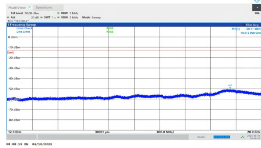
NTNV-n2-PC3-15-15-H-DFT-QPSK-Inner_1RB_Left-12000-20000-PASS
