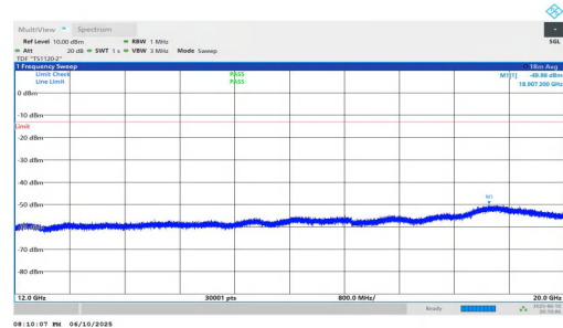
NTNV-n2-PC3-15-20-L-DFT-BPSK-Inner_1RB_Right-12000-2000 0-PASS
