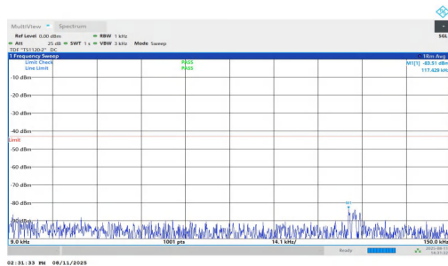
NTNV-n2-PC3-15-10-H-DFT-BPSK-Inner_1RB_Right-0.009-0.15-PASS
