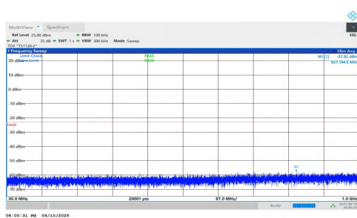
NTNV-n2-PC3-15-10-H-DFT-QPSK-Inner_1RB_Left-30-1000-PA SS
