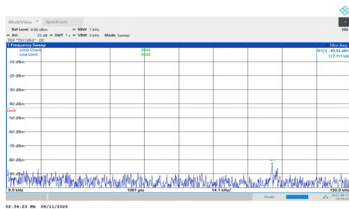
NTNV-n2-PC3-15-15-H-DFT-BPSK-Inner_1RB_Right-0.009-0.15-PASS
