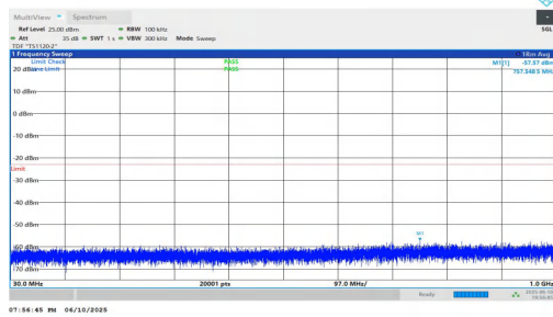
NTNV-n2-PC3-15-10-M-DFT-BPSK-Inner_1RB_Left-30-1000-PASS SS
