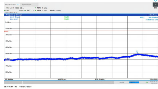
NTNV-n2-PC3-15-10-H-DFT-QPSK-Inner_1RB_Left-12000-20000-PASS
