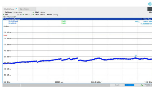
NTNV-n2-PC3-15-10-H-DFT-QPSK-Inner_1RB_Right-3000-12000-PASS
