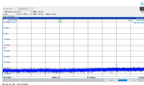
NTNV-n2-PC3-15-15-L-DFT-QPSK-Inner_1RB_Right-30-1000-PASS
