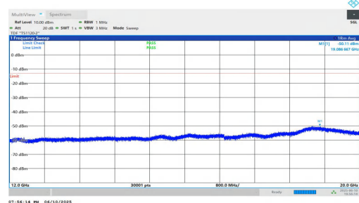
NTNV-n2-PC3-15-10-L-DFT-QPSK-Inner_1RB_Right-12000-20000-PASS
