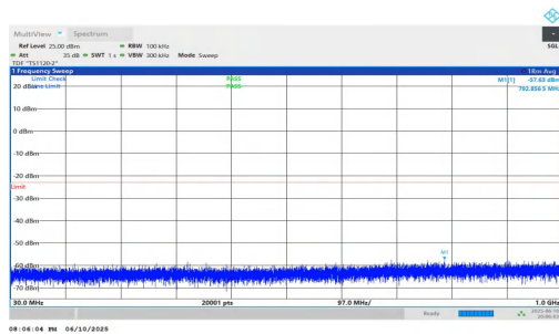
NTNV-n2-PC3-15-15-M-DFT-QPSK-Inner_1RB_Right-30-1000-P ASS
