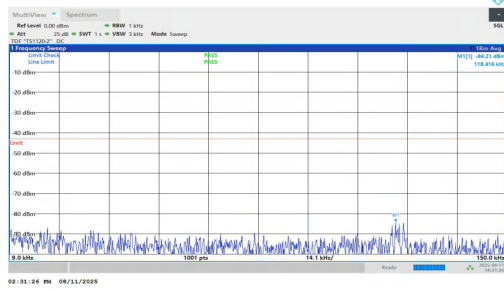
NTNV-n2-PC3-15-10-H-DFT-BPSK-Inner_1RB_Left-0.009-0.15-P ASS
