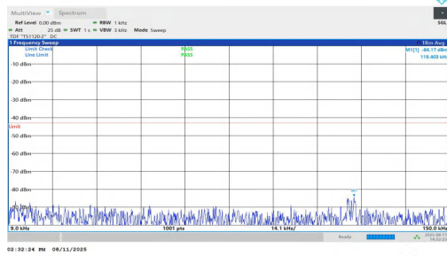
NTNV-n2-PC3-15-15-L-DFT-BPSK-Inner_1RB_Left-0.009-0.15-P ASS
