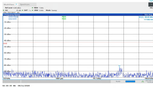
NTNV-n2-PC3-15-10-M-DFT-BPSK-Inner_1RB_Left-0.009-0.15-P ASS
