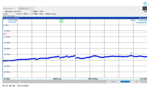
NTNV-n2-PC3-15-15-L-DFT-BPSK-Inner_1RB_Left-3000-12000- PASS
