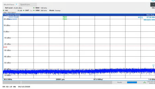
NTVN-n2-PC3-15-15-L-DFT-BPSK-Inner_1RB_Right-30-1000-PA SS
