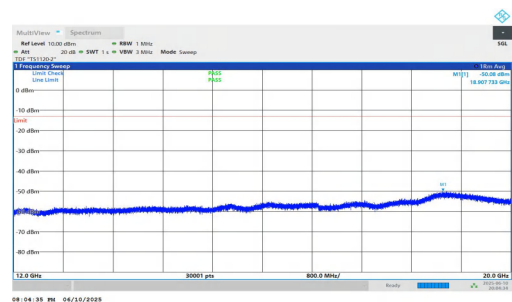
NTNV-n2-PC3-15-15-M-DFT-BPSK-Inner_1RB_Left-12000-20000-PASS
