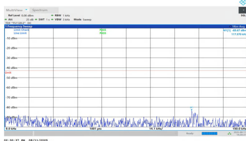
NTNV-n2-PC3-15-10-M-DFT-BPSK-Inner_1RB_Right-0.009-0.15 -PASS
