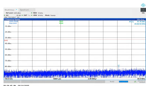
NTNV-n2-PC3-15-15-M-DFT-BPSK-Inner_1RB_Right-0.15-30-PASS
