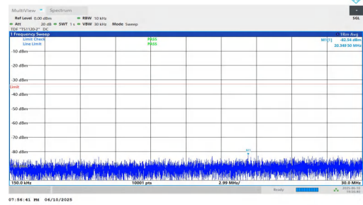
NTNV-n2-PC3-15-10-M-DFT-BPSK-Inner_1RB_Left-0.15-30-PAS S
