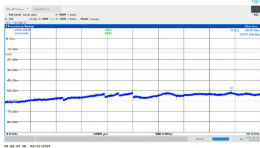
NTNV-n2-PC3-15-15-M-DFT-BPSK-Inner_1RB_Right-3000-1200 0-PASS
