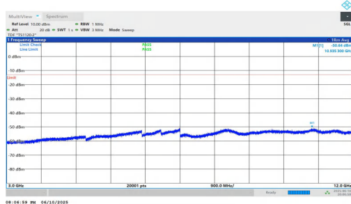
NTNV-n2-PC3-15-15-H-DFT-BPSK-Inner_1RB_Left-3000-12000-PASS
