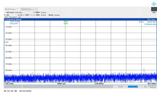
NTNV-n2-PC3-15-15-L-DFT-QPSK-Inner_1RB_Right-0.15-30-PASS
