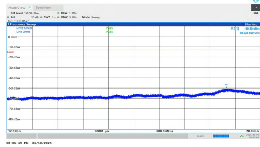
NTNV-n2-PC3-15-15-M-DFT-QPSK-Inner_1RB_Left-12000-20000 -PASS
