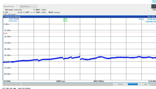
NTNV-n2-PC3-15-10-L-DFT-QPSK-Inner_1RB_Right-3000-12000-PASS
