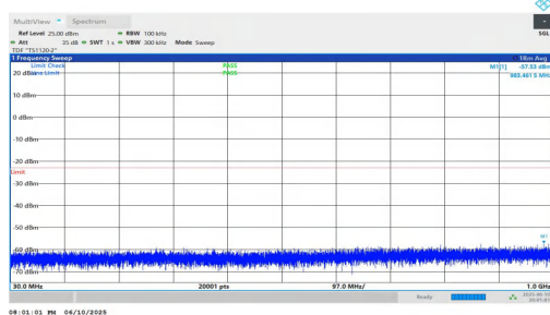
NTNV-n2-PC3-15-10-H-DFT-QPSK-Inner_1RB_Right-30-1000-PASS
