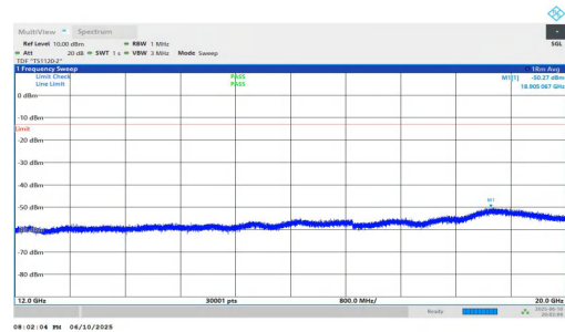
NTNV-n2-PC3-15-15-L-DFT-BPSK-Inner_1RB_Left-12000-20000- PASS
