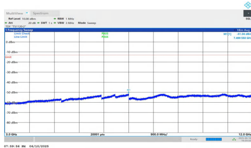
NTNV-n2-PC3-15-10-H-DFT-BPSK-Inner_1RB_Right-3000-12000 0-PASS
