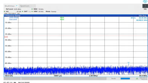
NTNV-n2-PC3-15-10-M-DFT-BPSK-Inner_1RB_Right-0.15-30-PASS SS
