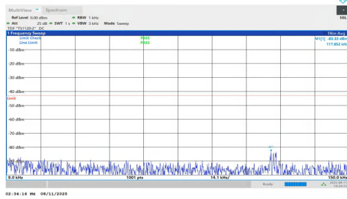
NTNV-n2-PC3-15-15-H-DFT-BPSK-Inner_1RB_Left-0.009-0.15-P ASS
