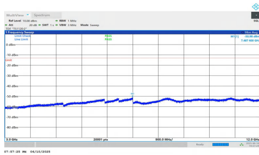
NTNV-n2-PC3-15-10-M-DFT-BPSK-Inner_1RB_Right-3000-1200 0-PASS
