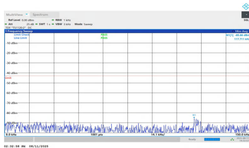
NTNV-n2-PC3-15-15-L-DFT-QPSK-Inner_1RB_Right-0.009-0.15-PASS
