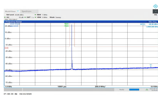
NTNV-n2-PC3-15-10-M-DFT-QPSK-Inner_1RB_Left-1000-3000-P ASS
