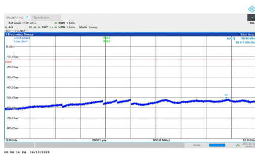
NTNV-n2-PC3-15-15-M-DFT-QPSK-Inner_1RB_Right-3000-1200 0-PASS
