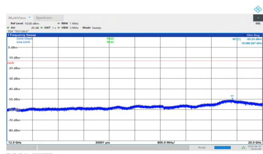
NTNV-n2-PC3-15-15-L-DFT-QPSK-Inner_1RB_Right-12000-20000-PASS
