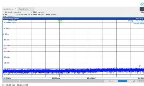
NTVN-n2-PC3-15-15-L-DFT-QPSK-Inner_1RB_Left-30-1000-PA SS
