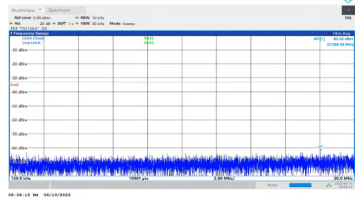
NTNV-n2-PC3-15-15-M-DFT-BPSK-Inner_1RB_Left-0.15-30-PAS S
