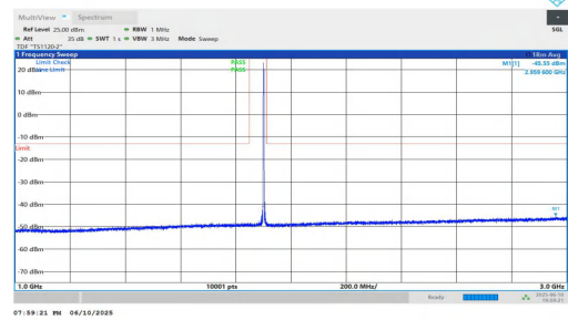
NTNV-n2-PC3-15-10-H-DFT-BPSK-Inner_1RB_Left-1000-3000-PASS
