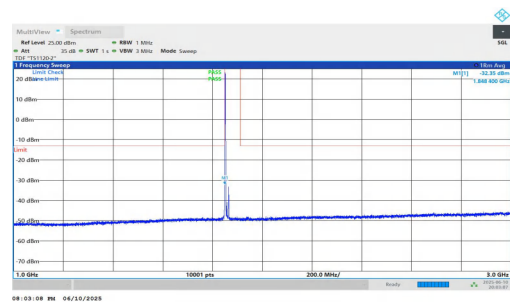
NTVN-n2-PC3-15-15-L-DFT-QPSK-Inner_1RB_Left-1000-3000-PA SS
