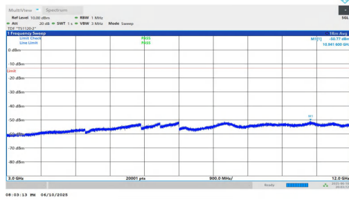
NTNV-n2-PC3-15-15-L-DFT-QPSK-Inner_1RB_Left-3000-12000-PASS
