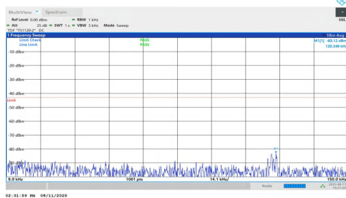
NTNV-n2-PC3-15-10-H-DFT-QPSK-Inner_1RB_Right-0.009-0.15-PASS
