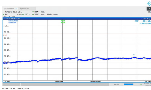
NTNV-n2-PC3-15-10-H-DFT-BPSK-Inner_1RB_Left-3000-12000-PASS
