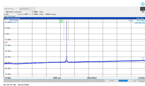
NTNV-n2-PC3-15-15-M-DFT-QPSK-Inner_1RB_Right-1000-3000- PASS
