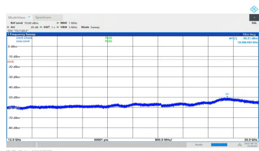
NTNV-n2-PC3-15-10-M-DFT-QPSK-Inner_1RB_Right-12000-2000 0-PASS
