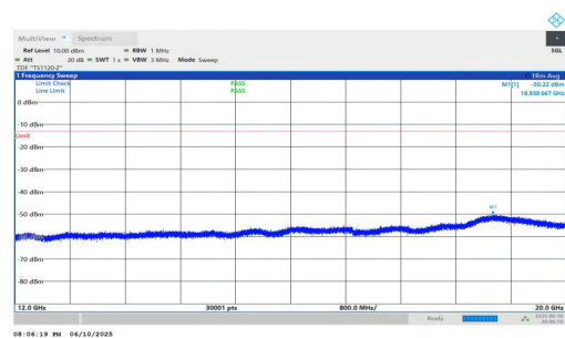
NTNV-n2-PC3-15-15-M-DFT-QPSK-Inner_1RB_Right-12000-2000 0-PASS
