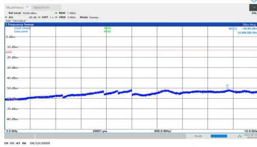
NTNV-n2-PC3-15-15-M-DFT-QPSK-Inner_1RB_Left-3000-12000 -PASS
