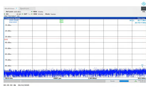
NTNV-n2-PC3-15-15-M-DFT-QPSK-Inner_1RB_Right-0.15-30-PA SS
