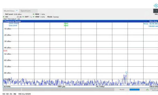
NTNV-n2-PC3-15-15-L-DFT-BPSK-Inner_1RB_Right-0.009-0.15- PASS
