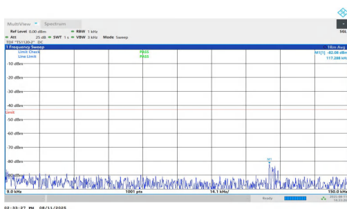
NTNV-n2-PC3-15-15-M-DFT-BPSK-Inner_1RB_Right-0.009-0.15 -PASS
