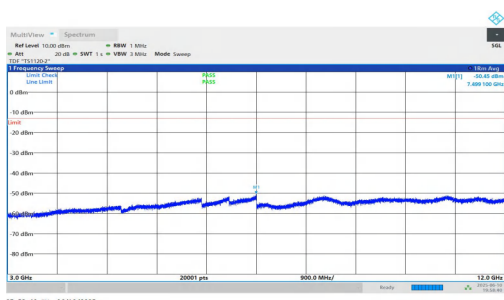
NTNV-n2-PC3-15-10-M-DFT-QPSK-Inner_1RB_Right-3000-1200 0-PASS
