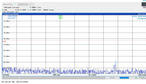
NTNV-n2-PC3-15-15-M-DFT-BPSK-Inner_1RB_Left-0.009-0.15-P ASS
