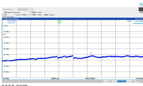
NTNV-n2-PC3-15-15-M-DFT-BPSK-Inner_1RB_Left-3000-12000-PASS
