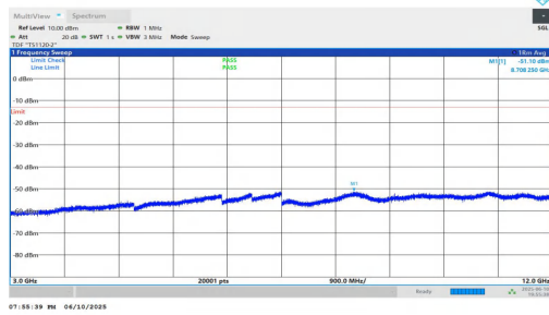
NTNV-n2-PC3-15-10-L-DFT-QPSK-Inner_1RB_Left-3000-12000-PASS
