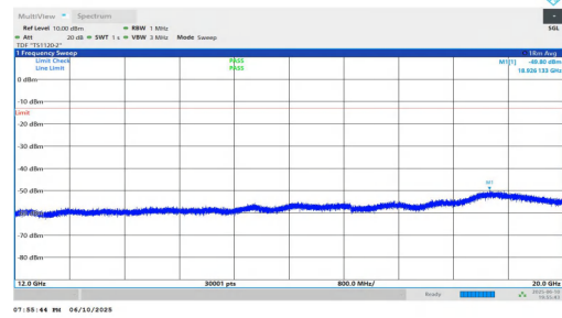
NTNV-n2-PC3-15-10-L-DFT-QPSK-Inner_1RB_Left-12000-20000-PASS
