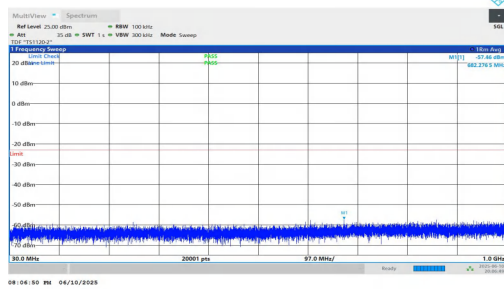
NTNV-n2-PC3-15-15-H-DFT-BPSK-Inner_1RB_Left-30-1000-PASS
