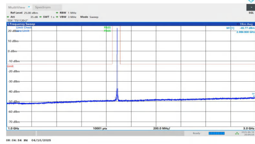
NTNV-n2-PC3-15-15-M-DFT-BPSK-Inner_1RB_Right-1000-3000-P PASS
