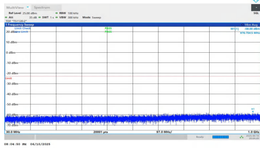
NTNV-n2-PC3-15-15-M-DFT-BPSK-Inner_1RB_Right-30-1000-P ASS
