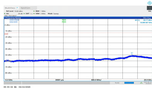
NTNV-n2-PC3-15-10-H-DFT-BPSK-Inner_1RB_Right-12000-20000 0-PASS
