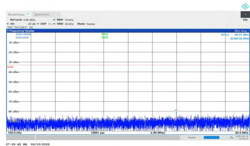
NTNV-n2-PC3-15-10-H-DFT-BPSK-Inner_1RB_Right-0.15-30-PASS
