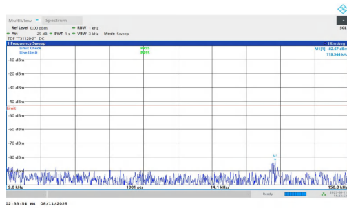
NTNV-n2-PC3-15-15-M-DFT-QPSK-Inner_1RB_Right-0.009-0.15 -PASS
