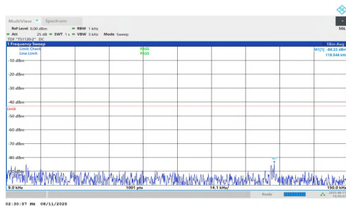
NTNV-n2-PC3-15-10-M-DFT-QPSK-Inner_1RB_Left-0.009-0.15- PASS
