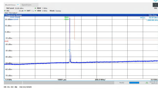
NTNV-n2-PC3-15-15-L-DFT-BPSK-Inner_1RB_Left-1000-3000-PASS SS
