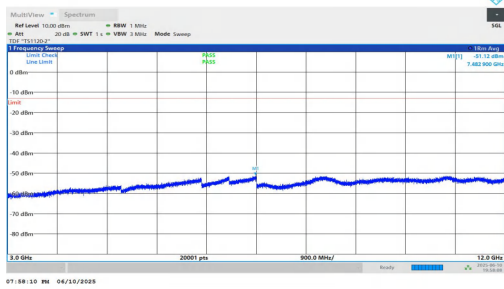
NTNV-n2-PC3-15-10-M-DFT-QPSK-Inner_1RB_Left-3000-12000 -PASS
