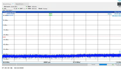
NTNV-n2-PC3-15-10-L-DFT-QPSK-Inner_1RB_Right-30-1000-PASS
