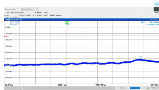
NTNV-n2-PC3-15-10-H-DFT-QPSK-Inner_1RB_Right-12000-20000-PASS
