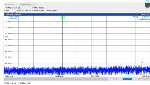
NTNV-n2-PC3-15-10-L-DFT-QPSK-Inner_1RB_Right-0.15-30-PASS
