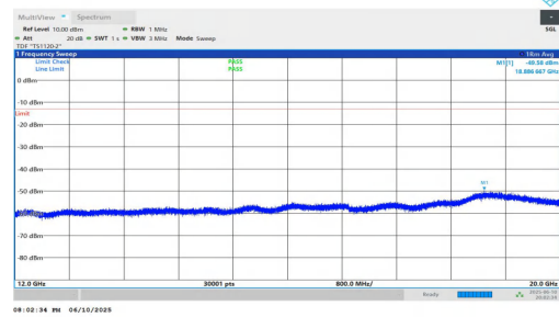
NTVN-n2-PC3-15-15-L-DFT-BPSK-Inner_1RB_Right-12000-2000 0-PASS
