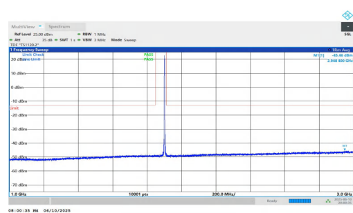
NTNV-n2-PC3-15-10-H-DFT-QPSK-Inner_1RB_Left-1000-3000-P ASS
