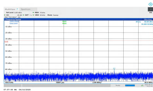
NTNV-n2-PC3-15-10-M-DFT-QPSK-Inner_1RB_Left-0.15-30-PAS S
