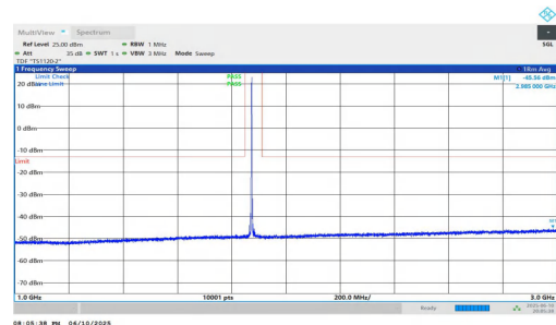
NTNV-n2-PC3-15-15-M-DFT-QPSK-Inner_1RB_Left-1000-3000-P ASS
