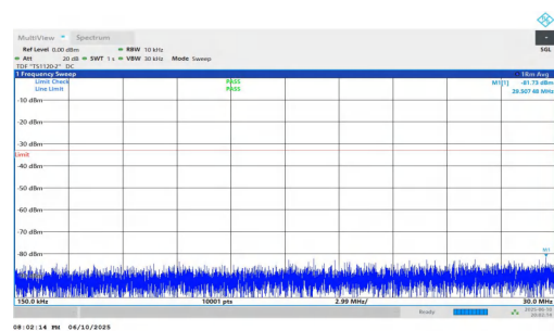
NTNV-n2-PC3-15-15-L-DFT-BPSK-Inner_1RB_Right-0.15-30-PASS S
