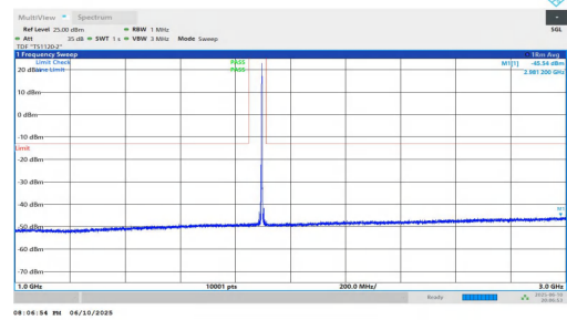
NTNV-n2-PC3-15-15-H-DFT-BPSK-Inner_1RB_Left-1000-3000-PASS
