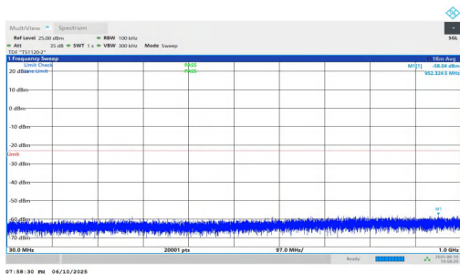
NTNV-n2-PC3-15-10-M-DFT-QPSK-Inner_1RB_Right-30-1000-P ASS
