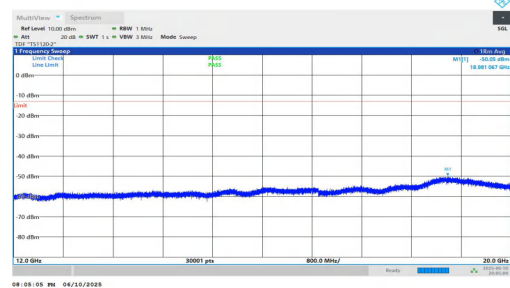
NTNV-n2-PC3-15-15-M-DFT-BPSK-Inner_1RB_Right-12000-2000 0-PASS
