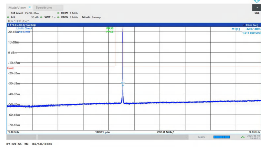
NTNV-n2-PC3-15-10-H-DFT-BPSK-Inner_1RB_Right-1000-3000-P PASS
