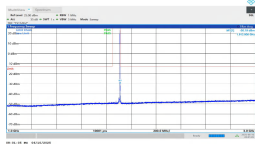
NTNV-n2-PC3-15-10-H-DFT-QPSK-Inner_1RB_Right-1000-3000-PASS
