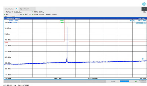
NTNV-n2-PC3-15-10-M-DFT-QPSK-Inner_1RB_Right-1000-3000- PASS
