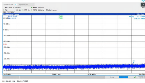
NTNV-n2-PC3-15-15-L-DFT-BPSK-Inner_1RB_Left-30-1000-PAS S
