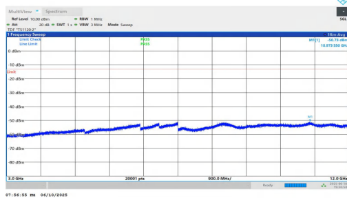
NTNV-n2-PC3-15-10-M-DFT-BPSK-Inner_1RB_Left-3000-12000-PASS PASS
