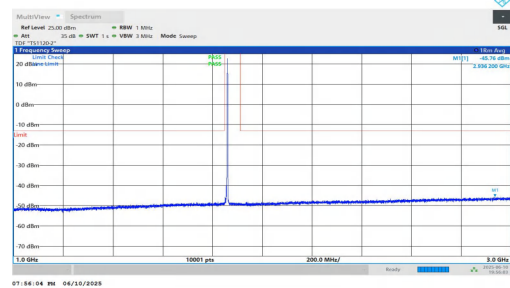
NTNV-n2-PC3-15-10-L-DFT-QPSK-Inner_1RB_Right-1000-3000-PASS
