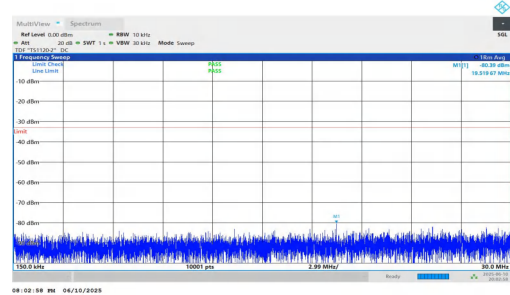
NTVN-n2-PC3-15-15-L-DFT-QPSK-Inner_1RB_Left-0.15-30-PASS
