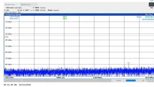
NTNV-n2-PC3-15-15-L-DFT-BPSK-Inner_1RB_Left-0.15-30-PASS
