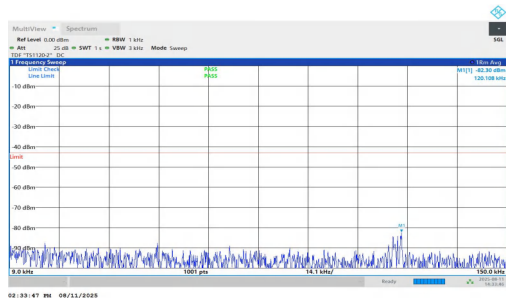
NTNV-n2-PC3-15-15-M-DFT-QPSK-Inner_1RB_Left-0.009-0.15- PASS
