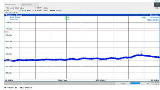
NTNV-n2-PC3-15-15-L-DFT-QPSK-Inner_1RB_Left-12000-20000-PASS
