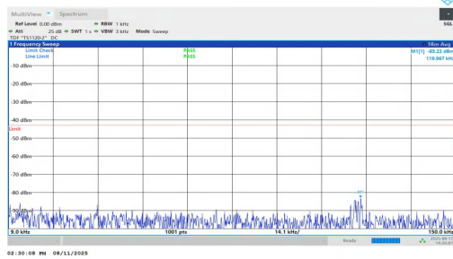
NTNV-n2-PC3-15-10-L-DFT-QPSK-Inner_1RB_Right-0.009-0.15-PASS
