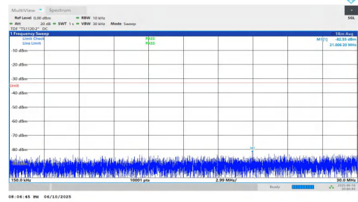
NTNV-n2-PC3-15-15-H-DFT-BPSK-Inner_1RB_Left-0.15-30-PASS
