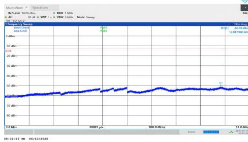
NTVN-n2-PC3-15-15-L-DFT-BPSK-Inner_1RB_Right-3000-12000 -PASS
