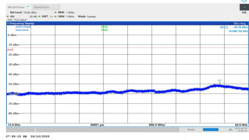
NTNV-n2-PC3-15-10-M-DFT-QPSK-Inner_1RB_Left-12000-20000 -PASS
