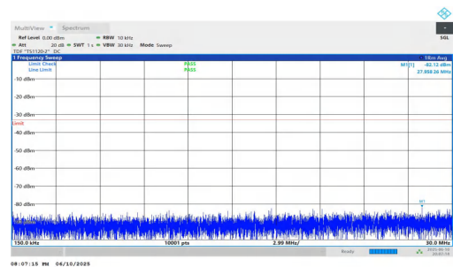
NTNV-n2-PC3-15-15-H-DFT-BPSK-Inner_1RB_Right-0.15-30-PASS
