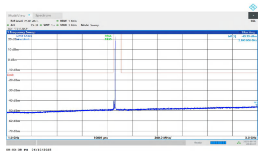
NTNV-n2-PC3-15-15-L-DFT-QPSK-Inner_1RB_Right-1000-3000-PASS
