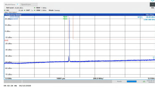
NTVN-n2-PC3-15-15-L-DFT-BPSK-Inner_1RB_Right-1000-3000-P ASS
