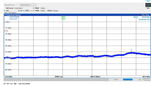
NTNV-n2-PC3-15-10-M-DFT-BPSK-Inner_1RB_Left-12000-20000-PASS PASS
