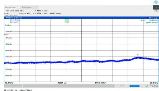
NTNV-n2-PC3-15-15-H-DFT-BPSK-Inner_1RB_Left-12000-20000-PASS
