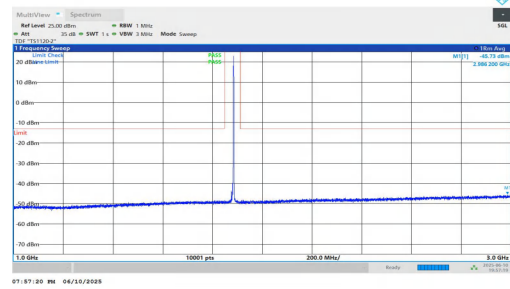
NTNV-n2-PC3-15-10-M-DFT-BPSK-Inner_1RB_Right-1000-3000-P PASS
