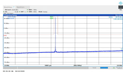
NTNV-n2-PC3-15-15-M-DFT-BPSK-Inner_1RB_Left-1000-3000-P ASS
