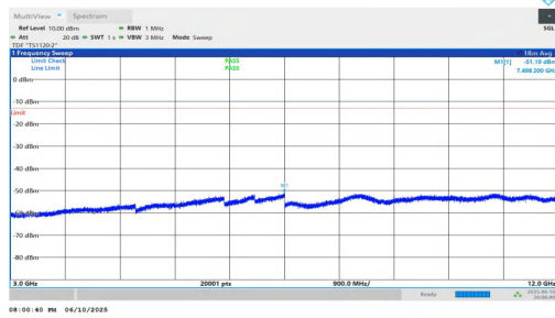
NTNV-n2-PC3-15-10-H-DFT-QPSK-Inner_1RB_Left-3000-12000-PASS
