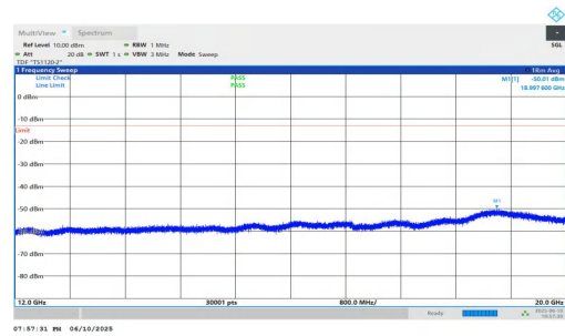
NTNV-n2-PC3-15-10-M-DFT-BPSK-Inner_1RB_Right-12000-2000 0-PASS
