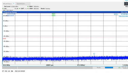
NTNV-n2-PC3-15-5-H-DFT-BPSK-Inner_1RB_Right-30-1000-PA SS
