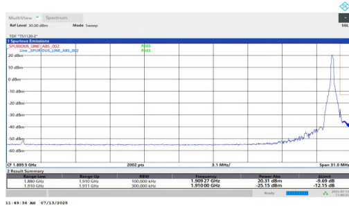
NTNV-n2-PC3-15-30-H-DFT-BPSK-Edge_1RB_Right-PASS
