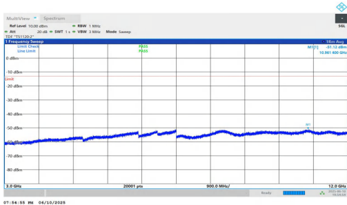
NTVN-n2-PC3-15-10-L-DFT-BPSK-Inner_1RB_Right-3000-12000 -PASS
