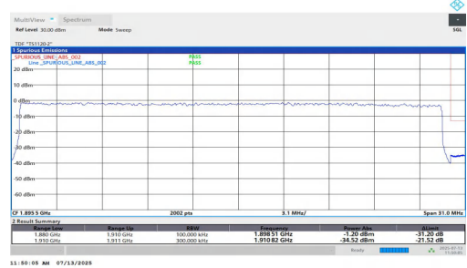
NTNV-n2-PC3-15-30-H-DFT-QPSK-Outer_Full-PASS
