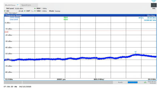
NTNV-n2-PC3-15-10-L-DFT-BPSK-Inner_1RB_Left-12000-20000-PASS
