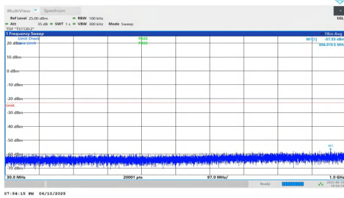
NTNV-n2-PC3-15-10-L-DFT-BPSK-Inner_1RB_Left-30-1000-PASS
