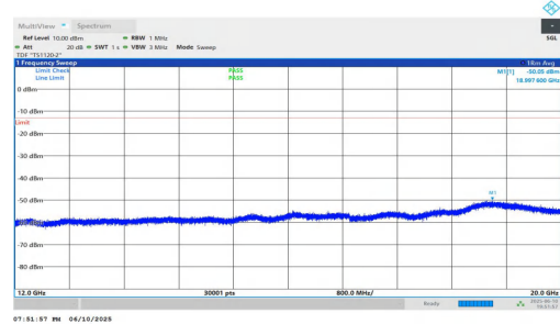
NTVN-n2-PC3-15-5-H-DFT-BPSK-Inner_1RB_Left-12000-20000-P ASS
