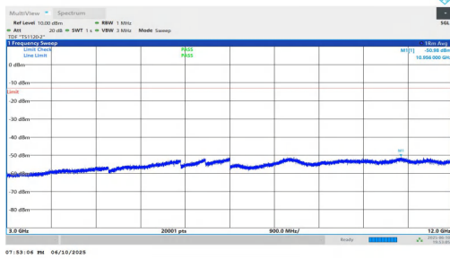
NTNV-n2-PC3-15-5-H-DFT-QPSK-Inner_1RB_Left-3000-12000-P ASS
