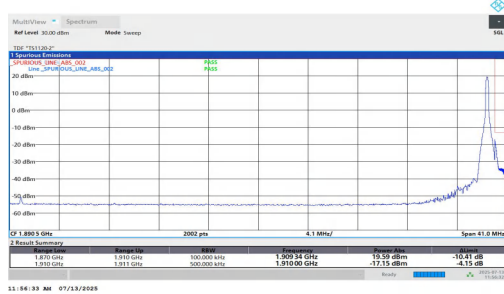
NTNV-n2-PC3-15-40-H-DFT-QPSK-Edge_1RB_Right-PASS
