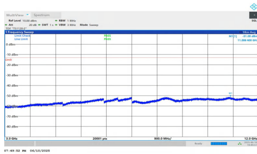
NTNV-n2-PC3-15-5-M-DFT-BPSK-Inner_1RB_Right-3000-12000 -PASS
