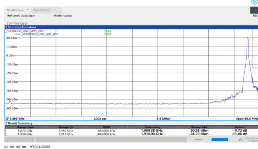
NTV-n2-PC3-15-35-H-DFT-BPSK-Edge_1RB_Right-PASS
