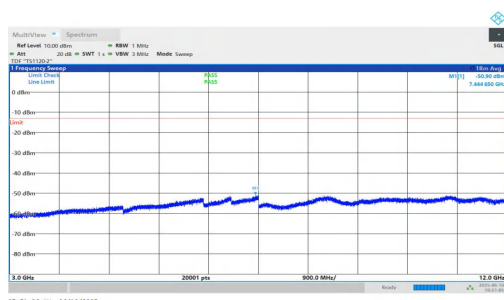
NTNV-n2-PC3-15-5-M-DFT-QPSK-Inner_1RB_Right-3000-12000-PASS
