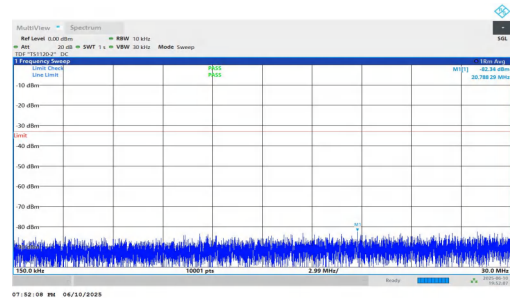
NTVN-n2-PC3-15-5-H-DFT-BPSK-Inner_1RB_Right-0.15-30-PAS S
