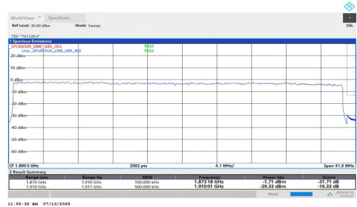
NTNV-n2-PC3-15-40-H-DFT-BPSK-Outer_Full-PASS
