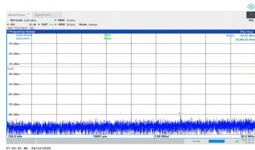
NTNV-n2-PC3-15-5-M-DFT-QPSK-Inner_1RB_Right-0.15-30-PASS
