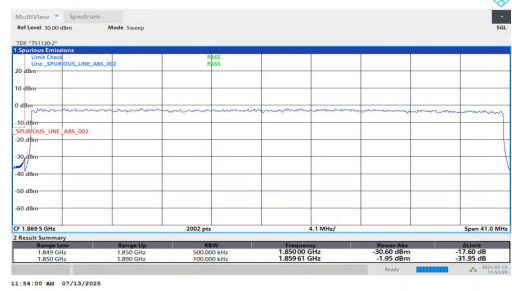
NTNV-n2-PC3-15-40-L-DFT-BPSK-Outer_Full-PASS
