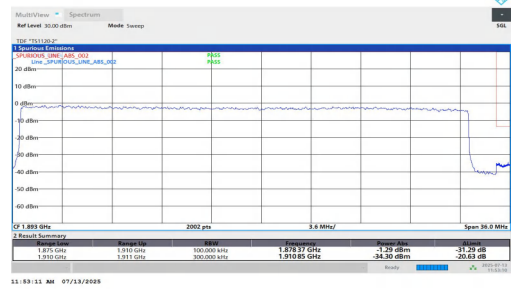
NTV-n2-PC3-15-35-H-DFT-QPSK-Outer_Full-PASS
