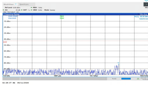
NTVN-n2-PC3-15-5-H-DFT-BPSK-Inner_1RB_Left-0.009-0.15-PA SS
