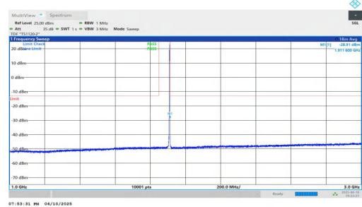
NTNV-n2-PC3-15-5-H-DFT-QPSK-Inner_1RB_Right-1000-3000-P ASS
