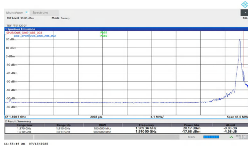
NTNV-n2-PC3-15-40-H-DFT-BPSK-Edge_1RB_Right-PASS
