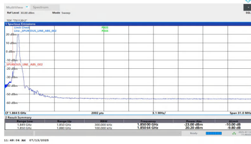
NTNV-n2-PC3-15-30-L-DFT-BPSK-Edge_1RB_Left-PASS
