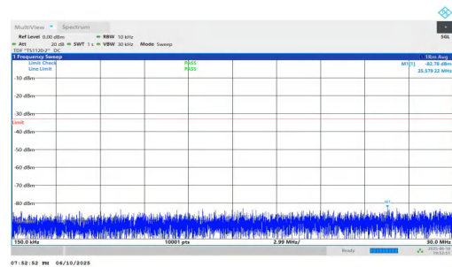
NTNV-n2-PC3-15-5-H-DFT-QPSK-Inner_1RB_Left-0.15-30-PASS
