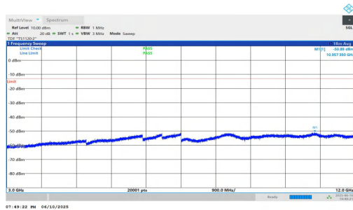
NTNV-n2-PC3-15-5-M-DFT-BPSK-Inner_1RB_Left-3000-12000-P ASS
