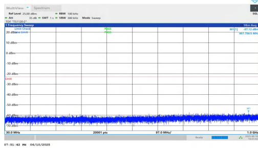
NTVN-n2-PC3-15-5-H-DFT-BPSK-Inner_1RB_Left-30-1000-PAS S
