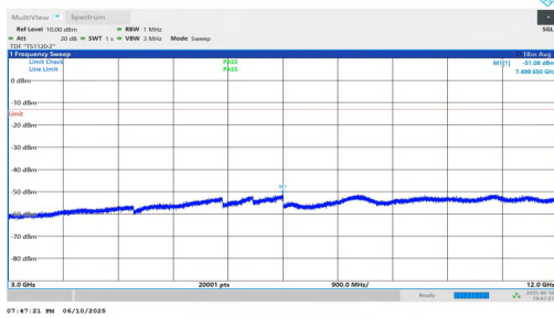
NTNV-n2-PC3-15-5-L-DFT-BPSK-Inner_1RB_Right-3000-12000- PASS
