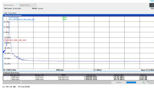
NTNV-n2-PC3-15-40-L-DFT-BPSK-Edge_1RB_Left-PASS
