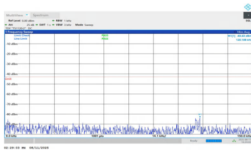
NTNV-n2-PC3-15-5-H-DFT-QPSK-Inner_1RB_Left-0.009-0.15-P ASS
