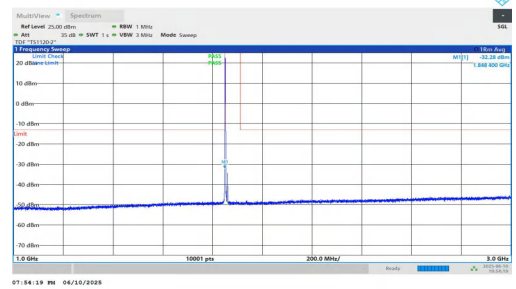
NTNV-n2-PC3-15-10-L-DFT-BPSK-Inner_1RB_Left-1000-3000-PASS
