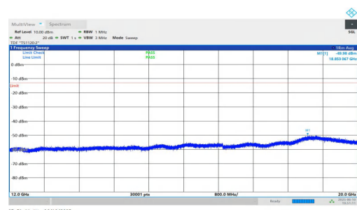
NTNV-n2-PC3-15-5-M-DFT-QPSK-Inner_1RB_Right-12000-20000-PASS
