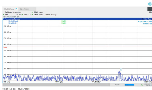
NTNV-n2-PC3-15-5-M-DFT-QPSK-Inner_1RB_Right-0.009-0.15-PASS
