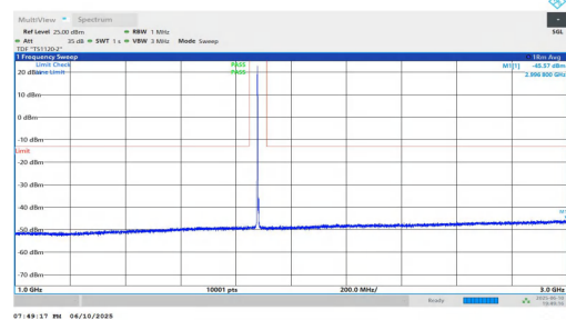
NTNV-n2-PC3-15-5-M-DFT-BPSK-Inner_1RB_Left-1000-3000-PASS SS
