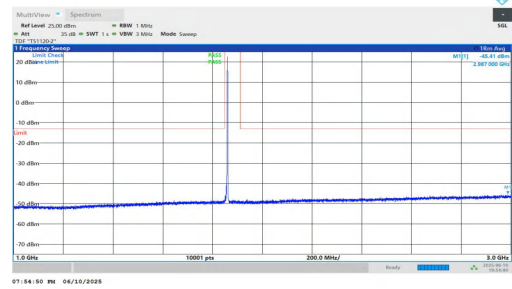
NTVN-n2-PC3-15-10-L-DFT-BPSK-Inner_1RB_Right-1000-3000-P ASS
