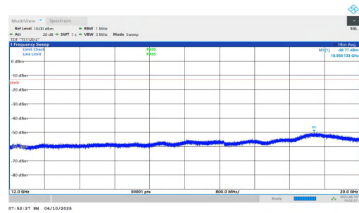
NTNV-n2-PC3-15-5-H-DFT-BPSK-Inner_1RB_Right-12000-20000- PASS
