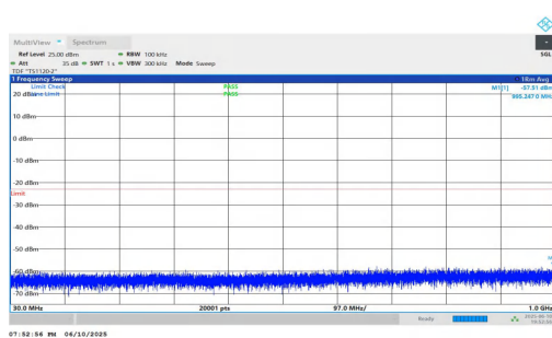
NTNV-n2-PC3-15-5-H-DFT-QPSK-Inner_1RB_Left-30-1000-PAS S
