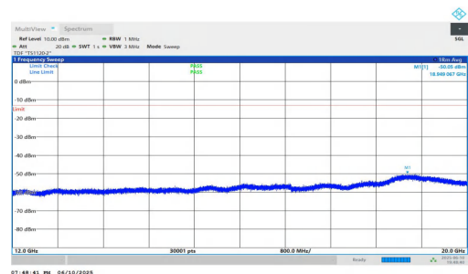
NTNV-n2-PC3-15-5-L-DFT-QPSK-Inner_1RB_Right-12000-20000- PASS
