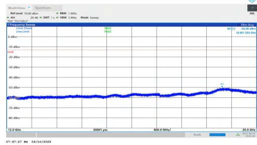
NTNV-n2-PC3-15-5-L-DFT-BPSK-Inner_1RB_Right-12000-20000- PASS
