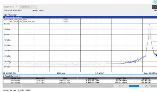
NTNV-n2-PC3-15-30-H-DFT-QPSK-Edge_1RB_Right-PASS
