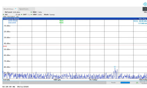
NTNV-n2-PC3-15-5-M-DFT-QPSK-Inner_1RB_Left-0.009-0.15-P ASS
