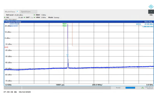
NTVN-n2-PC3-15-10-L-DFT-QPSK-Inner_1RB_Left-1000-3000-PA SS
