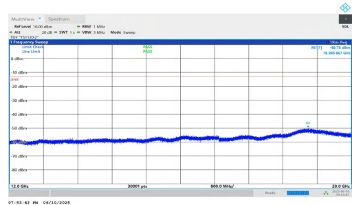
NTNV-n2-PC3-15-5-H-DFT-QPSK-Inner_1RB_Right-12000-20000 -PASS
