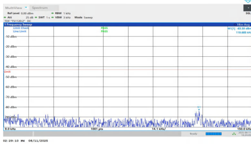
NTNV-n2-PC3-15-5-H-DFT-QPSK-Inner_1RB_Right-0.009-0.15- PASS
