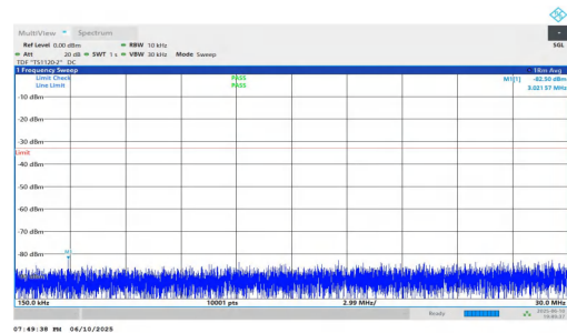
NTNV-n2-PC3-15-5-M-DFT-BPSK-Inner_1RB_Right-0.15-30-PASS S
