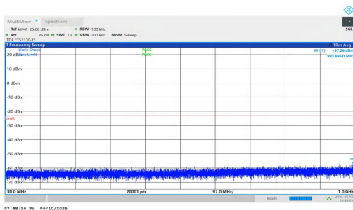
NTNV-n2-PC3-15-5-L-DFT-QPSK-Inner_1RB_Right-30-1000-PA SS
