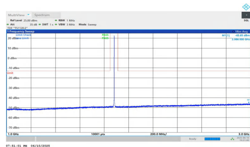
NTNV-n2-PC3-15-5-M-DFT-QPSK-Inner_1RB_Right-1000-3000-PASS
