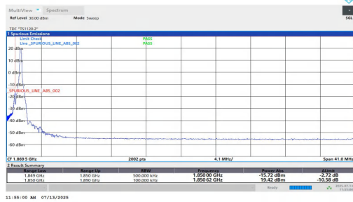
NTNV-n2-PC3-15-40-L-DFT-QPSK-Edge_1RB_Left-PASS
