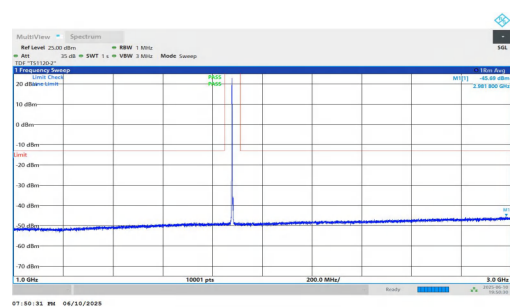
NTNV-n2-PC3-15-5-M-DFT-QPSK-Inner_1RB_Left-1000-3000-PA SS
