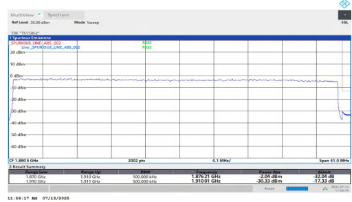
NTNV-n2-PC3-15-40-H-DFT-QPSK-Outer_Full-PASS
