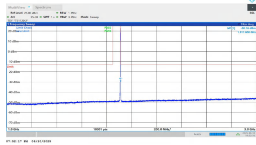
NTNV-n2-PC3-15-5-H-DFT-BPSK-Inner_1RB_Right-1000-3000-P ASS
