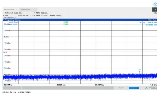
NTNV-n2-PC3-15-5-M-DFT-QPSK-Inner_1RB_Right-30-1000-PASS
