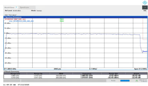
NTNV-n2-PC3-15-30-H-DFT-BPSK-Outer_Full-PASS
