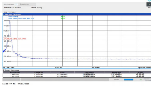
NTV-n2-PC3-15-35-L-DFT-BPSK-Edge_1RB_Left-PASS
