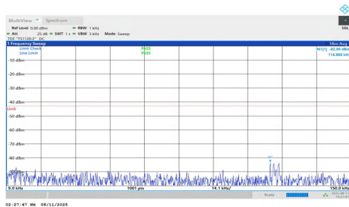
NTNV-n2-PC3-15-5-M-DFT-BPSK-Inner_1RB_Right-0.009-0.15-PASS
