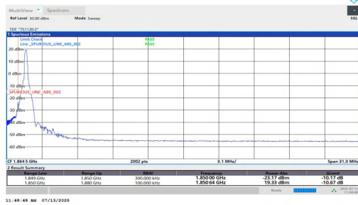
NTNV-n2-PC3-15-30-L-DFT-QPSK-Edge_1RB_Left-PASS
