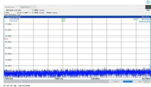
NTNV-n2-PC3-15-5-L-DFT-QPSK-Inner_1RB_Left-0.15-30-PASS
