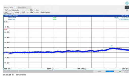
NTNV-n2-PC3-15-5-M-DFT-BPSK-Inner_1RB_Left-12000-20000-PASS
