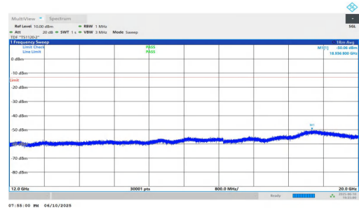
NTVN-n2-PC3-15-10-L-DFT-BPSK-Inner_1RB_Right-12000-2000 0-PASS
