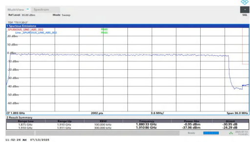
NTV-n2-PC3-15-35-H-DFT-BPSK-Outer_Full-PASS
