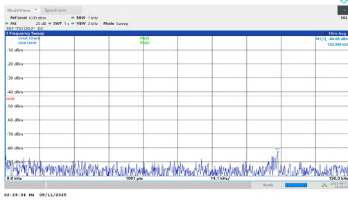
NTNV-n2-PC3-15-10-L-DFT-BPSK-Inner_1RB_Left-0.009-0.15-PASS
