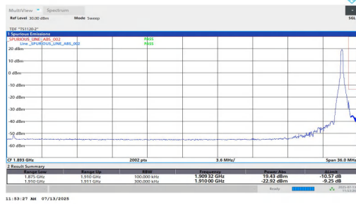
NTV-n2-PC3-15-35-H-DFT-QPSK-Edge_1RB_Right-PASS
