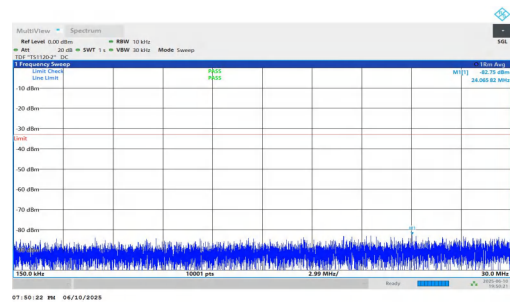
NTNV-n2-PC3-15-5-M-DFT-QPSK-Inner_1RB_Left-0.15-30-PASS
