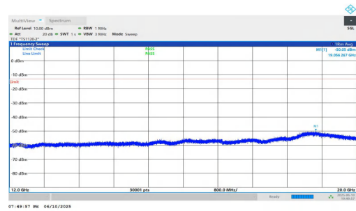
NTNV-n2-PC3-15-5-M-DFT-BPSK-Inner_1RB_Right-12000-20000 -PASS
