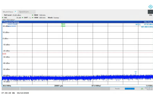
NTVN-n2-PC3-15-10-L-DFT-QPSK-Inner_1RB_Left-30-1000-PA SS
