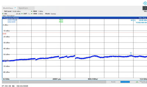
NTNV-n2-PC3-15-5-H-DFT-QPSK-Inner_1RB_Right-3000-12000 -PASS
