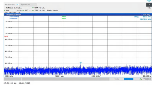
NTNV-n2-PC3-15-5-H-DFT-QPSK-Inner_1RB_Right-0.15-30-PAS S
