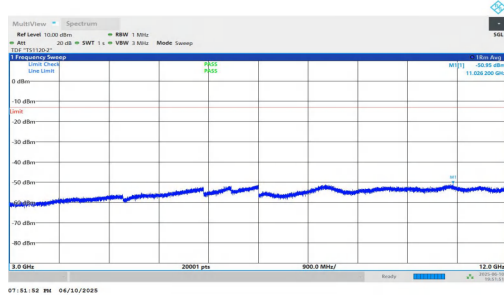
NTVN-n2-PC3-15-5-H-DFT-BPSK-Inner_1RB_Left-3000-12000-P ASS
