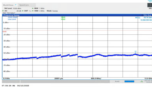
NTNV-n2-PC3-15-10-L-DFT-BPSK-Inner_1RB_Left-3000-12000-PASS
