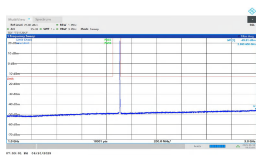
NTNV-n2-PC3-15-5-H-DFT-QPSK-Inner_1RB_Left-1000-3000-PA SS
