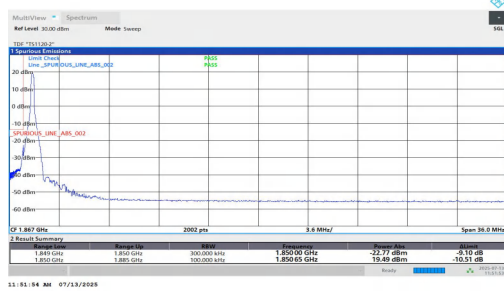
NTV-n2-PC3-15-35-L-DFT-QPSK-Edge_1RB_Left-PASS
