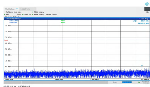
NTVN-n2-PC3-15-10-L-DFT-QPSK-Inner_1RB_Left-0.15-30-PASS
