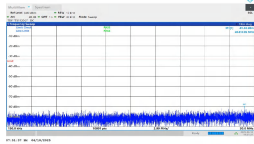
NTVN-n2-PC3-15-5-H-DFT-BPSK-Inner_1RB_Left-0.15-30-PASS
