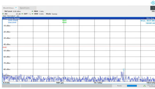
NTNV-n2-PC3-15-10-L-DFT-BPSK-Inner_1RB_Right-0.009-0.15-PASS
