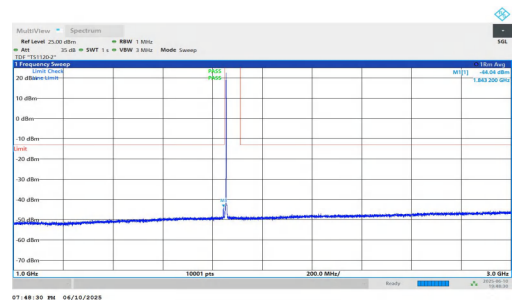
NTNV-n2-PC3-15-5-L-DFT-QPSK-Inner_1RB_Right-1000-3000-P ASS
