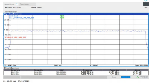
NTNV-n2-PC3-15-30-L-DFT-QPSK-Outer_Full-PASS
