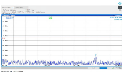
NTVN-n2-PC3-15-10-L-DFT-QPSK-Inner_1RB_Left-0.009-0.15-P ASS
