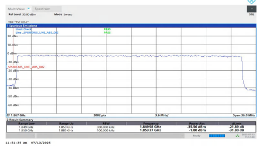
NTV-n2-PC3-15-35-L-DFT-QPSK-Outer_Full-PASS
