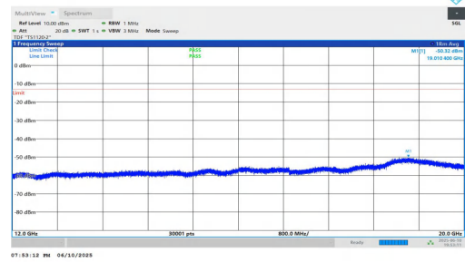
NTNV-n2-PC3-15-5-H-DFT-QPSK-Inner_1RB_Left-12000-20000-P PASS
