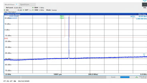
NTVN-n2-PC3-15-5-H-DFT-BPSK-Inner_1RB_Left-1000-3000-PA SS
