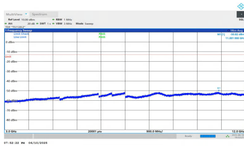
NTNV-n2-PC3-15-5-H-DFT-BPSK-Inner_1RB_Right-3000-12000- PASS
