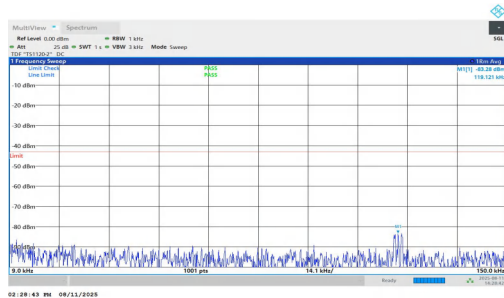
NTVN-n2-PC3-15-5-H-DFT-BPSK-Inner_1RB_Right-0.009-0.15-P ASS
