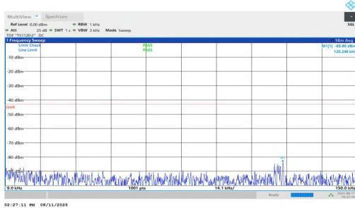
NTNV-n2-PC3-15-5-L-DFT-QPSK-Inner_1RB_Left-0.009-0.15-PA SS
