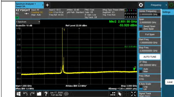
66-66-15MHz-10MHz-QPSK-QPSK-132047-132167-1RB#0-0RB #0-1000~3000MHz-PASS
