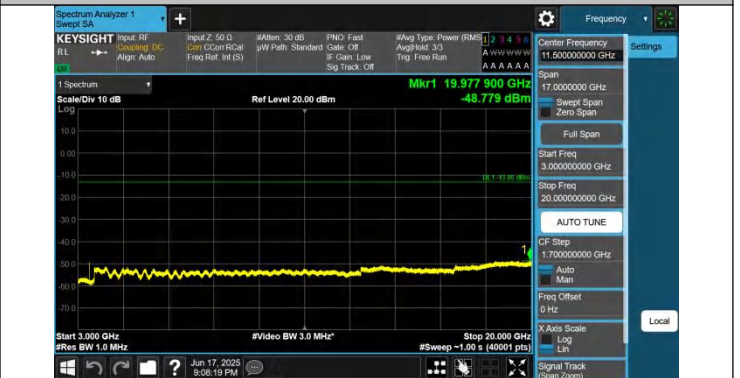
66-66-15MHz-20MHz-QPSK-QPSK-132050-132221-1RB#0-0RB #0-3000~20000MHz-PASS
