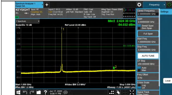
66-66-15MHz-20MHz-QPSK-QPSK-132050-132221-1RB#0-0RB #0-1000~3000MHz-PASS
