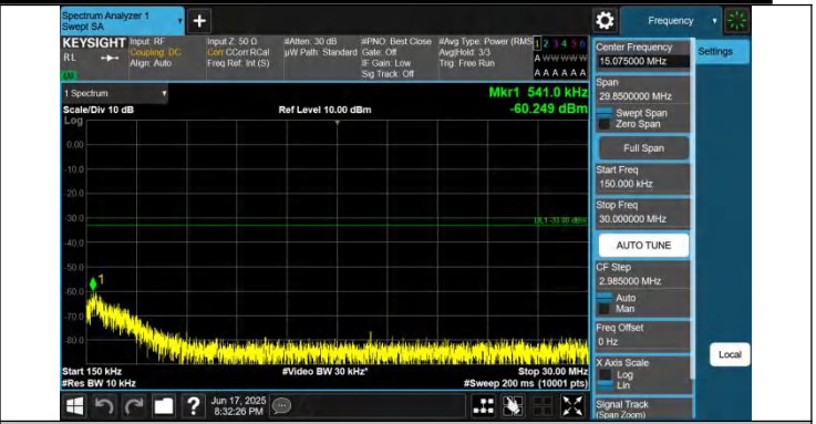
66-66-15MHz-15MHz-QPSK-QPSK-132047-132197-1RB#0-0RB #0-0.15~30MHz-PASS
