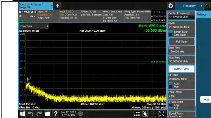
66-66-15MHz-20MHz-QPSK-QPSK-132050-132221-1RB#0-0RB #0-0.15~30MHz-PASS
