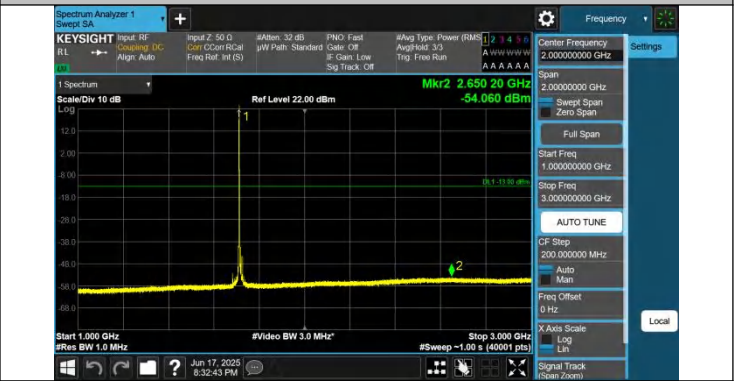
66-66-15MHz-15MHz-QPSK-QPSK-132047-132197-1RB#0-0RB #0-1000~3000MHz-PASS
