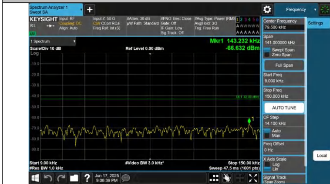
66-66-15MHz-20MHz-QPSK-QPSK-132325-132496-1RB#0-0RB #0-0.009~0.15MHz-PASS
