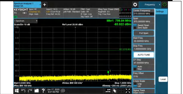
66-66-15MHz-20MHz-QPSK-QPSK-132050-132221-1RB#0-0RB #0-30~1000MHz-PASS
