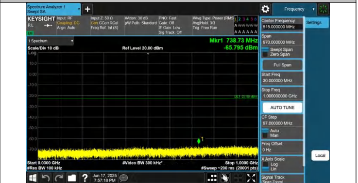
66-66-15MHz-10MHz-QPSK-QPSK-132047-132167-1RB#0-0RB #0-30~1000MHz-PASS
