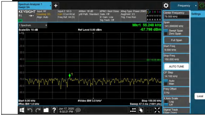
66-66-15MHz-15MHz-QPSK-QPSK-132047-132197-1RB#0-0RB #0-0.009~0.15MHz-PASS
