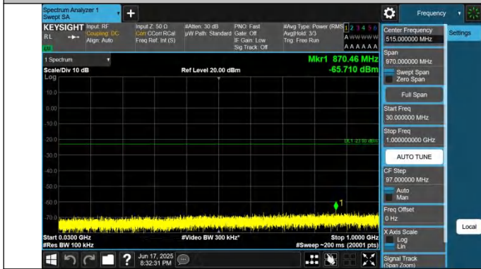
66-66-15MHz-15MHz-QPSK-QPSK-132047-132197-1RB#0-0RB #0-30~1000MHz-PASS
