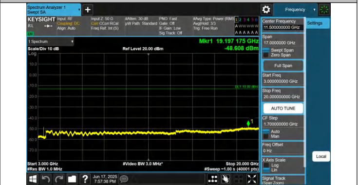
66-66-15MHz-10MHz-QPSK-QPSK-132047-132167-1RB#0-0RB #0-3000~20000MHz-PASS
