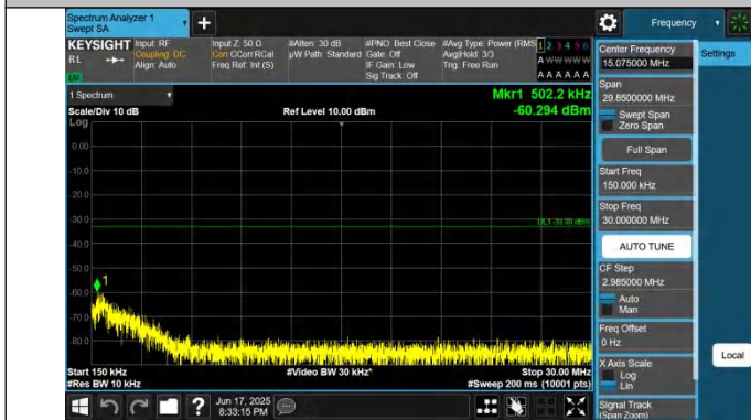
66-66-15MHz-15MHz-QPSK-QPSK-132347-132497-1RB#0-0RB #0-0.15~30MHz-PASS
