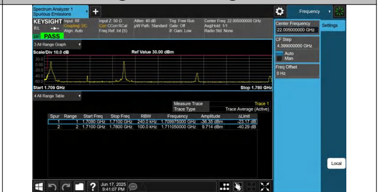
66-66-20MHz-5MHz-QPSK@QPSK-QPSK@QPSK-132072-132189-1RB#0@100RB#0-0RB#0@25RB#0-PASS
