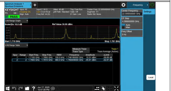
66-66-20MHz-15MHz-QPSK@QPSK-QPSK@QPSK-132423-1325 94-1RB#0@100RB#0-1RB#74@75RB#0-PASS
