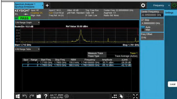
66-66-20MHz-15MHz-QPSK@QPSK-QPSK@QPSK-132423-13 2594-1RB#0@100RB#0-0RB#0@75RB#0-PASS
