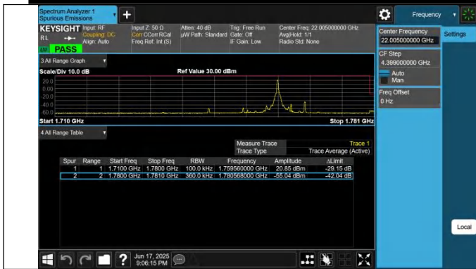
66-66-15MHz-20MHz-QPSK@QPSK-QPSK@QPSK-132401-132572-1RB#74@75RB#0-0RB#0@100RB#0-PASS
