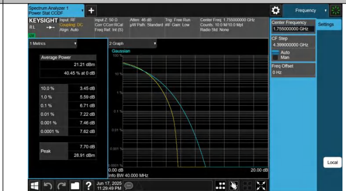
66-66-20MHz-20MHz-64QAM-64QAM-132323-132521-100RB#0 -100RB#0-PASS
