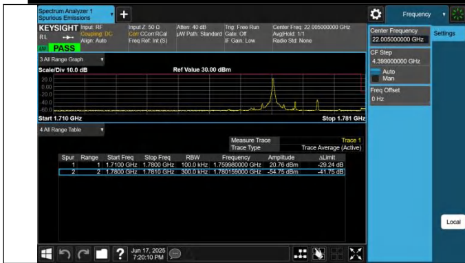
66-66-10MHz-20MHz-QPSK@QPSK-QPSK@QPSK-132428-13 2572-1RB#49@50RB#0-0RB#0@100RB#0-PASS
