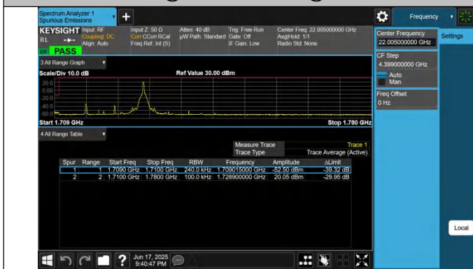
66-66-20MHz-5MHz-QPSK@QPSK-QPSK@QPSK-132072-132189-1RB#0@100RB#0-0RB#0@25RB#0-PASS
