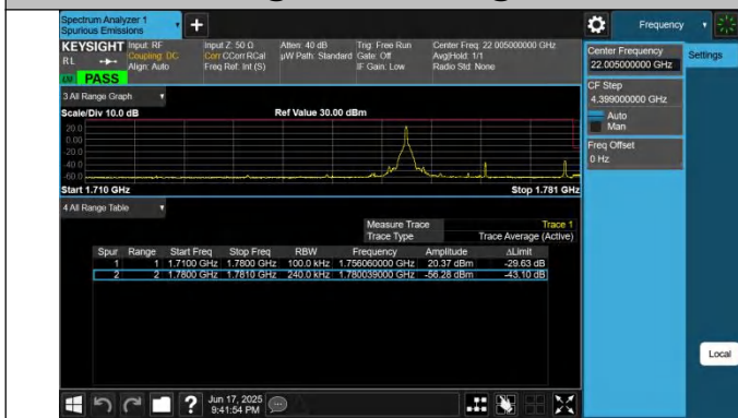
66-66-20MHz-5MHz-QPSK@QPSK-QPSK@QPSK-132522-132572-1RB#0@100RB#0-0RB#0@25RB#0-PASS
