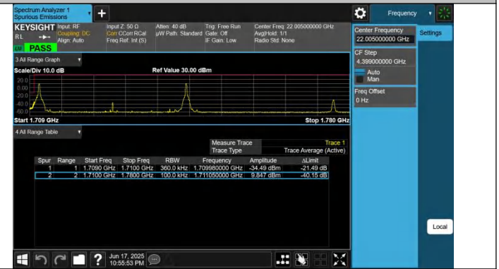
66-66-20MHz-15MHz-QPSK@QPSK-QPSK@QPSK-132072-1322 43-1RB#0@100RB#0-1RB#74@75RB#0-PASS
