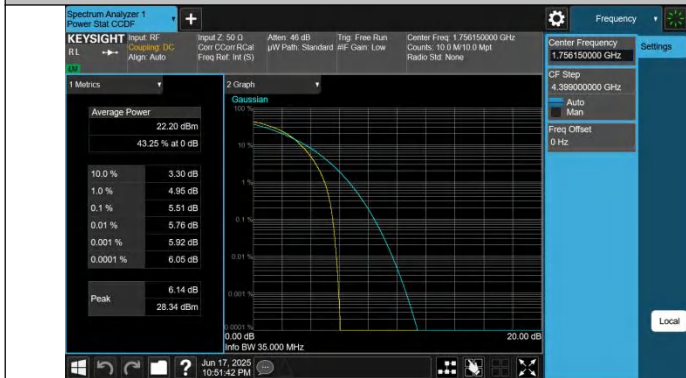
66-66-20MHz-15MHz-QPSK-QPSK-132348-132519-100RB#0-75 RB#0-PASS
