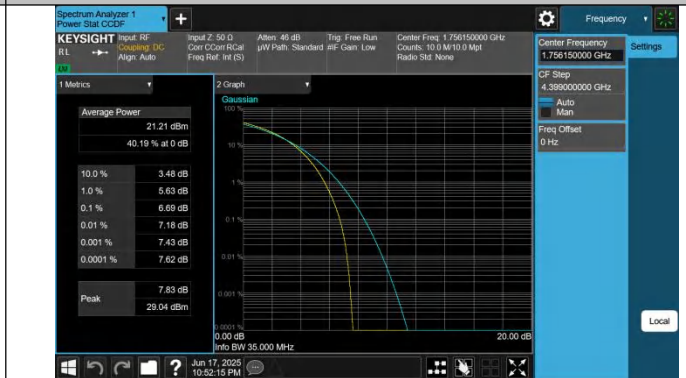
66-66-20MHz-15MHz-64QAM-64QAM-132348-132519-100RB#0 -75RB#0-PASS
