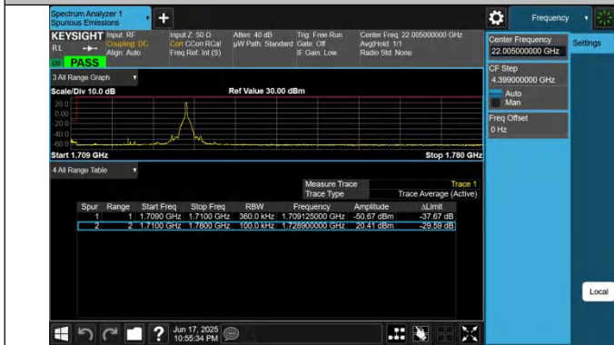
66-66-20MHz-15MHz-QPSK@QPSK-QPSK@QPSK-132072-13 2243-1RB#99@100RB#0-0RB#0@75RB#0-PASS
