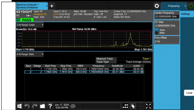
66-66-20MHz-10MHz-QPSK@QPSK-QPSK@QPSK-132473-13 2617-1RB#99@100RB#0-0RB#0@50RB#0-PASS
