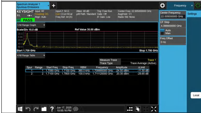
66-66-20MHz-15MHz-QPSK@QPSK-QPSK@QPSK-132072-13 2243-1RB#0@100RB#0-0RB#0@75RB#0-PASS
