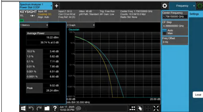
66-66-20MHz-15MHz-256QAM-256QAM-132348-132519-100RB# 0-75RB#0-PASS
