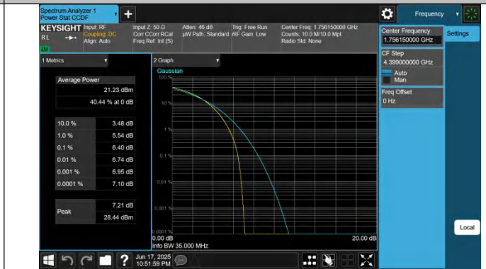
66-66-20MHz-15MHz-16QAM-16QAM-132348-132519-100RB#0 -75RB#0-PASS
