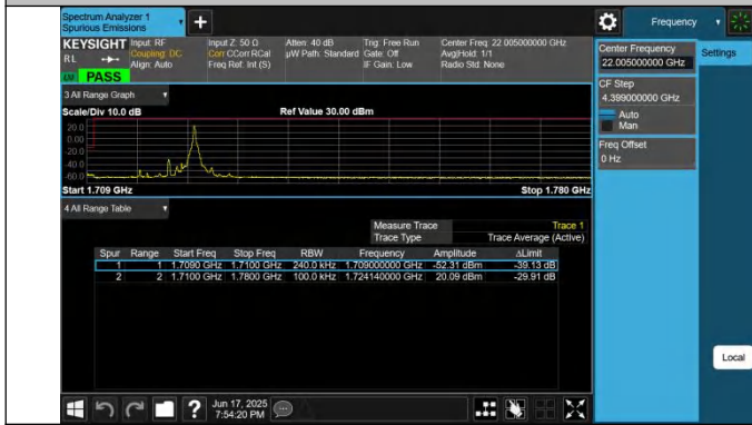
66-66-15MHz-10MHz-QPSK@QPSK-QPSK@QPSK-132047-13 2167-1RB#74@75RB#0-0RB#0@50RB#0-PASS
