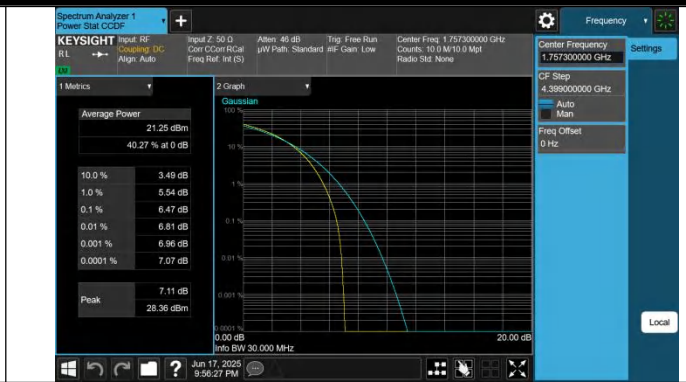
66-66-20MHz-10MHz-16QAM-16QAM-132373-132517-100RB#0 -50RB#0-PASS
