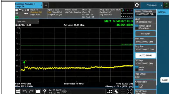
66-66-15MHz-5MHz-QPSK-QPSK-132549-132642-1RB#74-0RB #0-3000~20000MHz-PASS
