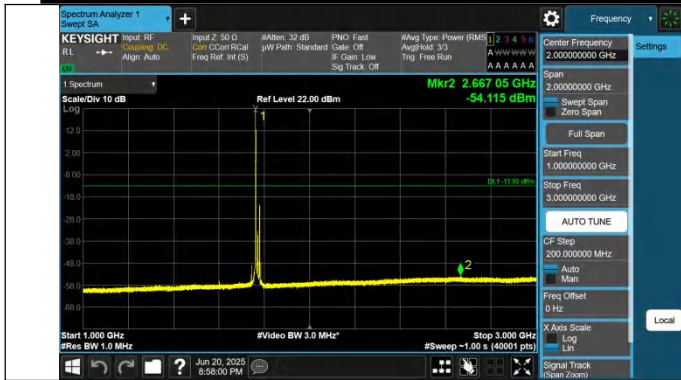
66-66-15MHz-5MHz-QPSK-QPSK-132549-132642-1RB#0-1RB# 24-1000~3000MHz-PASS
