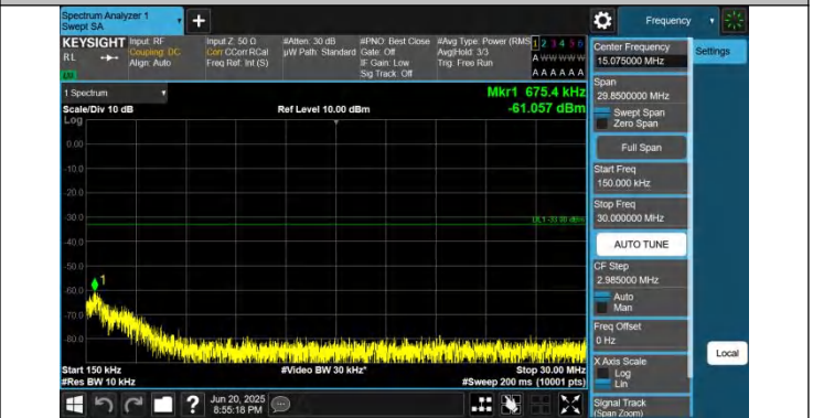
66-66-15MHz-5MHz-QPSK-QPSK-132398-132491-1RB#0-1RB# 24-0.15~30MHz-PASS
