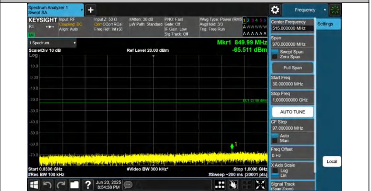
66-66-15MHz-5MHz-QPSK-QPSK-132398-132491-1RB#74-0RB #0-30~1000MHz-PASS
