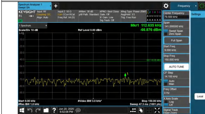
66-66-15MHz-5MHz-QPSK-QPSK-132047-132140-1RB#74-0RB #0-0.009~0.15MHz-PASS
