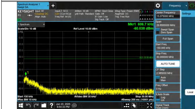
66-66-15MHz-5MHz-QPSK-QPSK-132398-132491-1RB#74-0RB #0-0.15~30MHz-PASS
