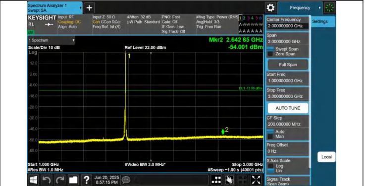
66-66-15MHz-5MHz-QPSK-QPSK-132549-132642-1RB#74-0RB #0-1000~3000MHz-PASS
