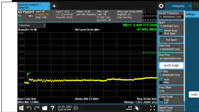
66-66-15MHz-5MHz-QPSK-QPSK-132047-132140-1RB#74-0RB #0-3000~20000MHz-PASS
