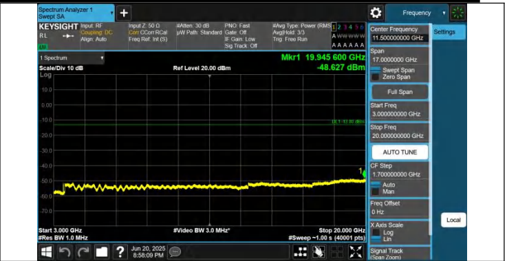
66-66-15MHz-5MHz-QPSK-QPSK-132549-132642-1RB#0-1RB# 24-3000~20000MHz-PASS
