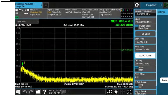
66-66-10MHz-10MHz-QPSK-QPSK-132022-132121-1RB#49-0R B#0-0.15~30MHz-PASS
