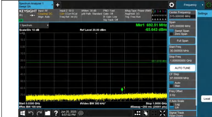
66-66-15MHz-5MHz-QPSK-QPSK-132549-132642-1RB#74-0RB #0-30~1000MHz-PASS
