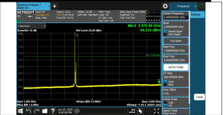
66-66-15MHz-5MHz-QPSK-QPSK-132398-132491-1RB#0-1RB# 24-1000~3000MHz-PASS
