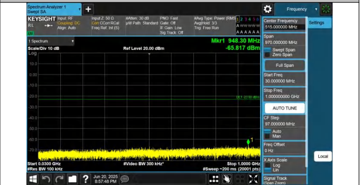
66-66-15MHz-5MHz-QPSK-QPSK-132549-132642-1RB#0-1RB# 24-30~1000MHz-PASS
