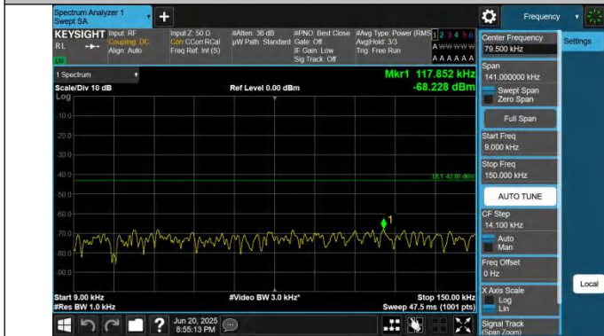
66-66-15MHz-5MHz-QPSK-QPSK-132398-132491-1RB#0-1RB# 24-0.009~0.15MHz-PASS
