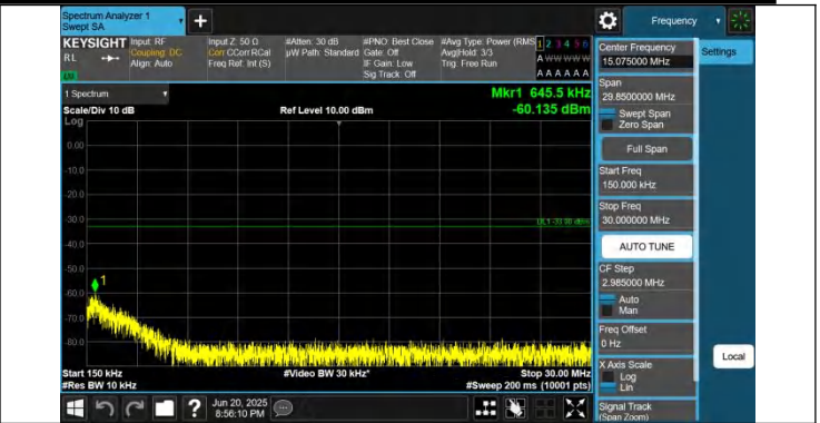
66-66-15MHz-5MHz-QPSK-QPSK-132549-132642-1RB#0-0RB# 0-0.15~30MHz-PASS
