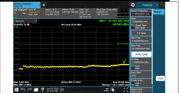
66-66-10MHz-5MHz-QPSK-QPSK-132022-132094-1RB#0-1RB# 24-3000~20000MHz-PASS
