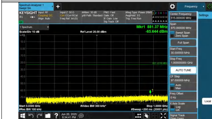
66-66-5MHz-15MHz-QPSK-QPSK-132002-132095-1RB#0-0RB# 0-30~1000MHz-PASS
