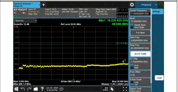
66-66-5MHz-15MHz-QPSK-QPSK-132002-132095-1RB#0-1RB# 74-3000~20000MHz-PASS
