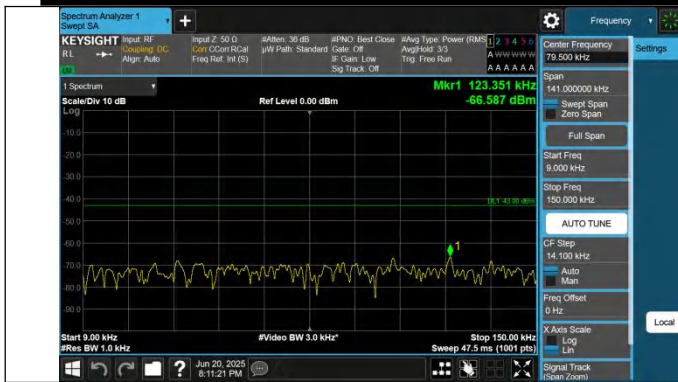
66-66-10MHz-5MHz-QPSK-QPSK-132572-132644-1RB#49-0RB #0-0.009~0.15MHz-PASS
