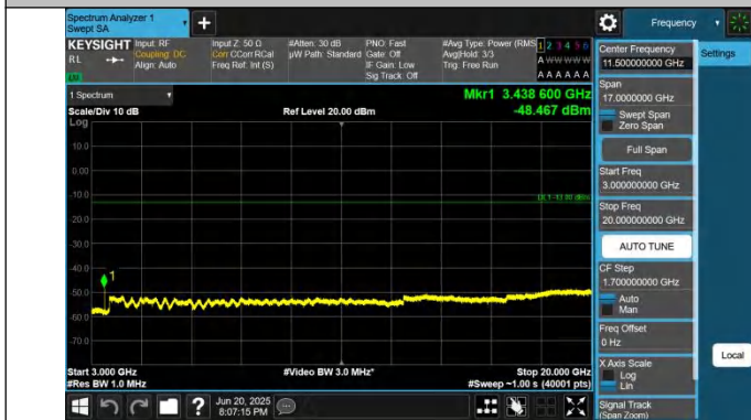
66-66-10MHz-5MHz-QPSK-QPSK-132022-132094-1RB#49-0RB #0-3000~20000MHz-PASS
