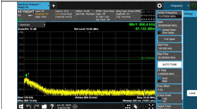
66-66-5MHz-15MHz-QPSK-QPSK-132002-132095-25RB#0-75R B#0-0.15~30MHz-PASS
