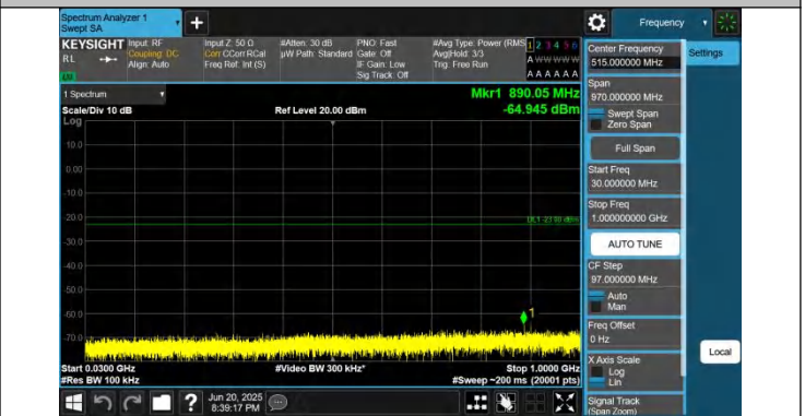
66-66-5MHz-15MHz-QPSK-QPSK-132353-132446-1RB#0-1RB# 74-30~1000MHz-PASS
