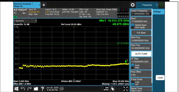
66-66-5MHz-15MHz-QPSK-QPSK-132353-132446-1RB#0-1RB# 74-3000~20000MHz-PASS
