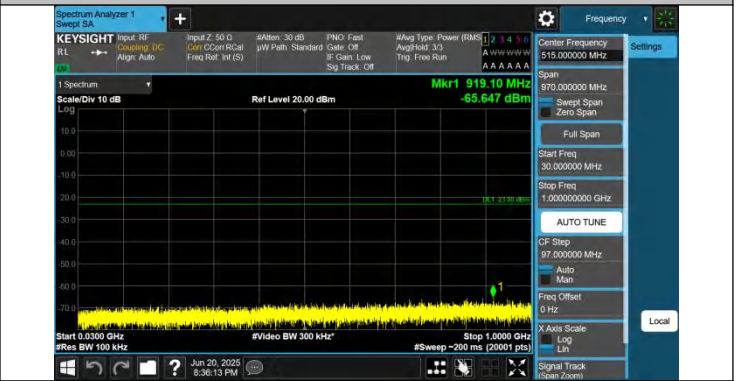
66-66-5MHz-15MHz-QPSK-QPSK-132002-132095-1RB#0-1RB# 74-30~1000MHz-PASS
