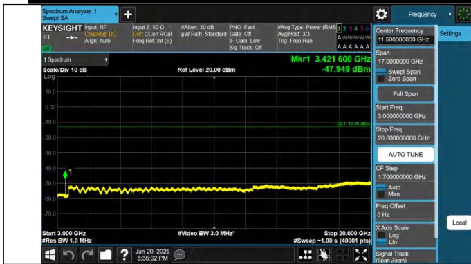
66-66-5MHz-15MHz-QPSK-QPSK-132002-132095-1RB#0-0RB# 0-3000~20000MHz-PASS
