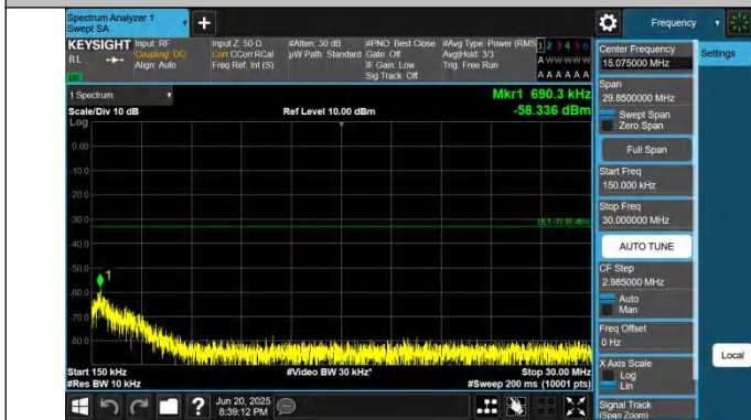
66-66-5MHz-15MHz-QPSK-QPSK-132353-132446-1RB#0-1RB# 74-0.15~30MHz-PASS
