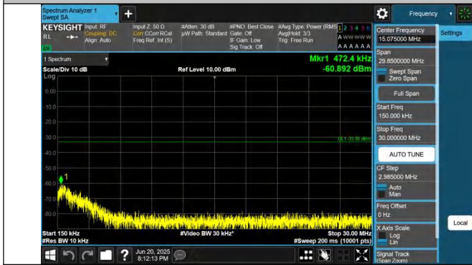
66-66-10MHz-5MHz-QPSK-QPSK-132572-132644-1RB#0-1RB# 24-0.15~30MHz-PASS
