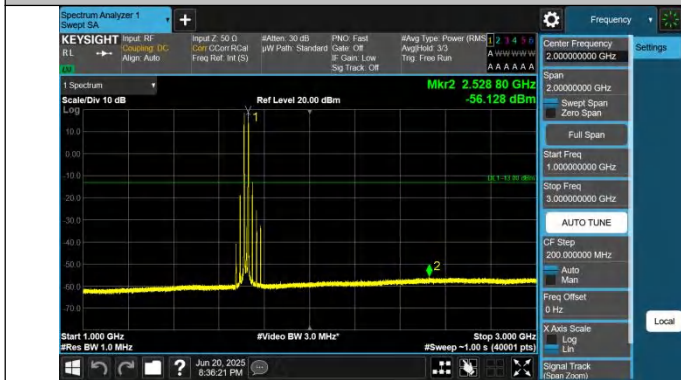
66-66-5MHz-15MHz-QPSK-QPSK-132002-132095-1RB#0-1RB# 74-1000~3000MHz-PASS
