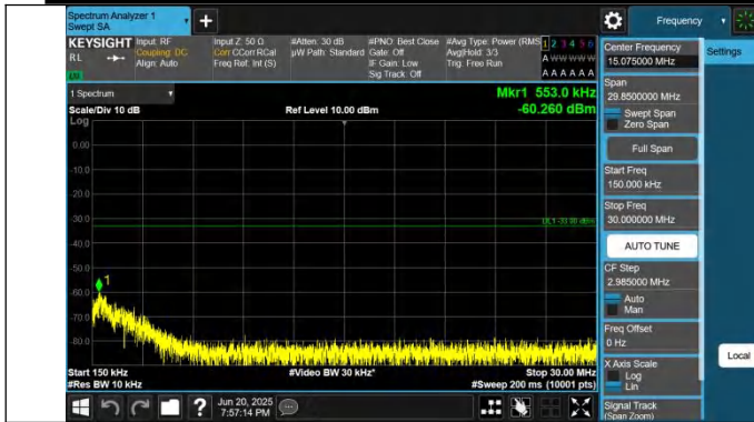
66-66-5MHz-10MHz-QPSK-QPSK-132550-132622-1RB#24-0RB #0-0.15~30MHz-PASS
