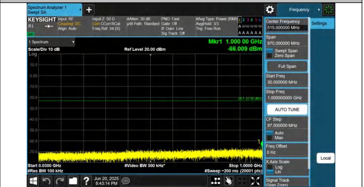
66-66-5MHz-15MHz-QPSK-QPSK-132504-132597-25RB#0-75R B#0-30~1000MHz-PASS
