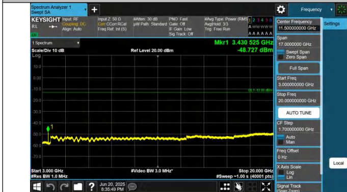
66-66-5MHz-15MHz-QPSK-QPSK-132002-132095-1RB#24-0RB #0-3000~20000MHz-PASS
