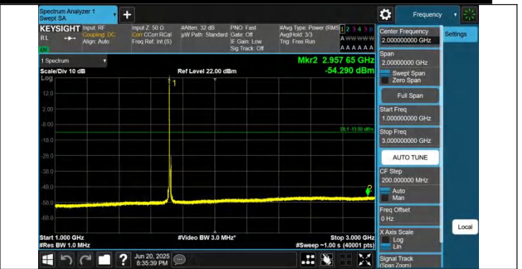
66-66-5MHz-15MHz-QPSK-QPSK-132002-132095-1RB#24-0RB #0-1000~3000MHz-PASS
