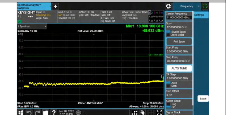
66-66-5MHz-15MHz-QPSK-QPSK-132002-132095-25RB#0-75R B#0-3000~20000MHz-PASS
