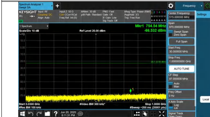
66-66-10MHz-5MHz-QPSK-QPSK-132572-132644-1RB#49-0RB #0-30~1000MHz-PASS
