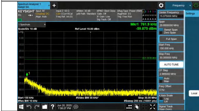
66-66-5MHz-10MHz-QPSK-QPSK-132550-132622-1RB#0-0RB# 0-0.15~30MHz-PASS
