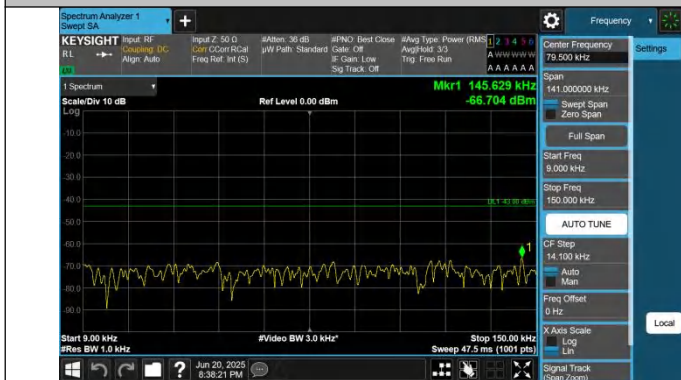
66-66-5MHz-15MHz-QPSK-QPSK-132353-132446-1RB#24-0RB #0-0.009~0.15MHz-PASS
