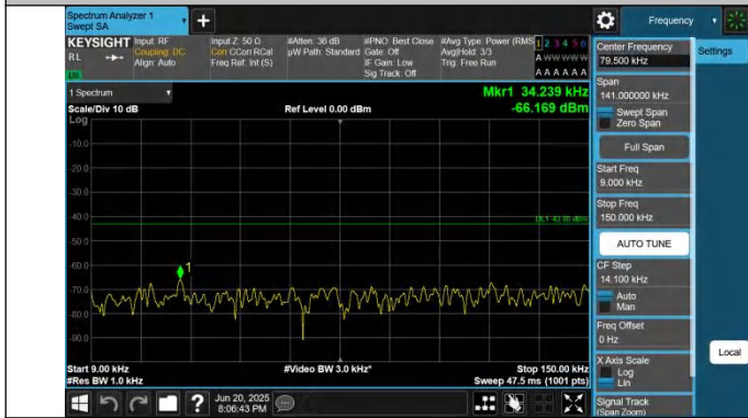
66-66-10MHz-5MHz-QPSK-QPSK-132022-132094-1RB#49-0RB #0-0.009~0.15MHz-PASS
