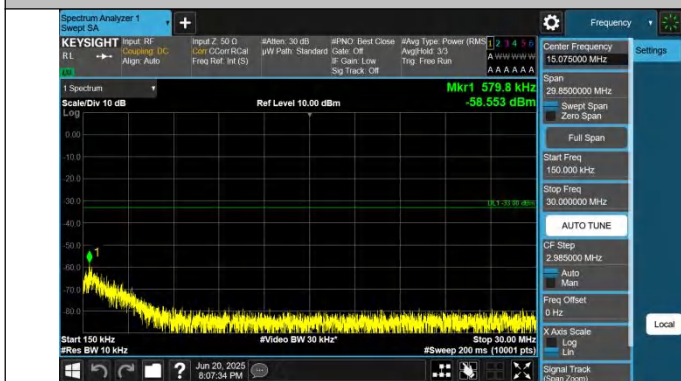
66-66-10MHz-5MHz-QPSK-QPSK-132022-132094-1RB#0-1RB# 24-0.15~30MHz-PASS
