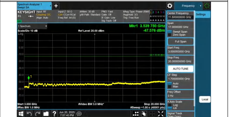
66-66-5MHz-10MHz-QPSK-QPSK-132550-132622-1RB#24-0RB #0-3000~20000MHz-PASS
