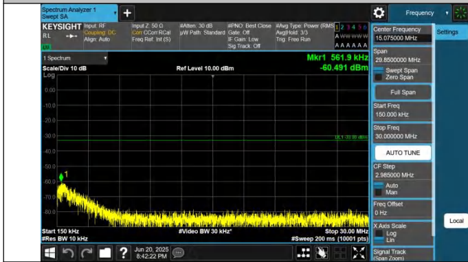
66-66-5MHz-15MHz-QPSK-QPSK-132504-132597-1RB#0-1RB# 74-0.15~30MHz-PASS
