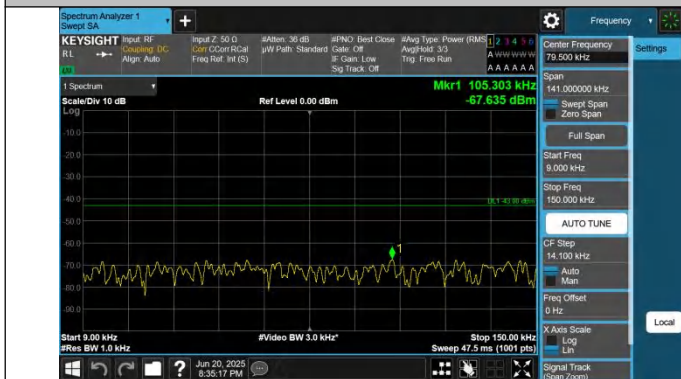
66-66-5MHz-15MHz-QPSK-QPSK-132002-132095-1RB#24-0RB #0-0.009~0.15MHz-PASS
