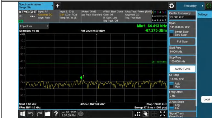
66-66-5MHz-10MHz-QPSK-QPSK-132550-132622-1RB#0-1RB# 49-0.009~0.15MHz-PASS
