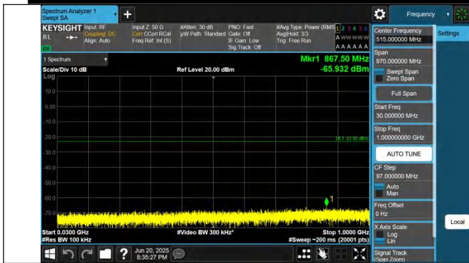
66-66-5MHz-15MHz-QPSK-QPSK-132002-132095-1RB#24-0RB #0-30~1000MHz-PASS
