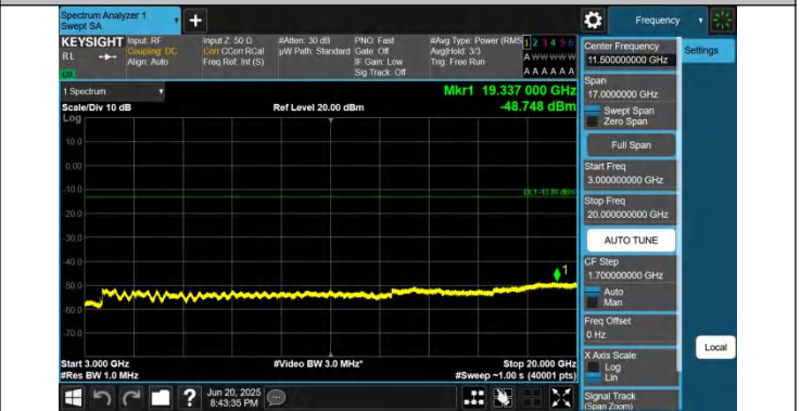
66-66-5MHz-15MHz-QPSK-QPSK-132504-132597-25RB#0-75R B#0-3000~20000MHz-PASS
