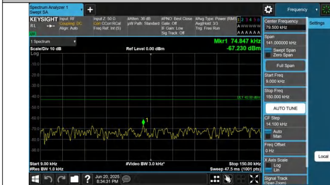
66-66-5MHz-15MHz-QPSK-QPSK-132002-132095-1RB#0-0RB# 0-0.009~0.15MHz-PASS
