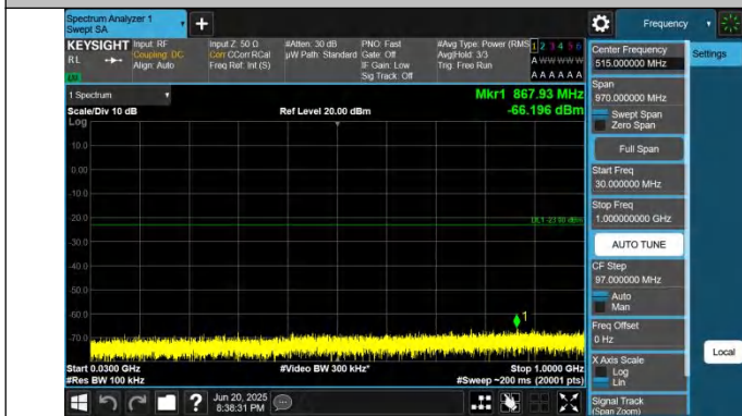
66-66-5MHz-15MHz-QPSK-QPSK-132353-132446-1RB#24-0RB #0-30~1000MHz-PASS
