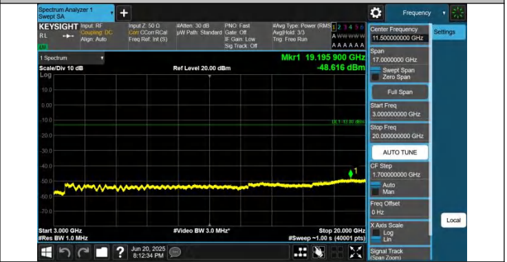
66-66-10MHz-5MHz-QPSK-QPSK-132572-132644-1RB#0-1RB# 24-3000~20000MHz-PASS
