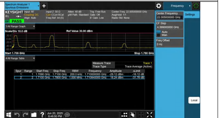
66-66-15MHz-5MHz-QPSK@QPSK-QPSK@QPSK-132047-1321 40-1RB#0@75RB#0-1RB#24@25RB#0-PASS
