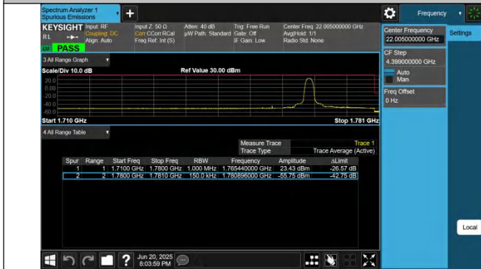
66-66-10MHz-5MHz-QPSK@QPSK-QPSK@QPSK-132572-1326 44-1RB#0@50RB#0-0RB#0@25RB#0-PASS
