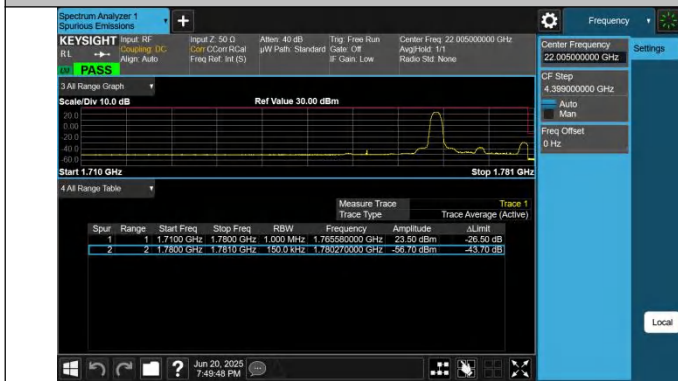
66-66-5MHz-10MHz-QPSK@QPSK-QPSK@QPSK-132550-1326 22-1RB#0@25RB#0-0RB#0@50RB#0-PASS
