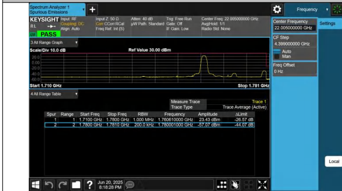
66-66-10MHz-10MHz-QPSK@QPSK-QPSK@QPSK-132523-132 622-1RB#0@50RB#0-0RB#0@50RB#0-PASS
