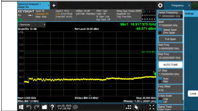
66-66-5MHz-5MHz-QPSK-QPSK-132398-132446-1RB#0-1RB#1 5-3000~20000MHz-PASS
