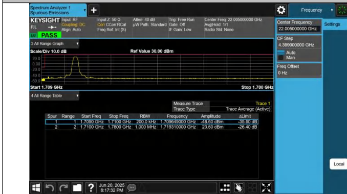
66-66-10MHz-10MHz-QPSK@QPSK-QPSK@QPSK-132022-132 121-1RB#49@50RB#0-0RB#0@50RB#0-PASS
