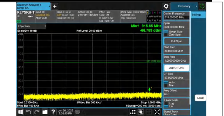
66-66-5MHz-5MHz-QPSK-QPSK-131997-132045-1RB#0-1RB#1 5-30~1000MHz-PASS
