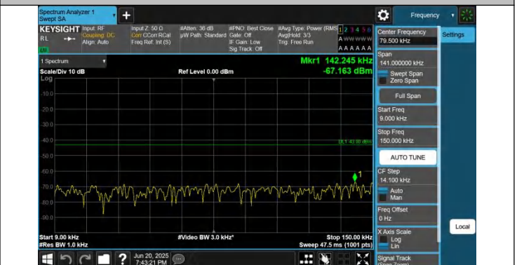
66-66-5MHz-5MHz-QPSK-QPSK-132599-132647-1RB#0-1RB#1 5-0.009~0.15MHz-PASS
