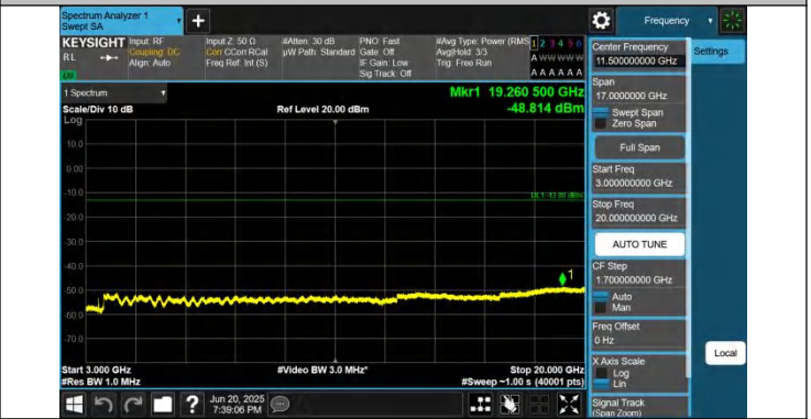
66-66-5MHz-5MHz-QPSK-QPSK-131997-132045-1RB#0-1RB#1 5-3000~20000MHz-PASS
