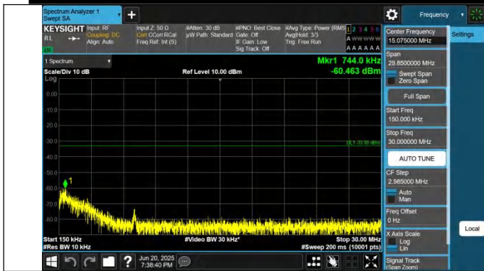
66-66-5MHz-5MHz-QPSK-QPSK-131997-132045-1RB#0-1RB#1 5-0.15~30MHz-PASS
