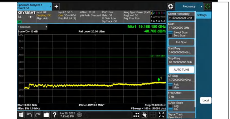
66-66-5MHz-5MHz-QPSK-QPSK-132599-132647-1RB#0-1RB#1 5-3000~20000MHz-PASS
