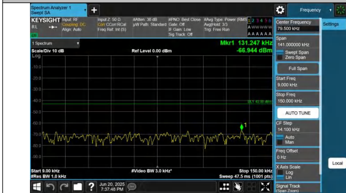
66-66-5MHz-5MHz-QPSK-QPSK-131997-132045-1RB#24-0RB# 0-0.009~0.15MHz-PASS
