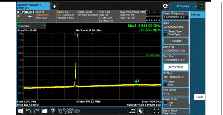
66-66-5MHz-5MHz-QPSK-QPSK-132398-132446-1RB#0-1RB#1 5-1000~3000MHz-PASS
