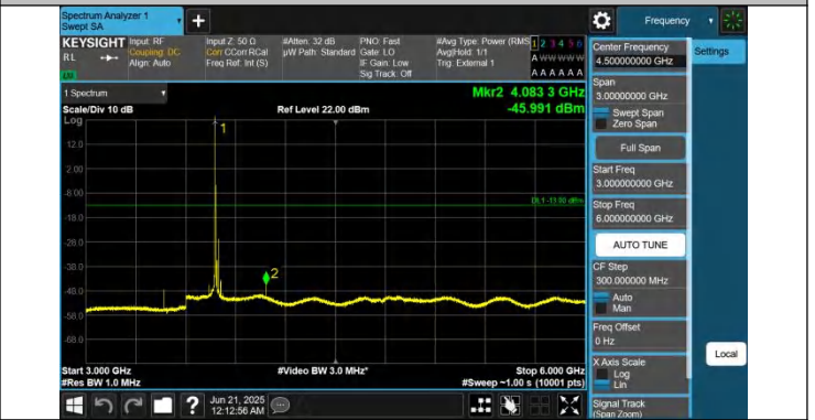
43-43-20MHz-5MHz-QPSK-QPSK-45440-45557-1RB#0-0RB#0-3 000~6000MHz-PASS
