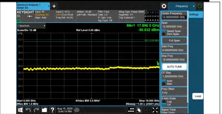
43-43-15MHz-20MHz-QPSK-QPSK-44668-44839-1RB#0-0RB#0-6000~18000MHz-PASS
