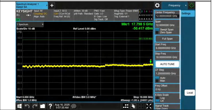
43-43-10MHz-20MHz-QPSK-QPSK-44996-45140-1RB#0-0RB#0-6000~18000MHz-PASS
