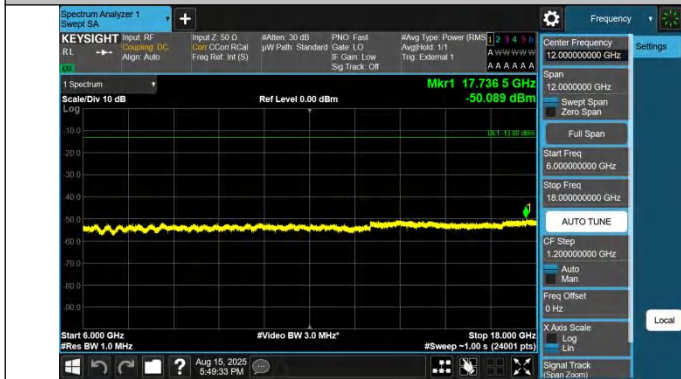
43-43-20MHz-5MHz-QPSK-QPSK-44690-44807-1RB#0-0RB#0-6000~18000MHz-PASS
