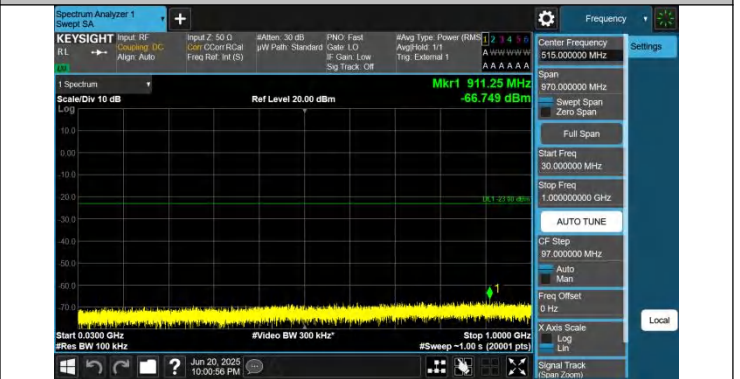
43-43-10MHz-20MHz-QPSK-QPSK-45346-45490-1RB#0-0RB#0-30~1000MHz-PASS
