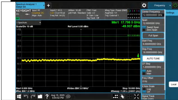
43-43-20MHz-15MHz-QPSK-QPSK-44690-44861-1RB#0-0RB#0-6000~18000MHz-PASS
