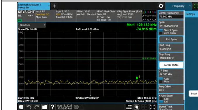
43-43-10MHz-20MHz-QPSK-QPSK-44996-45140-1RB#0-0RB#0-0.009~0.15MHz-PASS
