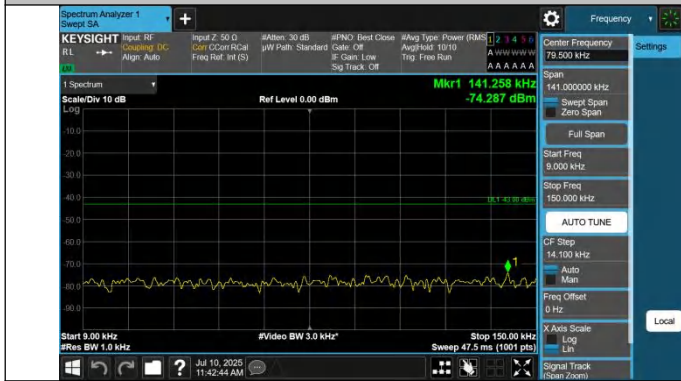
43-43-20MHz-15MHz-QPSK-QPSK-45016-45187-1RB#0-0RB#0-0.009~0.15MHz-PASS
