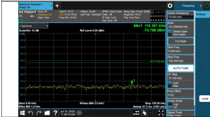
43-43-15MHz-20MHz-QPSK-QPSK-45319-45490-1RB#0-0RB#0-0.009~0.15MHz-PASS
