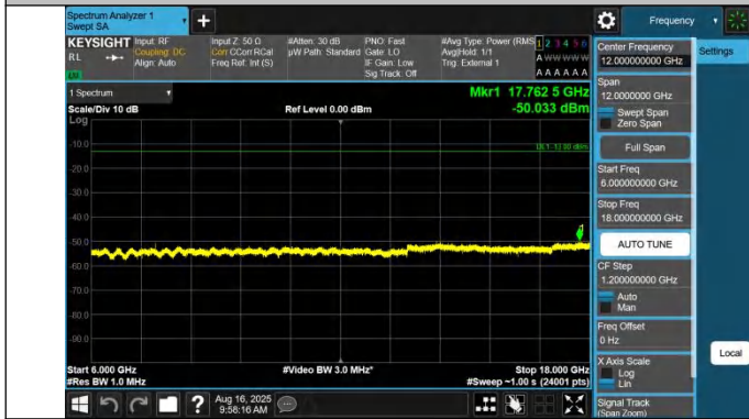
43-43-10MHz-20MHz-QPSK-QPSK-45346-45490-1RB#0-0RB#0-6000~18000MHz-PASS
