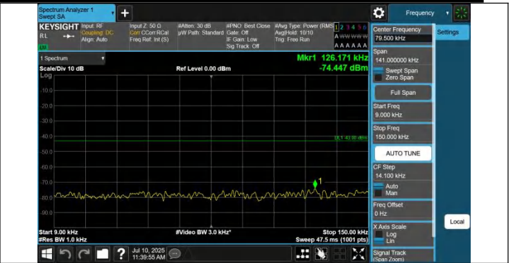
43-43-20MHz-5MHz-QPSK-QPSK-44690-44807-1RB#0-0RB#0-0.009~0.15MHz-PASS
