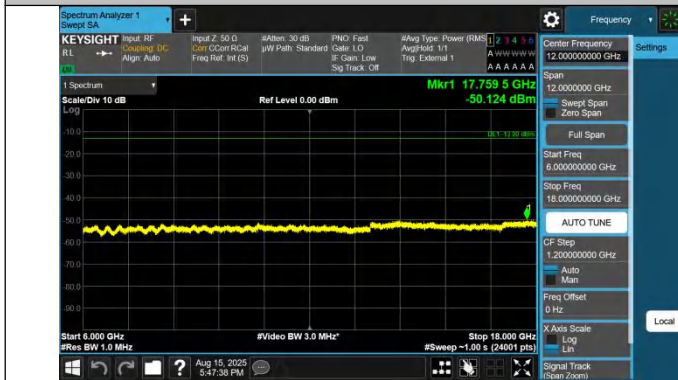
43-43-20MHz-20MHz-QPSK-QPSK-44991-45189-1RB#0-0RB#0-6000~18000MHz-PASS
