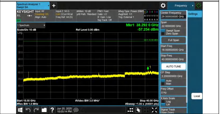
43-43-10MHz-20MHz-QPSK-QPSK-45346-45490-1RB#0-0RB#0-18000~40000MHz-PASS
