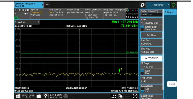
43-43-20MHz-15MHz-QPSK-QPSK-44690-44861-1RB#0-0RB#0-0.009~0.15MHz-PASS
