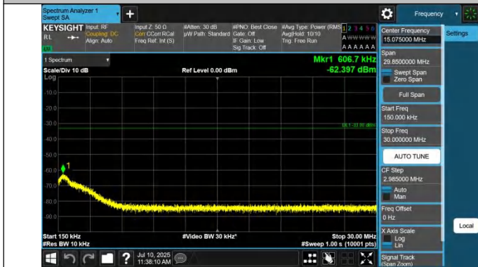
43-43-15MHz-20MHz-QPSK-QPSK-44993-45164-1RB#0-0RB#0-0.15~30MHz-PASS
