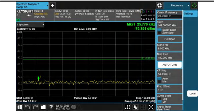
43-43-15MHz-20MHz-QPSK-QPSK-44993-45164-1RB#0-0RB#0-0.009~0.15MHz-PASS
