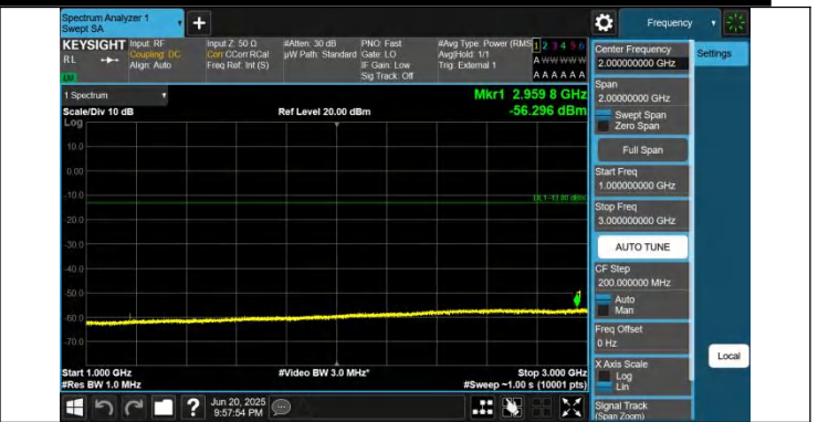
43-43-10MHz-20MHz-QPSK-QPSK-44996-45140-1RB#0-0RB#0-1000~3000MHz-PASS
