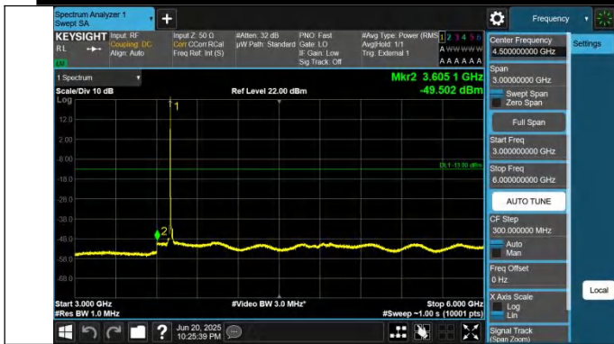
43-43-15MHz-20MHz-QPSK-QPSK-44668-44839-1RB#0-0RB#0-3000~6000MHz-PASS
