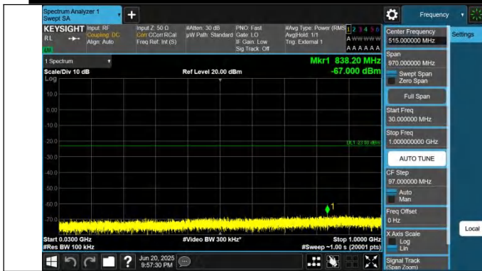
43-43-10MHz-20MHz-QPSK-QPSK-44996-45140-1RB#0-0RB#0-30~1000MHz-PASS
