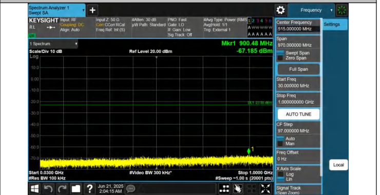
43-43-20MHz-15MHz-QPSK-QPSK-44690-44861-1RB#0-0RB#0-30~1000MHz-PASS
