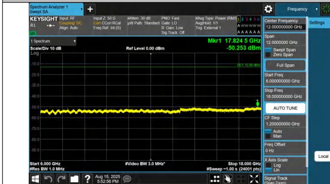
43-43-20MHz-10MHz-QPSK-QPSK-45041-45185-1RB#0-0RB#0-6000~18000MHz-PASS
