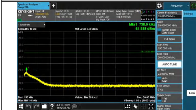
43-43-20MHz-15MHz-QPSK-QPSK-44690-44861-1RB#0-0RB#0-0.15~30MHz-PASS
