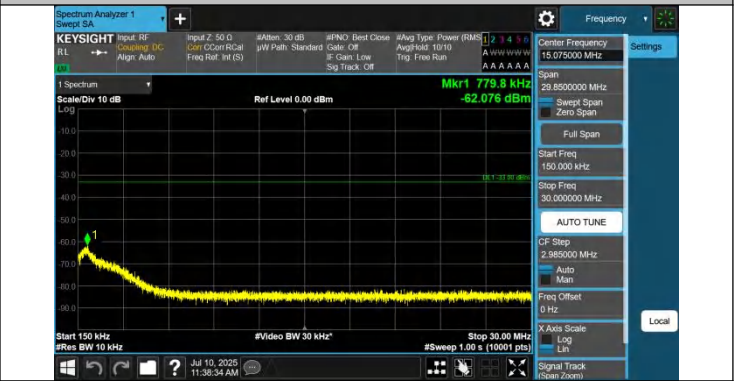
43-43-15MHz-20MHz-QPSK-QPSK-45319-45490-1RB#0-0RB#0-0.15~30MHz-PASS
