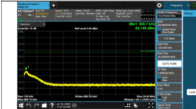
43-43-10MHz-20MHz-QPSK-QPSK-45346-45490-1RB#0-0RB#0-0.15~30MHz-PASS
