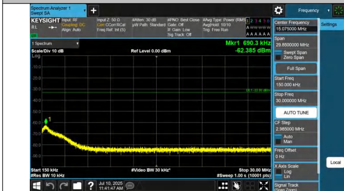
43-43-20MHz-10MHz-QPSK-QPSK-45041-45185-1RB#0-0RB#0-0.15~30MHz-PASS
