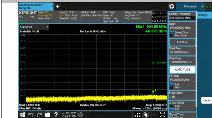
43-43-15MHz-20MHz-QPSK-QPSK-44668-44839-1RB#0-0RB#0-30~1000MHz-PASS
