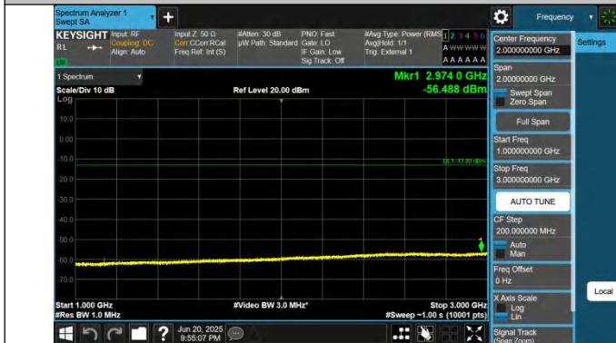
43-43-10MHz-20MHz-QPSK-QPSK-44645-44789-1RB#0-0RB#0-1000~3000MHz-PASS
