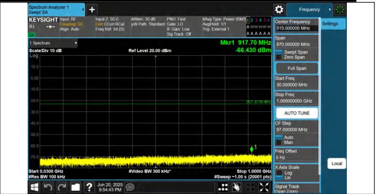
43-43-10MHz-20MHz-QPSK-QPSK-44645-44789-1RB#0-0RB#0-30~1000MHz-PASS
