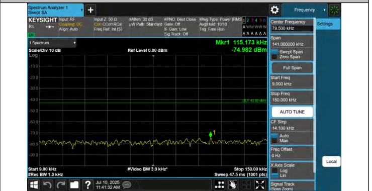
43-43-20MHz-10MHz-QPSK-QPSK-45041-45185-1RB#0-0RB#0-0.009~0.15MHz-PASS
