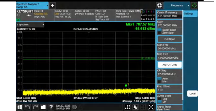
43-43-20MHz-20MHz-QPSK-QPSK-44991-45189-1RB#0-0RB#0-30~1000MHz-PASS
