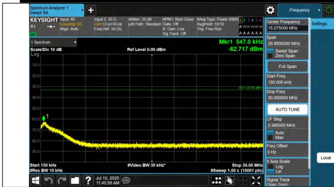
43-43-20MHz-5MHz-QPSK-QPSK-45440-45557-1RB#0-0RB#0-0 0.15~30MHz-PASS
