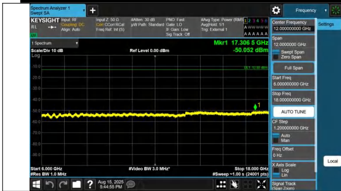
43-43-15MHz-20MHz-QPSK-QPSK-44993-45164-1RB#0-0RB#0-6000~18000MHz-PASS
