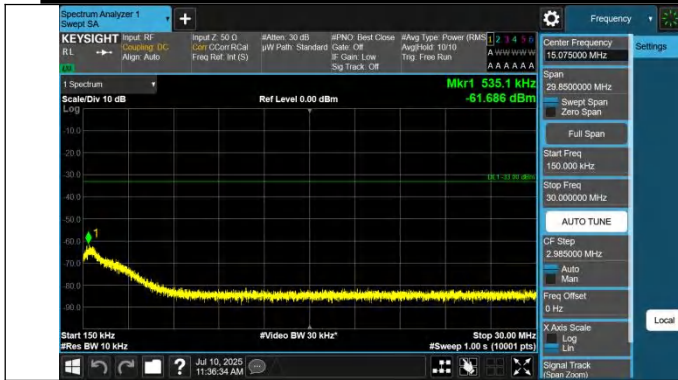
43-43-10MHz-20MHz-QPSK-QPSK-44645-44789-1RB#0-0RB#0-0.15~30MHz-PASS
