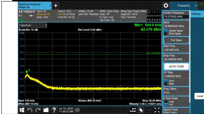
43-43-20MHz-20MHz-QPSK-QPSK-44991-45189-1RB#0-0RB#0-0.15~30MHz-PASS
