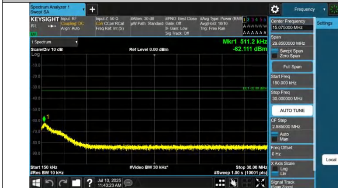
43-43-20MHz-15MHz-QPSK-QPSK-45341-45512-1RB#0-0RB#0-0.15~30MHz-PASS
