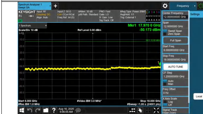
43-43-10MHz-20MHz-QPSK-QPSK-44645-44789-1RB#0-0RB#0-6000~18000MHz-PASS
