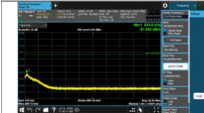
43-43-20MHz-5MHz-QPSK-QPSK-44690-44807-1RB#0-0RB#0-0.15~30MHz-PASS
