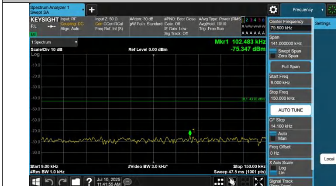
43-43-20MHz-10MHz-QPSK-QPSK-45391-45535-1RB#0-0RB#0-0.009~0.15MHz-PASS
