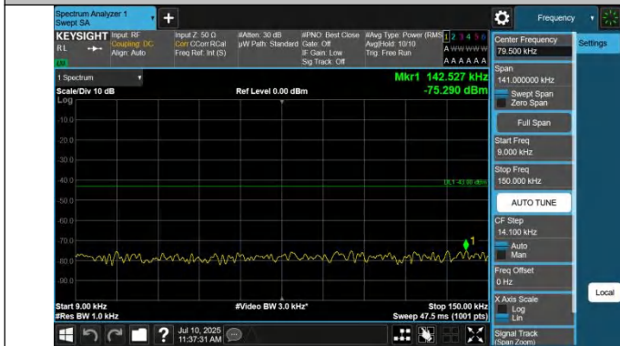
43-43-15MHz-20MHz-QPSK-QPSK-44668-44839-1RB#0-0RB#0-0.009~0.15MHz-PASS
