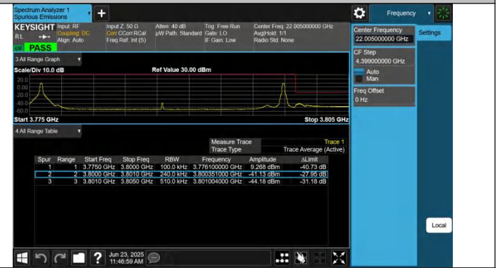
43-43-20MHz-5MHz-QPSK@QPSK-QPSK@QPSK-45440-45557- 1RB#0@100RB#0-1RB#24@25RB#0-PASS
