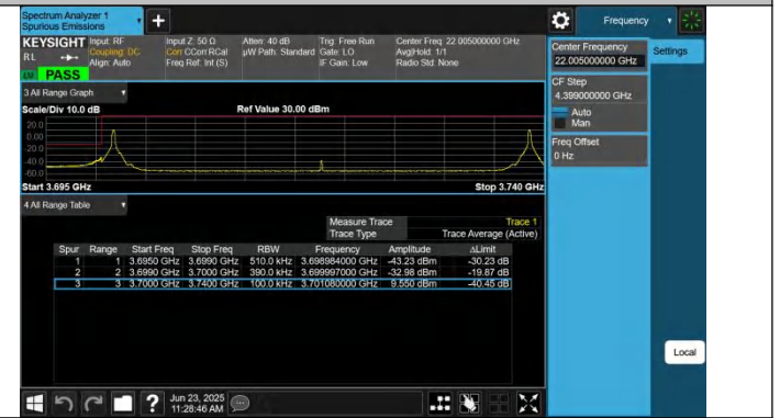
43-43-20MHz-20MHz-QPSK@QPSK-QPSK-44690-44888 -1RB#0@100RB#0-1RB#99@100RB#0-PASS
