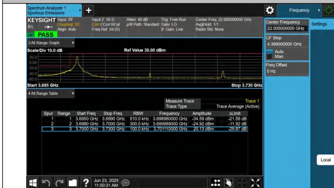
43-43-20MHz-10MHz-QPSK@QPSK-QPSK@QPSK-44690-448 34-1RB#0@100RB#0-0RB#0@50RB#0-PASS
