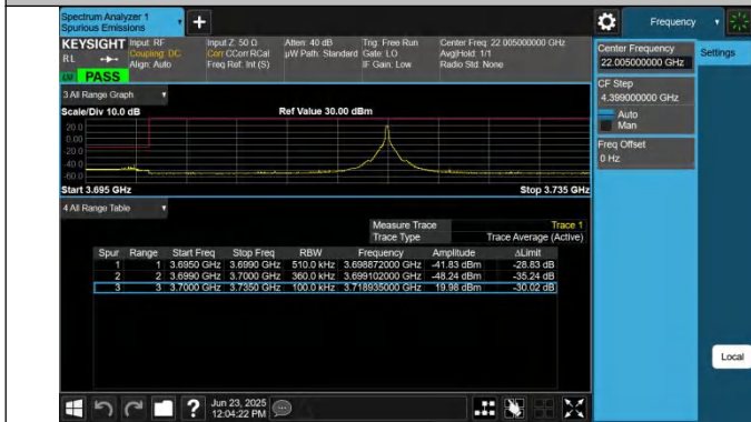
43-43-20MHz-15MHz-QPSK@QPSK-QPSK@QPSK-44690-448 61-1RB#99@100RB#0-0RB#0@75RB#0-PASS
