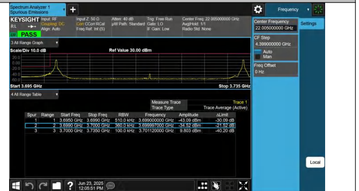
43-43-20MHz-15MHz-QPSK@QPSK-QPSK@QPSK-44690-44861 -1RB#0@100RB#0-1RB#74@75RB#0-PASS
