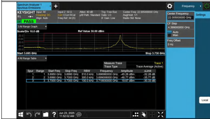
43-43-20MHz-10MHz-QPSK@QPSK-QPSK@QPSK-44690-448 34-1RB#99@100RB#0-0RB#0@50RB#0-PASS
