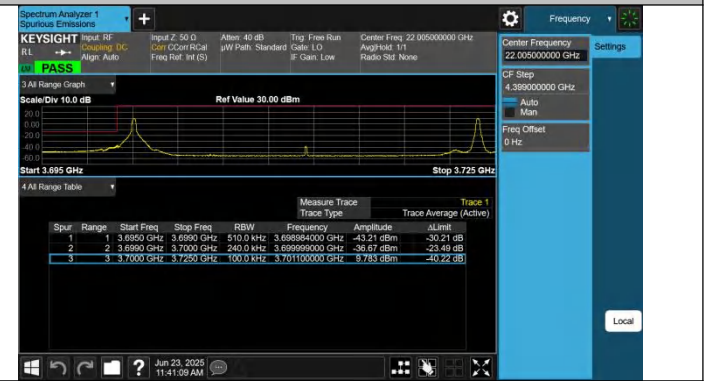
43-43-20MHz-5MHz-QPSK@QPSK-QPSK@QPSK-44690-44807- 1RB#0@100RB#0-1RB#24@25RB#0-PASS
