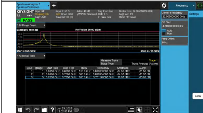
43-43-20MHz-15MHz-QPSK@QPSK-QPSK@QPSK-44690-448 61-1RB#0@100RB#0-0RB#0@75RB#0-PASS
