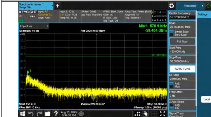
43-43-5MHz-20MHz-QPSK-QPSK-44998-45115-1RB#0-0RB#0-0 .15~30MHz-PASS
