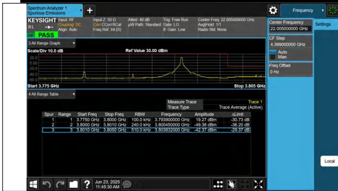
43-43-20MHz-5MHz-QPSK@QPSK-QPSK@QPSK-45440-4555 7-1RB#99@100RB#0-0RB#0@25RB#0-PASS
