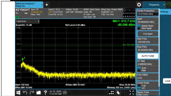
42-42-20MHz-20MHz-QPSK-QPSK-42491-42689-1RB#0-0RB#0-0.15~30MHz-PASS
