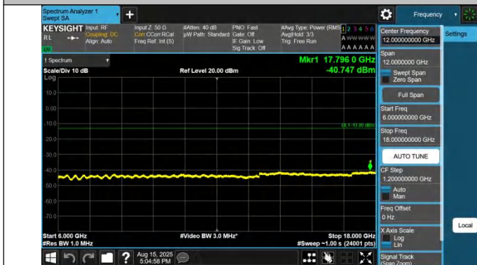
42-42-20MHz-15MHz-QPSK-QPSK-42841-43012-1RB#0-0RB#0-6000~18000MHz-PASS
