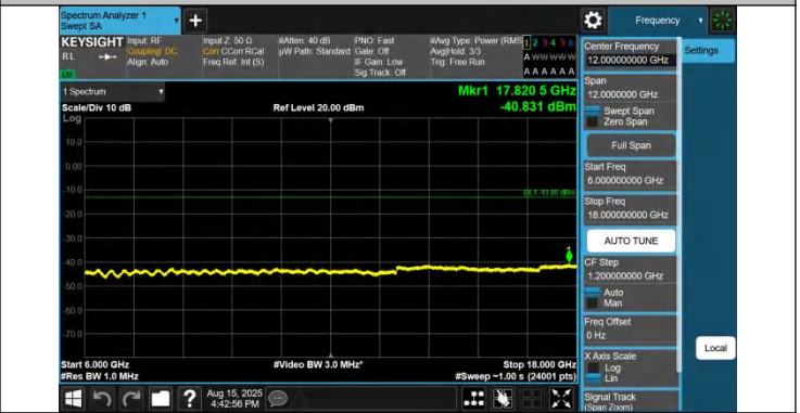
42-42-10MHz-20MHz-QPSK-QPSK-42496-42640-1RB#0-0RB#0-6000~18000MHz-PASS
