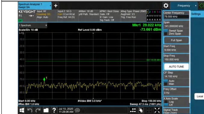
42-42-20MHz-20MHz-QPSK-QPSK-42792-42990-1RB#0-0RB#0-0.009~0.15MHz-PASS
