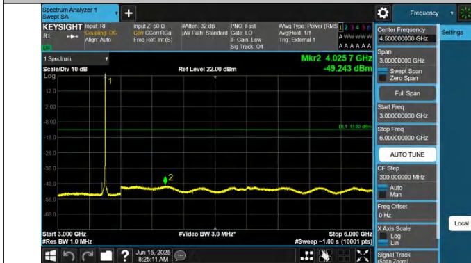
42-42-20MHz-10MHz-QPSK-QPSK-42190-42334-1RB#0-0RB#0-3000~6000MHz-PASS
