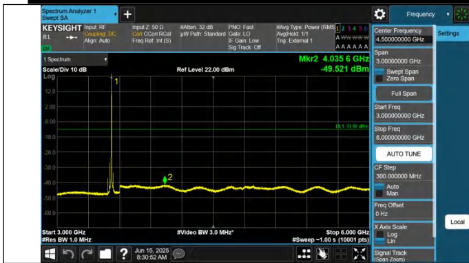
42-42-20MHz-10MHz-QPSK-QPSK-42891-43035-1RB#0-0RB#0-3000~6000MHz-PASS
