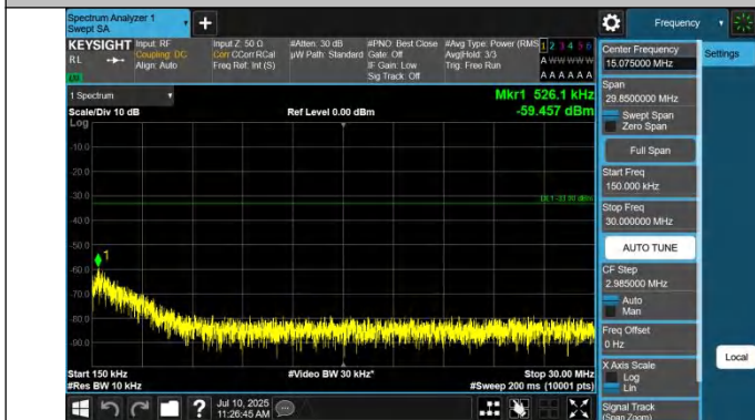
42-42-10MHz-20MHz-QPSK-QPSK-42846-42990-1RB#0-0RB#0-0.15~30MHz-PASS
