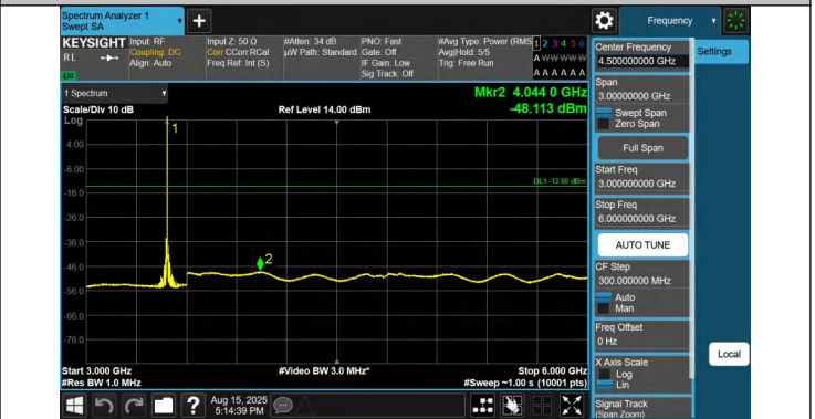
42-42-20MHz-15MHz-QPSK-QPSK-42190-42361-1RB#0-0RB#0-3000~6000MHz-PASS
