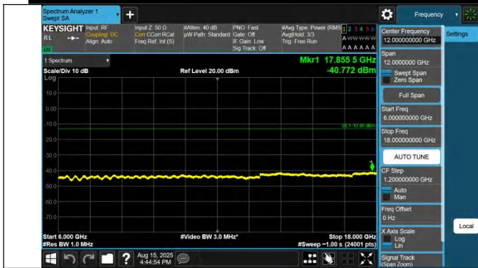
42-42-15MHz-20MHz-QPSK-QPSK-42493-42664-1RB#0-0RB#0-6000~18000MHz-PASS
