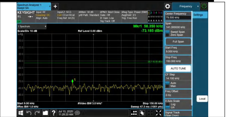
42-42-20MHz-5MHz-QPSK-QPSK-42190-42307-1RB#0-0RB#0-0.009~0.15MHz-PASS
