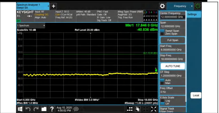
42-42-20MHz-10MHz-QPSK-QPSK-42891-43035-1RB#0-0RB#0-6000~18000MHz-PASS
