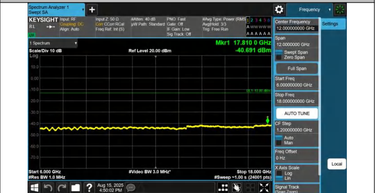
42-42-20MHz-10MHz-QPSK-QPSK-42190-42334-1RB#0-0RB#0-6000~18000MHz-PASS
