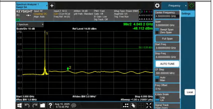
42-42-20MHz-15MHz-QPSK-QPSK-42841-43012-1RB#0-0RB#0-3000~6000MHz-PASS
