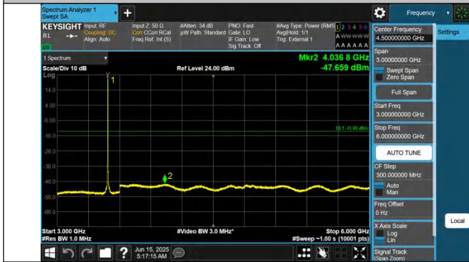
42-42-10MHz-20MHz-QPSK-QPSK-42496-42640-1RB#0-0RB#0-3000~6000MHz-PASS
