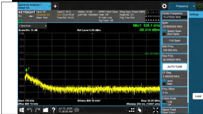
42-42-20MHz-5MHz-QPSK-QPSK-42940-43057-1RB#0-0RB#0-0 0.15~30MHz-PASS
