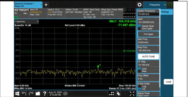
42-42-20MHz-15MHz-QPSK-QPSK-42841-43012-1RB#0-0RB#0-0.009~0.15MHz-PASS
