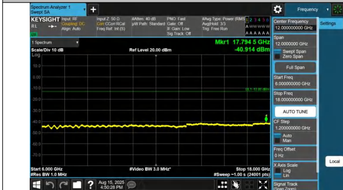
42-42-20MHz-10MHz-QPSK-QPSK-42541-42685-1RB#0-0RB#0-6000~18000MHz-PASS
