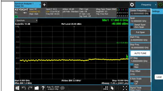
42-42-20MHz-5MHz-QPSK-QPSK-42940-43057-1RB#0-0RB#0-6 000~18000MHz-PASS
