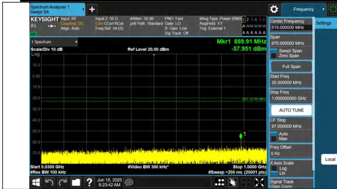
42-42-20MHz-10MHz-QPSK-QPSK-42190-42334-1RB#0-0RB#0-30~1000MHz-PASS
