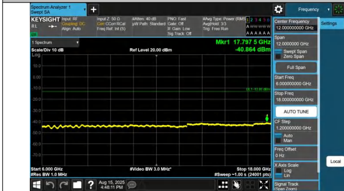
42-42-20MHz-5MHz-QPSK-QPSK-42190-42307-1RB#0-0RB#0-6000~18000MHz-PASS
