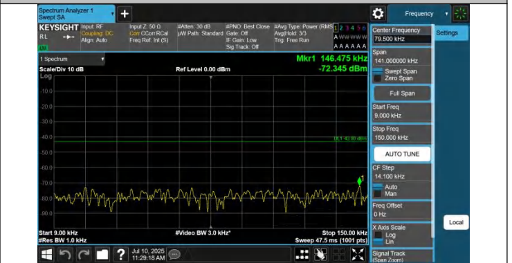
42-42-20MHz-10MHz-QPSK-QPSK-42541-42685-1RB#0-0RB#0-0.009~0.15MHz-PASS
