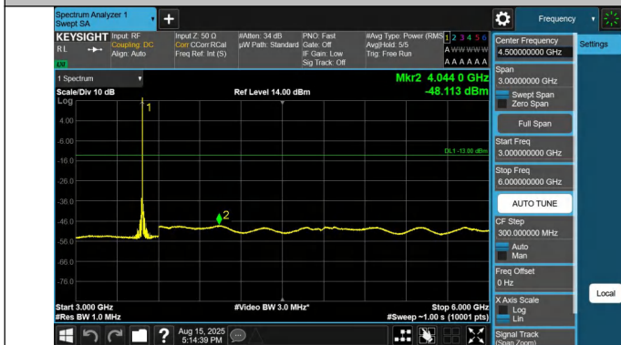
42-42-20MHz-15MHz-QPSK-QPSK-42516-42687-1RB#0-0RB#0-3000~6000MHz-PASS
