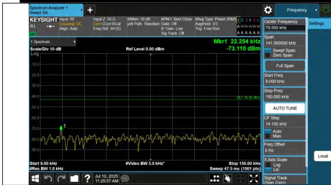
42-42-5MHz-20MHz-QPSK-QPSK-42873-42990-1RB#0-0RB#0-0 .009~0.15MHz-PASS
