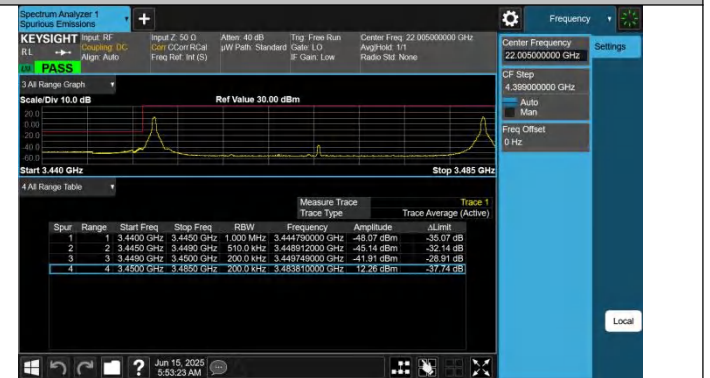
42-42-15MHz-20MHz-QPSK@QPSK-QPSK@QPSK-42168-42339 -1RB#0@75RB#0-1RB#99@100RB#0-PASS
