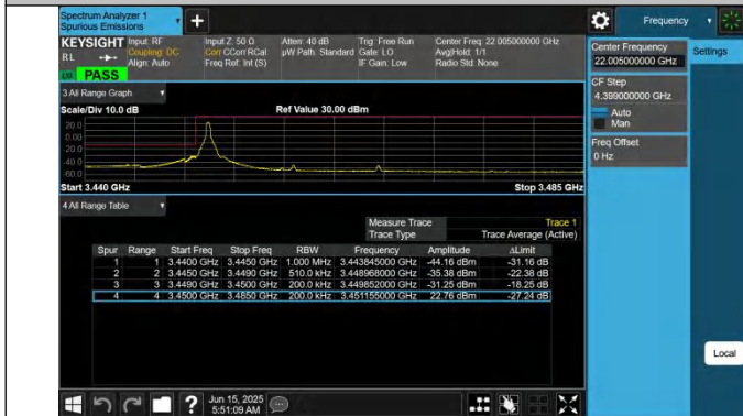
42-42-15MHz-20MHz-QPSK@QPSK-QPSK@QPSK-42168-423 39-1RB#0@75RB#0-0RB#0@100RB#0-PASS
