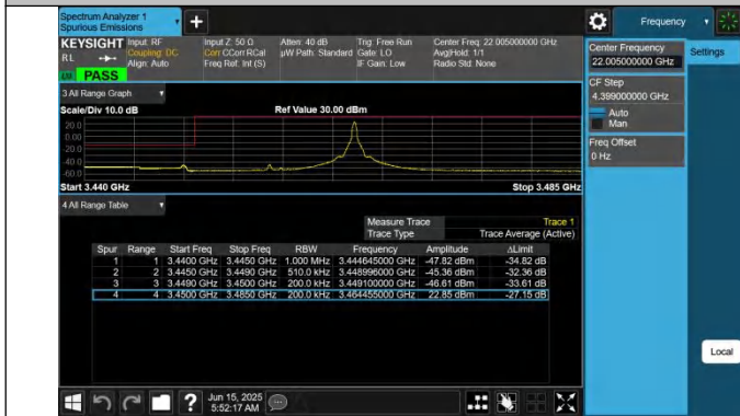
42-42-15MHz-20MHz-QPSK@QPSK-QPSK@QPSK-42168-423 39-1RB#74@75RB#0-0RB#0@100RB#0-PASS
