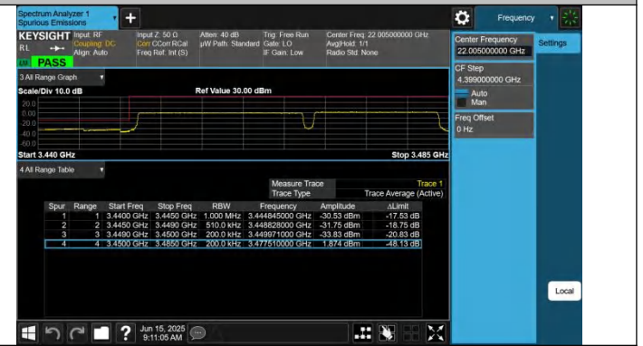
42-42-20MHz-15MHz-QPSK@QPSK-QPSK@QPSK-42190-42361 -100RB#0@100RB#0-75RB#0@75RB#0-PASS
