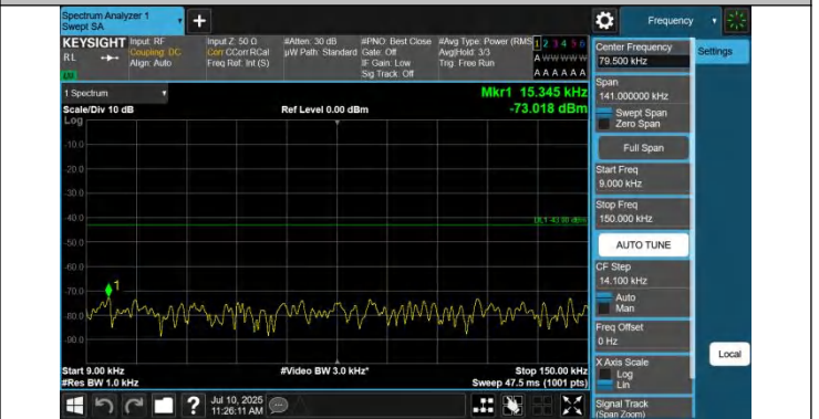
42-42-10MHz-20MHz-QPSK-QPSK-42145-42289-1RB#0-0RB#0-0 0.009~0.15MHz-PASS
