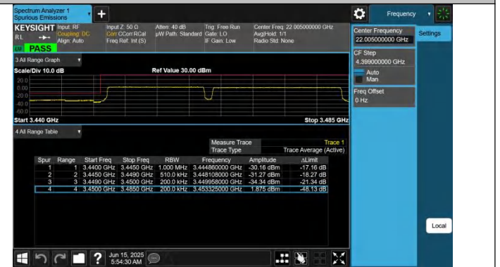
42-42-15MHz-20MHz-QPSK@QPSK-QPSK@QPSK-42168-42339 -75RB#0@75RB#0-100RB#0@100RB#0-PASS
