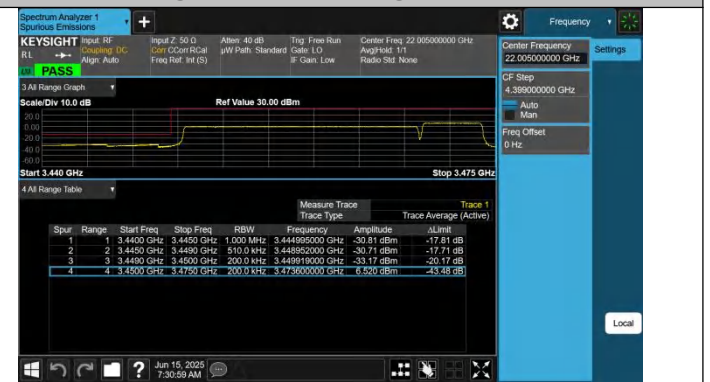
42-42-20MHz-5MHz-QPSK@QPSK-QPSK@QPSK-42190-42307- 100RB#0@100RB#0-25RB#0@25RB#0-PASS
