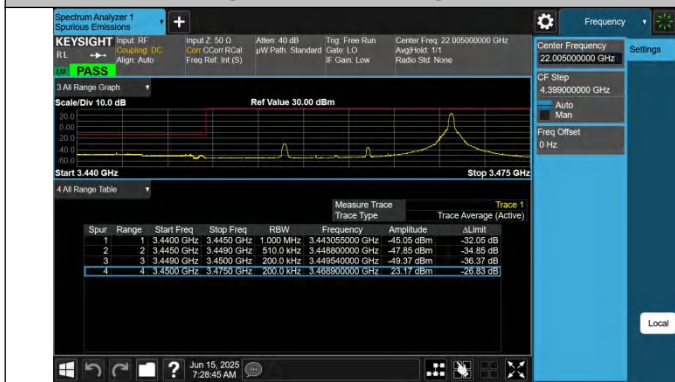
42-42-20MHz-5MHz-QPSK@QPSK-QPSK@QPSK-42190-4230 7-1RB#99@100RB#0-0RB#0@25RB#0-PASS
