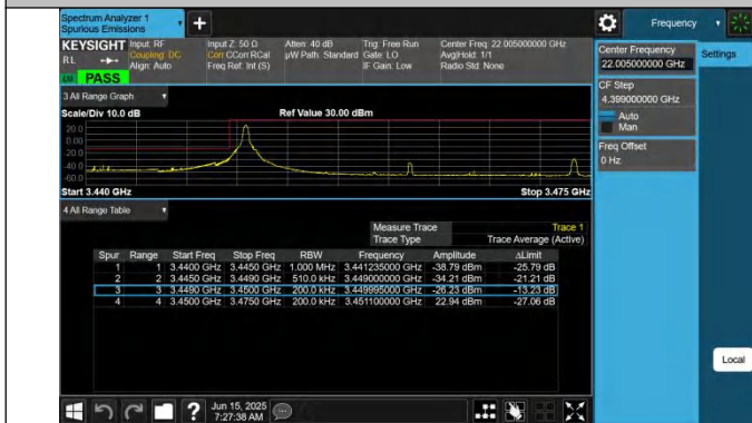
42-42-20MHz-5MHz-QPSK@QPSK-QPSK@QPSK-42190-4230 7-1RB#0@100RB#0-0RB#0@25RB#0-PASS
