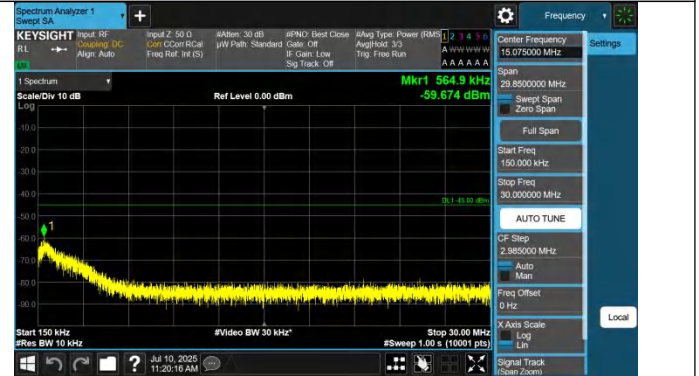
41-41-15MHz-10MHz-QPSK-QPSK-41417-41537-1RB#0-0RB#0- 0.15~30MHz-PASS
