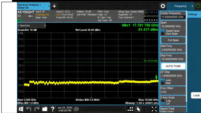
41-41-10MHz-15MHz-QPSK-QPSK-39703-39823-1RB#0-0RB#0 -3000~18000MHz-PASS
