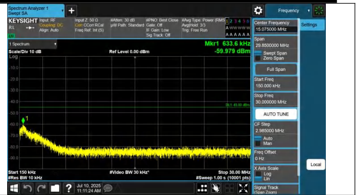
41-41-10MHz-15MHz-QPSK-QPSK-41395-41515-1RB#0-0RB#0- 0.15~30MHz-PASS
