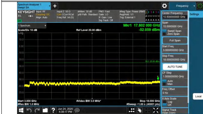
41-41-5MHz-20MHz-QPSK-QPSK-40528-40645-1RB#0-0RB#0-3000~18000MHz-PASS
