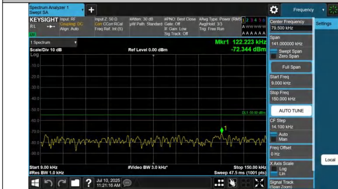
41-15MHz-20MHz-QPSK-QPSK-39728-39899-1RB#0-0RB#0 -0.009~0.15MHz-PASS
