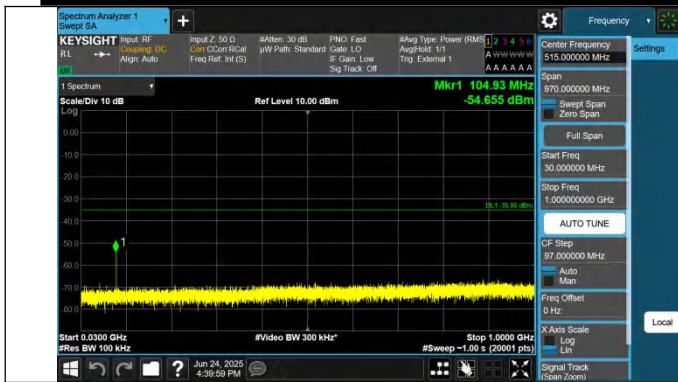
41-41-5MHz-20MHz-QPSK-QPSK-41373-41490-1RB#0-0RB#0-30~1000MHz-PASS
