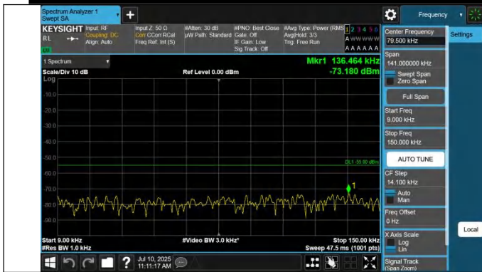
41-41-10MHz-15MHz-QPSK-QPSK-41395-41515-1RB#0-0RB#0 -0.009~0.15MHz-PASS
