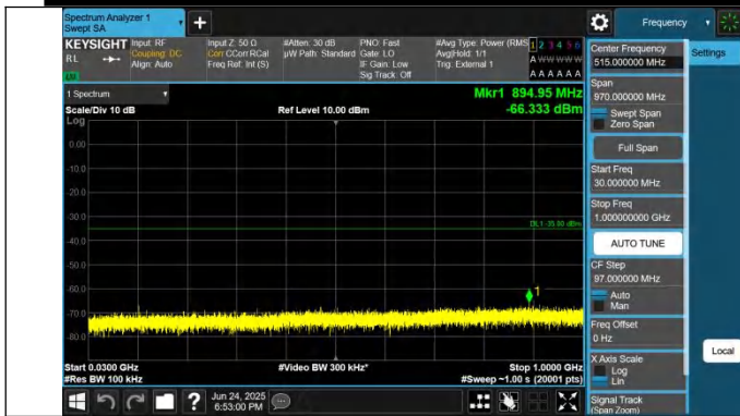
41-41-20MHz-5MHz-QPSK-QPSK-39750-39867-1RB#0-0RB#0-30~1000MHz-PASS
