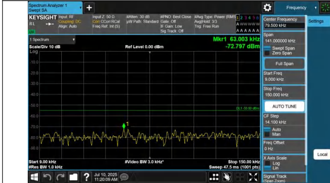
41-41-15MHz-10MHz-QPSK-QPSK-41417-41537-1RB#0-0RB#0 -0.009~0.15MHz-PASS
