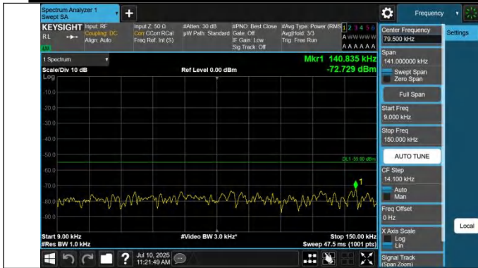
41-41-15MHz-20MHz-QPSK-QPSK-41319-41490-1RB#0-0RB#0 -0.009~0.15MHz-PASS
