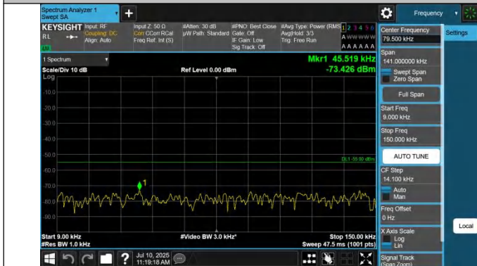
41-41-10MHz-20MHz-QPSK-QPSK-41346-41490-1RB#0-0RB#0 -0.009~0.15MHz-PASS
