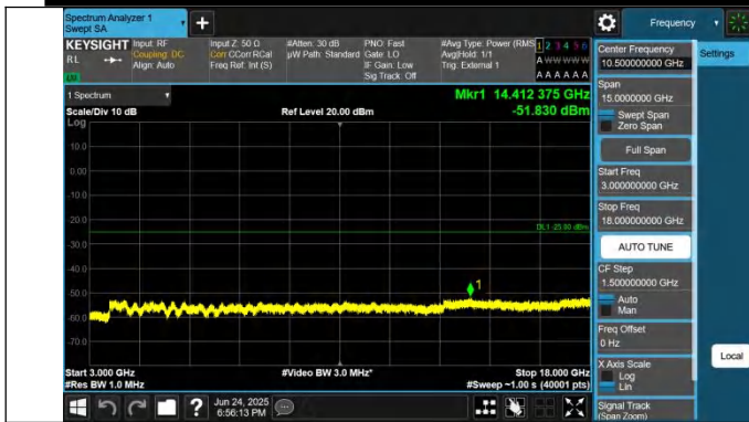
41-41-20MHz-5MHz-QPSK-QPSK-40595-40712-1RB#0-0RB#0-3000~18000MHz-PASS
