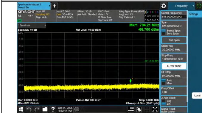
41-41-15MHz-20MHz-QPSK-QPSK-40523-40694-1RB#0-0RB#0 -30~1000MHz-PASS
