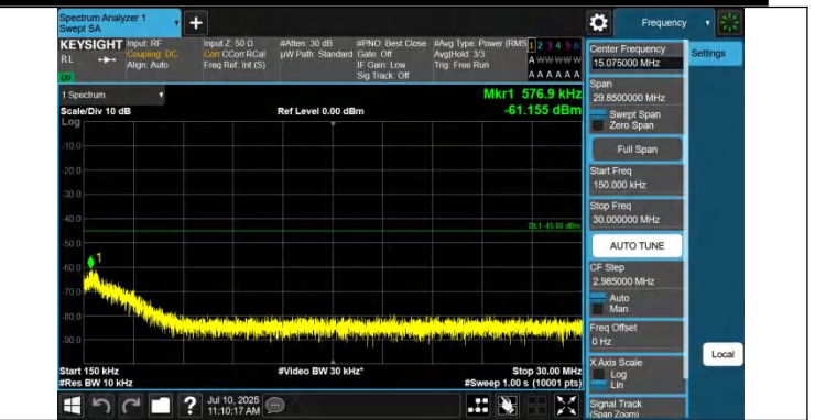
41-41-5MHz-20MHz-QPSK-QPSK-40528-40645-1RB#0-0RB#0-0.15~30MHz-PASS
