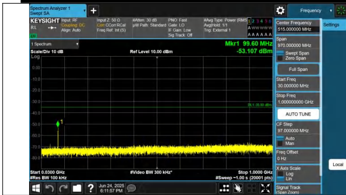
41-15MHz-15MHz-QPSK-QPSK-41365-41515-1RB#0-0RB#0 -30~1000MHz-PASS
