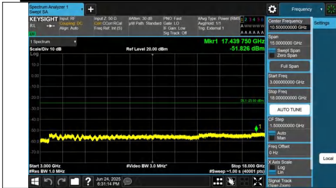
41-41-15MHz-20MHz-QPSK-QPSK-39728-39899-1RB#0-0RB#0 -3000~18000MHz-PASS
