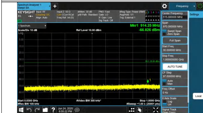
41-41-20MHz-5MHz-QPSK-QPSK-40595-40712-1RB#0-0RB#0-30~1000MHz-PASS
