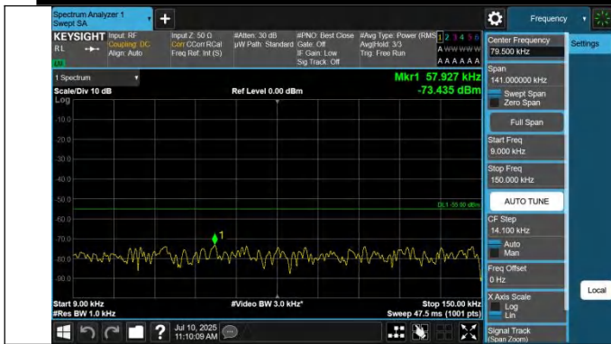
41-41-5MHz-20MHz-QPSK-QPSK-40528-40645-1RB#0-0RB#0-0.009~0.15MHz-PASS
