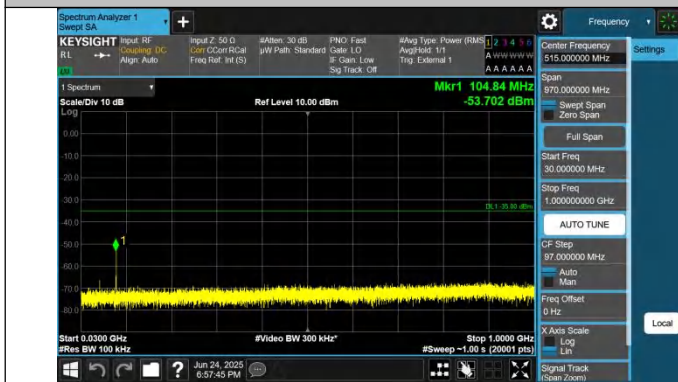
41-41-20MHz-5MHz-QPSK-QPSK-41440-41557-1RB#0-0RB#0-30~1000MHz-PASS
