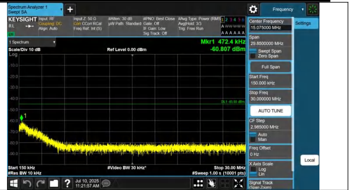
41-41-15MHz-20MHz-QPSK-QPSK-41319-41490-1RB#0-0RB#0- 0.15~30MHz-PASS
