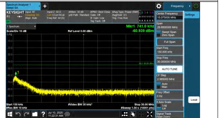
41-41-20MHz-5MHz-QPSK-QPSK-40595-40712-1RB#0-0RB#0-0.15~30MHz-PASS
