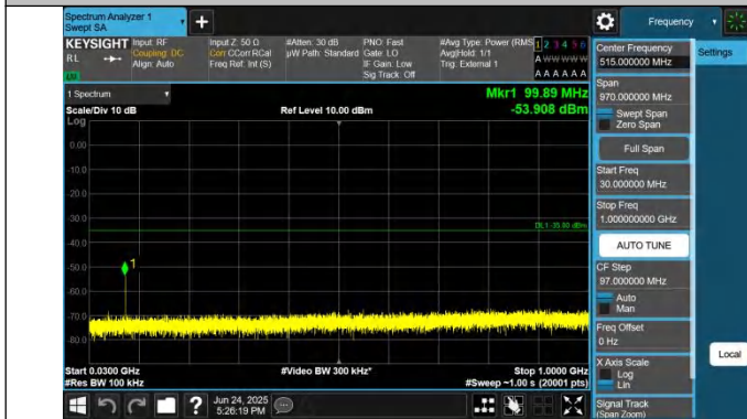
41-41-10MHz-20MHz-QPSK-QPSK-41346-41490-1RB#0-0RB#0 -30~1000MHz-PASS
