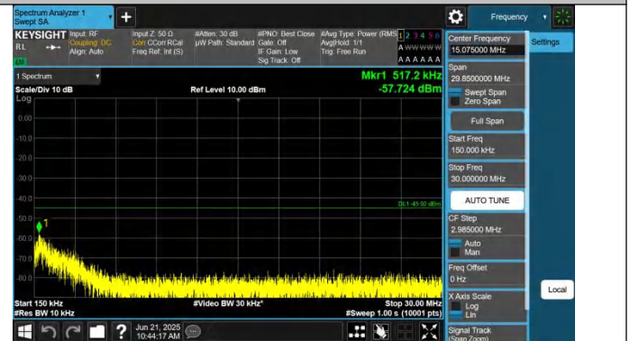
7-7-20MHz-10MHz-QPSK-QPSK-20850-20994-1RB#0-0RB#0-0.1 5~30MHz-PASS
