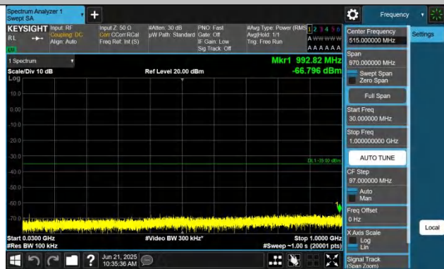
7-7-15MHz-20MHz-QPSK-QPSK-21179-21350-1RB#0-0RB#0-30 ~1000MHz-PASS
