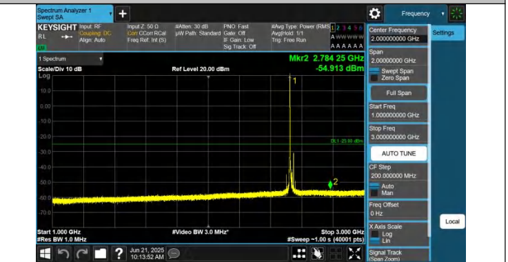
7-7-15MHz-10MHz-QPSK-QPSK-21051-21171-1RB#0-0RB#0-10 00~3000MHz-PASS
