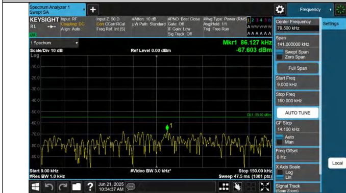
7-7-15MHz-20MHz-QPSK-QPSK-21003-21174-1RB#0-0RB#0-0. 009~0.15MHz-PASS
