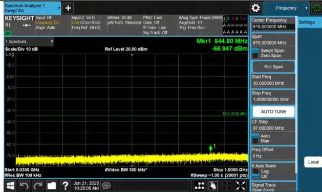
7-7-15MHz-15MHz-QPSK-QPSK-21225-21375-1RB#0-0RB#0-3 0~1000MHz-PASS
