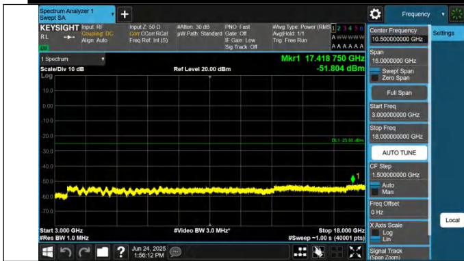
7-7-20MHz-20MHz-QPSK-QPSK-21001-21199-1RB#0-0RB#0-30 00~18000MHz-PASS
