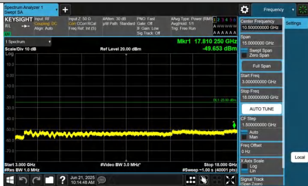
7-7-15MHz-10MHz-QPSK-QPSK-21277-21397-1RB#0-0RB#0-3 000~18000MHz-PASS
