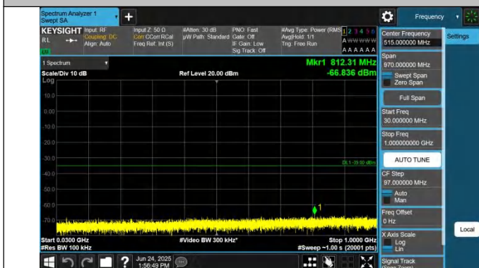
7-7-20MHz-20MHz-QPSK-QPSK-21152-21350-1RB#0-0RB#0-30 ~1000MHz-PASS
