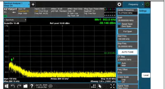
7-7-20MHz-20MHz-QPSK-QPSK-20850-21048-1RB#0-0RB#0-0.1 5~30MHz-PASS
