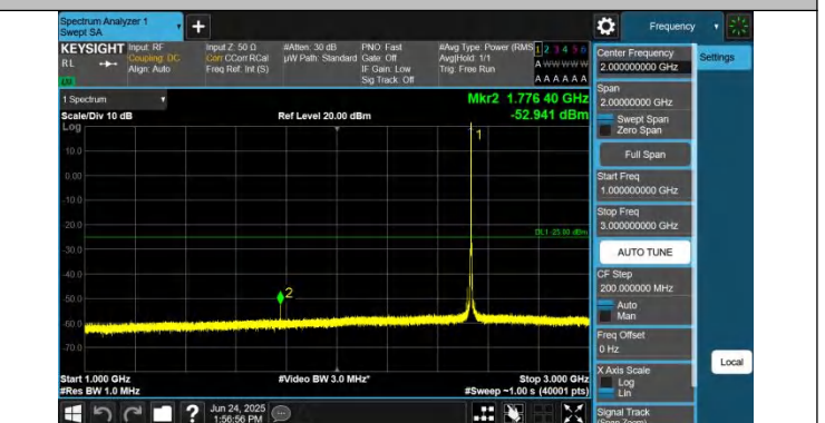
7-7-20MHz-20MHz-QPSK-QPSK-21152-21350-1RB#0-0RB#0-10 00~3000MHz-PASS
