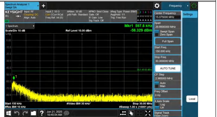
7-7-20MHz-10MHz-QPSK-QPSK-21251-21395-1RB#0-0RB#0-0.1 5~30MHz-PASS
