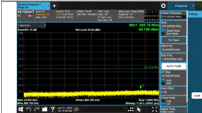
7-7-15MHz-10MHz-QPSK-QPSK-21051-21171-1RB#0-0RB#0-30 ~1000MHz-PASS
