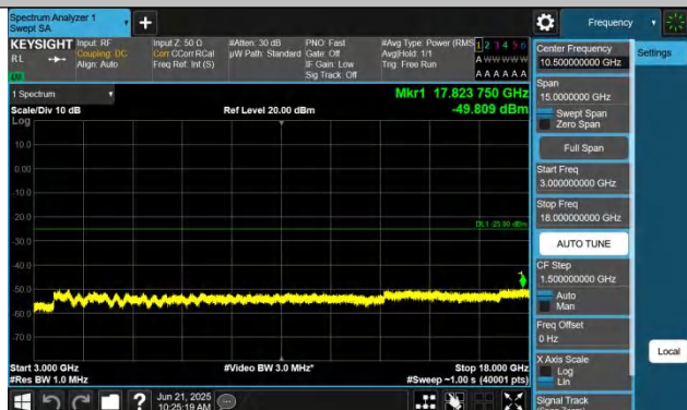
7-7-15MHz-15MHz-QPSK-QPSK-21225-21375-1RB#0-0RB#0-3 000~18000MHz-PASS
