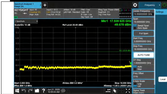
7-7-20MHz-15MHz-QPSK-QPSK-20850-21021-1RB#0-0RB#0-3 000~18000MHz-PASS
