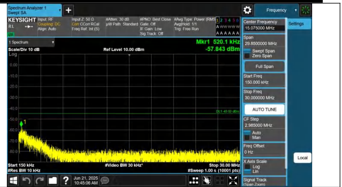
7-7-20MHz-10MHz-QPSK-QPSK-21051-21195-1RB#0-0RB#0-0.1 5~30MHz-PASS
