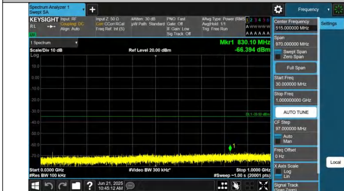
7-7-20MHz-10MHz-QPSK-QPSK-21051-21195-1RB#0-0RB#0-30 ~1000MHz-PASS
