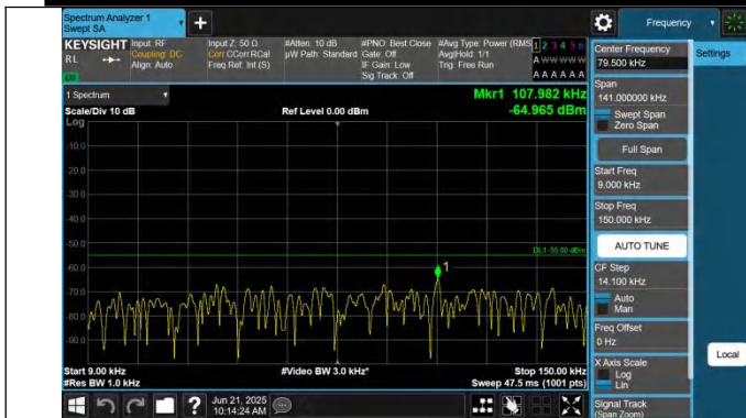
7-7-15MHz-10MHz-QPSK-QPSK-21277-21397-1RB#0-0RB#0-0. 009~0.15MHz-PASS
