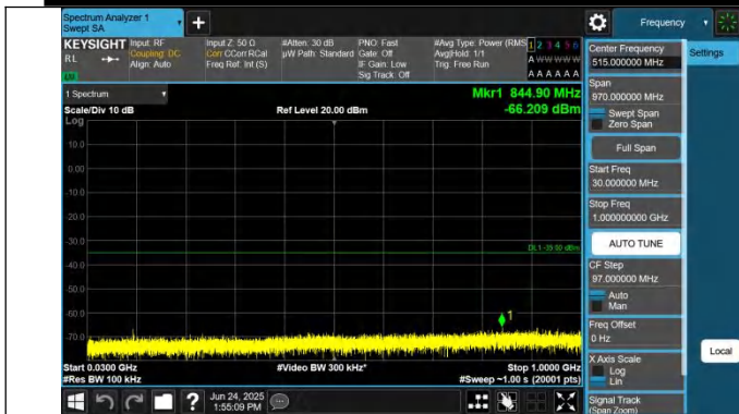
7-7-20MHz-20MHz-QPSK-QPSK-20850-21048-1RB#0-0RB#0-3 0~1000MHz-PASS
