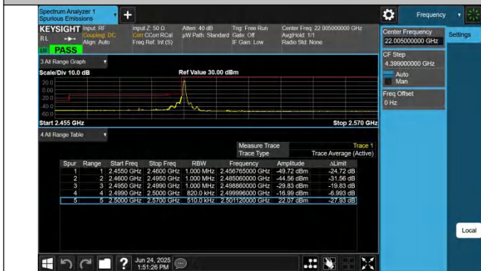
7-7-20MHz-20MHz-QPSK@QPSK-QPSK@QPSK-20850-21048-1RB#0@100RB#0-0RB#0@100RB#0-PASS
