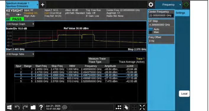
7-7-20MHz-10MHz-QPSK@QPSK-QPSK@QPSK-20850-20994-100RB#0@100RB#0-50RB#0@50RB#0-PASS
