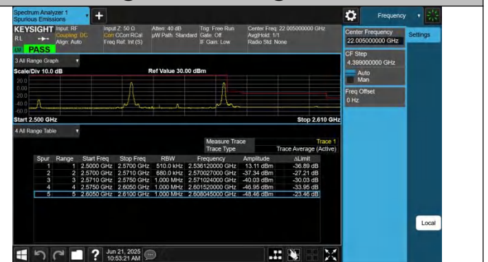
7-7-20MHz-15MHz-QPSK@QPSK-QPSK@QPSK-21201-21372-1RB#0@100RB#0-1RB#74@75RB#0-PASS
