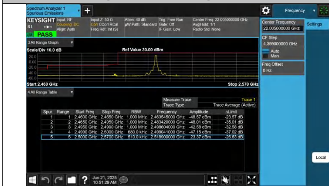
7-7-20MHz-15MHz-QPSK@QPSK-QPSK@QPSK-20850-21021-1RB#99@100RB#0-0RB#0@75RB#0-PASS
