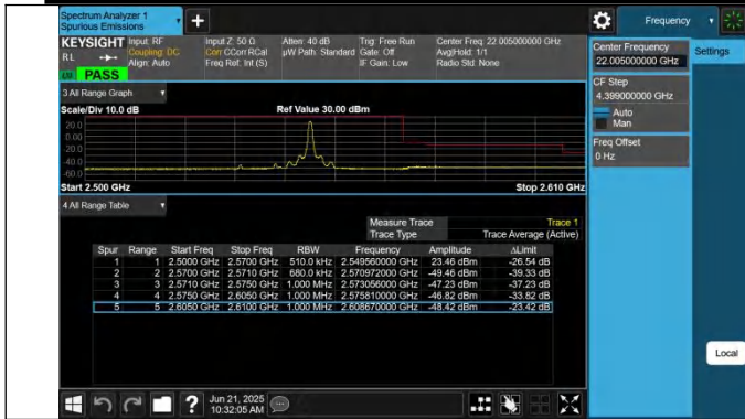
7-7-15MHz-20MHz-QPSK@QPSK-QPSK@QPSK-21179-21350-1RB#74@75RB#0-0RB#0@100RB#0-PASS
