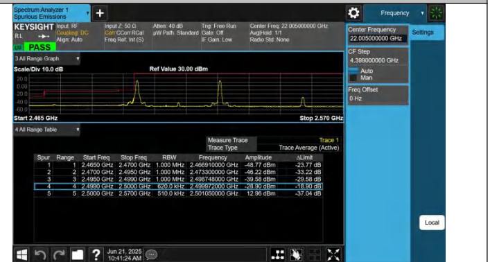
7-7-20MHz-10MHz-QPSK@QPSK-QPSK@QPSK-20850-20994-1RB#0@100RB#0-1RB#49@50RB#0-PASS
