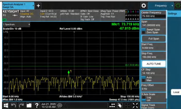
7-7-15MHz-10MHz-QPSK-QPSK-20825-20945-1RB#0-0RB#0-0. 009~0.15MHz-PASS
