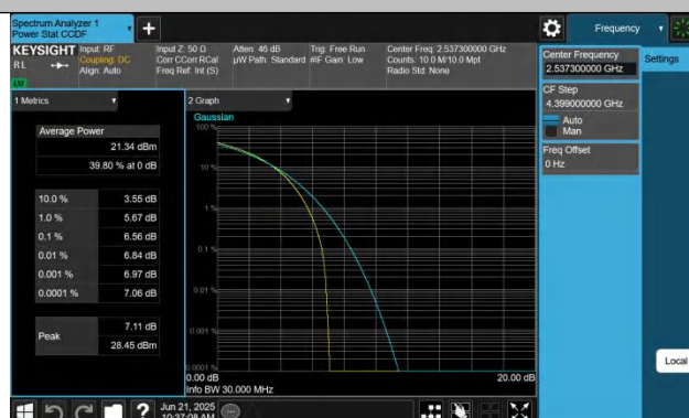
7-7-20MHz-10MHz-16QAM-16QAM-21051-21195-100RB#0-50R
