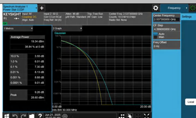
7-7-20MHz-10MHz-256QAM-256QAM-21051-21195-100RB#0-50
