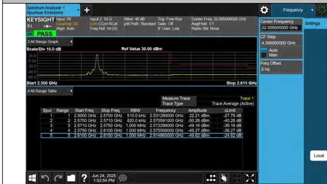
7-7-20MHz-20MHz-QPSK@QPSK-QPSK@QPSK-21152-21350-1RB#0@100RB#0-0RB#0@100RB#0-PASS
