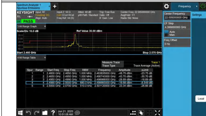
7-7-20MHz-15MHz-QPSK@QPSK-QPSK@QPSK-20850-21021-1RB#0@100RB#0-0RB#0@75RB#0-PASS
