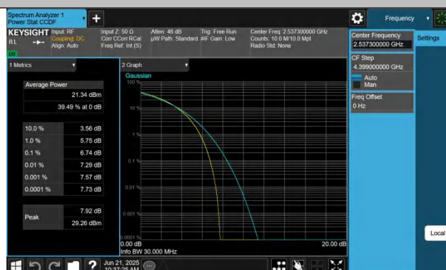
7-7-20MHz-10MHz-64QAM-64QAM-21051-21195-100RB#0-50R
