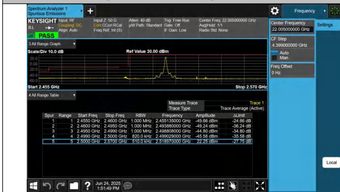
7-7-20MHz-20MHz-QPSK@QPSK-QPSK@QPSK-20850-21048-1RB#99@100RB#0-0RB#0@100RB#0-PASS
