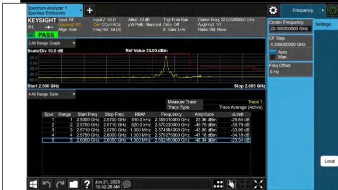
7-7-20MHz-10MHz-QPSK@QPSK-QPSK@QPSK-21251-21395-1RB#99@100RB#0-0RB#0@50RB#0-PASS
