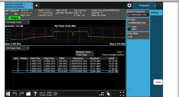
7-7-20MHz-15MHz-QPSK@QPSK-QPSK@QPSK-20850-21021-100RB#0@100RB#0-75RB#0@75RB#0-PASS
