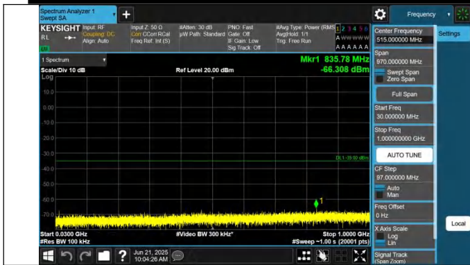
7-7-10MHz-20MHz-QPSK-QPSK-21206-21350-1RB#0-0RB#0-3 0~1000MHz-PASS
