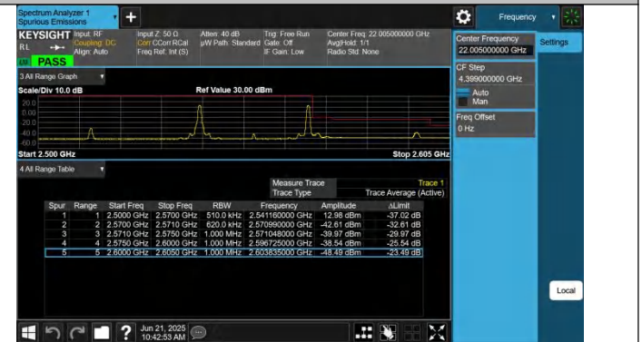
7-7-20MHz-10MHz-QPSK@QPSK-QPSK@QPSK-21251-21395-1RB#0@100RB#0-1RB#49@50RB#0-PASS
