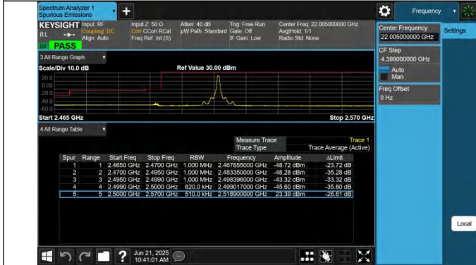
7-7-20MHz-10MHz-QPSK@QPSK-QPSK@QPSK-20850-20994-1RB#99@100RB#0-0RB#0@50RB#0-PASS
