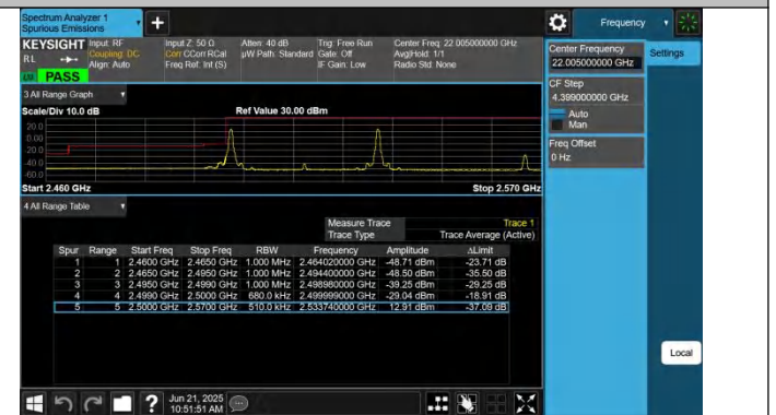
7-7-20MHz-15MHz-QPSK@QPSK-QPSK@QPSK-20850-21021-1RB#0@100RB#0-1RB#74@75RB#0-PASS
