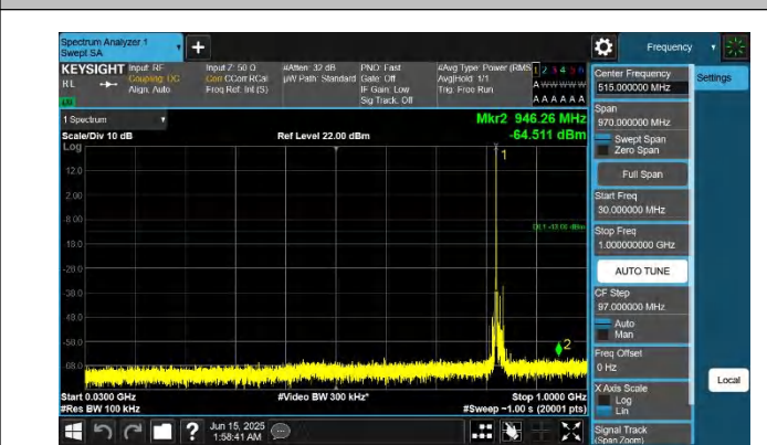
5-5-10MHz-5MHz-QPSK-QPSK-20450-20522-1RB#0-ORB#0-30~ 1000MHz-PASS
