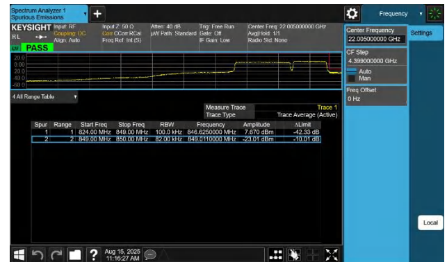
5-5-5MHz-3MHz-QPSK@QPSK-QPSK@QPSK-20595-20634-25 RB#0@25RB#0-15RB#0@15RB#0-PASS
