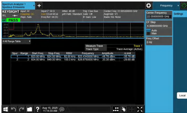
5-5-5MHz-3MHz-QPSK@QPSK-QPSK@QPSK-20425-20464-1R B#24@25RB#0-0RB#0@15RB#0-PASS
