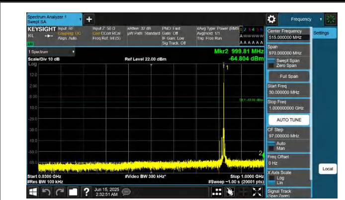
5-5-10MHz-10MHz-QPSK-QPSK-20476-20575-1RB#0-ORB#0-30 ~1000MHz-PASS
