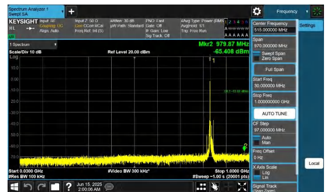
5-5-10MHz-5MHz-QPSK-QPSK-20550-20622-1RB#0-0RB#0-30~ 1000MHz-PASS
