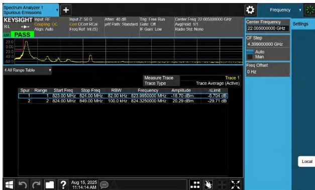
5-5-5MHz-3MHz-QPSK@QPSK-QPSK@QPSK-20425-20464-1R B#0@25RB#0-0RB#0@15RB#0-PASS
