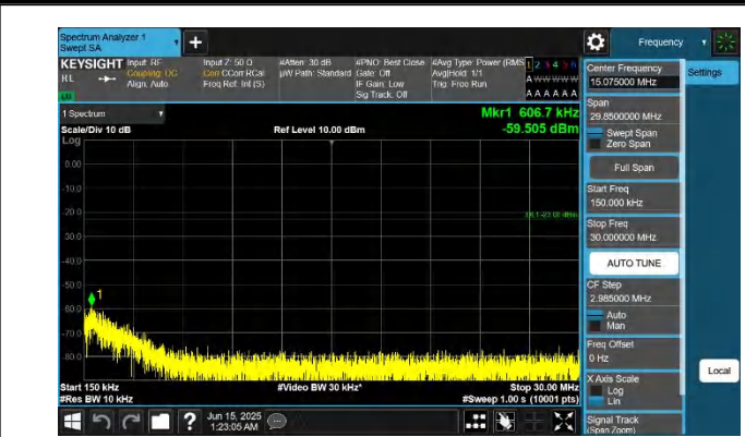
5-5-5MHz-10MHz-QPSK-QPSK-20428-20500-1RB#0-ORB#0-0.1 5~30MHz-PASS
