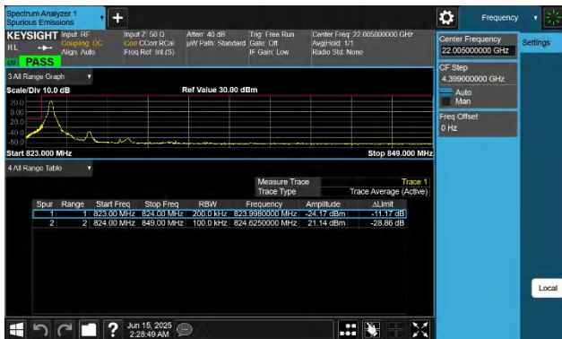
5-5-10MHz-10MHz-QPSK@QPSK-QPSK@QPSK-20450-20549-1 1RB#0@50RB#0-0RB#0@50RB#0-PASS
