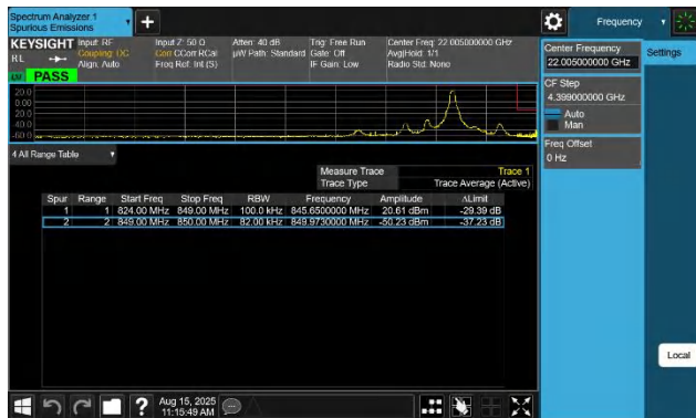
5-5-5MHz-3MHz-QPSK@QPSK-QPSK@QPSK-20595-20634-1R B#24@25RB#0-0RB#0@15RB#0-PASS
