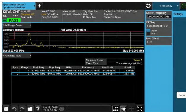
5-5-3MHz-5MHz-QPSK@QPSK-QPSK@QPSK-20416-20455-1R B#14@15RB#0-0RB#0@25RB#0-PASS
