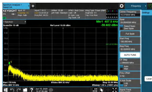
5-5-5MHz-3MHz-QPSK-QPSK-20510-20549-1RB#0-0RB#0-0.15 ~30MHz-PASS
