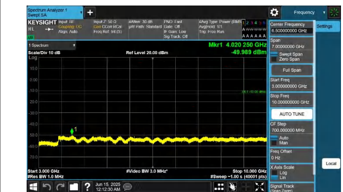
5-5-3MHz-5MHz-QPSK-QPSK-20501-20540-1RB#0-0RB#0-3000 ~10000MHz-PASS
