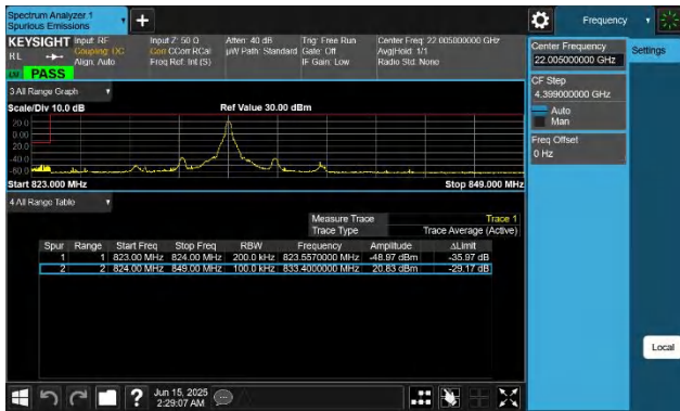
5-5-10MHz-10MHz-QPSK@QPSK-QPSK@QPSK-20450-20549-1 1RB#49@50RB#0-0RB#0@50RB#0-PASS
