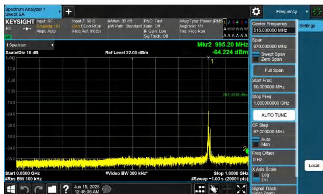
5-5-5MHz-3MHz-QPSK-QPSK-20510-20549-1RB#0-0RB#0-30~1 000MHz-PASS
