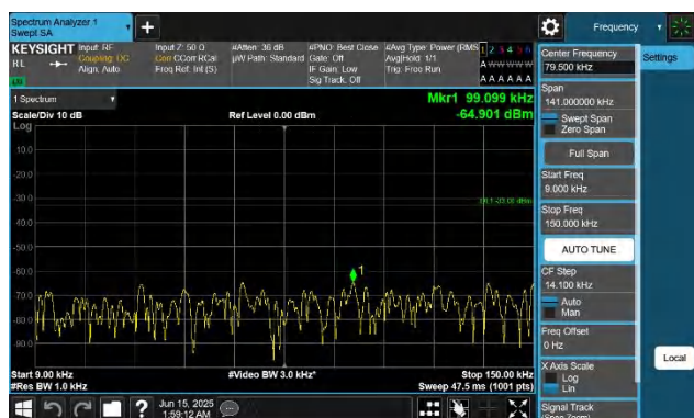
5-5-10MHz-5MHz-QPSK-QPSK-20500-20572-1RB#0-0RB#0-0.0 09~0.15MHz-PASS
