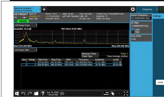
5-5-10MHz-5MHz-QPSK@QPSK-QPSK@QPSK-20450-20522-1 RB#0@50RB#0-0RB#0@25RB#0-PASS
