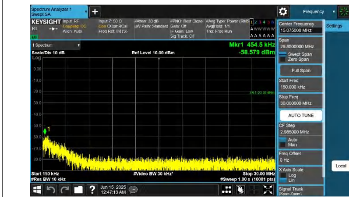
5-5-5MHz-3MHz-QPSK-QPSK-20425-20464-1RB#0-ORB#0-0.15 ~30MHz-PASS
