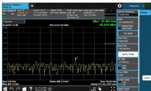
5-5-5MHz-3MHz-QPSK-QPSK-20510-20549-1RB#0-0RB#0-0.00 9~0.15MHz-PASS
