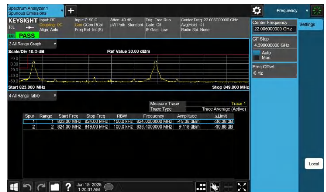
5-5-5MHz-10MHz-QPSK@QPSK-QPSK@QPSK-20428-20500-1 RB#0@25RB#0-1RB#49@50RB#0-PASS
