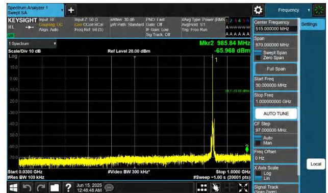
5-5-5MHz-3MHz-QPSK-QPSK-20595-20634-1RB#0-ORB#0-30~1 000MHz-PASS
