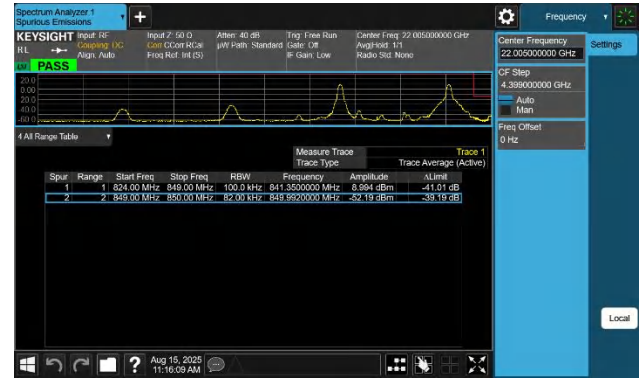
5-5-5MHz-3MHz-QPSK@QPSK-QPSK@QPSK-20595-20634-1R B#0@25RB#0-1RB#15@15RB#0-PASS
