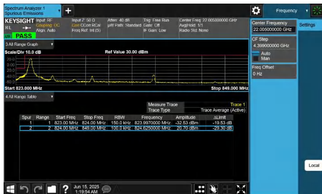
5-5-5MHz-10MHz-QPSK@QPSK-QPSK@QPSK-20428-20500-1 RB#0@25RB#0-0RB#0@50RB#0-PASS
