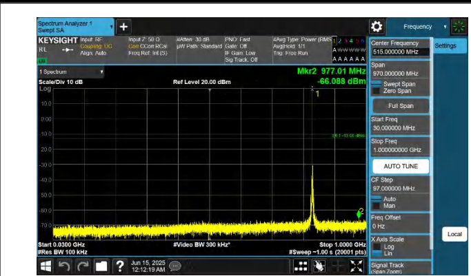
5-5-3MHz-5MHz-QPSK-QPSK-20501-20540-1RB#0-0RB#0-30~1 000MHz-PASS
