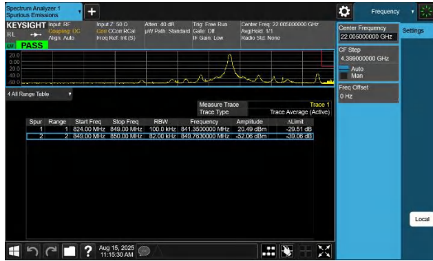
5-5-5MHz-3MHz-QPSK@QPSK-QPSK@QPSK-20595-20634-1R B#0@25RB#0-0RB#0@15RB#0-PASS
