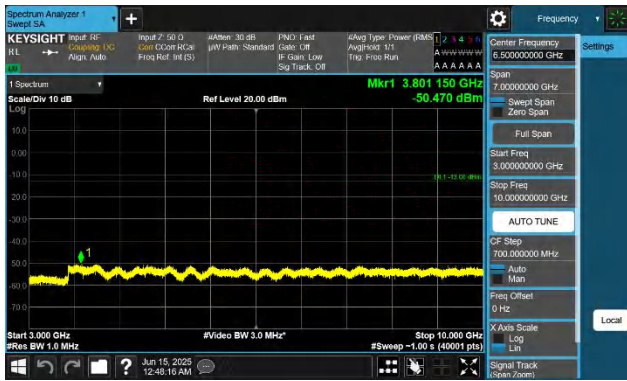
5-5-5MHz-3MHz-QPSK-QPSK-20510-20549-1RB#0-ORB#0-3000 ~10000MHz-PASS
