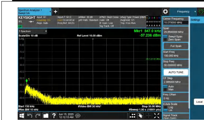
5-5-3MHz-5MHz-QPSK-QPSK-20501-20540-1RB#0-0RB#0-0.15 ~30MHz-PASS
