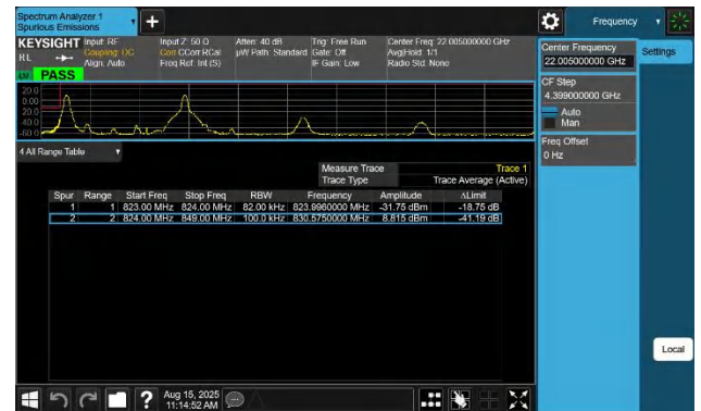
5-5-5MHz-3MHz-QPSK@QPSK-QPSK@QPSK-20425-20464-1R B#0@25RB#0-1RB#15@15RB#0-PASS
