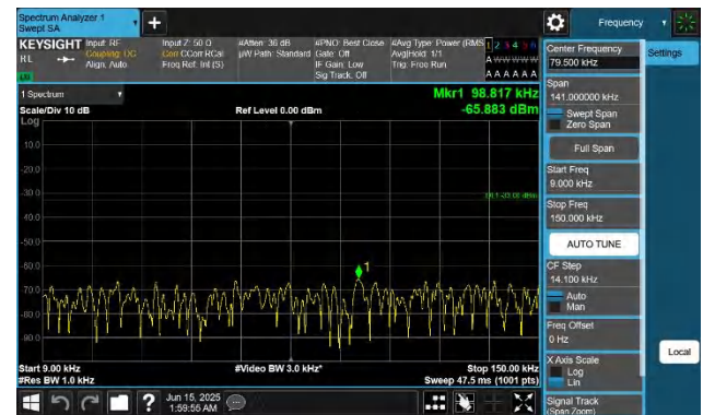
5-5-10MHz-5MHz-QPSK-QPSK-20550-20622-1RB#0-0RB#0-0.0 09~0.15MHz-PASS
