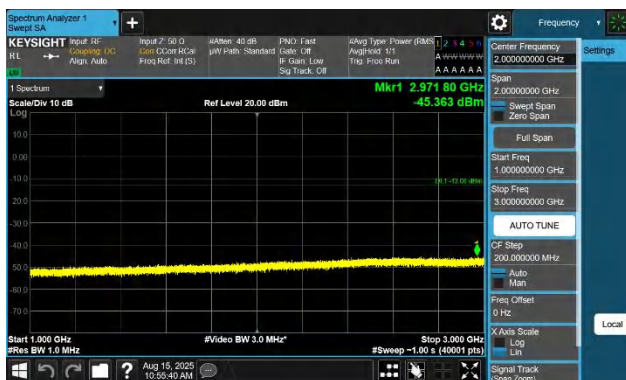
5-5-10MHz-5MHz-QPSK-QPSK-20550-20622-1RB#0-0RB#0-100 0~3000MHz-PASS
