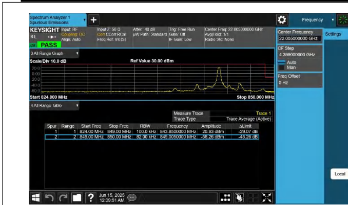
5-5-3MHz-5MHz-QPSK@QPSK-QPSK@QPSK-20586-20625-1R B#14@15RB#0-0RB#0@25RB#0-PASS
