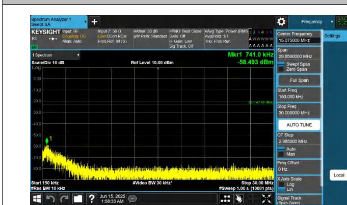
5-5-10MHz-5MHz-QPSK-QPSK-20450-20522-1RB#0-ORB#0-0.1 5~30MHz-PASS
