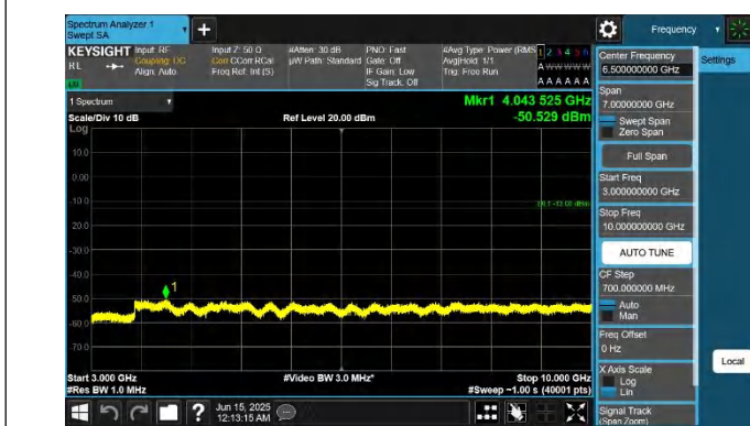
5-5-3MHz-5MHz-QPSK-QPSK-20586-20625-1RB#0-ORB#0-3000 ~10000MHz-PASS
