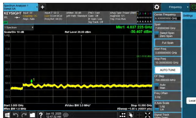
5-5-5MHz-3MHz-QPSK-QPSK-20425-20464-1RB#0-0RB#0-3000 ~10000MHz-PASS
