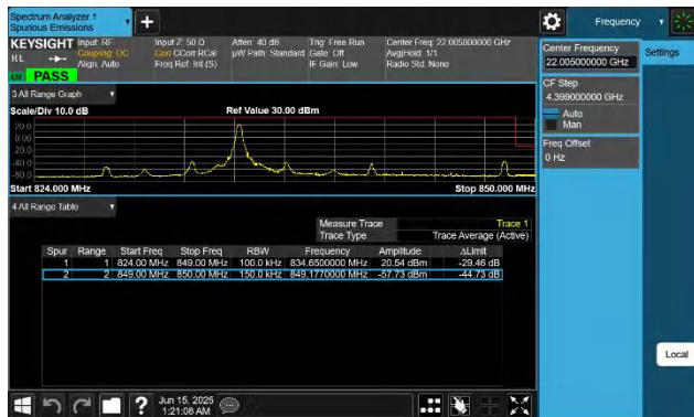
5-5-5MHz-10MHz-QPSK@QPSK-QPSK@QPSK-20528-20600-1 RB#0@25RB#0-0RB#0@50RB#0-PASS
