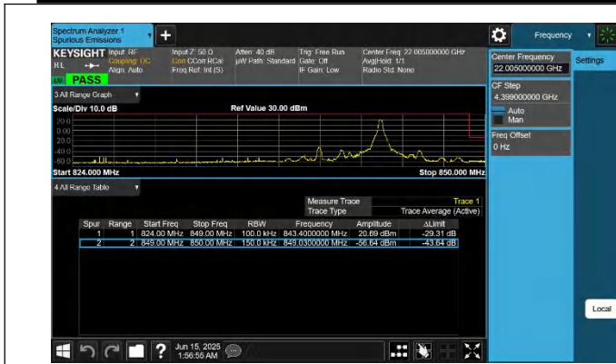
5-5-10MHz-5MHz-QPSK@QPSK-QPSK@QPSK-20550-20622-1 RB#49@50RB#0-0RB#0@25RB#0-PASS
