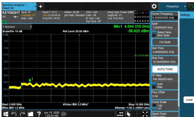
5-5-5MHz-10MHz-QPSK-QPSK-20428-20500-1RB#0-ORB#0-300 0~10000MHz-PASS
