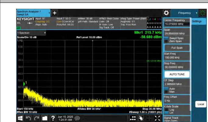
5-5-5MHz-10MHz-QPSK-QPSK-20528-20600-1RB#0-ORB#0-0.1 5~30MHz-PASS
