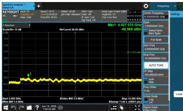
5-5-10MHz-5MHz-QPSK-QPSK-20500-20572-1RB#0-0RB#0-300 0~10000MHz-PASS
