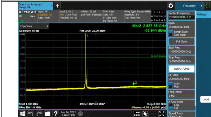
2-2-15MHz-10MHz-QPSK-QPSK-18675-18795-1RB#0-ORB#0-10 00~3000MHz-PASS
