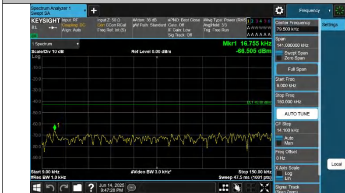
2-2-15MHz-20MHz-QPSK-QPSK-18803-18974-1RB#0-0RB#0-0. 009~0.15MHz-PASS
