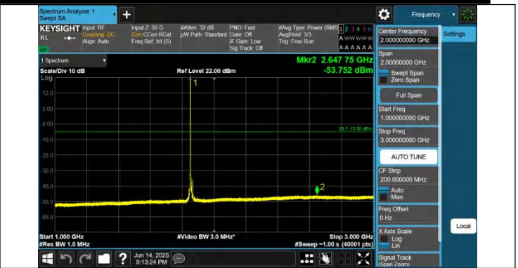
2-2-15MHz-15MHz-QPSK-QPSK-18675-18825-1RB#0-0RB#0-10 00~3000MHz-PASS
