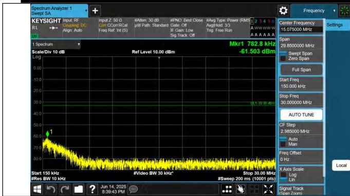
2-2-15MHz-10MHz-QPSK-QPSK-18675-18795-1RB#0-ORB#0-0. 15~30MHz-PASS
