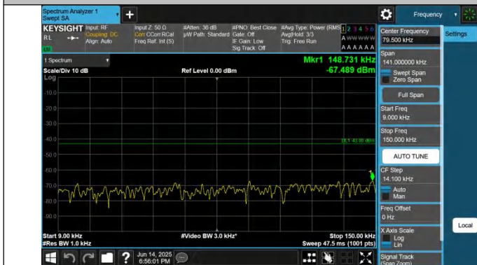
2-2-10MHz-15MHz-QPSK-QPSK-18829-18949-1RB#0-ORB#0-0. 009~0.15MHz-PASS
