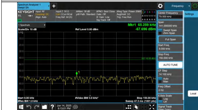
2-2-15MHz-15MHz-QPSK-QPSK-18675-18825-1RB#0-ORB#0-0. 009~0.15MHz-PASS
