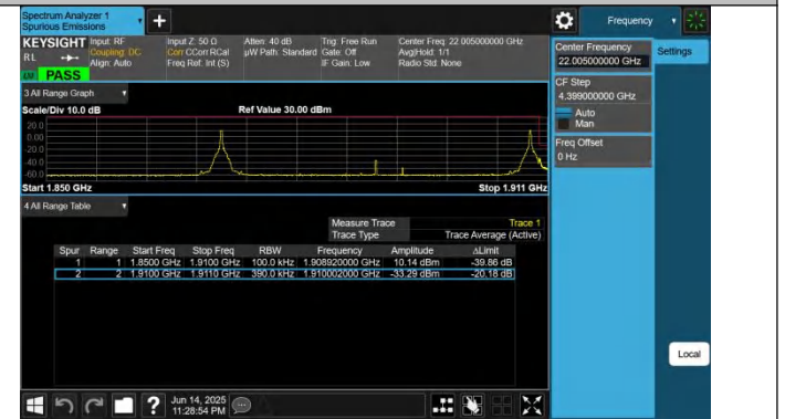
2-2-20MHz-20MHz-QPSK@QPSK-QPSK@QPSK-18902-19100-1RB#0@100RB#0-1RB#99@100RB#0-PASS
