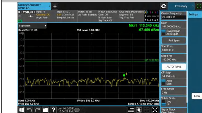
2-2-20MHz-15MHz-QPSK-QPSK-18700-18871-1RB#0-0RB#0-0. 009~0.15MHz-PASS
