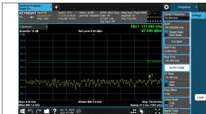
2-2-5MHz-20MHz-QPSK-QPSK-18633-18750-1RB#0-ORB#0-0.0 09~0.15MHz-PASS
