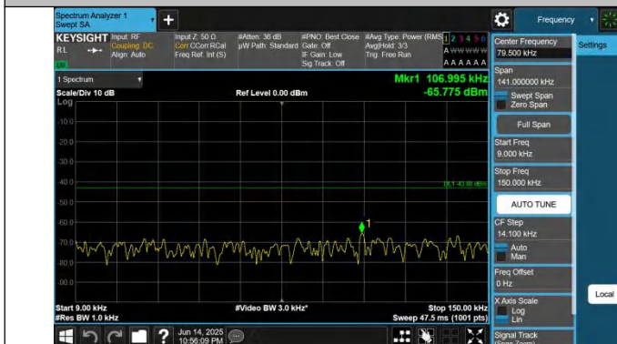
2-2-20MHz-15MHz-QPSK-QPSK-18951-19122-1RB#0-0RB#0-0. 009~0.15MHz-PASS
