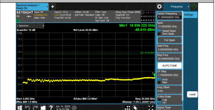
2-2-15MHz-15MHz-QPSK-QPSK-18825-18975-1RB#0-0RB#0-30 00~20000MHz-PASS
