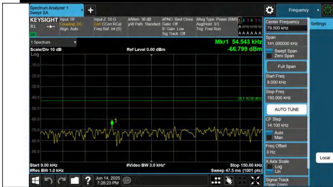
2-2-10MHz-20MHz-QPSK-QPSK-18655-18799-1RB#0-ORB#0-0. 009~0.15MHz-PASS
