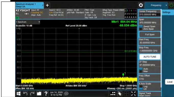
2-2-15MHz-15MHz-QPSK-QPSK-18675-18825-1RB#0-0RB#0-30 ~1000MHz-PASS
