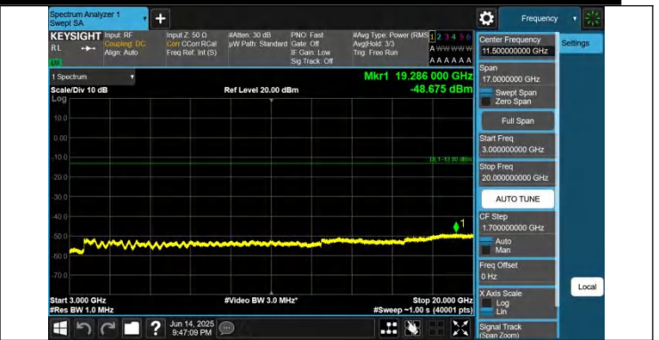
2-2-15MHz-20MHz-QPSK-QPSK-18678-18849-1RB#0-0RB#0-30 00~20000MHz-PASS
