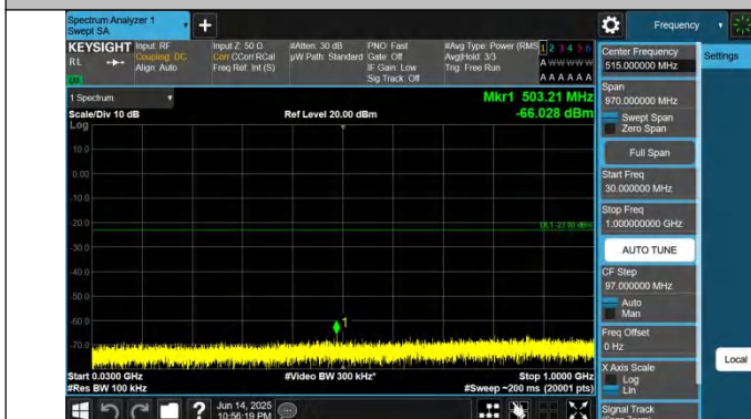
2-2-20MHz-15MHz-QPSK-QPSK-18951-19122-1RB#0-0RB#0-30 ~1000MHz-PASS
