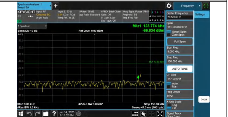
2-2-15MHz-15MHz-QPSK-QPSK-18825-18975-1RB#0-0RB#0-0. 009~0.15MHz-PASS
