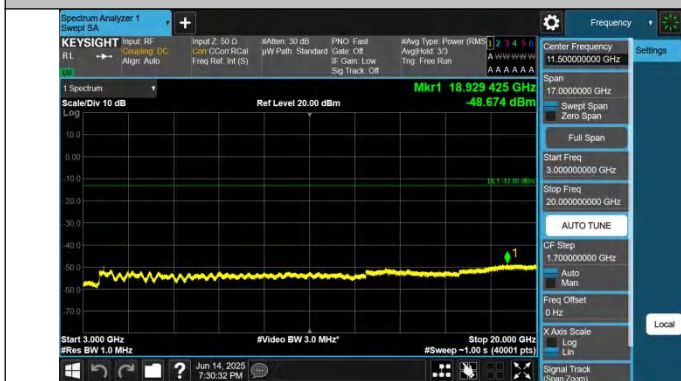
2-2-10MHz-20MHz-QPSK-QPSK-18956-19100-1RB#0-0RB#0-30 00~20000MHz-PASS
