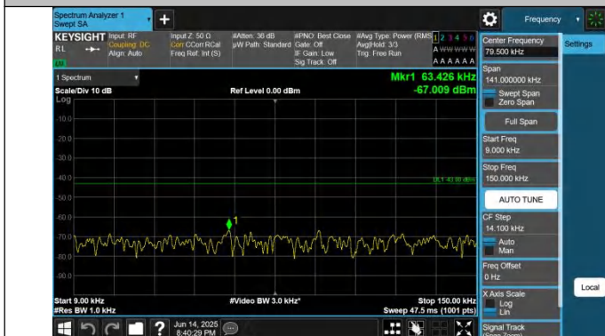
2-2-15MHz-10MHz-QPSK-QPSK-18851-18971-1RB#0-ORB#0-0. 009~0.15MHz-PASS
