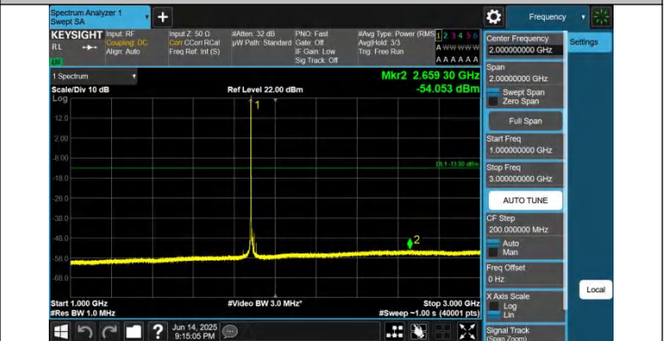
2-2-15MHz-15MHz-QPSK-QPSK-18975-19125-1RB#0-0RB#0-10 00~3000MHz-PASS
