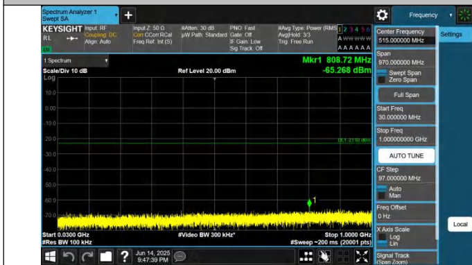
2-2-15MHz-20MHz-QPSK-QPSK-18803-18974-1RB#0-0RB#0-30 ~1000MHz-PASS
