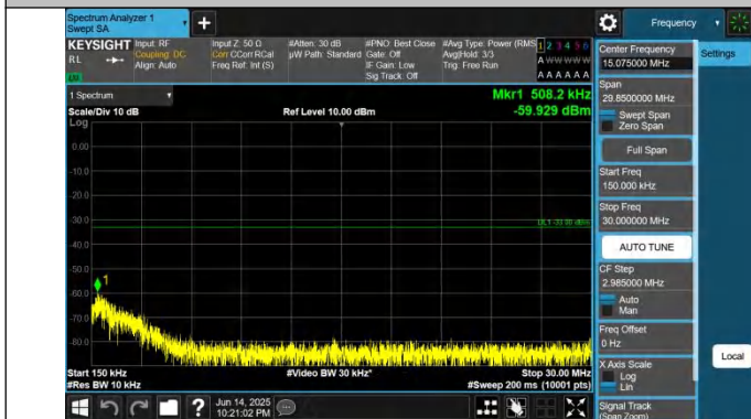
2-2-20MHz-5MHz-QPSK-QPSK-18875-18992-1RB#0-ORB#0-0.1 5~30MHz-PASS
