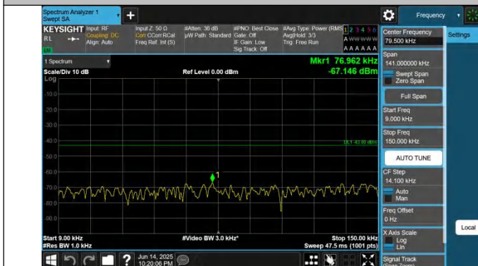
2-2-20MHz-5MHz-QPSK-QPSK-18700-18817-1RB#0-ORB#0-0.0 09~0.15MHz-PASS
