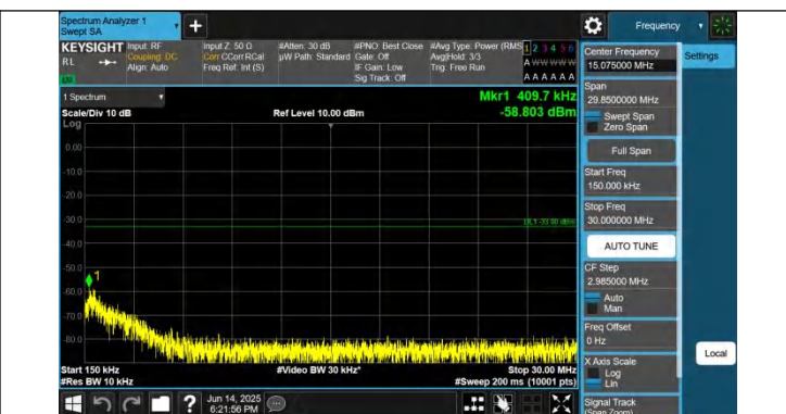
2-2-5MHz-20MHz-QPSK-QPSK-18633-18750-1RB#0-ORB#0-0.1 5~30MHz-PASS
