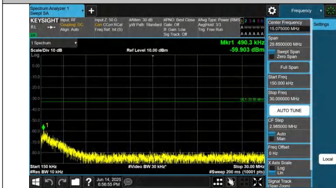
2-2-10MHz-15MHz-QPSK-QPSK-19005-19125-1RB#0-0RB#0-0. 15~30MHz-PASS
