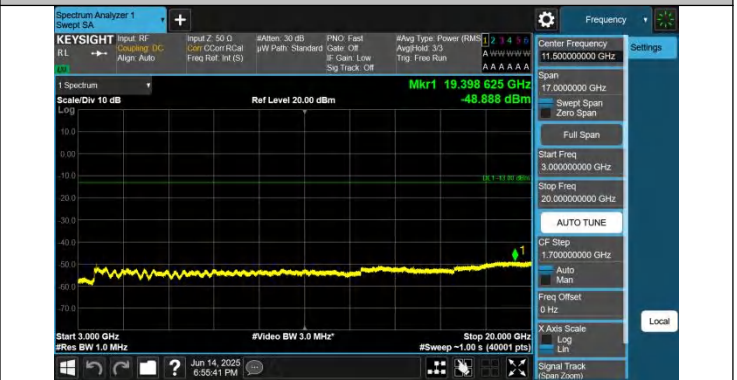
2-2-10MHz-15MHz-QPSK-QPSK-18653-18773-1RB#0-ORB#0-30 00~20000MHz-PASS
