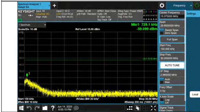
2-2-10MHz-15MHz-QPSK-QPSK-18653-18773-1RB#0-ORB#0-0. 15~30MHz-PASS
