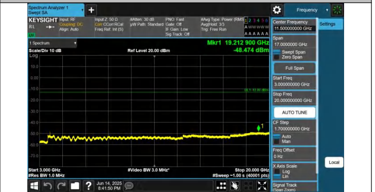
2-2-15MHz-10MHz-QPSK-QPSK-19027-19147-1RB#0-ORB#0-30 00~20000MHz-PASS
