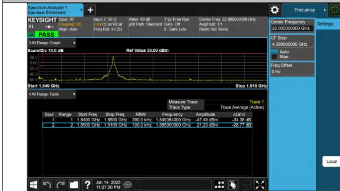
2-2-20MHz-20MHz-QPSK@QPSK-QPSK@QPSK-18700-18898-1RB#99@100RB#0-0RB#0@100RB#0-PASS
