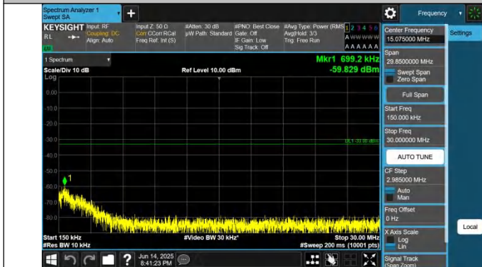
2-2-15MHz-10MHz-QPSK-QPSK-19027-19147-1RB#0-ORB#0-0. 15~30MHz-PASS
