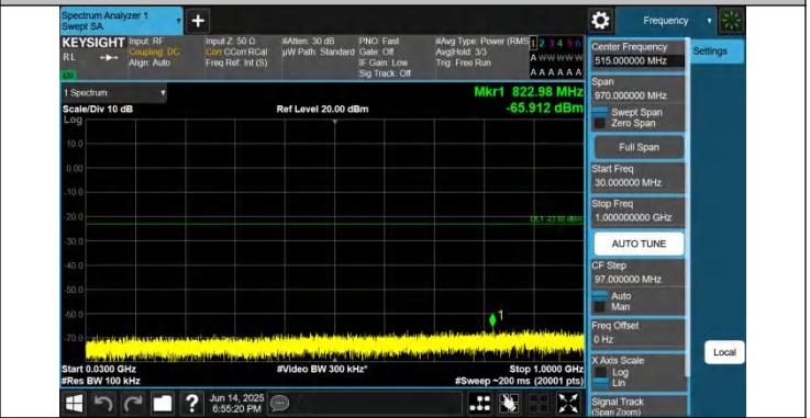
2-2-10MHz-15MHz-QPSK-QPSK-18653-18773-1RB#0-ORB#0-30 ~1000MHz-PASS
