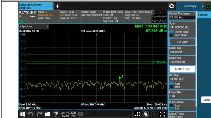
2-2-5MHz-20MHz-QPSK-QPSK-18983-19100-1RB#0-ORB#0-0.0 09~0.15MHz-PASS
