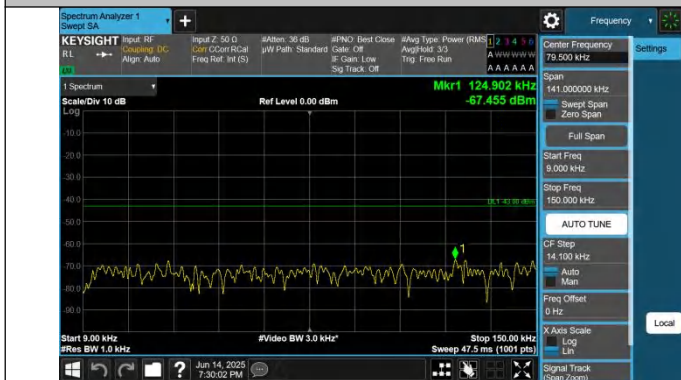
2-2-10MHz-20MHz-QPSK-QPSK-18956-19100-1RB#0-0RB#0-0. 009~0.15MHz-PASS
