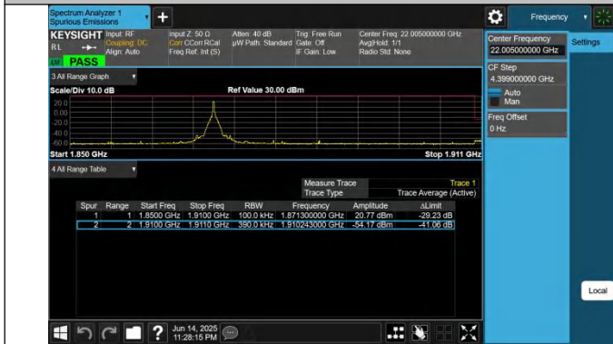
2-2-20MHz-20MHz-QPSK@QPSK-QPSK@QPSK-18902-19100-1RB#0@100RB#0-0RB#0@100RB#0-PASS
