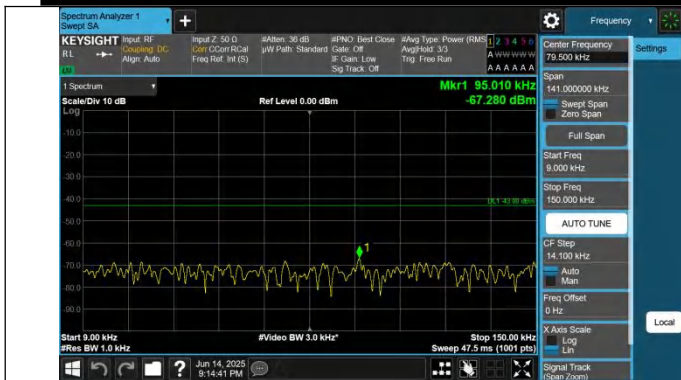
2-2-15MHz-15MHz-QPSK-QPSK-18975-19125-1RB#0-0RB#0-0. 009~0.15MHz-PASS
