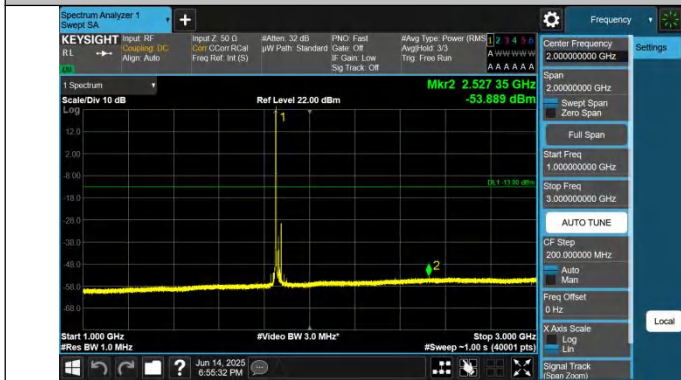
2-2-10MHz-15MHz-QPSK-QPSK-18653-18773-1RB#0-ORB#0-10 00~3000MHz-PASS
