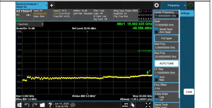
2-2-15MHz-20MHz-QPSK-QPSK-18929-19100-1RB#0-ORB#0-30 00~20000MHz-PASS
