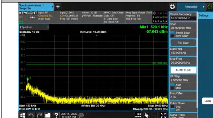
2-2-15MHz-15MHz-QPSK-QPSK-18825-18975-1RB#0-0RB#0-0. 15~30MHz-PASS
