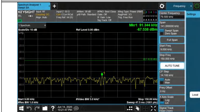
2-2-20MHz-5MHz-QPSK-QPSK-19050-19167-1RB#0-ORB#0-0.0 09~0.15MHz-PASS
