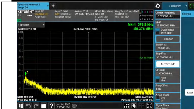
2-2-5MHz-20MHz-QPSK-QPSK-18808-18925-1RB#0-ORB#0-0.1 5~30MHz-PASS
