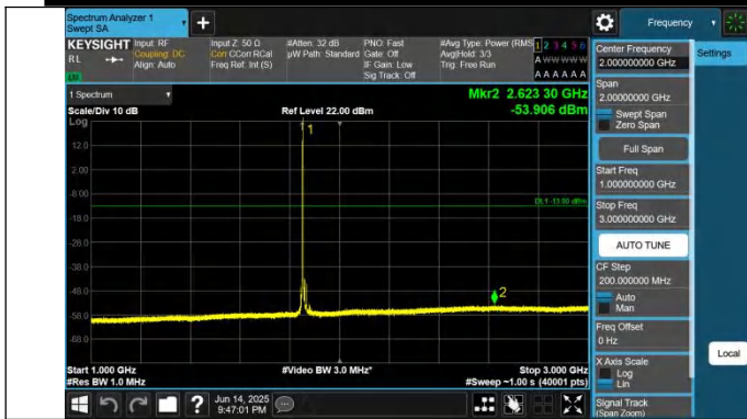
2-2-15MHz-20MHz-QPSK-QPSK-18678-18849-1RB#0-0RB#0-10 00~3000MHz-PASS
