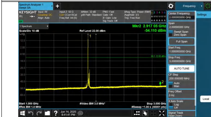
2-2-15MHz-10MHz-QPSK-QPSK-19027-19147-1RB#0-ORB#0-10 00~3000MHz-PASS
