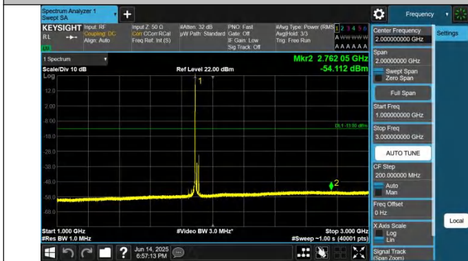
2-2-10MHz-15MHz-QPSK-QPSK-19005-19125-1RB#0-0RB#0-10 00~3000MHz-PASS
