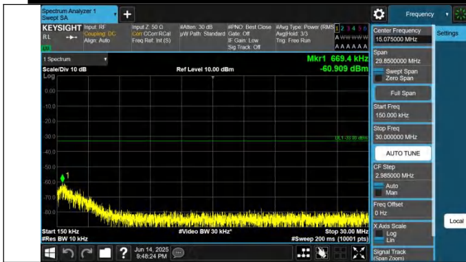
2-2-15MHz-20MHz-QPSK-QPSK-18929-19100-1RB#0-ORB#0-0. 15~30MHz-PASS
