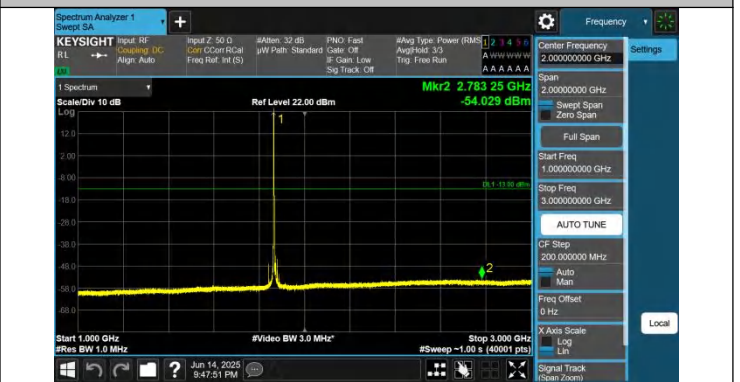
2-2-15MHz-20MHz-QPSK-QPSK-18803-18974-1RB#0-0RB#0-10 00~3000MHz-PASS
