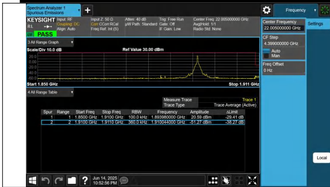
2-2-20MHz-15MHz-QPSK@QPSK-QPSK@QPSK-18951-19122-1RB#99@100RB#0-0RB#0@75RB#0-PASS
