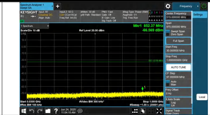
Band66-3MHz-QPSK-131987-1RB#0-30~1000-PASS
