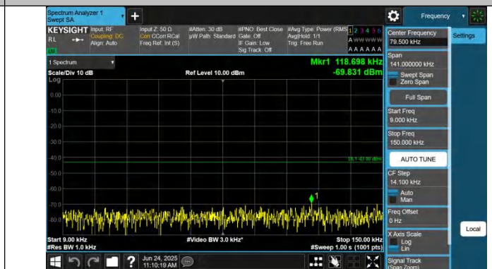
Band66-5MHz-QPSK-132322-1RB#0-0.009~0.15-PASS
