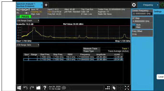
Band66-15MHz-QPSK-132047-1RB#0-PASS
