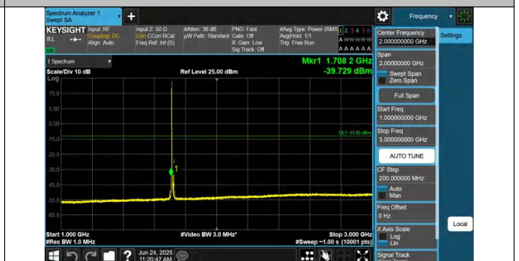
Band66-15MHz-QPSK-132047-1RB#0-1000~3000-PASS
