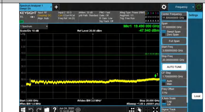
Band66-5MHz-QPSK-132322-1RB#0-3000~20000-PASS
