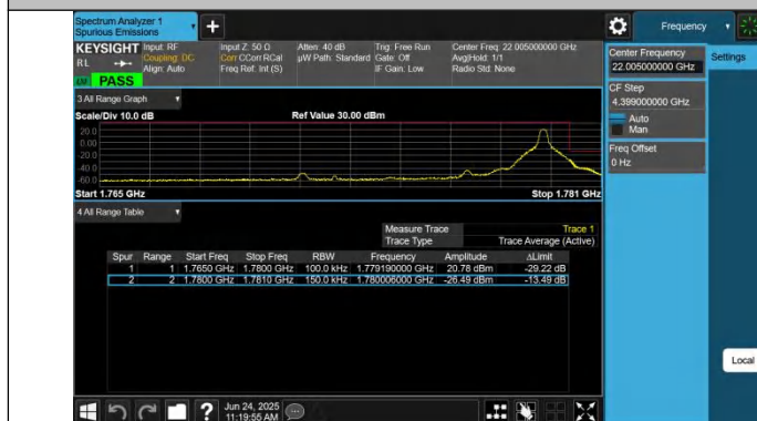
Band66-15MHz-QPSK-132597-1RB#74-PASS
