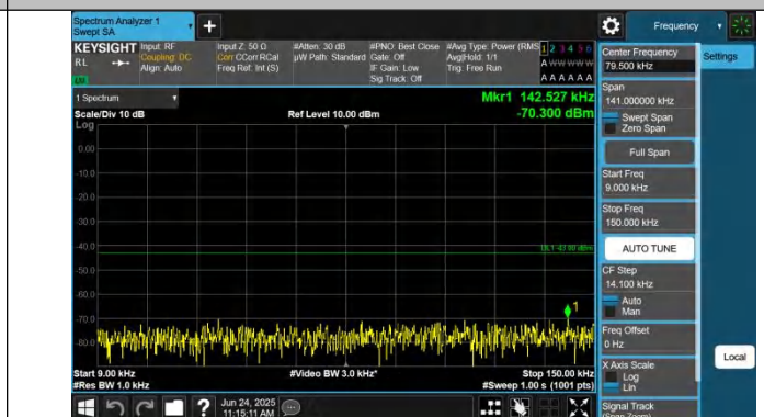
Band66-10MHz-QPSK-132022-1RB#0-0.009~0.15-PASS
