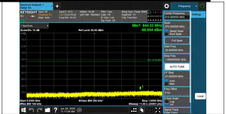
Band66-10MHz-QPSK-132622-1RB#0-30~1000-PASS
