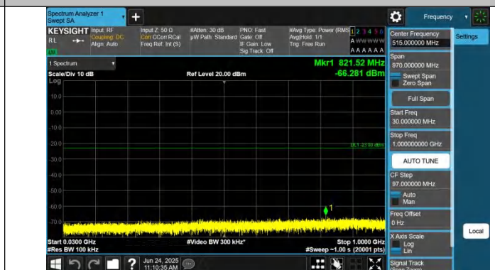
Band66-5MHz-QPSK-132322-1RB#0-30~1000-PASS
