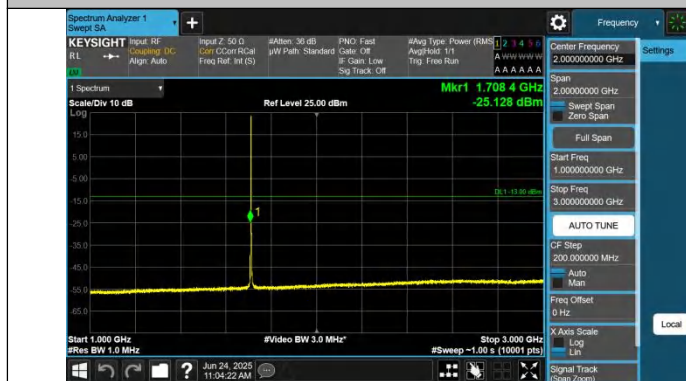
Band66-3MHz-QPSK-131987-1RB#0-1000~3000-PASS
