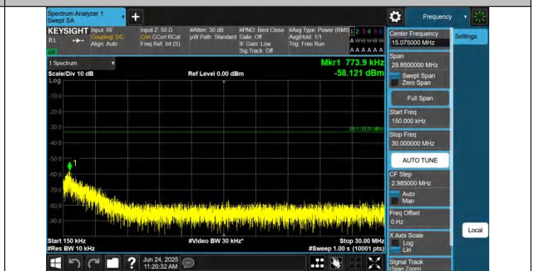
Band66-15MHz-QPSK-132047-1RB#0-0.15~30-PASS
