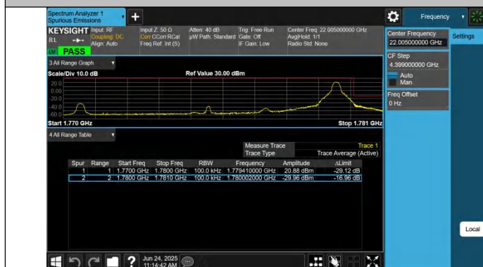
Band66-10MHz-QPSK-132622-1RB#49-PASS
