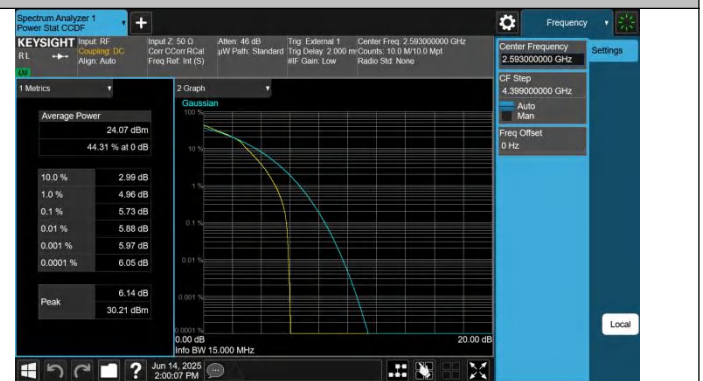
Band41-15MHz-16QAM-40620-75RB#0-PASS
