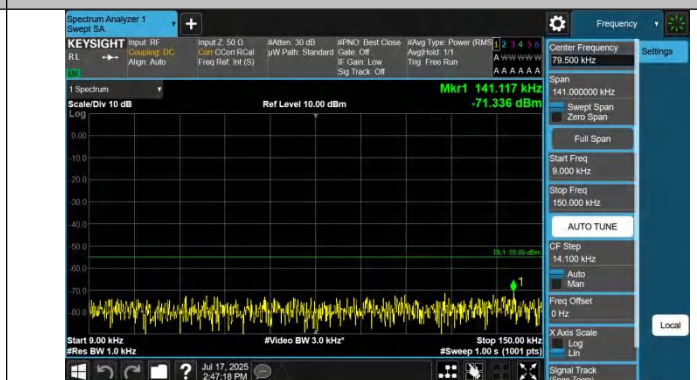
Band41-20MHz-QPSK-39750-1RB#0-0.009~0.15-PASS
