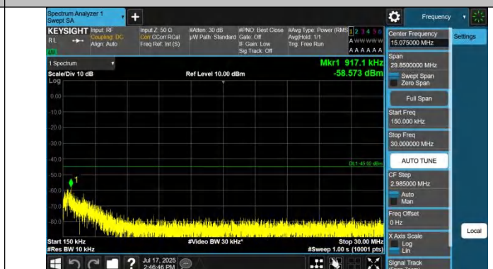
Band41-15MHz-QPSK-39725-1RB#0-0.15-30-PASS
