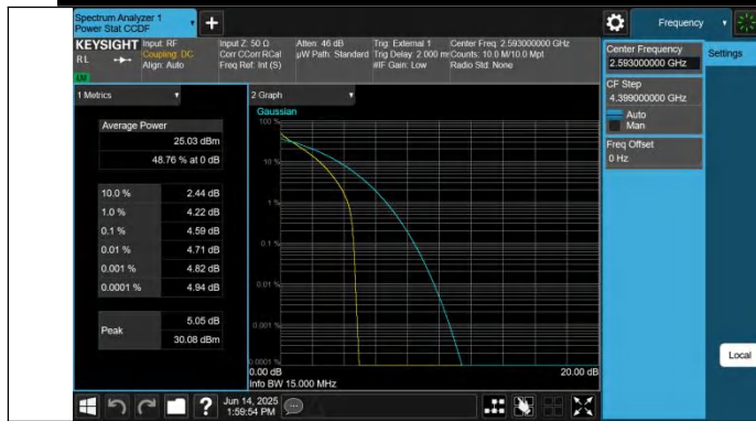
Band41-15MHz-QPSK-40620-75RB#0-PASS
