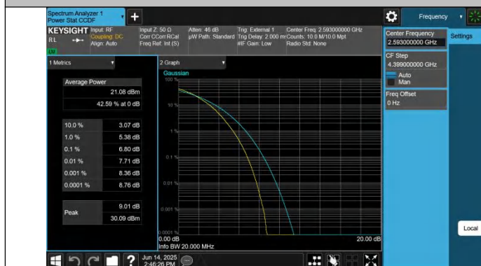
Band41-20MHz-256QAM-40620-100RB#0-PASS
