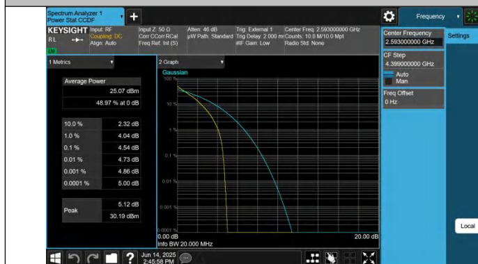
Band41-20MHz-QPSK-40620-100RB#0-PASS
