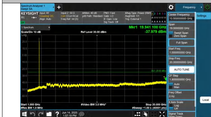
Band41-15MHz-QPSK-40620-1RB#0-1000~20000-PASS
