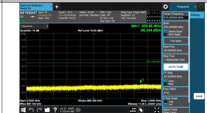
Band41-10MHz-QPSK-41540-1RB#0-30-1000-PASS
