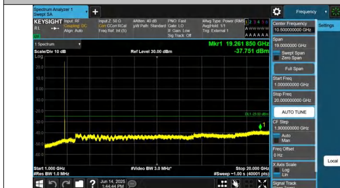
Band41-10MHz-QPSK-41540-1RB#0-1000-20000-PASS
