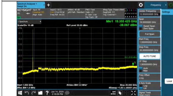
Band41-20MHz-QPSK-41490-1RB#0-1000~20000-PASS
