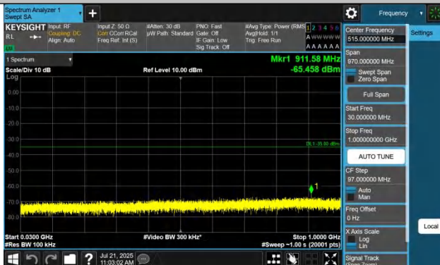
Band41-5MHz-QPSK-41565-1RB#0-30~1000-PASS
