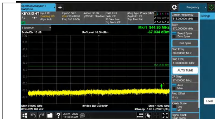
Band41-15MHz-QPSK-39725-1RB#0-30~1000-PASS
