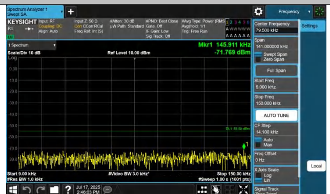
Band41-10MHz-QPSK-39700-1RB#0-0.009~0.15-PASS
