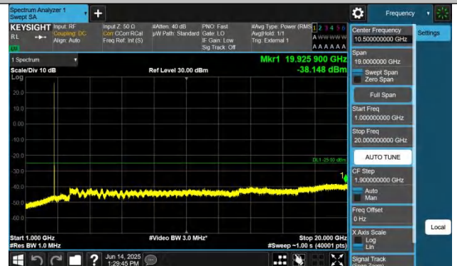
Band41-5MHz-QPSK-41565-1RB#0-1000~20000-PASS
