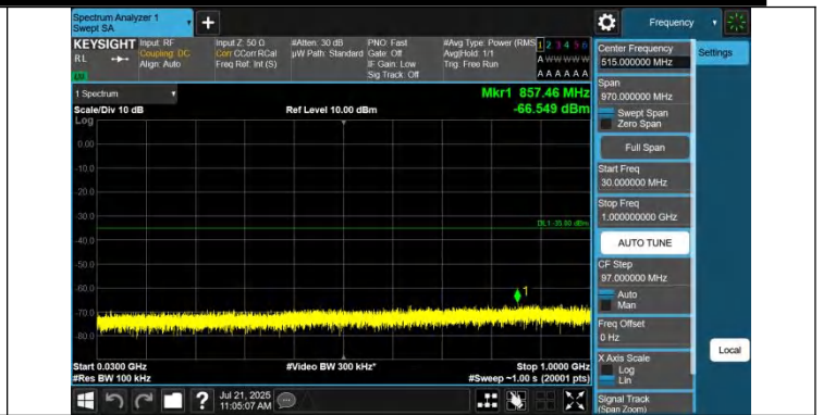
Band41-20MHz-QPSK-41490-1RB#0-30~1000-PASS
