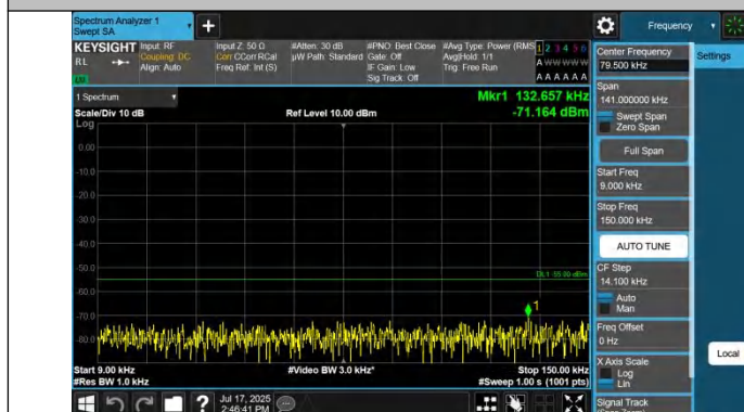
Band41-15MHz-QPSK-39725-1RB#0-0.009-0.15-PASS
