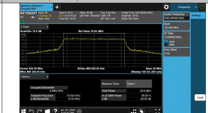
Band26(824-849)-10MHz-16QAM-26915-50RB#0-PASS
