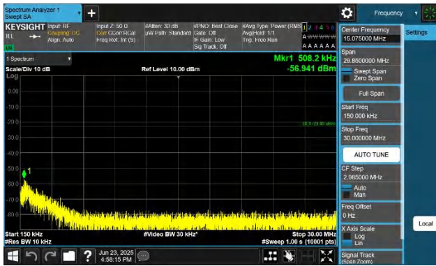
Band26(824-849)-5MHz-QPSK-26915-1RB#0-0.15~30-PASS
