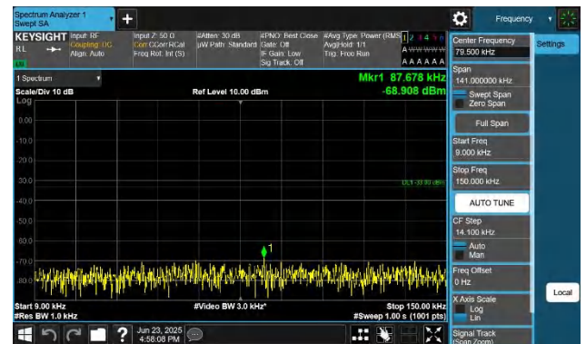
Band26(824-849)-5MHz-QPSK-26915-1RB#0-0.009~0.15-PASS
