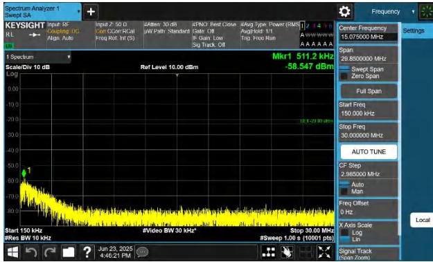
Band26(824-849)-1.4MHz-QPSK-26915-1RB#0-0.15~30-PASS
