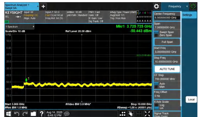
Band26(824-849)-3MHz-QPSK-27025-1RB#0-3000~10000-PASS
