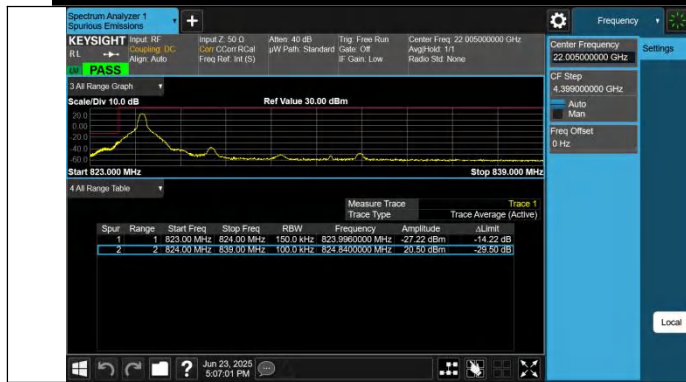
Band26(824-849)-15MHz-QPSK-26865-1RB#0-PASS
