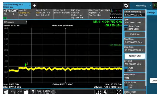
Band26(824-849)-15MHz-QPSK-26915-1RB#0-3000~10000-PAS S
