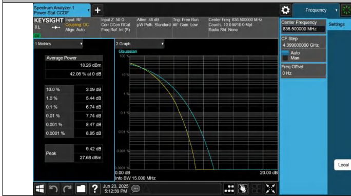
Band26(824-849)-15MHz-256QAM-26915-75RB#0-PASS
