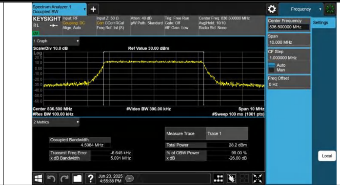
Band26(824-849)-5MHz-64QAM-26915-25RB#0-PASS
