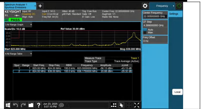
Band26(824-849)-15MHz-QPSK-26865-1RB#74-PASS
