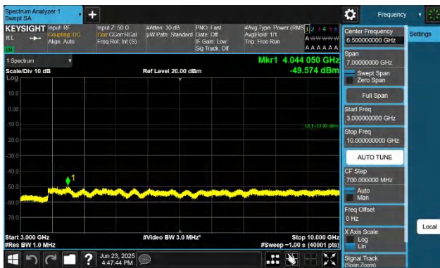
Band26(824-849)-1.4MHz-QPSK-27033-1RB#0-3000~10000-PASS S
