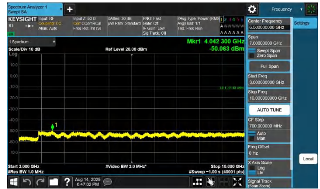
Band26(824-849)-3MHz-QPSK-26805-1RB#0-3000~10000-PASS
