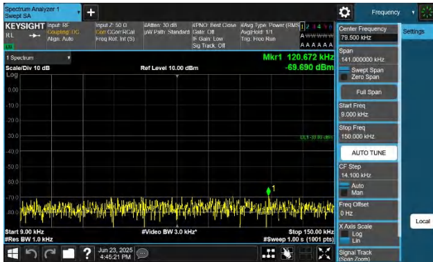
Band26(824-849)-1.4MHz-QPSK-26797-1RB#0-0.009~0.15-PASS
