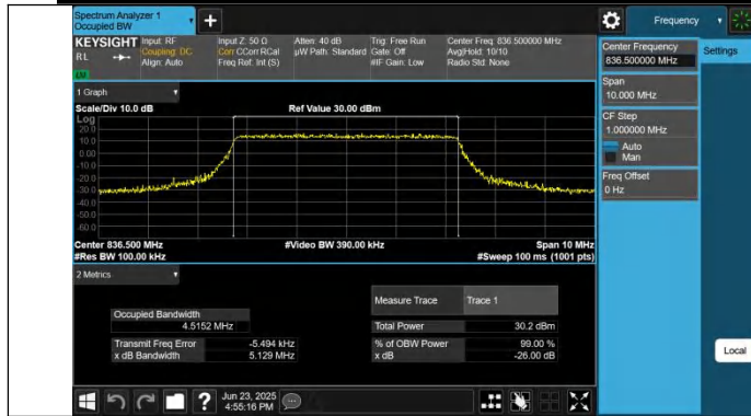
Band26(824-849)-5MHz-QPSK-26915-25RB#0-PASS
