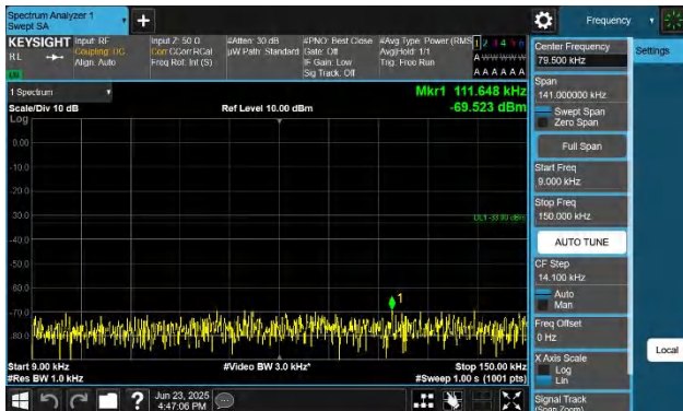
Band26(824-849)-1.4MHz-QPSK-27033-1RB#0-0.009~0.15-PASS
