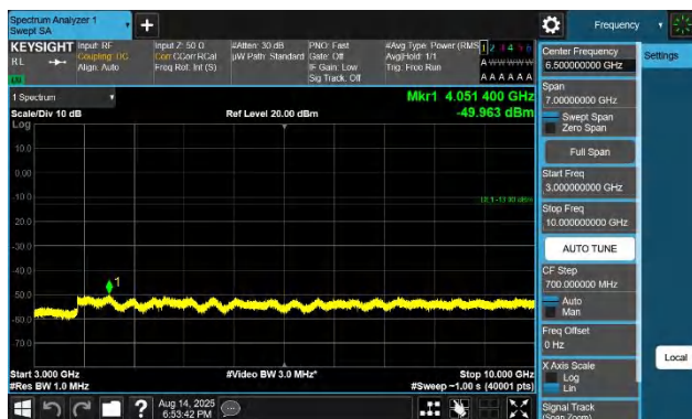
Band26(824-849)-15MHz-QPSK-26965-1RB#0-3000~10000-PAS
