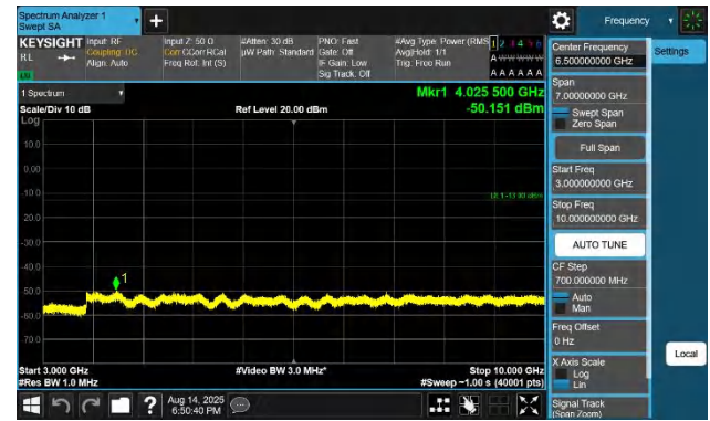
Band26(824-849)-10MHz-QPSK-26840-1RB#0-3000~10000-PAS
