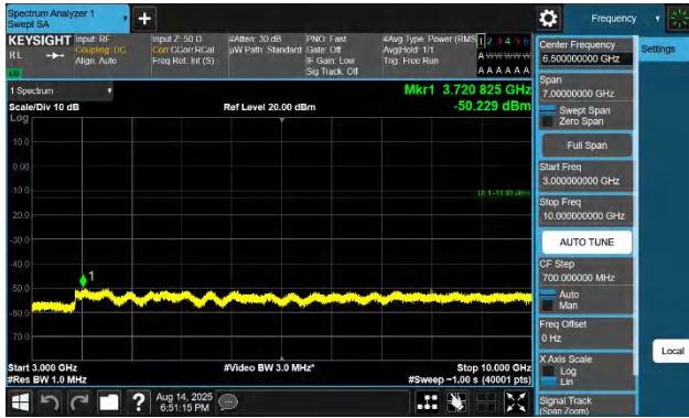
Band26(824-849)-10MHz-QPSK-26915-1RB#0-3000~10000-PAS S
