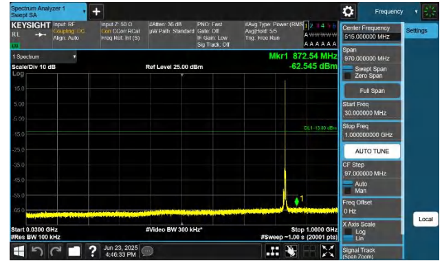
Band26(824-849)-1.4MHz-QPSK-26915-1RB#0-30~1000-PASS
