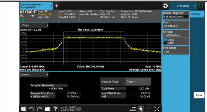
Band26(824-849)-5MHz-16QAM-26915-25RB#0-PASS
