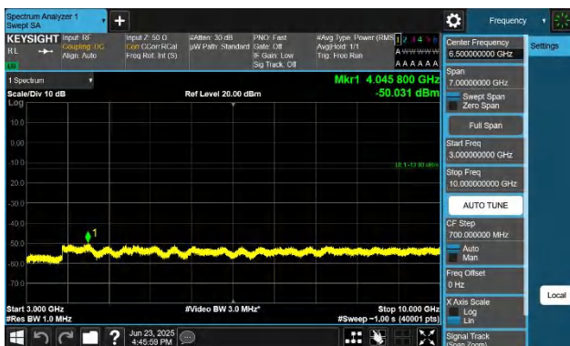
Band26(824-849)-1.4MHz-QPSK-26797-1RB#0-3000~10000-PAS
