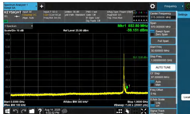
Band26(824-849)-15MHz-QPSK-26915-1RB#0-30~1000-PASS
