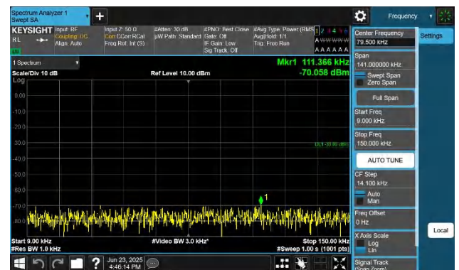
Band26(824-849)-1.4MHz-QPSK-26915-1RB#0-0.009~0.15-PASS
