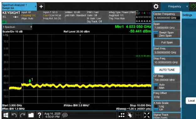
Band26(824-849)-5MHz-QPSK-27015-1RB#0-3000~10000-PASS
