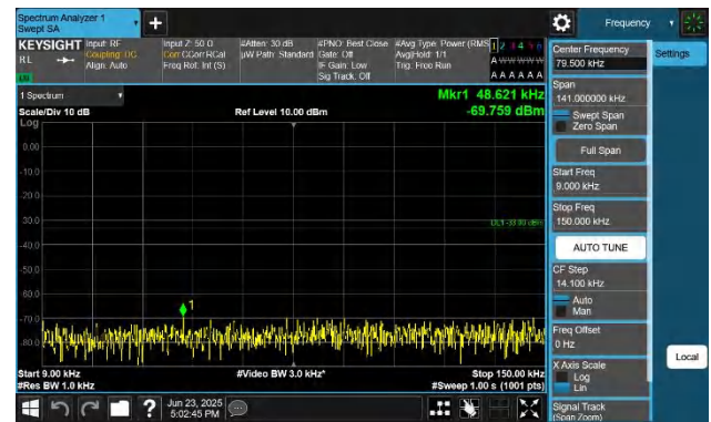
Band26(824-849)-10MHz-QPSK-26840-1RB#0-0.009~0.15-PASS
