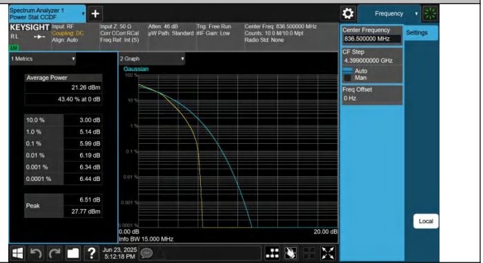
Band26(824-849)-15MHz-16QAM-26915-75RB#0-PASS
