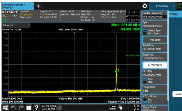
Band26(824-849)-1.4MHz-QPSK-26797-1RB#0-30~1000-PASS
