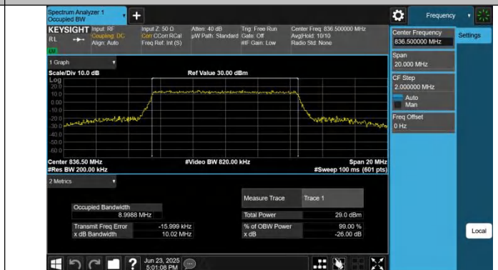
Band26(824-849)-10MHz-64QAM-26915-50RB#0-PASS
