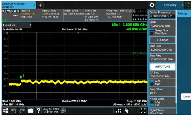
Band26(824-849)-3MHz-QPSK-26915-1RB#0-3000~10000-PASS
