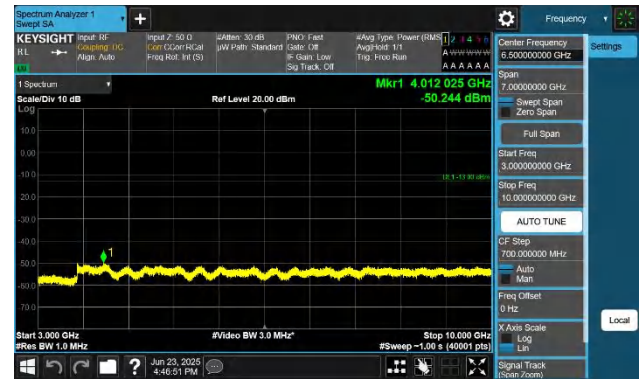
Band26(824-849)-1.4MHz-QPSK-26915-1RB#0-3000~10000-PASS
