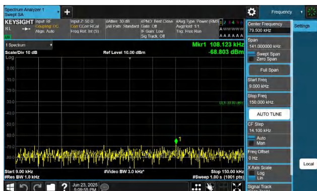
Band26(824-849)-15MHz-QPSK-26965-1RB#0-0.009~0.15-PASS
