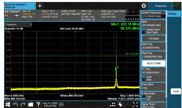
Band26(824-849)-10MHz-QPSK-26840-1RB#0-30~1000-PASS
