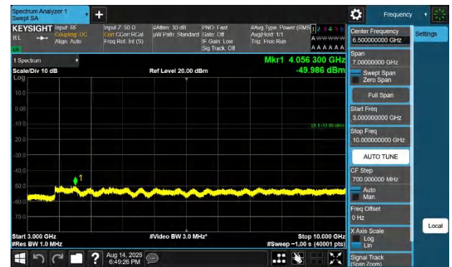
Band26(824-849)-5MHz-QPSK-26915-1RB#0-3000~10000-PASS
