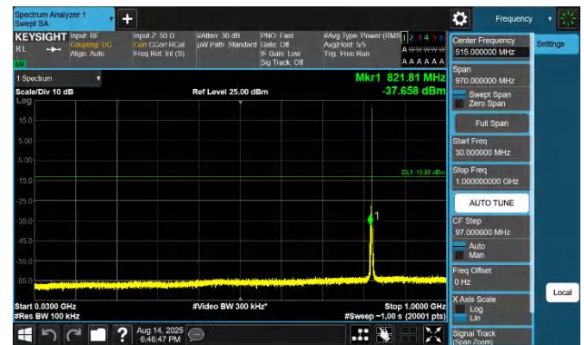
Band26(824-849)-3MHz-QPSK-26805-1RB#0-30~1000-PASS
