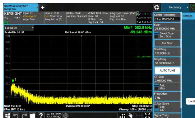
Band26(824-849)-15MHz-QPSK-26965-1RB#0-0.15~30-PASS
