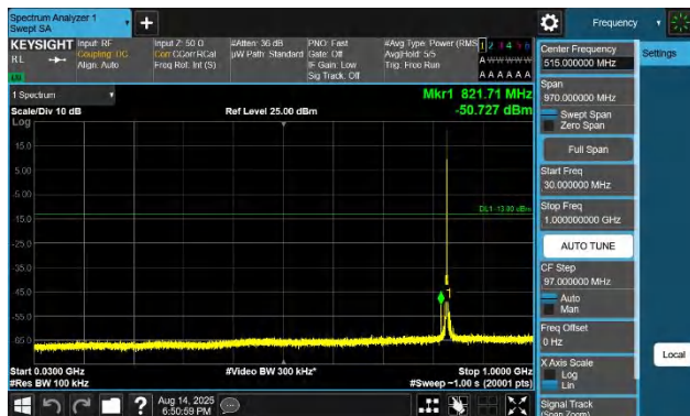
Band26(824-849)-10MHz-QPSK-26915-1RB#0-30~1000-PASS
