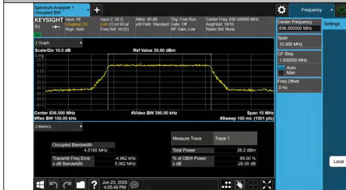
Band26(824-849)-5MHz-256QAM-26915-25RB#0-PASS
