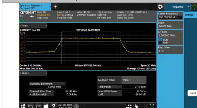
Band26(824-849)-10MHz-256QAM-26915-50RB#0-PASS
