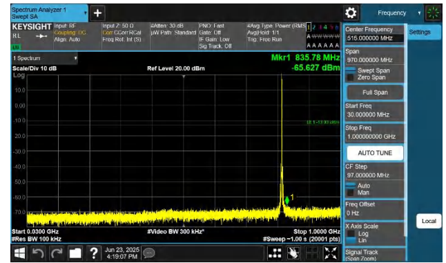
Band26(814-824)-1.4MHz-QPSK-26740-1RB#0-30~1000-PASS
