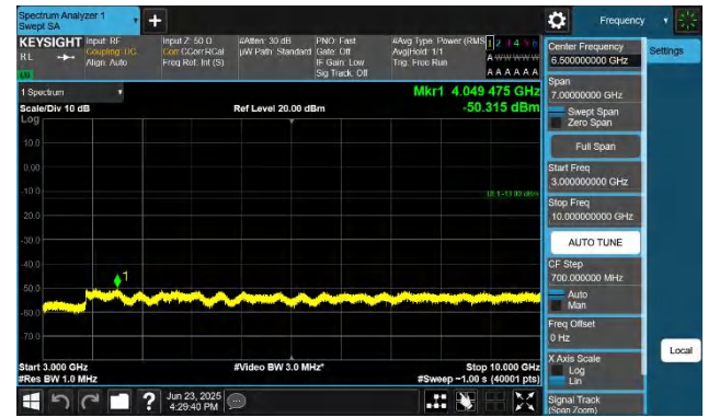
Band26(814-824)-3MHz-QPSK-26705-1RB#0-3000~10000-PASS
