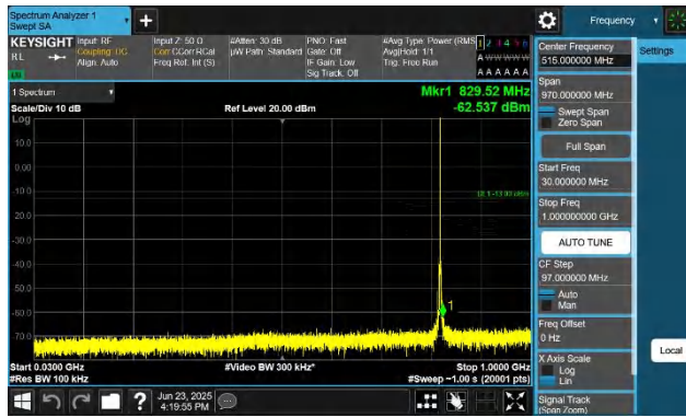
Band26(814-824)-1.4MHz-QPSK-26783-1RB#0-30~1000-PASS
