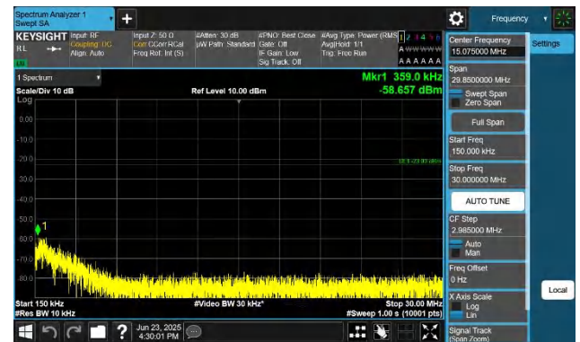
Band26(814-824)-3MHz-QPSK-26740-1RB#0-0.15~30-PASS
