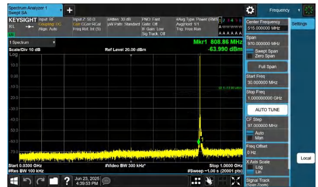
Band26(814-824)-10MHz-QPSK-26740-1RB#0-30~1000-PASS
