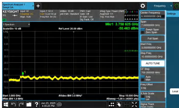
Band26(814-824)-5MHz-QPSK-26715-1RB#0-3000~10000-PASS
