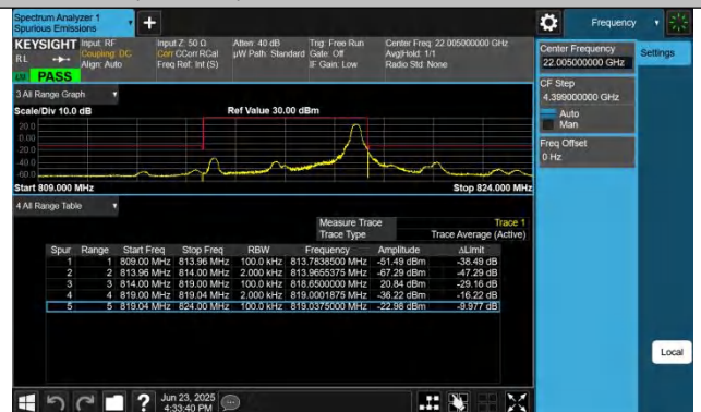
Band26(814-824)-5MHz-QPSK-26715-1RB#24-PASS
