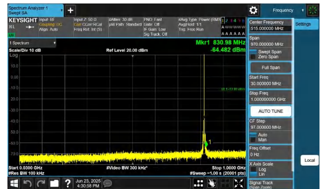
Band26(814-824)-3MHz-QPSK-26775-1RB#0-30~1000-PASS
