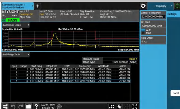
Band26(814-824)-5MHz-QPSK-26715-1RB#0-PASS
