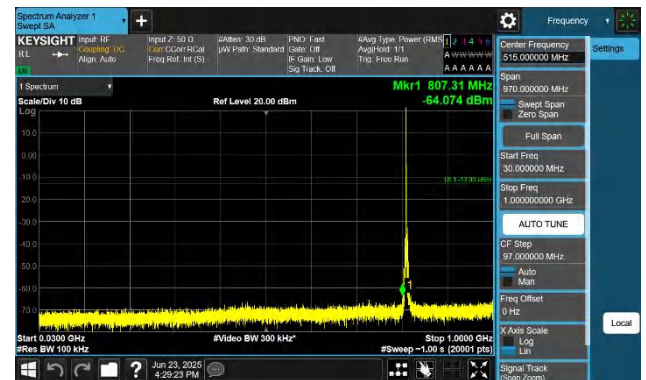
Band26(814-824)-3MHz-QPSK-26705-1RB#0-30~1000-PASS
