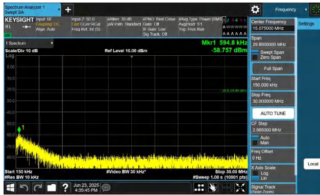
Band26(814-824)-5MHz-QPSK-26740-1RB#0-0.15~30-PASS
