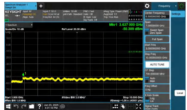
Band26(814-824)-3MHz-QPSK-26775-1RB#0-3000~10000-PASS
