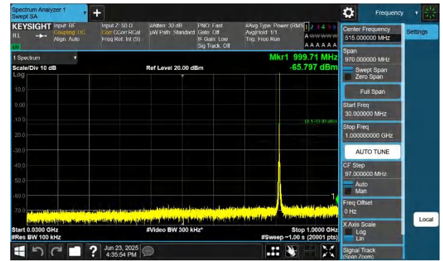
Band26(814-824)-5MHz-QPSK-26740-1RB#0-30~1000-PASS
