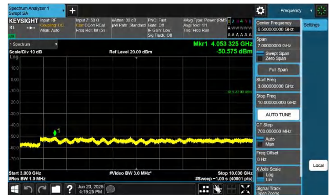
Band26(814-824)-1.4MHz-QPSK-26740-1RB#0-3000~10000-PASS S
