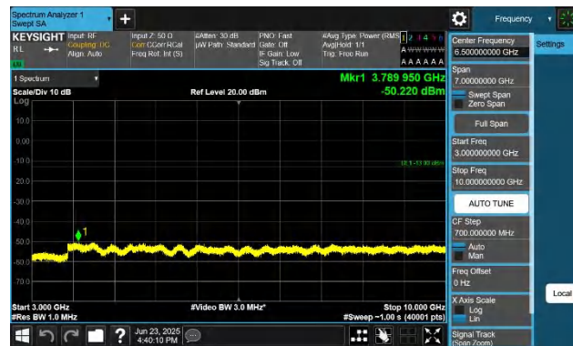
Band26(814-824)-10MHz-QPSK-26740-1RB#0-3000~10000-PAS
