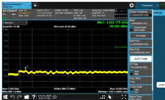
Band26(814-824)-1.4MHz-QPSK-26783-1RB#0-3000~10000-PAS S
