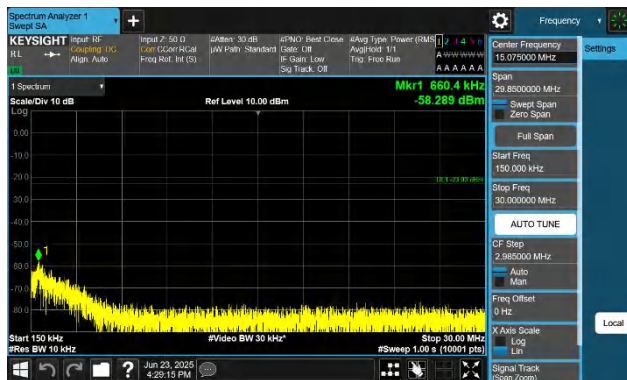
Band26(814-824)-3MHz-QPSK-26705-1RB#0-0.15~30-PASS
