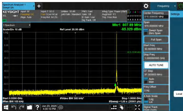
Band26(814-824)-3MHz-QPSK-26740-1RB#0-30~1000-PASS
