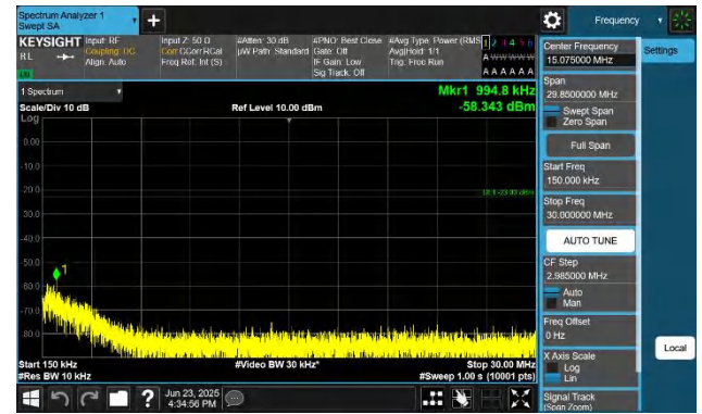
Band26(814-824)-5MHz-QPSK-26715-1RB#0-0.15~30-PASS
