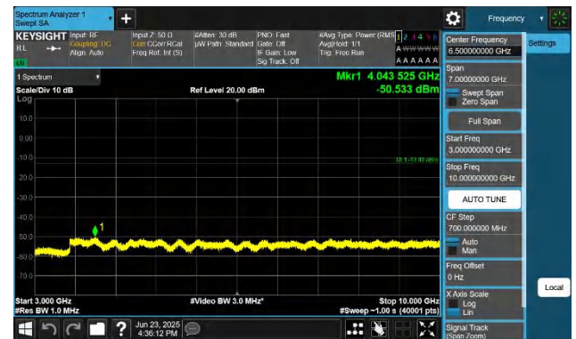
Band26(814-824)-5MHz-QPSK-26740-1RB#0-3000~10000-PASS
