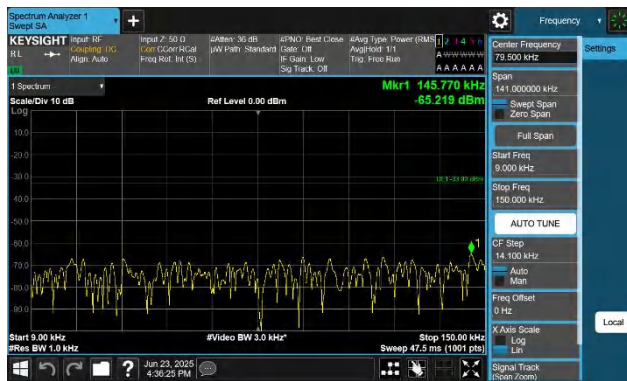
Band26(814-824)-5MHz-QPSK-26765-1RB#0-0.009~0.15-PASS
