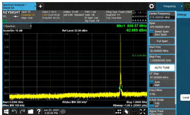
Band26(814-824)-5MHz-QPSK-26715-1RB#0-30~1000-PASS
