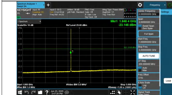
Band25-3MHz-QPSK-26055-1RB#0-1000~3000-PASS
