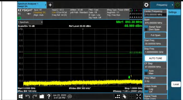
Band25-3MHz-QPSK-26055-1RB#0-30~1000-PASS
