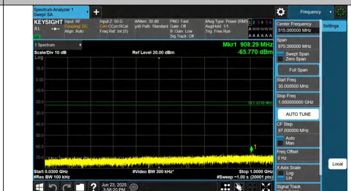
Band25-10MHz-QPSK-26090-1RB#0-30~1000-PASS
