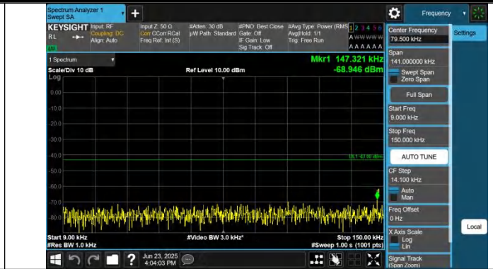
Band25-15MHz-QPSK-26365-1RB#0-0.009~0.15-PASS
