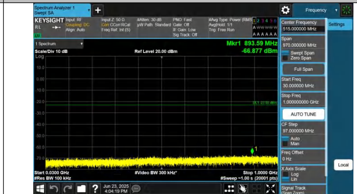
Band25-15MHz-QPSK-26365-1RB#0-30~1000-PASS
