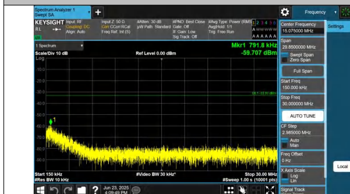
Band25-20MHz-QPSK-26590-1RB#0-0.15~30-PASS
