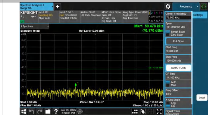
Band25-10MHz-QPSK-26090-1RB#0-0.009~0.15-PASS
