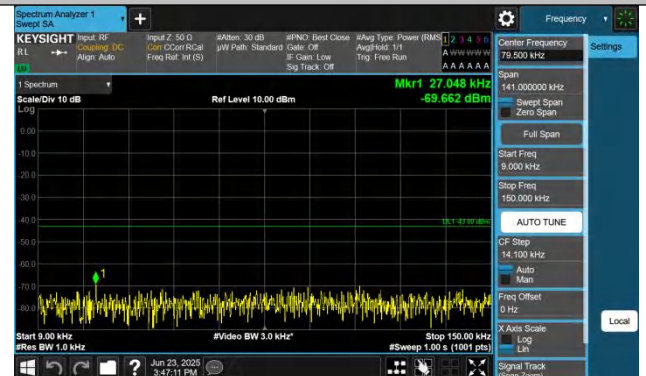
Band25-3MHz-QPSK-26055-1RB#0-0.009~0.15-PASS
