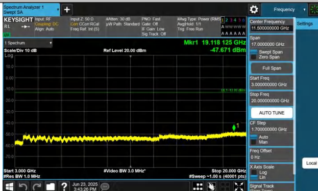
Band25-1.4MHz-QPSK-26683-1RB#0-3000~20000-PASS
