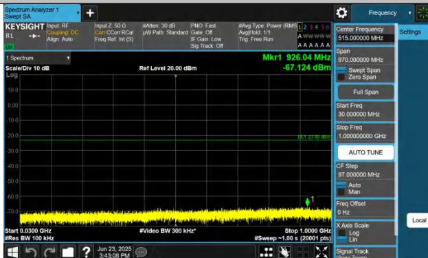
Band25-1.4MHz-QPSK-26683-1RB#0-30~1000-PASS
