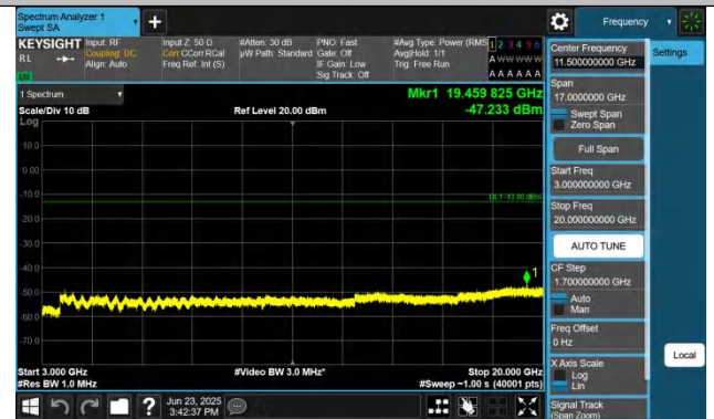
Band25-1.4MHz-QPSK-26365-1RB#0-3000~20000-PASS
