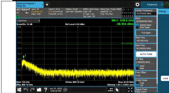
Band25-10MHz-QPSK-26640-1RB#0-0.15~30-PASS
