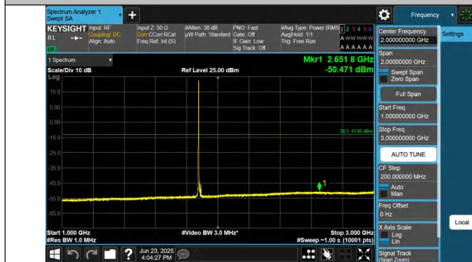
Band25-15MHz-QPSK-26365-1RB#0-1000~3000-PASS
