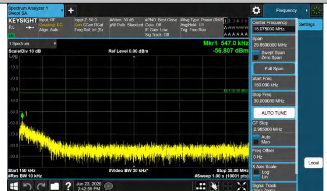
Band25-1.4MHz-QPSK-26683-1RB#0-0.15~30-PASS
