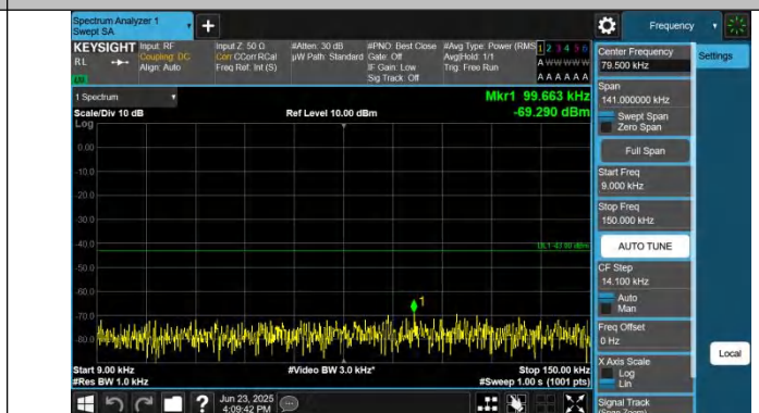
Band25-20MHz-QPSK-26590-1RB#0-0.009~0.15-PASS
