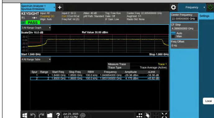
Band25-10MHz-QPSK-26090-1RB#0-PASS
