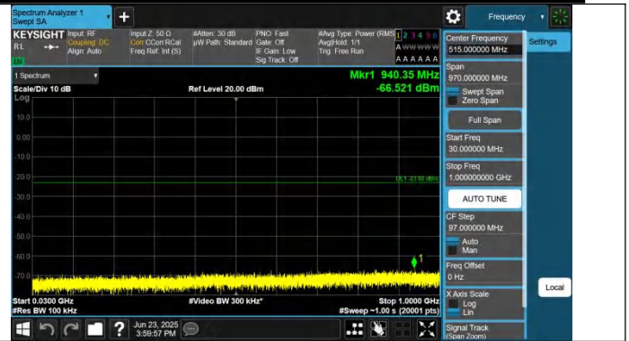
Band25-10MHz-QPSK-26640-1RB#0-30~1000-PASS
