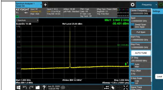
Band25-10MHz-QPSK-26640-1RB#0-1000~3000-PASS
