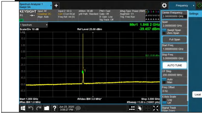
Band25-10MHz-QPSK-26090-1RB#0-1000~3000-PASS
