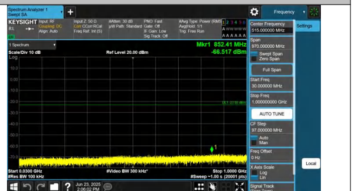
Band4-5MHz-QPSK-20175-1RB#0-30~1000-PASS
