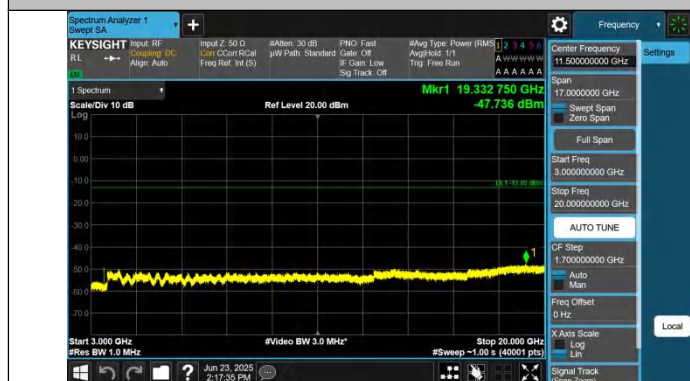
Band4-15MHz-QPSK-20325-1RB#0-3000~20000-PASS
