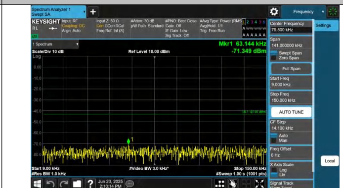
Band4-10MHz-QPSK-20000-1RB#0-0.009~0.15-PASS
