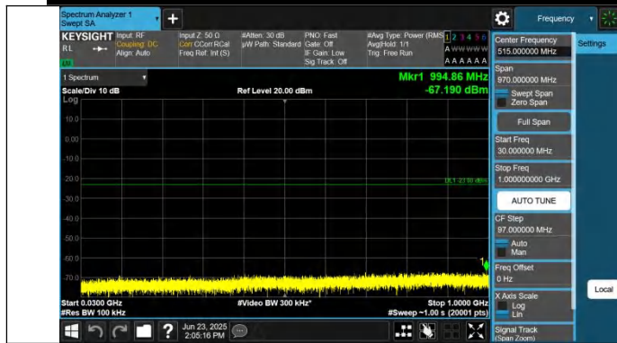
Band4-5MHz-QPSK-19975-1RB#0-30~1000-PASS
