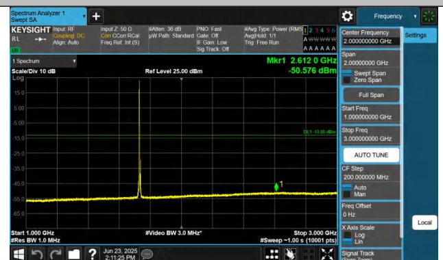
Band4-10MHz-QPSK-20175-1RB#0-1000~3000-PASS
