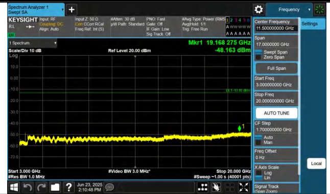
Band4-10MHz-QPSK-20000-1RB#0-3000~20000-PASS
