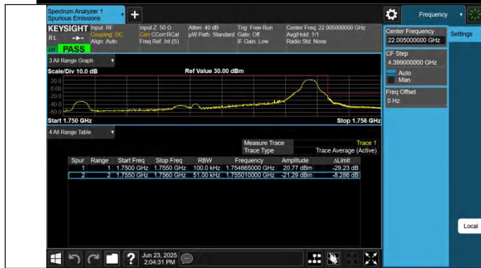
Band4-5MHz-QPSK-20375-1RB#24-PASS
