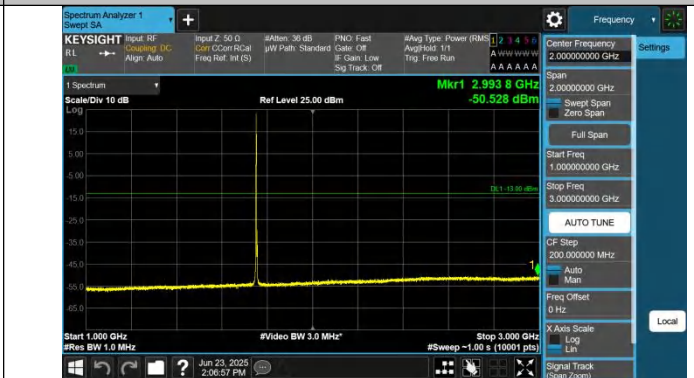
Band4-5MHz-QPSK-20375-1RB#0-1000~3000-PASS
