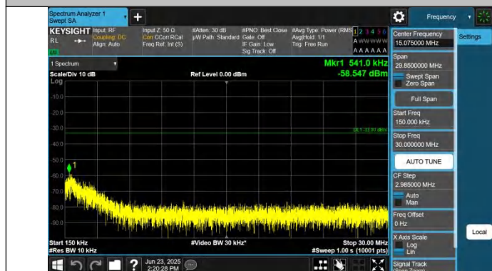
Band4-20MHz-QPSK-20050-1RB#0-0.15~30-PASS
