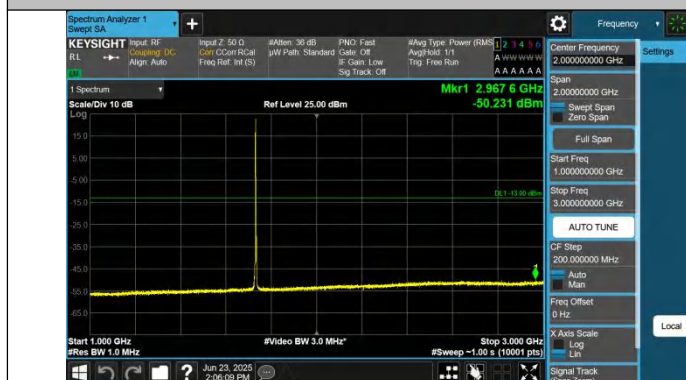
Band4-5MHz-QPSK-20175-1RB#0-1000~3000-PASS
