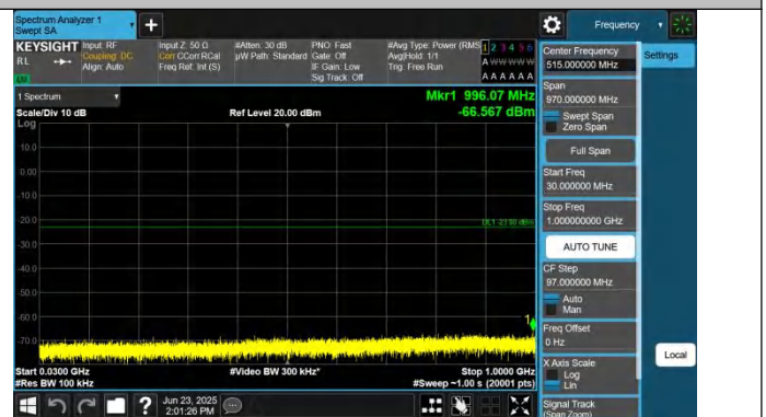
Band4-3MHz-QPSK-20385-1RB#0-30~1000-PASS
