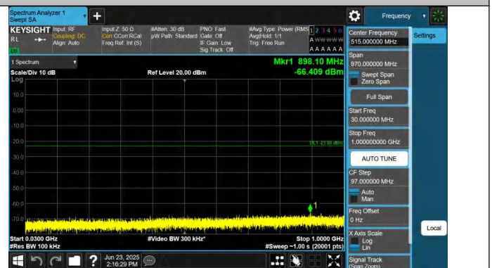
Band4-15MHz-QPSK-20175-1RB#0-30~1000-PASS
