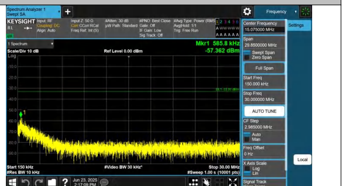
Band4-15MHz-QPSK-20325-1RB#0-0.15~30-PASS
