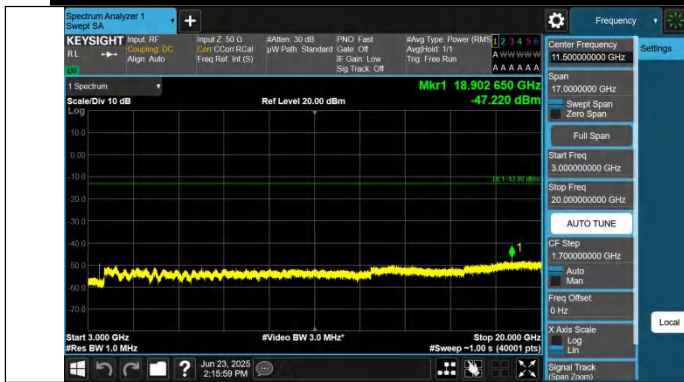
Band4-15MHz-QPSK-20025-1RB#0-3000~20000-PASS
