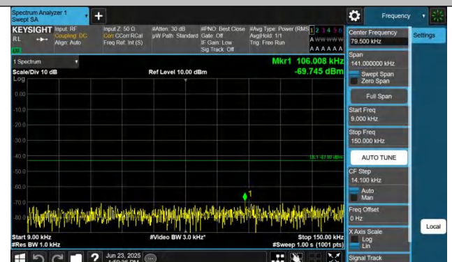
Band4-3MHz-QPSK-19965-1RB#0-0.009~0.15-PASS
