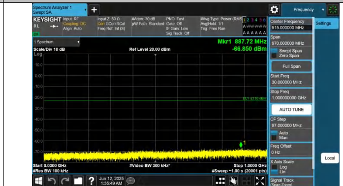
Band2-15MHz-QPSK-18900-1RB#0-30~1000-PASS
