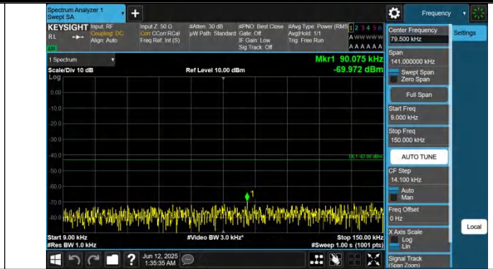
Band2-15MHz-QPSK-18900-1RB#0-0.009~0.15-PASS
