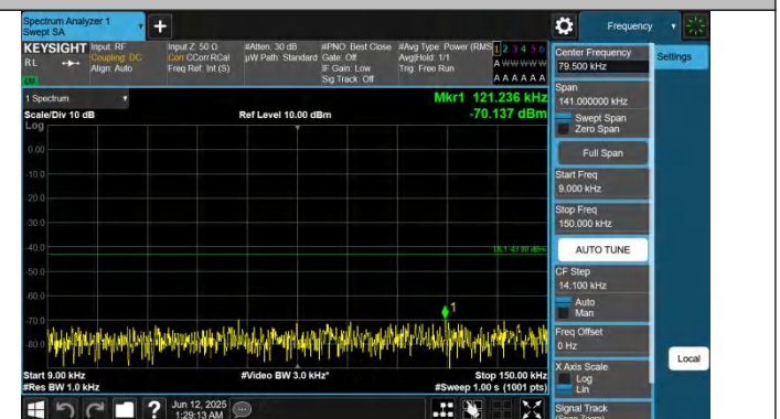
Band2-10MHz-QPSK-18650-1RB#0-0.009~0.15-PASS
