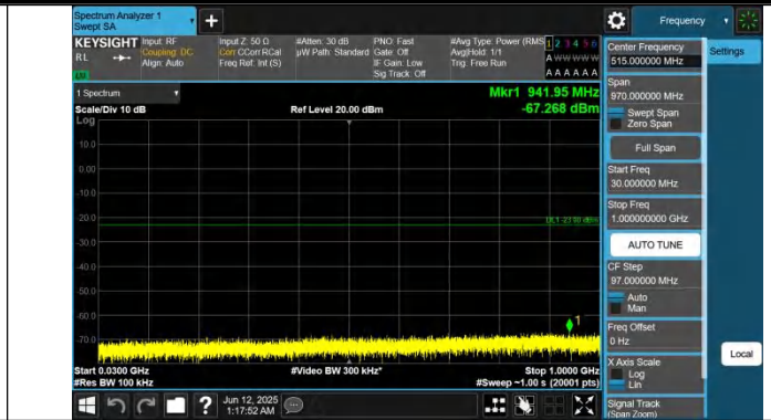
Band2-3MHz-QPSK-18615-1RB#0-30~1000-PASS
