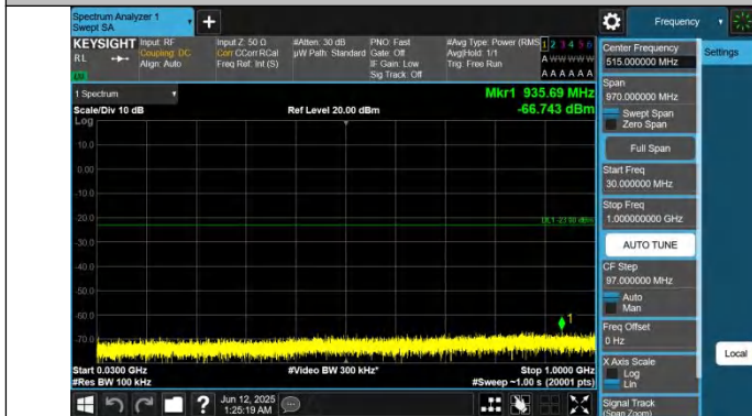
Band2-5MHz-QPSK-19175-1RB#0-30~1000-PASS
