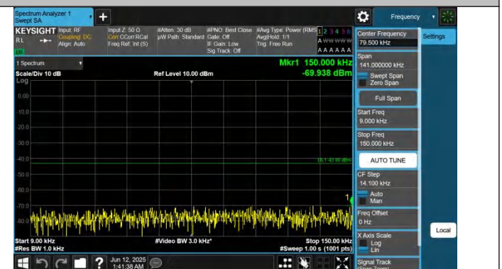
Band2-20MHz-QPSK-19100-1RB#0-0.009~0.15-PASS
