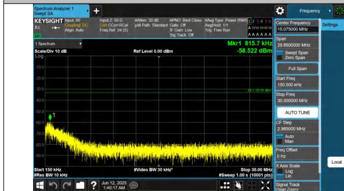
Band2-20MHz-QPSK-18700-1RB#0-0.15~30-PASS
