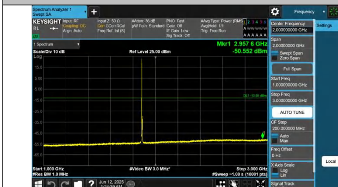
Band2-5MHz-QPSK-18900-1RB#0-1000~3000-PASS
