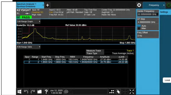
Band2-15MHz-QPSK-18675-1RB#0-PASS
