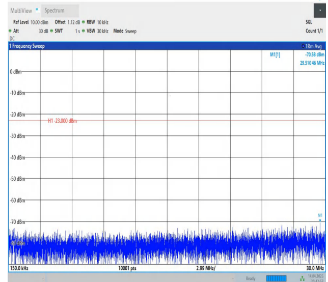
Band26(824-849)-10MHz-QPSK-26990-1RB#0-0.15~30-PASS
