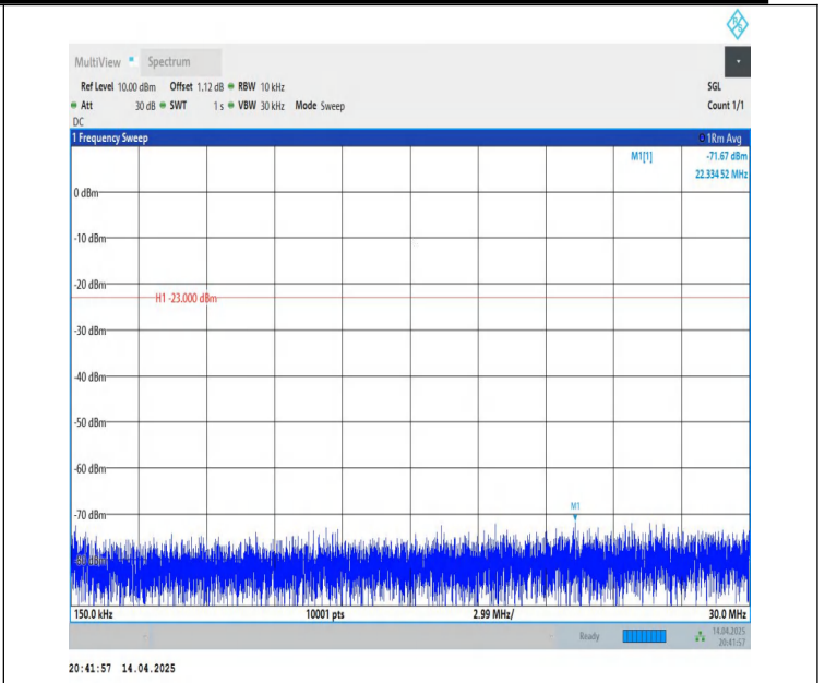
Band26(824-849)-10MHz-QPSK-26915-1RB#0-0.15~30-PASS
