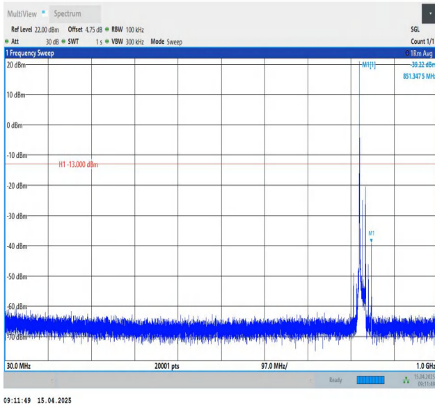
Band26(824-849)-15MHz-QPSK-26865-1RB#0-30~1000-PASS
