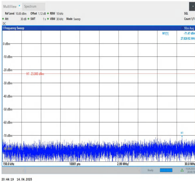
Band26(824-849)-15MHz-QPSK-26865-1RB#74-0.15~30-PASS
