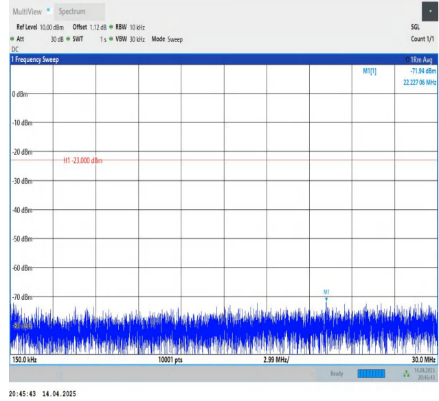
Band26(824-849)-15MHz-QPSK-26965-1RB#0-0.15~30-PASS
