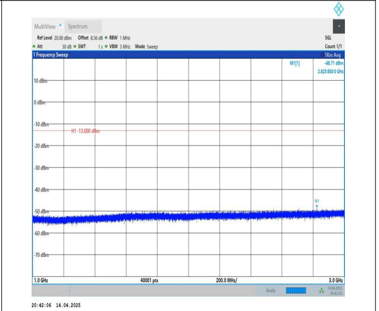
Band26(824-849)-10MHz-QPSK-26915-1RB#0-1000~3000-PASS
