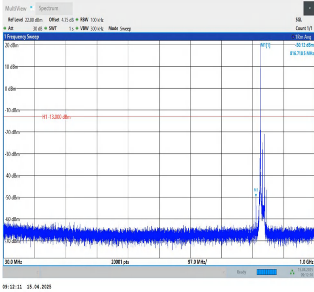
Band26(824-849)-15MHz-QPSK-26915-1RB#0-30~1000-PASS
