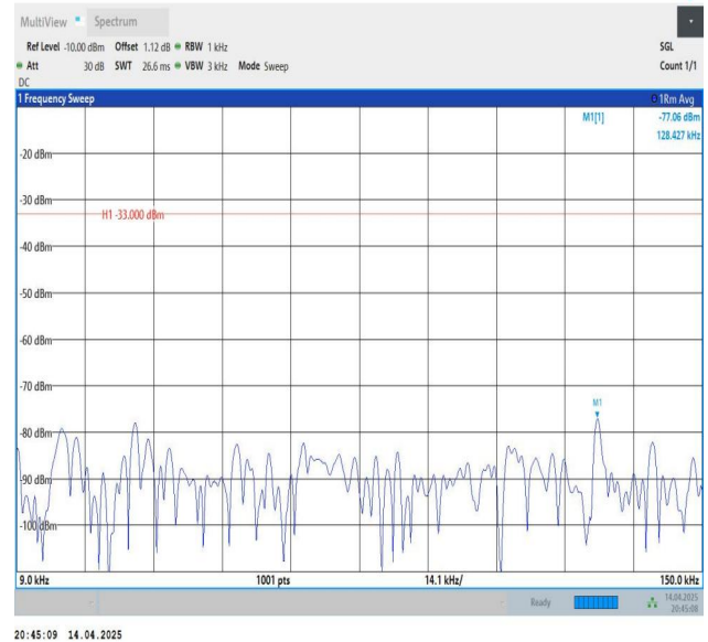
Band26(824-849)-15MHz-QPSK-26915-1RB#74-0.009~0.15-PASS
