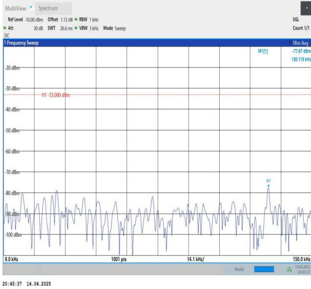
Band26(824-849)-15MHz-QPSK-26965-1RB#0-0.009~0.15-PASS
