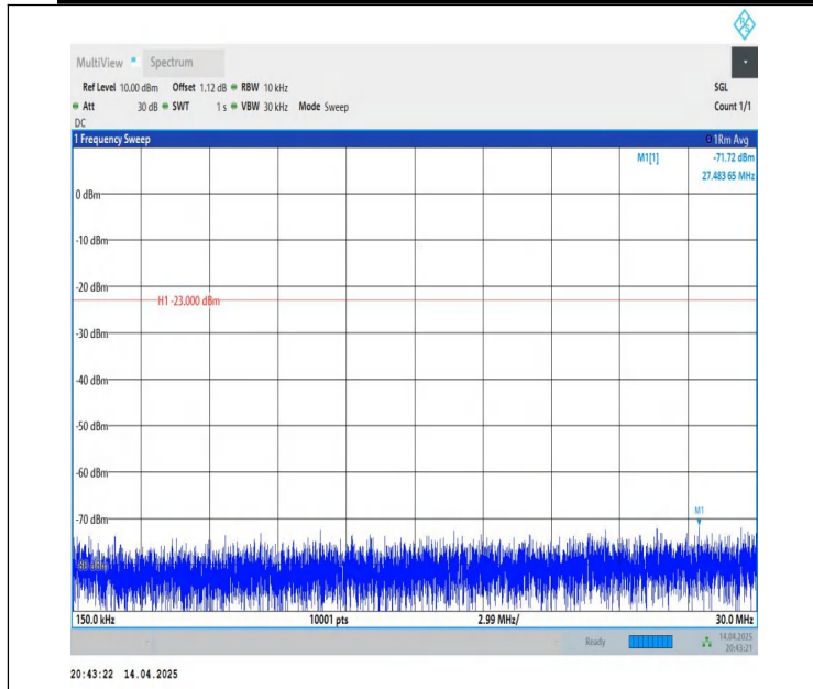
Band26(824-849)-10MHz-QPSK-26990-1RB#49-0.15~30-PASS
