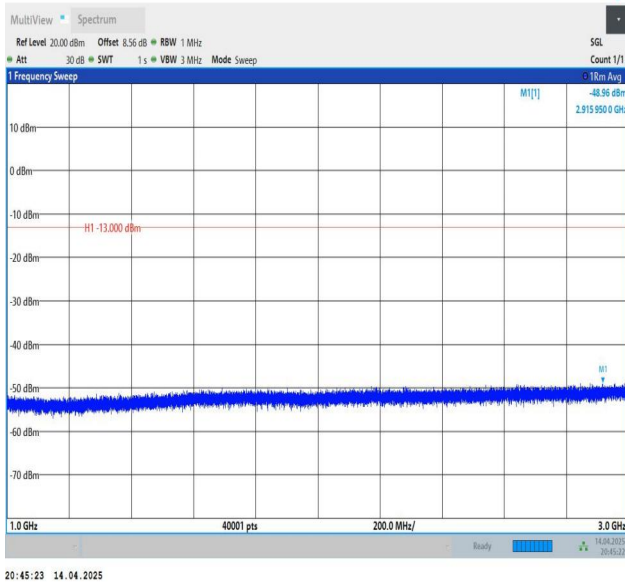
Band26(824-849)-15MHz-QPSK-26915-1RB#74-1000~3000-PAS
