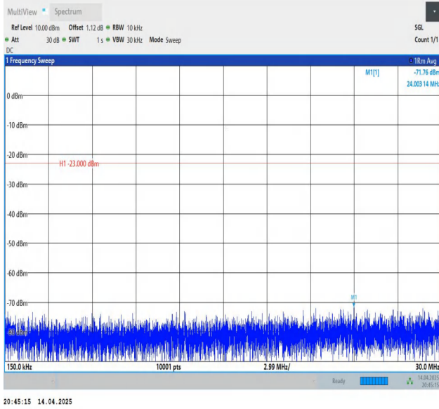
Band26(824-849)-15MHz-QPSK-26915-1RB#74-0.15~30-PASS
