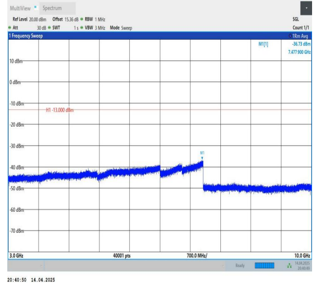
Band26(824-849)-5MHz-QPSK-27015-1RB#24-3000~10000-PASS
