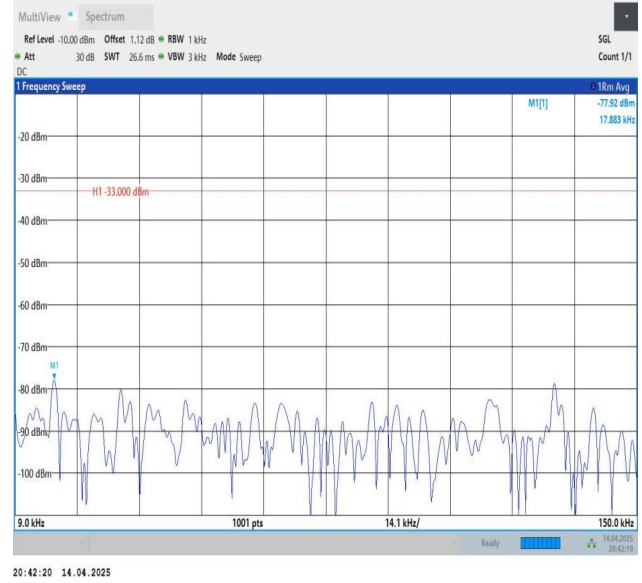
Band26(824-849)-10MHz-QPSK-26915-1RB#49-0.009~0.15-PASS
