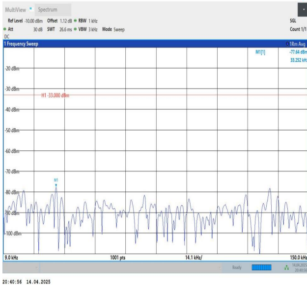
Band26(824-849)-10MHz-QPSK-26840-1RB#0-0.009~0.15-PASS
