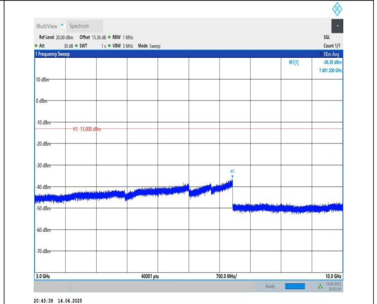
Band26(824-849)-10MHz-QPSK-26990-1RB#49-3000~10000-PAS
