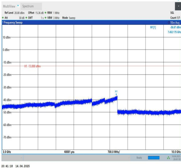
Band26(824-849)-10MHz-QPSK-26840-1RB#0-3000~10000-PAS
