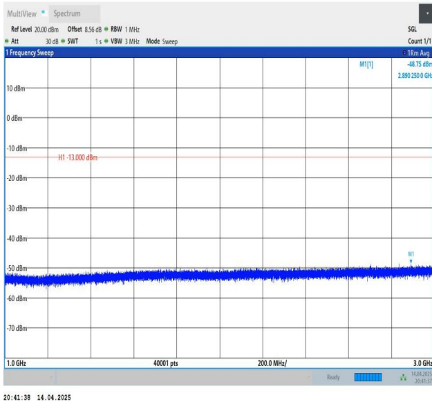
Band26(824-849)-10MHz-QPSK-26840-1RB#49-1000~3000-PAS
