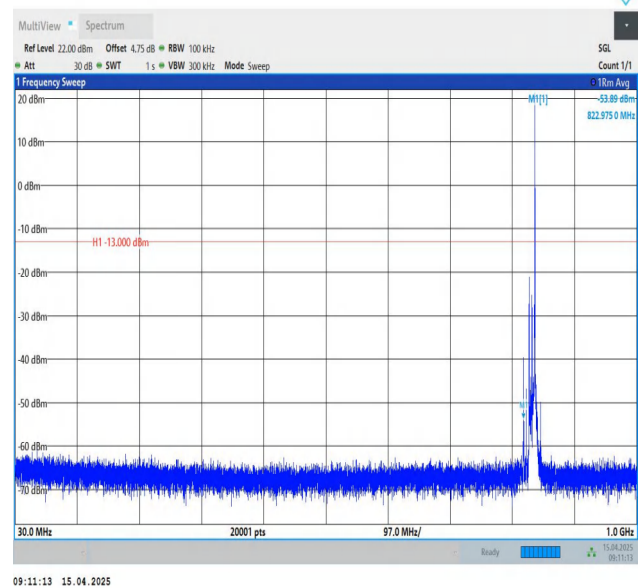
Band26(824-849)-10MHz-QPSK-26915-1RB#49-30~1000-PASS
