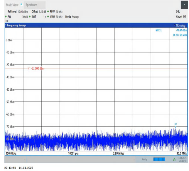
Band26(824-849)-15MHz-QPSK-26865-1RB#0-0.15~30-PASS
