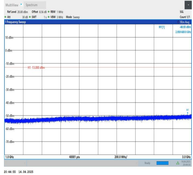
Band26(824-849)-15MHz-QPSK-26915-1RB#0-1000~3000-PASS
