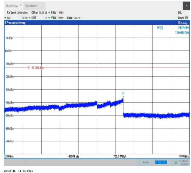
Band26(824-849)-10MHz-QPSK-26840-1RB#49-3000~10000-PAS
