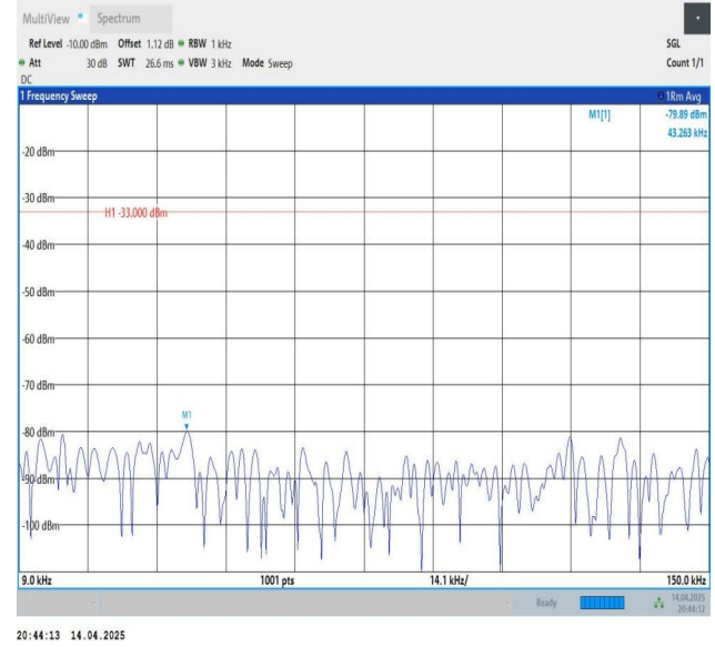
Band26(824-849)-15MHz-QPSK-26865-1RB#74-0.009~0.15-PASS
