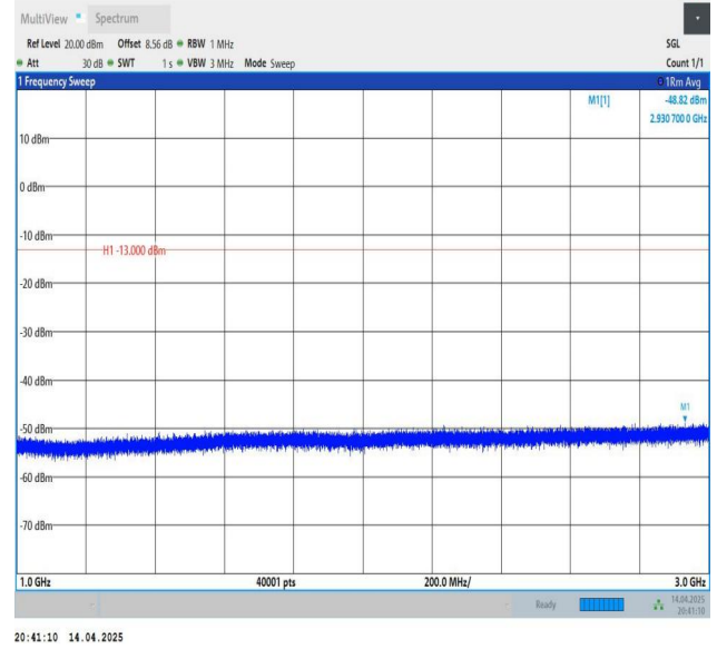
Band26(824-849)-10MHz-QPSK-26840-1RB#0-1000~3000-PASS
