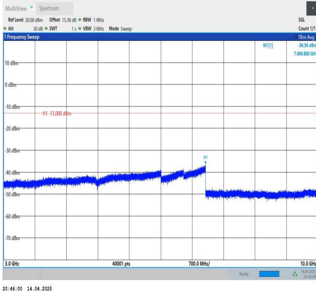
Band26(824-849)-15MHz-QPSK-26965-1RB#0-3000~10000-PAS S
