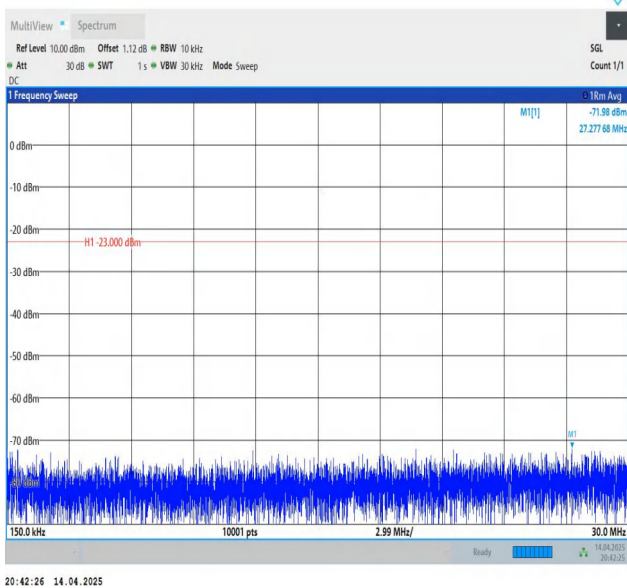
Band26(824-849)-10MHz-QPSK-26915-1RB#49-0.15~30-PASS
