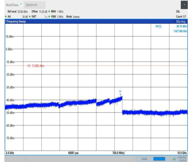
Band26(824-849)-10MHz-QPSK-26915-1RB#49-3000~10000-PAS
