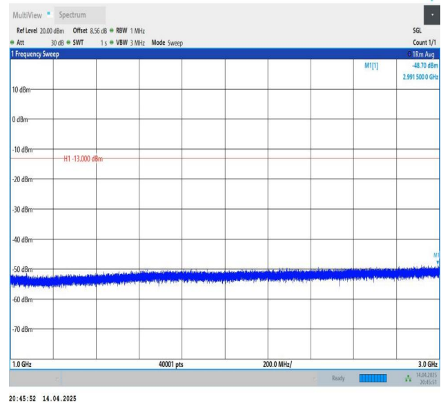
Band26(824-849)-15MHz-QPSK-26965-1RB#0-1000~3000-PASS
