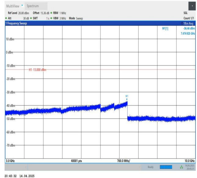
Band26(824-849)-15MHz-QPSK-26915-1RB#74-3000~10000-PAS
