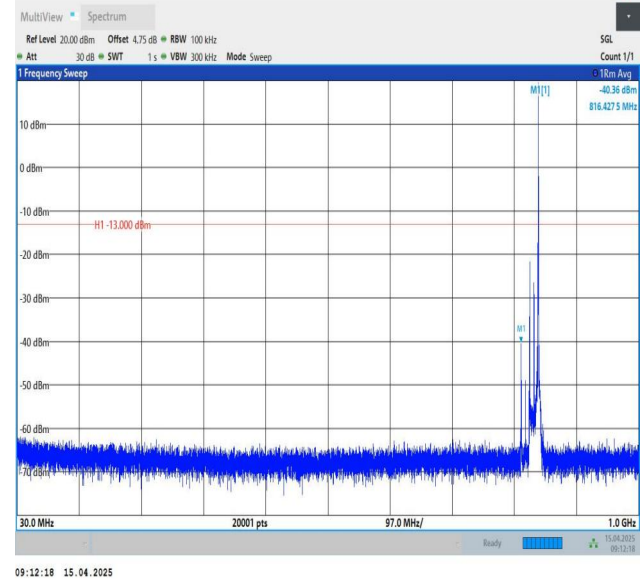
Band26(824-849)-15MHz-QPSK-26915-1RB#74-30~1000-PASS
