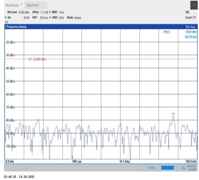
Band26(824-849)-15MHz-QPSK-26965-1RB#74-0.009~0.15-PASS
