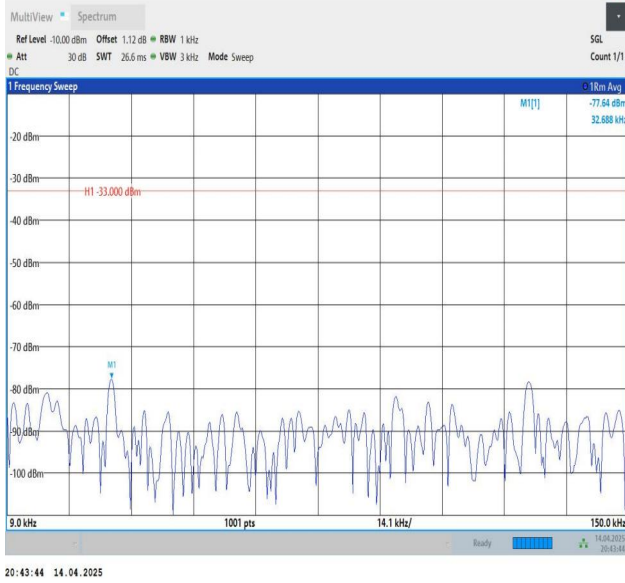
Band26(824-849)-15MHz-QPSK-26865-1RB#0-0.009~0.15-PASS
