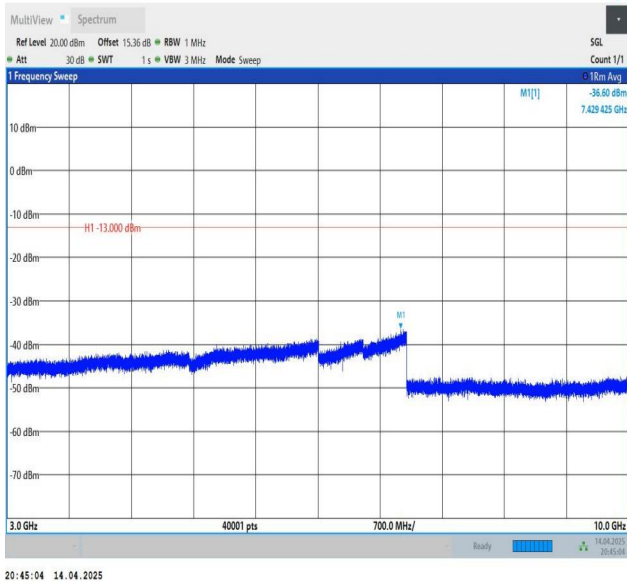
Band26(824-849)-15MHz-QPSK-26915-1RB#0-3000~10000-PAS
