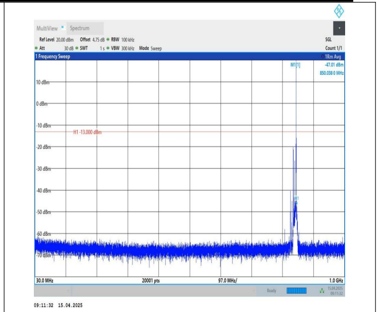
Band26(824-849)-10MHz-QPSK-26990-1RB#49-30~1000-PASS
