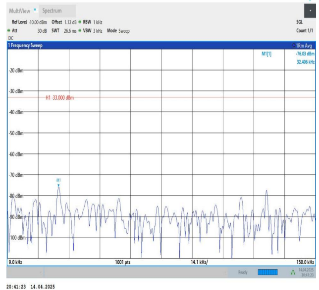
Band26(824-849)-10MHz-QPSK-26840-1RB#49-0.009~0.15-PASS
