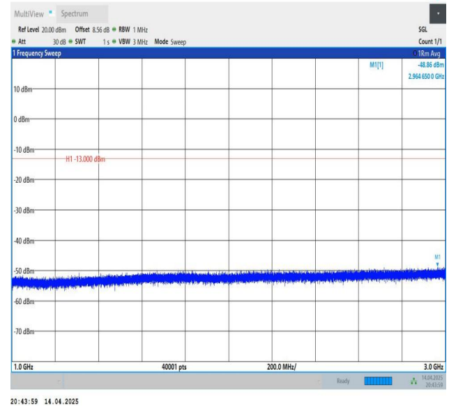
Band26(824-849)-15MHz-QPSK-26865-1RB#0-1000~3000-PASS
