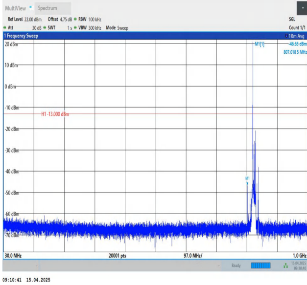
Band26(824-849)-10MHz-QPSK-26840-1RB#0-30~1000-PASS
