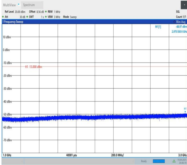
Band26(824-849)-15MHz-QPSK-26965-1RB#74-1000~3000-PAS
