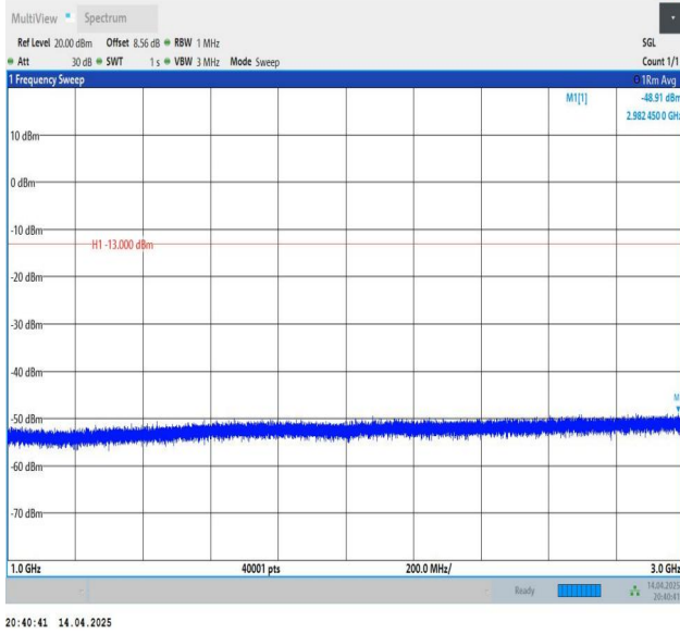
Band26(824-849)-5MHz-QPSK-27015-1RB#24-1000~3000-PASS
