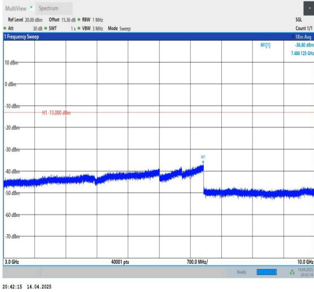
Band26(824-849)-10MHz-QPSK-26915-1RB#0-3000~10000-PAS S
