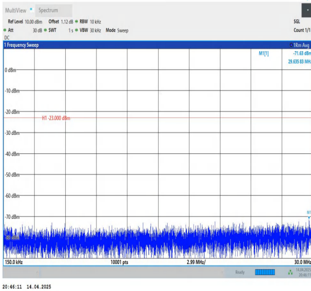
Band26(824-849)-15MHz-QPSK-26965-1RB#74-0.15~30-PASS
