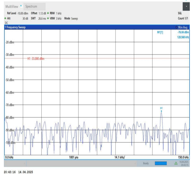
Band26(824-849)-10MHz-QPSK-26990-1RB#49-0.009~0.15-PASS
