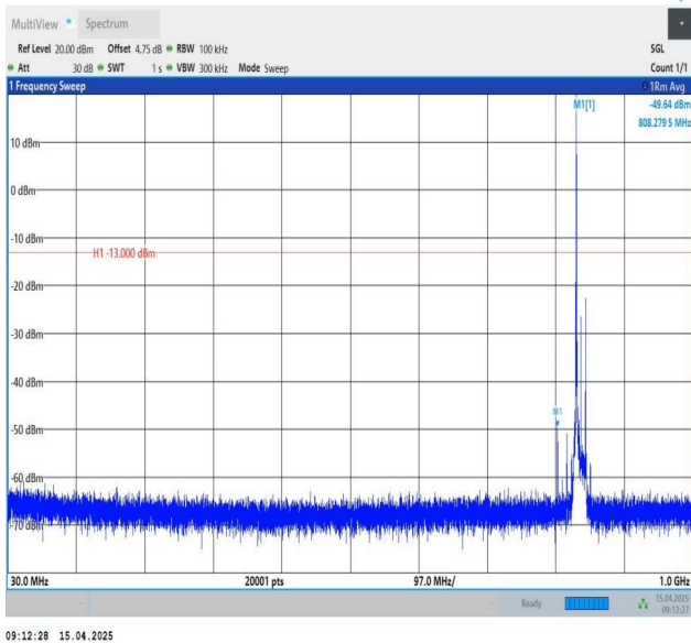
Band26(824-849)-15MHz-QPSK-26965-1RB#0-30~1000-PASS
