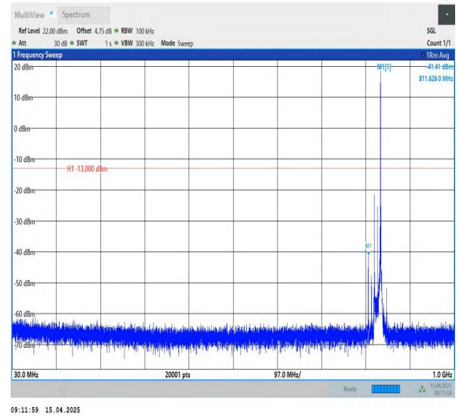
Band26(824-849)-15MHz-QPSK-26865-1RB#74-30~1000-PASS
