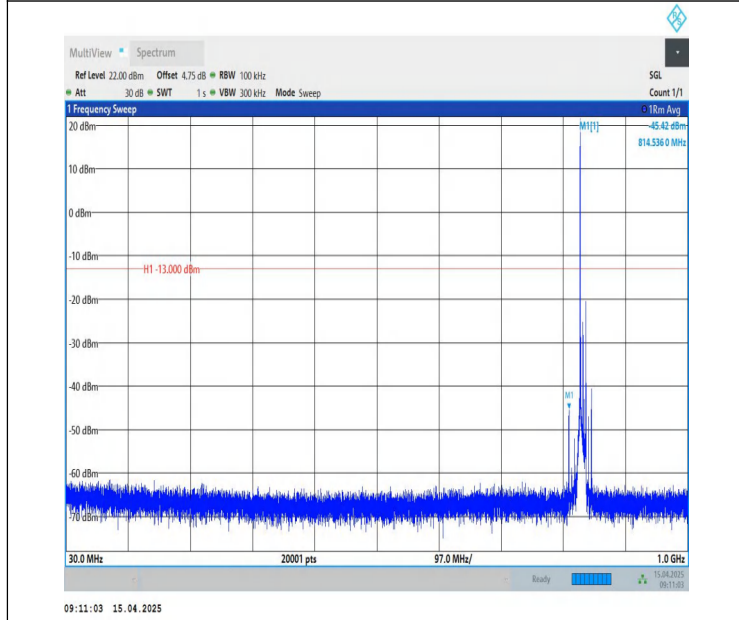
Band26(824-849)-10MHz-QPSK-26915-1RB#0-30~1000-PASS
