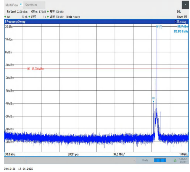
Band26(824-849)-10MHz-QPSK-26840-1RB#49-30~1000-PASS
