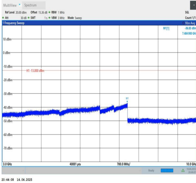
Band26(824-849)-15MHz-QPSK-26865-1RB#0-3000~10000-PAS S
