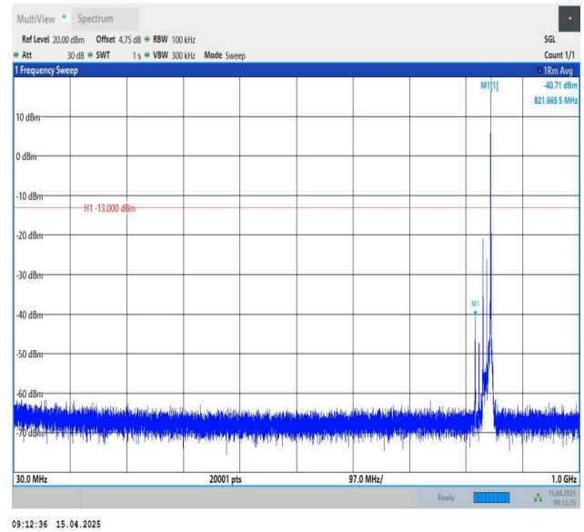
Band26(824-849)-15MHz-QPSK-26965-1RB#74-30~1000-PASS
