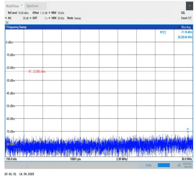
Band26(824-849)-10MHz-QPSK-26840-1RB#0-0.15~30-PASS
