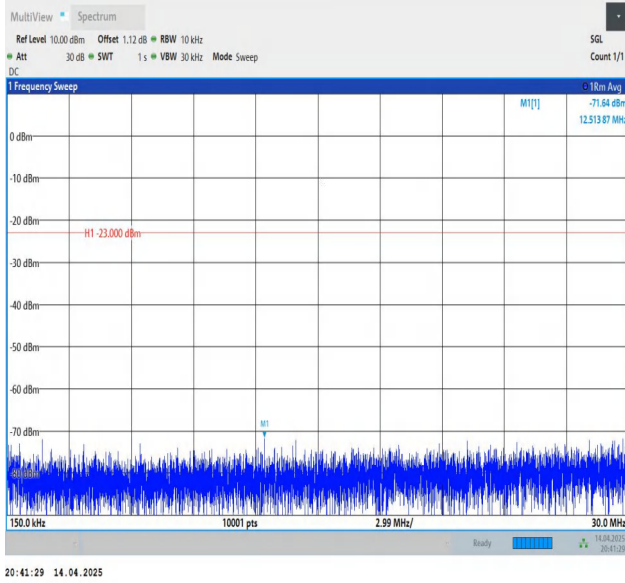
Band26(824-849)-10MHz-QPSK-26840-1RB#49-0.15~30-PASS
