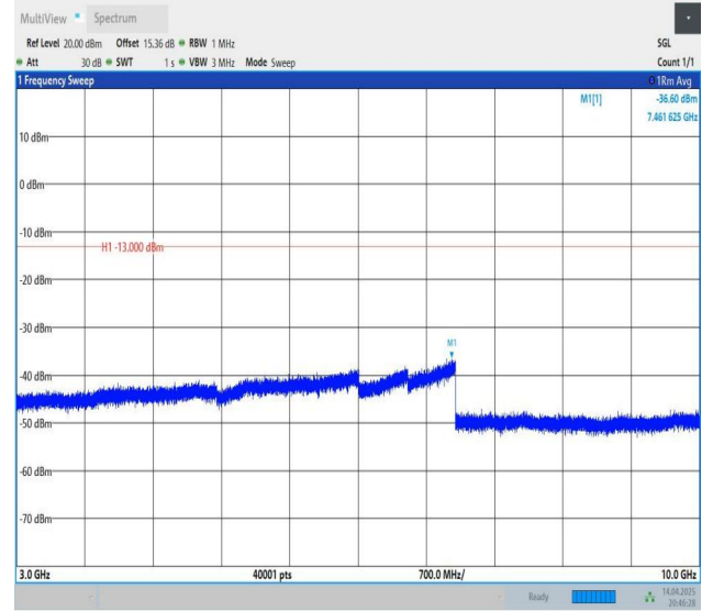
Band26(824-849)-15MHz-QPSK-26965-1RB#74-3000~10000-PAS
