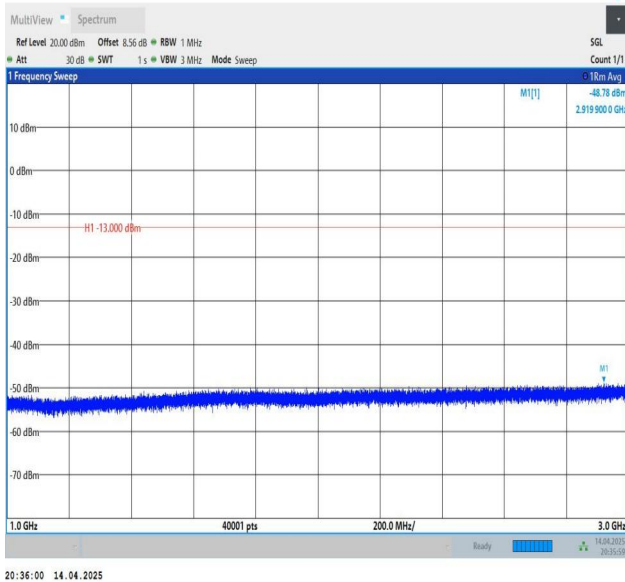
Band26(824-849)-3MHz-QPSK-26805-1RB#14-1000~3000-PASS
