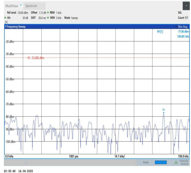
Band26(824-849)-3MHz-QPSK-26805-1RB#14-0.009~0.15-PASS
