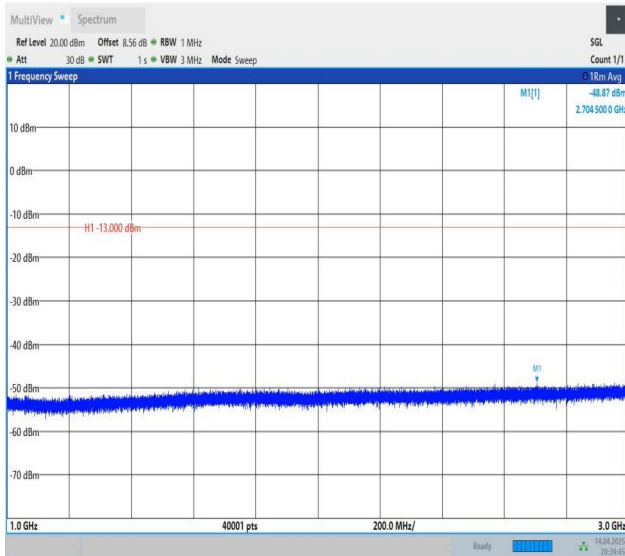
Band26(824-849)-5MHz-QPSK-26915-1RB#24-1000~3000-PASS
