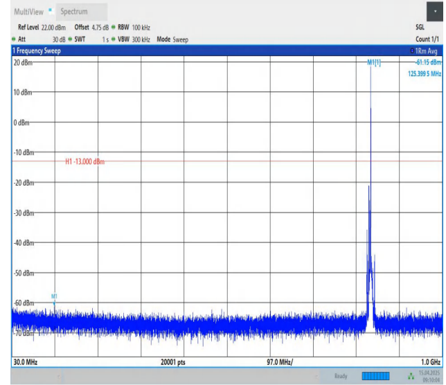
Band26(824-849)-5MHz-QPSK-26915-1RB#24-30~1000-PASS
