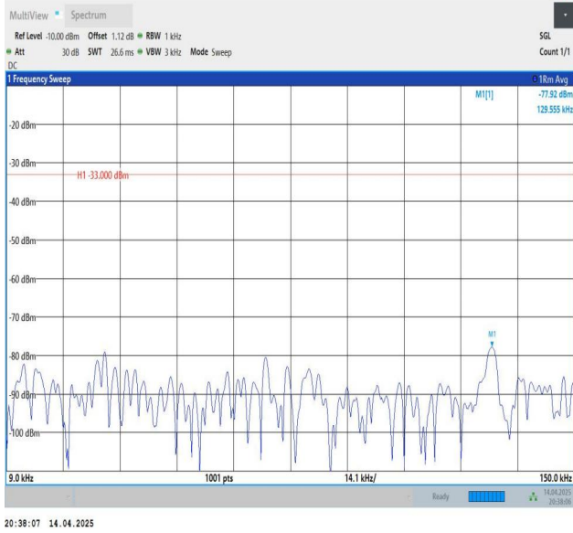
Band26(824-849)-5MHz-QPSK-26815-1RB#0-0.009~0.15-PASS
