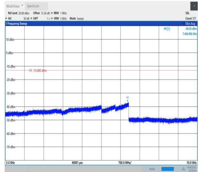
Band26(824-849)-5MHz-QPSK-26915-1RB#24-3000~10000-PASS
