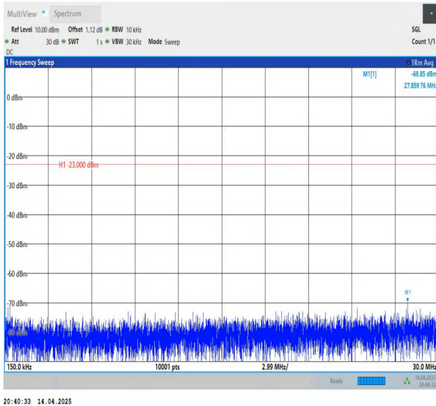
Band26(824-849)-5MHz-QPSK-27015-1RB#24-0.15~30-PASS
