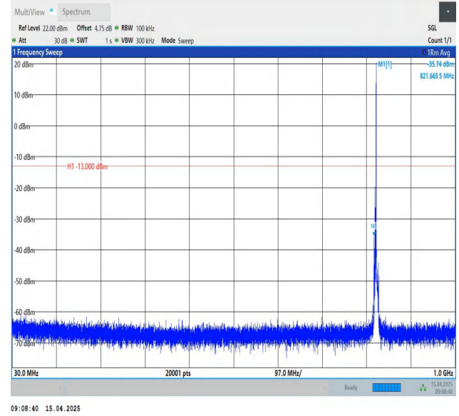
Band26(824-849)-3MHz-QPSK-26805-1RB#14-30~1000-PASS
