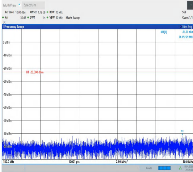
Band26(824-849)-5MHz-QPSK-26915-1RB#24-0.15~30-PASS
