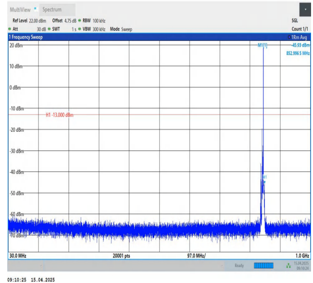
Band26(824-849)-5MHz-QPSK-27015-1RB#24-30~1000-PASS
