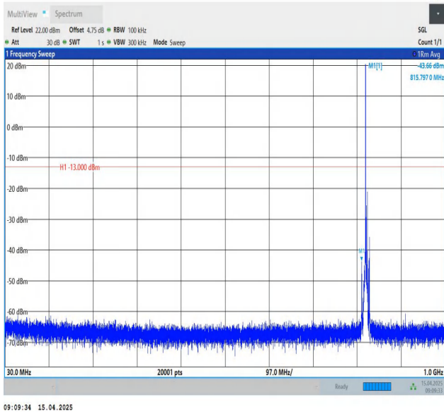
Band26(824-849)-5MHz-QPSK-26815-1RB#0-30~1000-PASS
