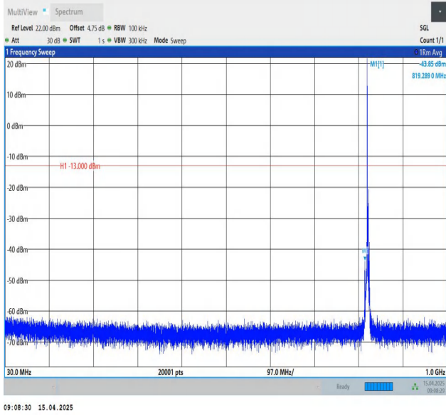
Band26(824-849)-3MHz-QPSK-26805-1RB#0-30~1000-PASS
