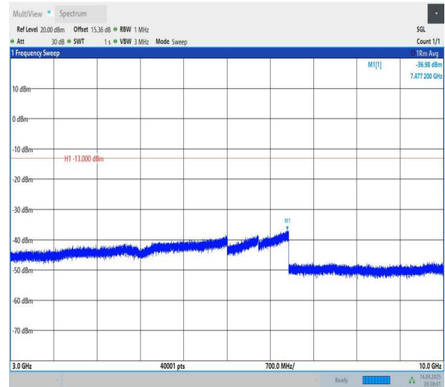
Band26(824-849)-3MHz-QPSK-27025-1RB#14-3000~10000-PASS
