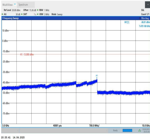
Band26(824-849)-3MHz-QPSK-26805-1RB#0-3000~10000-PASS
