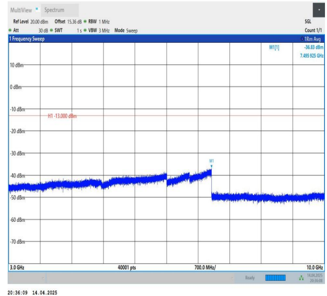
Band26(824-849)-3MHz-QPSK-26805-1RB#14-3000~10000-PASS
