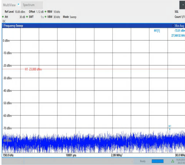
Band26(824-849)-3MHz-QPSK-27025-1RB#14-0.15~30-PASS
