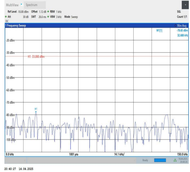
Band26(824-849)-5MHz-QPSK-27015-1RB#24-0.009~0.15-PASS
