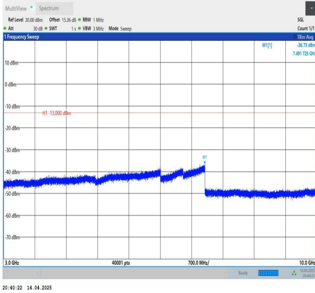
Band26(824-849)-5MHz-QPSK-27015-1RB#0-3000~10000-PASS
