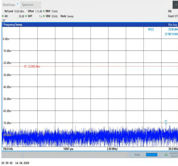
Band26(824-849)-3MHz-QPSK-26805-1RB#14-0.15~30-PASS
