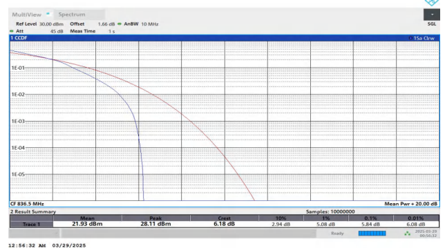
Band26(824-849)-10MHz-16QAM-26915-27RB#0-PASS
