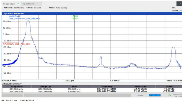
Band26(824-849)-10MHz-QPSK-26840-1RB#0-PASS
