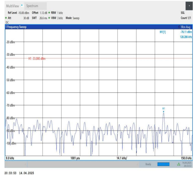
Band26(824-849)-1.4MHz-QPSK-26915-1RB#5-0.009~0.15-PASS
