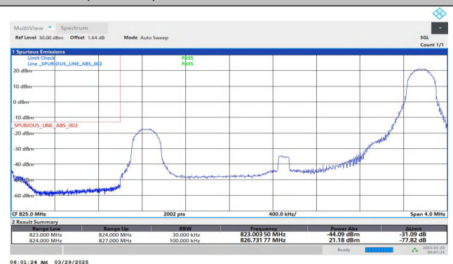
Band26(824-849)-1.4MHz-QPSK-27033-6RB#0-PASS
