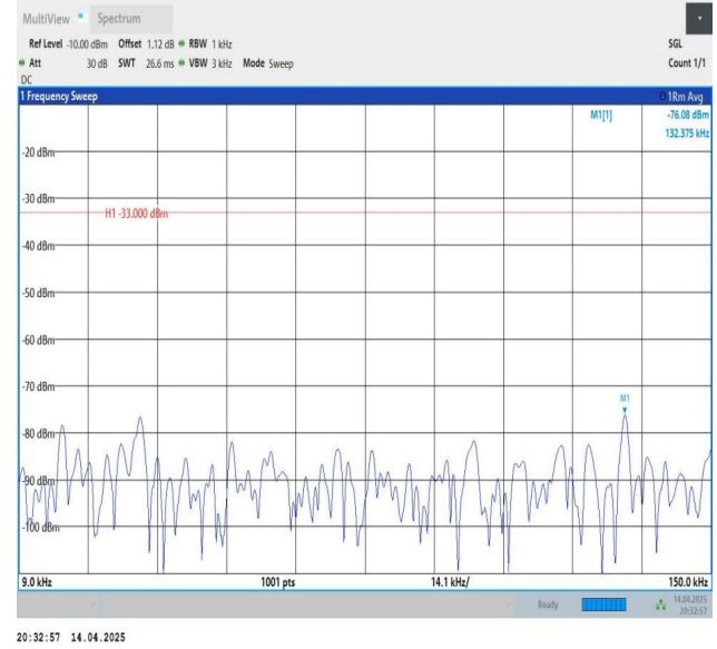
Band26(824-849)-1.4MHz-QPSK-26797-1RB#5-0.009~0.15-PASS
