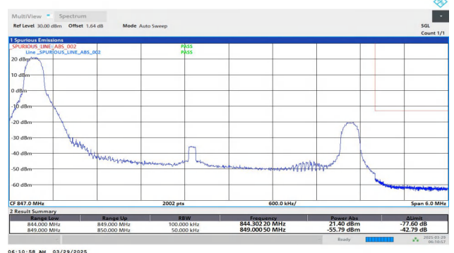
Band26(824-849)-5MHz-QPSK-27015-1RB#0-PASS
