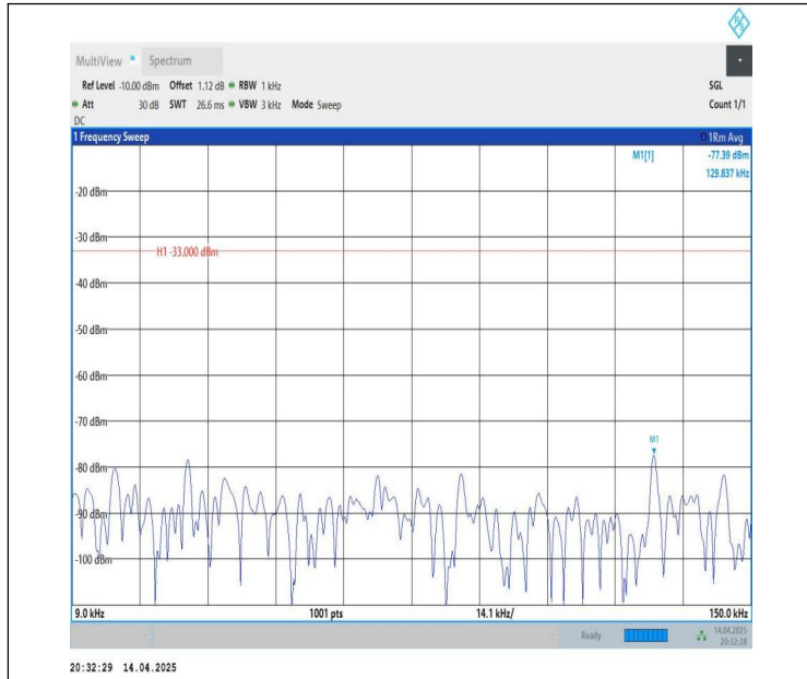
Band26(824-849)-1.4MHz-QPSK-26797-1RB#0-0.009~0.15-PASS
