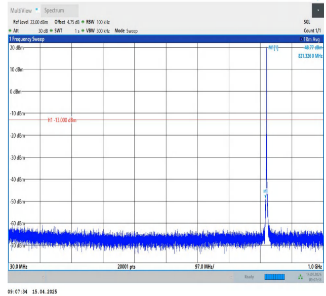
Band26(824-849)-1.4MHz-QPSK-26797-1RB#5-30~1000-PASS
