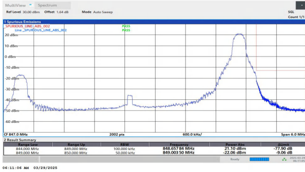
Band26(824-849)-5MHz-QPSK-27015-1RB#24-PASS
