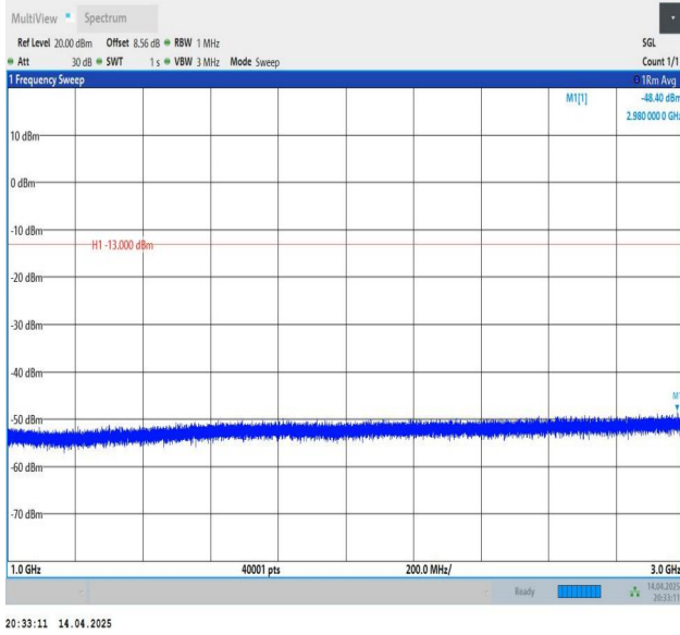
Band26(824-849)-1.4MHz-QPSK-26797-1RB#5-1000~3000-PASS
