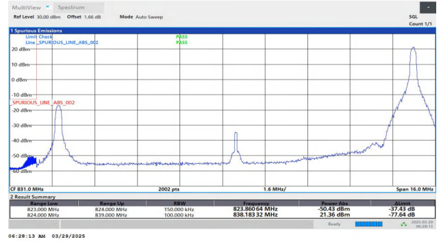
Band26(824-849)-15MHz-QPSK-26865-1RB#74-PASS
