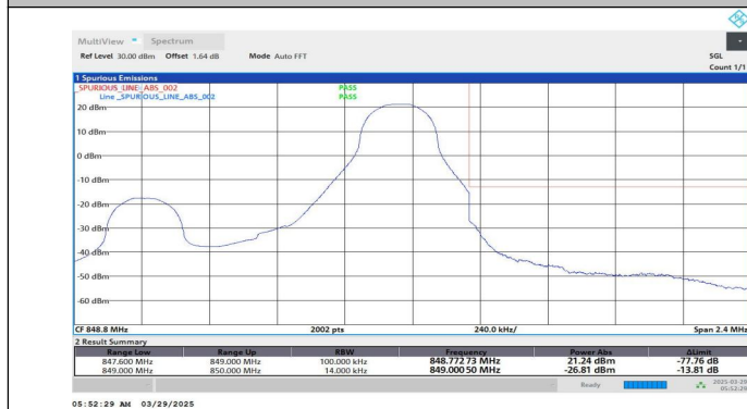
Band26(824-849)-1.4MHz-QPSK-27033-1RB#5-PASS
