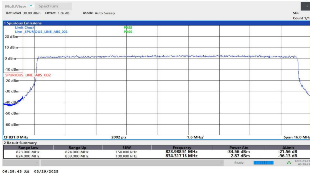
Band26(824-849)-15MHz-QPSK-26865-75RB#0-PASS
