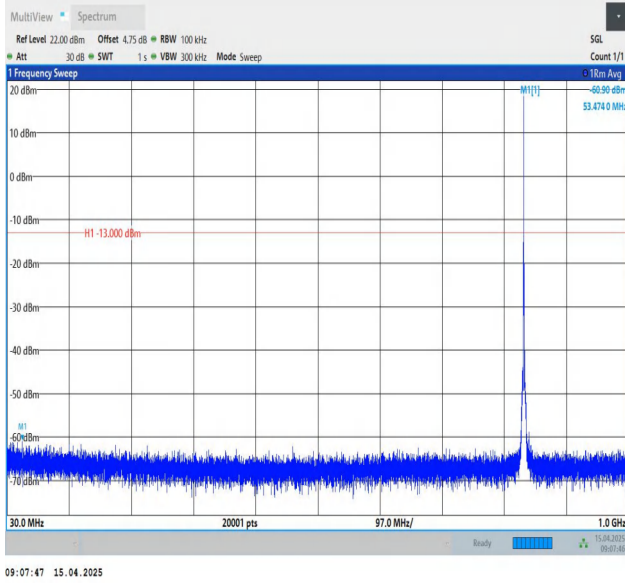
Band26(824-849)-1.4MHz-QPSK-26915-1RB#0-30~1000-PASS
