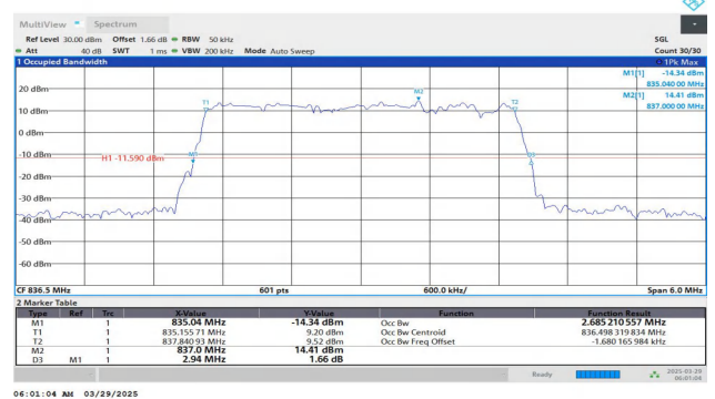
Band26(824-849)-3MHz-16QAM-26915-15RB#0-PASS
