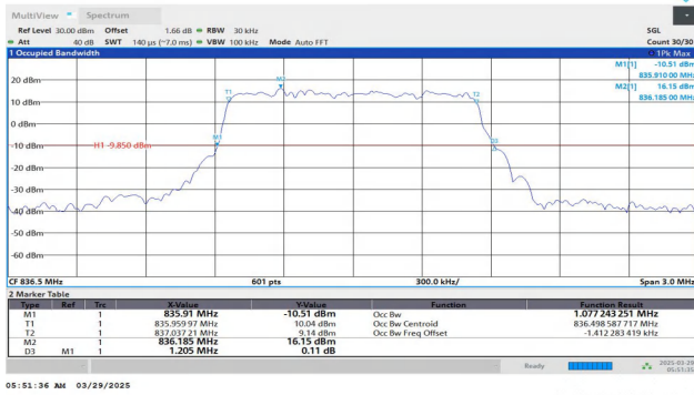
Band26(824-849)-1.4MHz-QPSK-26915-6RB#0-PASS
