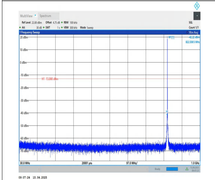
Band26(824-849)-1.4MHz-QPSK-26797-1RB#0-30~1000-PASS
