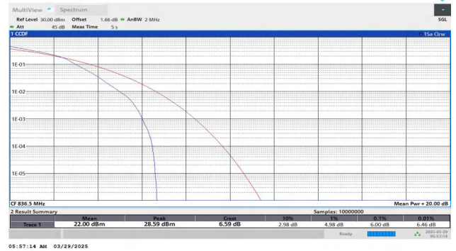
Band26(824-849)-1.4MHz-16QAM-26915-6RB#0-PASS
