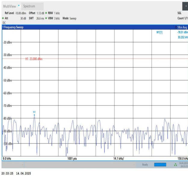
Band26(824-849)-1.4MHz-QPSK-26915-1RB#0-0.009~0.15-PASS
