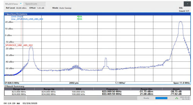
Band26(824-849)-10MHz-QPSK-26840-1RB#49-PASS
