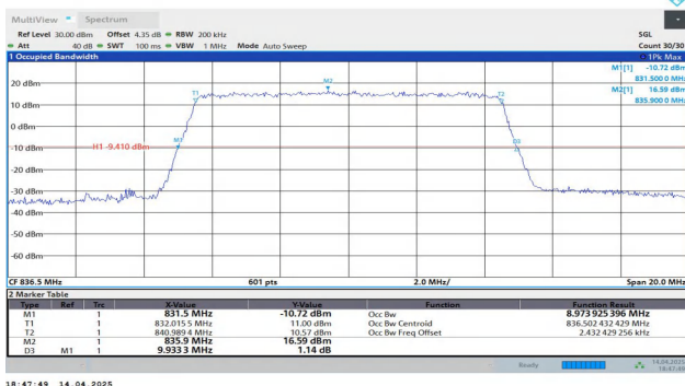
Band26(824-849)-10MHz-QPSK-26915-50RB#0-PASS
