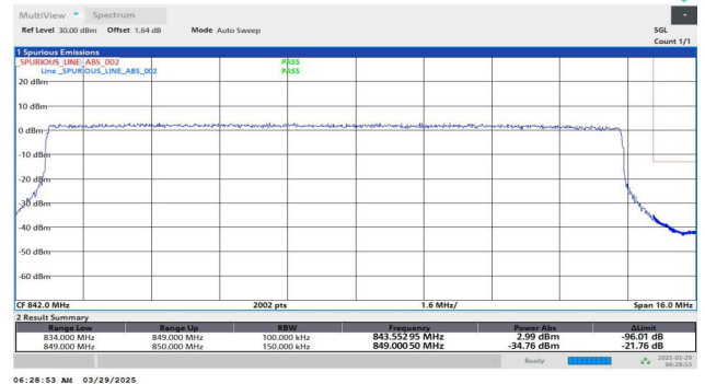
Band26(824-849)-15MHz-QPSK-26965-75RB#0-PASS
