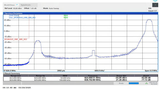
Band26(824-849)-5MHz-QPSK-26815-1RB#24-PASS
