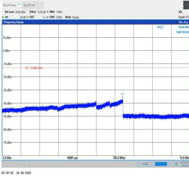
Band26(824-849)-1.4MHz-QPSK-26797-1RB#0-3000~10000-PAS S
