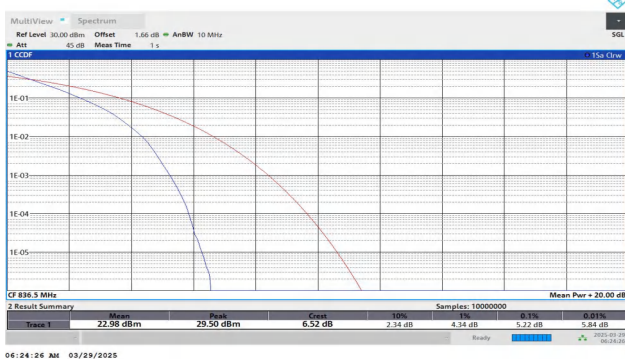
Band26(824-849)-10MHz-QPSK-26915-50RB#0-PASS
