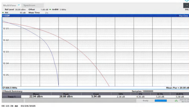
Band26(824-849)-5MHz-QPSK-26915-25RB#0-PASS
