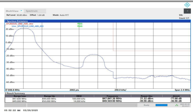
Band26(824-849)-1.4MHz-QPSK-27033-1RB#0-PASS
