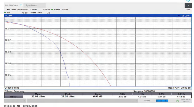
Band26(824-849)-5MHz-16QAM-26915-25RB#0-PASS
