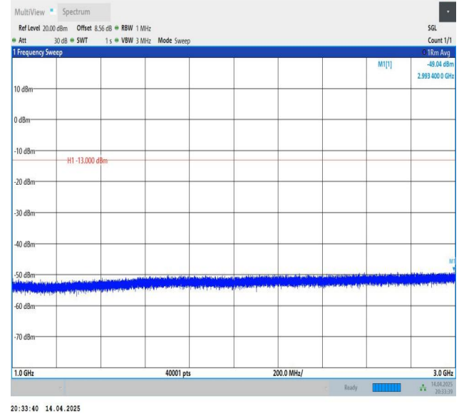
Band26(824-849)-1.4MHz-QPSK-26915-1RB#0-1000~3000-PASS
