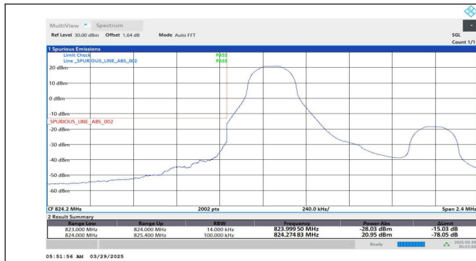
Band26(824-849)-1.4MHz-QPSK-26797-1RB#0-PASS
