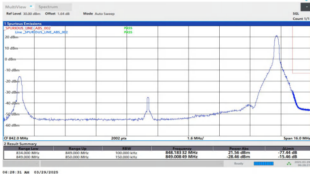
Band26(824-849)-15MHz-QPSK-26965-1RB#74-PASS
