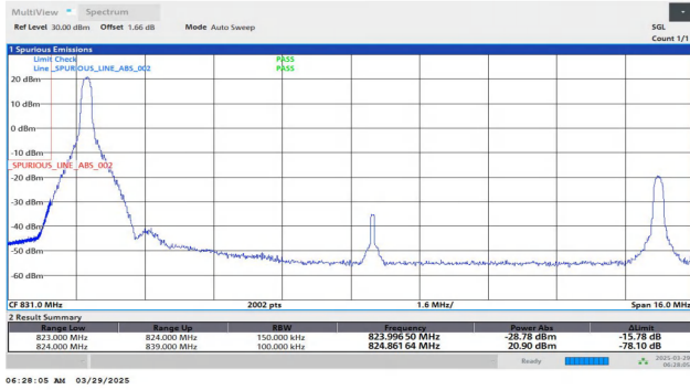
Band26(824-849)-15MHz-QPSK-26865-1RB#0-PASS
