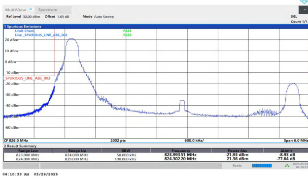
Band26(824-849)-5MHz-QPSK-26815-1RB#0-PASS
