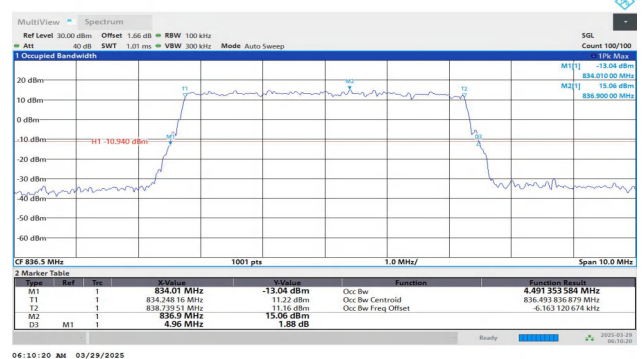
Band26(824-849)-5MHz-16QAM-26915-25RB#0-PASS
