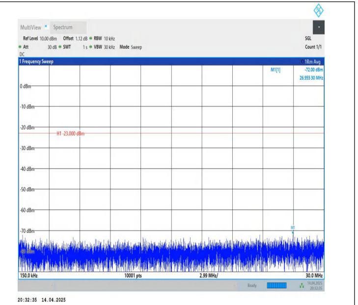
Band26(824-849)-1.4MHz-QPSK-26797-1RB#0-0.15~30-PASS
