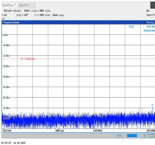
Band26(824-849)-1.4MHz-QPSK-26797-1RB#5-0.15~30-PASS
