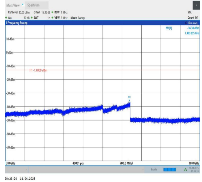
Band26(824-849)-1.4MHz-QPSK-26797-1RB#5-3000~10000-PASS S
