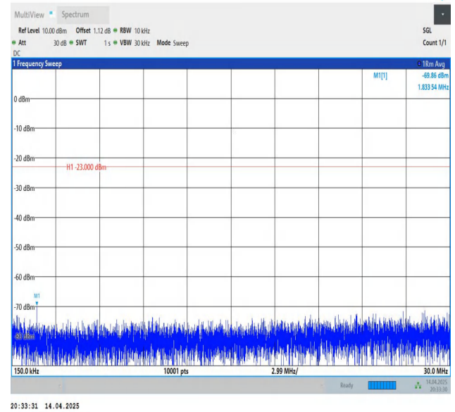
Band26(824-849)-1.4MHz-QPSK-26915-1RB#0-0.15~30-PASS
