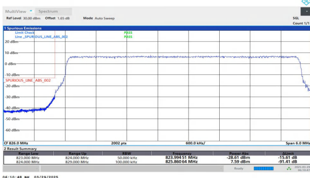
Band26(824-849)-5MHz-QPSK-26815-25RB#0-PASS
