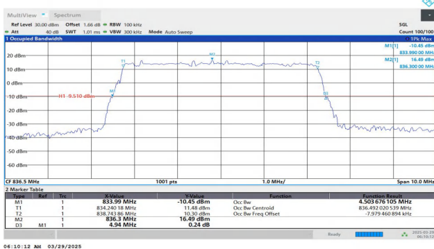
Band26(824-849)-5MHz-QPSK-26915-25RB#0-PASS
