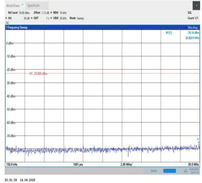
Band26(814-824)-10MHz-QPSK-26740-1RB#0-0.15~30-PASS
