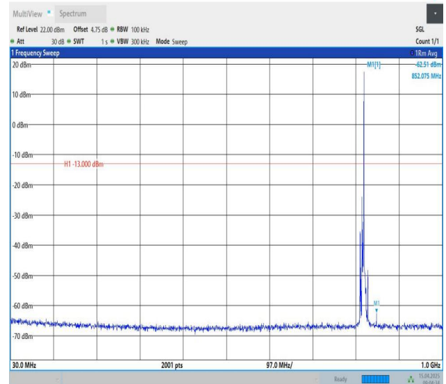
Band26(814-824)-5MHz-QPSK-26765-1RB#24-30~1000-PASS
