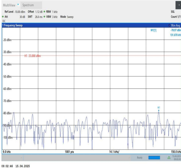
Band26(814-824)-3MHz-QPSK-26775-1RB#0-0.009~0.15-PASS
