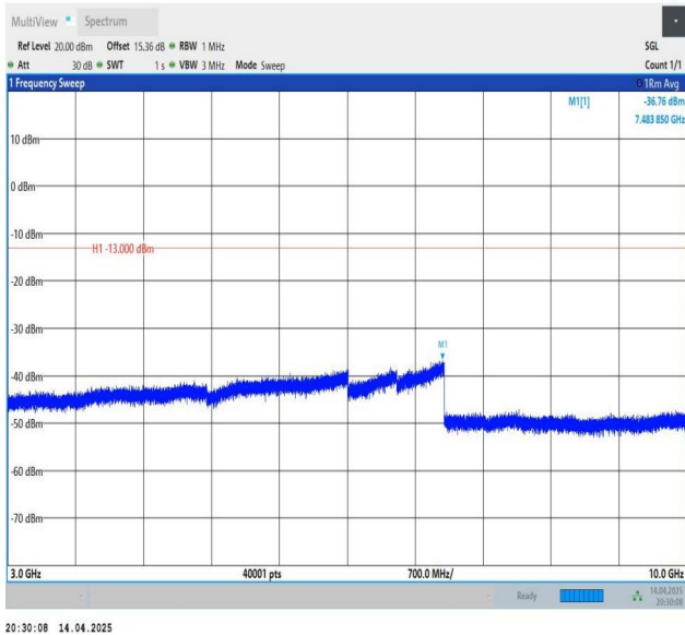
Band26(814-824)-5MHz-QPSK-26740-1RB#0-3000~10000-PASS
