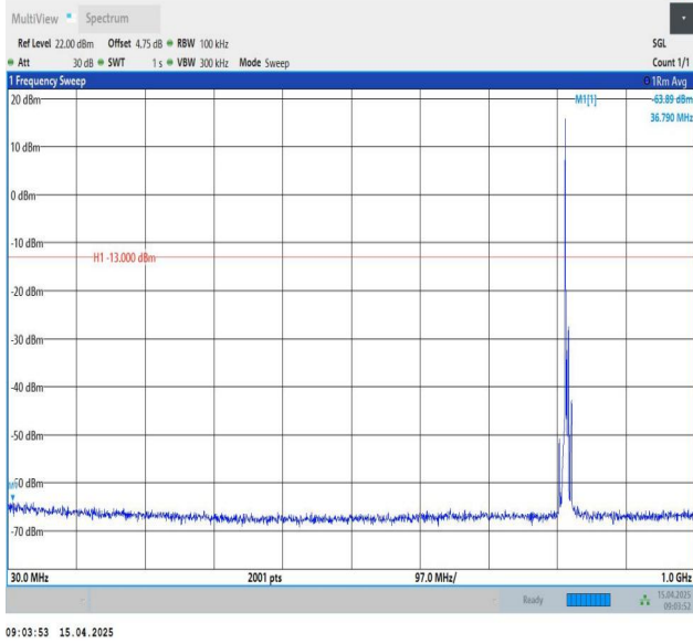
Band26(814-824)-5MHz-QPSK-26740-1RB#0-30~1000-PASS
