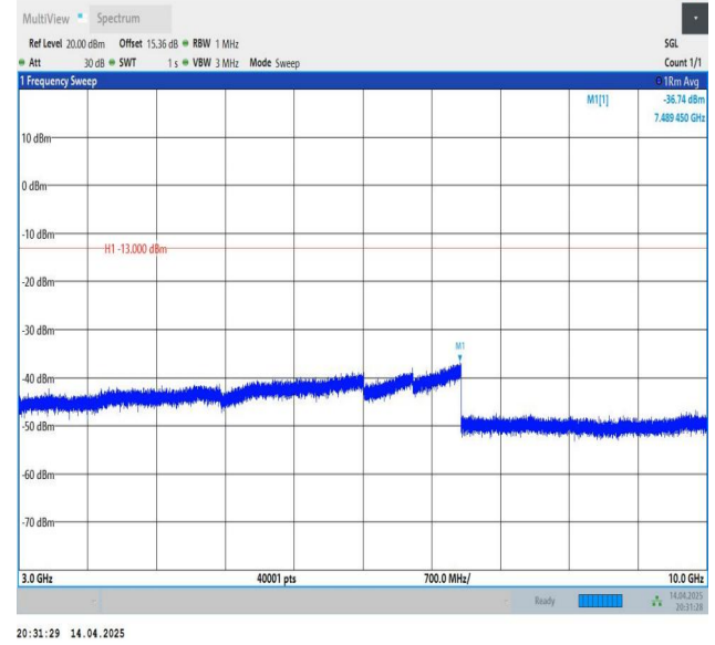
Band26(814-824)-5MHz-QPSK-26765-1RB#24-3000~10000-PASS
