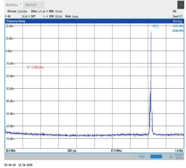
Band26(814-824)-5MHz-QPSK-26740-1RB#24-30~1000-PASS
