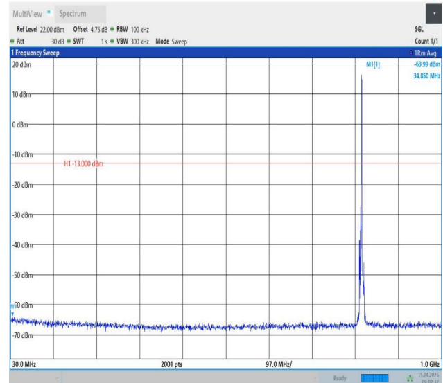
Band26(814-824)-3MHz-QPSK-26740-1RB#14-30~1000-PASS
