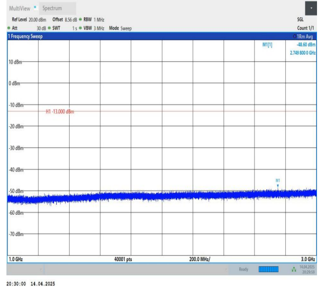
Band26(814-824)-5MHz-QPSK-26740-1RB#0-1000~3000-PASS
