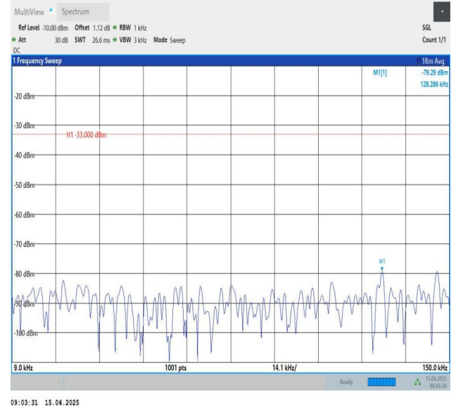
Band26(814-824)-5MHz-QPSK-26715-1RB#24-0.009~0.15-PASS
