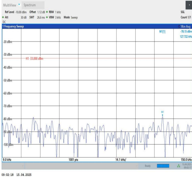
Band26(814-824)-3MHz-QPSK-26740-1RB#0-0.009~0.15-PASS
