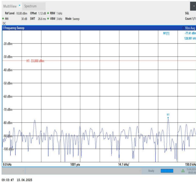
Band26(814-824)-5MHz-QPSK-26740-1RB#0-0.009~0.15-PASS
