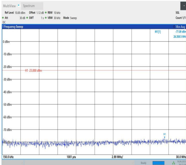
Band26(814-824)-3MHz-QPSK-26740-1RB#14-0.15~30-PASS
