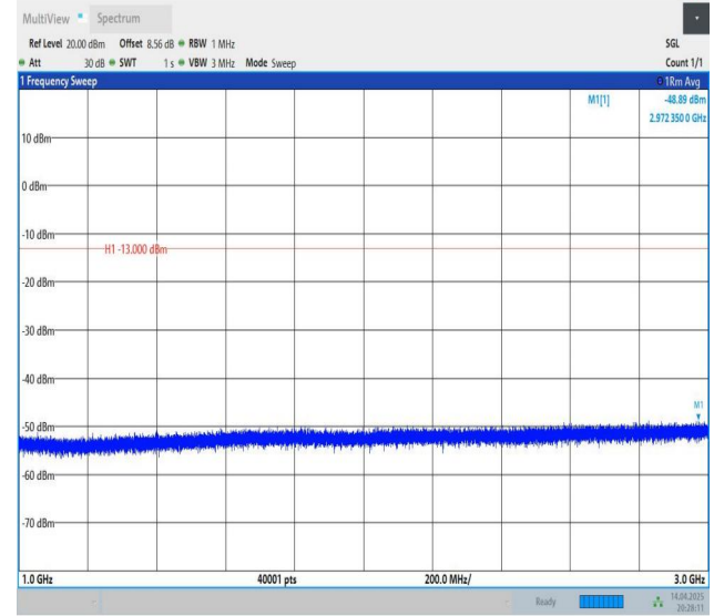
Band26(814-824)-3MHz-QPSK-26775-1RB#0-1000~3000-PASS
