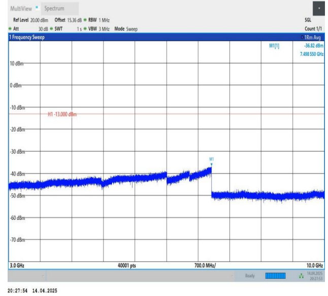
Band26(814-824)-3MHz-QPSK-26740-1RB#14-3000~10000-PASS
