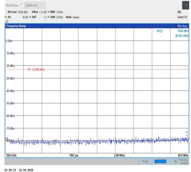
Band26(814-824)-3MHz-QPSK-26775-1RB#0-0.15~30-PASS
