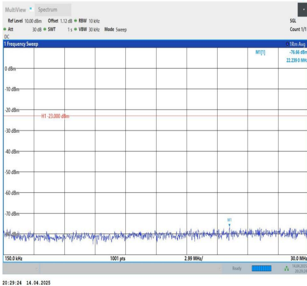
Band26(814-824)-5MHz-QPSK-26715-1RB#24-0.15~30-PASS
