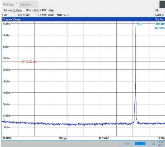
Band26(814-824)-3MHz-QPSK-26775-1RB#0-30~1000-PASS
