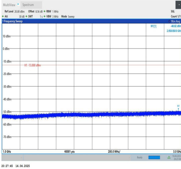
Band26(814-824)-3MHz-QPSK-26740-1RB#14-1000~3000-PASS
