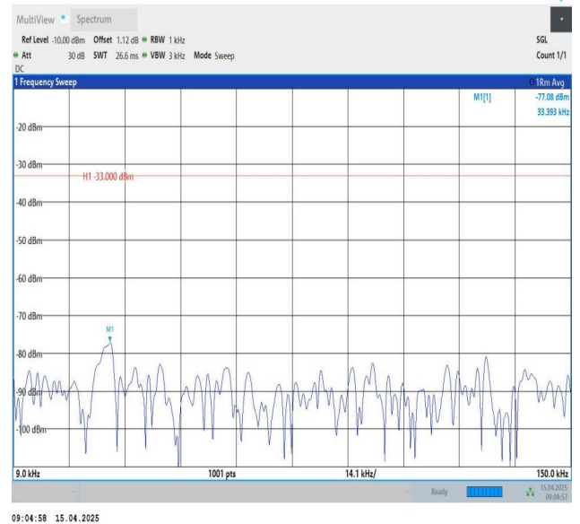
Band26(814-824)-10MHz-QPSK-26740-1RB#49-0.009~0.15-PASS
