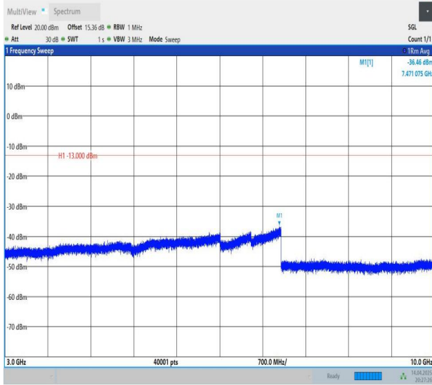
Band26(814-824)-3MHz-QPSK-26740-1RB#0-3000~10000-PASS
