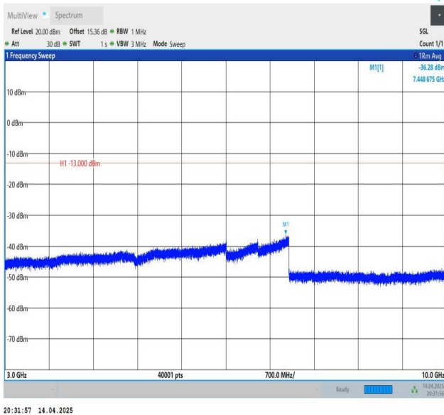
Band26(814-824)-10MHz-QPSK-26740-1RB#0-3000~10000-PAS
