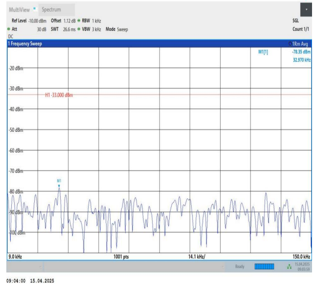
Band26(814-824)-5MHz-QPSK-26740-1RB#24-0.009~0.15-PASS
