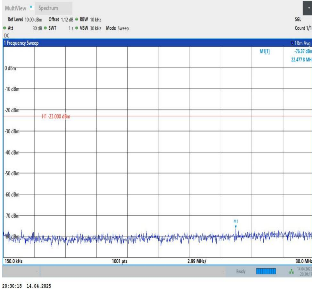
Band26(814-824)-5MHz-QPSK-26740-1RB#24-0.15~30-PASS
