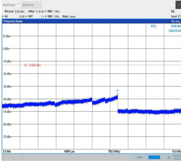
Band26(814-824)-5MHz-QPSK-26765-1RB#0-3000~10000-PASS
