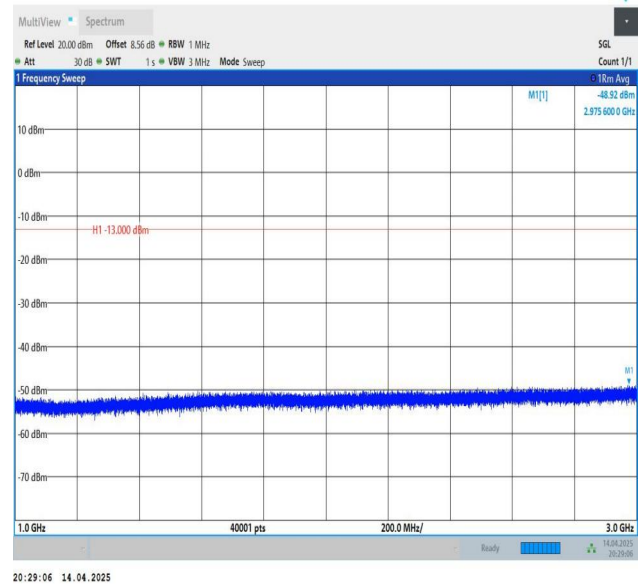
Band26(814-824)-5MHz-QPSK-26715-1RB#0-1000~3000-PASS
