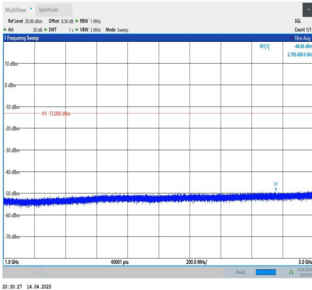
Band26(814-824)-5MHz-QPSK-26740-1RB#24-1000~3000-PASS
