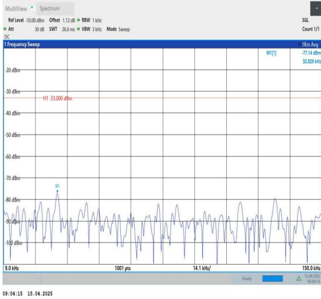
Band26(814-824)-5MHz-QPSK-26765-1RB#0-0.009~0.15-PASS
