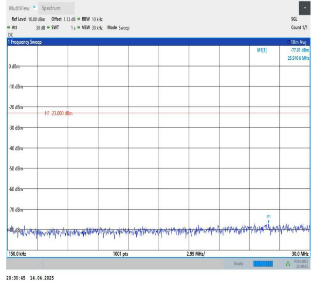
Band26(814-824)-5MHz-QPSK-26765-1RB#0-0.15~30-PASS
