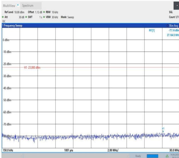
Band26(814-824)-5MHz-QPSK-26765-1RB#24-0.15~30-PASS
