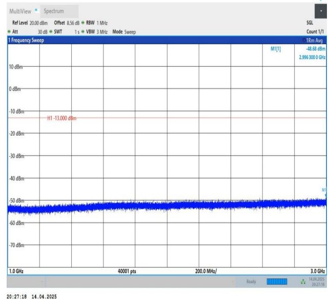
Band26(814-824)-3MHz-QPSK-26740-1RB#0-1000~3000-PASS
