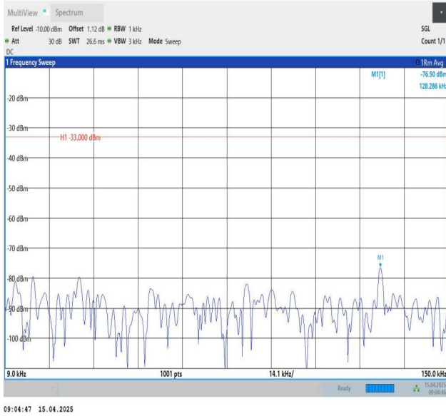
Band26(814-824)-10MHz-QPSK-26740-1RB#0-0.009~0.15-PASS
