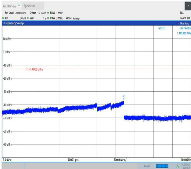
Band26(814-824)-3MHz-QPSK-26775-1RB#0-3000~10000-PASS
