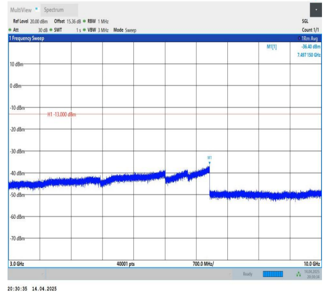
Band26(814-824)-5MHz-QPSK-26740-1RB#24-3000~10000-PASS
