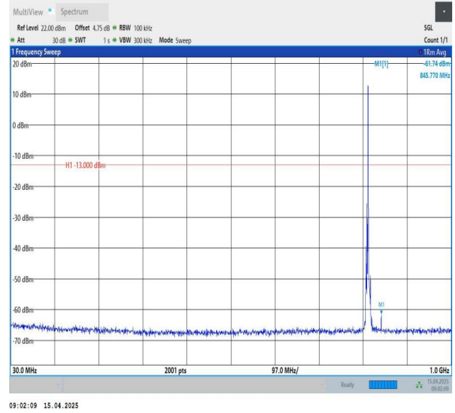
Band26(814-824)-3MHz-QPSK-26705-1RB#14-30~1000-PASS
