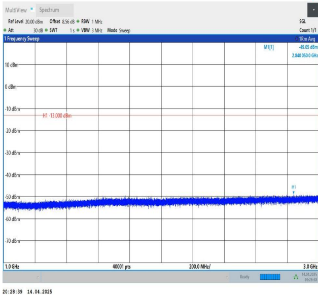
Band26(814-824)-3MHz-QPSK-26775-1RB#14-1000~3000-PASS
