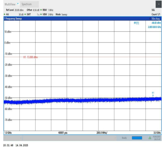
Band26(814-824)-10MHz-QPSK-26740-1RB#0-1000~3000-PASS
