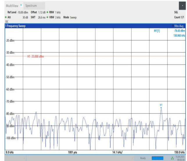
Band26(814-824)-3MHz-QPSK-26775-1RB#14-0.009~0.15-PASS
