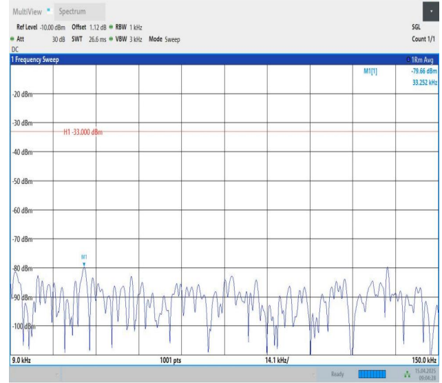
Band26(814-824)-5MHz-QPSK-26765-1RB#24-0.009~0.15-PASS
