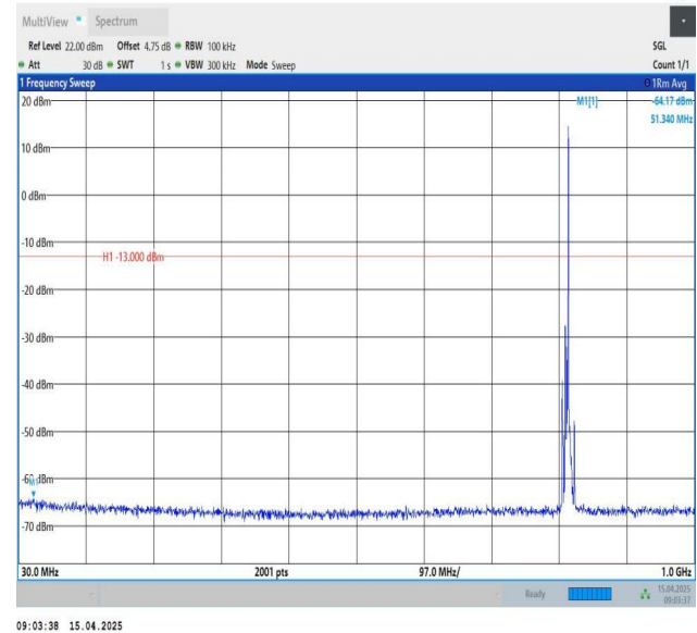
Band26(814-824)-5MHz-QPSK-26715-1RB#24-30~1000-PASS
