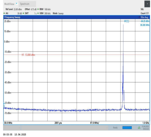
Band26(814-824)-3MHz-QPSK-26775-1RB#14-30~1000-PASS
