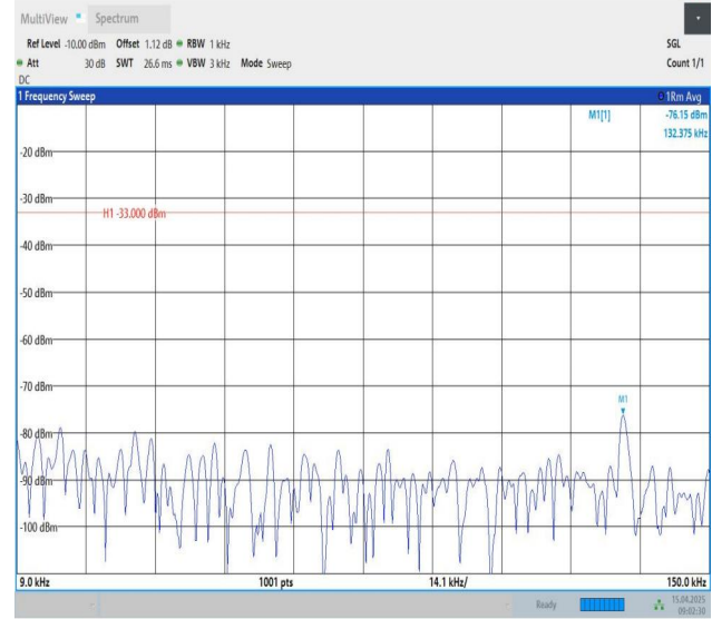
Band26(814-824)-3MHz-QPSK-26740-1RB#14-0.009~0.15-PASS
