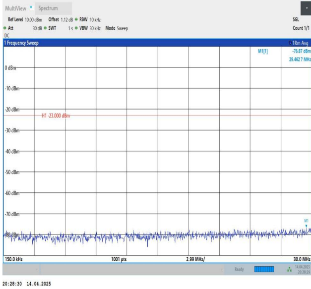
Band26(814-824)-3MHz-QPSK-26775-1RB#14-0.15~30-PASS
