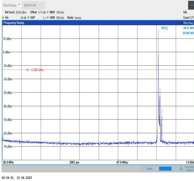
Band26(814-824)-10MHz-QPSK-26740-1RB#0-30~1000-PASS
