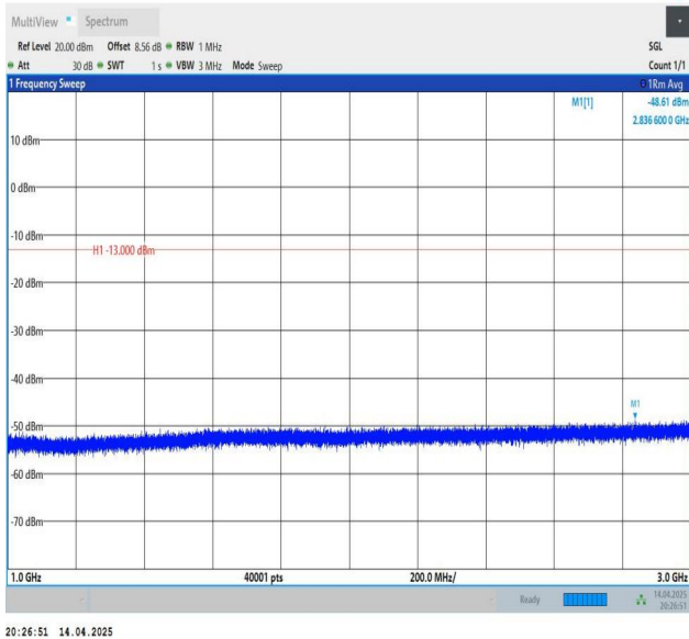
Band26(814-824)-3MHz-QPSK-26705-1RB#14-1000~3000-PASS
