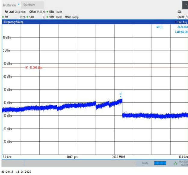
Band26(814-824)-5MHz-QPSK-26715-1RB#0-3000~10000-PASS
