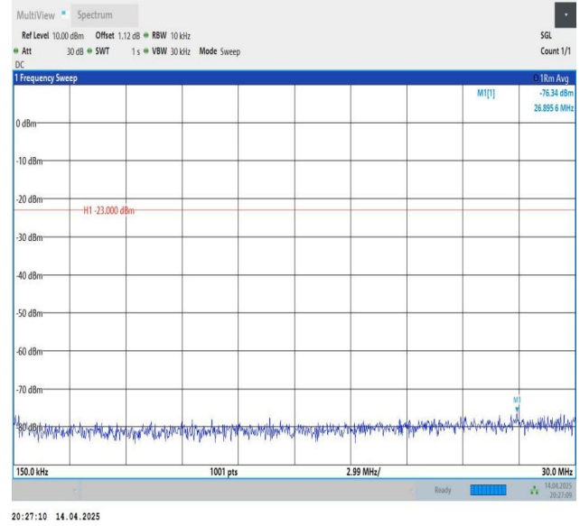
Band26(814-824)-3MHz-QPSK-26740-1RB#0-0.15~30-PASS
