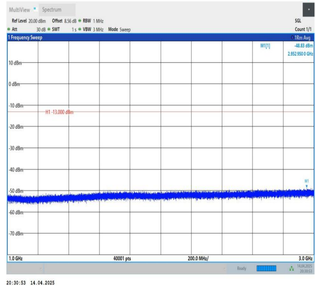
Band26(814-824)-5MHz-QPSK-26765-1RB#0-1000~3000-PASS
