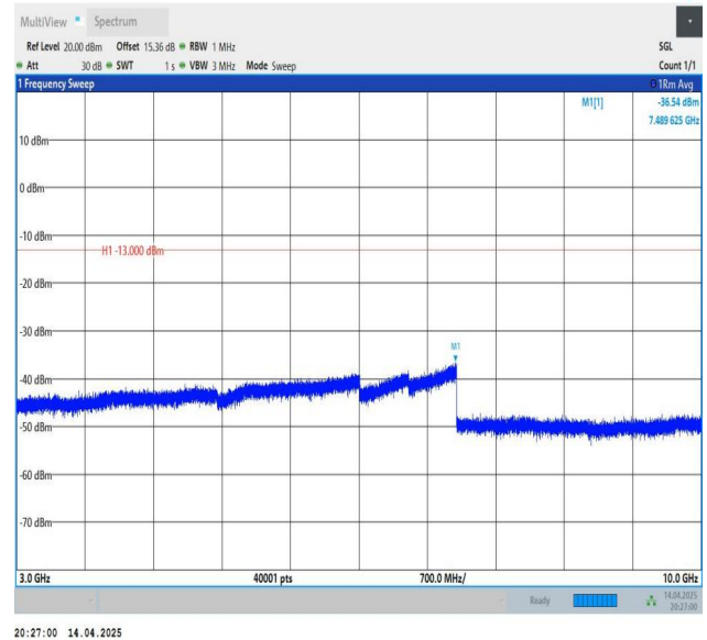
Band26(814-824)-3MHz-QPSK-26705-1RB#14-3000~10000-PASS
