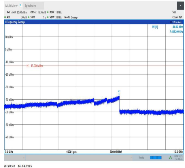
Band26(814-824)-3MHz-QPSK-26775-1RB#14-3000~10000-PASS
