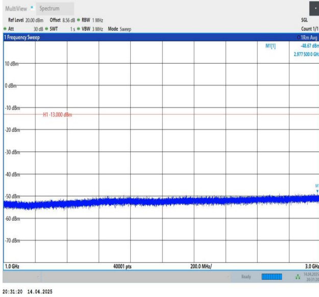
Band26(814-824)-5MHz-QPSK-26765-1RB#24-1000~3000-PASS
