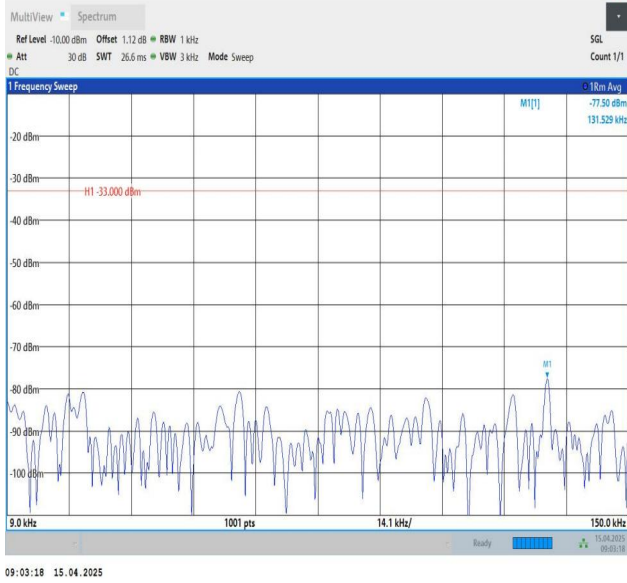
Band26(814-824)-5MHz-QPSK-26715-1RB#0-0.009~0.15-PASS
