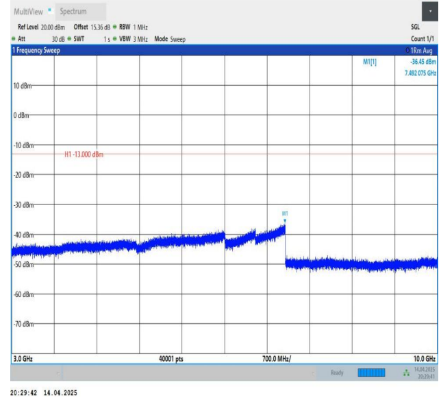
Band26(814-824)-5MHz-QPSK-26715-1RB#24-3000~10000-PASS
