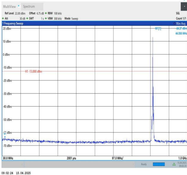
Band26(814-824)-3MHz-QPSK-26740-1RB#0-30~1000-PASS
