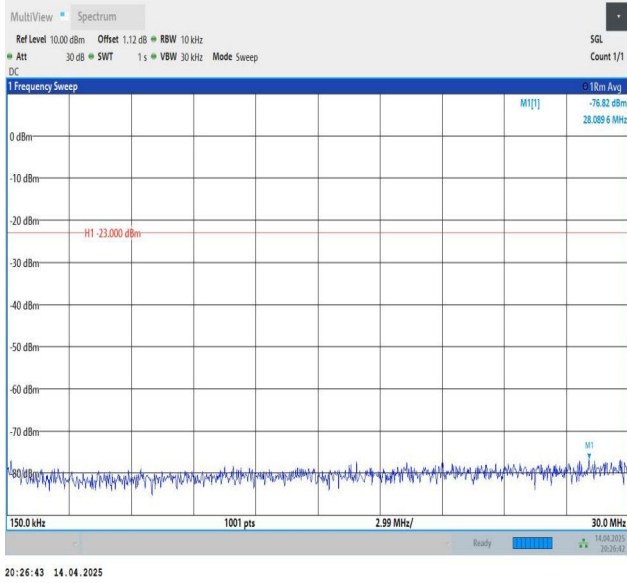
Band26(814-824)-3MHz-QPSK-26705-1RB#14-0.15~30-PASS
