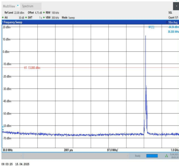
Band26(814-824)-5MHz-QPSK-26715-1RB#0-30~1000-PASS
