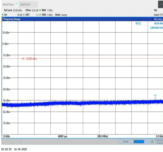
Band26(814-824)-5MHz-QPSK-26715-1RB#24-1000~3000-PASS
