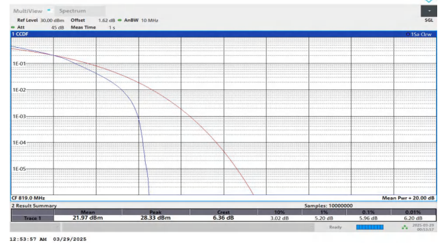
Band26(814-824)-10MHz-16QAM-26740-27RB#0-PASS
