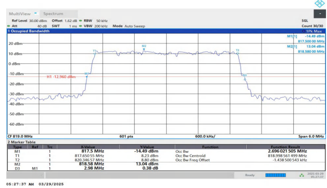
Band26(814-824)-3MHz-16QAM-26740-15RB#0-PASS
