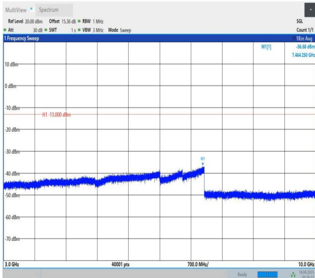
Band26(814-824)-3MHz-QPSK-26705-1RB#0-3000~10000-PASS
