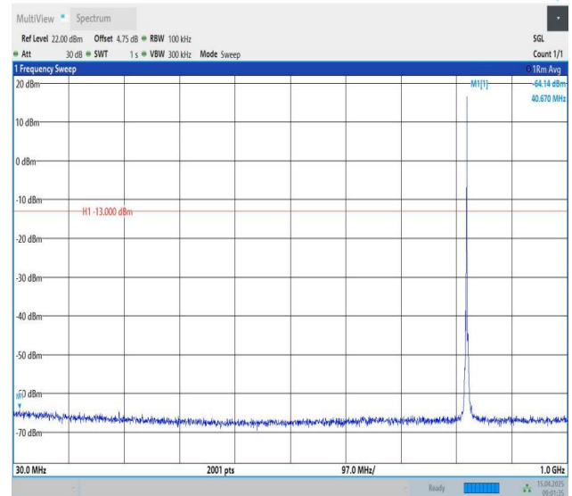
Band26(814-824)-1.4MHz-QPSK-26783-1RB#5-30~1000-PASS
