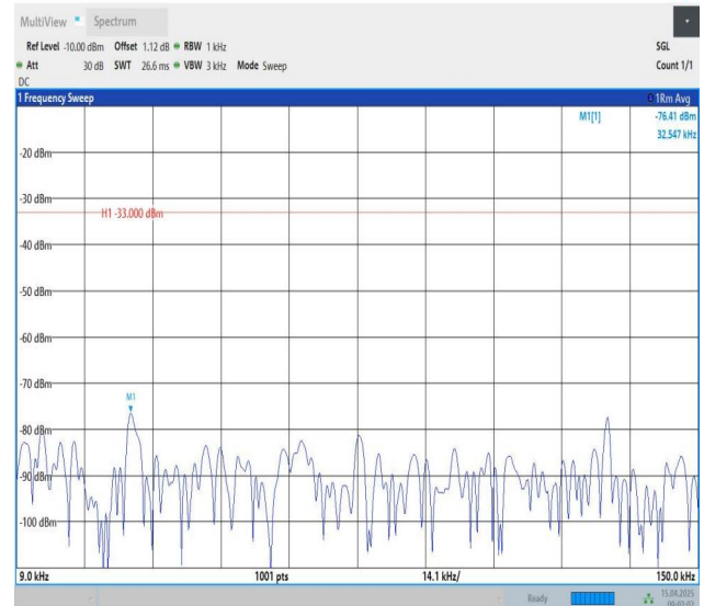
Band26(814-824)-3MHz-QPSK-26705-1RB#14-0.009~0.15-PASS
