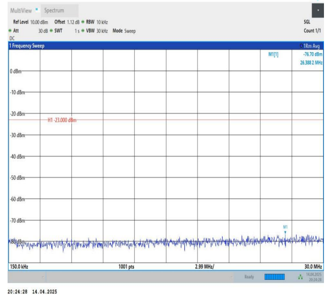
Band26(814-824)-1.4MHz-QPSK-26740-1RB#0-0.15~30-PASS
