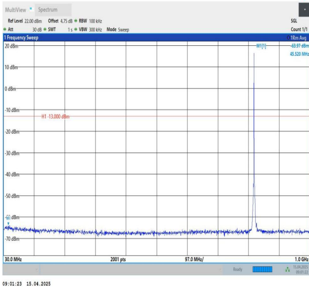
Band26(814-824)-1.4MHz-QPSK-26783-1RB#0-30~1000-PASS
