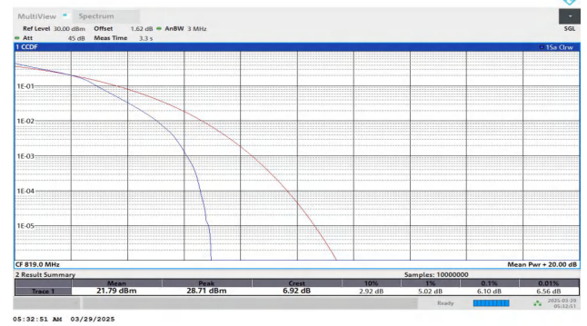
Band26(814-824)-3MHz-16QAM-26740-15RB#0-PASS
