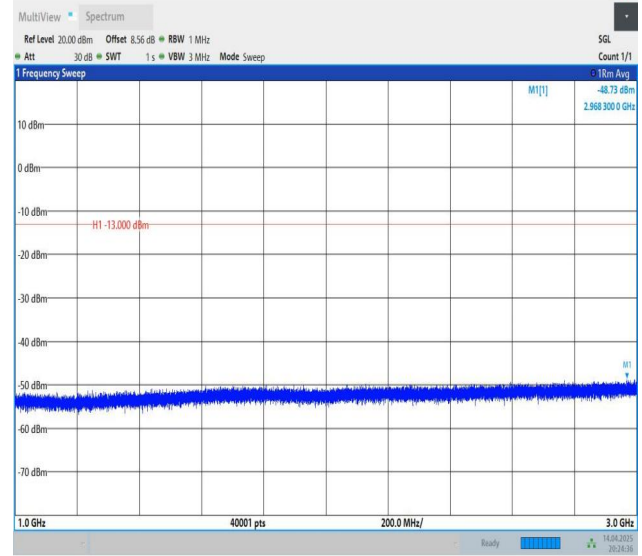
Band26(814-824)-1.4MHz-QPSK-26740-1RB#0-1000~3000-PASS
