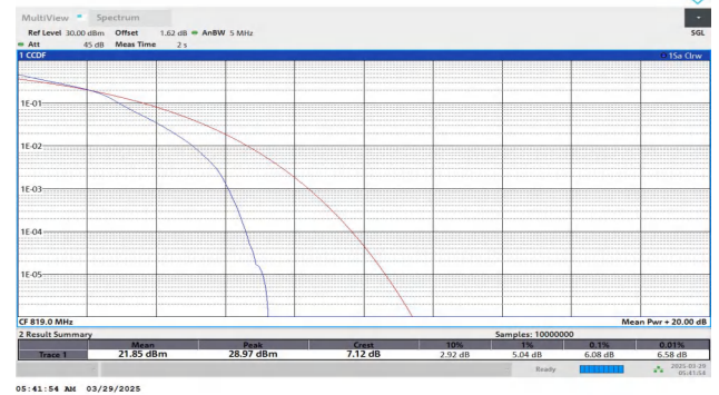
Band26(814-824)-5MHz-16QAM-26740-25RB#0-PASS
