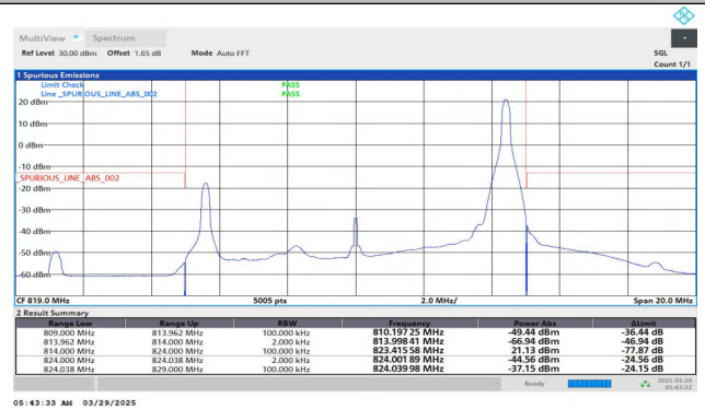
Band26(814-824)-10MHz-QPSK-26740-1RB#49-PASS
