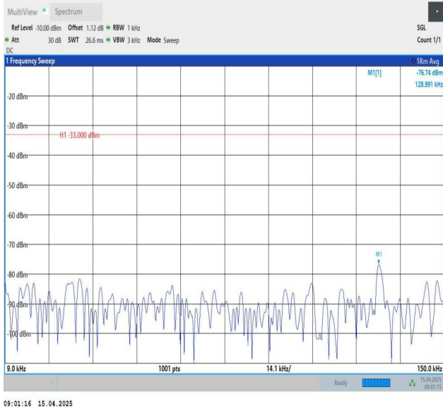
Band26(814-824)-1.4MHz-QPSK-26783-1RB#0-0.009~0.15-PASS
