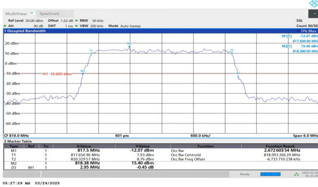
Band26(814-824)-3MHz-QPSK-26740-15RB#0-PASS
