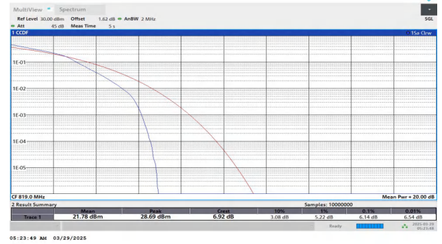
Band26(814-824)-1.4MHz-16QAM-26740-6RB#0-PASS
