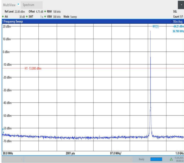
Band26(814-824)-1.4MHz-QPSK-26740-1RB#0-30~1000-PASS
