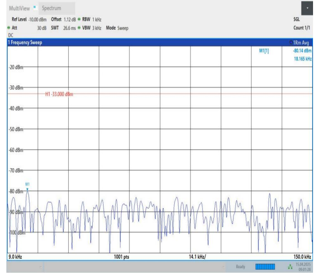
Band26(814-824)-1.4MHz-QPSK-26783-1RB#5-0.009~0.15-PASS
