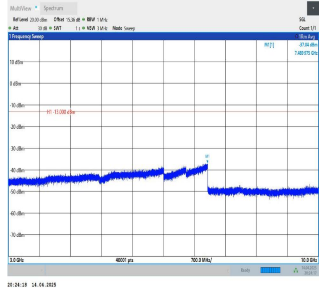
Band26(814-824)-1.4MHz-QPSK-26697-1RB#5-3000~10000-PASS S
