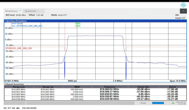
Band26(814-824)-5MHz-QPSK-26765-25RB#0-PASS
