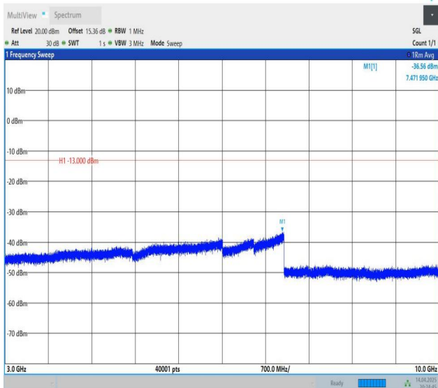
Band26(814-824)-1.4MHz-QPSK-26740-1RB#0-3000~10000-PAS
