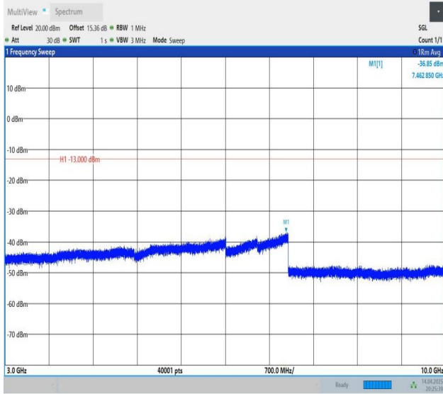
Band26(814-824)-1.4MHz-QPSK-26783-1RB#0-3000~10000-PAS S
