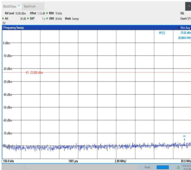
Band26(814-824)-1.4MHz-QPSK-26783-1RB#5-0.15~30-PASS
