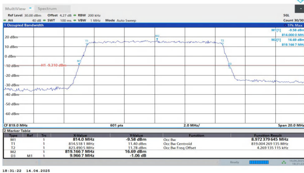
Band26(814-824)-10MHz-QPSK-26740-50RB#0-PASS
