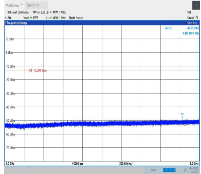
Band26(814-824)-3MHz-QPSK-26705-1RB#0-1000~3000-PASS
