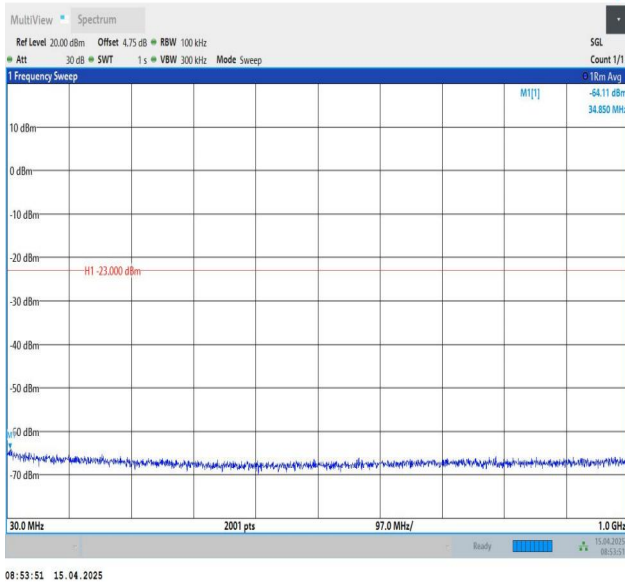
Band25-15MHz-QPSK-26615-1RB#0-30~1000-PASS
