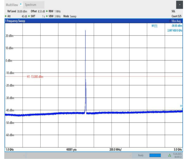
Band25-10MHz-QPSK-26640-1RB#0-1000~3000-PASS
