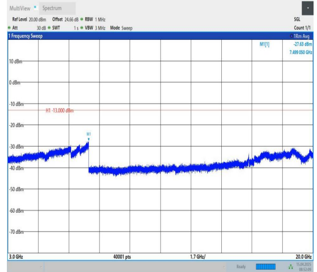
Band25-15MHz-QPSK-26115-1RB#74-3000~20000-PASS
