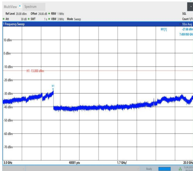
Band25-10MHz-QPSK-26640-1RB#0-3000~20000-PASS
