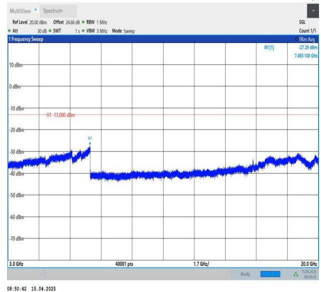
Band25-10MHz-QPSK-26640-1RB#49-3000~20000-PASS
