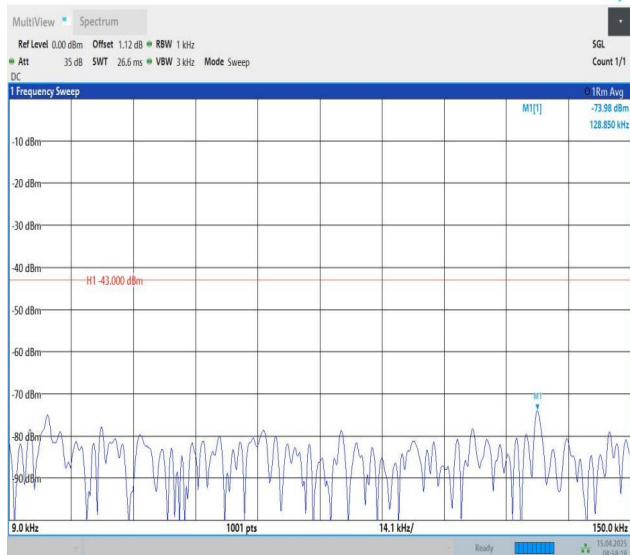
Band25-20MHz-QPSK-26590-1RB#0-0.009~0.15-PASS
