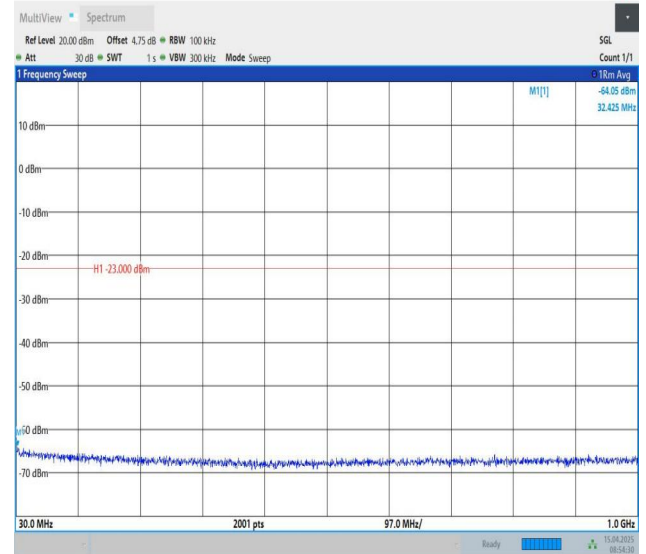
Band25-15MHz-QPSK-26615-1RB#74-30~1000-PASS
