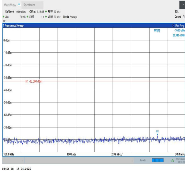
Band25-20MHz-QPSK-26140-1RB#99-0.15~30-PASS
