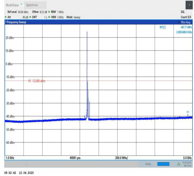
Band25-15MHz-QPSK-26365-1RB#0-1000~3000-PASS
