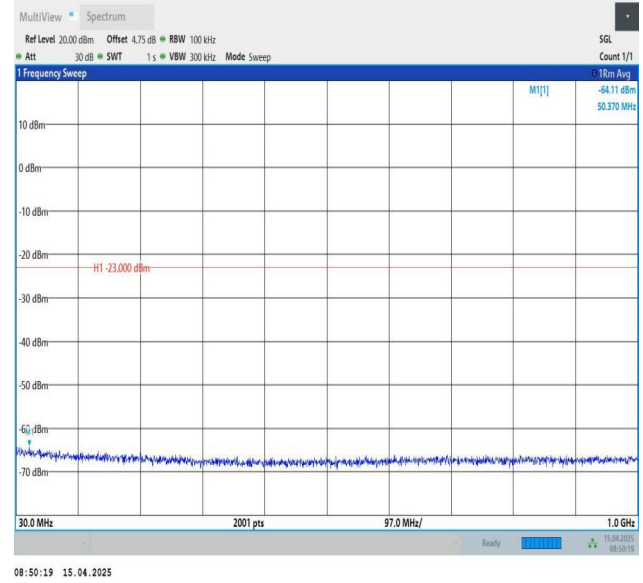
Band25-10MHz-QPSK-26640-1RB#49-30~1000-PASS
