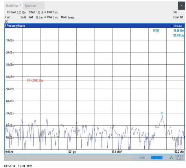
Band25-20MHz-QPSK-26140-1RB#99-0.009~0.15-PASS
