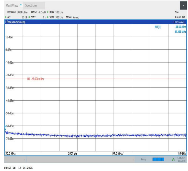
Band25-15MHz-QPSK-26365-1RB#74-30~1000-PASS
