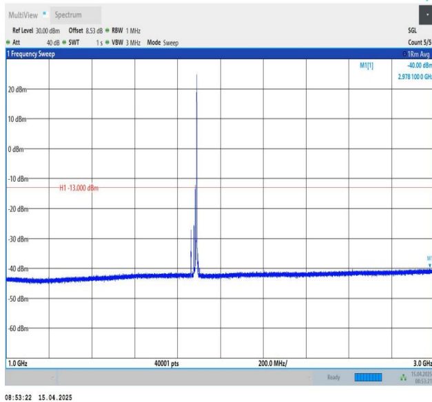
Band25-15MHz-QPSK-26365-1RB#74-1000~3000-PASS
