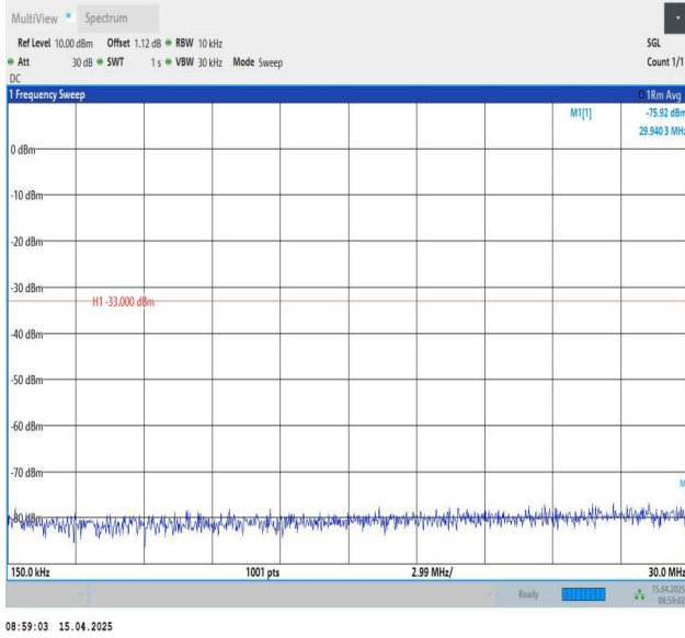
Band25-20MHz-QPSK-26590-1RB#99-0.15~30-PASS
