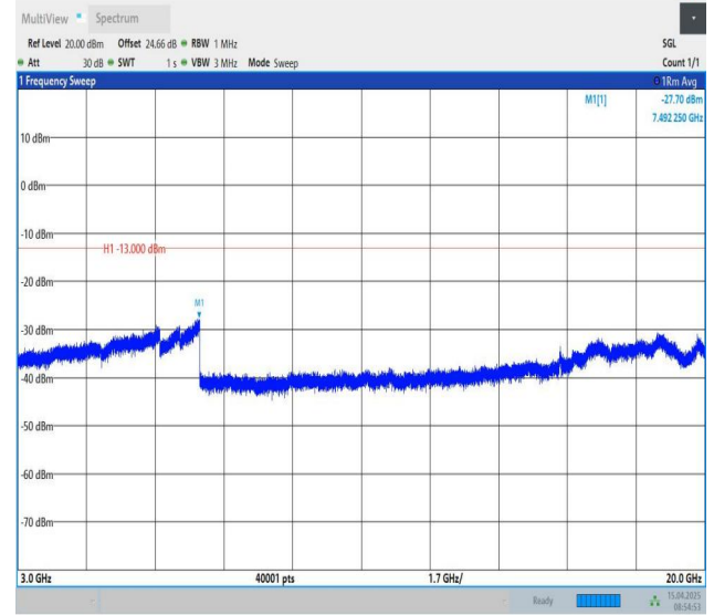
Band25-15MHz-QPSK-26615-1RB#74-3000~20000-PASS
