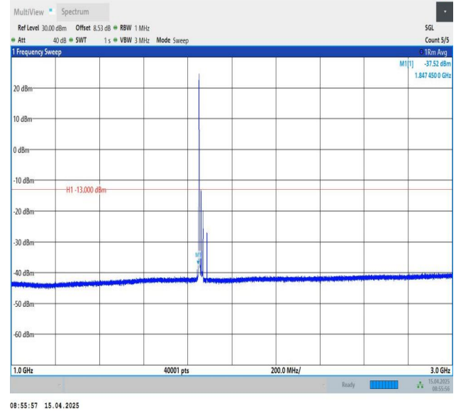
Band25-20MHz-QPSK-26140-1RB#0-1000~3000-PASS
