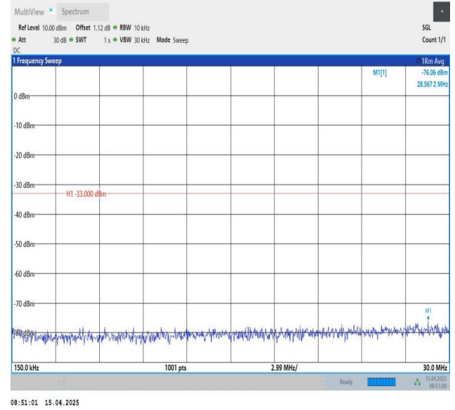
Band25-15MHz-QPSK-26115-1RB#0-0.15~30-PASS
