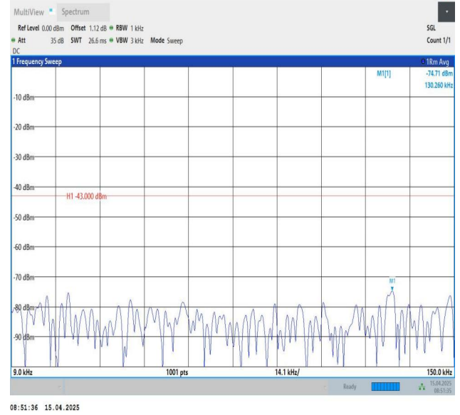
Band25-15MHz-QPSK-26115-1RB#74-0.009~0.15-PASS
