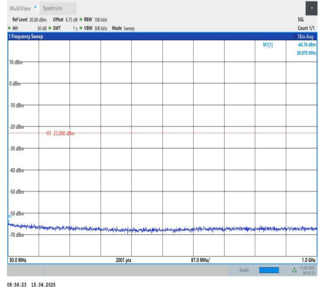
Band25-20MHz-QPSK-26140-1RB#99-30~1000-PASS
