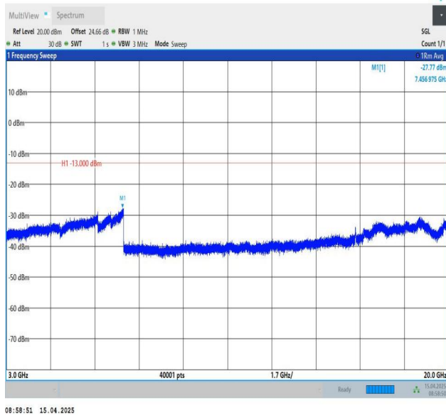
Band25-20MHz-QPSK-26590-1RB#0-3000~20000-PASS
