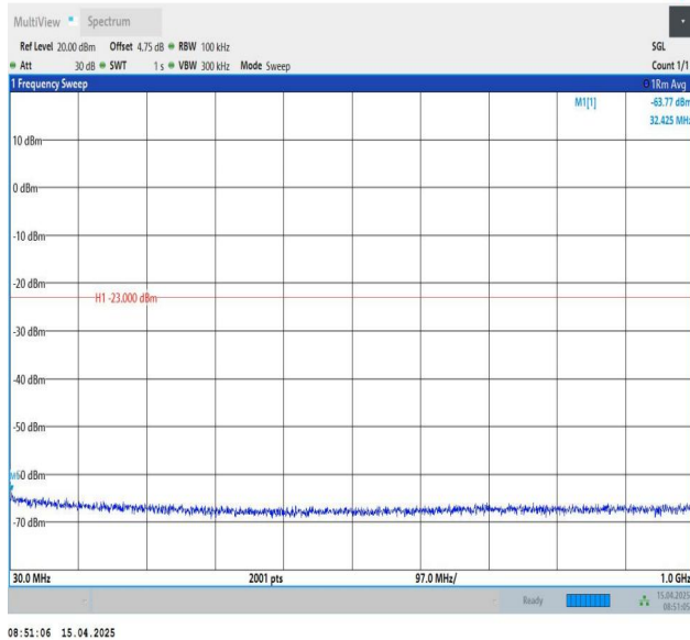
Band25-15MHz-QPSK-26115-1RB#0-30~1000-PASS
