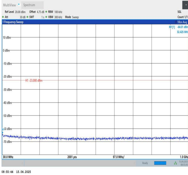
Band25-20MHz-QPSK-26140-1RB#0-30~1000-PASS
