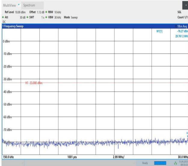
Band25-15MHz-QPSK-26615-1RB#74-0.15~30-PASS
