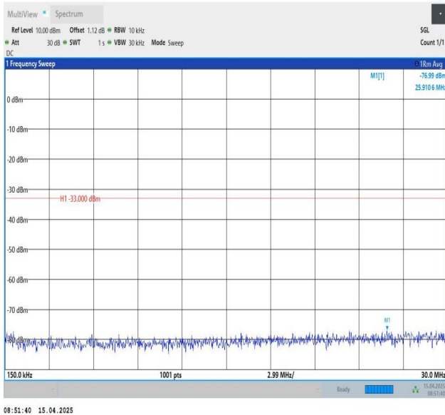
Band25-15MHz-QPSK-26115-1RB#74-0.15~30-PASS
