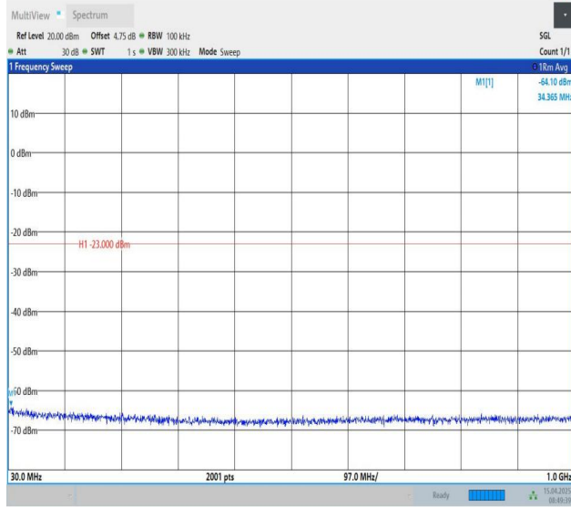
Band25-10MHz-QPSK-26640-1RB#0-30~1000-PASS
