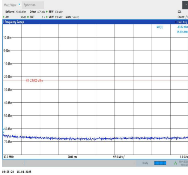
Band25-20MHz-QPSK-26590-1RB#0-30~1000-PASS
