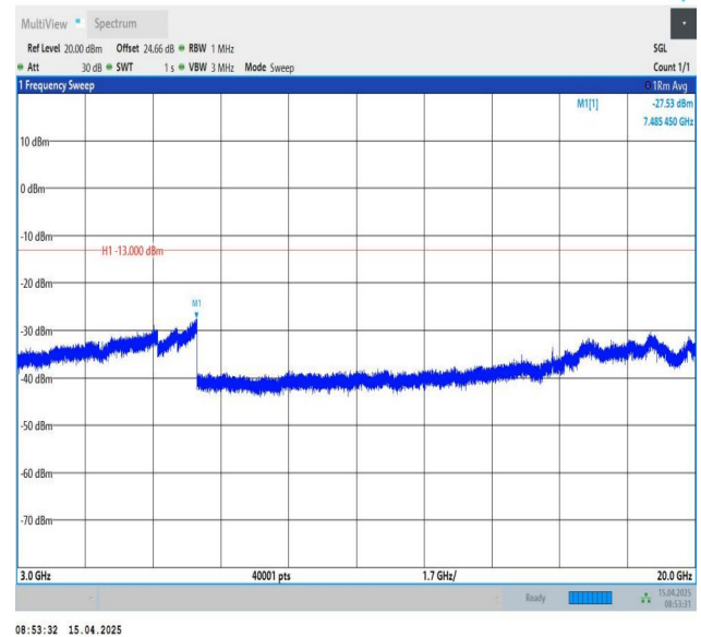
Band25-15MHz-QPSK-26365-1RB#74-3000~20000-PASS
