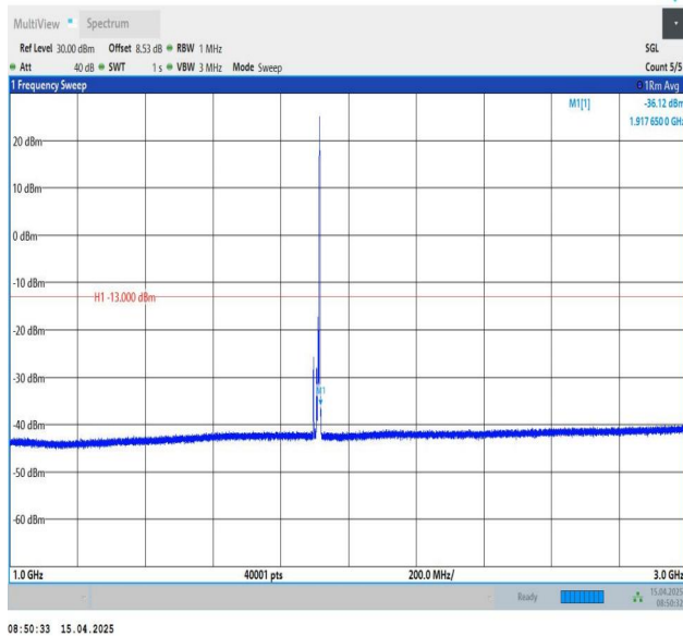
Band25-10MHz-QPSK-26640-1RB#49-1000~3000-PASS
