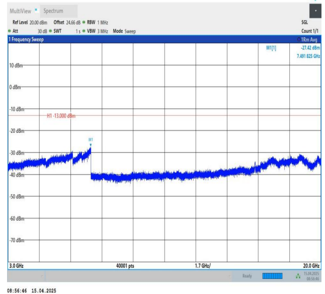
Band25-20MHz-QPSK-26140-1RB#99-3000~20000-PASS
