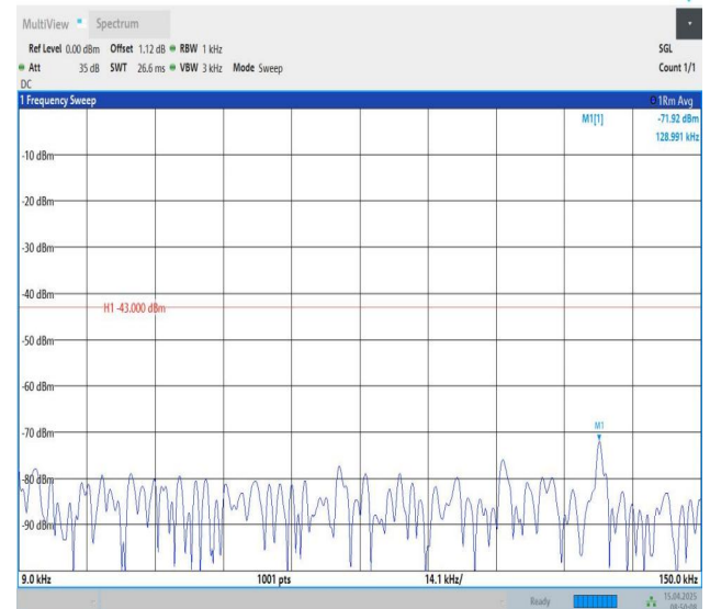
Band25-10MHz-QPSK-26640-1RB#49-0.009~0.15-PASS
