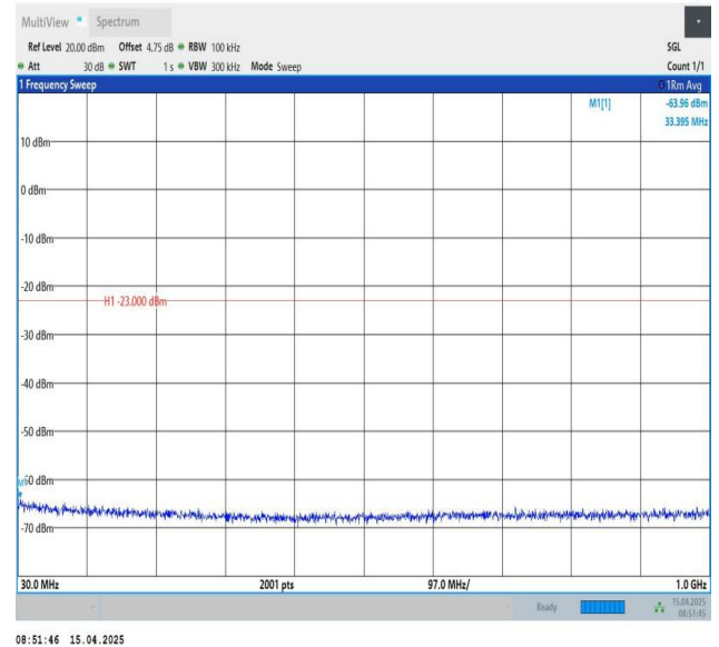
Band25-15MHz-QPSK-26115-1RB#74-30~1000-PASS
