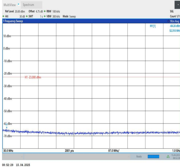
Band25-15MHz-QPSK-26365-1RB#0-30~1000-PASS
