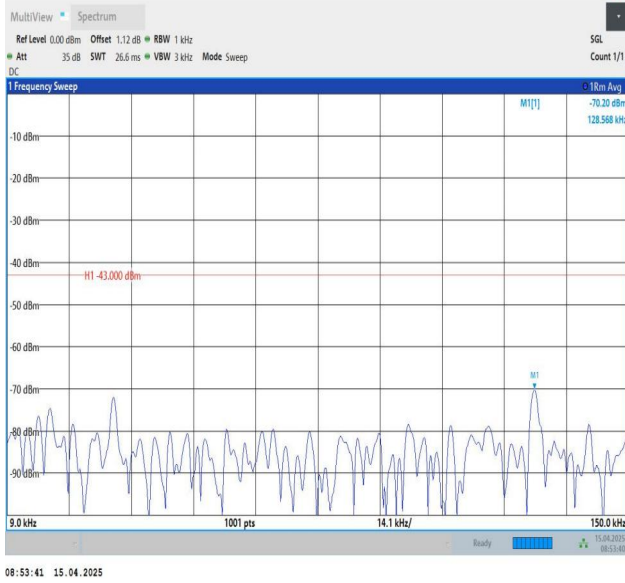
Band25-15MHz-QPSK-26615-1RB#0-0.009~0.15-PASS
