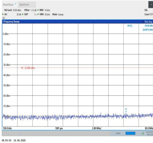
Band25-15MHz-QPSK-26365-1RB#74-0.15~30-PASS
