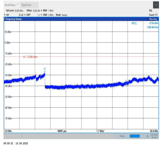
Band25-20MHz-QPSK-26590-1RB#99-3000~20000-PASS
