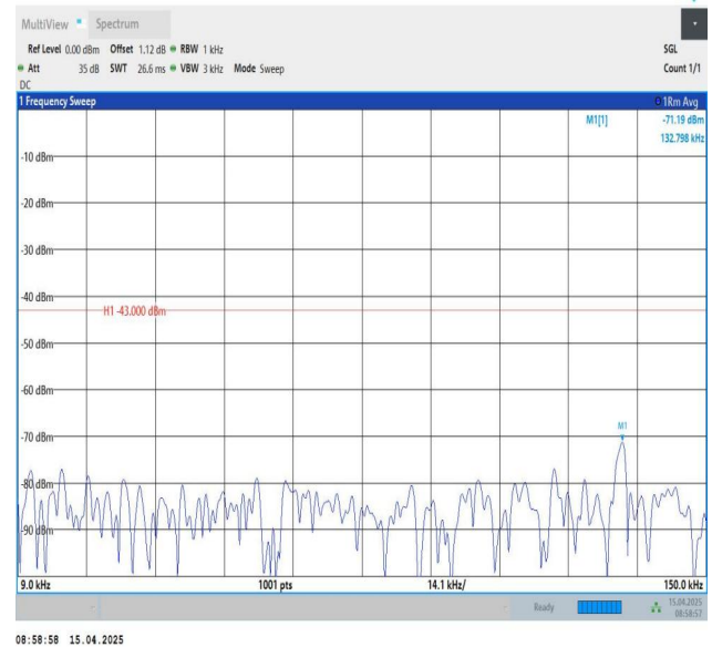
Band25-20MHz-QPSK-26590-1RB#99-0.009~0.15-PASS
