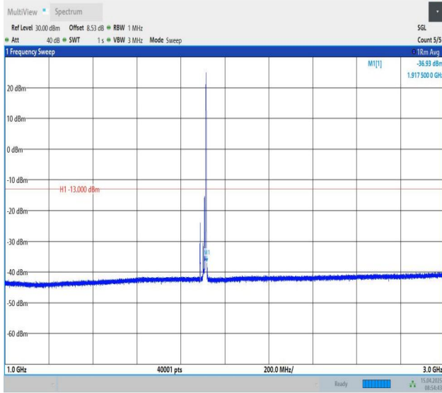
Band25-15MHz-QPSK-26615-1RB#74-1000~3000-PASS
