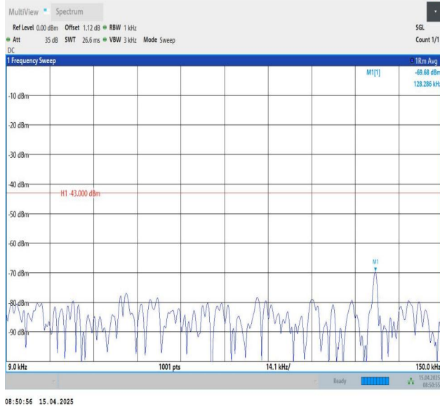
Band25-15MHz-QPSK-26115-1RB#0-0.009~0.15-PASS
