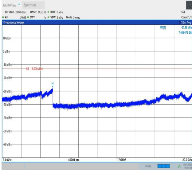
Band25-15MHz-QPSK-26615-1RB#0-3000~20000-PASS
