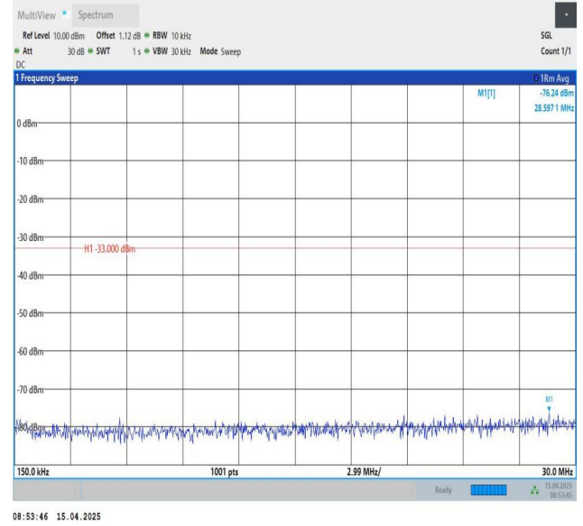
Band25-15MHz-QPSK-26615-1RB#0-0.15~30-PASS
