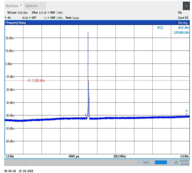
Band25-15MHz-QPSK-26615-1RB#0-1000~3000-PASS
