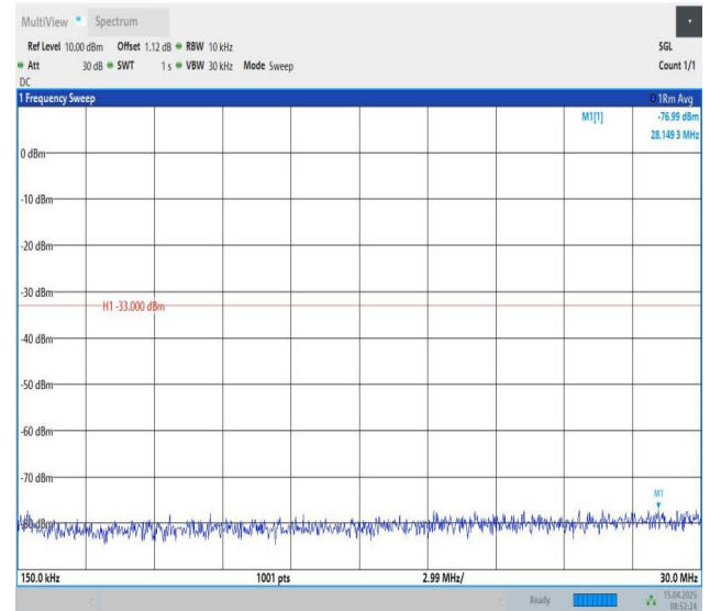
Band25-15MHz-QPSK-26365-1RB#0-0.15~30-PASS
