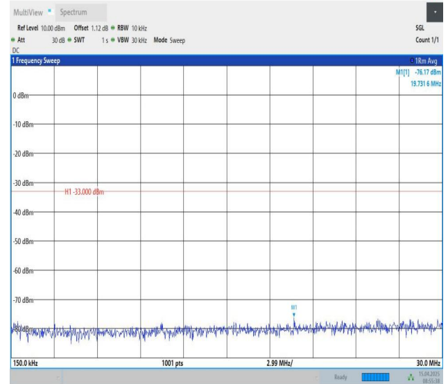
Band25-20MHz-QPSK-26140-1RB#0-0.15~30-PASS
