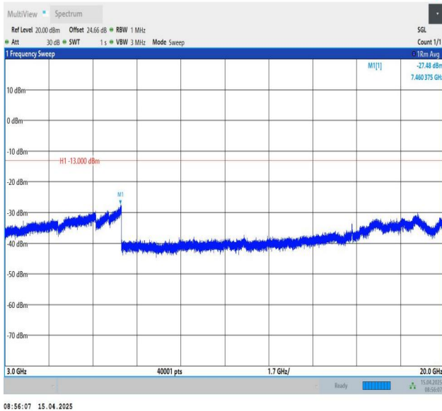
Band25-20MHz-QPSK-26140-1RB#0-3000~20000-PASS
