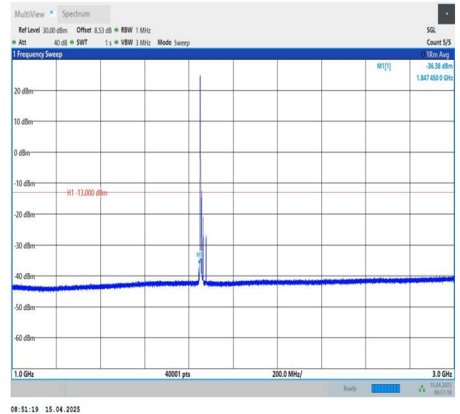
Band25-15MHz-QPSK-26115-1RB#0-1000~3000-PASS
