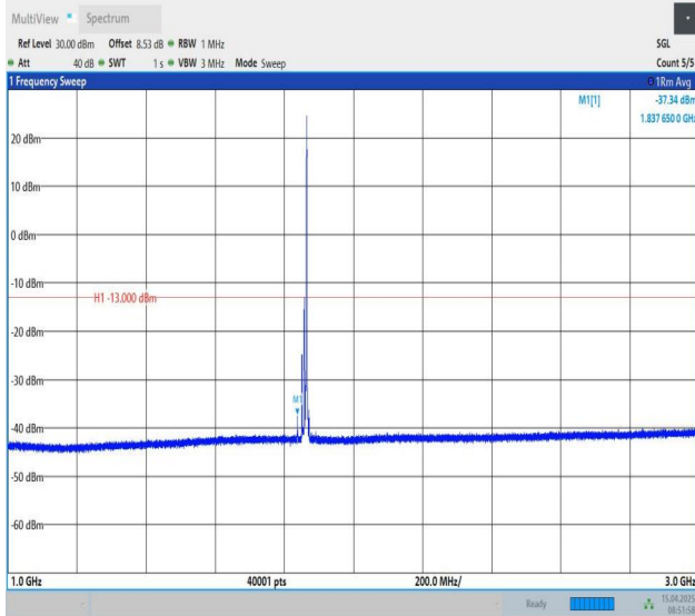
Band25-15MHz-QPSK-26115-1RB#74-1000~3000-PASS
