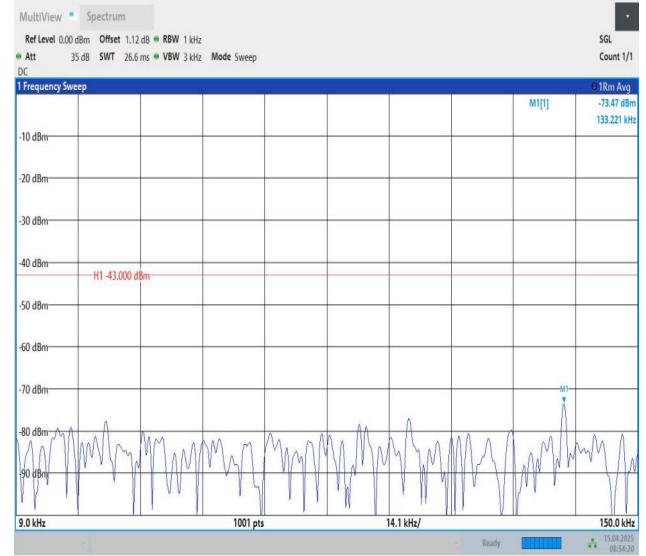
Band25-15MHz-QPSK-26615-1RB#74-0.009~0.15-PASS
