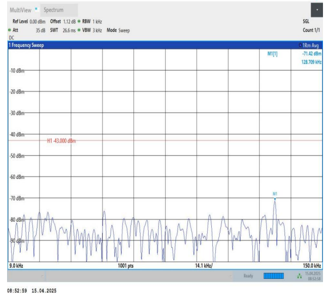
Band25-15MHz-QPSK-26365-1RB#74-0.009~0.15-PASS
