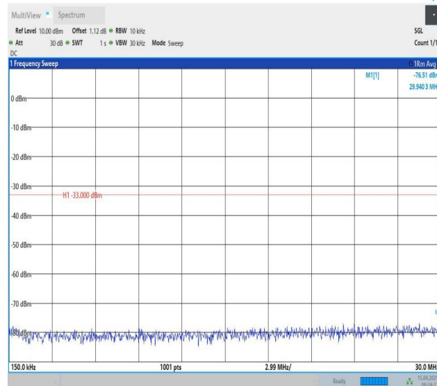
Band25-20MHz-QPSK-26590-1RB#0-0.15~30-PASS
