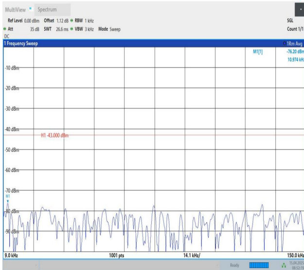
Band25-15MHz-QPSK-26365-1RB#0-0.009~0.15-PASS
