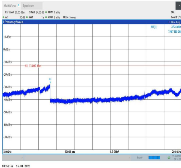
Band25-15MHz-QPSK-26365-1RB#0-3000~20000-PASS
