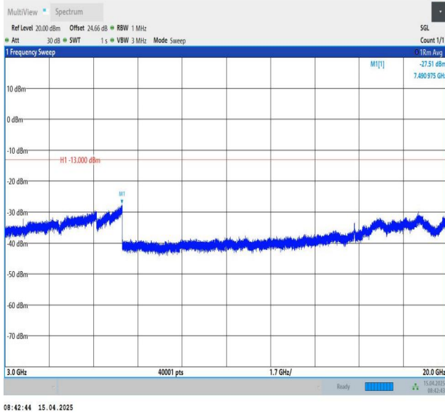
Band25-5MHz-QPSK-26065-1RB#0-3000~20000-PASS
