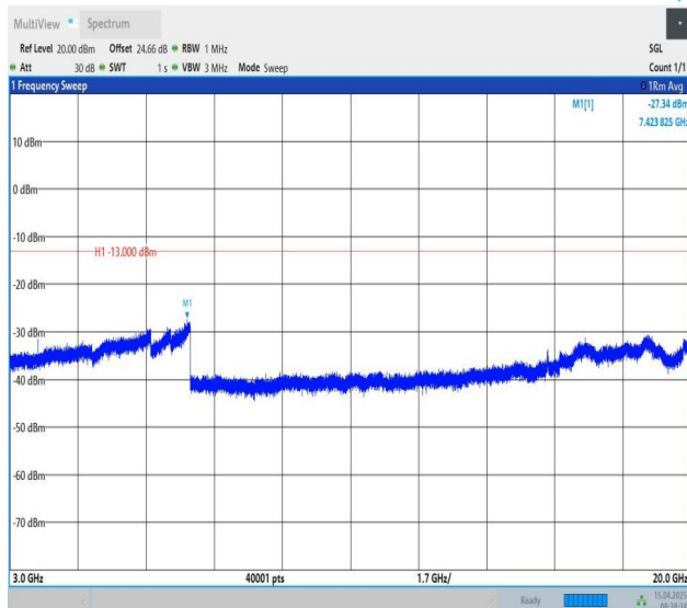
Band25-3MHz-QPSK-26055-1RB#0-3000~20000-PASS
