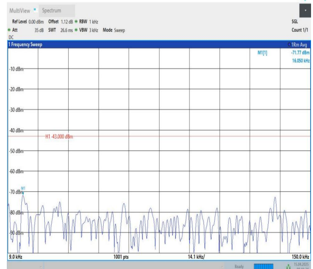
Band25-3MHz-QPSK-26675-1RB#14-0.009~0.15-PASS
