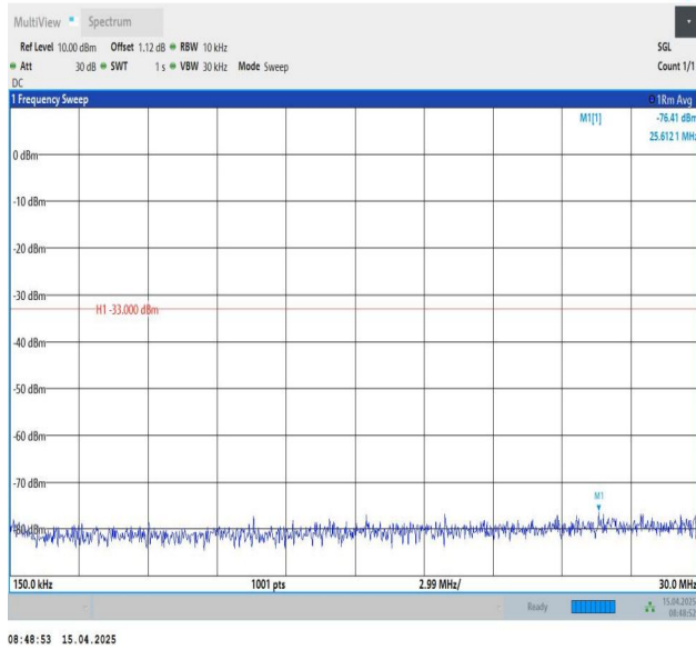
Band25-10MHz-QPSK-26365-1RB#49-0.15~30-PASS
