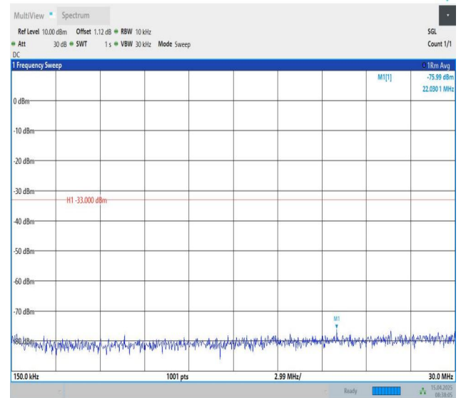
Band25-3MHz-QPSK-26055-1RB#0-0.15~30-PASS
