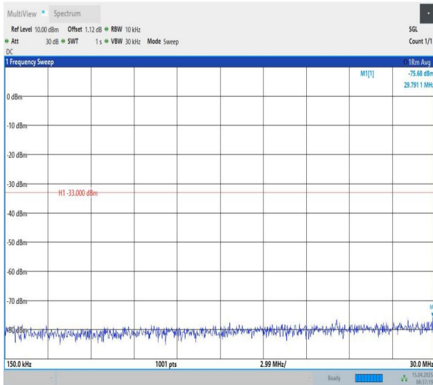
Band25-1.4MHz-QPSK-26683-1RB#5-0.15~30-PASS
