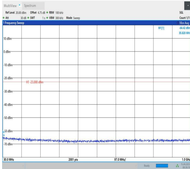
Band25-3MHz-QPSK-26055-1RB#0-30~1000-PASS
