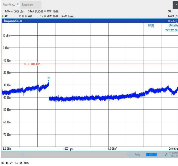
Band25-5MHz-QPSK-26665-1RB#0-3000~20000-PASS
