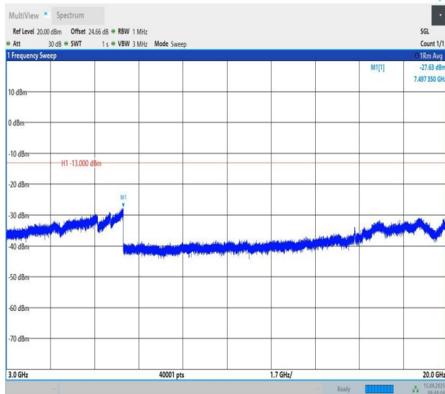
Band25-5MHz-QPSK-26365-1RB#0-3000~20000-PASS
