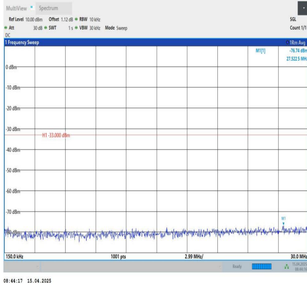
Band25-5MHz-QPSK-26365-1RB#24-0.15~30-PASS
