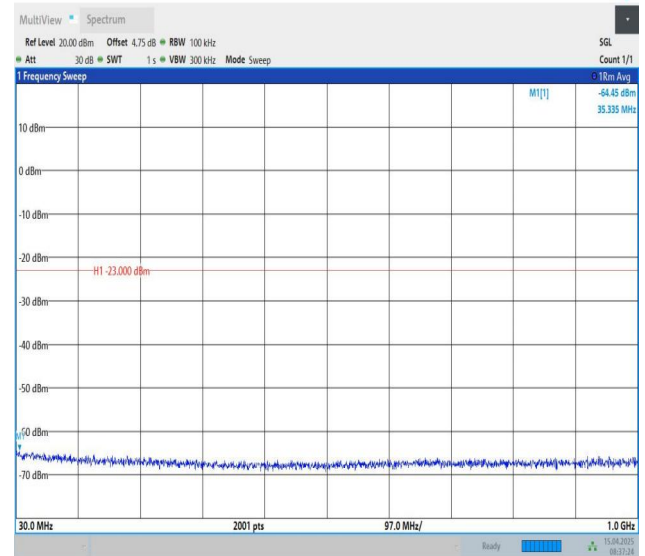
Band25-1.4MHz-QPSK-26683-1RB#5-30~1000-PASS
