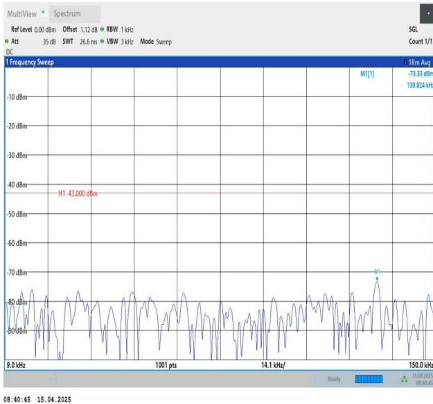
Band25-3MHz-QPSK-26675-1RB#0-0.009~0.15-PASS
