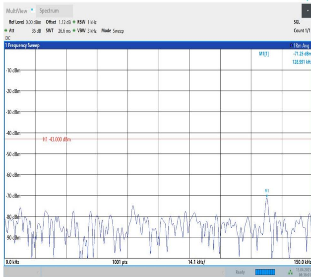
Band25-3MHz-QPSK-26055-1RB#0-0.009~0.15-PASS
