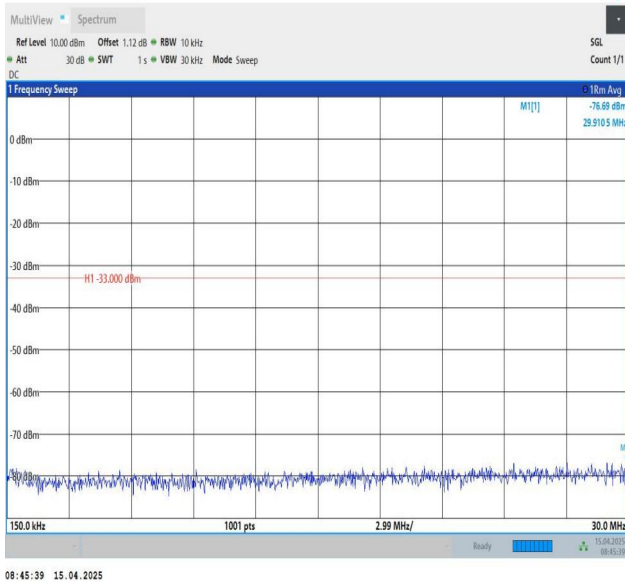
Band25-5MHz-QPSK-26665-1RB#24-0.15~30-PASS
