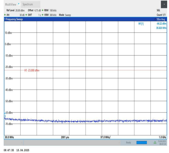
Band25-10MHz-QPSK-26090-1RB#49-30~1000-PASS
