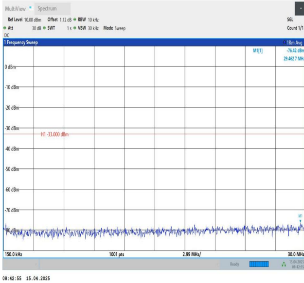
Band25-5MHz-QPSK-26065-1RB#24-0.15~30-PASS
