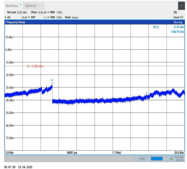
Band25-10MHz-QPSK-26090-1RB#49-3000~20000-PASS
