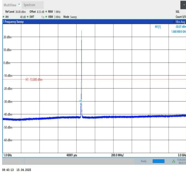
Band25-5MHz-QPSK-26065-1RB#24-1000~3000-PASS
