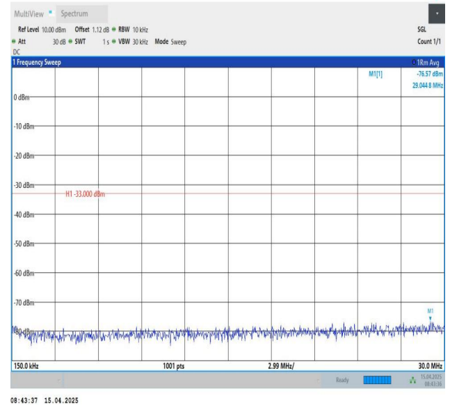
Band25-5MHz-QPSK-26365-1RB#0-0.15~30-PASS
