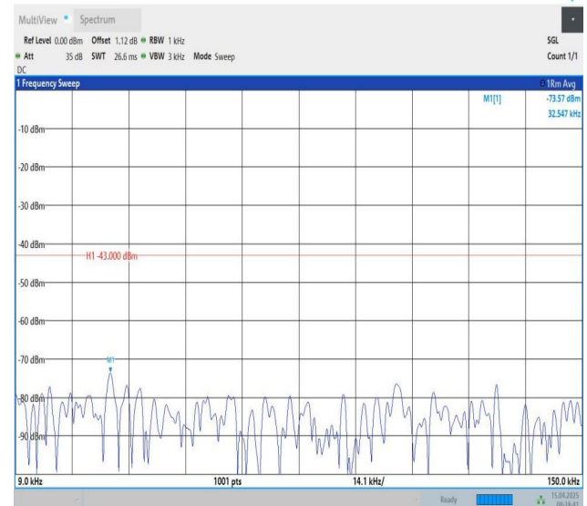
Band25-3MHz-QPSK-26055-1RB#14-0.009~0.15-PASS
