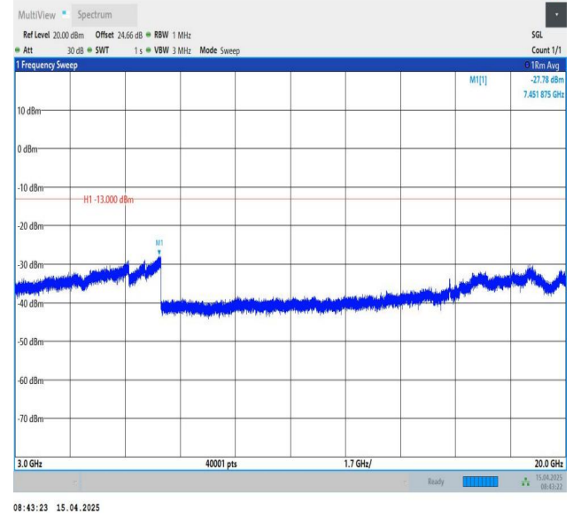
Band25-5MHz-QPSK-26065-1RB#24-3000~20000-PASS
