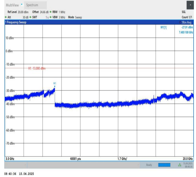
Band25-3MHz-QPSK-26365-1RB#14-3000~20000-PASS
