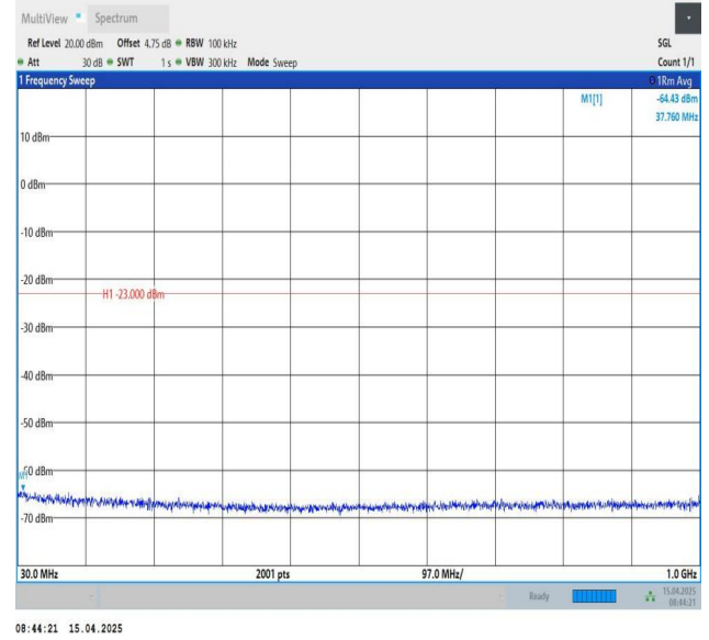
Band25-5MHz-QPSK-26365-1RB#24-30~1000-PASS
