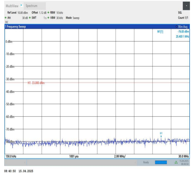
Band25-3MHz-QPSK-26675-1RB#0-0.15~30-PASS
