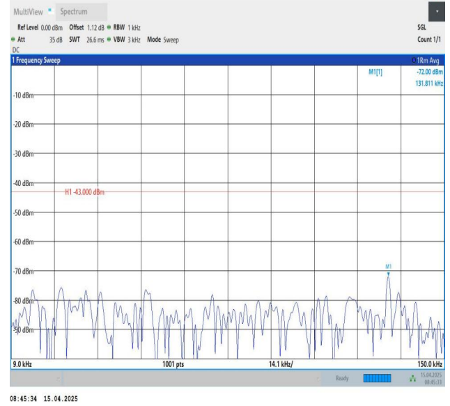
Band25-5MHz-QPSK-26665-1RB#24-0.009~0.15-PASS
