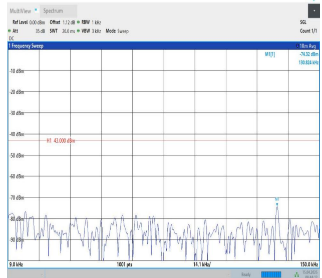
Band25-5MHz-QPSK-26365-1RB#24-0.009~0.15-PASS
