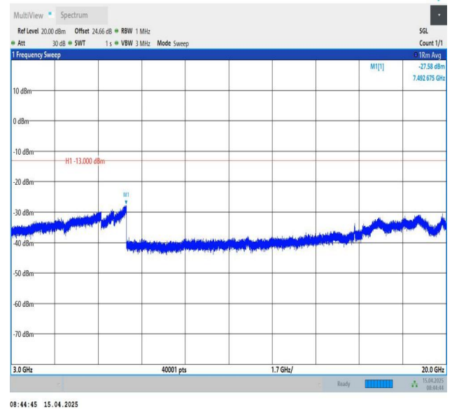
Band25-5MHz-QPSK-26365-1RB#24-3000~20000-PASS
