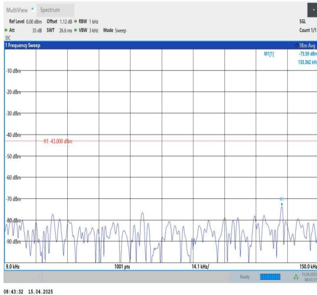
Band25-5MHz-QPSK-26365-1RB#0-0.009~0.15-PASS
