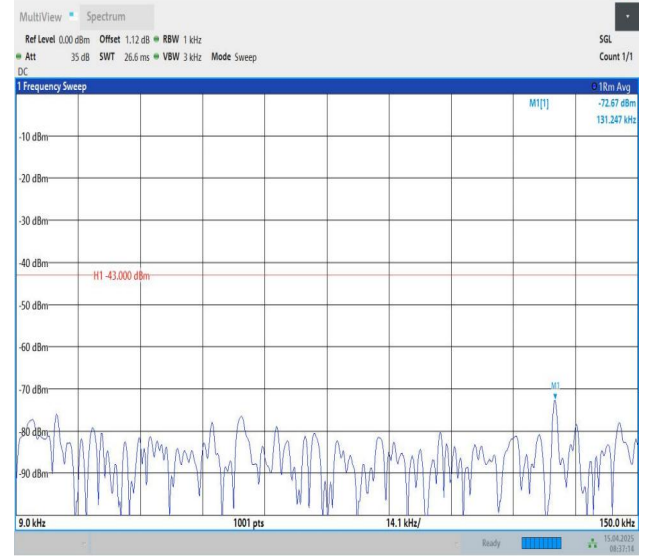
Band25-1.4MHz-QPSK-26683-1RB#5-0.009~0.15-PASS
