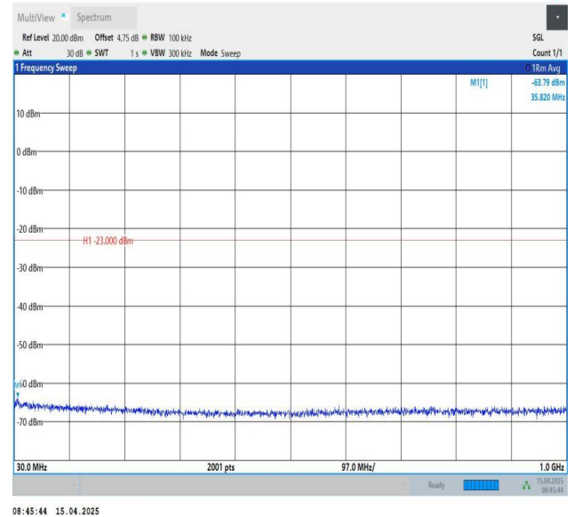
Band25-5MHz-QPSK-26665-1RB#24-30~1000-PASS
