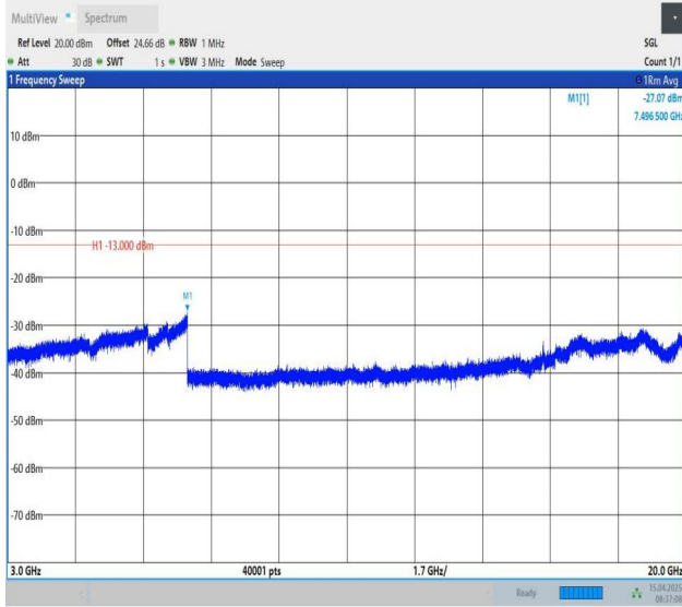
Band25-1.4MHz-QPSK-26683-1RB#0-3000~20000-PASS
