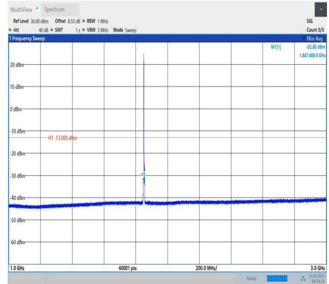
Band25-3MHz-QPSK-26055-1RB#0-1000~3000-PASS
