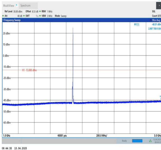
Band25-5MHz-QPSK-26365-1RB#24-1000~3000-PASS
