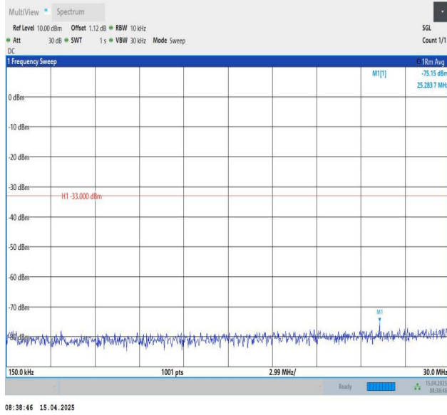
Band25-3MHz-QPSK-26055-1RB#14-0.15~30-PASS
