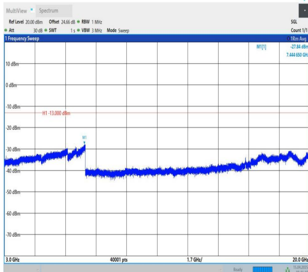
Band25-3MHz-QPSK-26675-1RB#0-3000~20000-PASS
