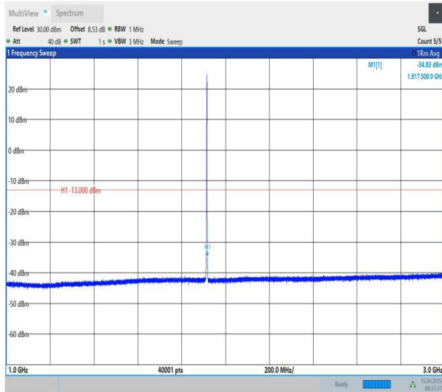
Band25-1.4MHz-QPSK-26683-1RB#5-1000~3000-PASS
