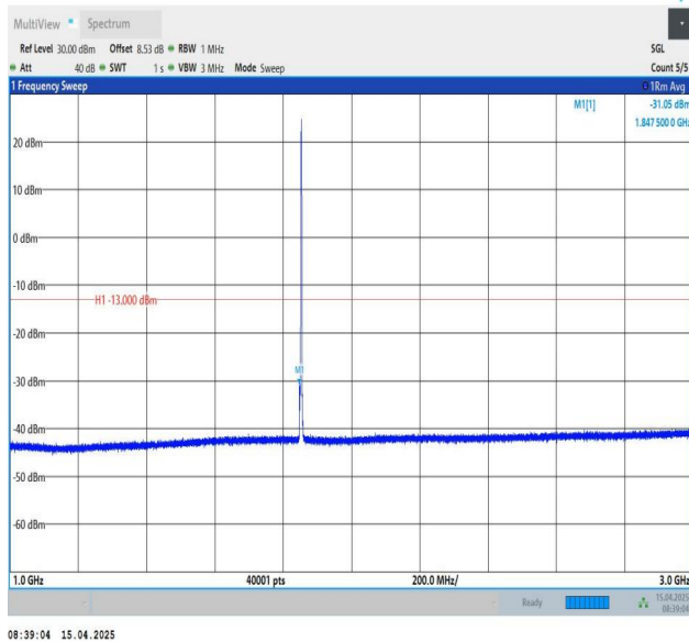
Band25-3MHz-QPSK-26055-1RB#14-1000~3000-PASS
