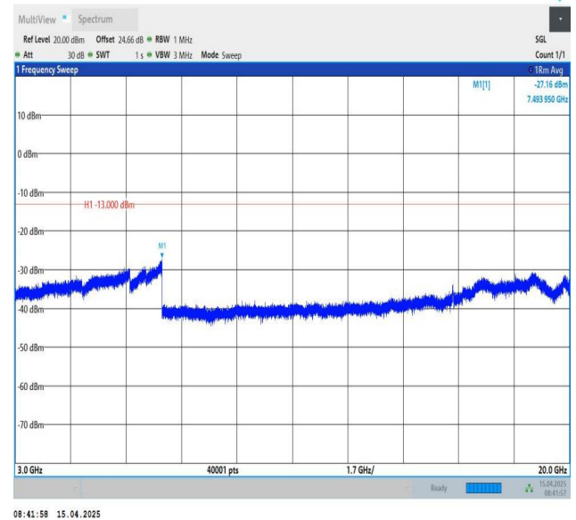
Band25-3MHz-QPSK-26675-1RB#14-3000~20000-PASS
