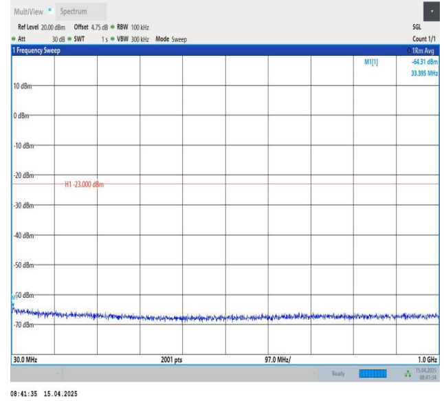
Band25-3MHz-QPSK-26675-1RB#14-30~1000-PASS
